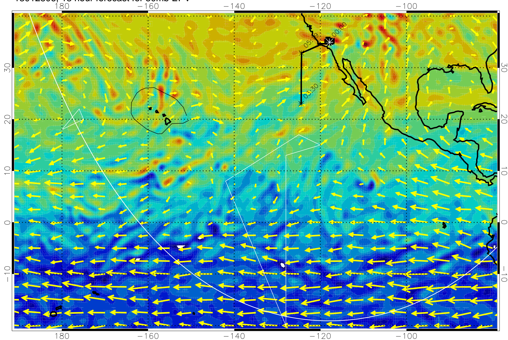
13012806, 18 hour forecast for 50mb EPV
