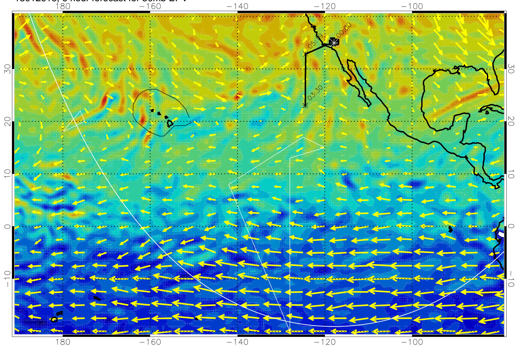
13012618, 6 hour forecast for 50mb EPV
