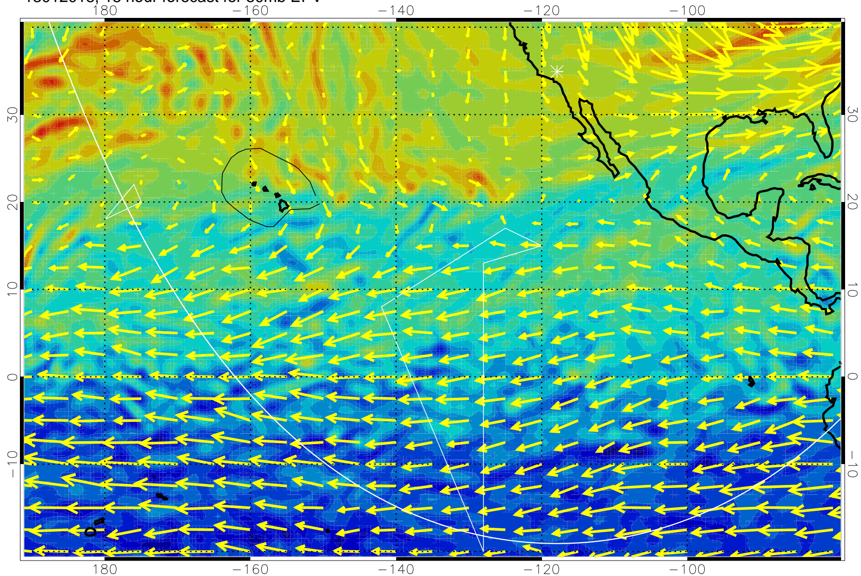
13012018, 18 hour forecast for 50mb EPV
