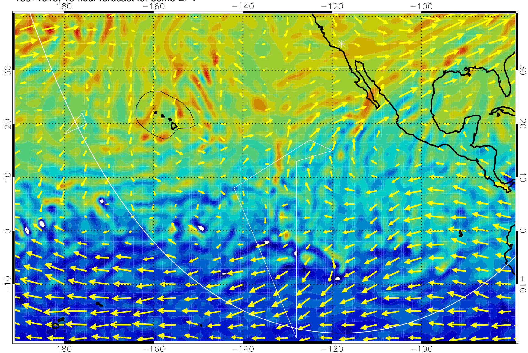
13011618, 18 hour forecast for 50mb EPV
