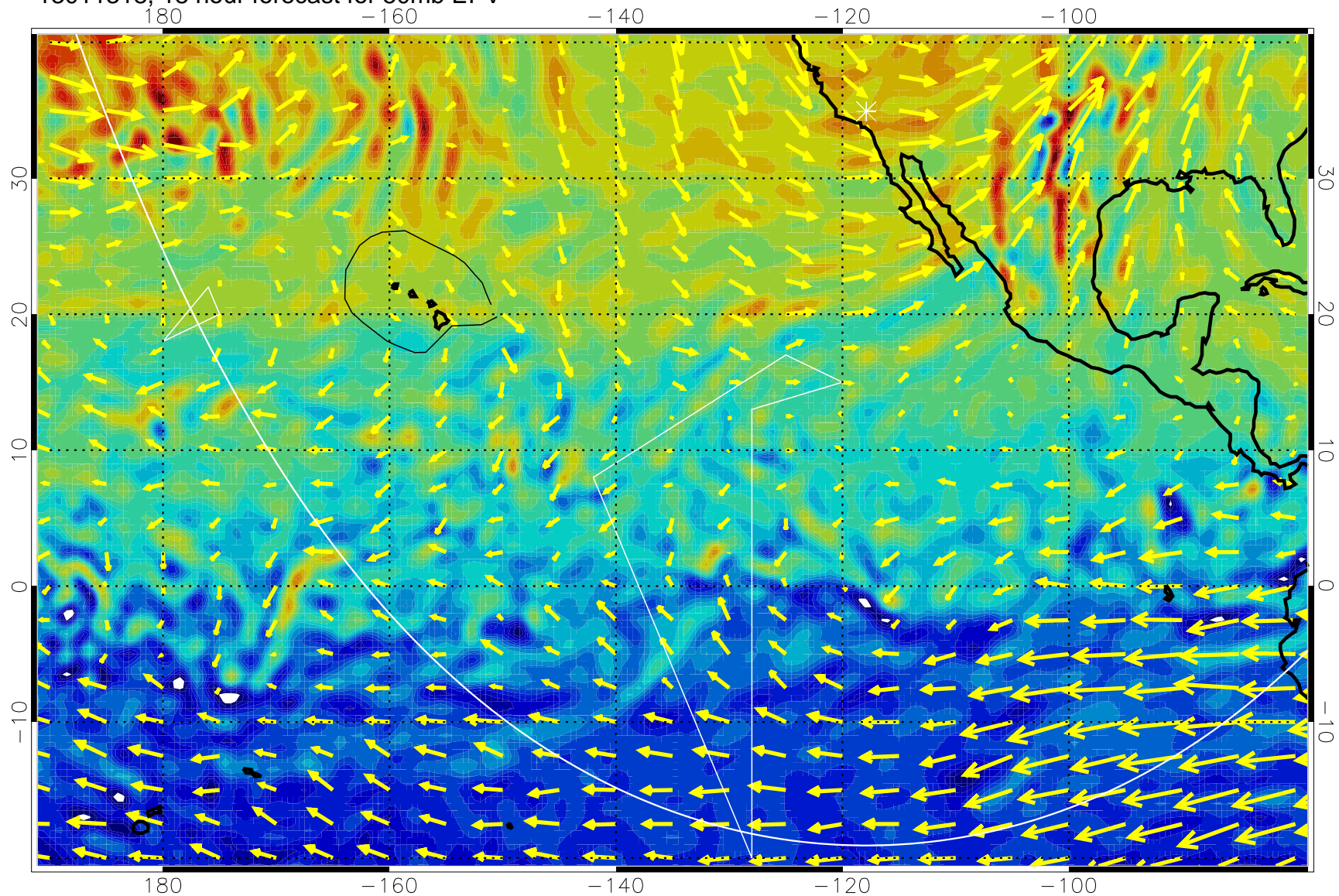
13011318, 18 hour forecast for 50mb EPV
