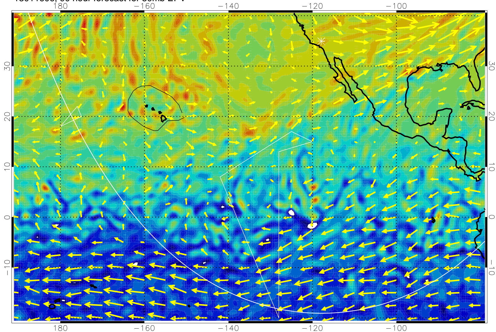
13011606, 90 hour forecast for 50mb EPV
