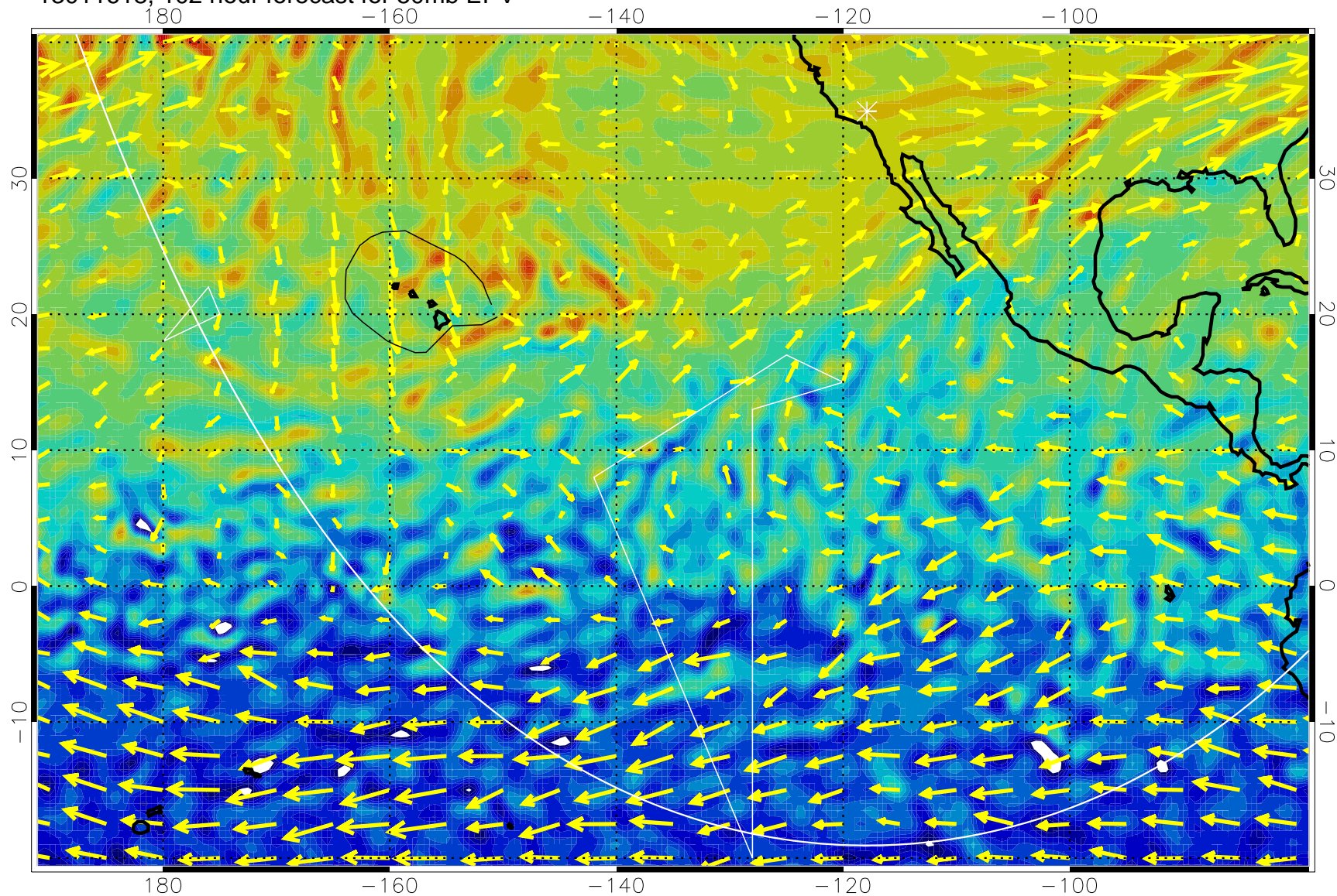
13011618, 102 hour forecast for 50mb EPV
