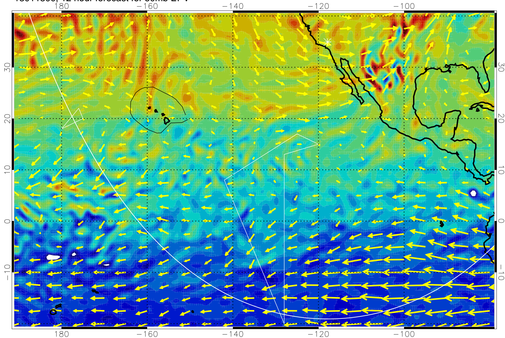
13011300, 12 hour forecast for 50mb EPV
