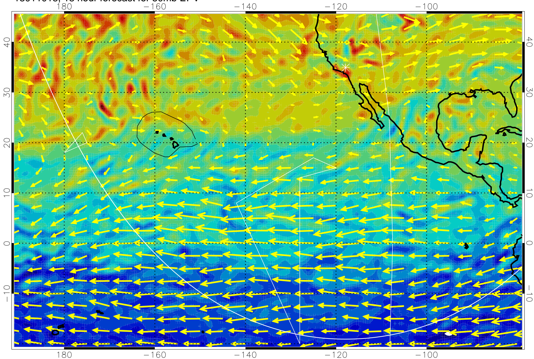
13011018, 18 hour forecast for 50mb EPV
