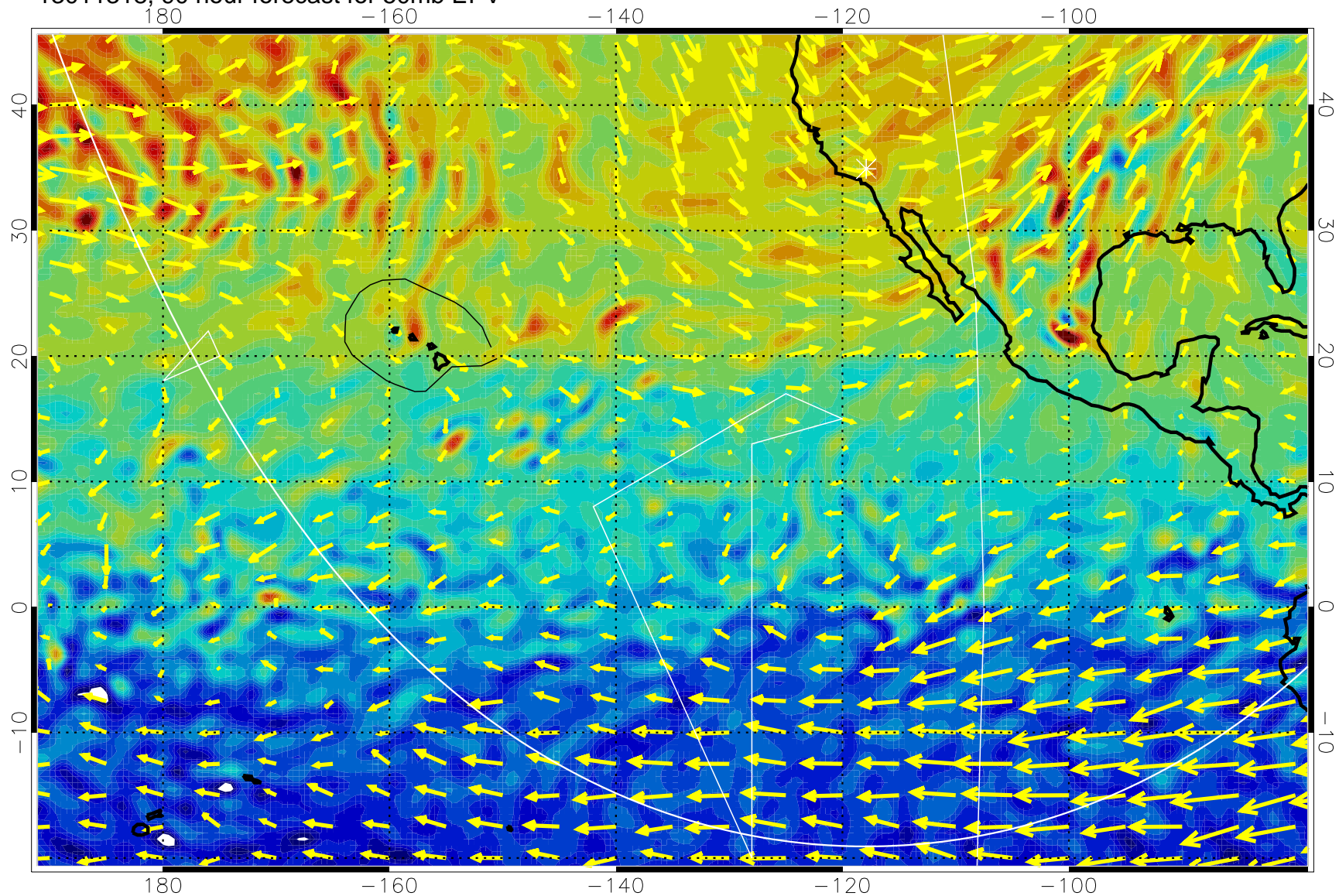
13011318, 90 hour forecast for 50mb EPV
