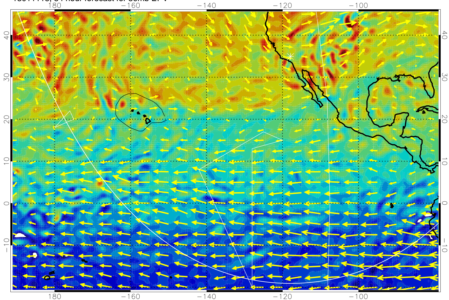
13011118, 54 hour forecast for 50mb EPV
