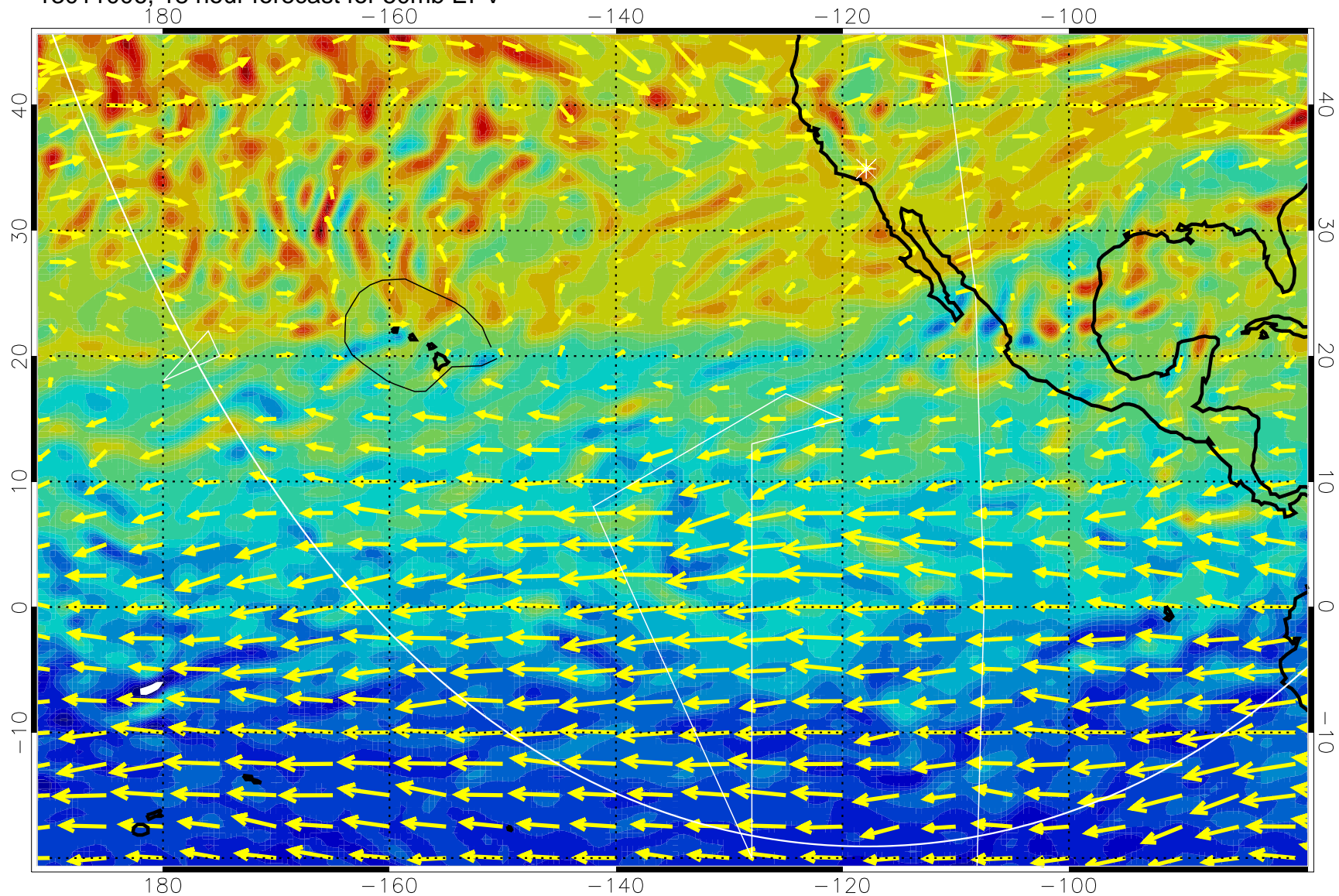
13011006, 18 hour forecast for 50mb EPV
