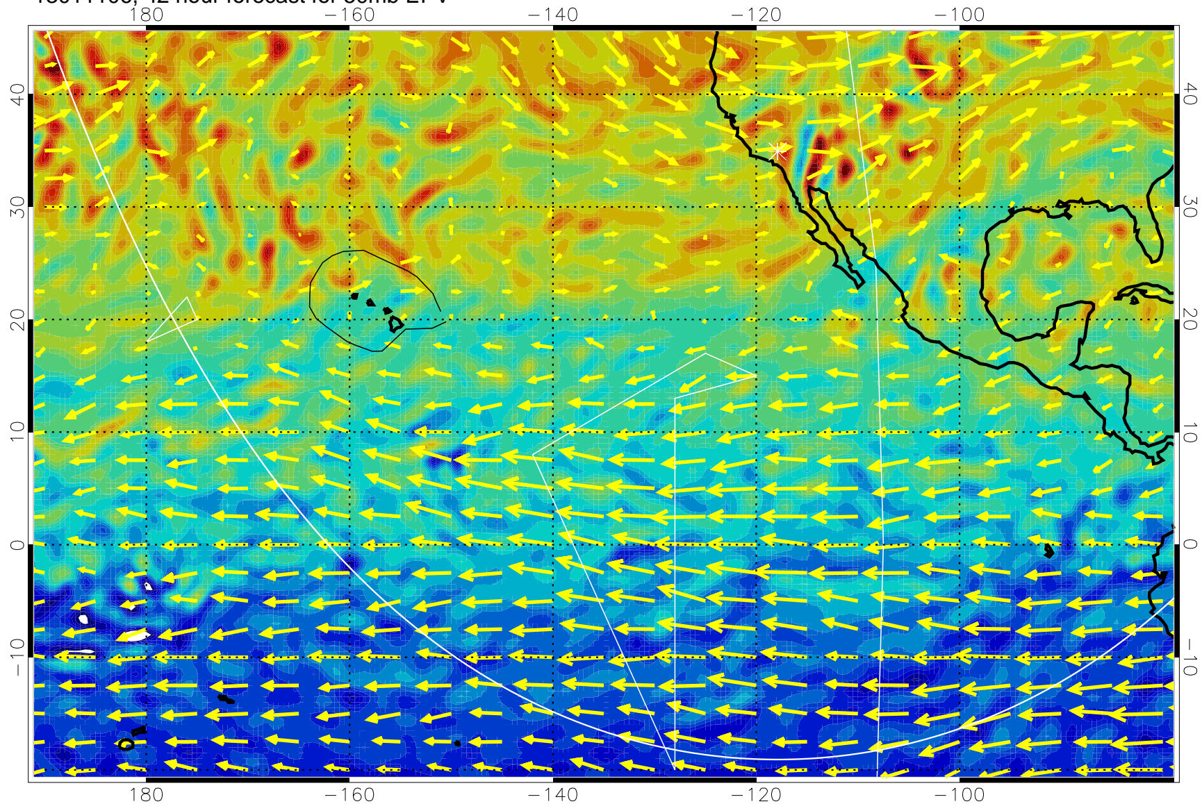
13011106, 42 hour forecast for 50mb EPV
