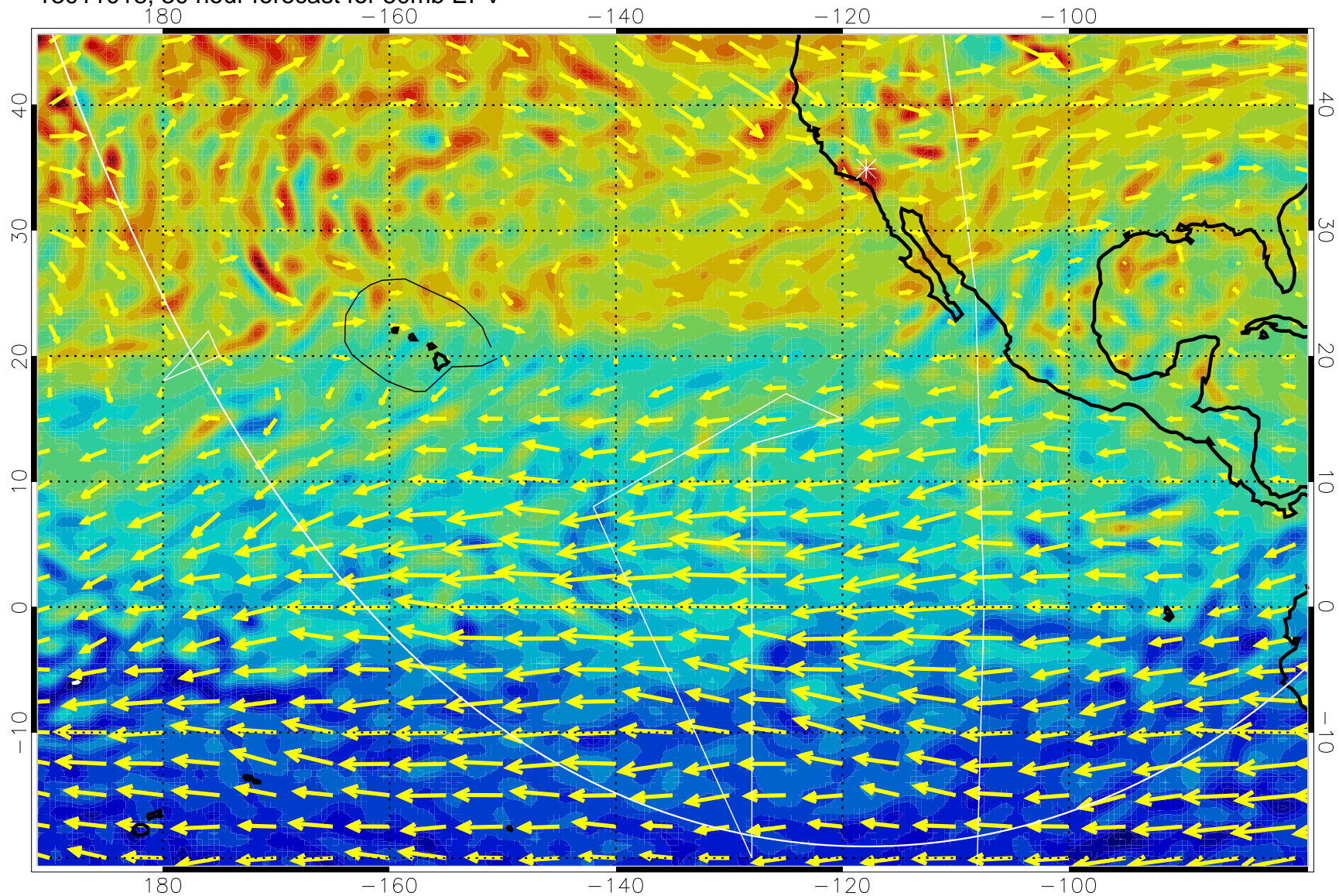
13011018, 30 hour forecast for 50mb EPV
