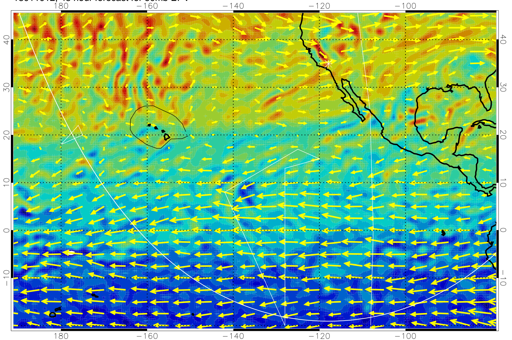
13011012, 48 hour forecast for 50mb EPV
