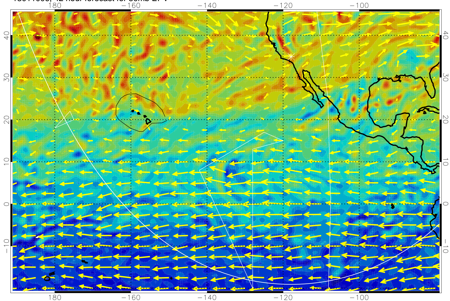
13011006, 42 hour forecast for 50mb EPV
