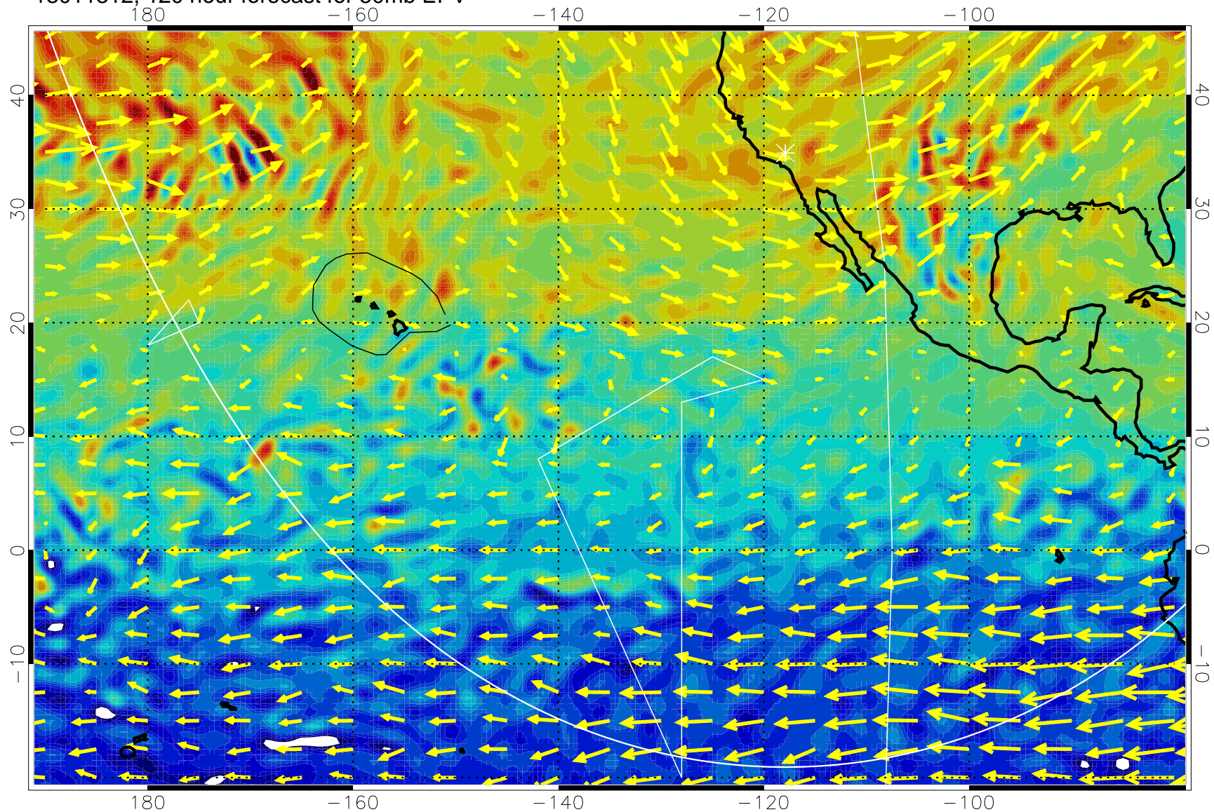
13011312, 120 hour forecast for 50mb EPV
