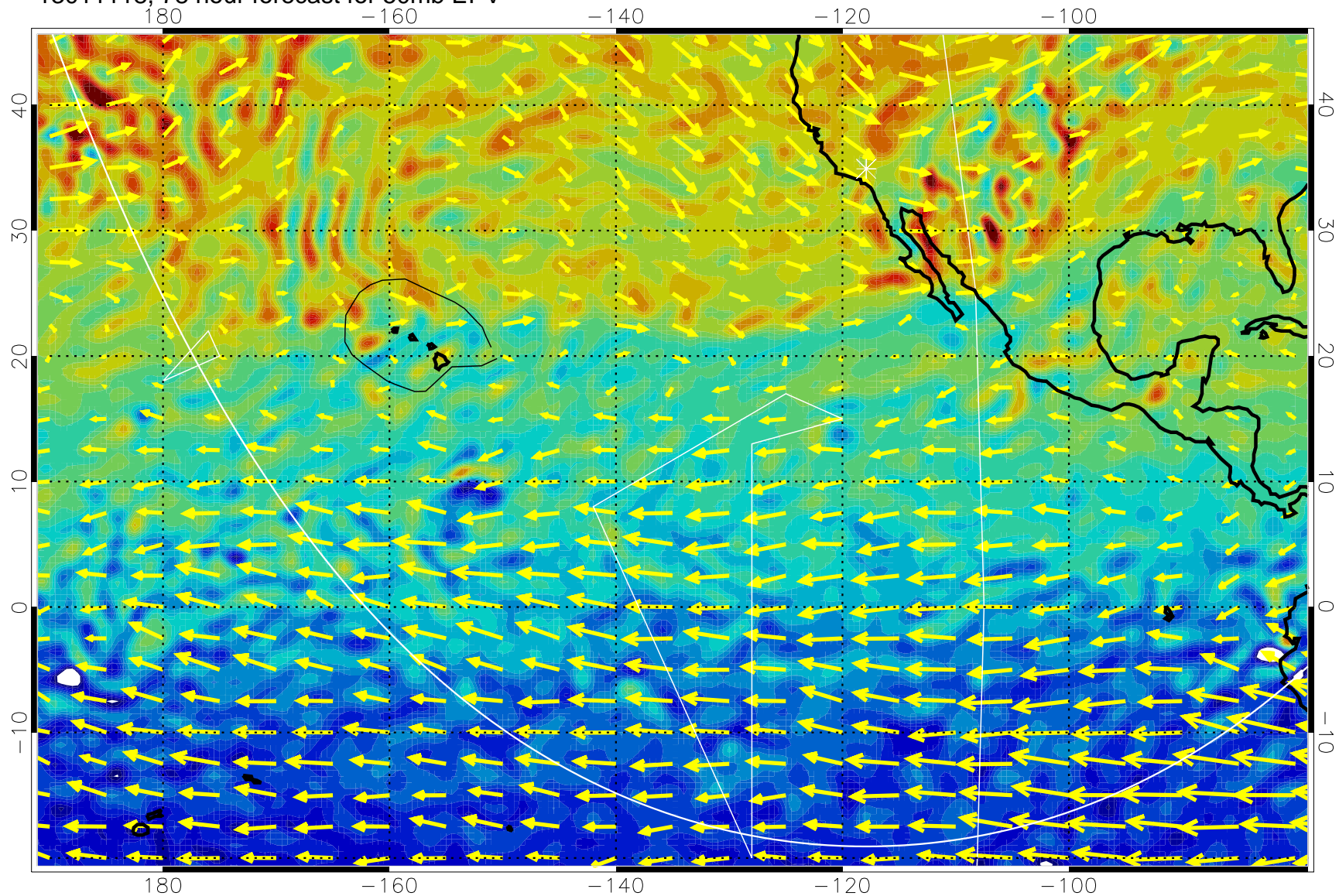
13011118, 78 hour forecast for 50mb EPV
