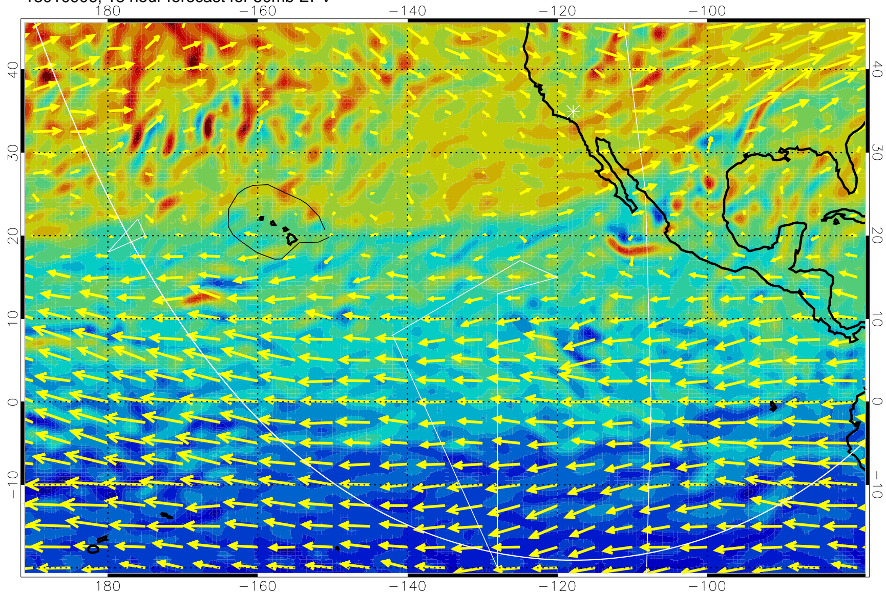
13010906, 18 hour forecast for 50mb EPV
