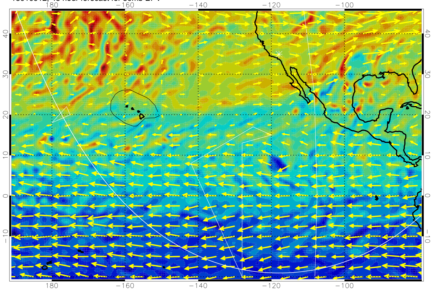
13010912, 48 hour forecast for 50mb EPV
