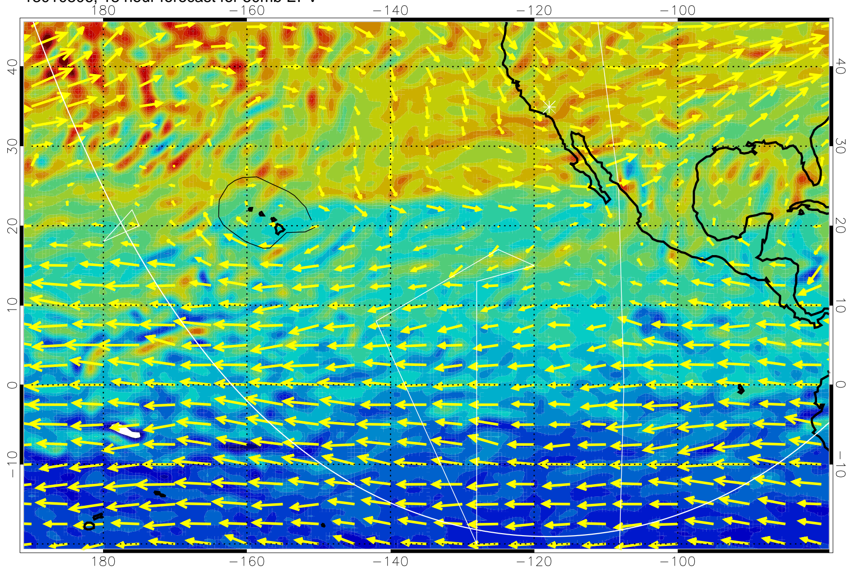
13010806, 18 hour forecast for 50mb EPV
