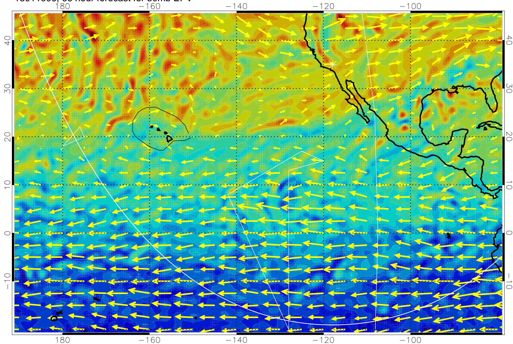
13011006, 66 hour forecast for 50mb EPV
