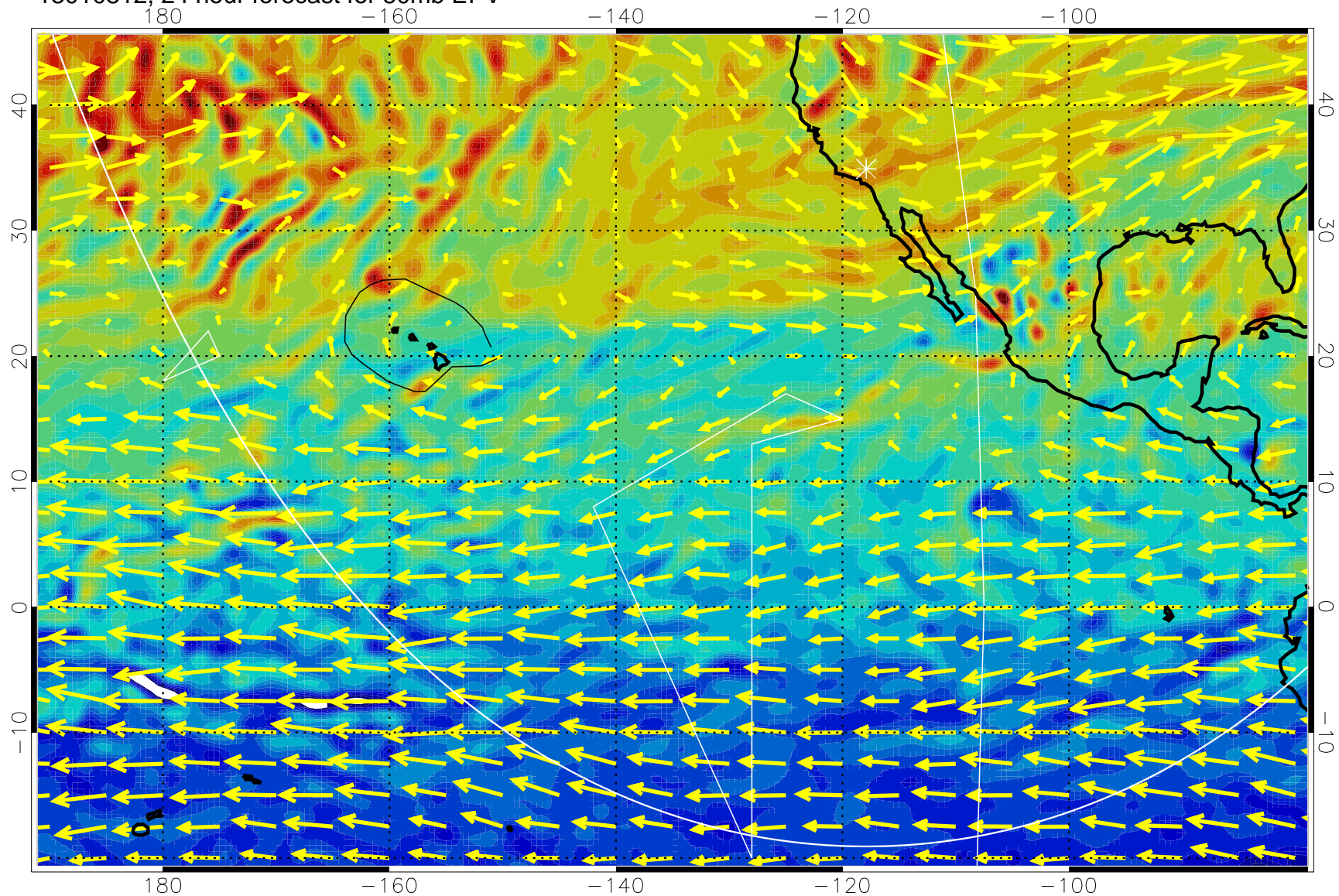
13010812, 24 hour forecast for 50mb EPV
