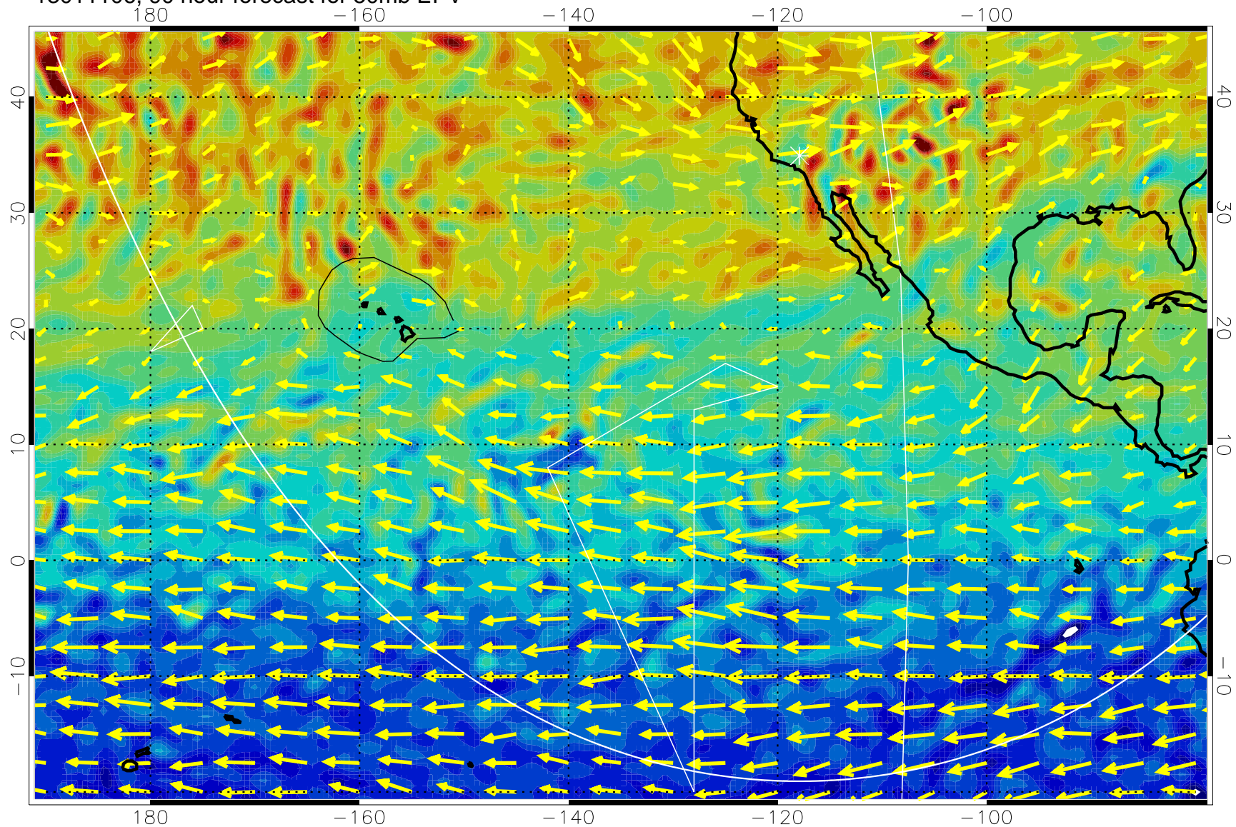
13011106, 90 hour forecast for 50mb EPV
