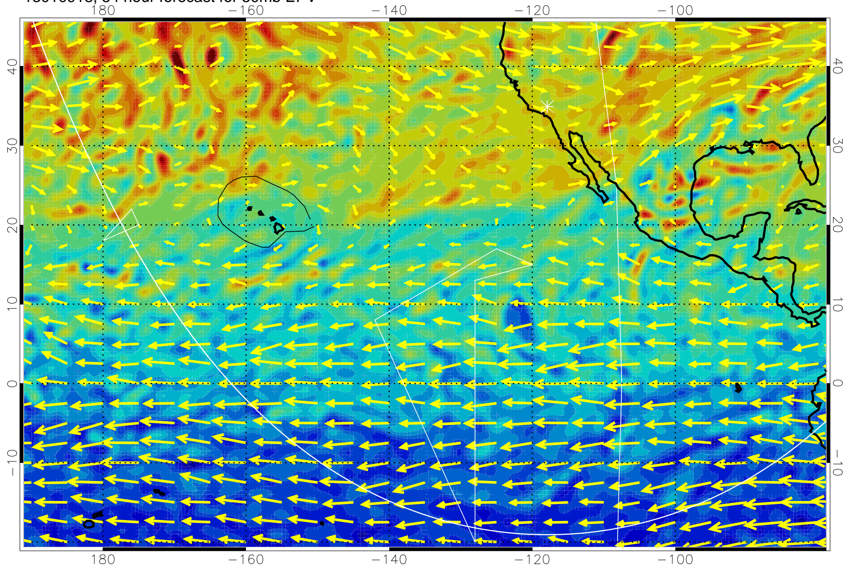
13010918, 54 hour forecast for 50mb EPV
