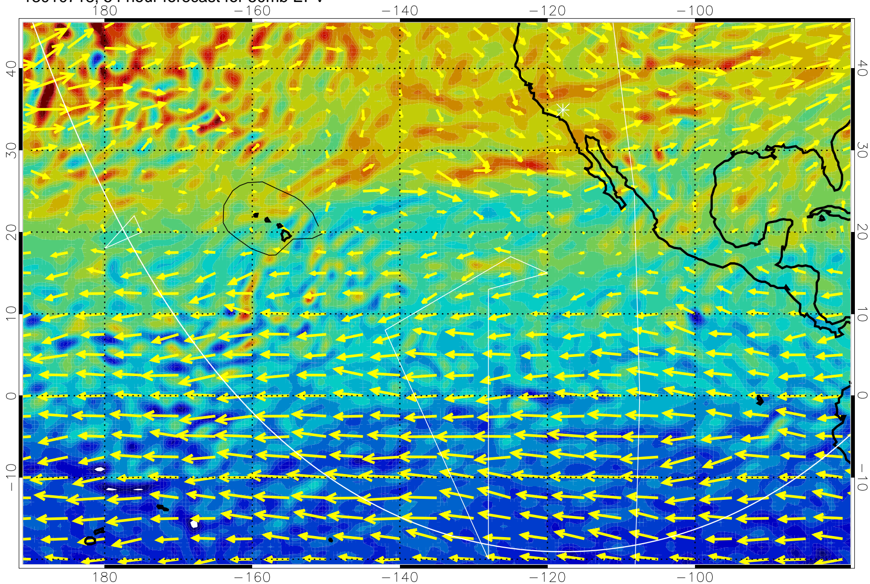
13010718, 54 hour forecast for 50mb EPV
