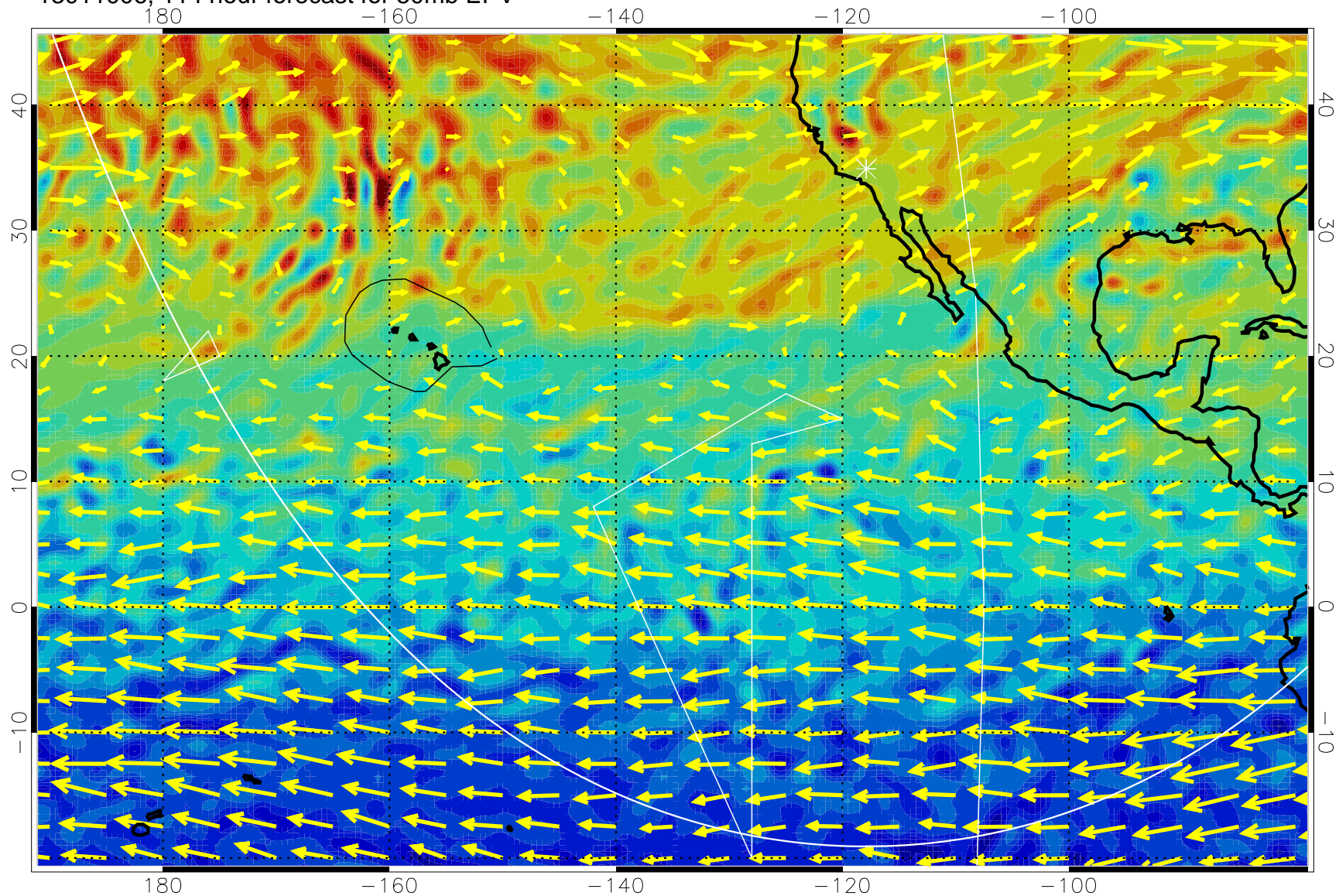
13011006, 114 hour forecast for 50mb EPV
