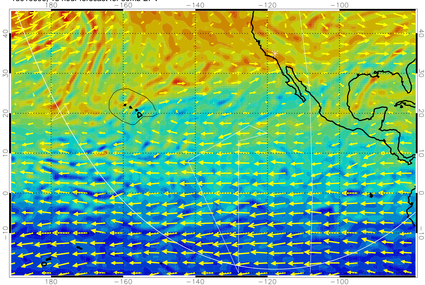
13010606, 18 hour forecast for 50mb EPV
