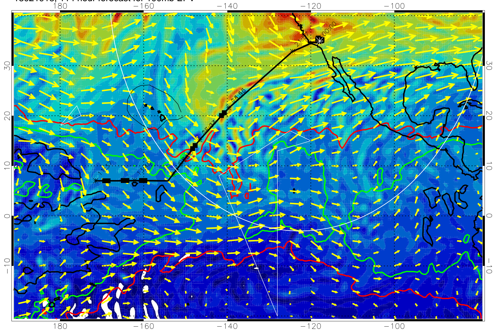
13021918, 114 hour forecast for 100mb EPV
