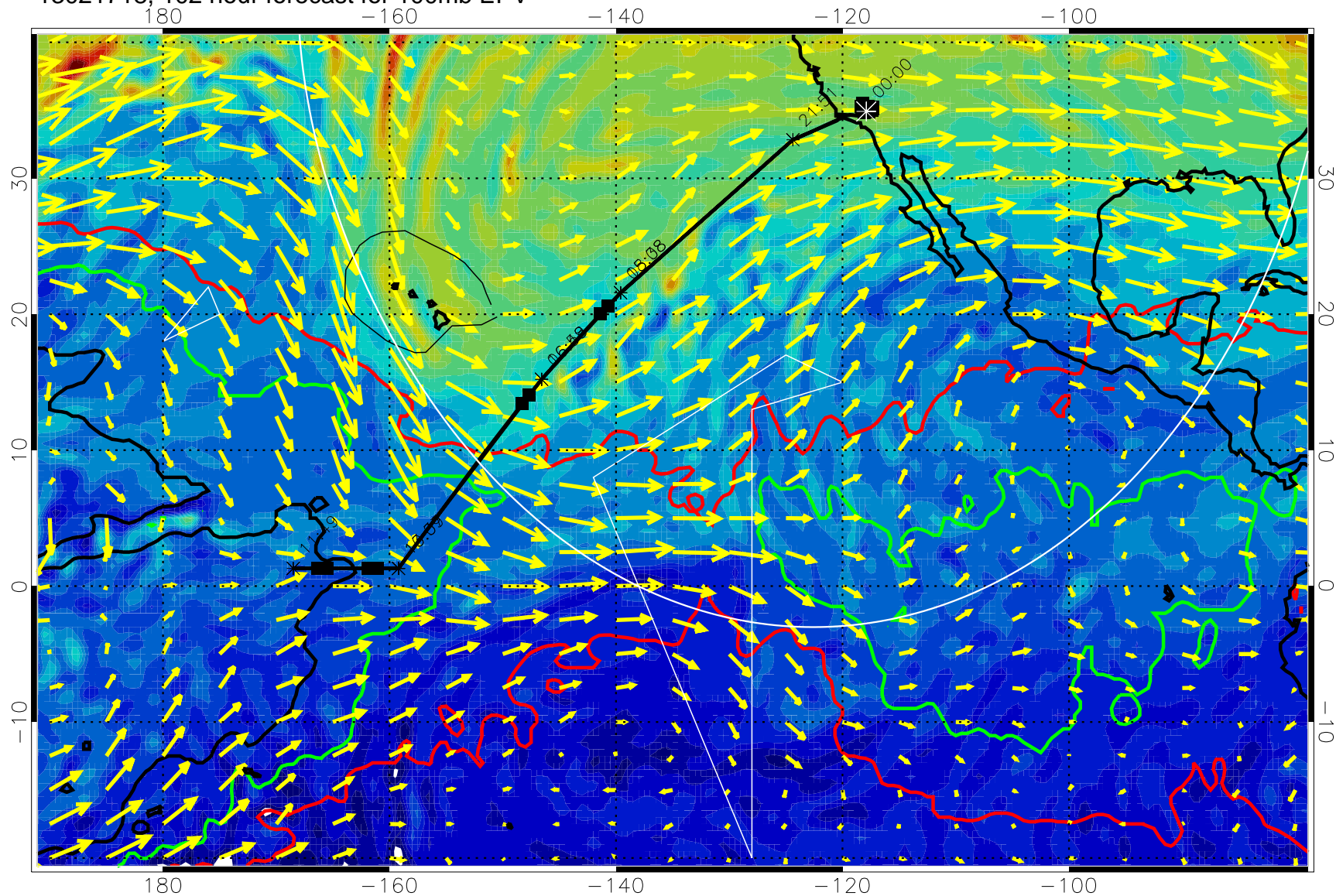
13021718, 102 hour forecast for 100mb EPV
