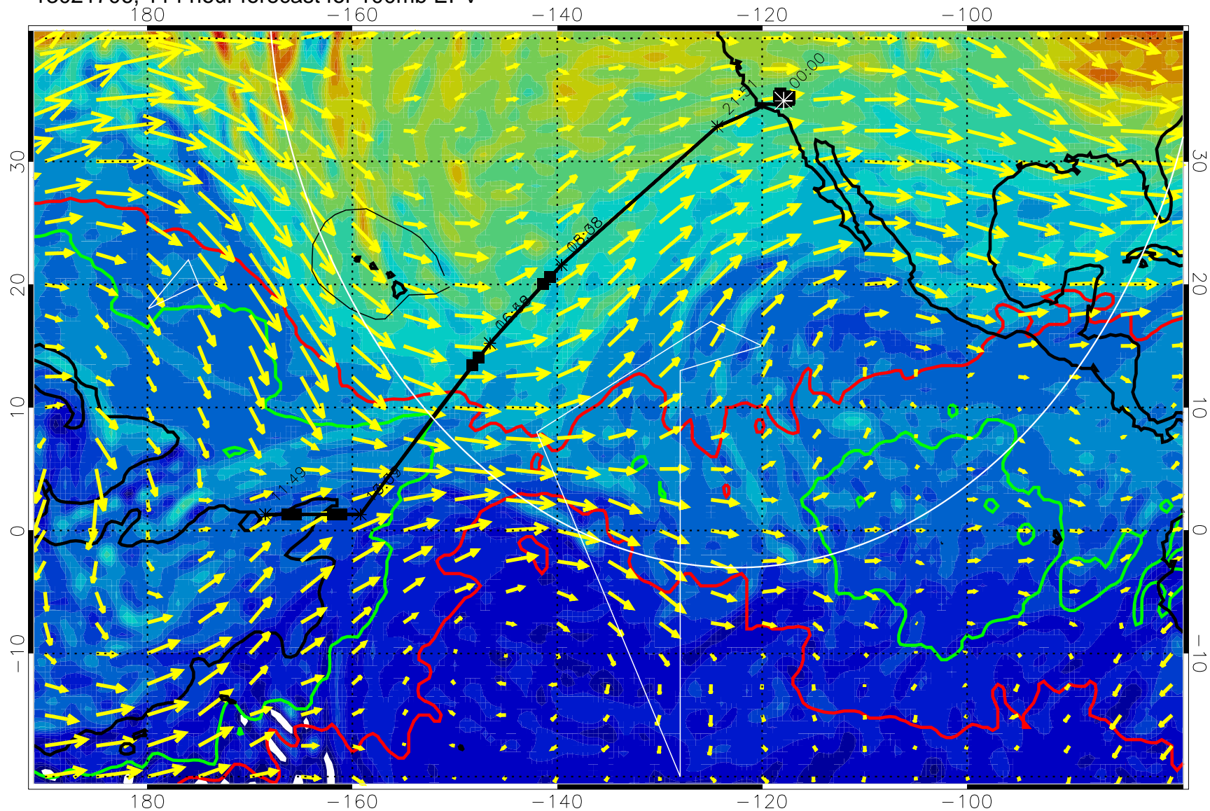
13021706, 114 hour forecast for 100mb EPV
