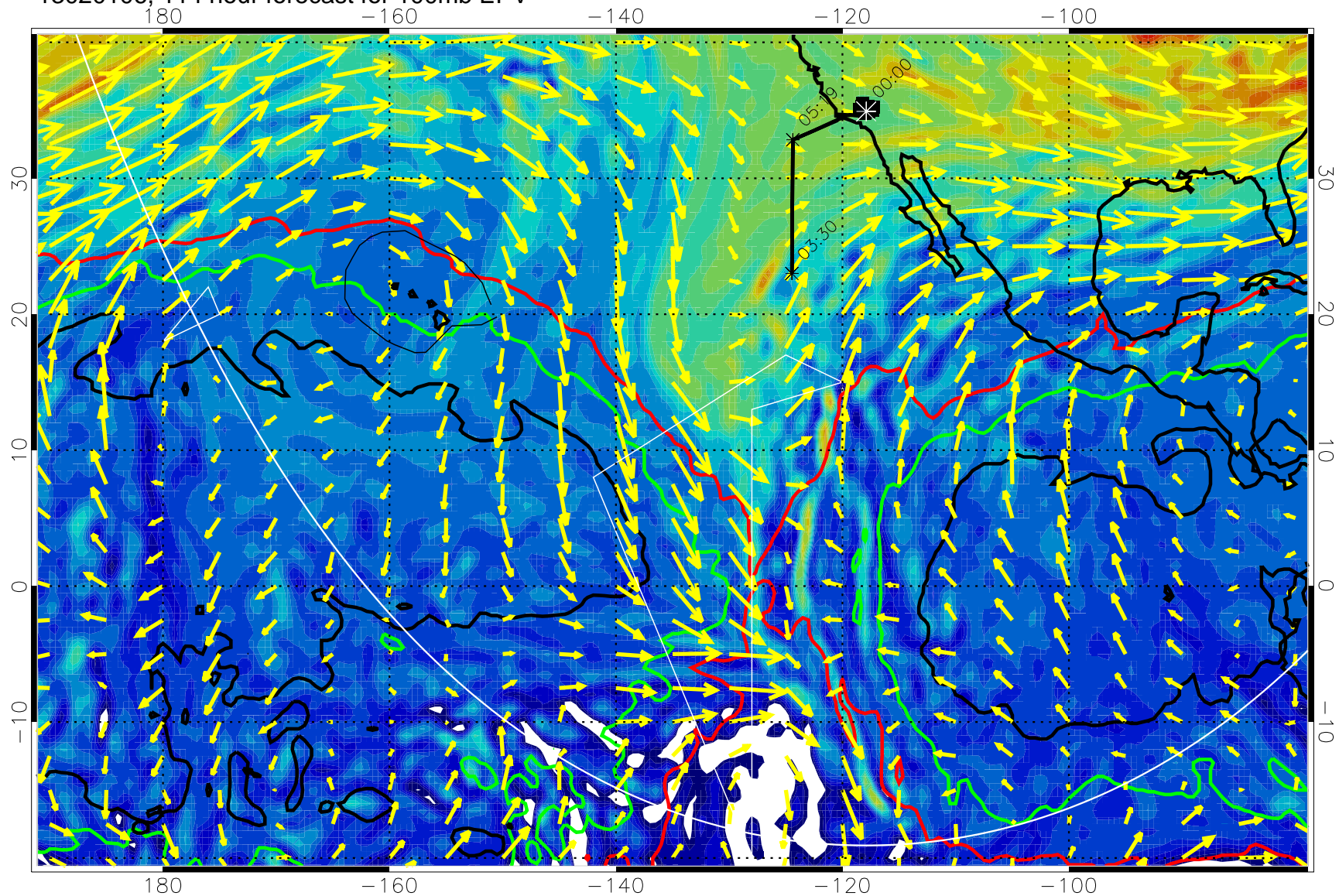
13020106, 114 hour forecast for 100mb EPV
