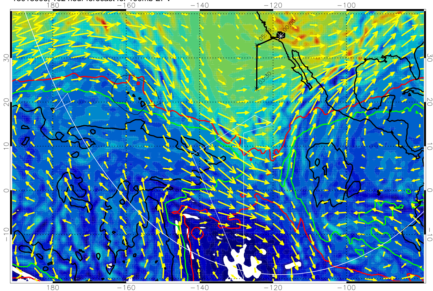
13013006, 102 hour forecast for 100mb EPV
