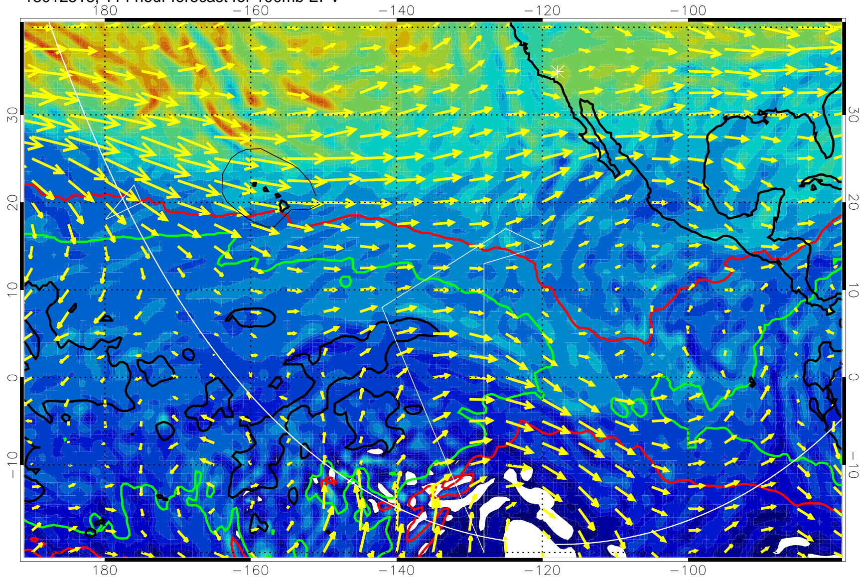
13012518, 114 hour forecast for 100mb EPV
