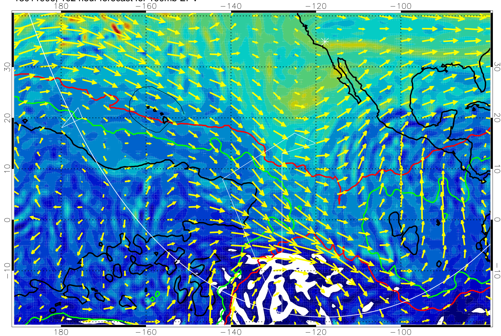
13011906, 102 hour forecast for 100mb EPV
