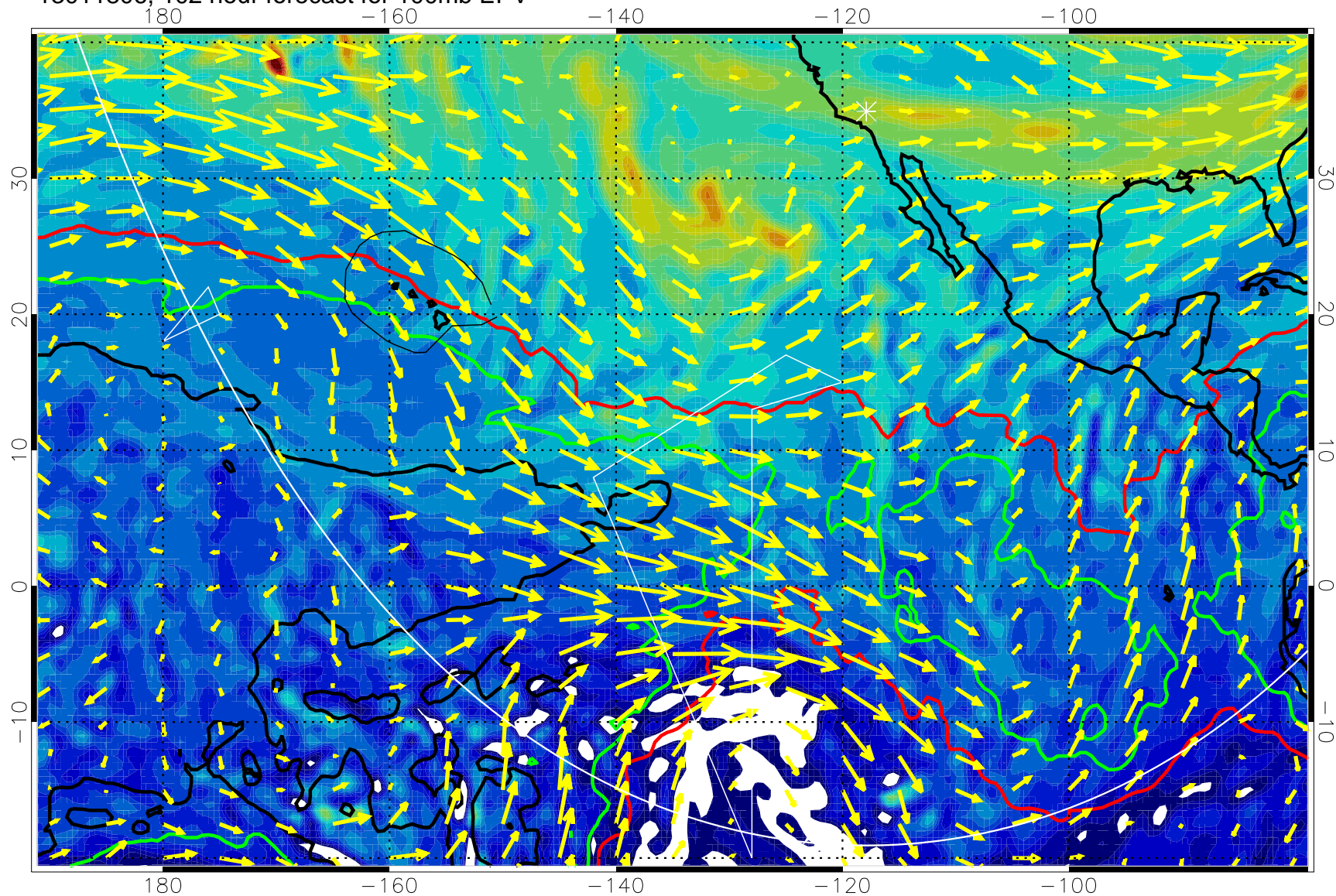
13011806, 102 hour forecast for 100mb EPV
