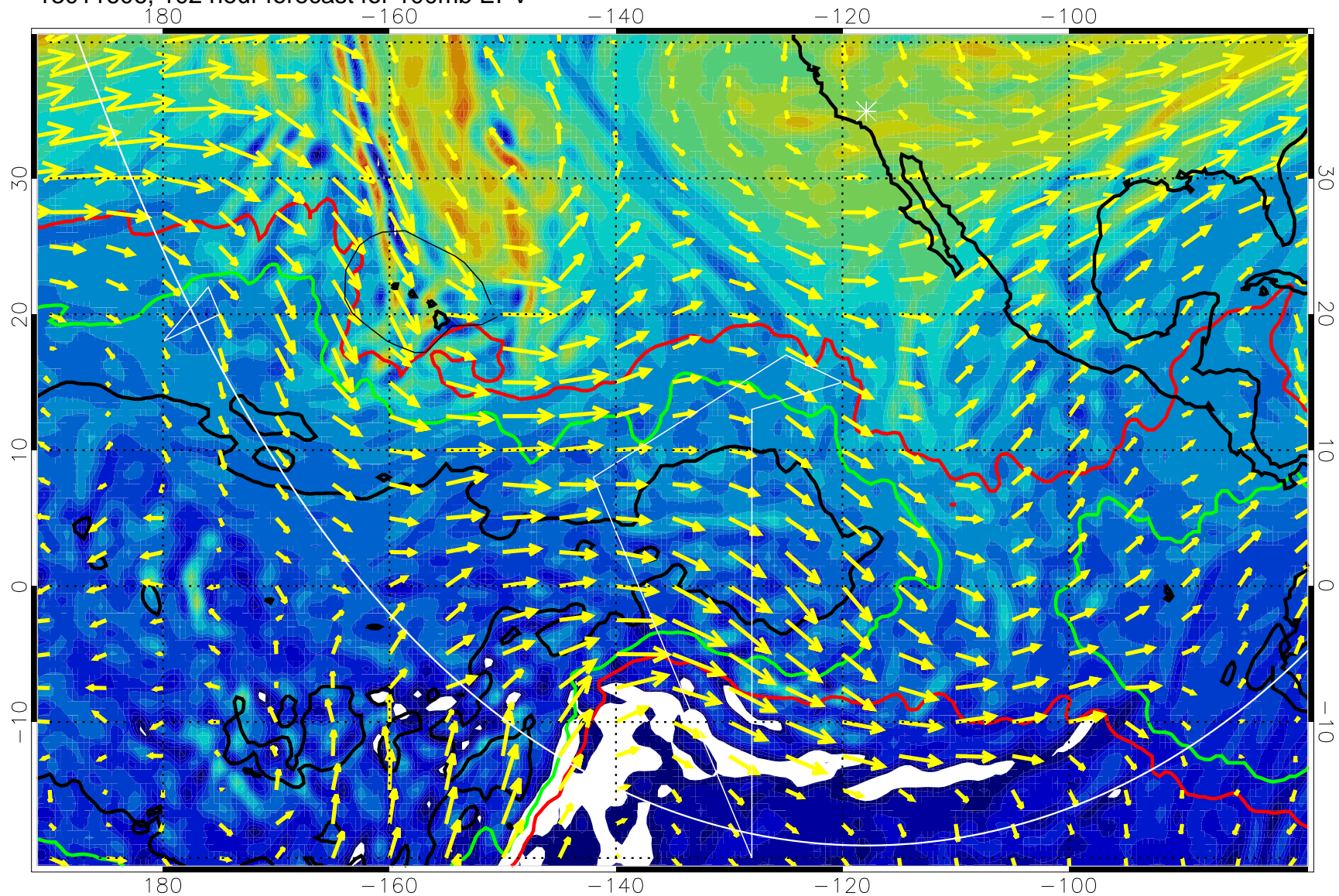
13011606, 102 hour forecast for 100mb EPV
