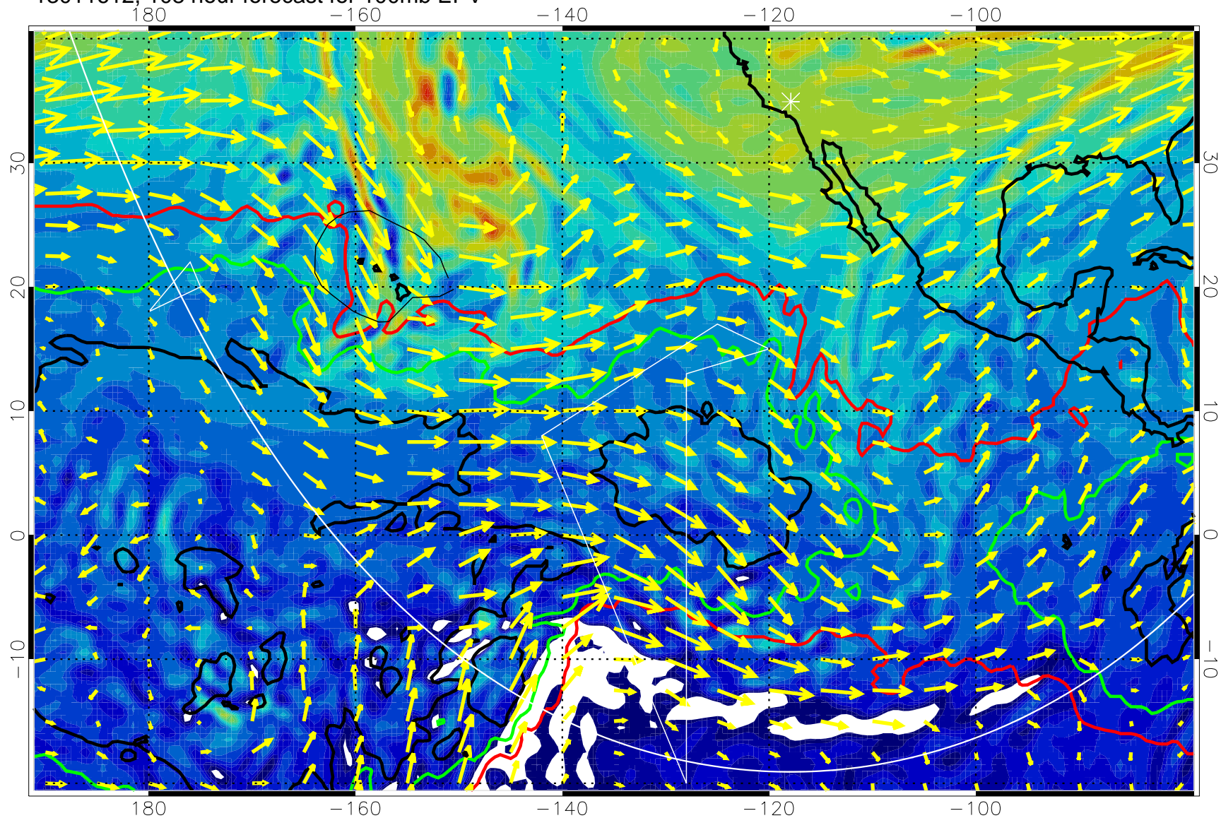
13011612, 108 hour forecast for 100mb EPV
