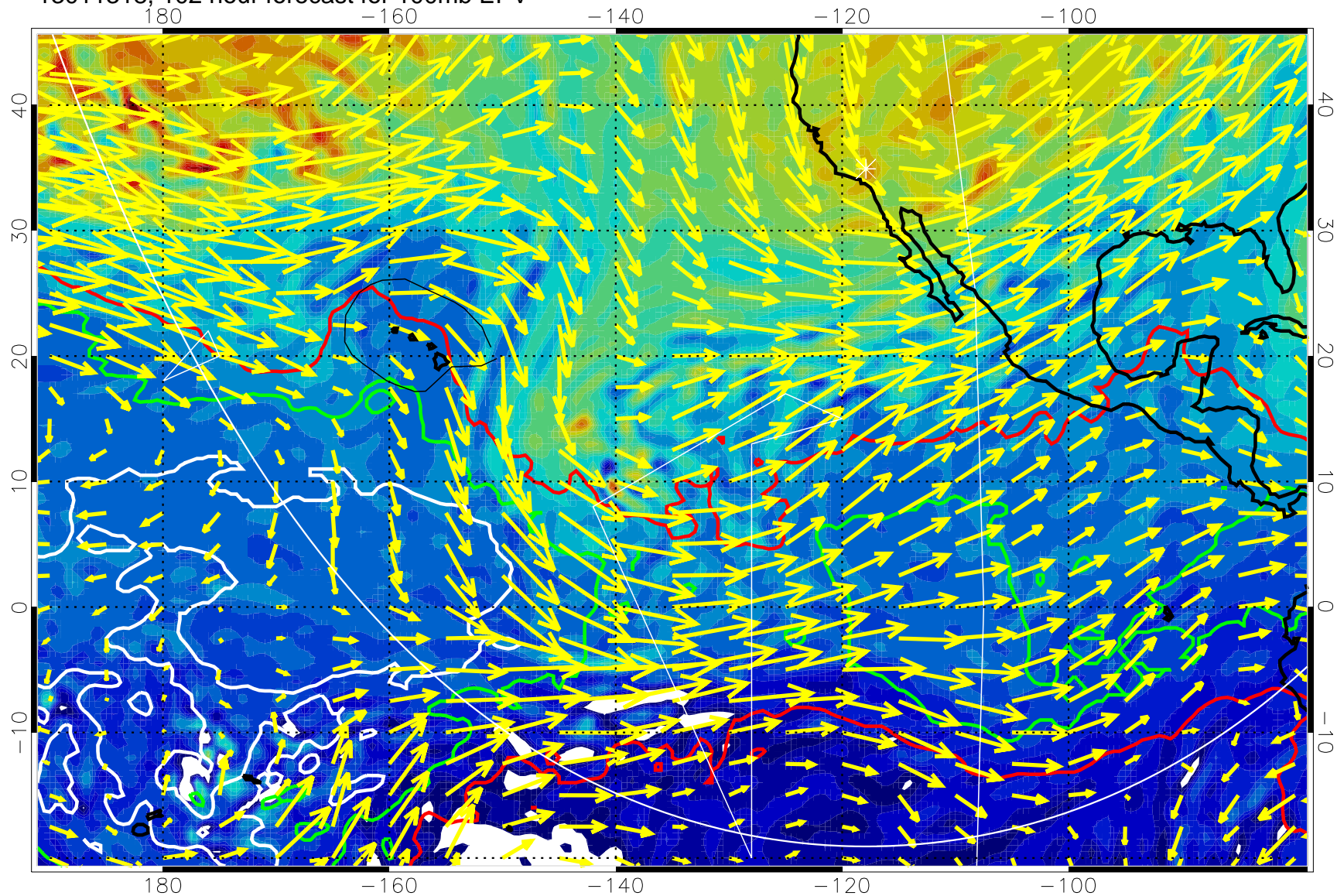
13011318, 102 hour forecast for 100mb EPV
