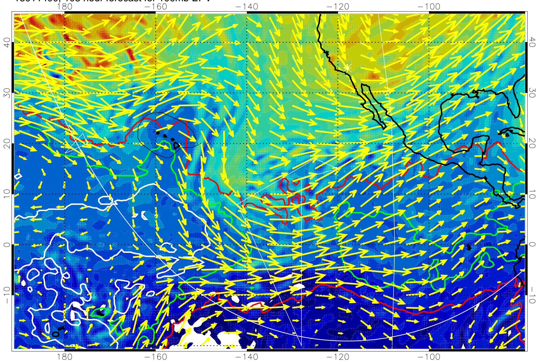
13011400, 108 hour forecast for 100mb EPV
