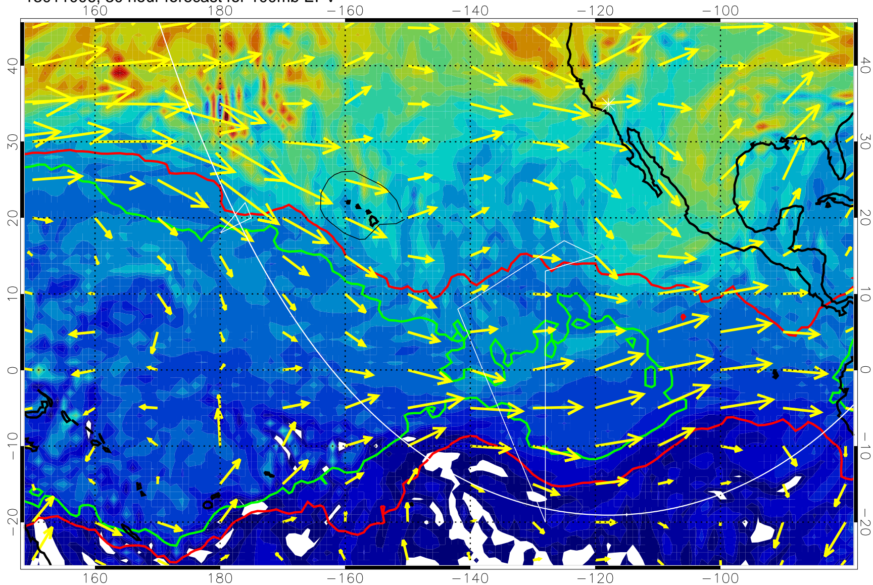
13011006, 30 hour forecast for 100mb EPV
