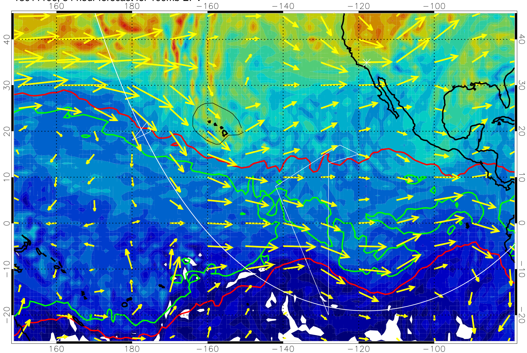
13011106, 54 hour forecast for 100mb EPV
