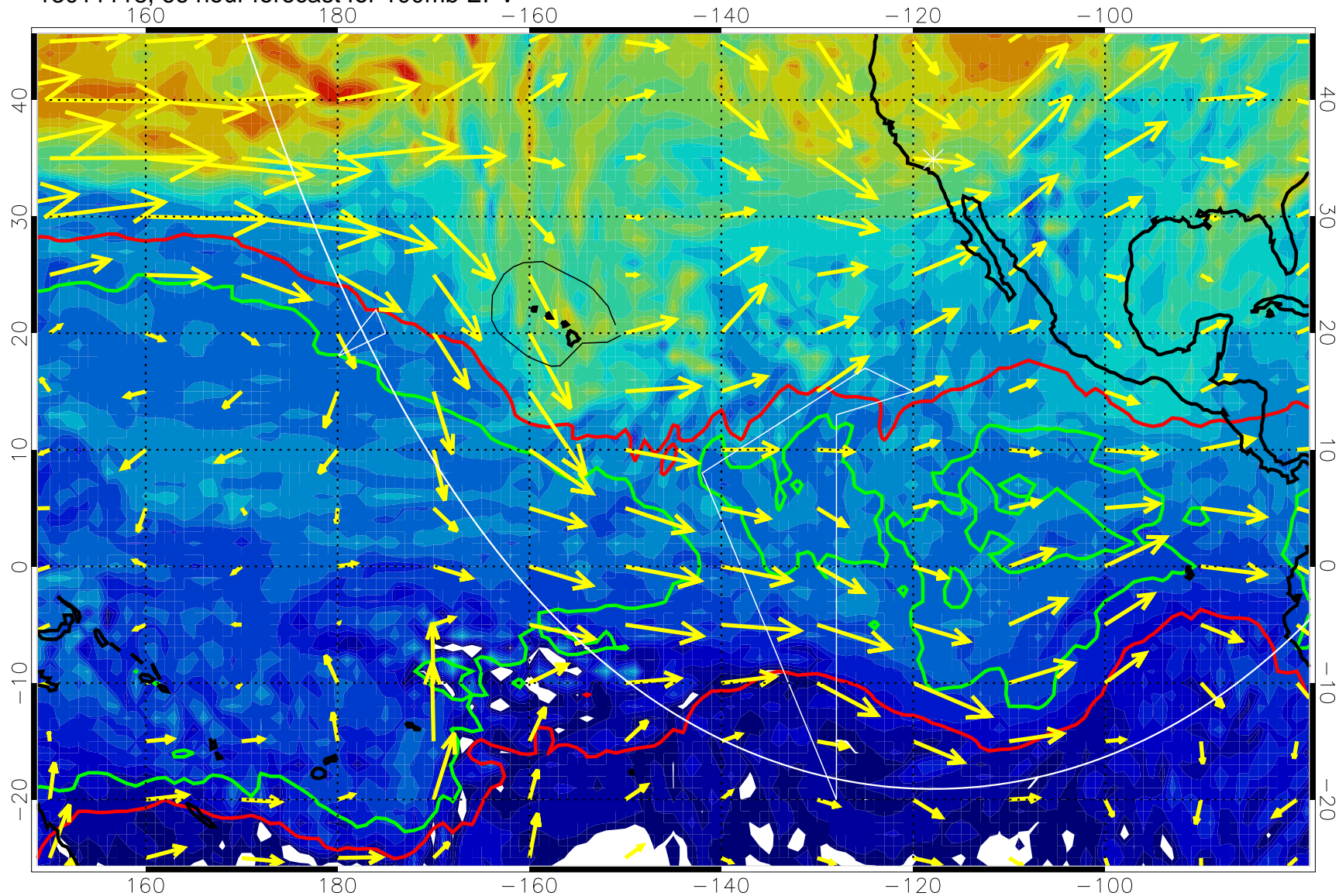
13011118, 66 hour forecast for 100mb EPV
