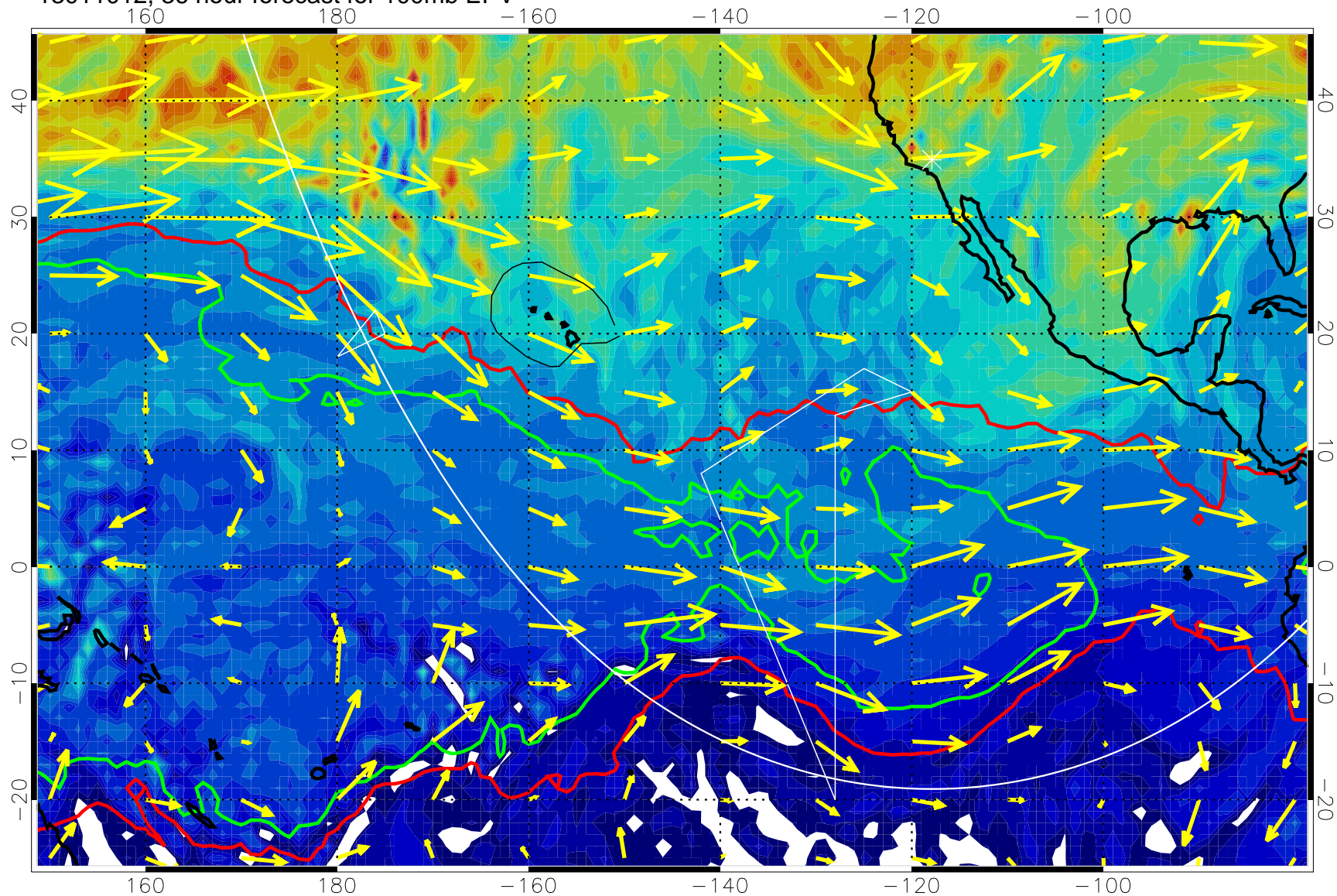
13011012, 36 hour forecast for 100mb EPV
