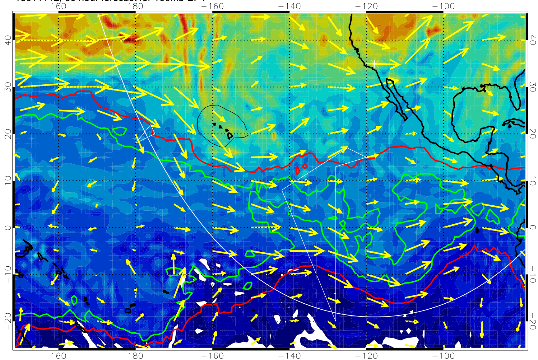
13011112, 60 hour forecast for 100mb EPV
