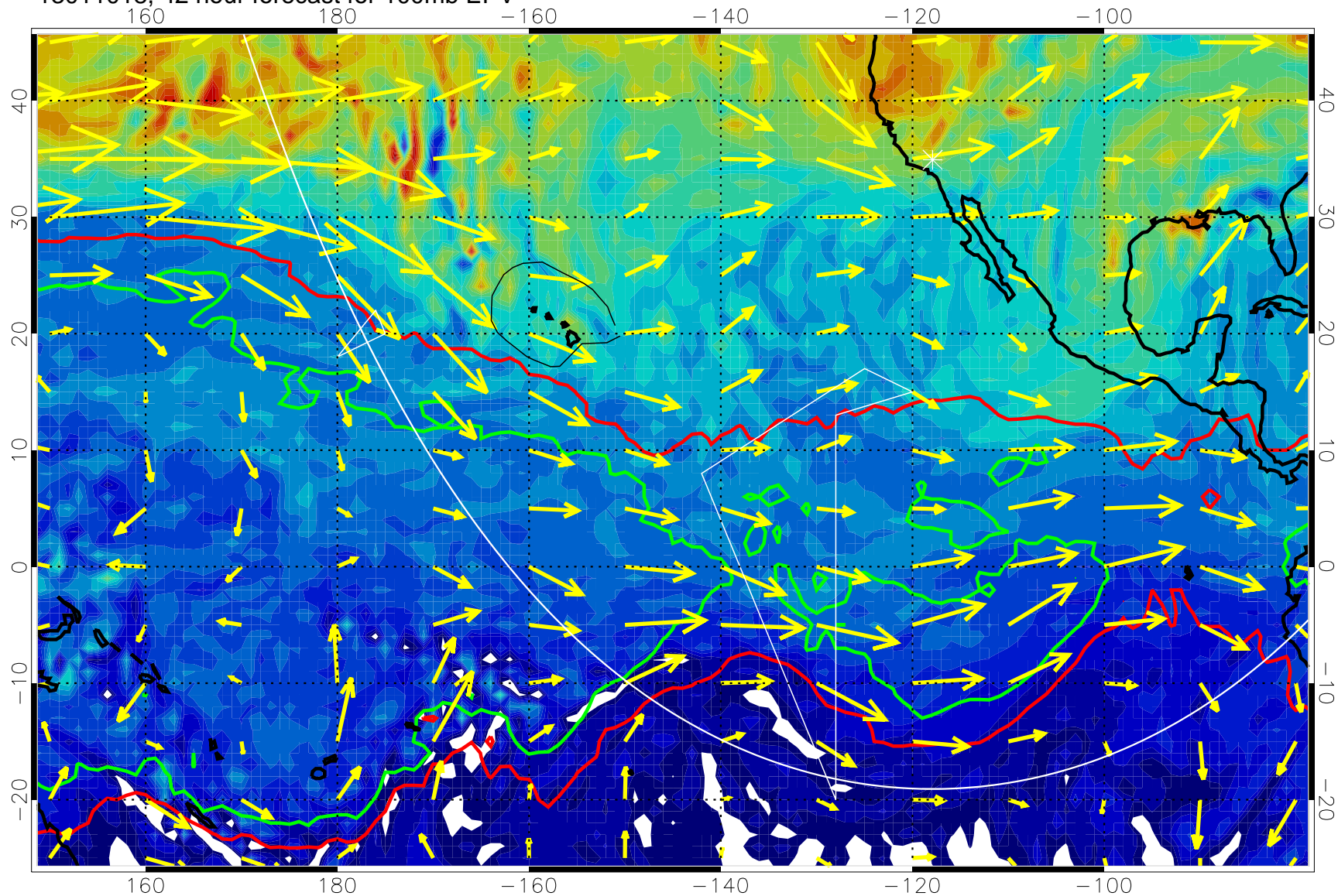
13011018, 42 hour forecast for 100mb EPV
