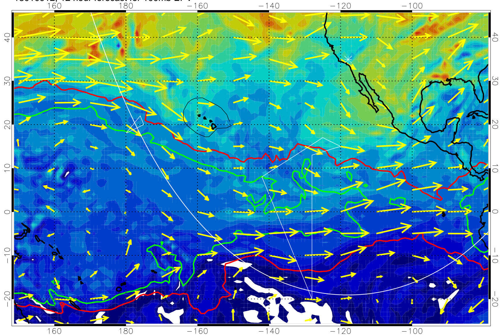
13010912, 12 hour forecast for 100mb EPV
