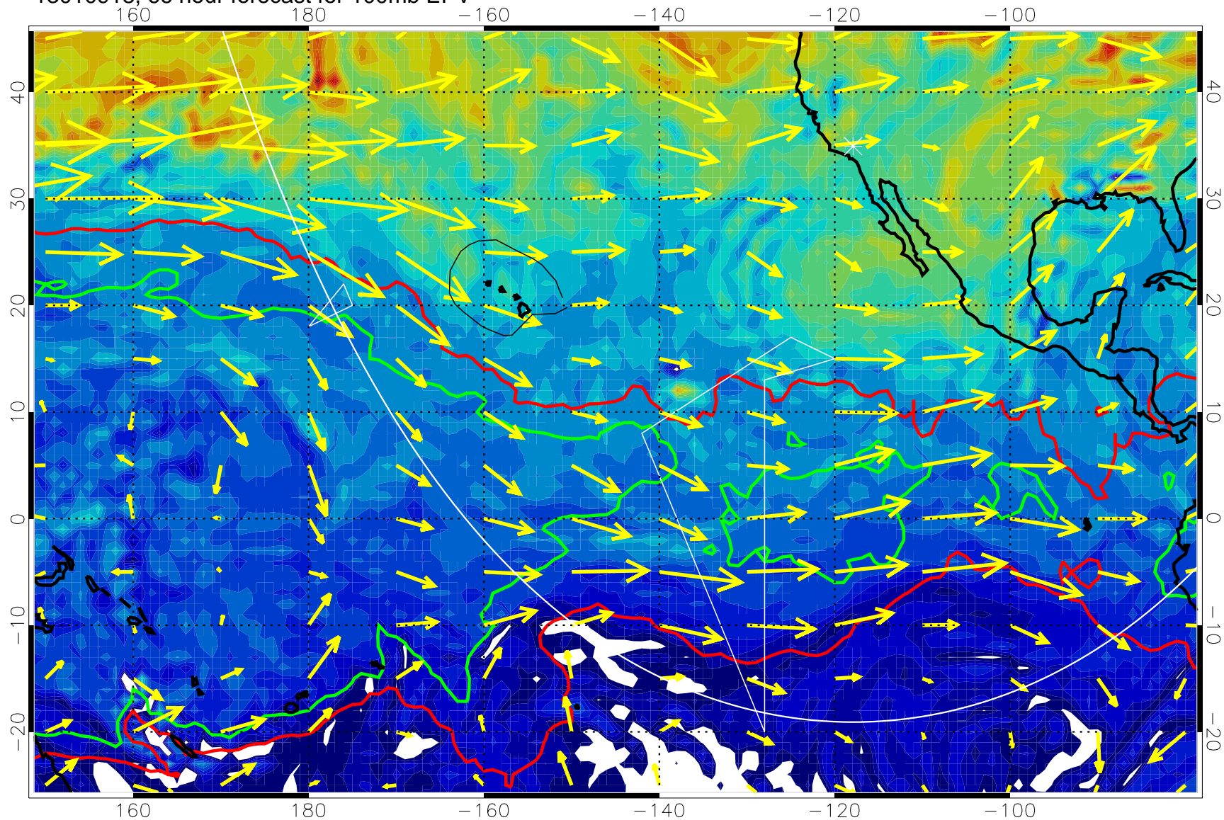
13010918, 66 hour forecast for 100mb EPV
