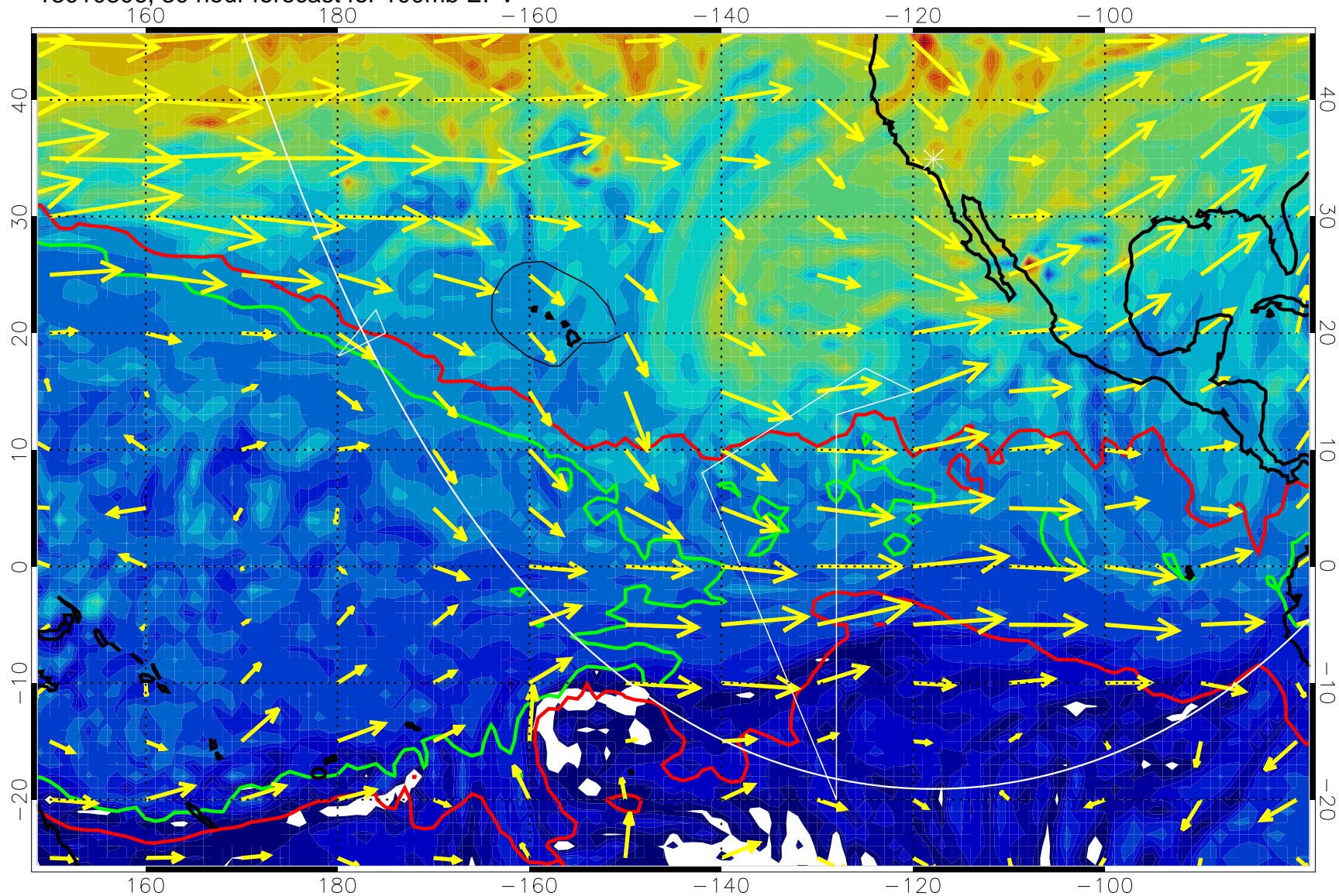
13010806, 30 hour forecast for 100mb EPV
