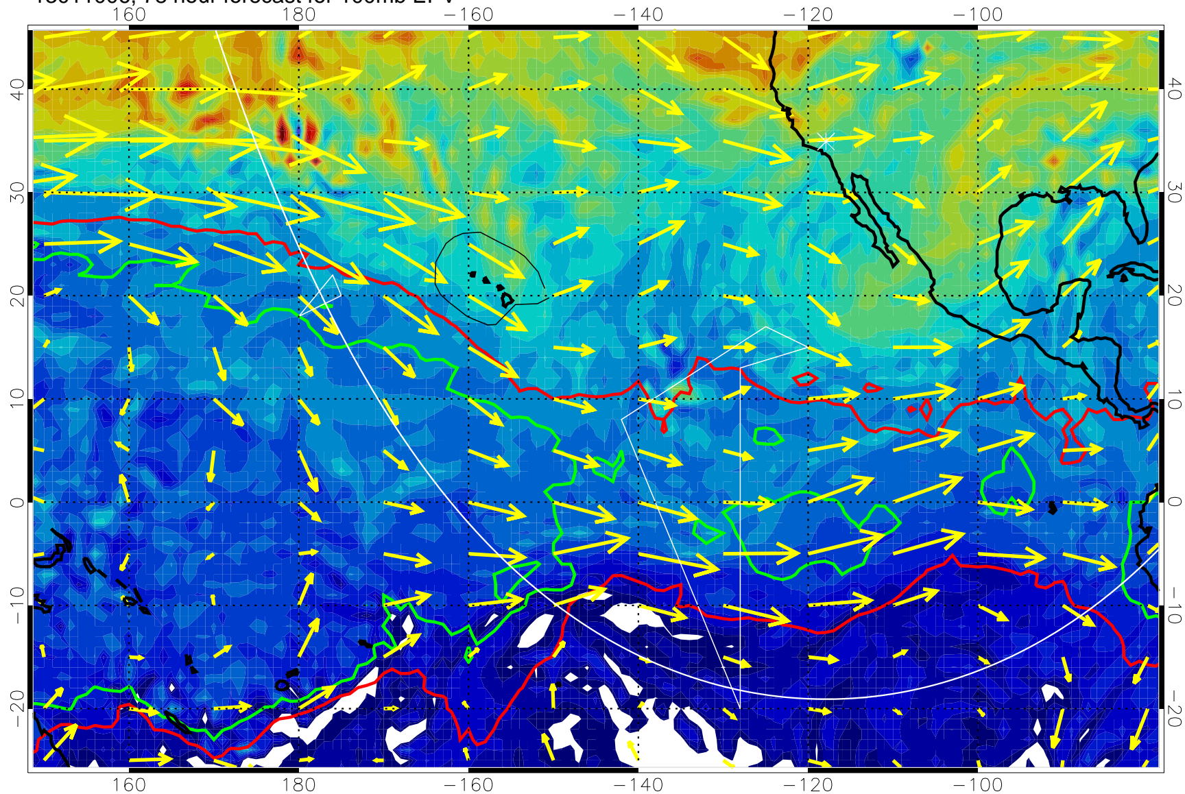
13011006, 78 hour forecast for 100mb EPV
