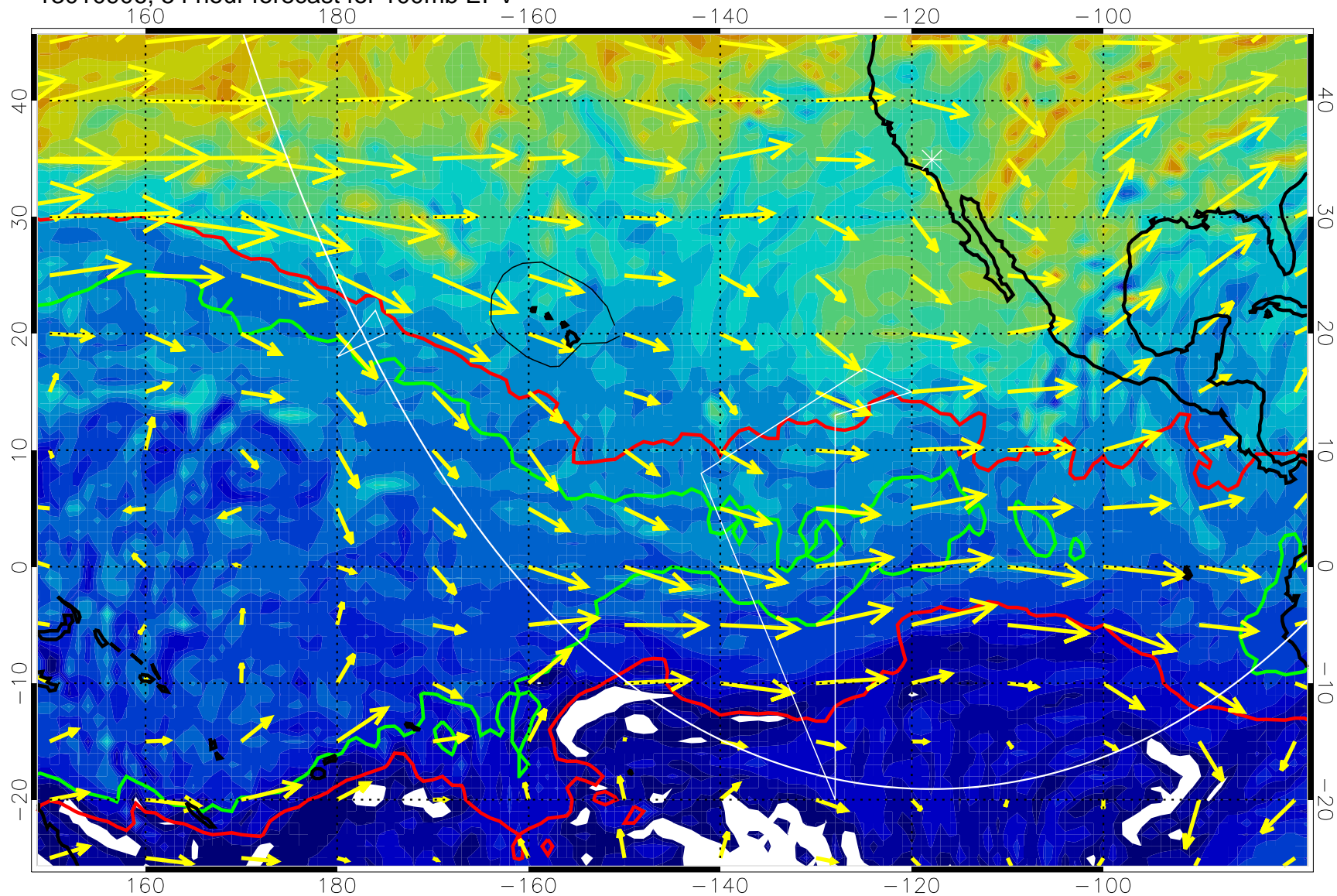
13010906, 54 hour forecast for 100mb EPV
