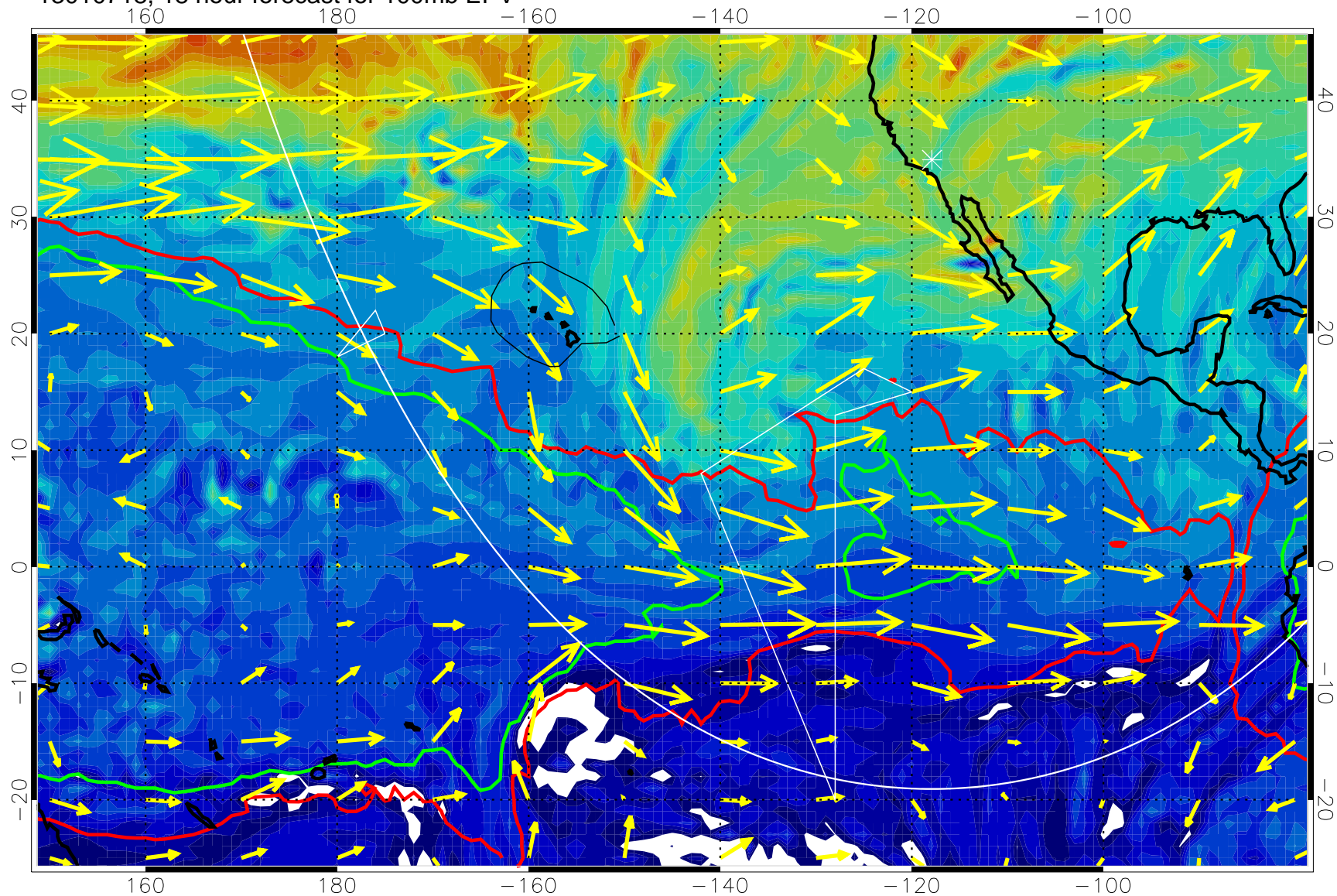
13010718, 18 hour forecast for 100mb EPV
