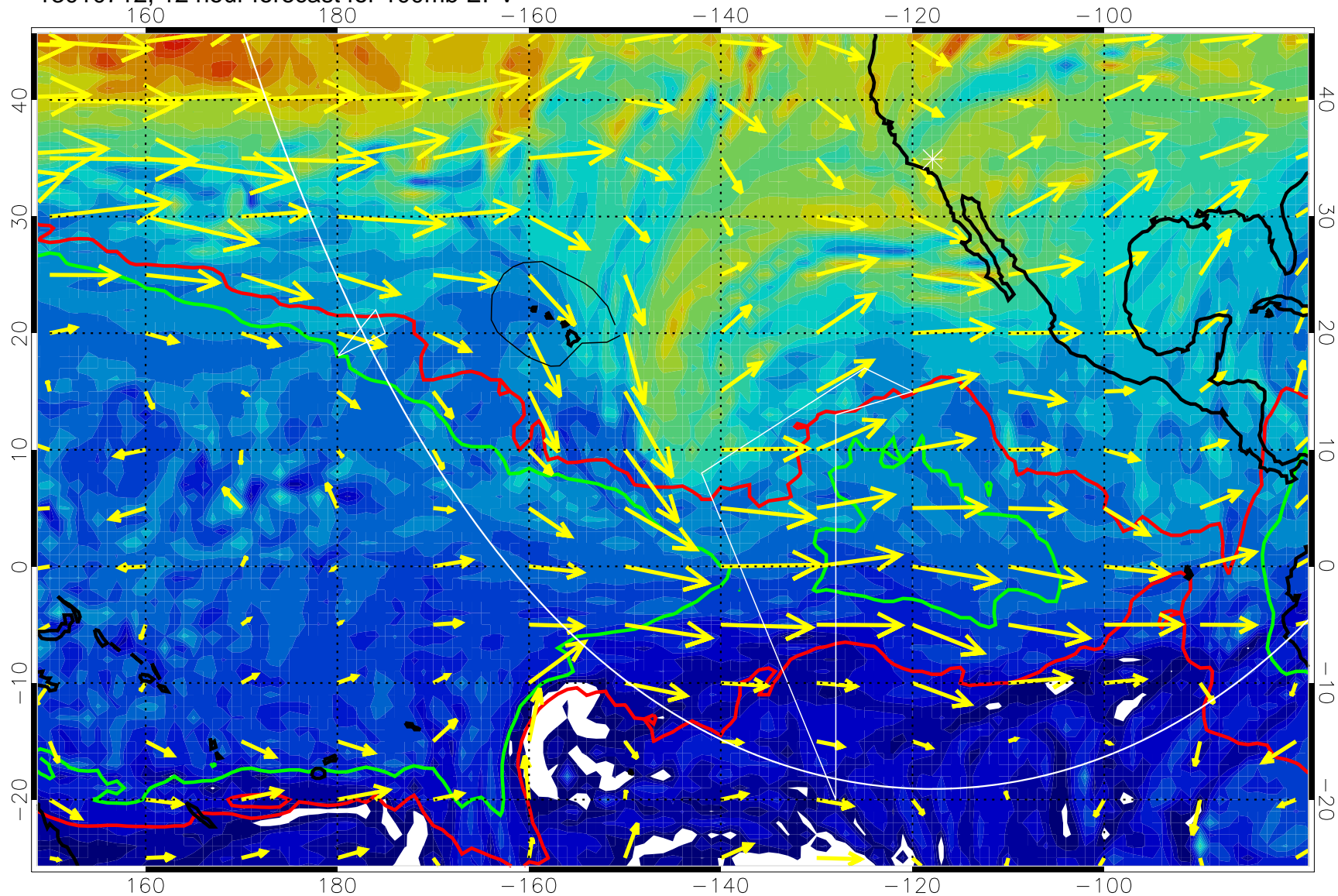
13010712, 12 hour forecast for 100mb EPV
