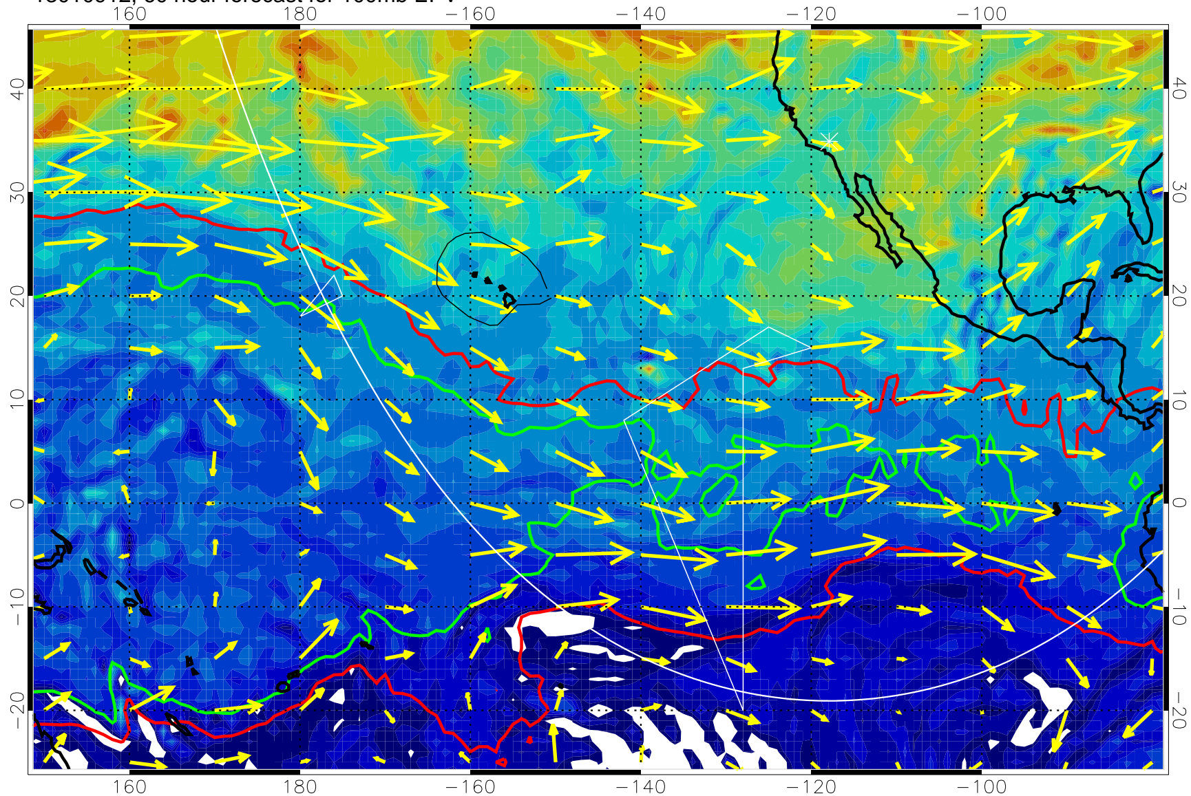
13010912, 60 hour forecast for 100mb EPV
