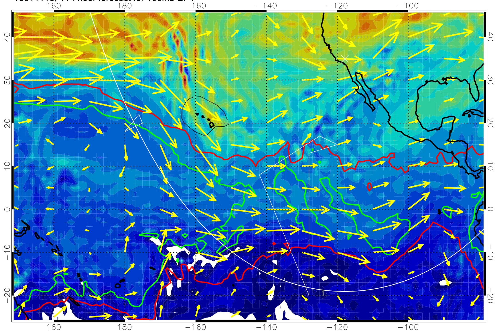
13011118, 114 hour forecast for 100mb EPV
