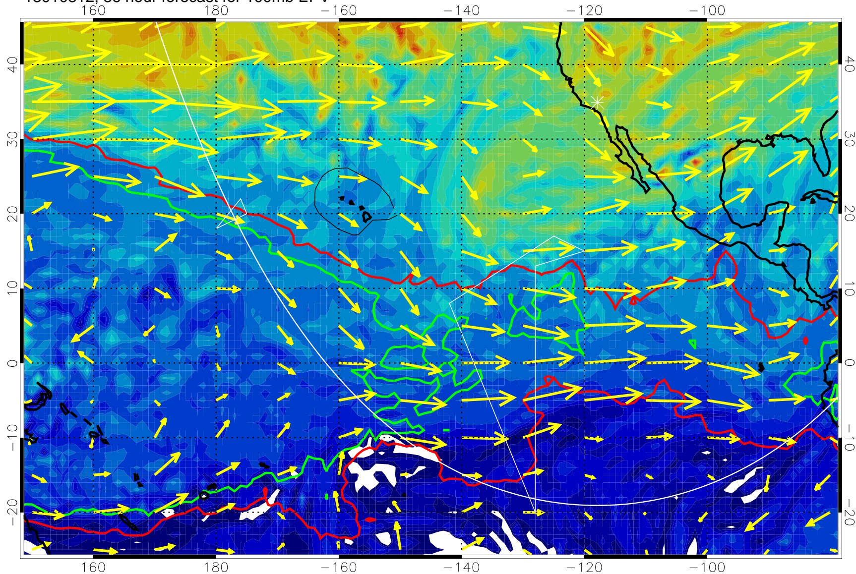
13010812, 36 hour forecast for 100mb EPV
