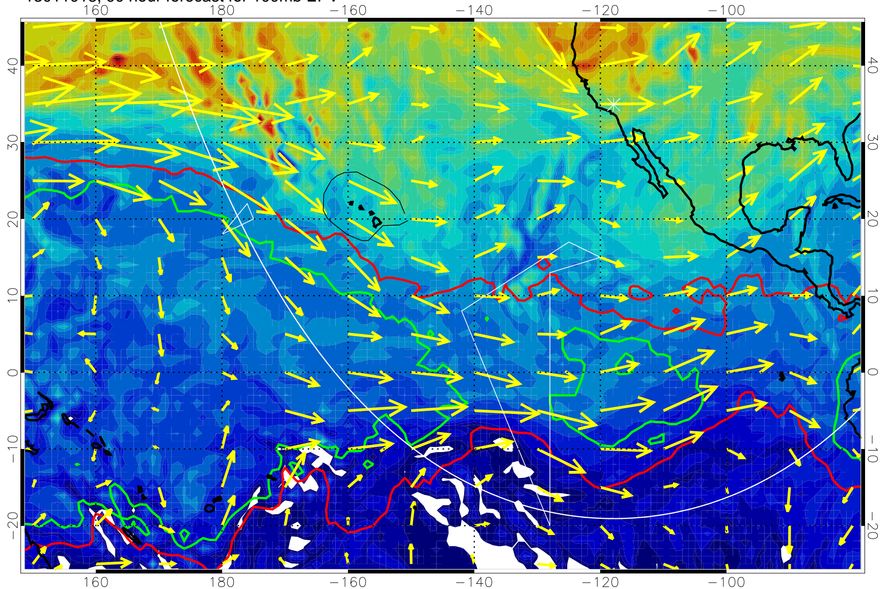
13011018, 90 hour forecast for 100mb EPV
