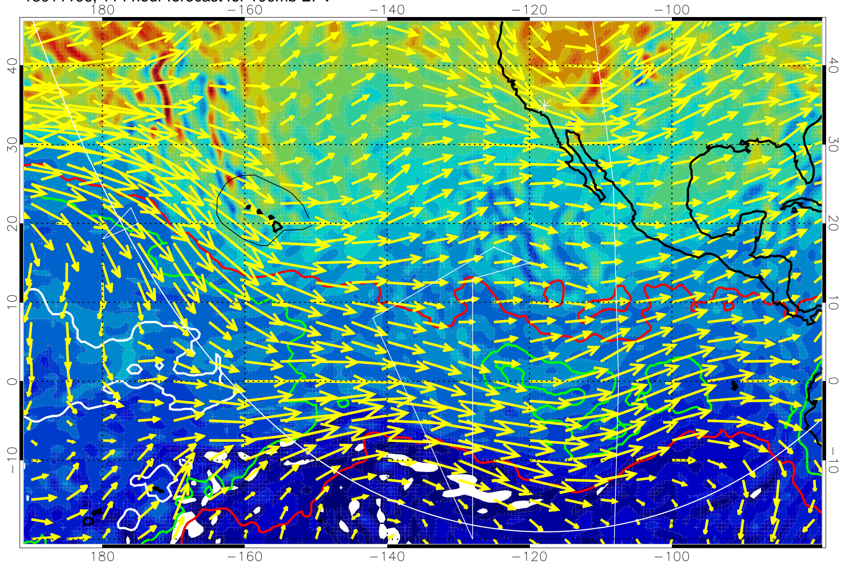
13011106, 114 hour forecast for 100mb EPV
