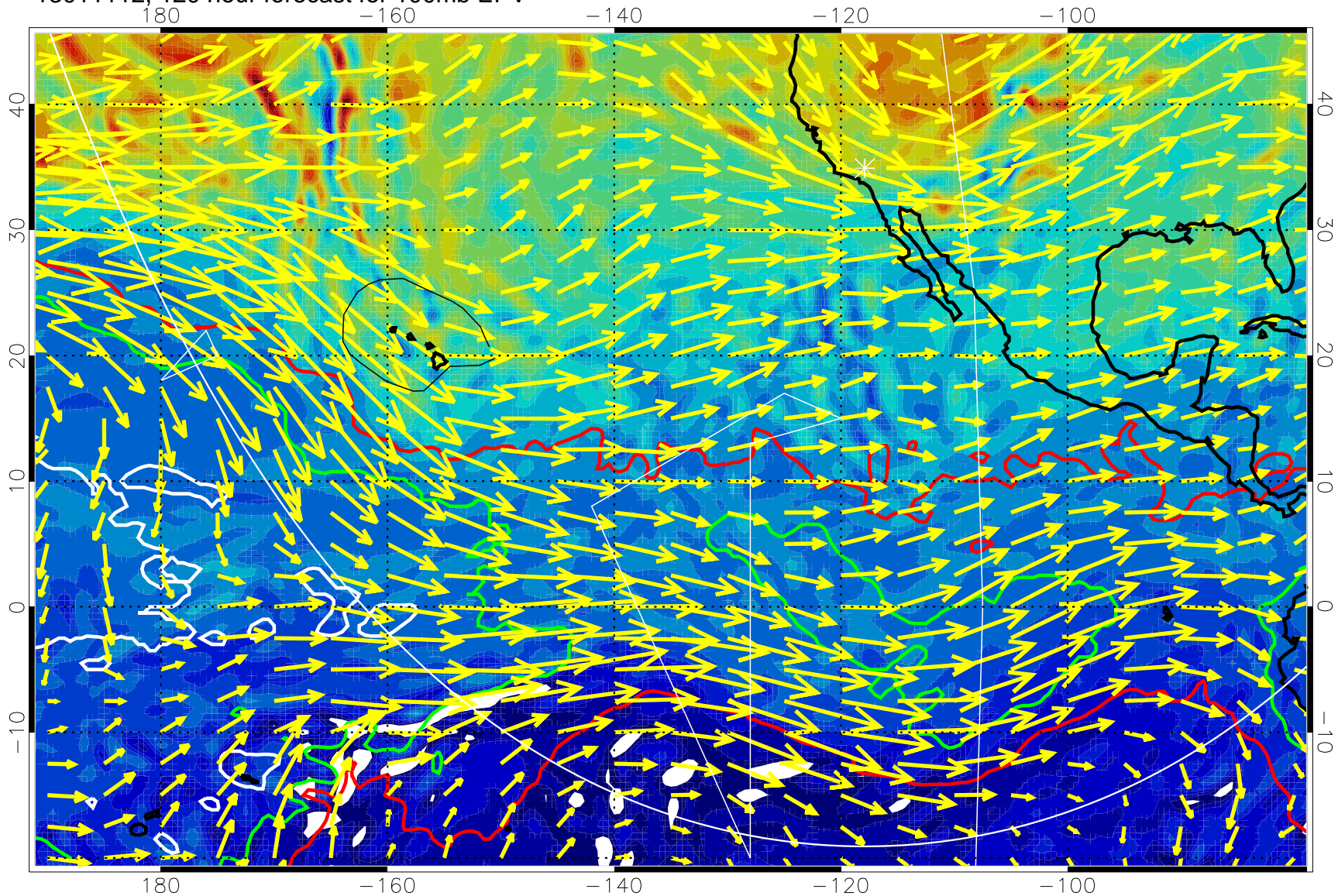
13011112, 120 hour forecast for 100mb EPV
