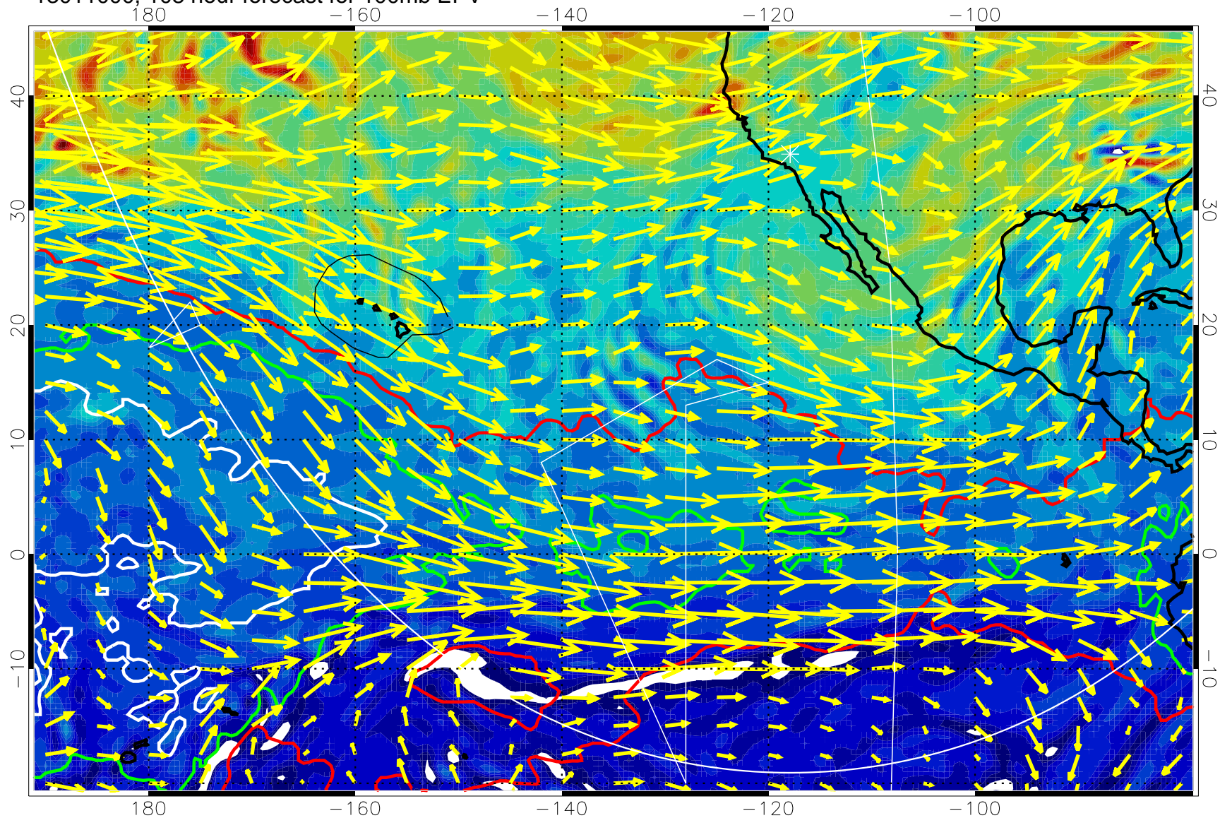
13011000, 108 hour forecast for 100mb EPV
