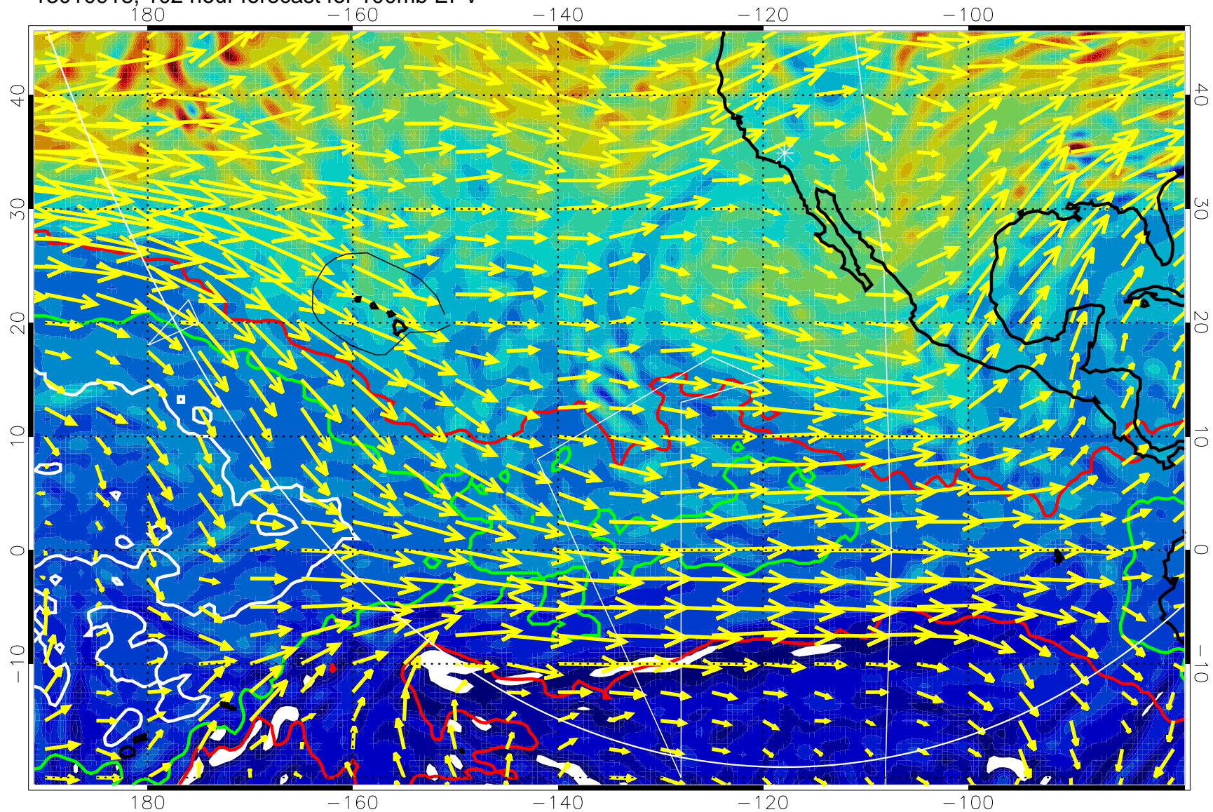
13010918, 102 hour forecast for 100mb EPV
