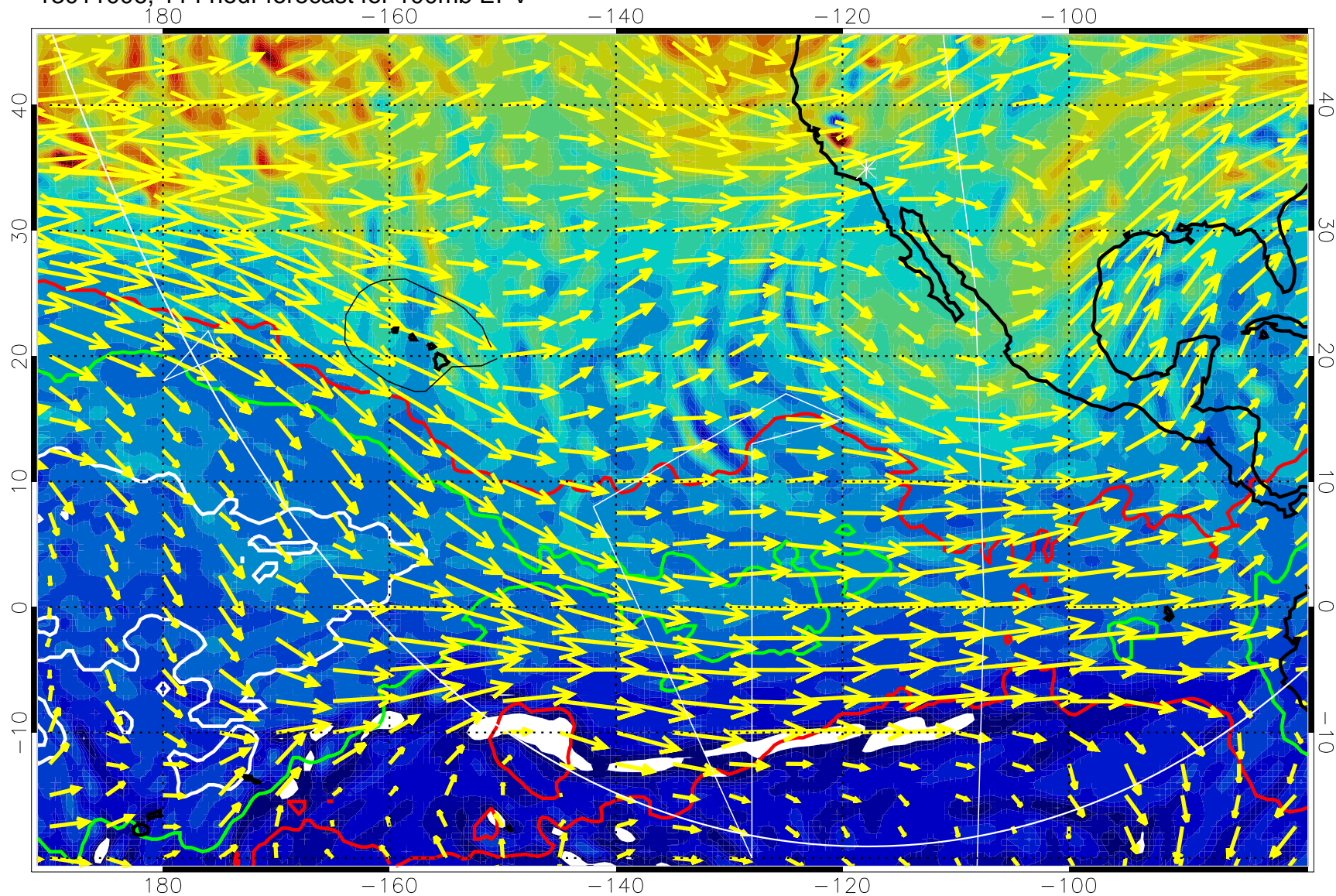
13011006, 114 hour forecast for 100mb EPV
