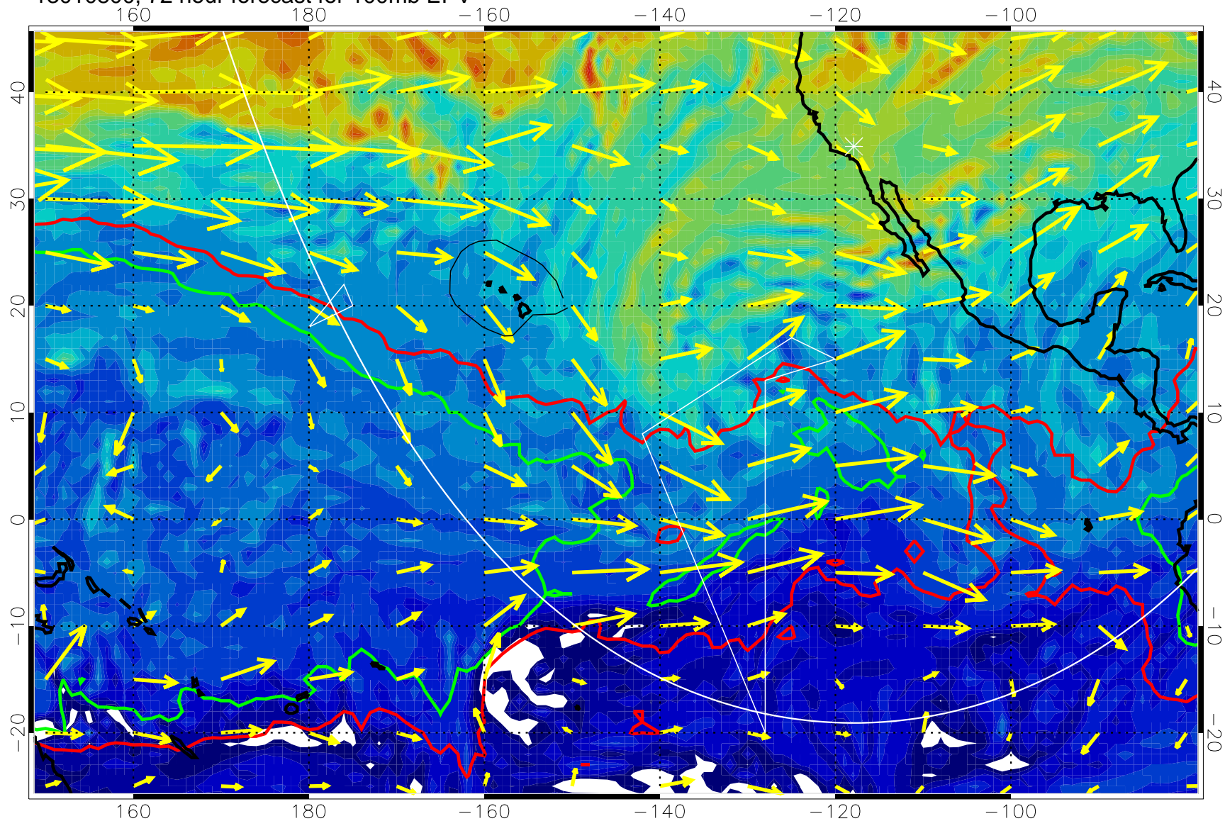
13010800, 72 hour forecast for 100mb EPV
