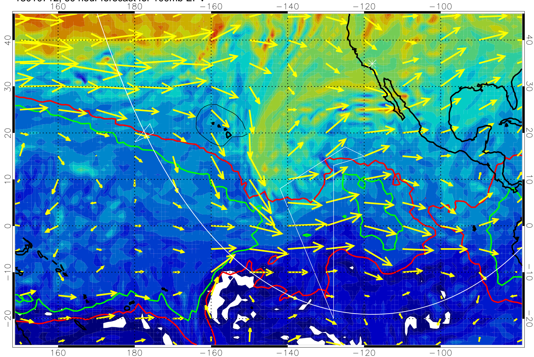
13010712, 60 hour forecast for 100mb EPV
