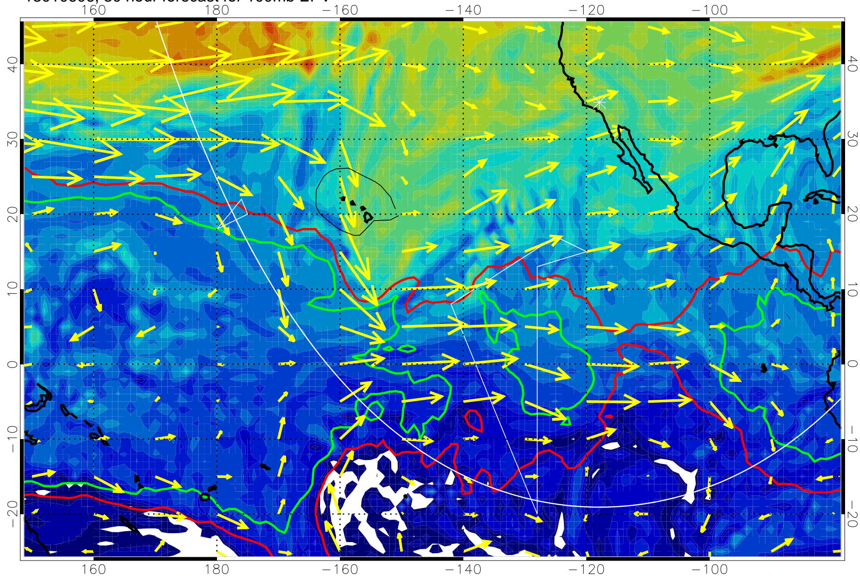
13010606, 30 hour forecast for 100mb EPV
