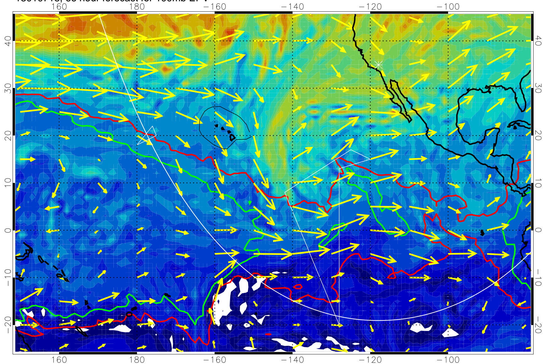
13010718, 66 hour forecast for 100mb EPV
