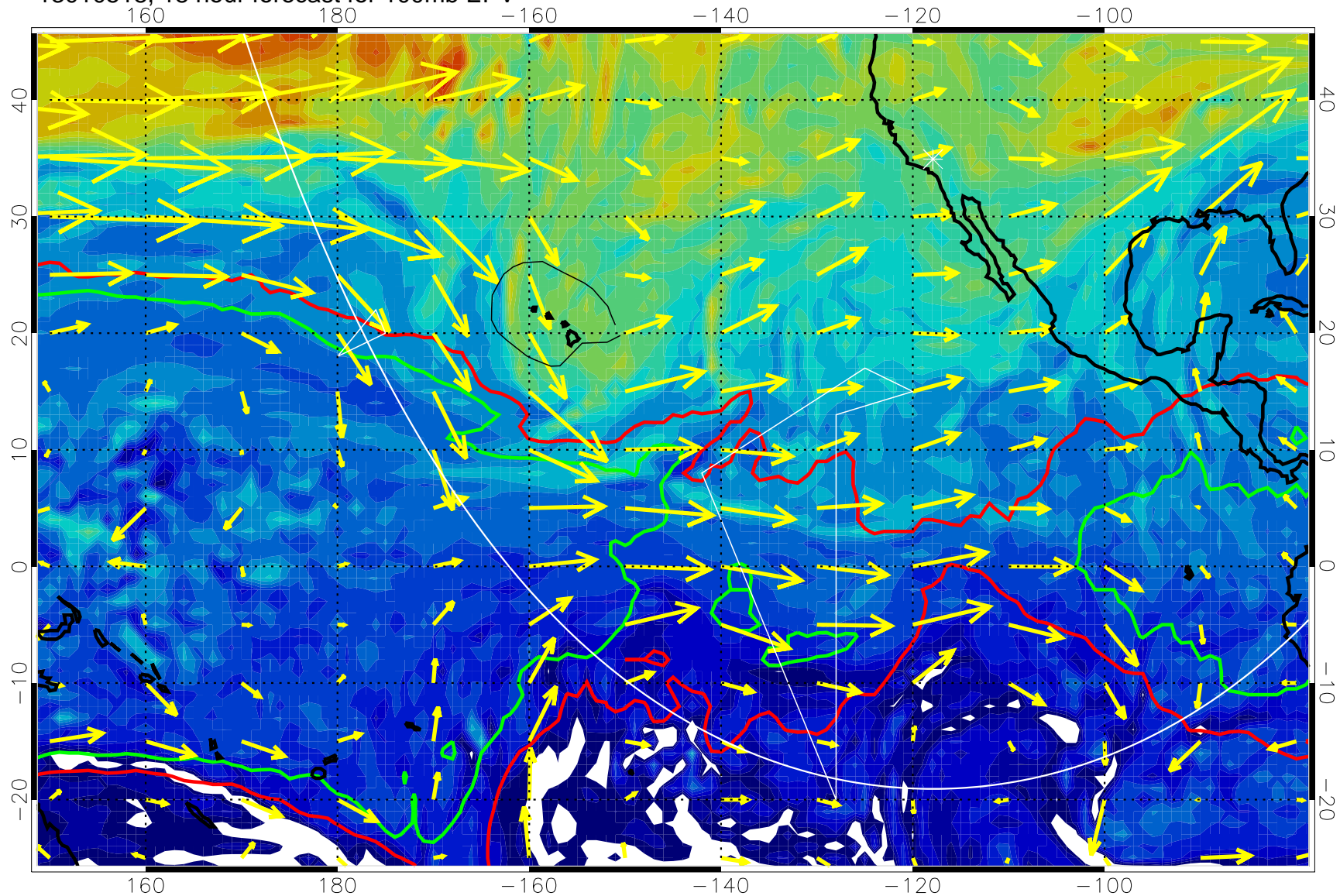
13010518, 18 hour forecast for 100mb EPV
