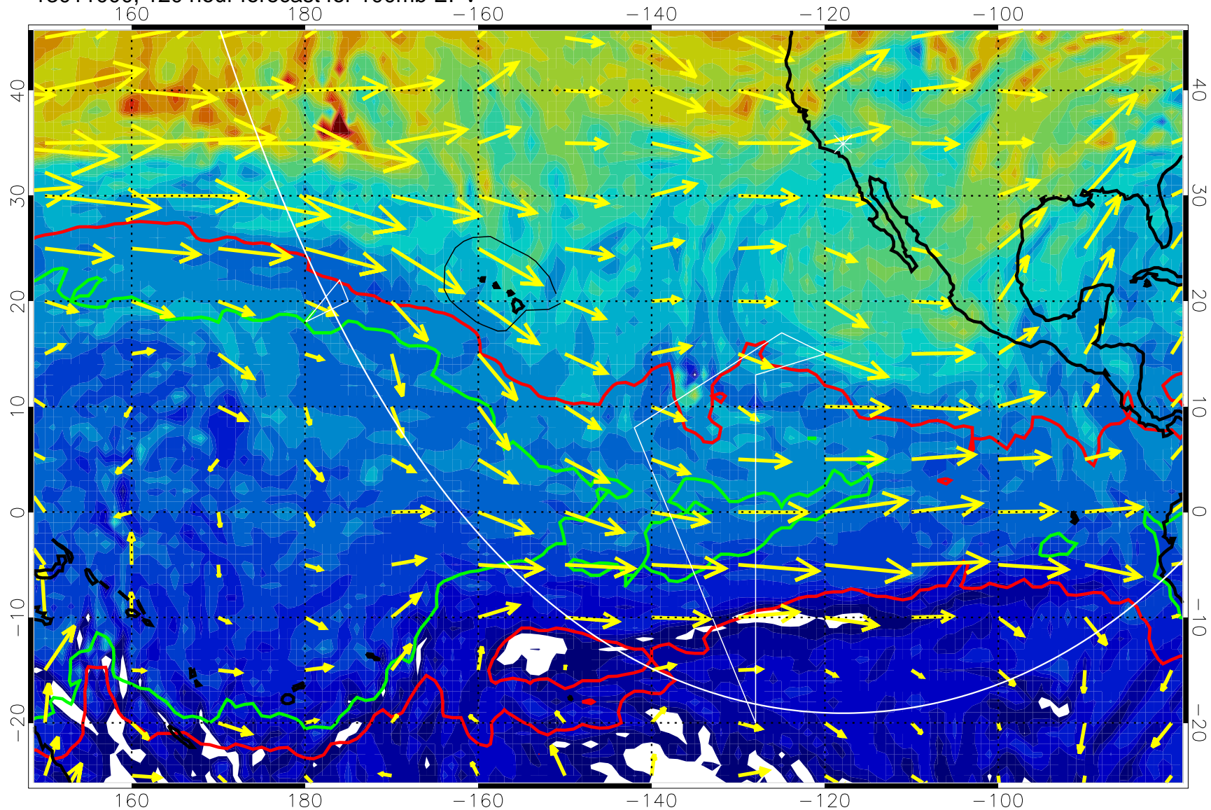
13011000, 120 hour forecast for 100mb EPV
