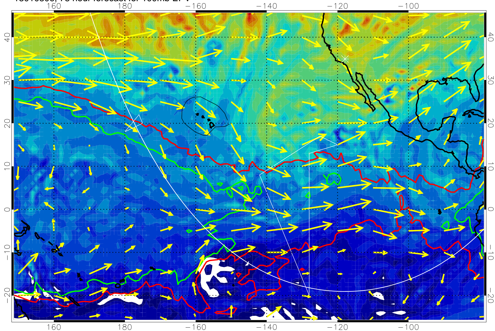
13010806, 78 hour forecast for 100mb EPV
