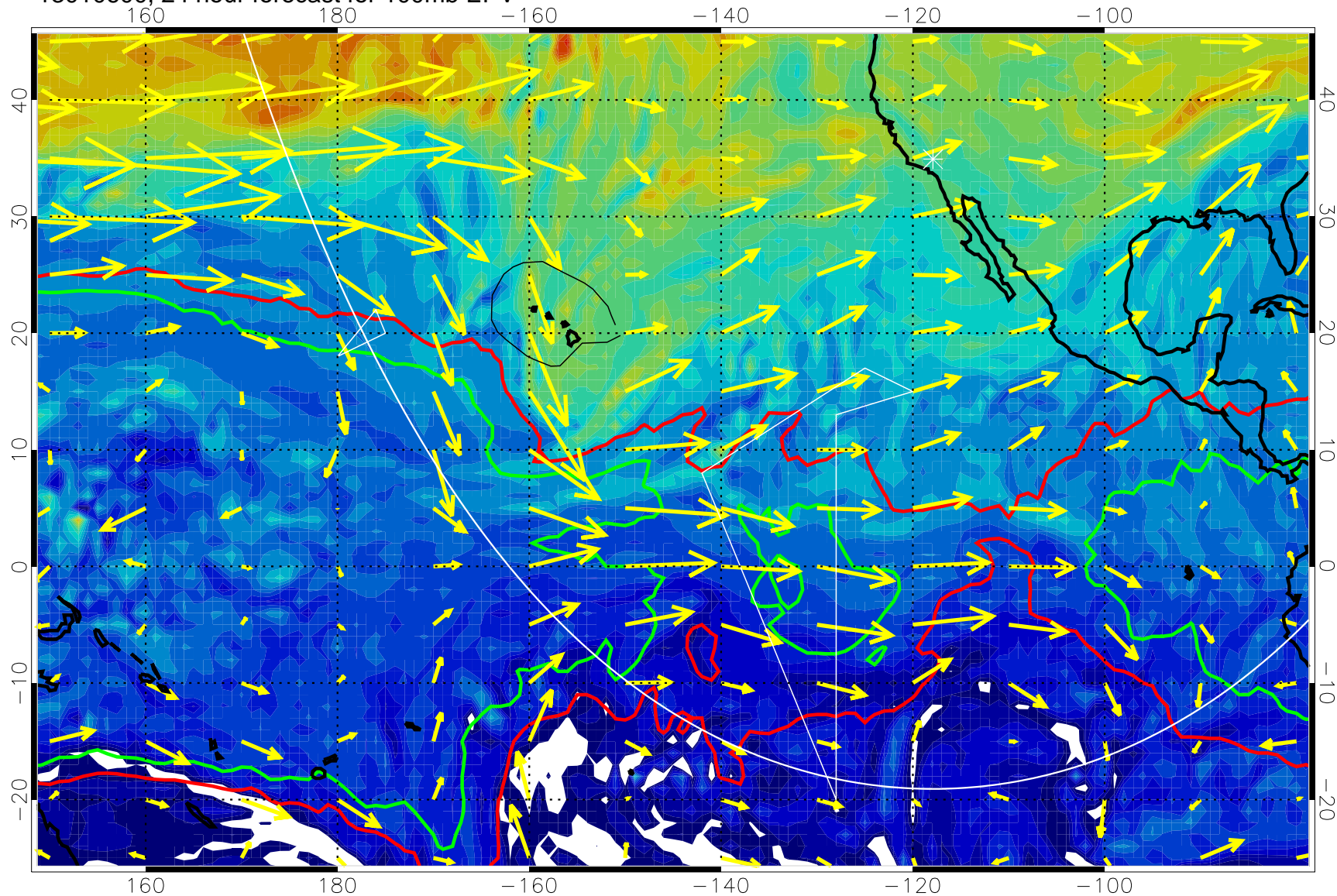
13010600, 24 hour forecast for 100mb EPV
