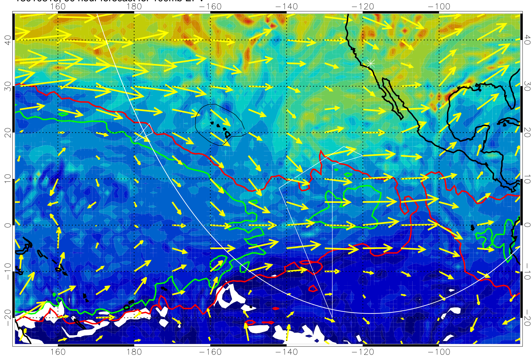
13010818, 90 hour forecast for 100mb EPV
