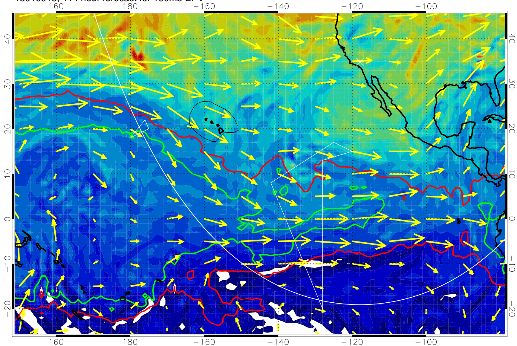
13010918, 114 hour forecast for 100mb EPV
