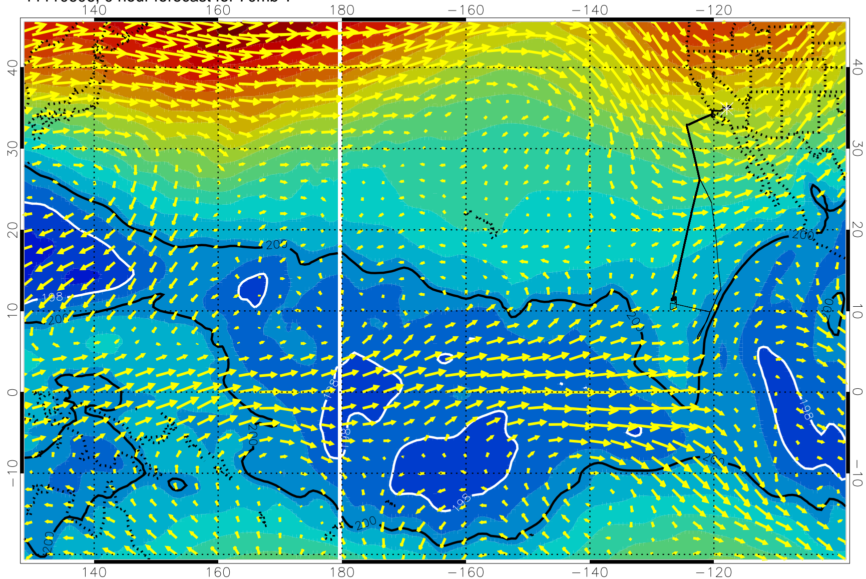
11110606, 0 hour forecast for 70mb T
