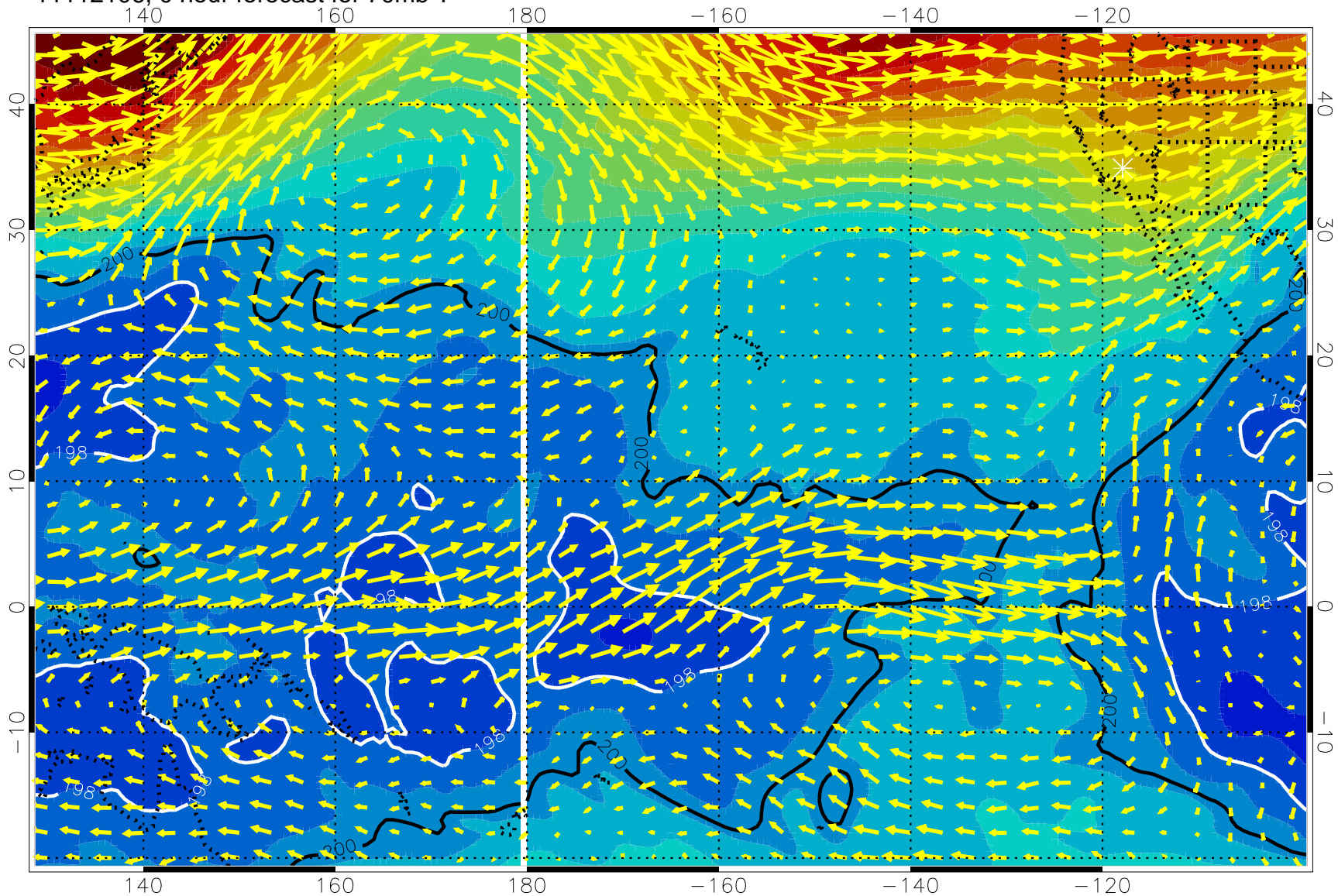
11112106, 0 hour forecast for 70mb T
