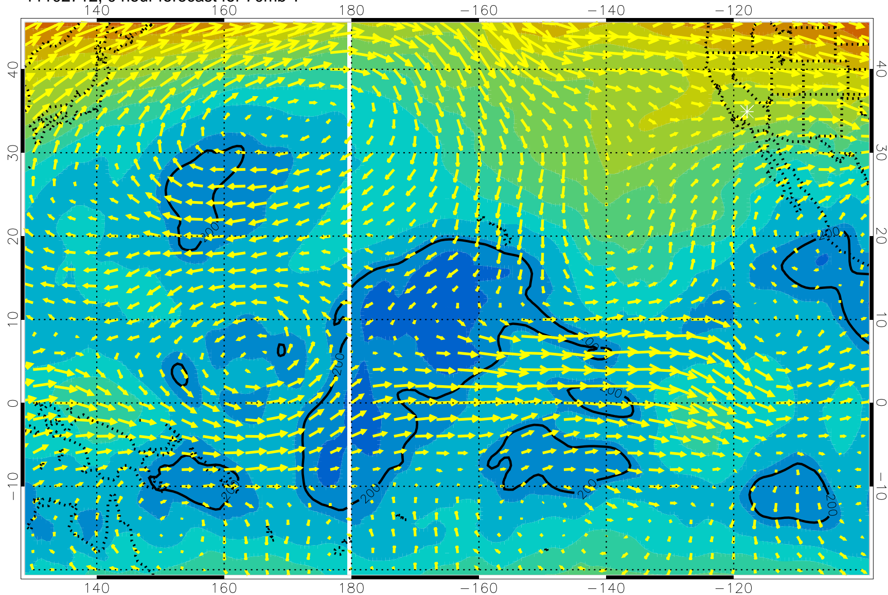
11102712, 0 hour forecast for 70mb T
