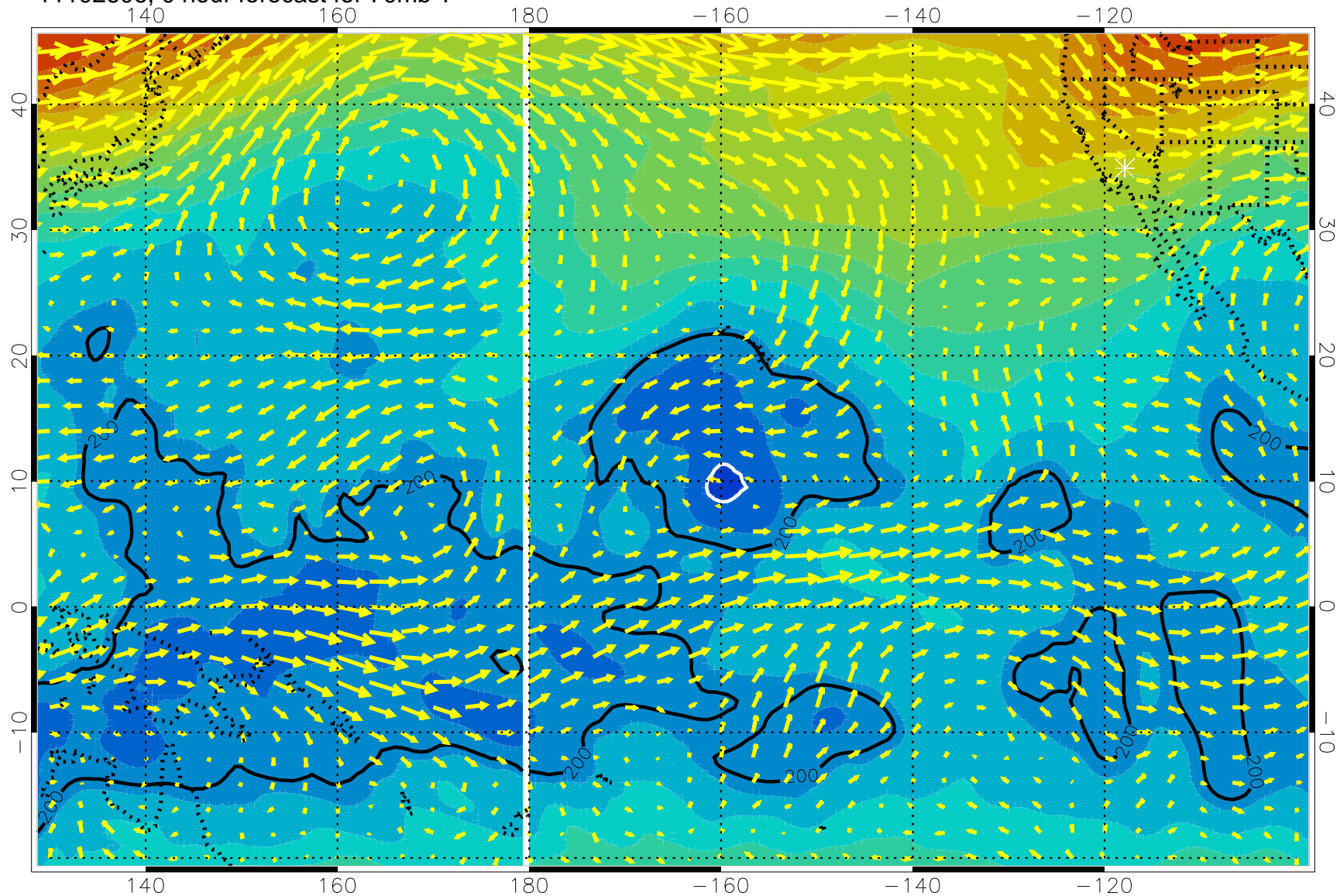
11102606, 0 hour forecast for 70mb T
