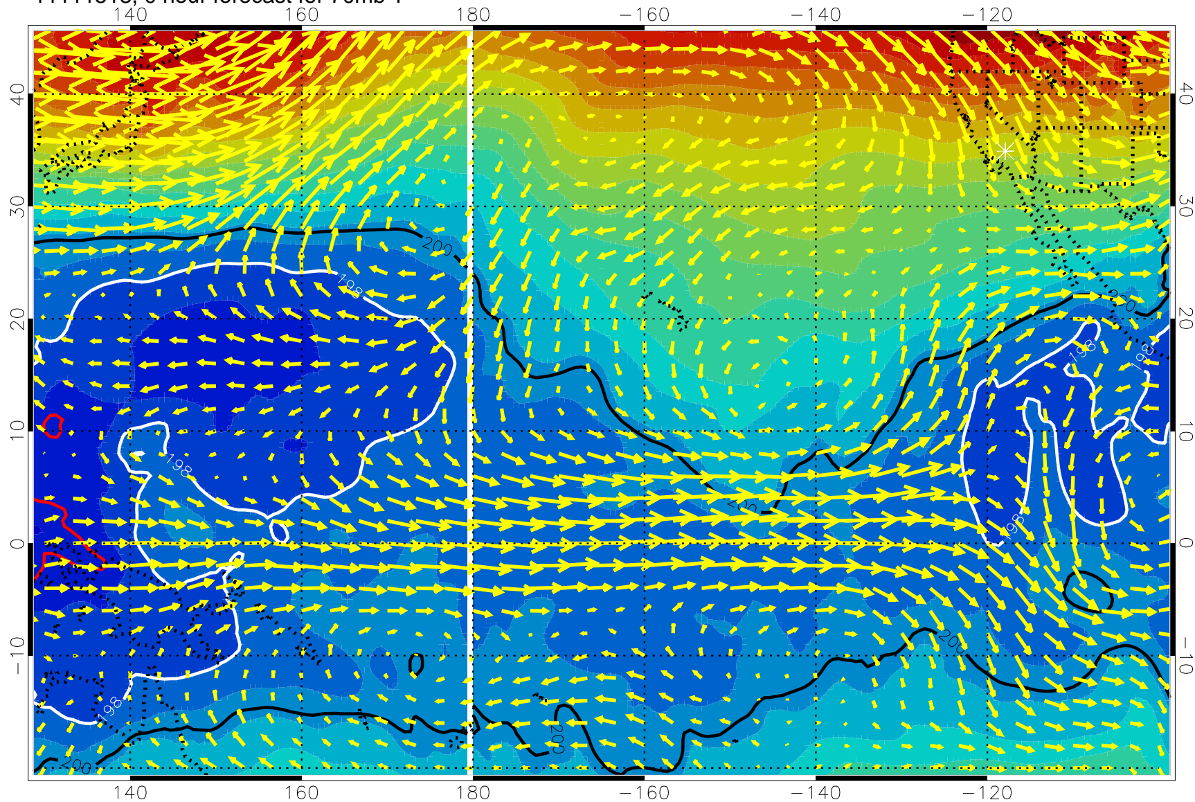
11111518, 0 hour forecast for 70mb T
