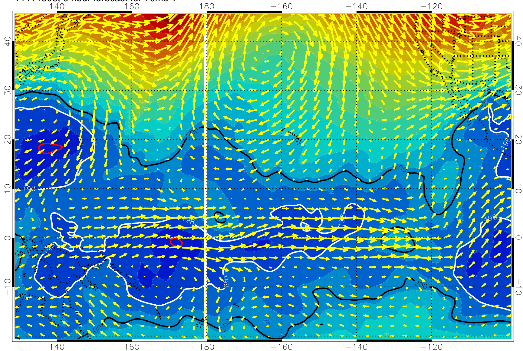
11111906, 0 hour forecast for 70mb T
