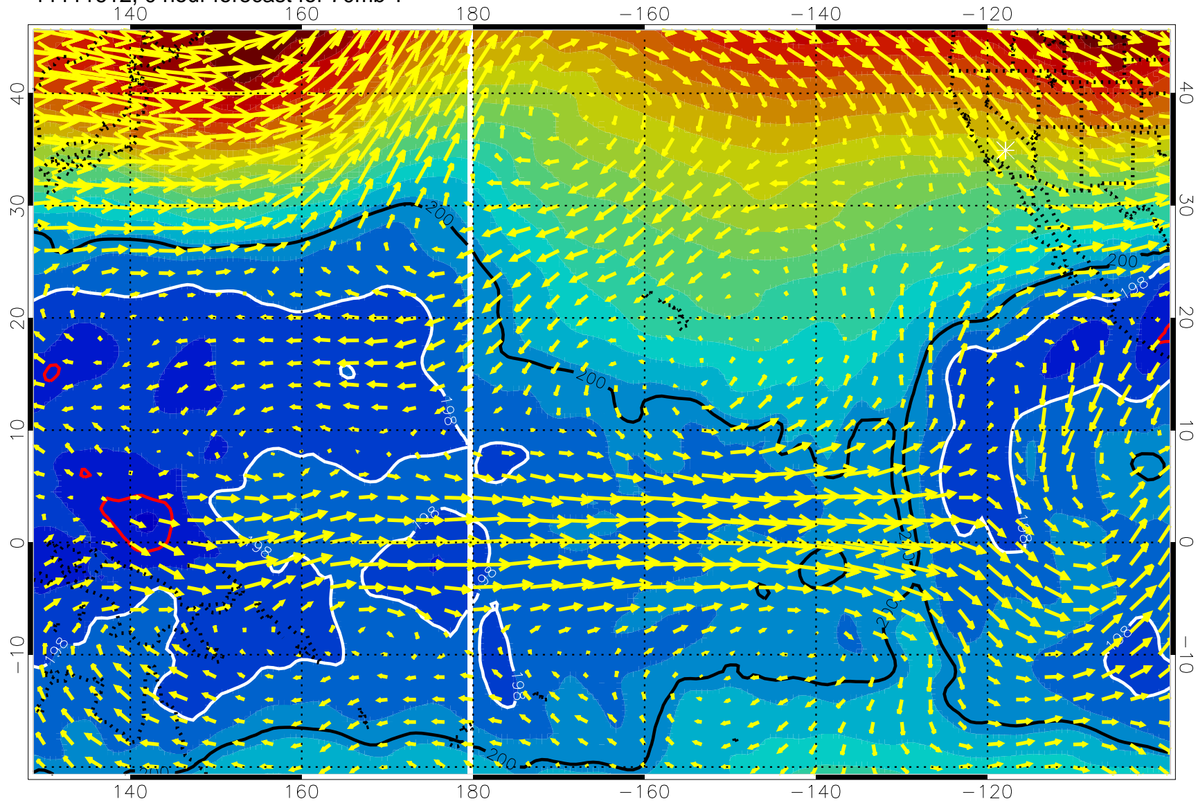
11111612, 0 hour forecast for 70mb T
