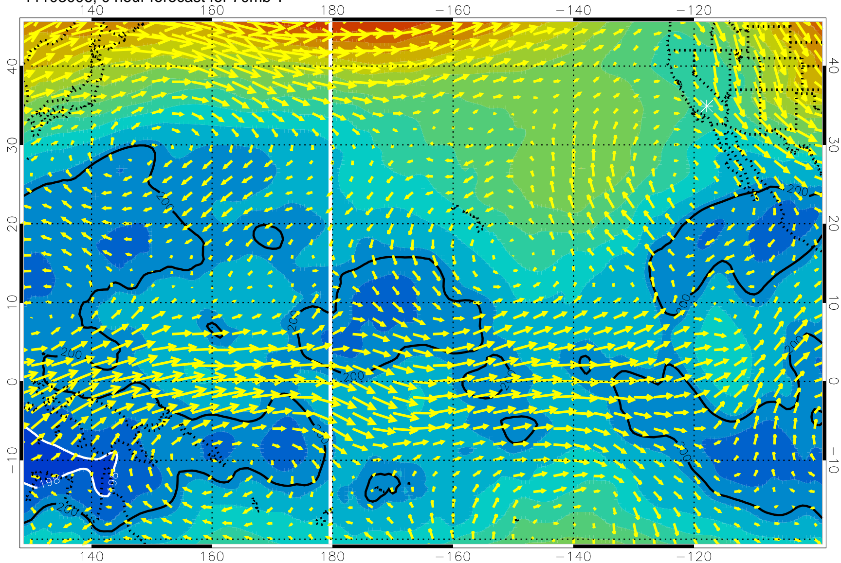
11103006, 0 hour forecast for 70mb T
