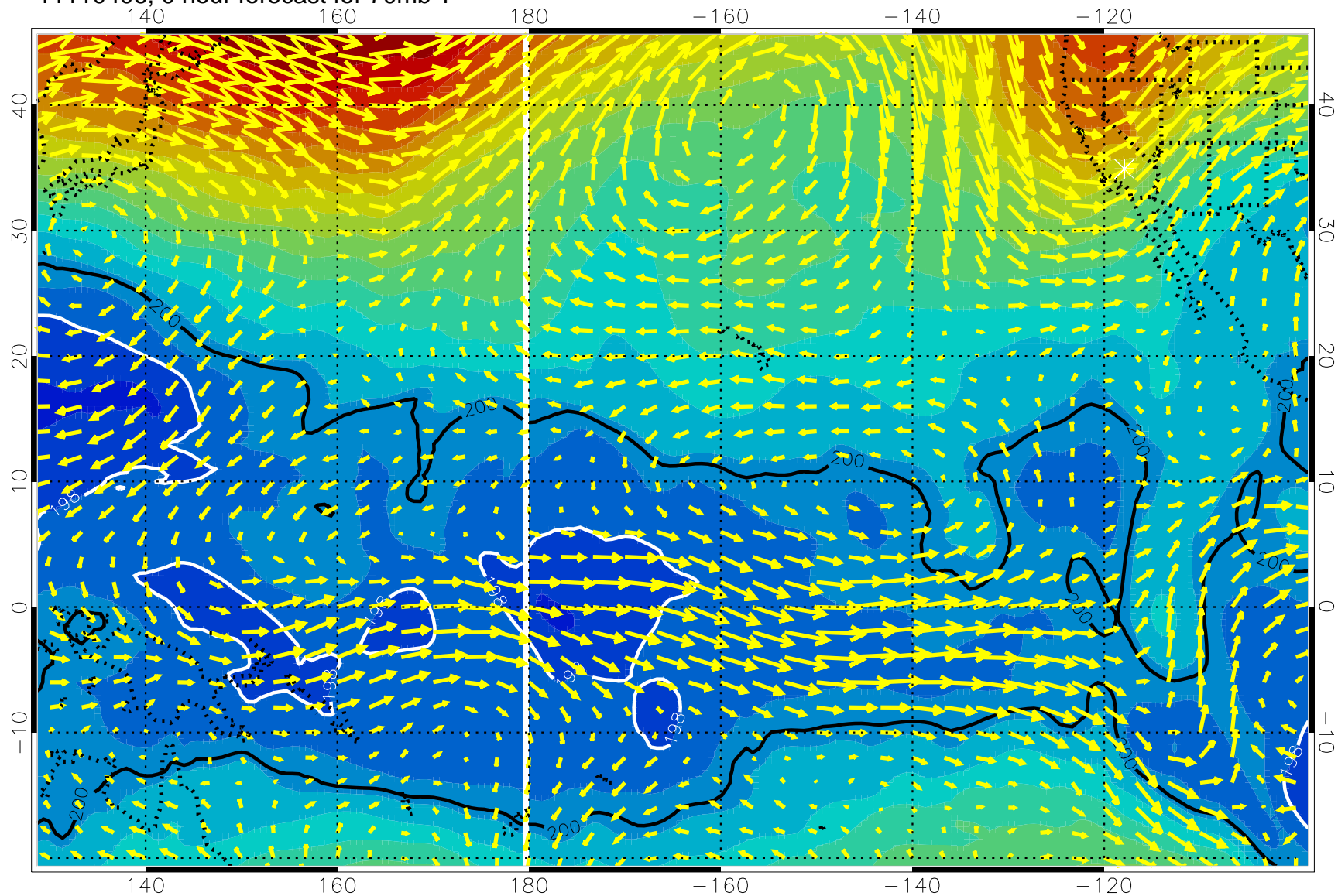
11110406, 0 hour forecast for 70mb T
