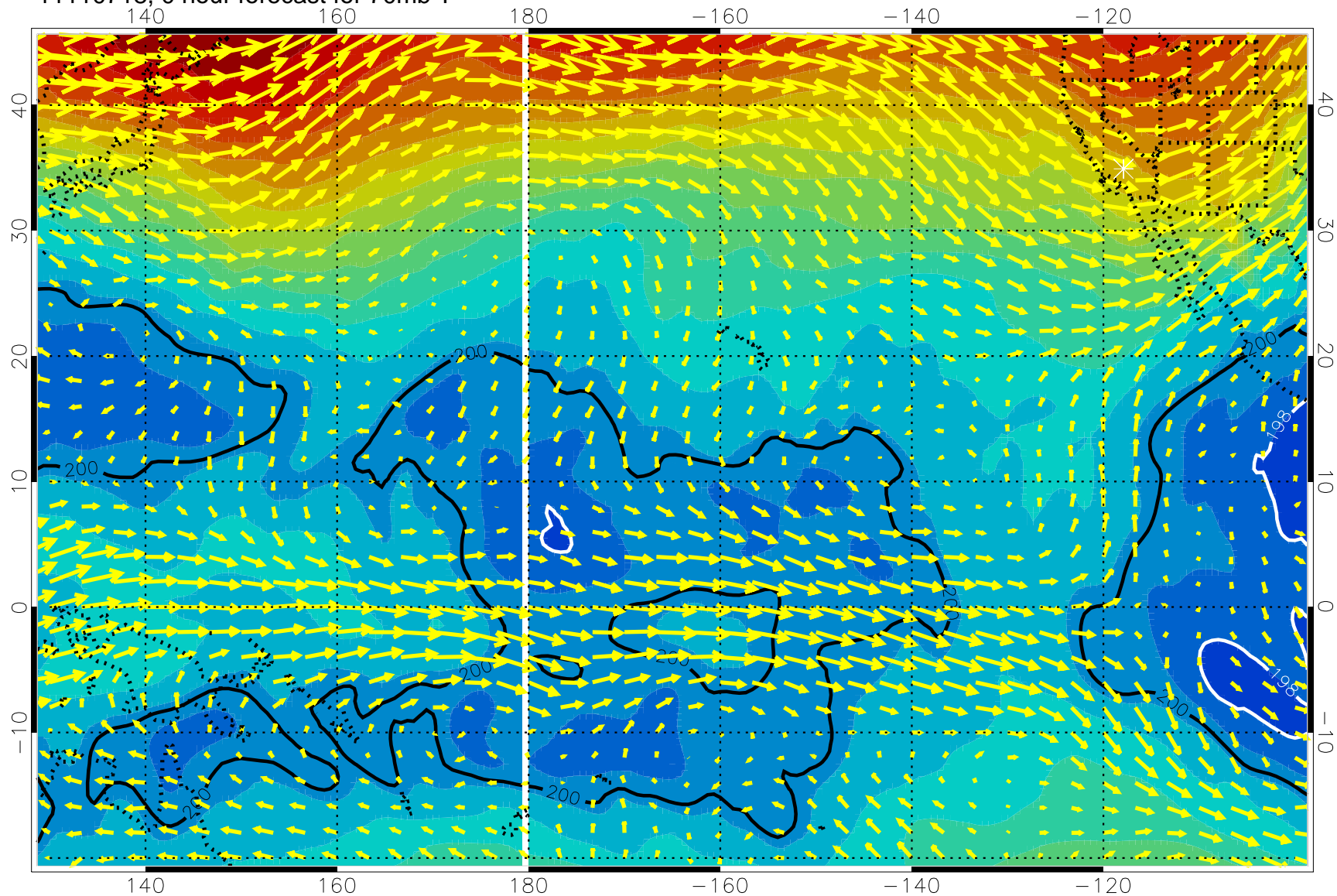
11110718, 0 hour forecast for 70mb T
