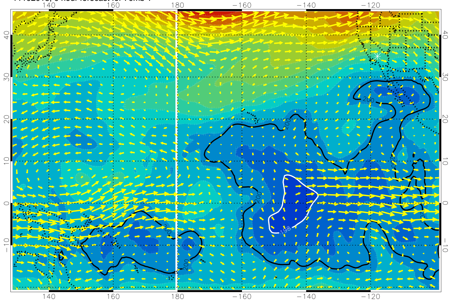
11102018, 0 hour forecast for 70mb T
