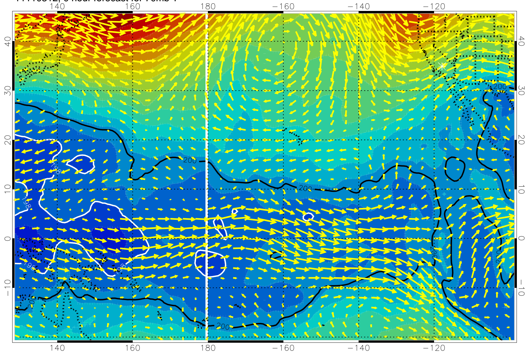
11110312, 0 hour forecast for 70mb T
