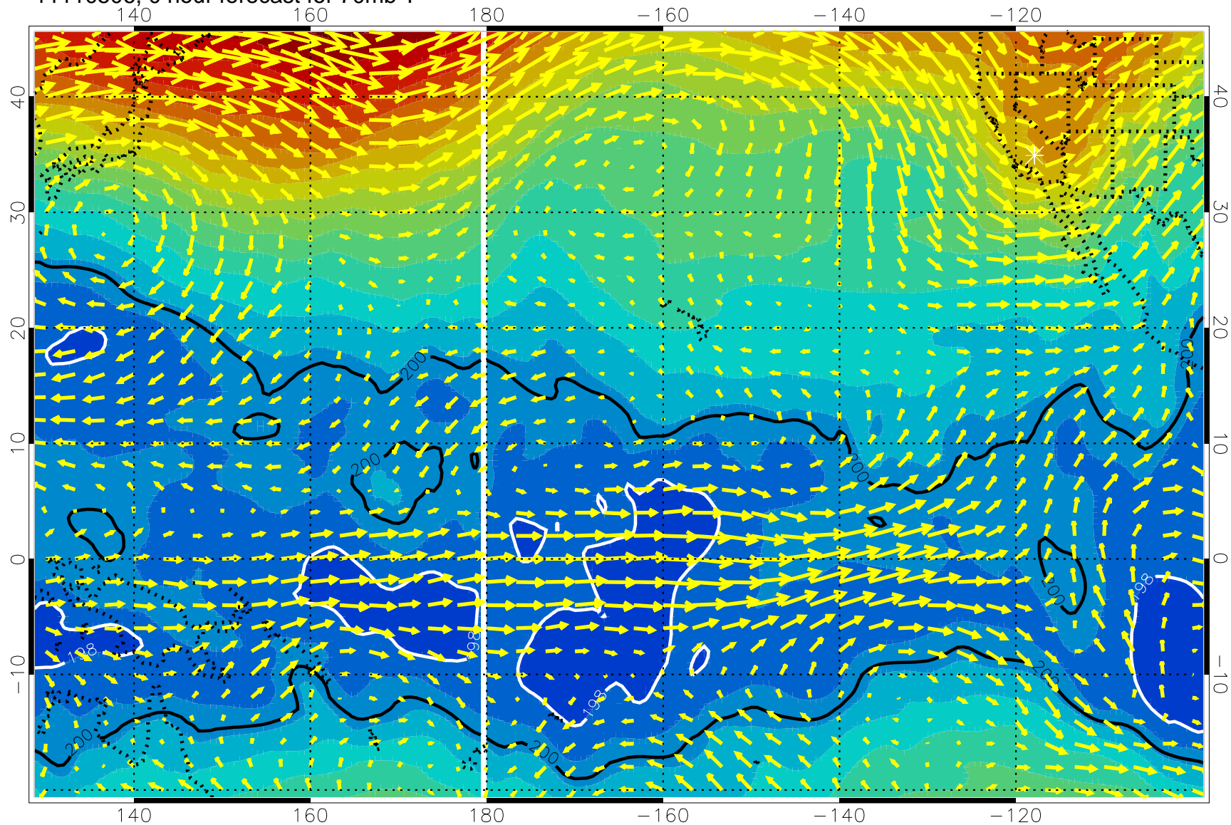
11110506, 0 hour forecast for 70mb T
