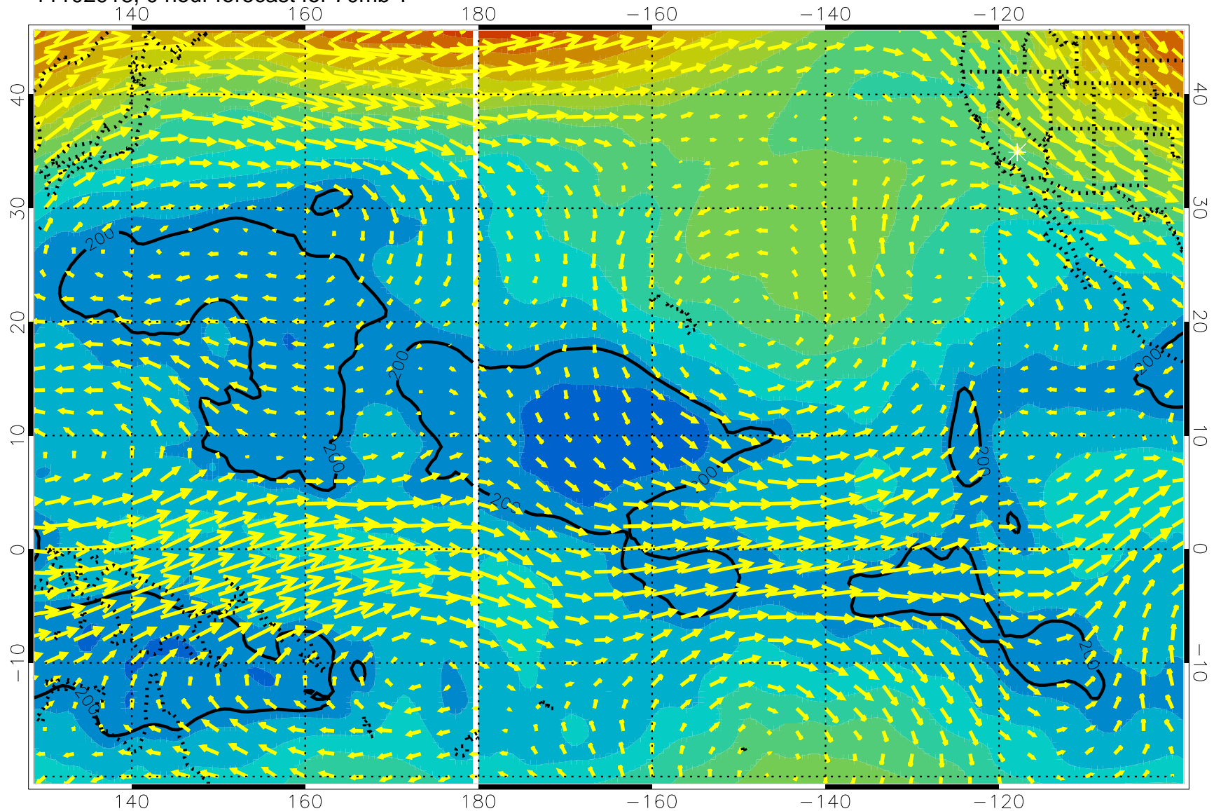
11102918, 0 hour forecast for 70mb T
