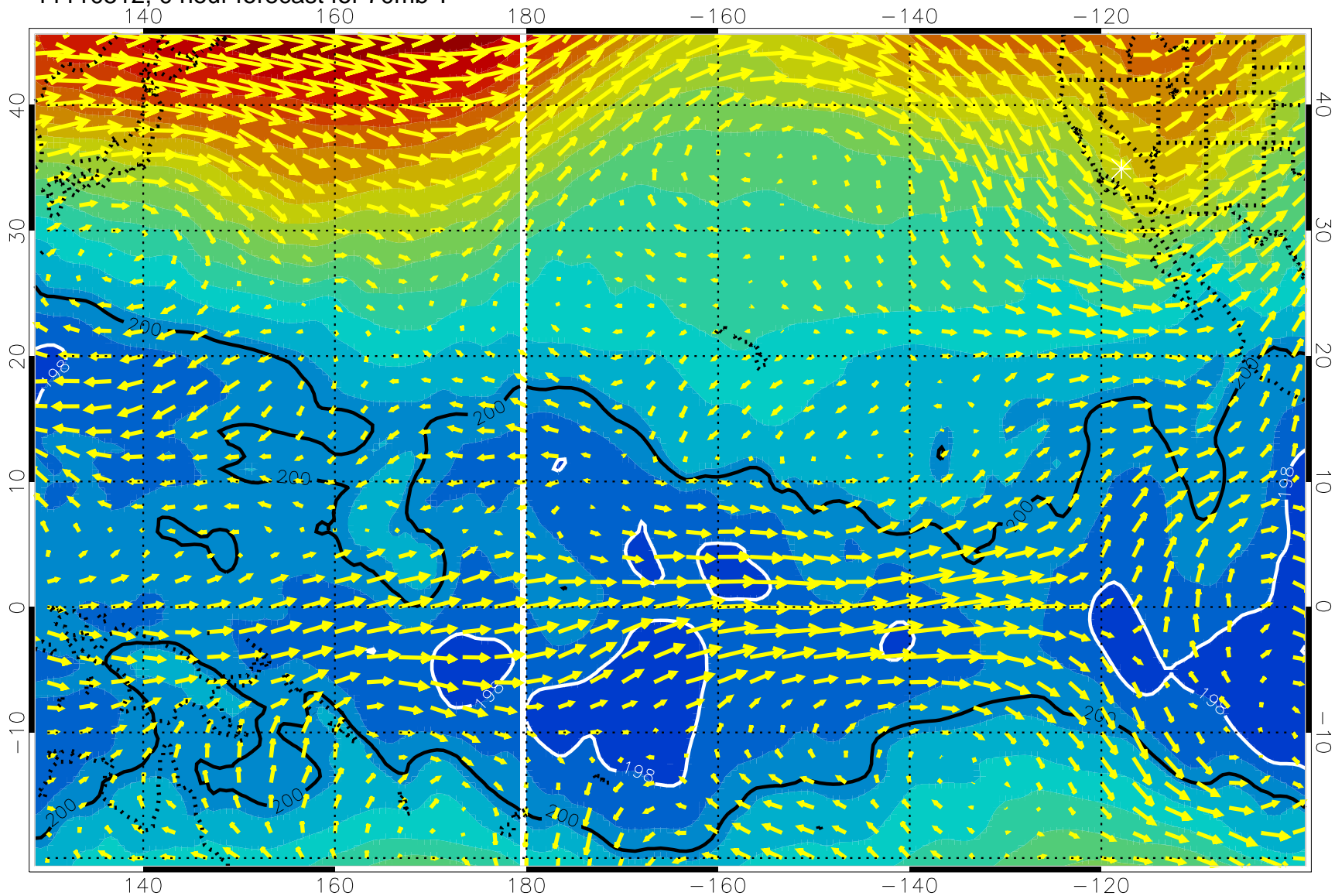
11110512, 0 hour forecast for 70mb T
