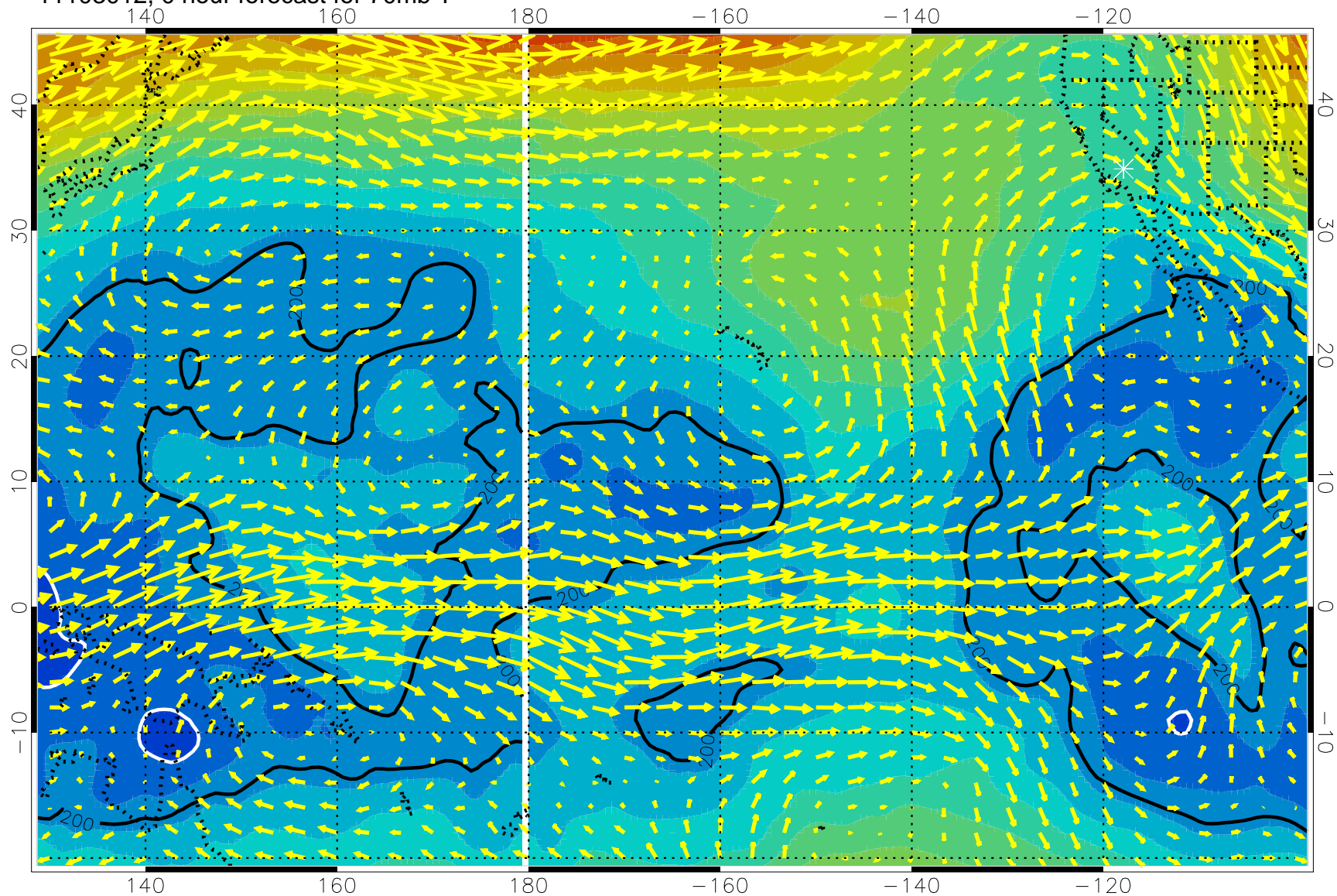
11103012, 0 hour forecast for 70mb T
