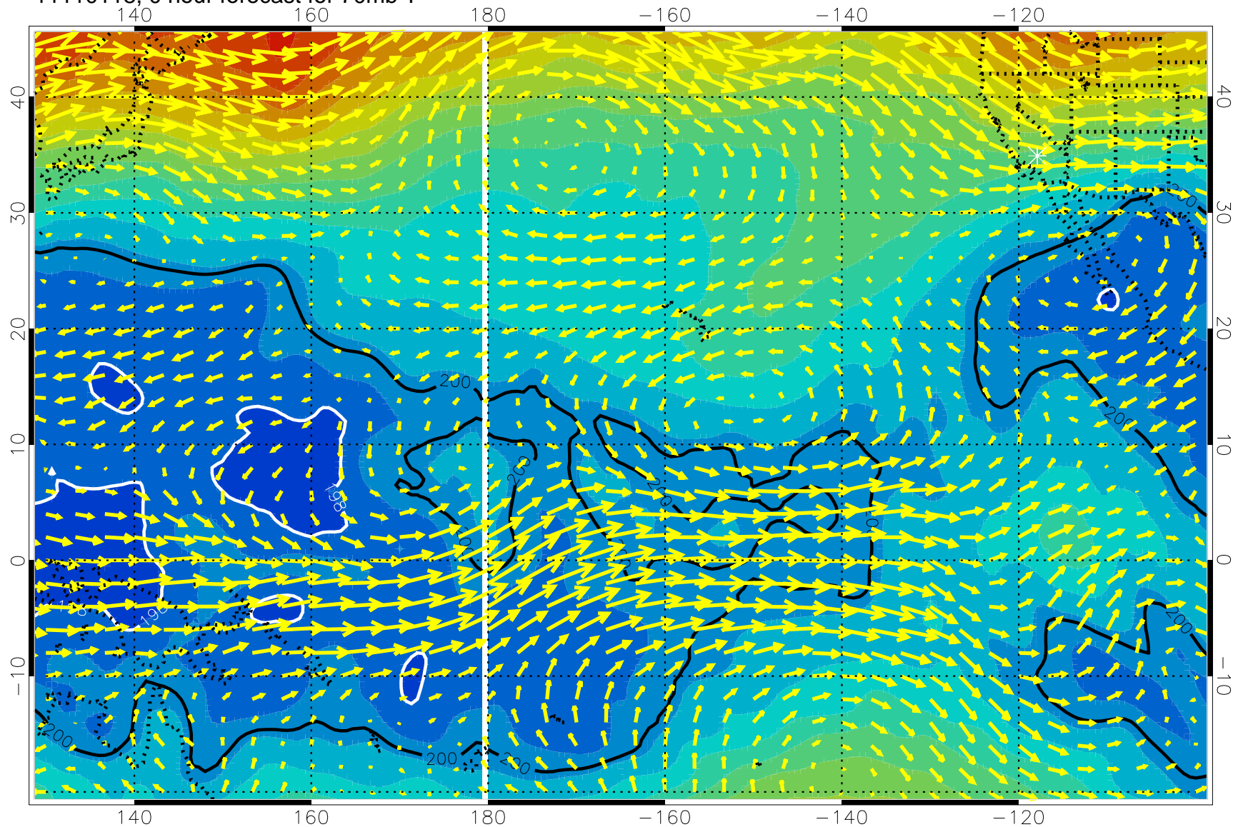
11110118, 0 hour forecast for 70mb T
