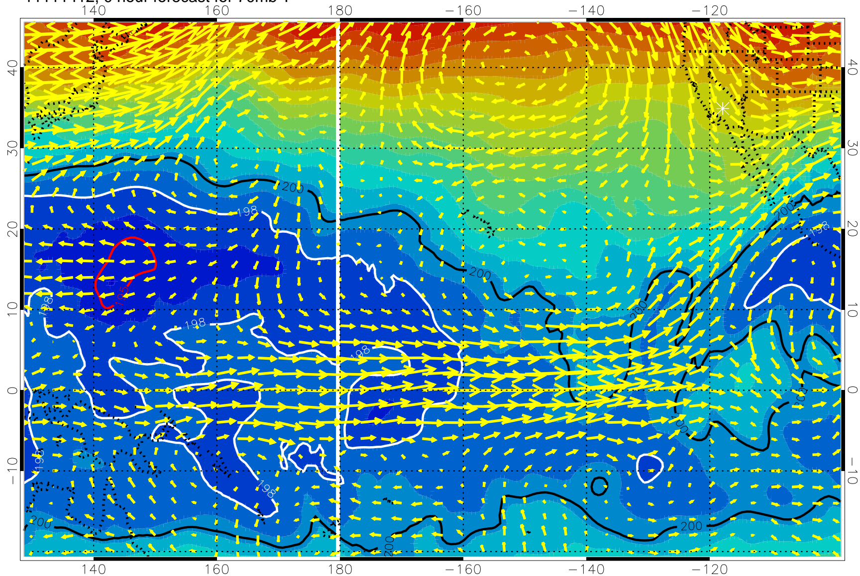
11111412, 0 hour forecast for 70mb T
