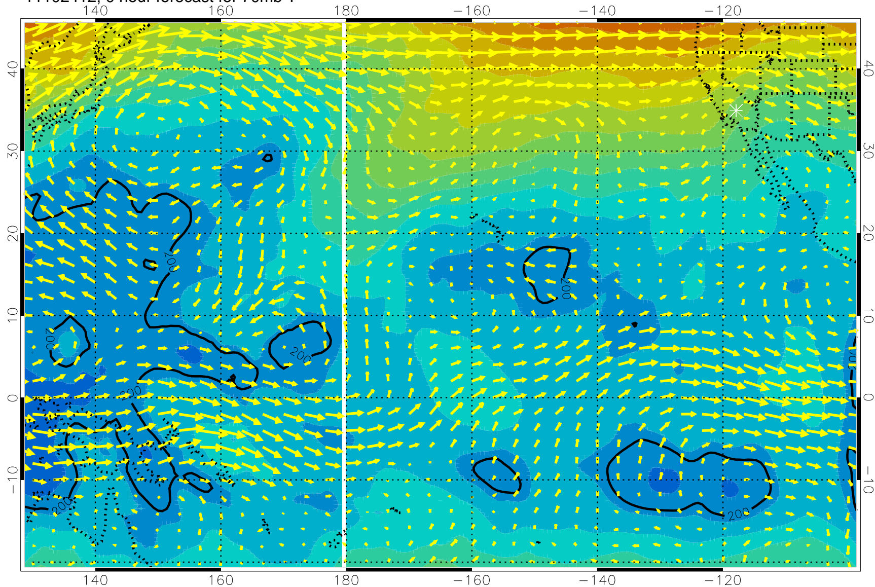
11102412, 0 hour forecast for 70mb T
