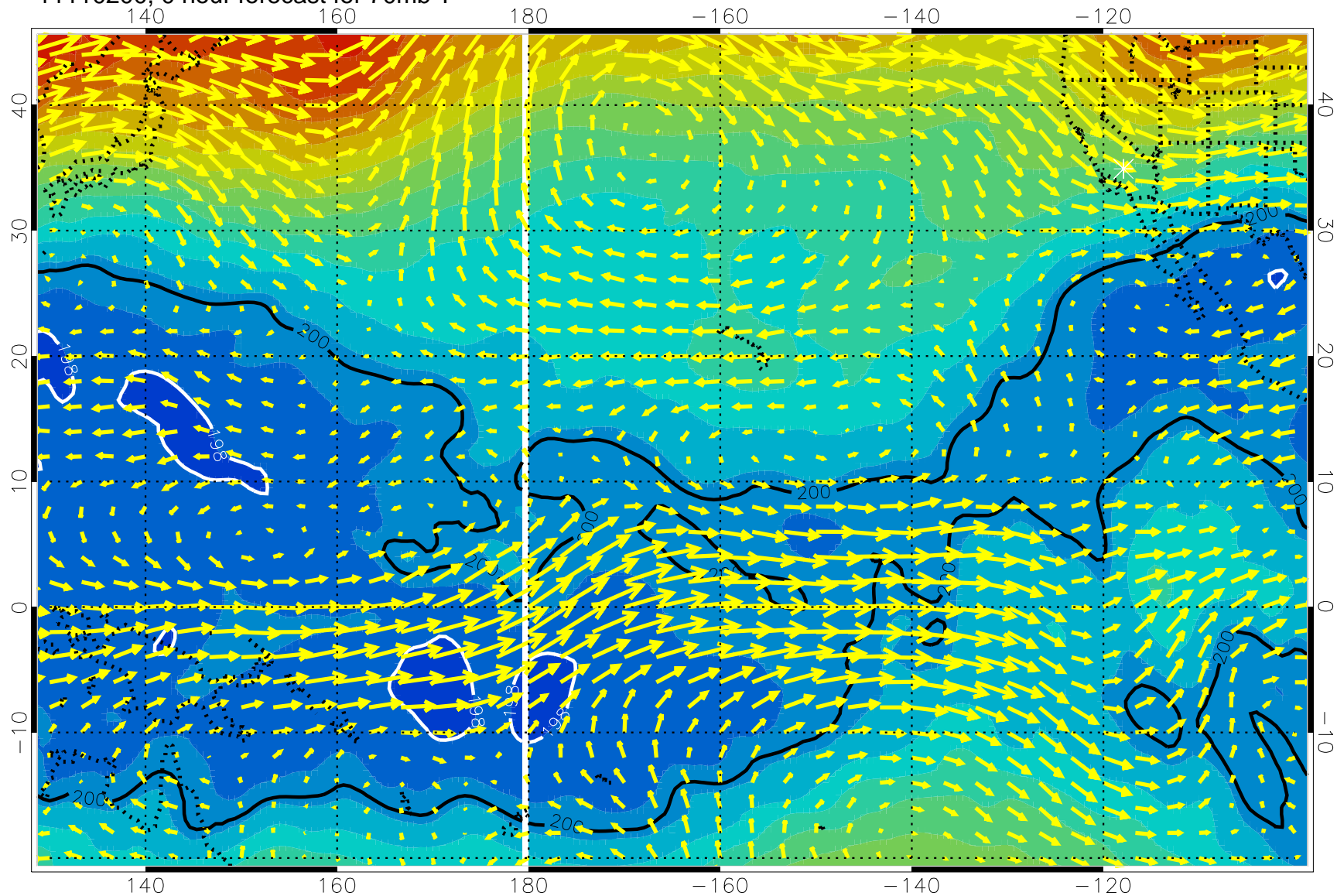
11110200, 0 hour forecast for 70mb T
