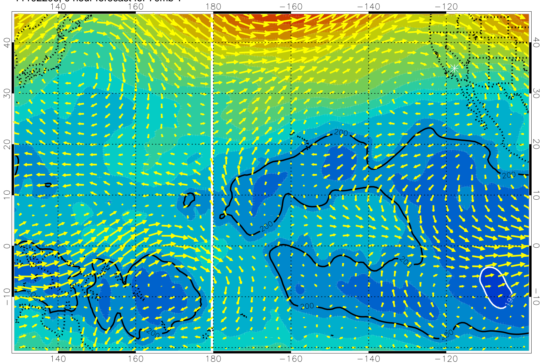
11102206, 0 hour forecast for 70mb T
