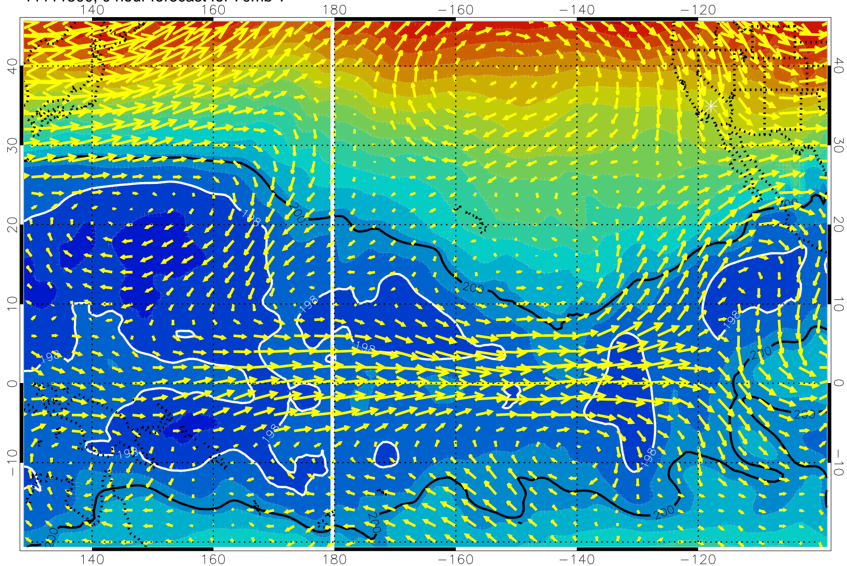
11111500, 0 hour forecast for 70mb T
