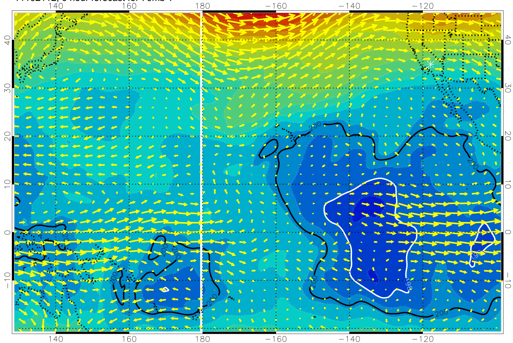
11102112, 0 hour forecast for 70mb T
