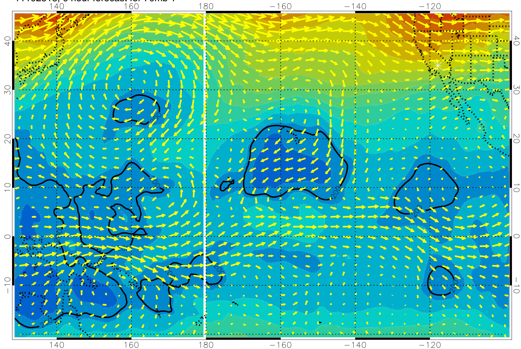
11102518, 0 hour forecast for 70mb T
