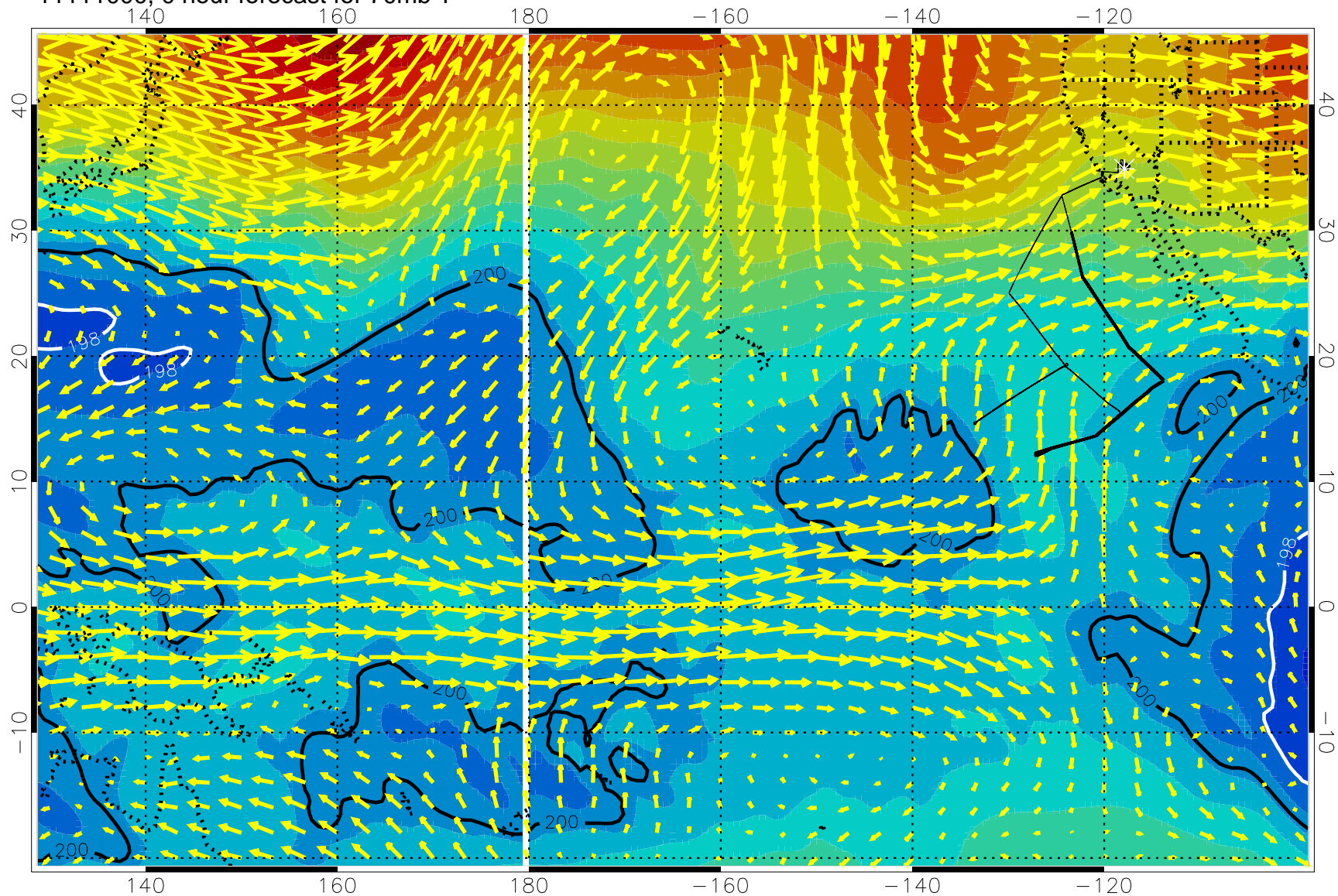
11111000, 0 hour forecast for 70mb T
