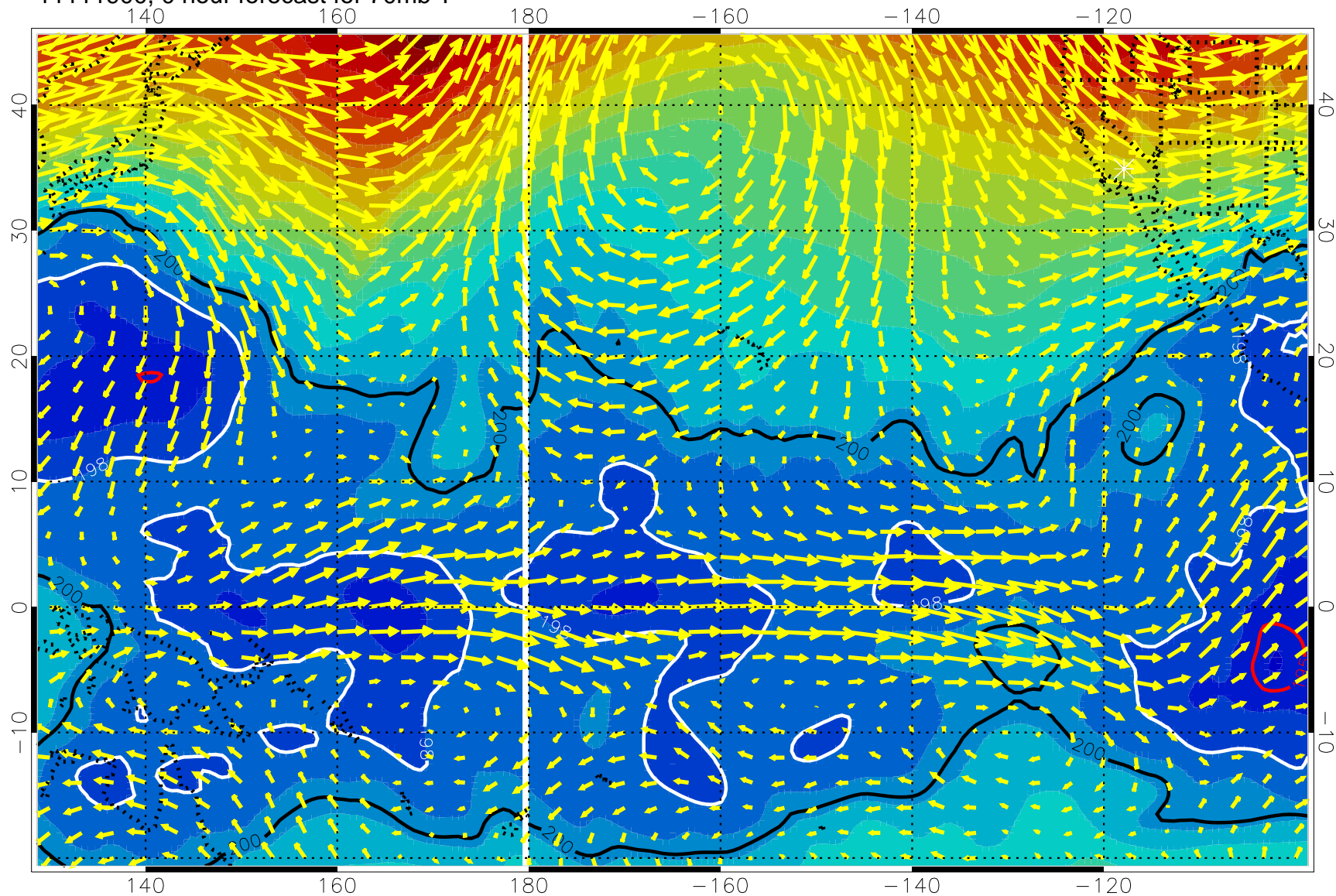
11111900, 0 hour forecast for 70mb T
