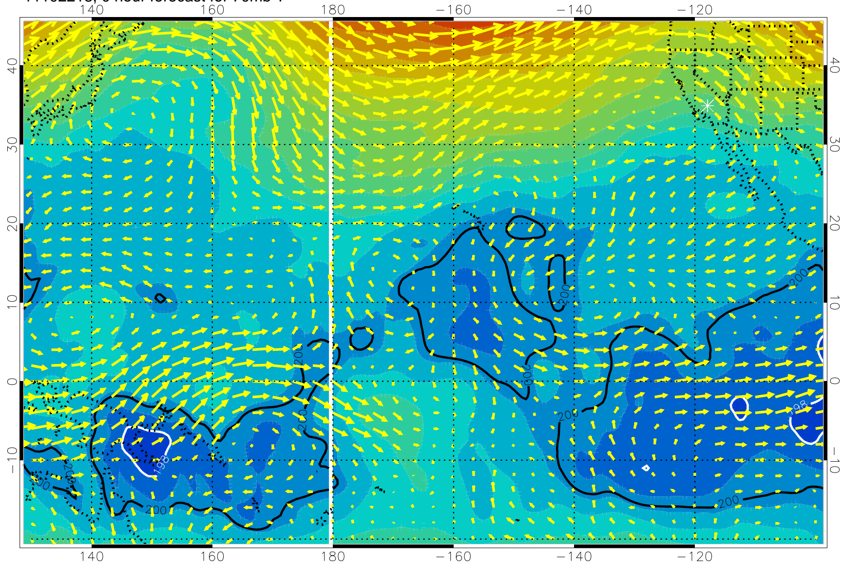
11102218, 0 hour forecast for 70mb T
