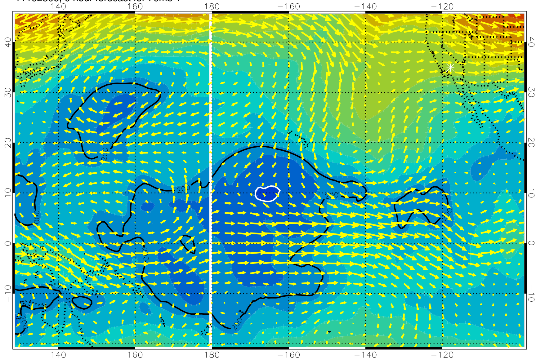
11102806, 0 hour forecast for 70mb T
