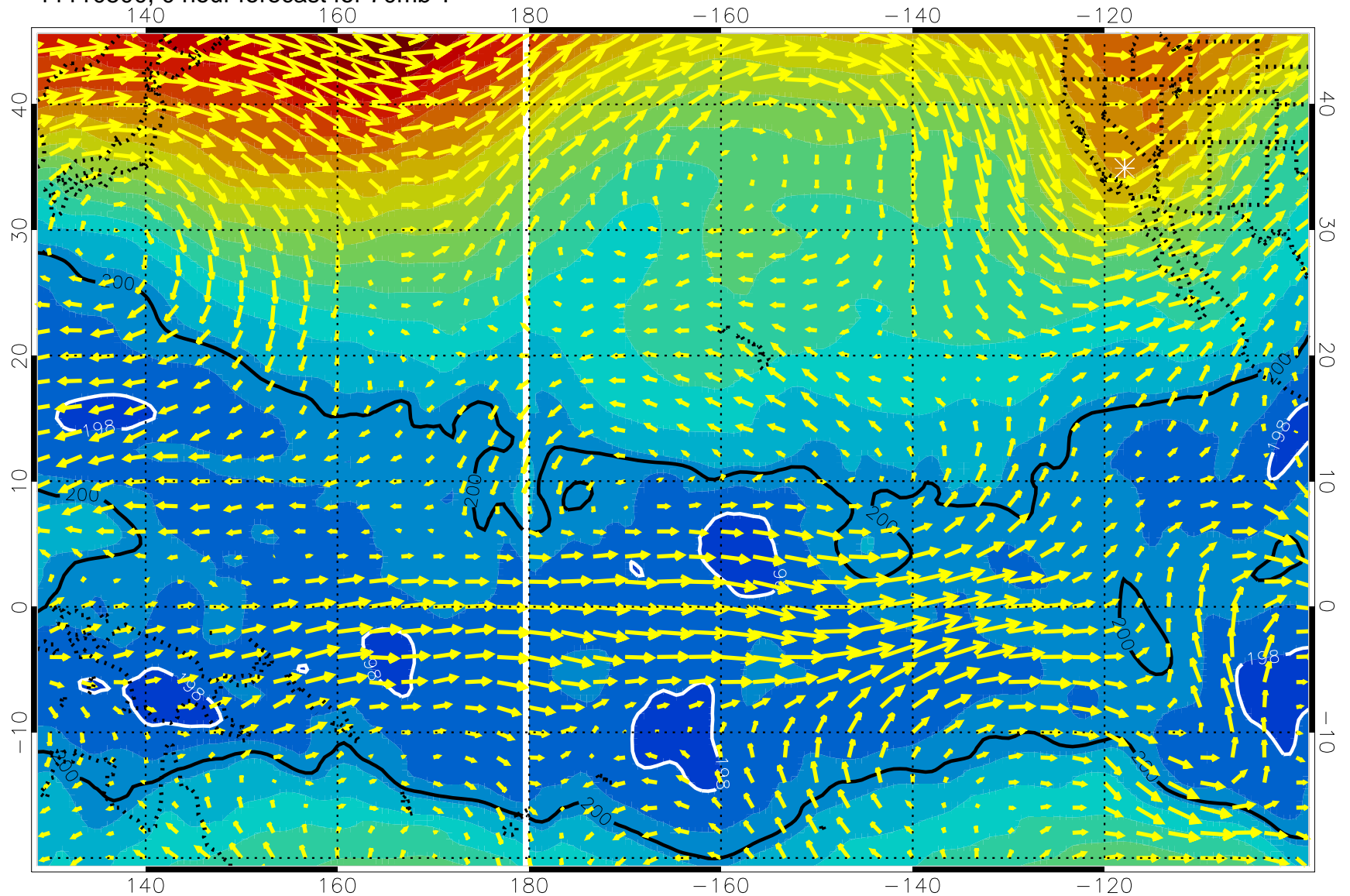
11110500, 0 hour forecast for 70mb T
