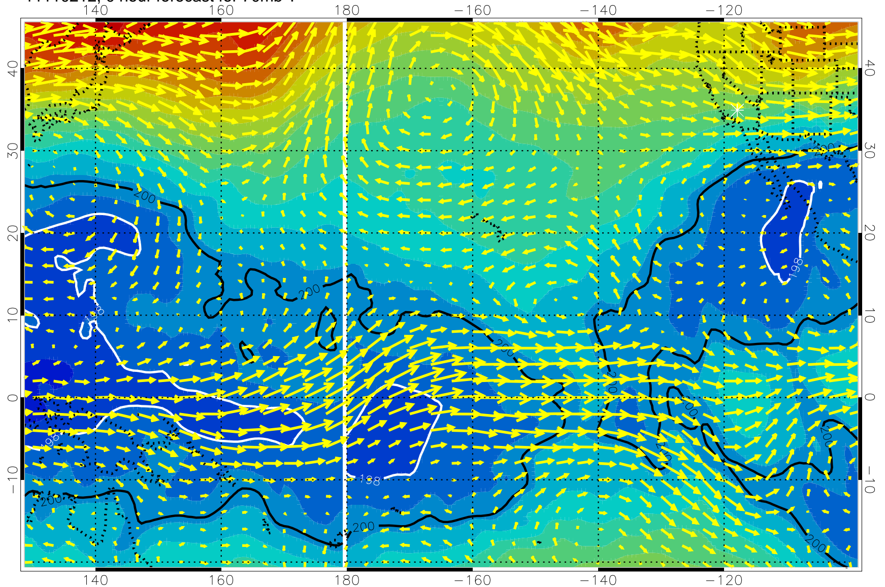
11110212, 0 hour forecast for 70mb T
