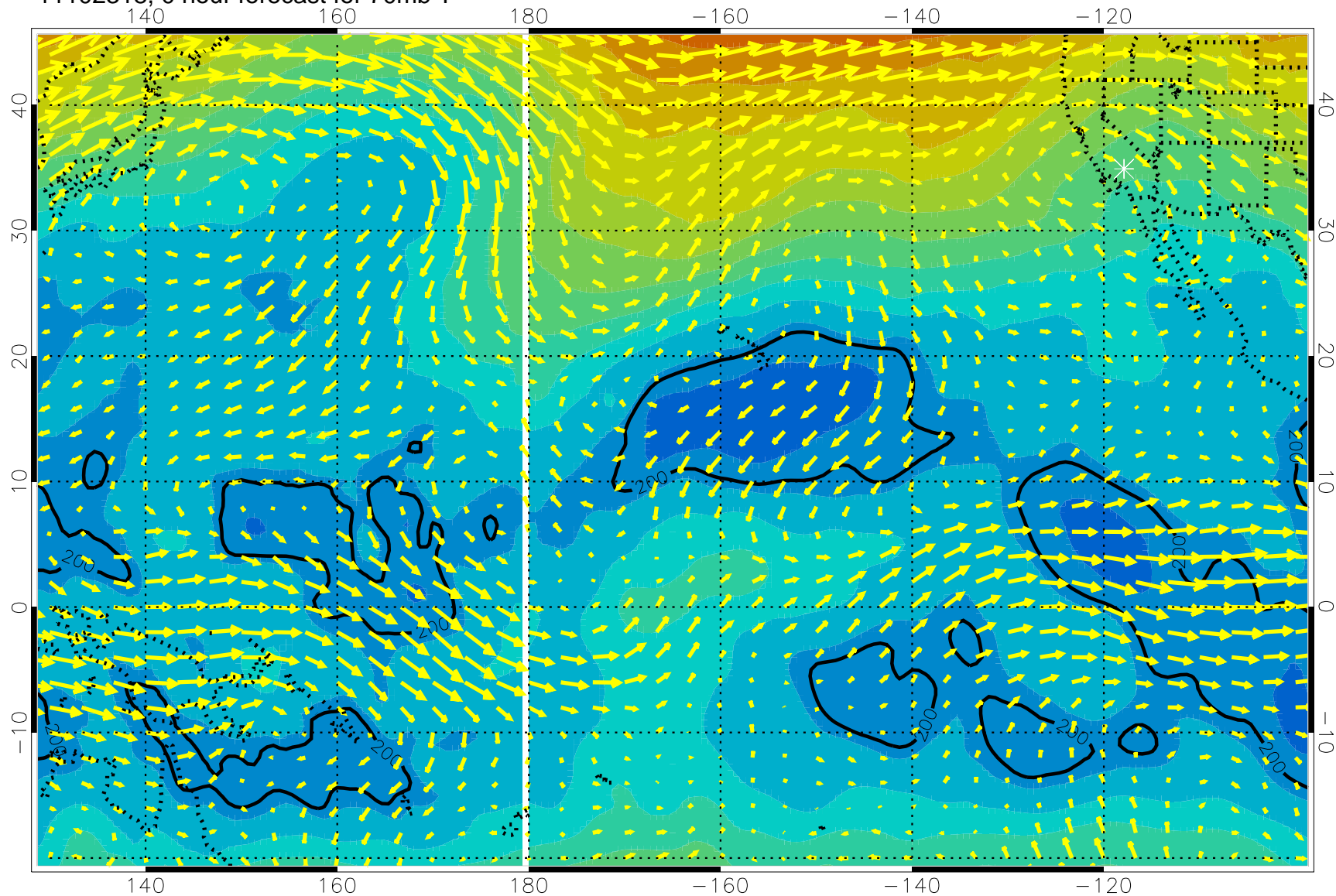
11102318, 0 hour forecast for 70mb T
