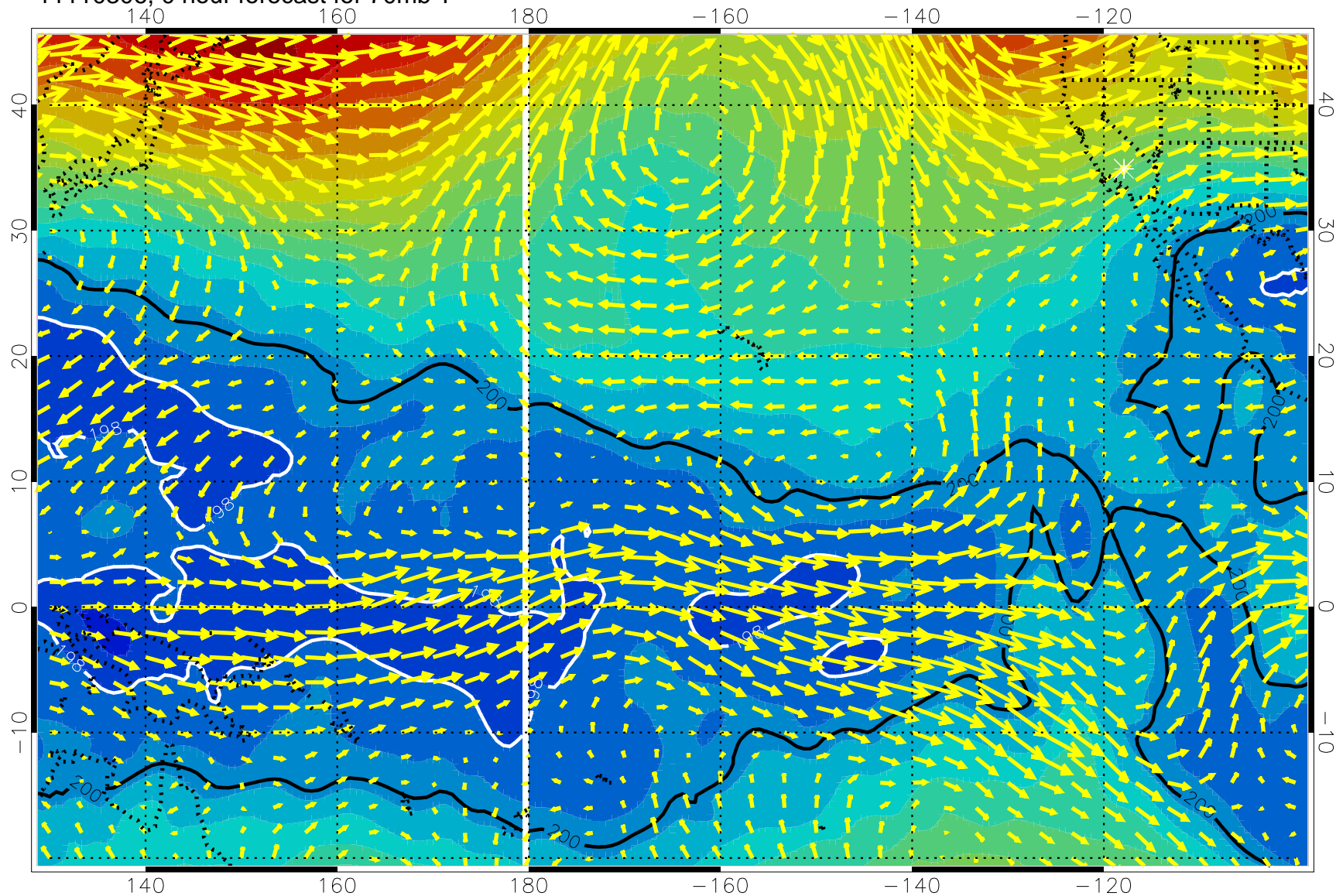
11110306, 0 hour forecast for 70mb T
