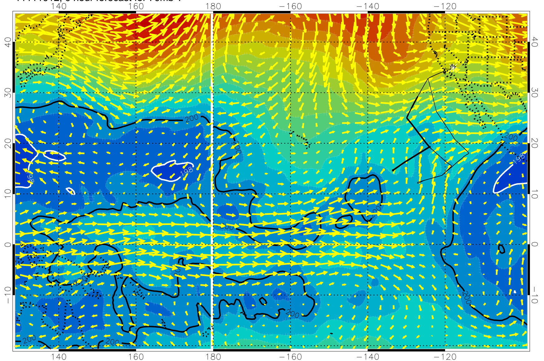
11111012, 0 hour forecast for 70mb T
