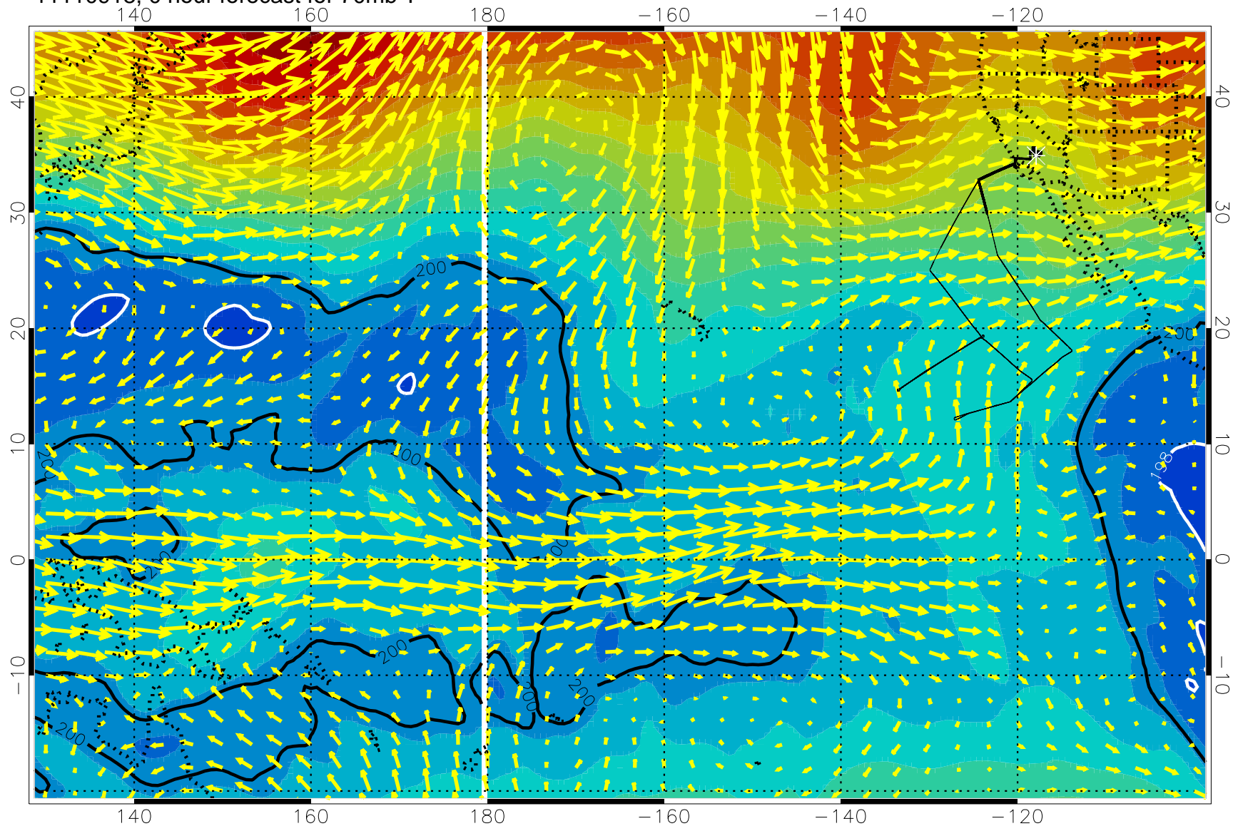
11110918, 0 hour forecast for 70mb T
