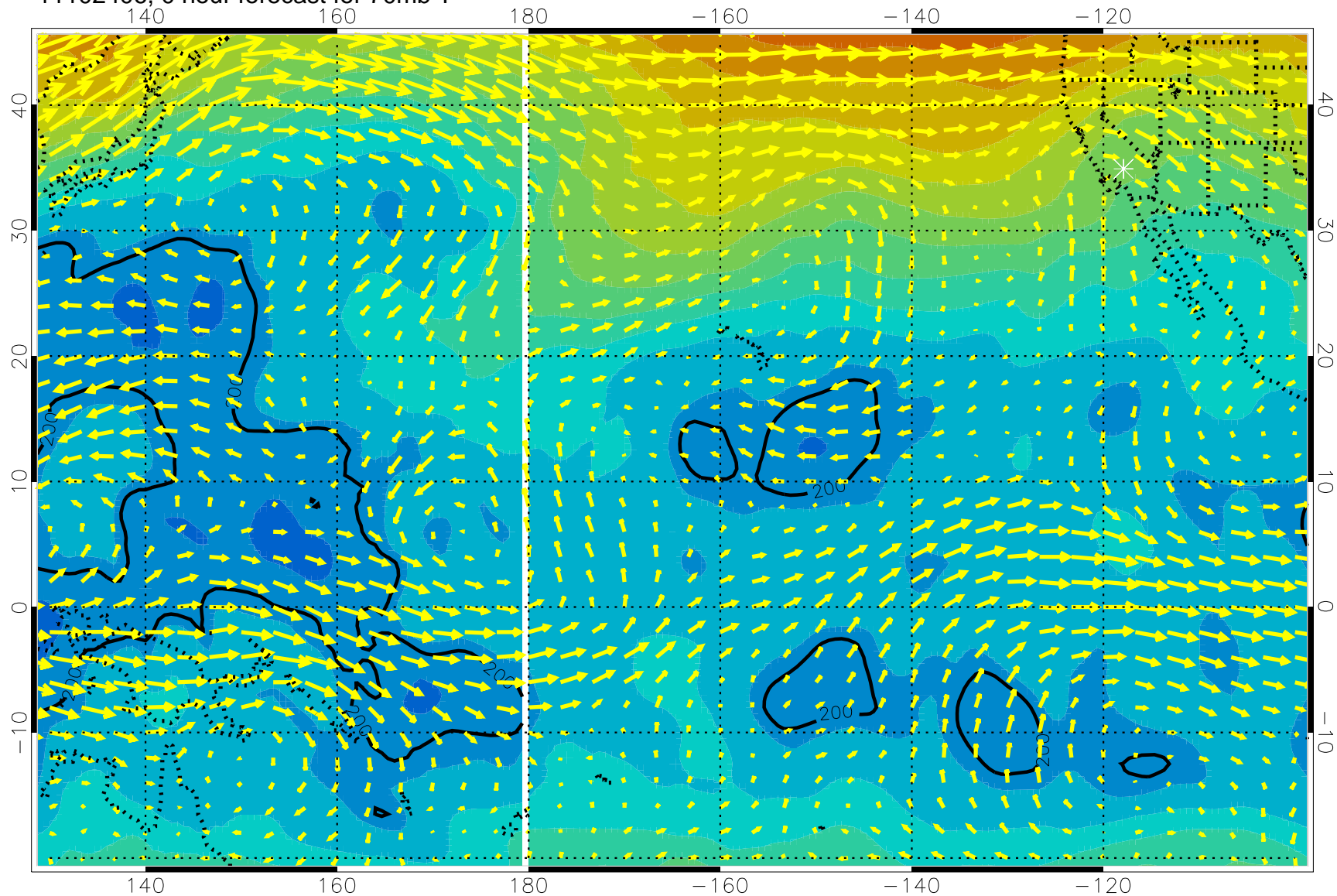
11102406, 0 hour forecast for 70mb T
