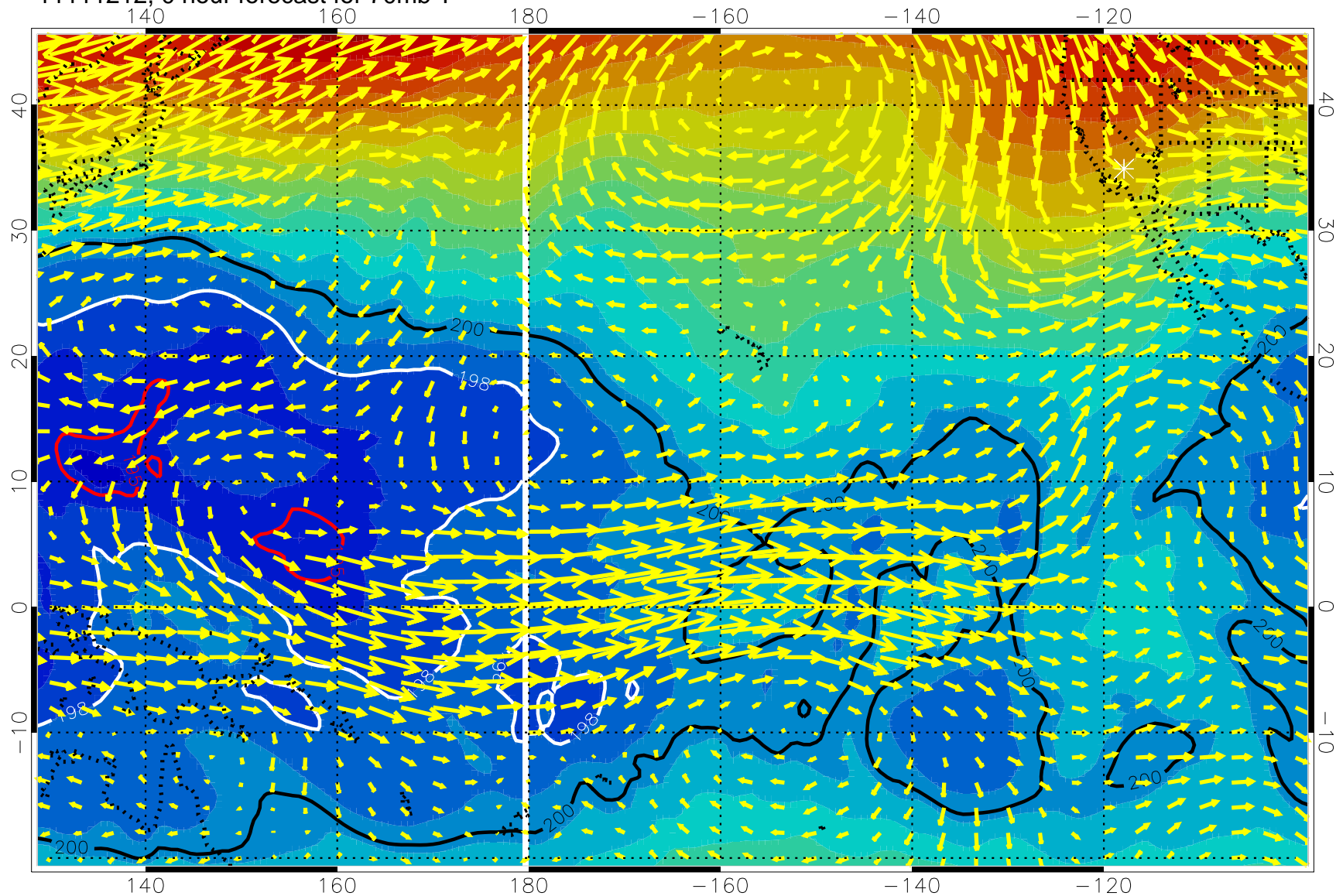
11111212, 0 hour forecast for 70mb T
