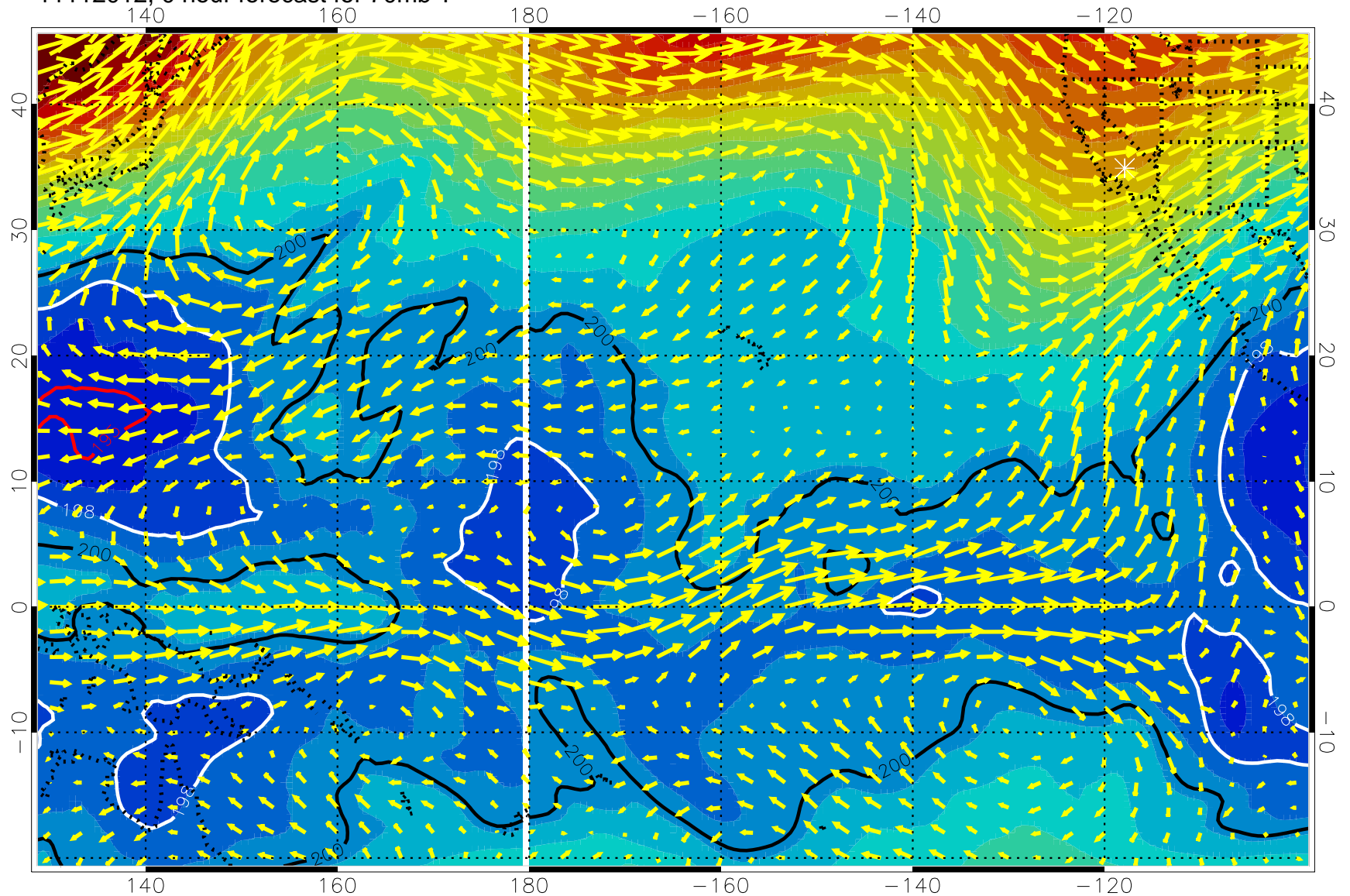
11112012, 0 hour forecast for 70mb T
