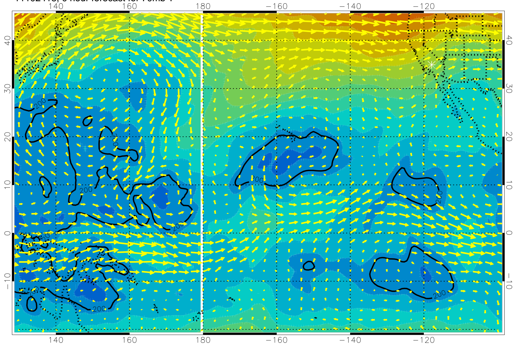
11102418, 0 hour forecast for 70mb T
