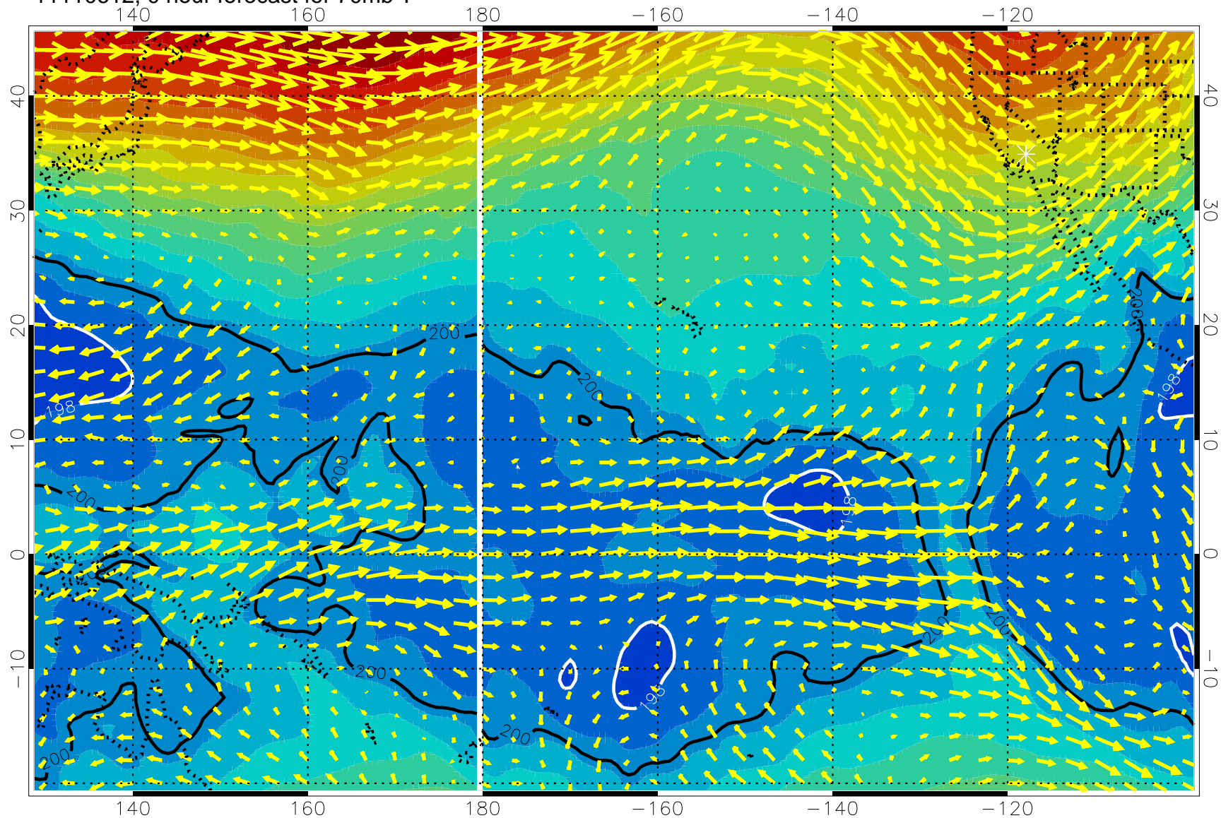
11110612, 0 hour forecast for 70mb T
