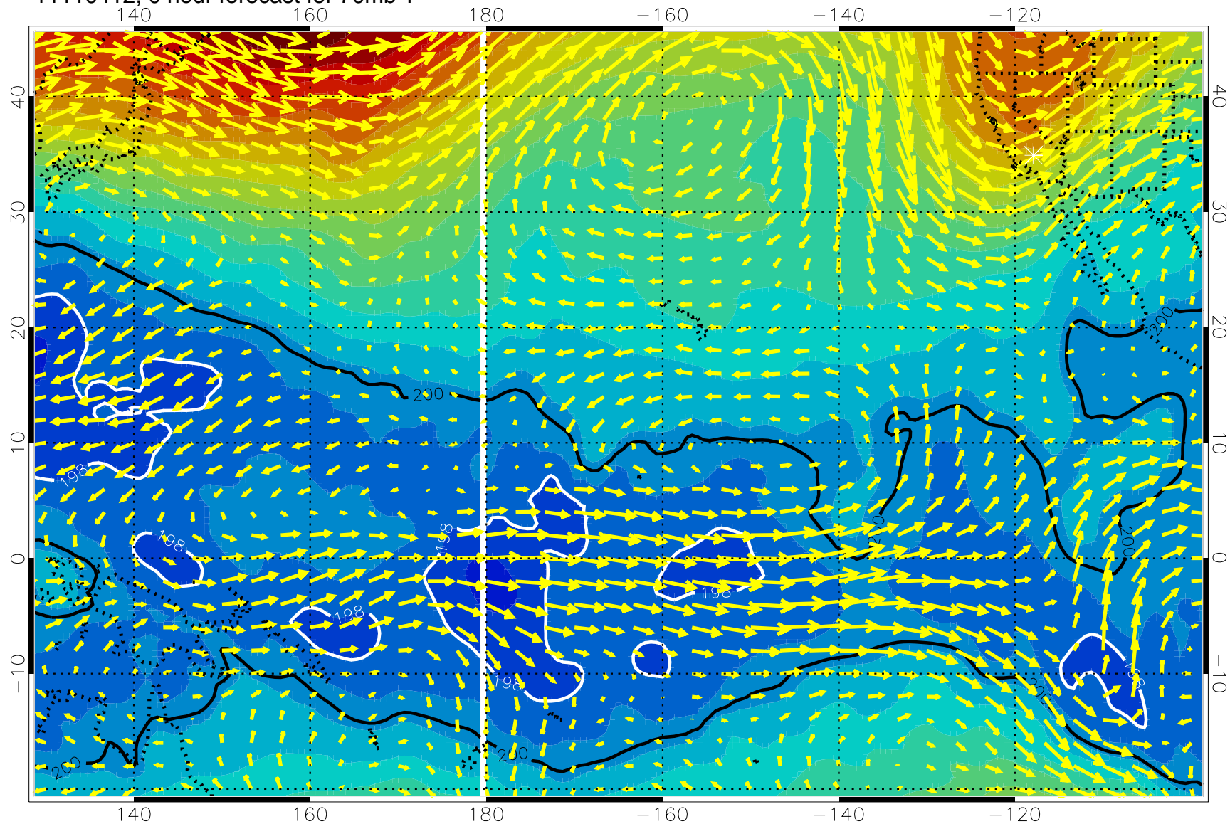
11110412, 0 hour forecast for 70mb T
