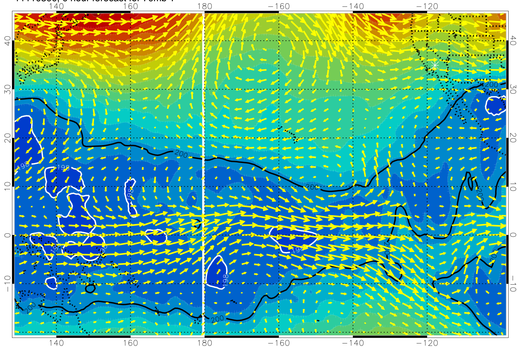
11110300, 0 hour forecast for 70mb T
