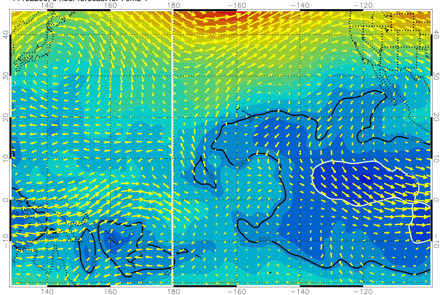
11102200, 0 hour forecast for 70mb T
