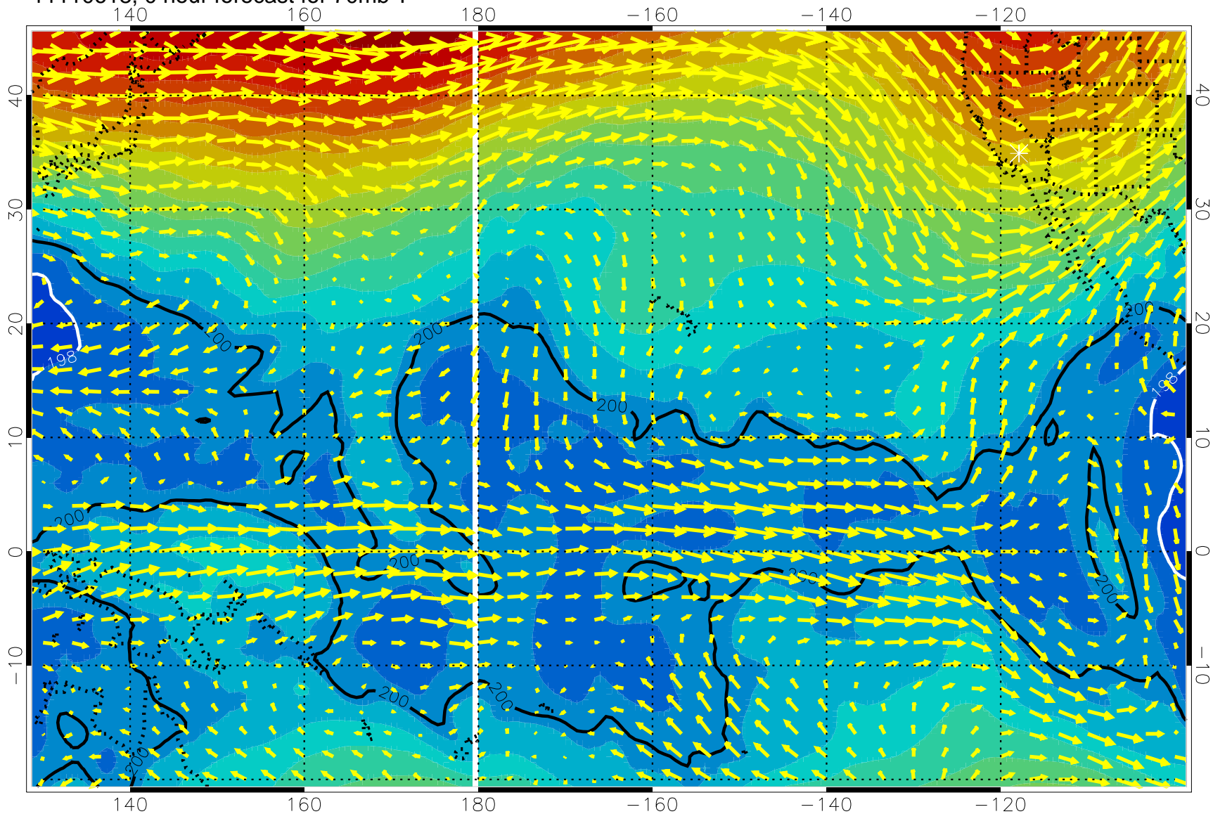
11110618, 0 hour forecast for 70mb T
