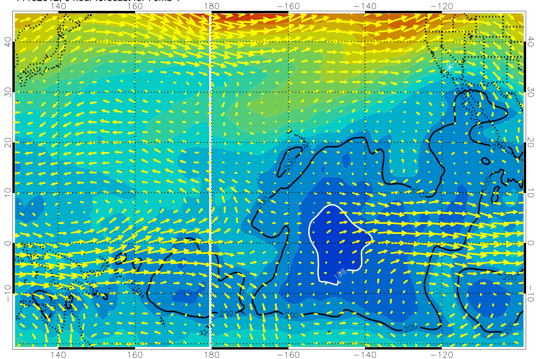
11102012, 0 hour forecast for 70mb T
