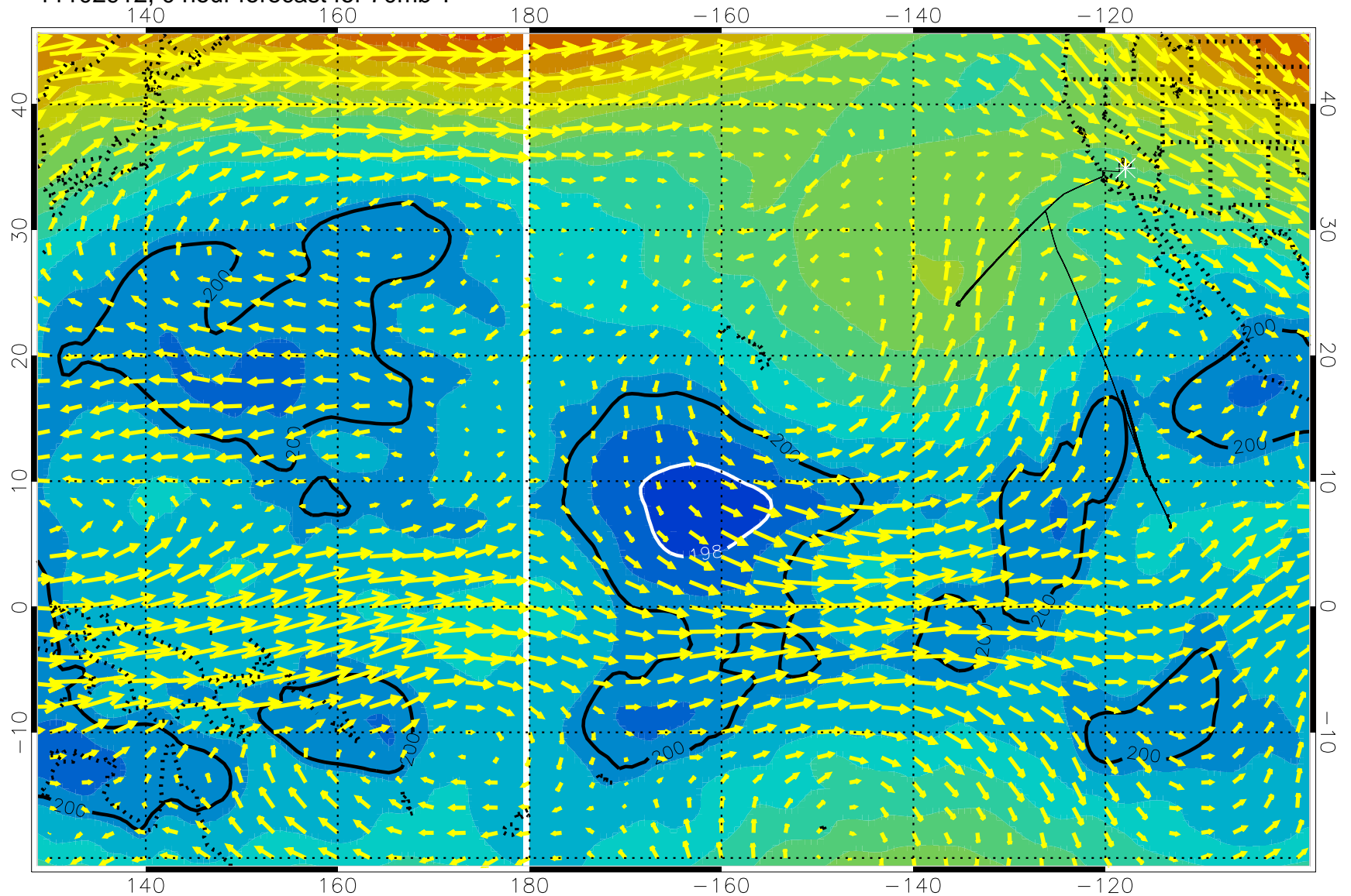
11102912, 0 hour forecast for 70mb T
