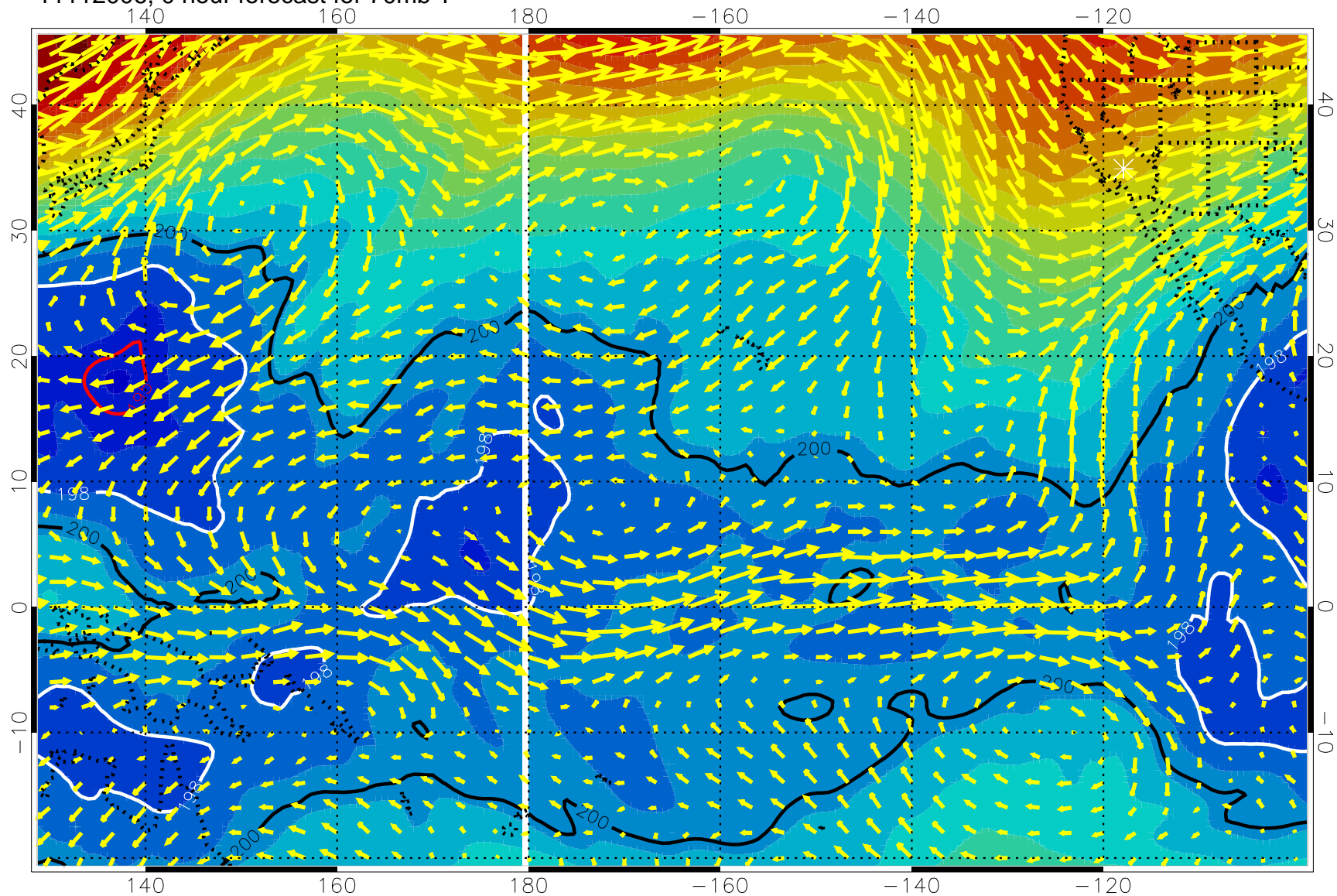
11112006, 0 hour forecast for 70mb T
