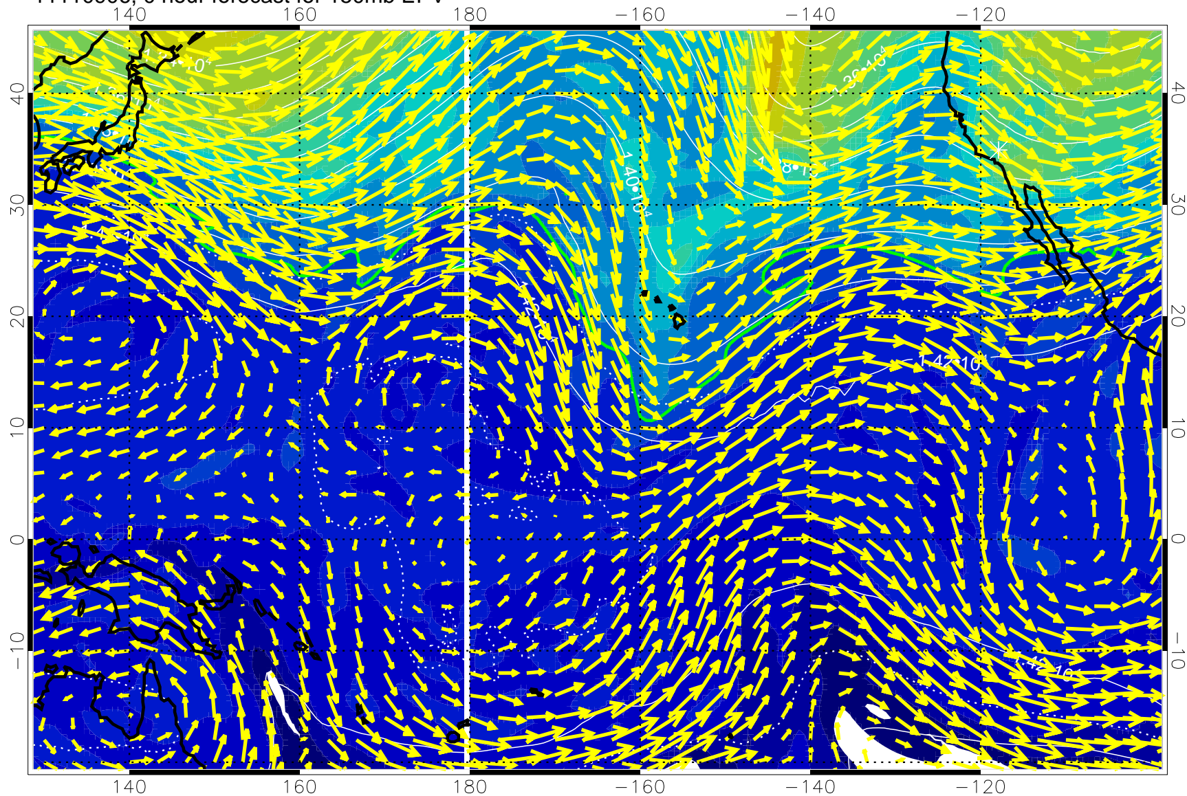
11110906, 0 hour forecast for 150mb EPV
