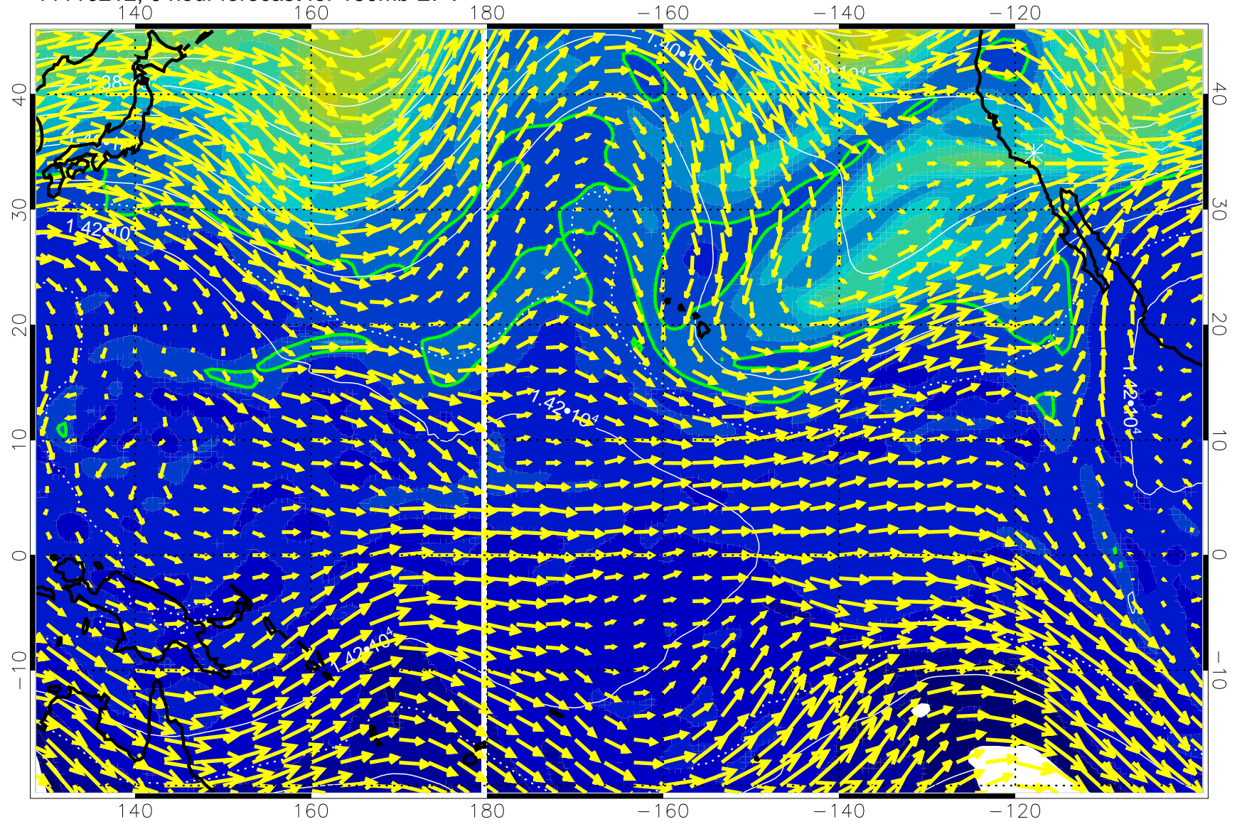
11110212, 0 hour forecast for 150mb EPV
