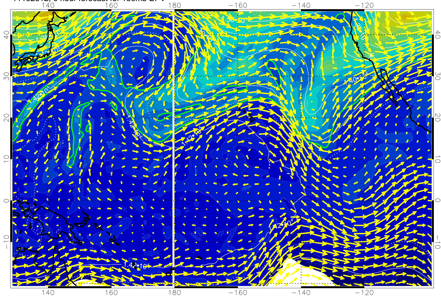
11102612, 0 hour forecast for 150mb EPV
