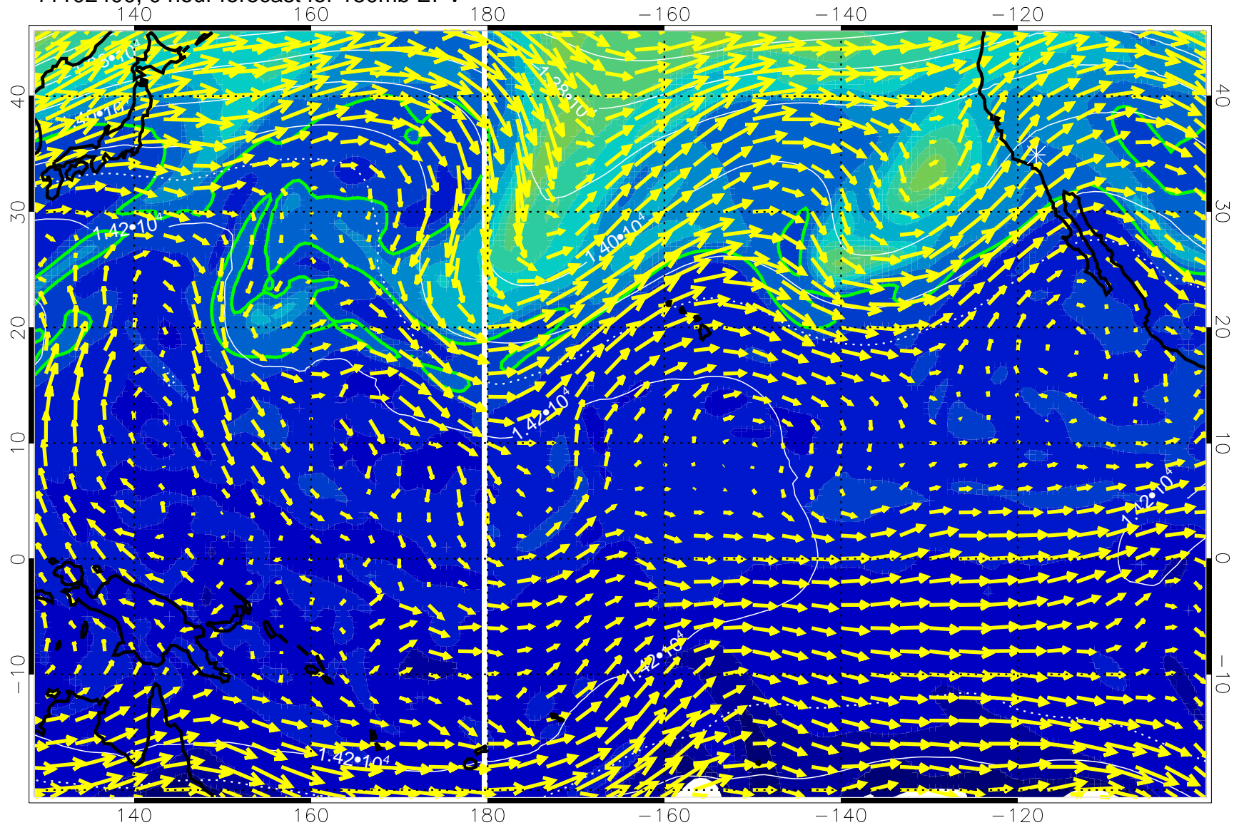
11102400, 0 hour forecast for 150mb EPV
