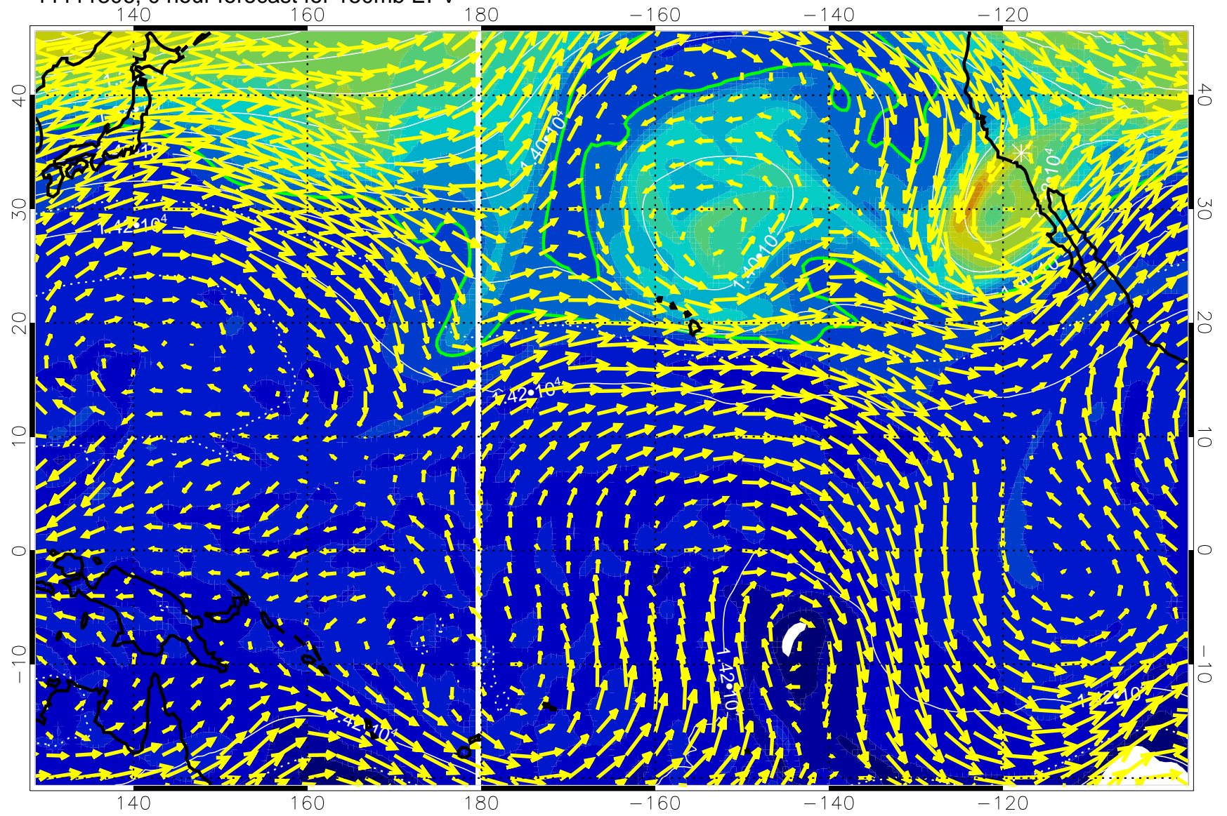
11111306, 0 hour forecast for 150mb EPV
