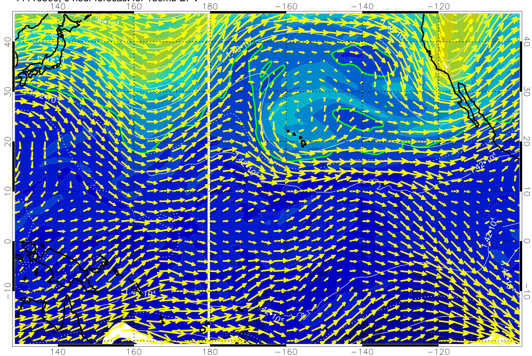
11110500, 0 hour forecast for 150mb EPV
