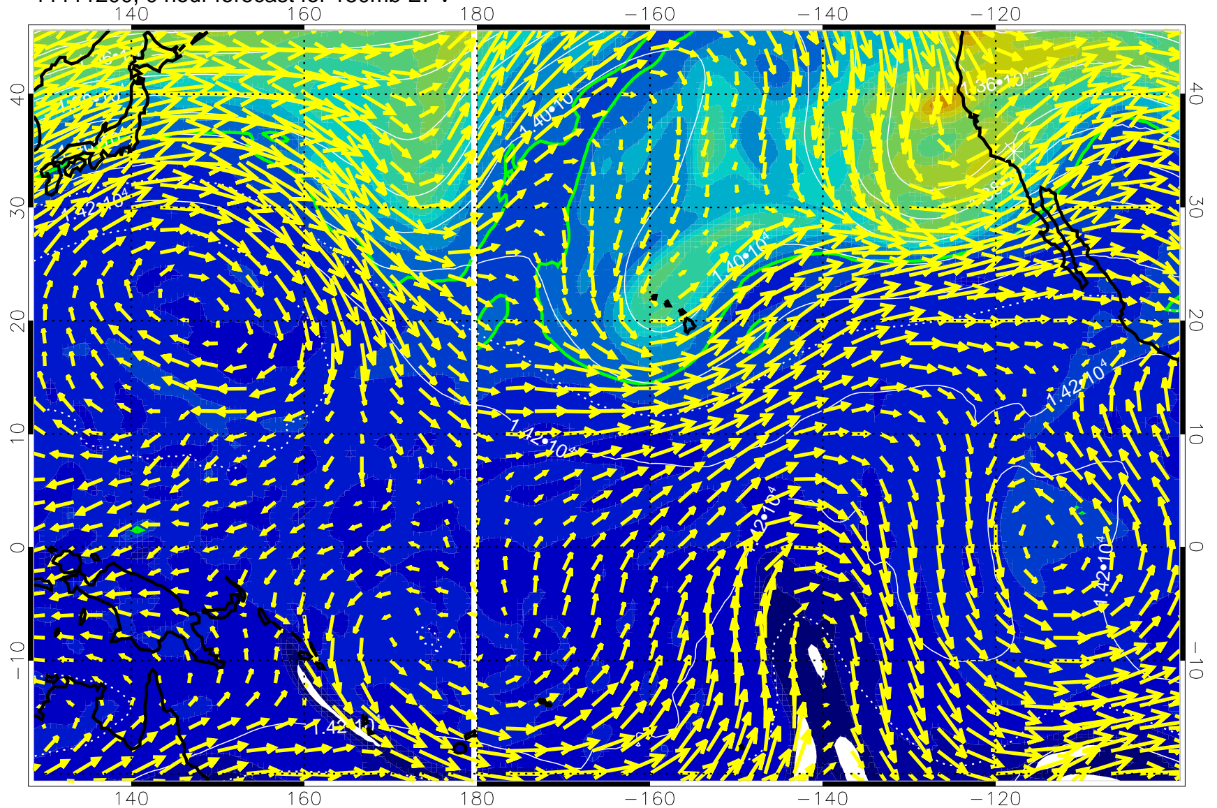
11111200, 0 hour forecast for 150mb EPV
