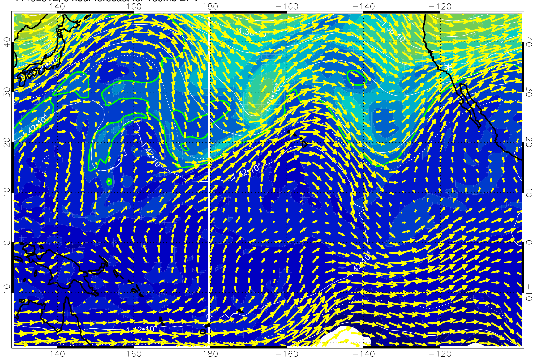
11102512, 0 hour forecast for 150mb EPV
