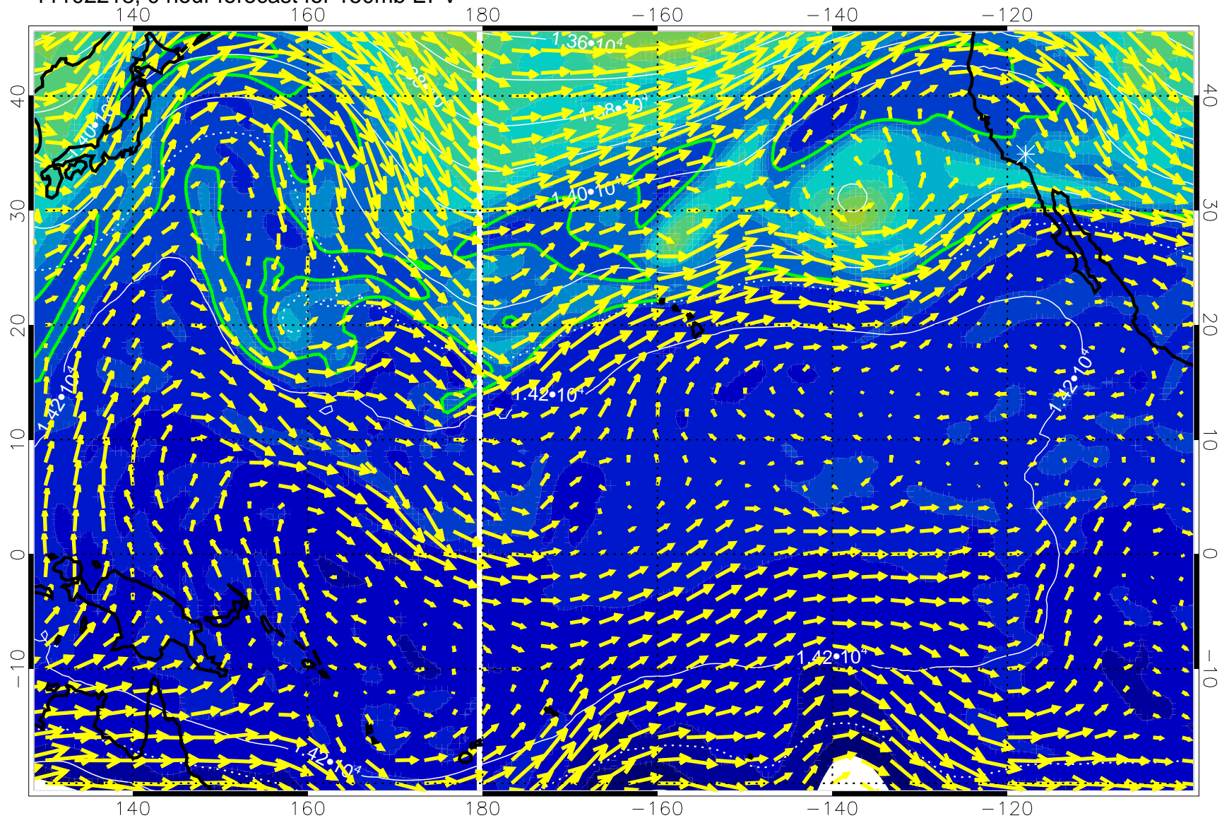
11102218, 0 hour forecast for 150mb EPV
