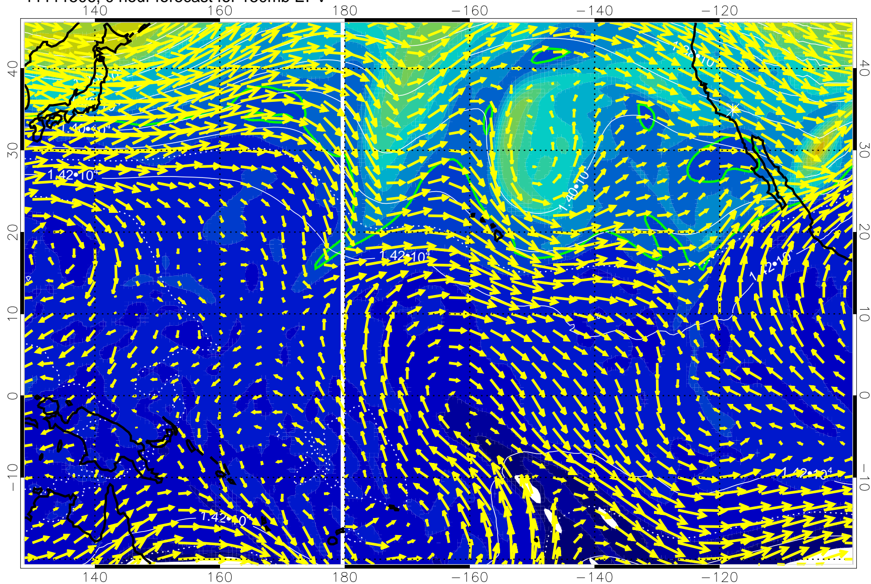
11111506, 0 hour forecast for 150mb EPV
