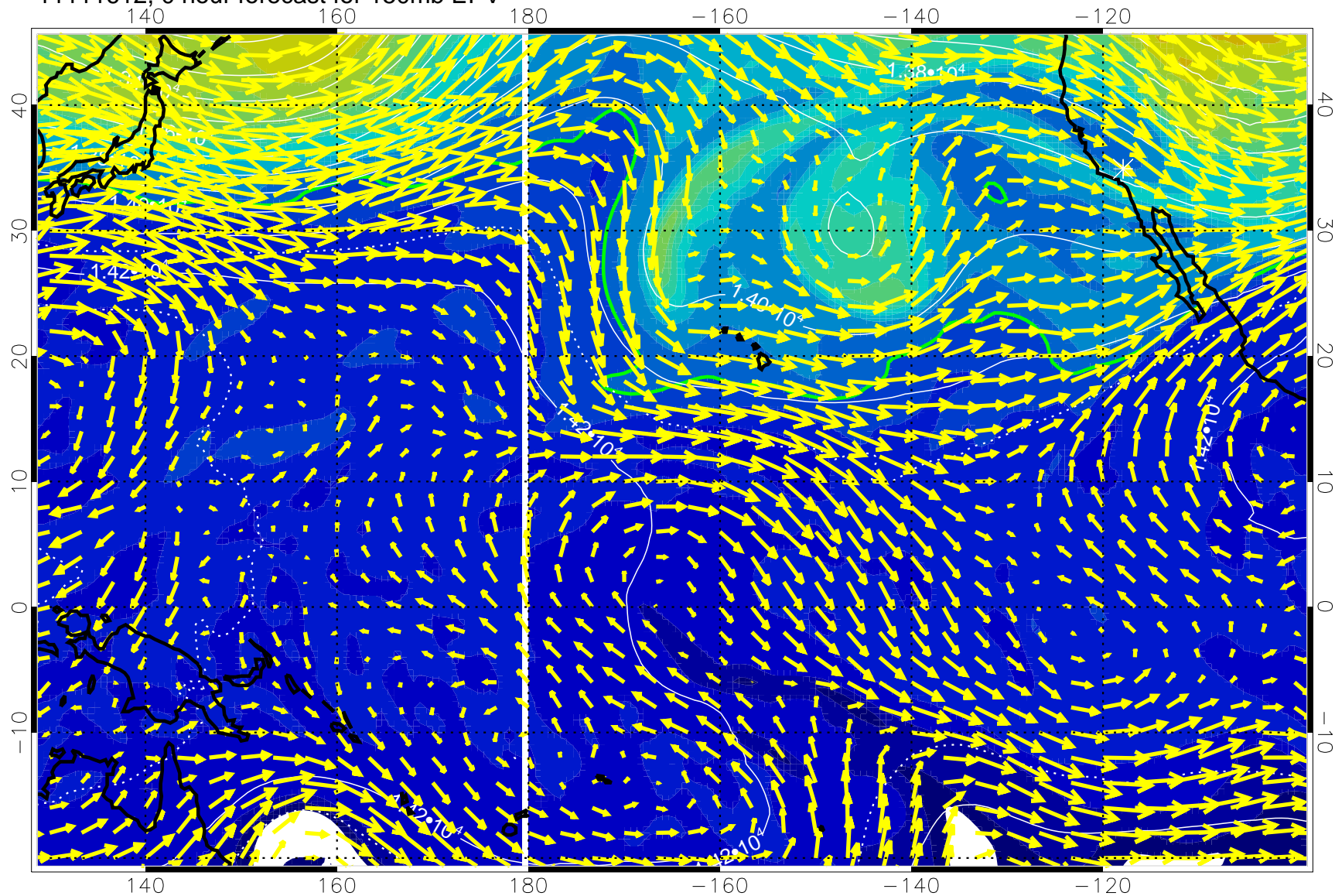
11111612, 0 hour forecast for 150mb EPV
