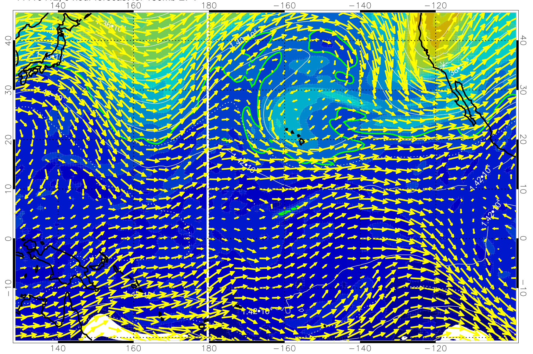
11110412, 0 hour forecast for 150mb EPV
