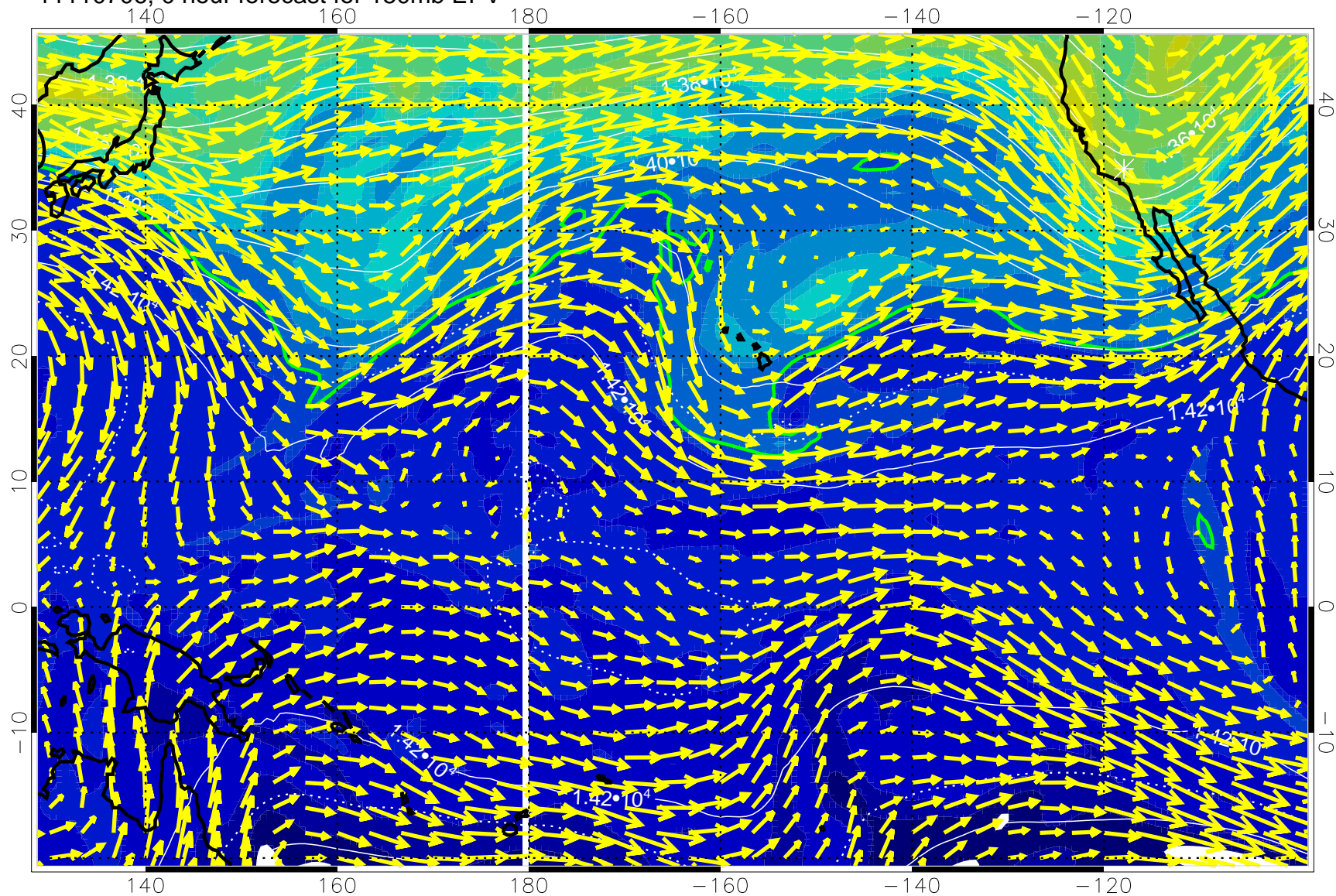
11110706, 0 hour forecast for 150mb EPV
