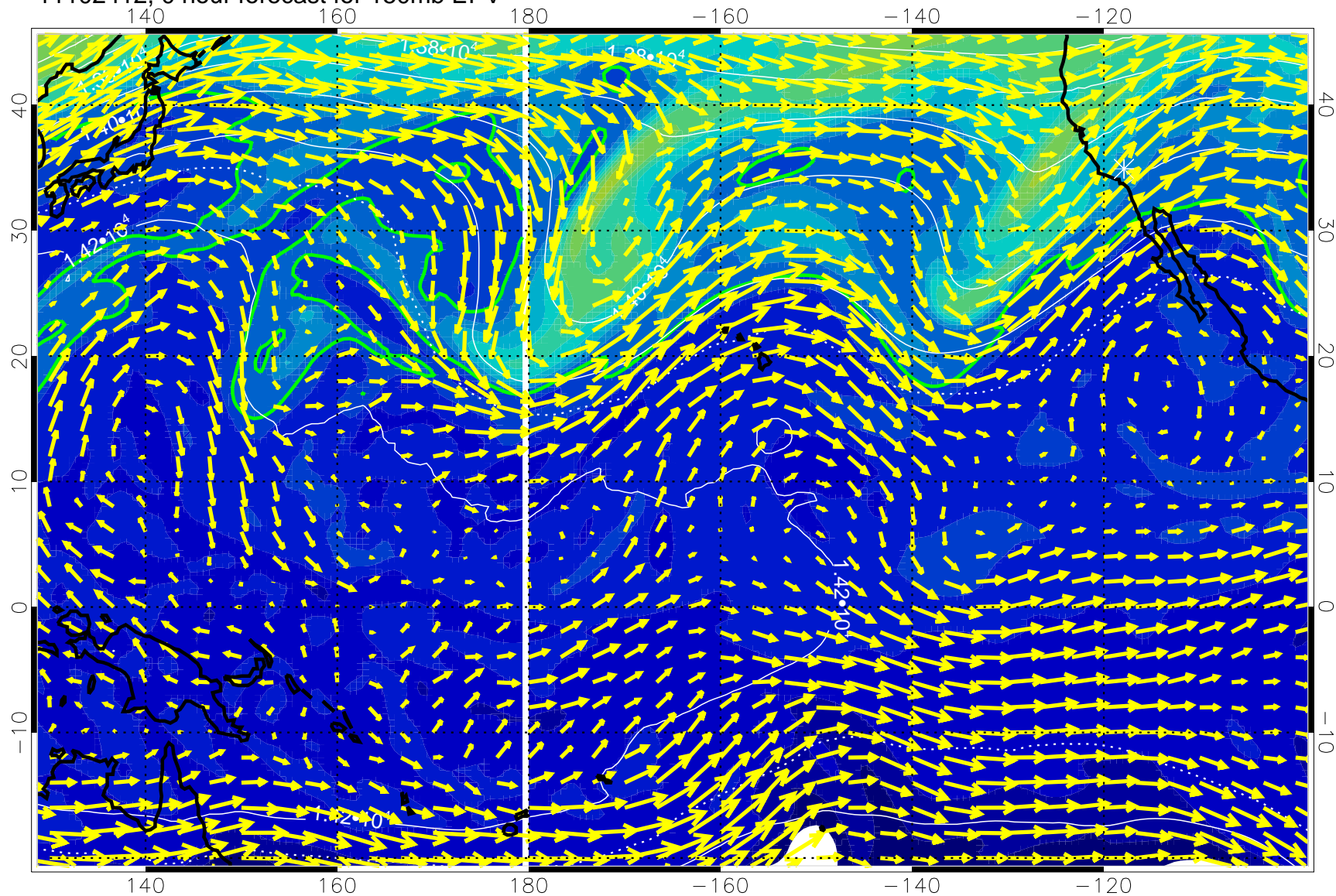
11102412, 0 hour forecast for 150mb EPV
