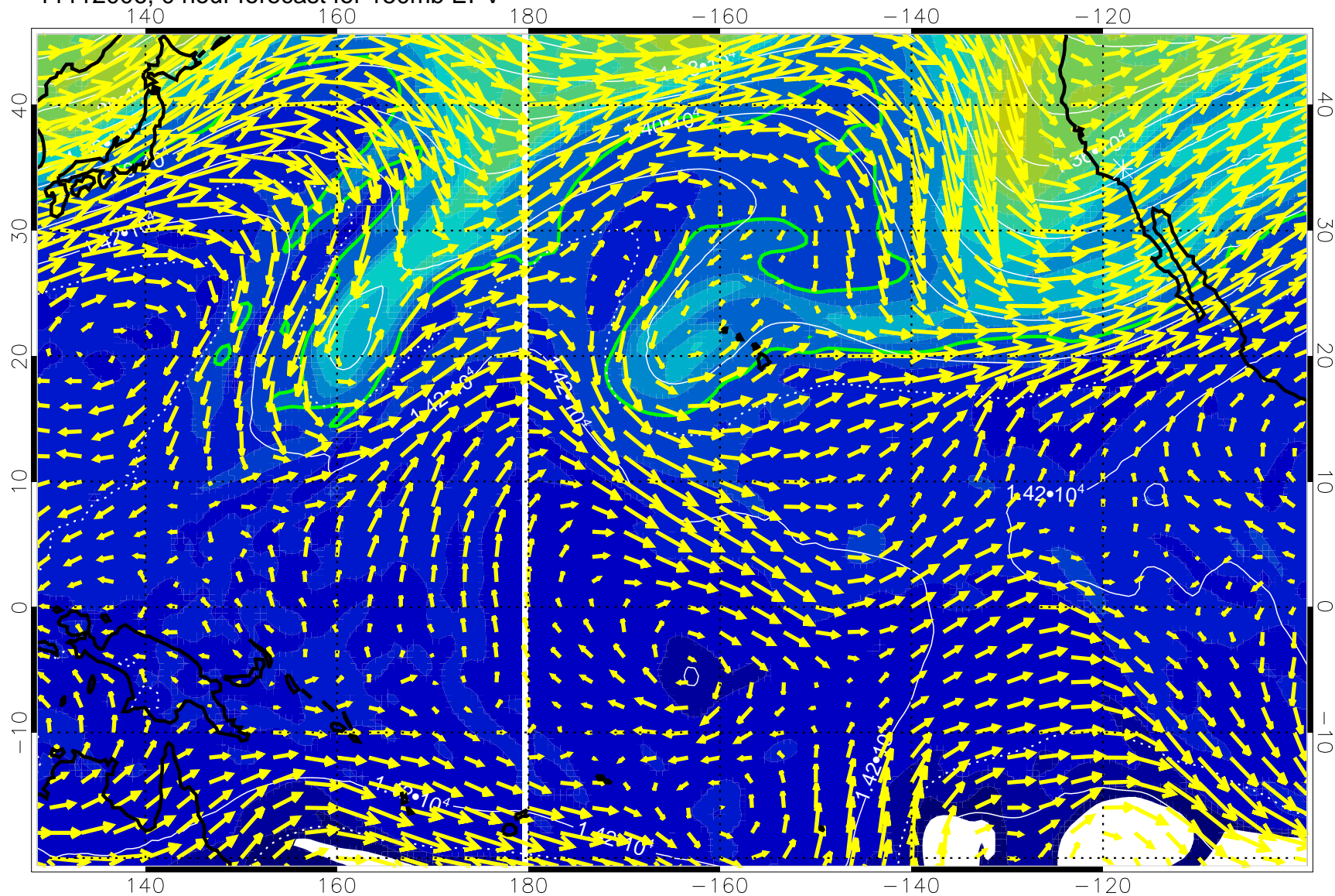
11112006, 0 hour forecast for 150mb EPV
