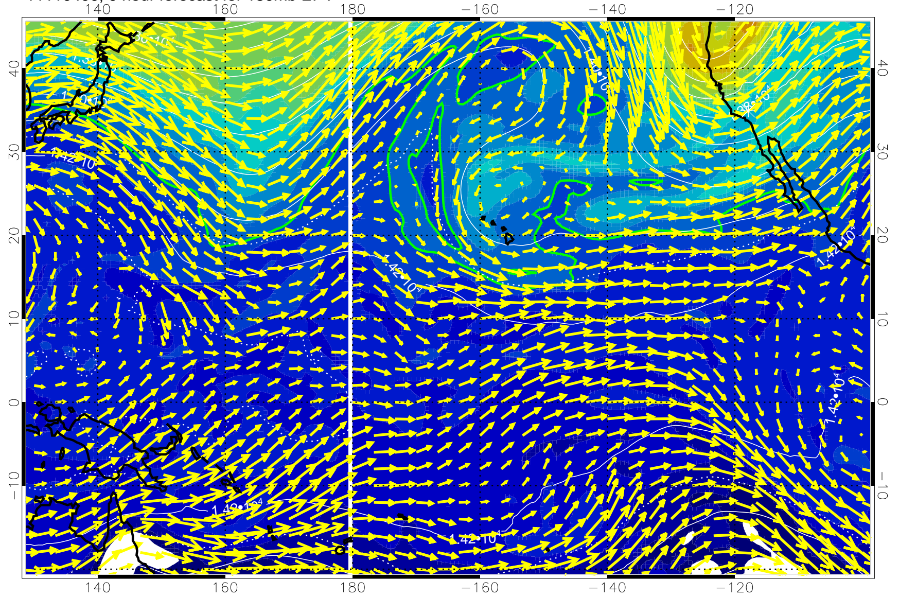
11110400, 0 hour forecast for 150mb EPV
