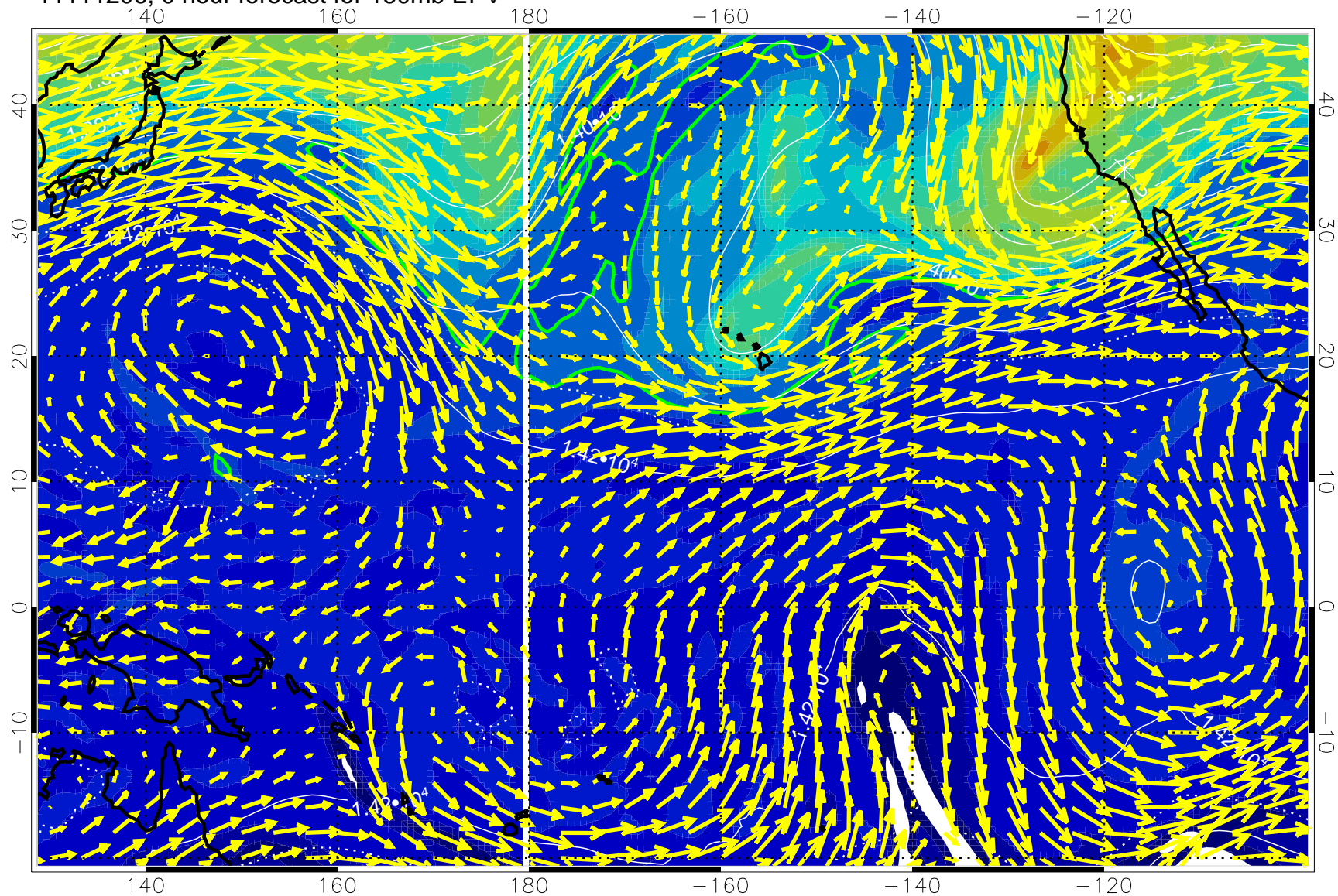
11111206, 0 hour forecast for 150mb EPV
