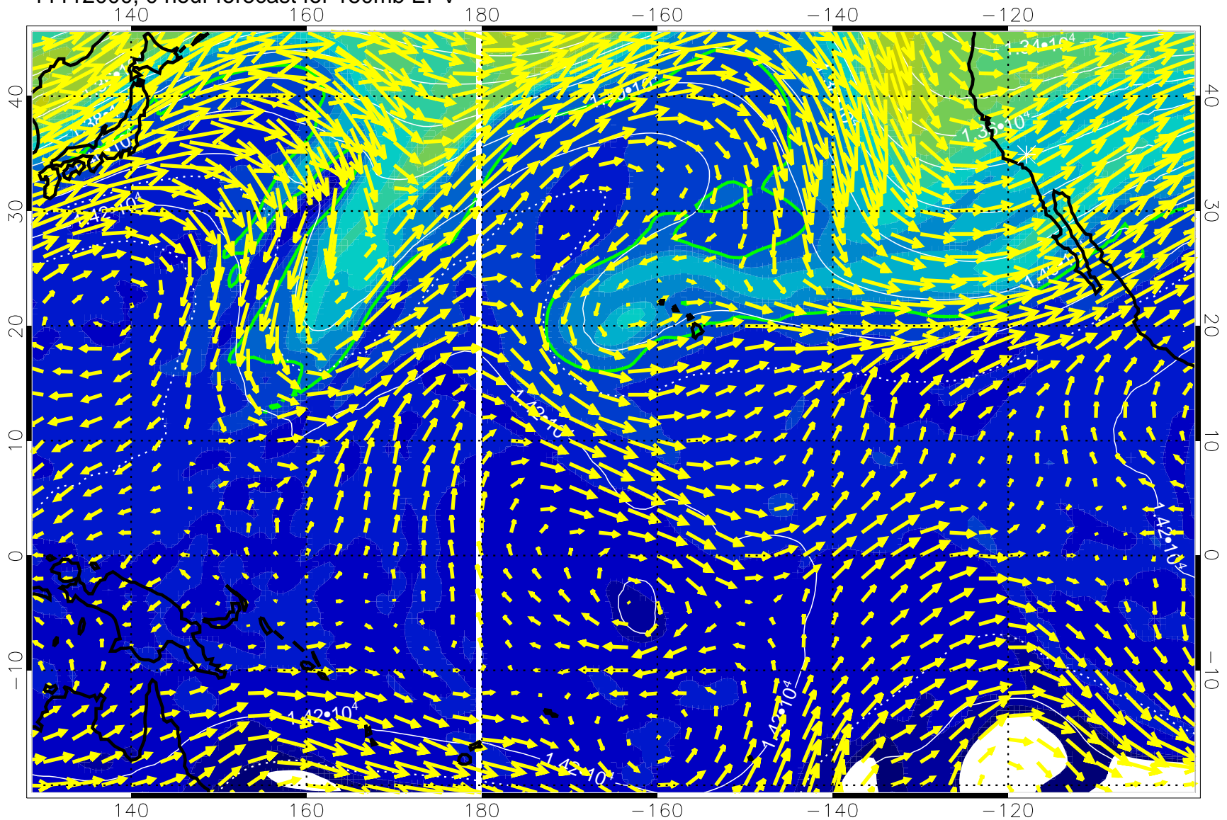
11112000, 0 hour forecast for 150mb EPV
