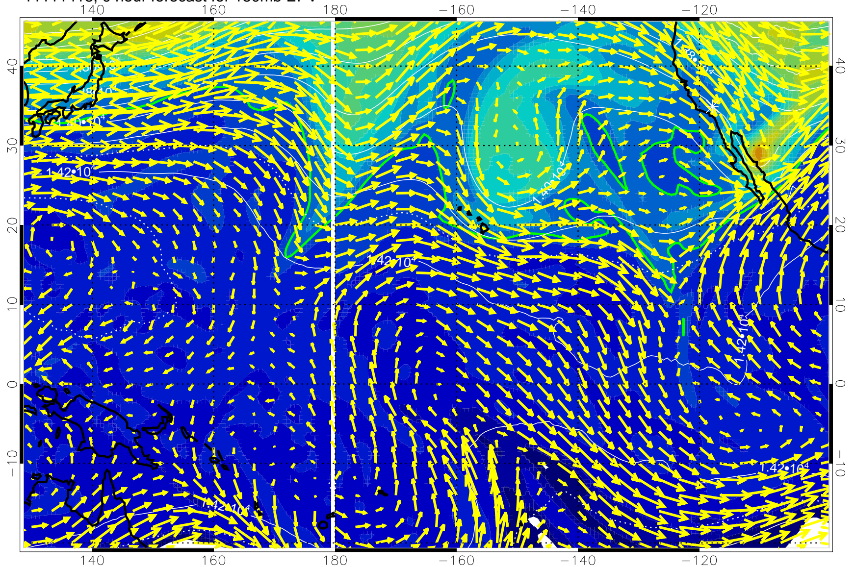
11111418, 0 hour forecast for 150mb EPV
