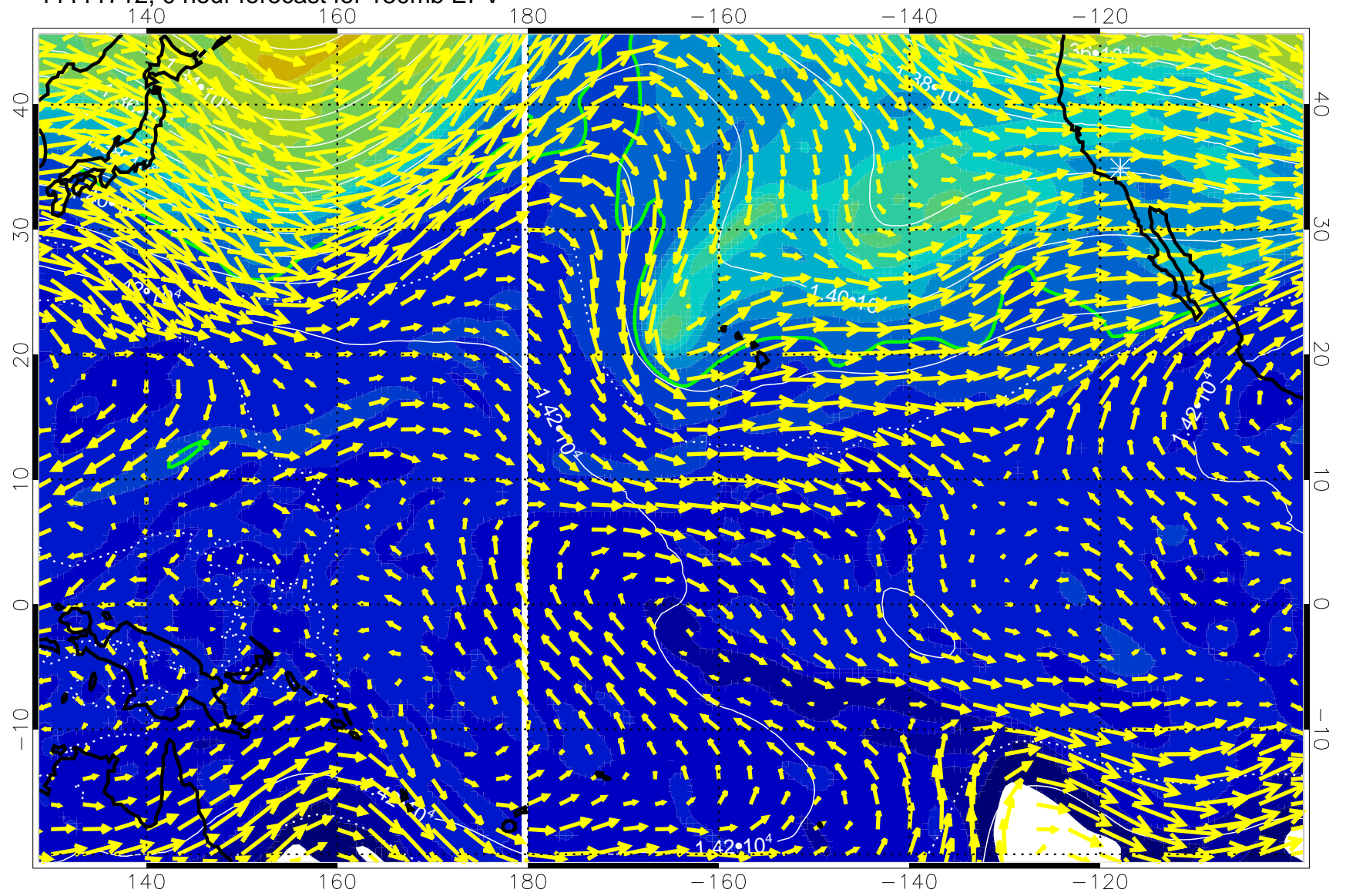
11111712, 0 hour forecast for 150mb EPV
