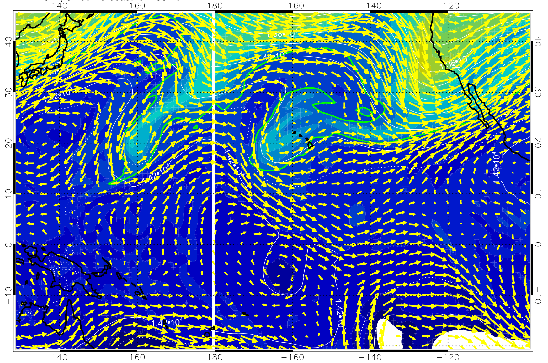
11112012, 0 hour forecast for 150mb EPV
