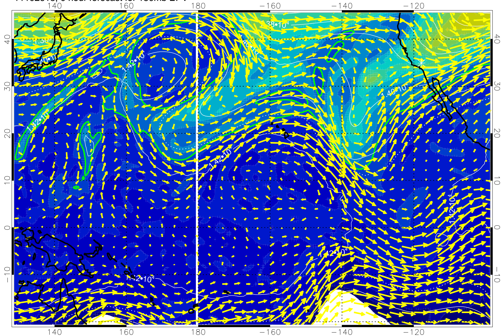
11102618, 0 hour forecast for 150mb EPV
