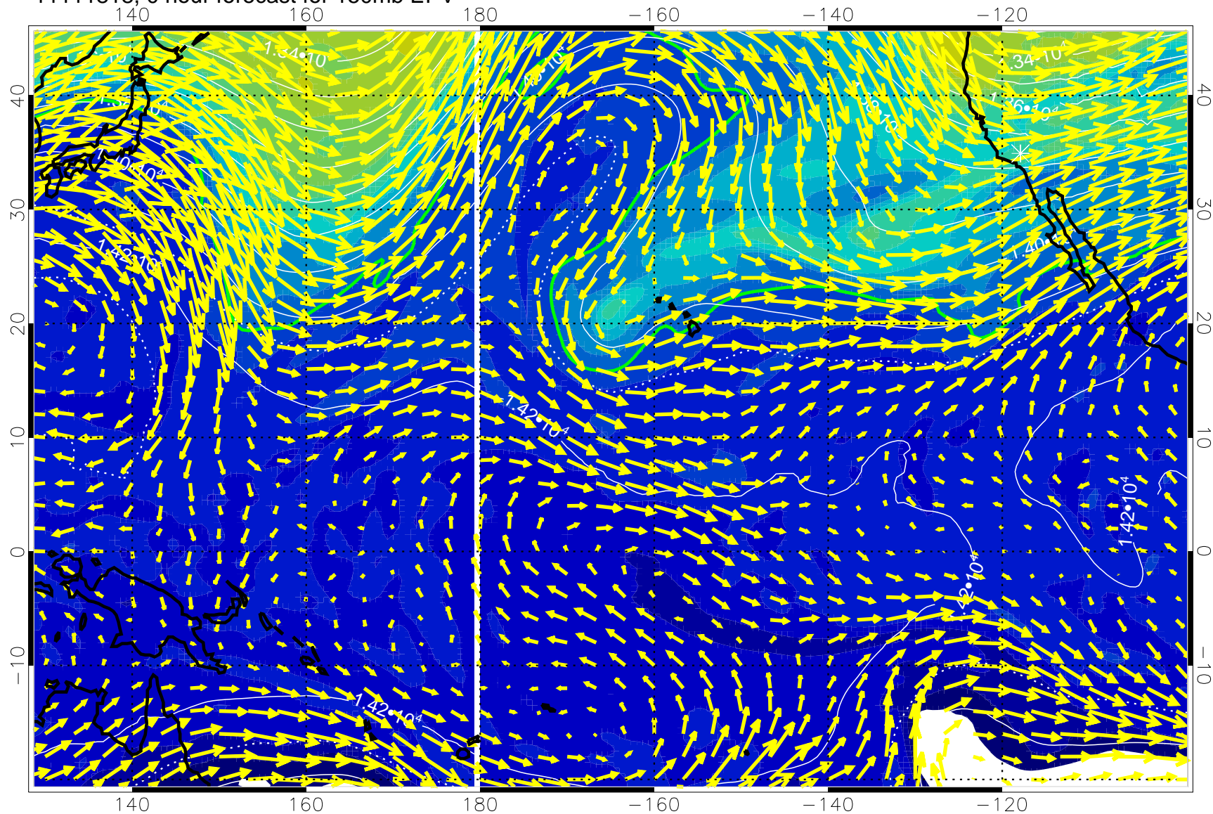
11111818, 0 hour forecast for 150mb EPV
