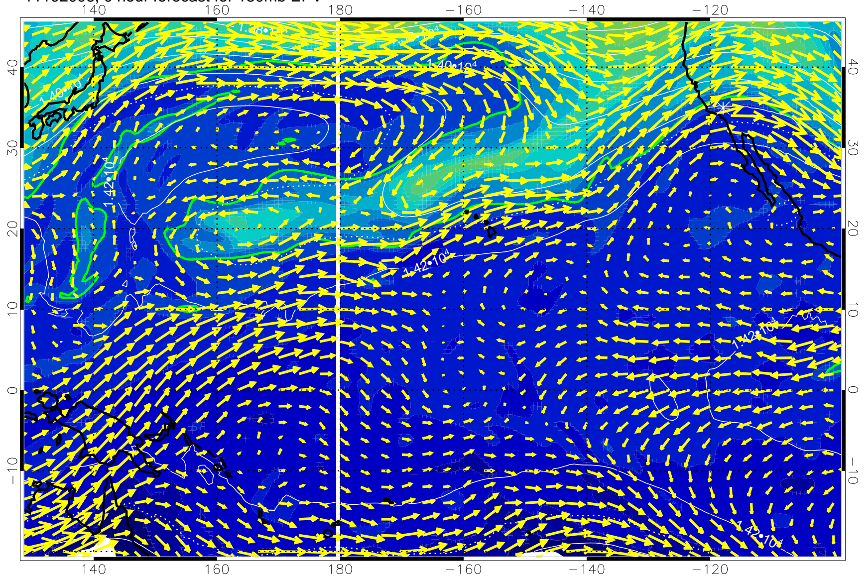
11102006, 0 hour forecast for 150mb EPV
