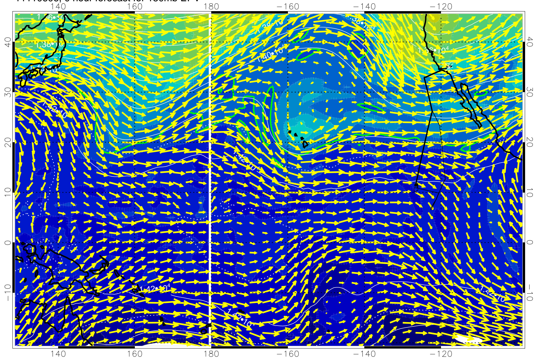
11110606, 0 hour forecast for 150mb EPV
