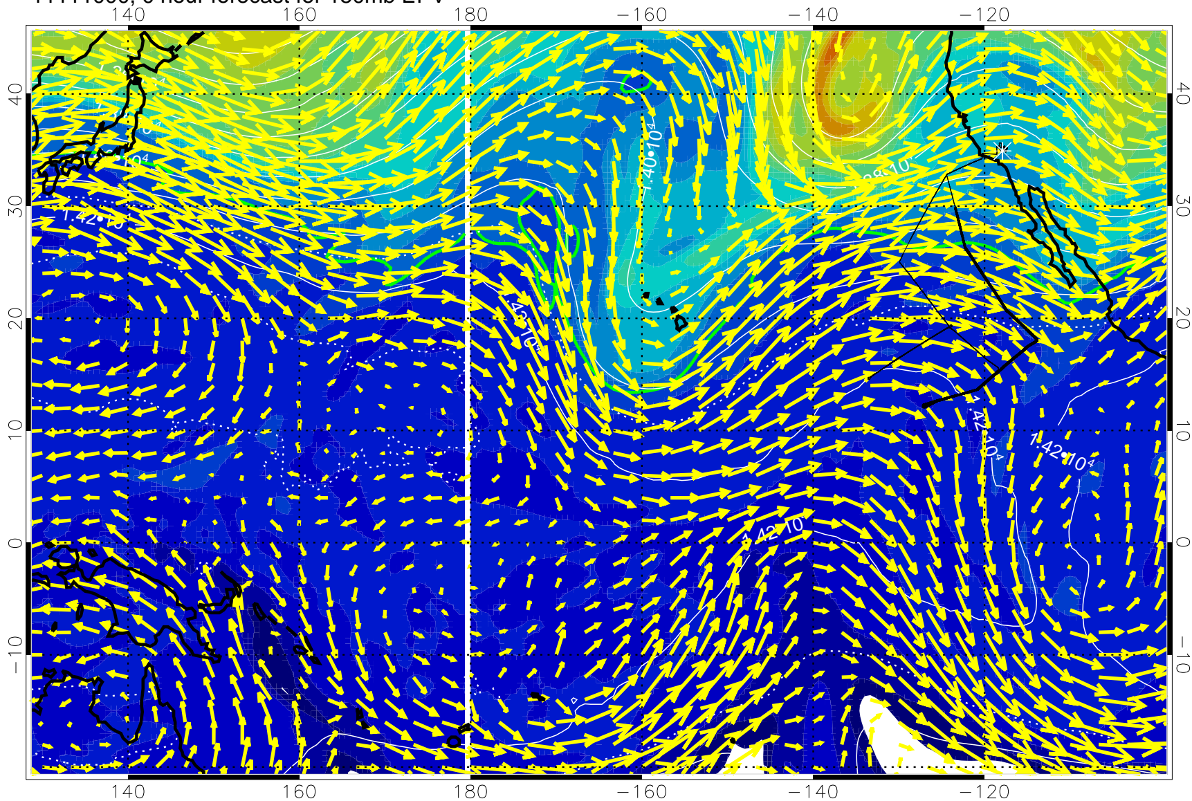
11111000, 0 hour forecast for 150mb EPV
