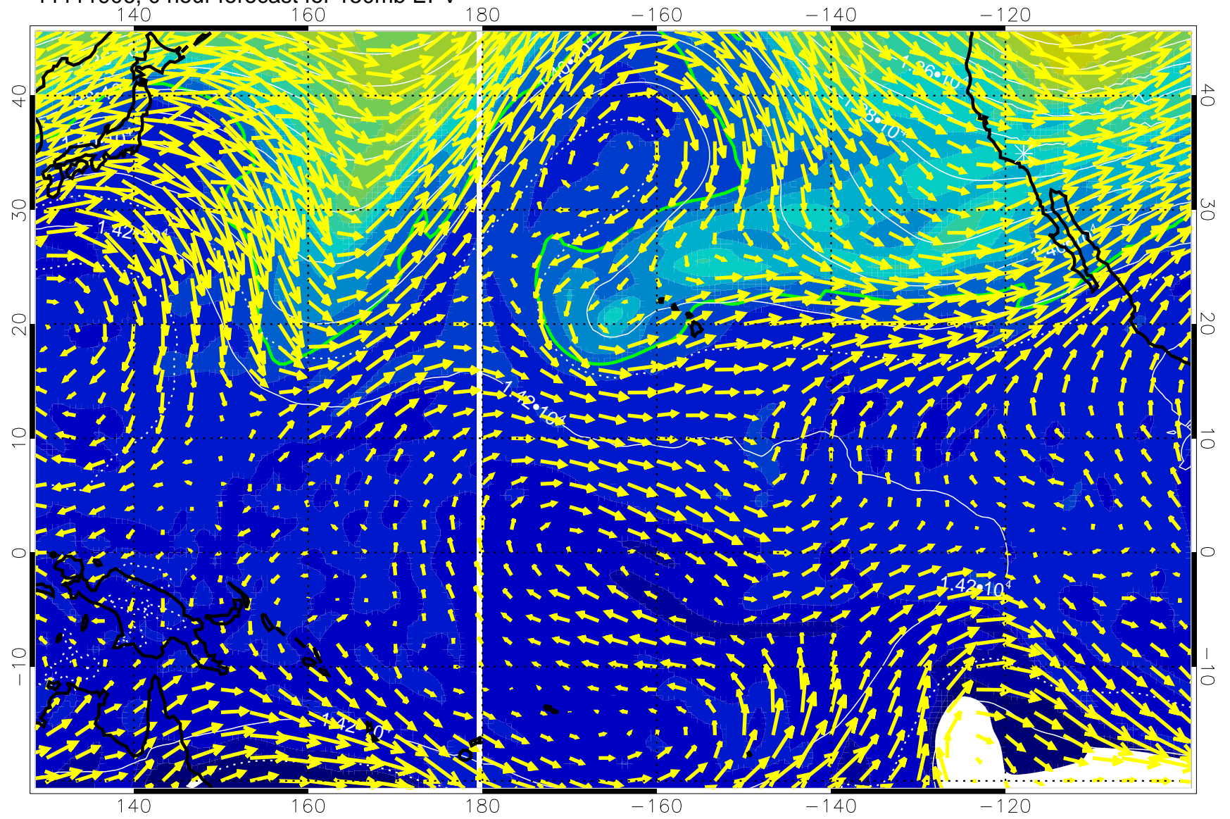
11111906, 0 hour forecast for 150mb EPV
