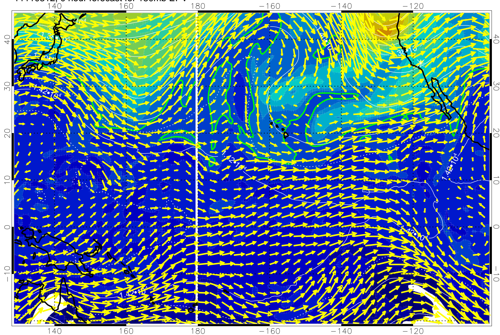
11110312, 0 hour forecast for 150mb EPV
