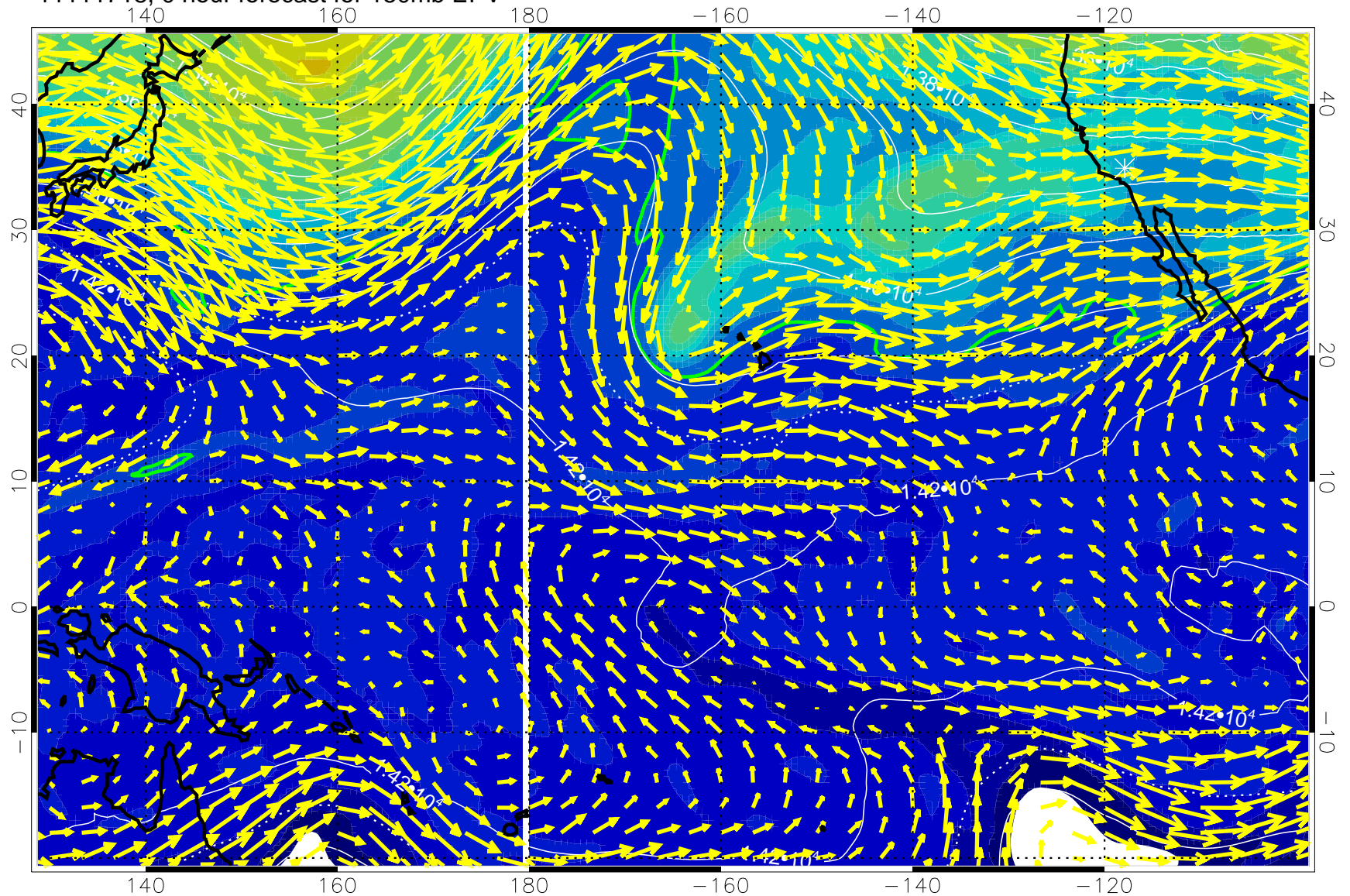
11111718, 0 hour forecast for 150mb EPV
