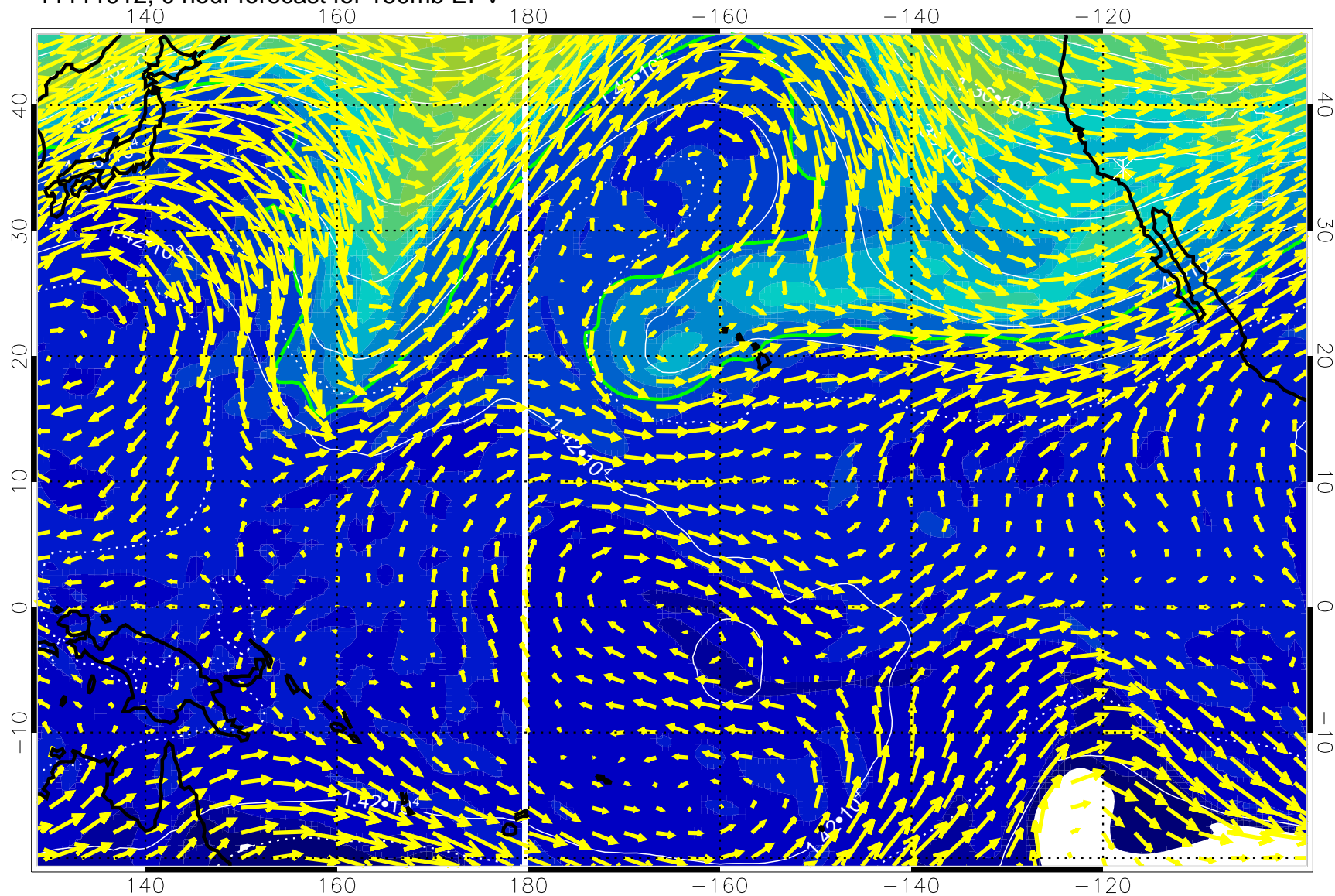
11111912, 0 hour forecast for 150mb EPV
