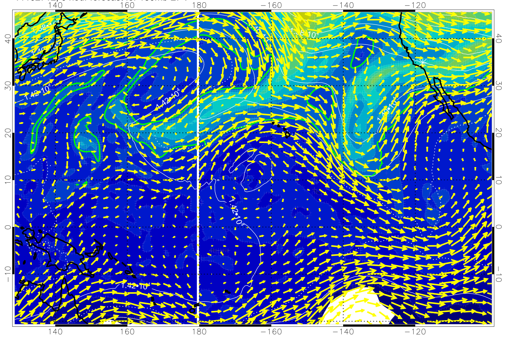
11102712, 0 hour forecast for 150mb EPV
