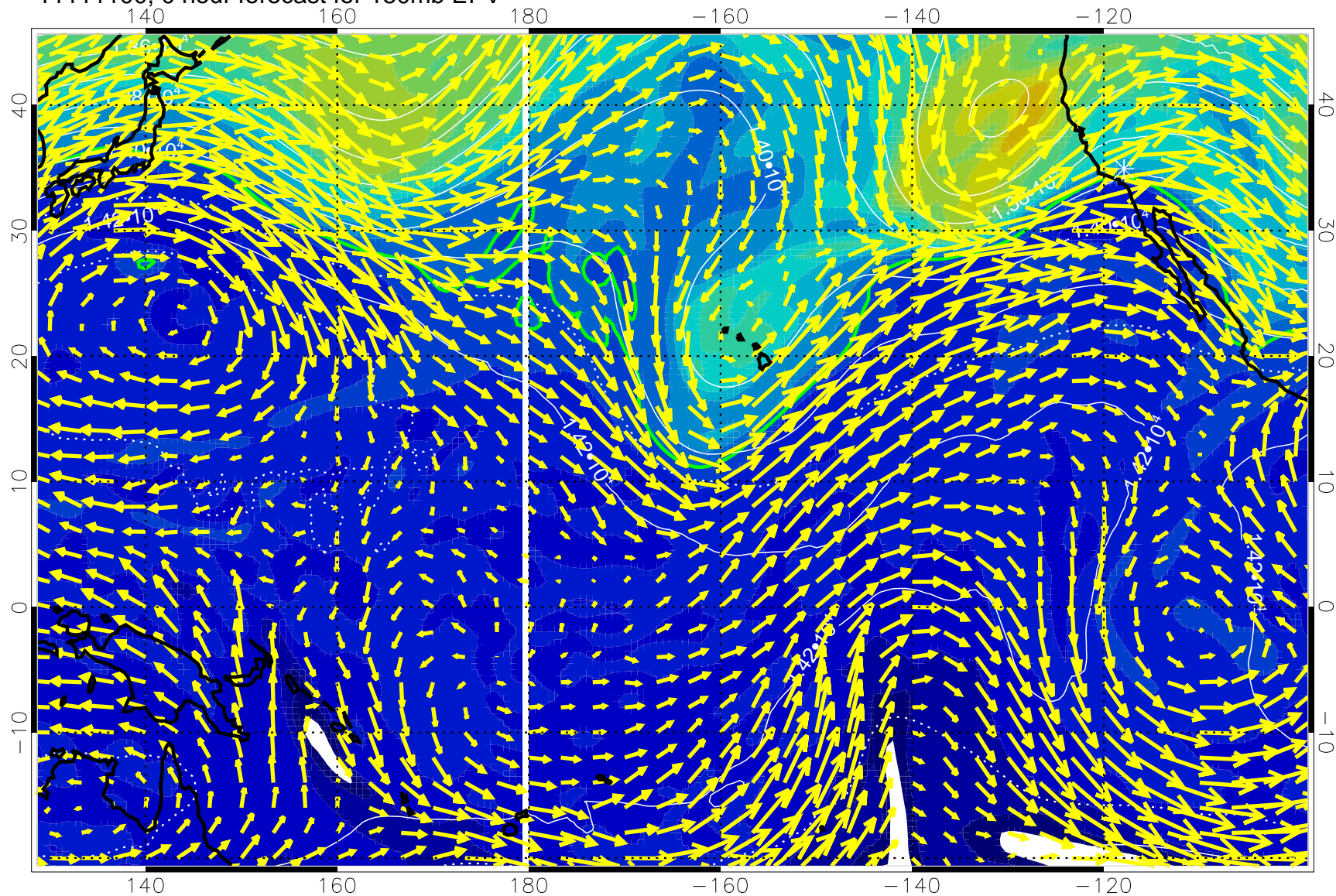
11111100, 0 hour forecast for 150mb EPV
