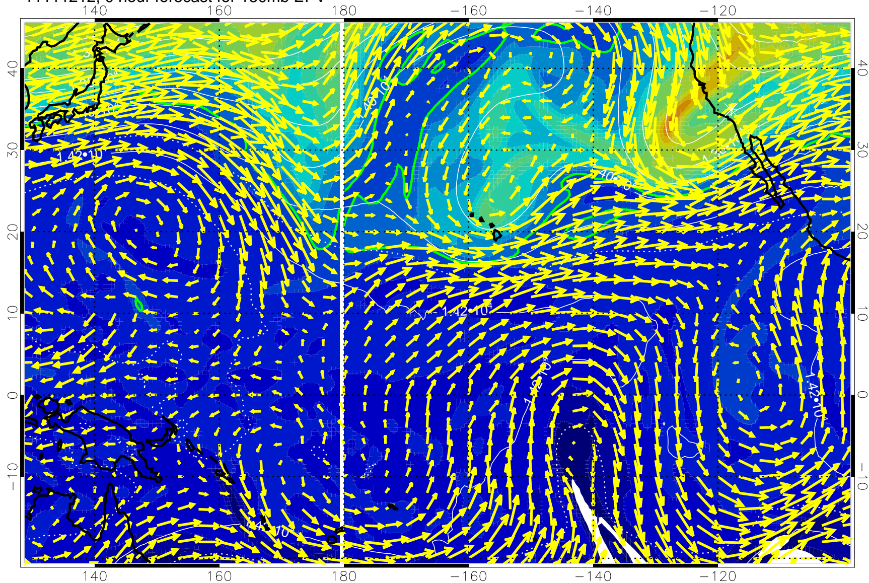
11111212, 0 hour forecast for 150mb EPV
