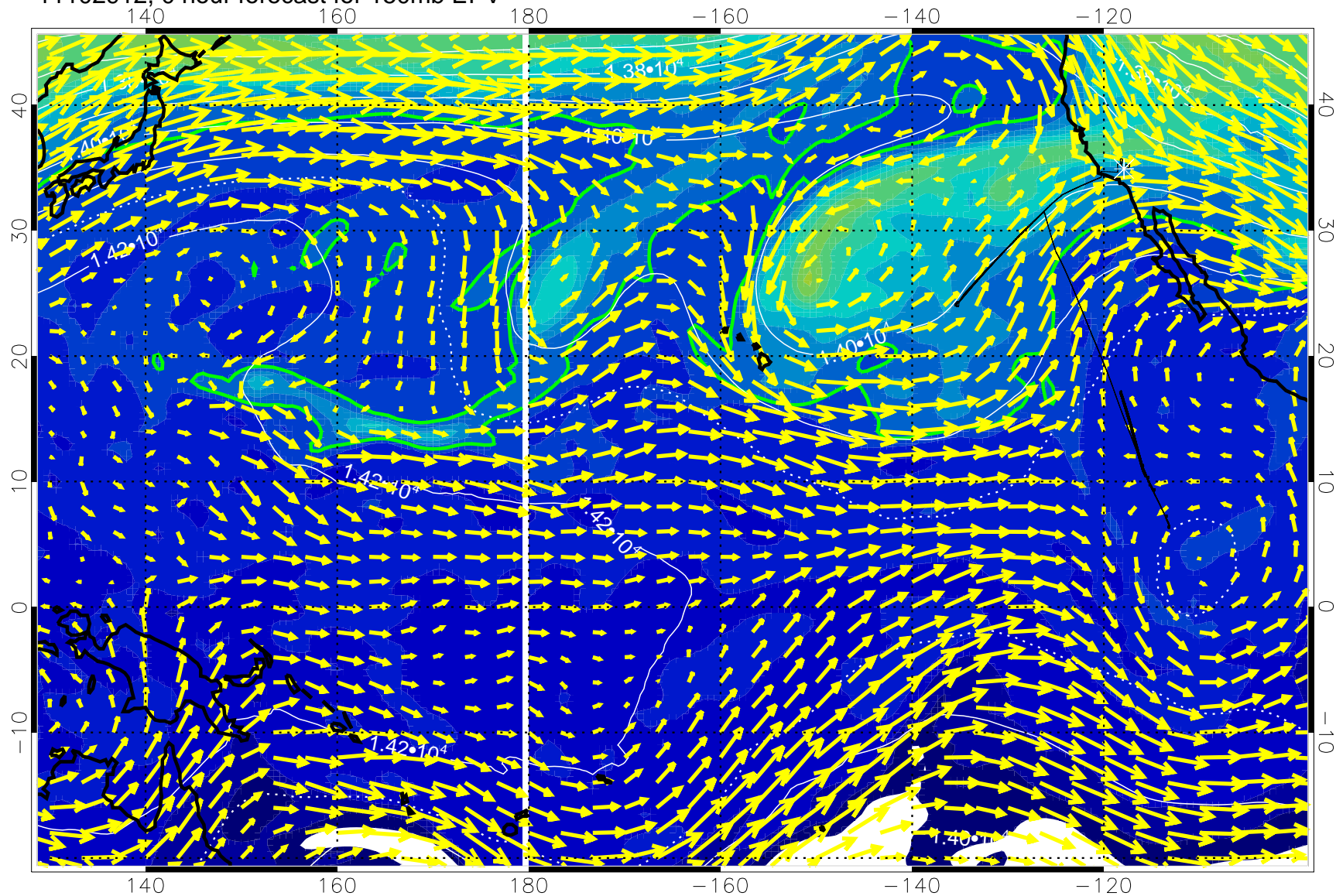
11102912, 0 hour forecast for 150mb EPV
