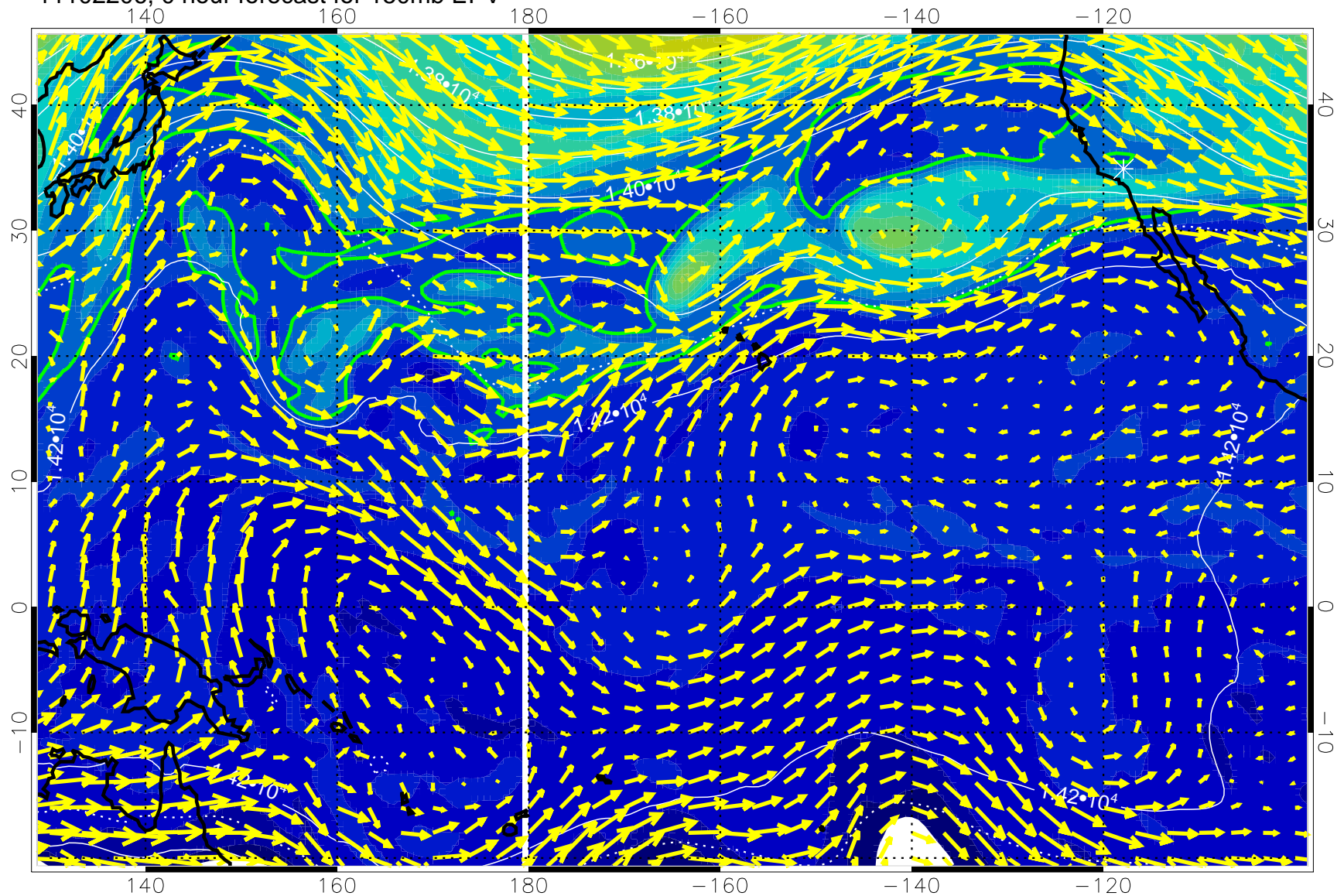
11102206, 0 hour forecast for 150mb EPV
