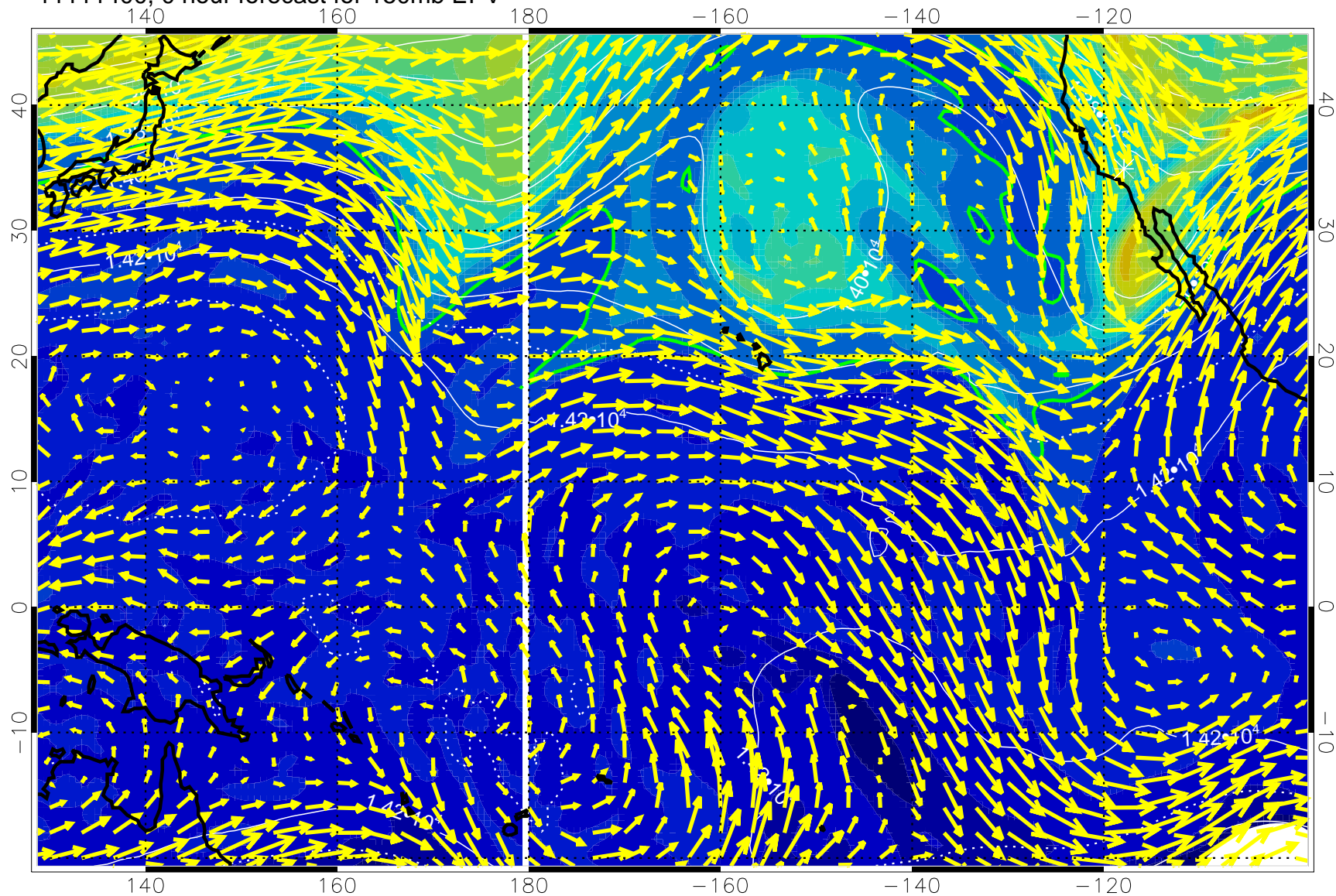
11111400, 0 hour forecast for 150mb EPV
