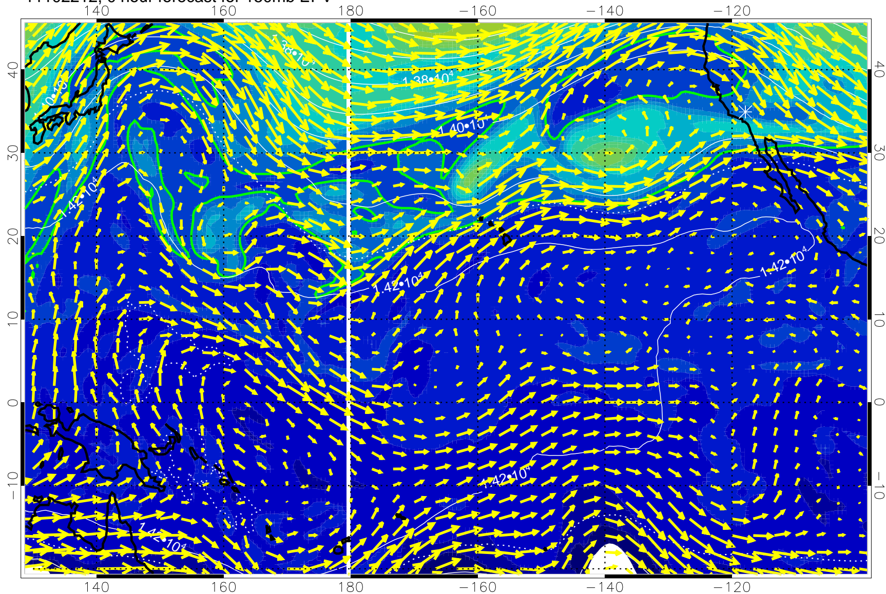
11102212, 0 hour forecast for 150mb EPV
