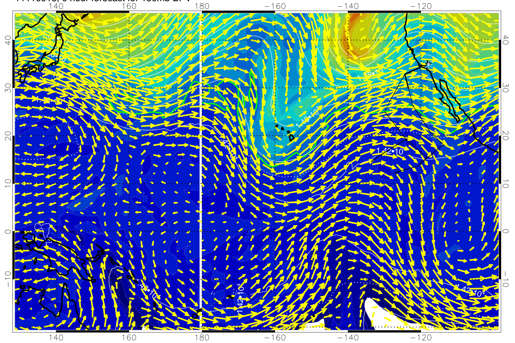
11110918, 0 hour forecast for 150mb EPV
