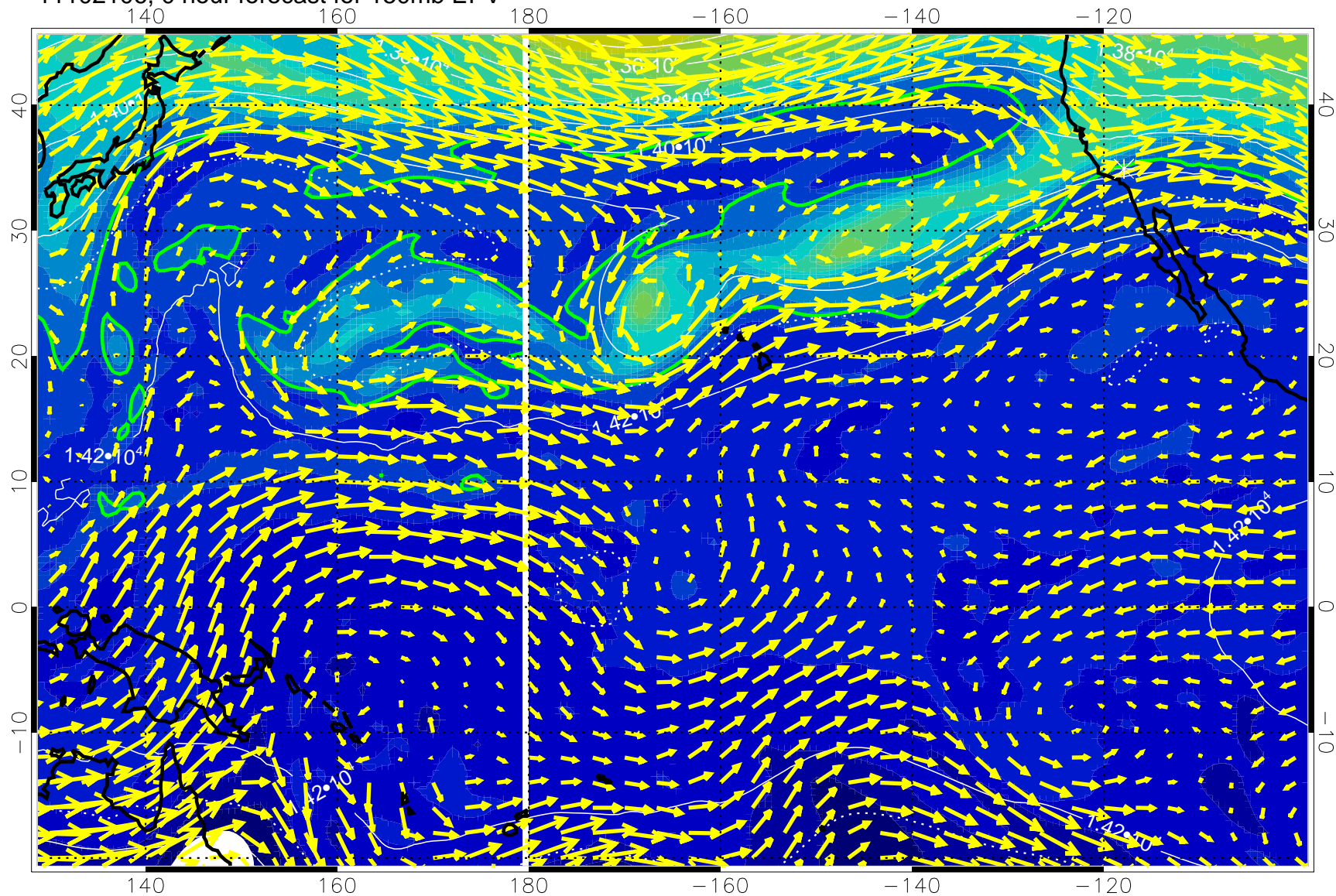
11102106, 0 hour forecast for 150mb EPV
