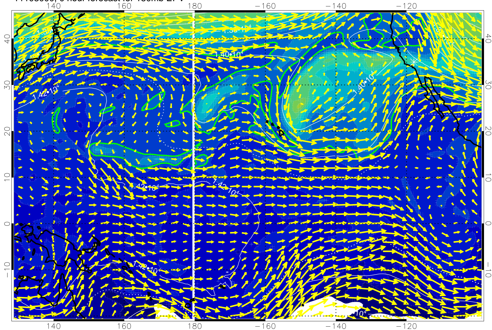
11103000, 0 hour forecast for 150mb EPV
