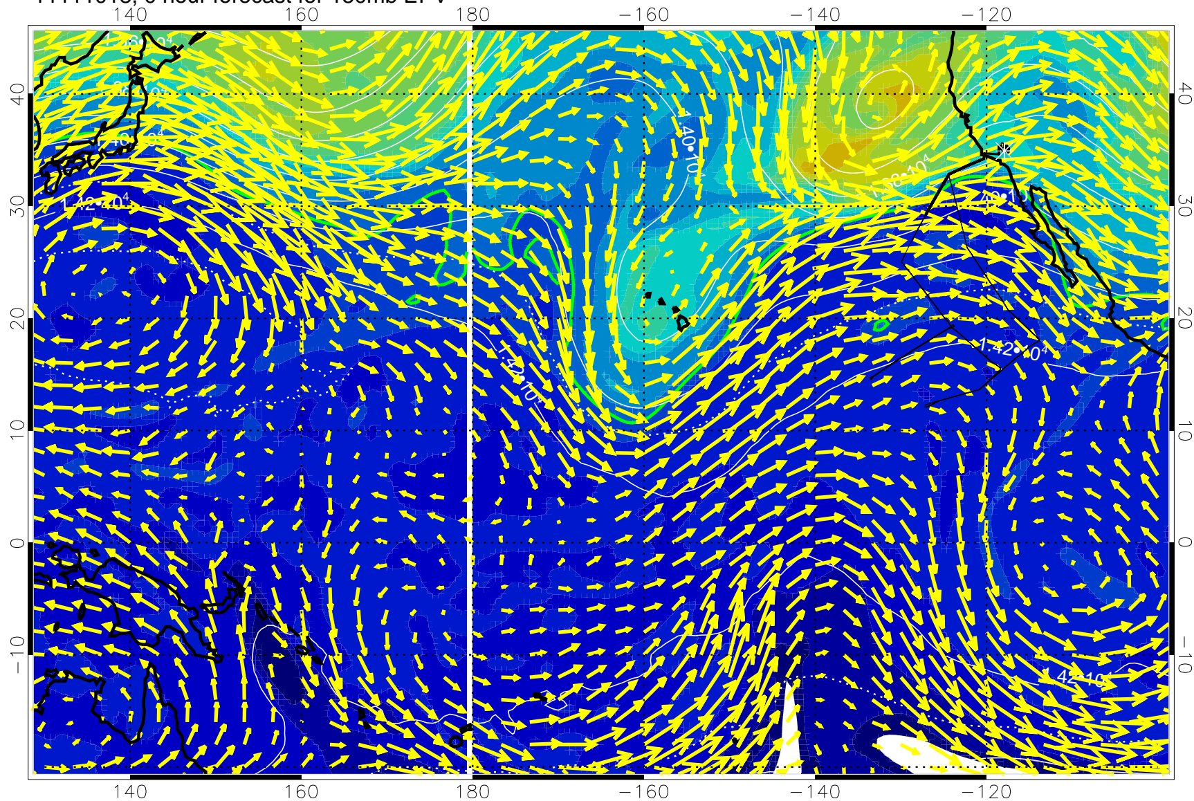
11111018, 0 hour forecast for 150mb EPV
