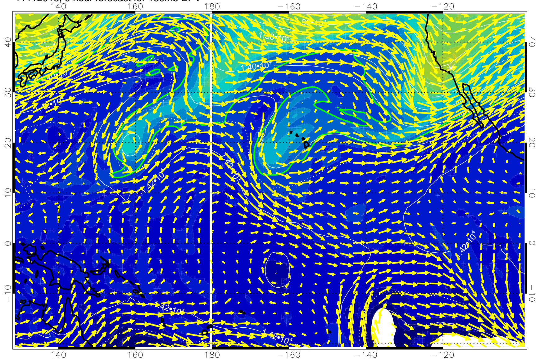
11112018, 0 hour forecast for 150mb EPV
