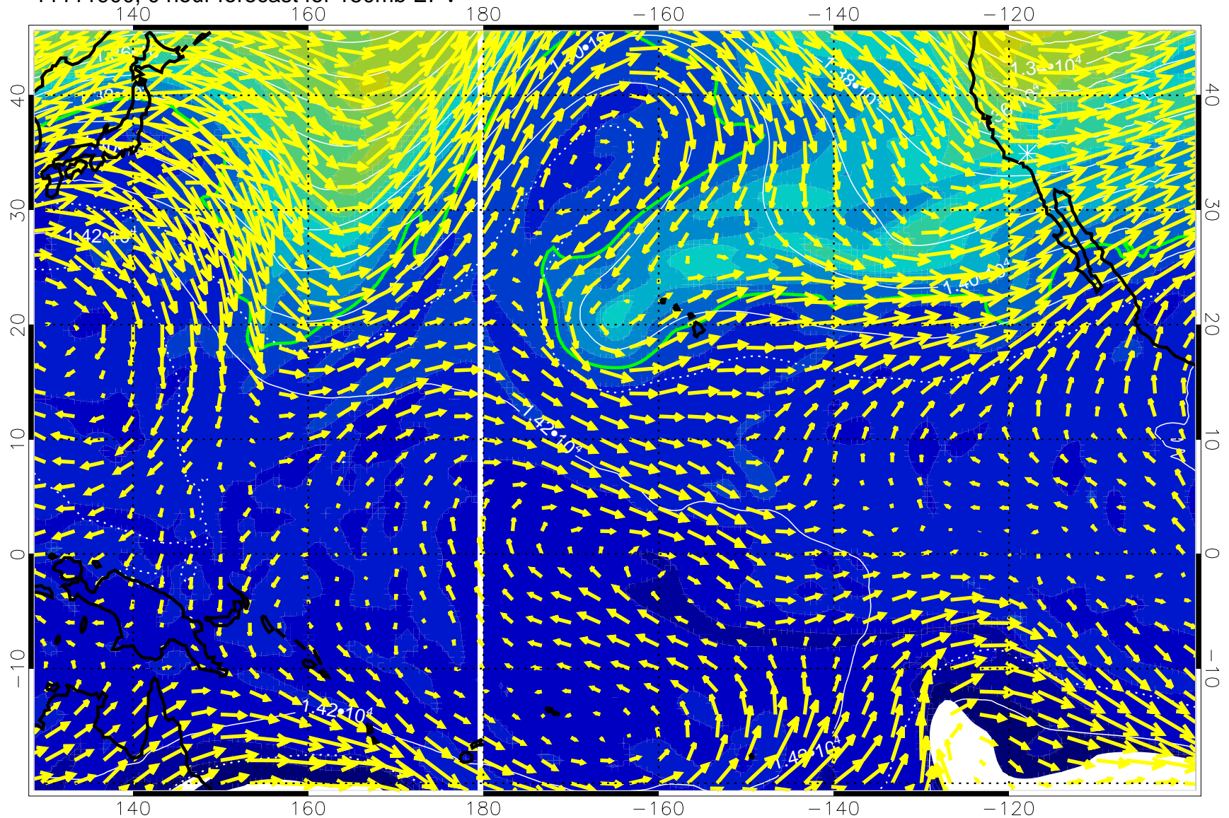
11111900, 0 hour forecast for 150mb EPV
