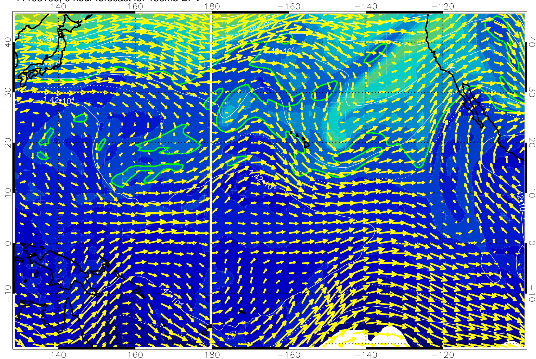
11103106, 0 hour forecast for 150mb EPV
