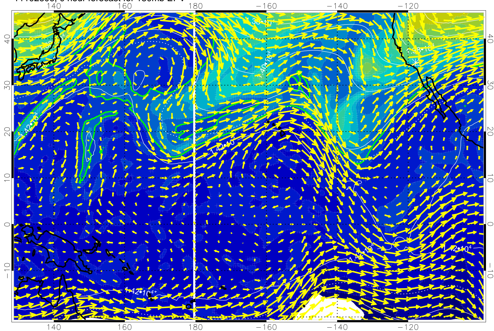
11102606, 0 hour forecast for 150mb EPV
