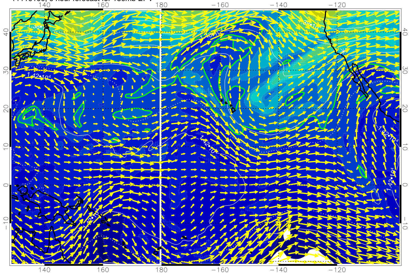
11110100, 0 hour forecast for 150mb EPV
