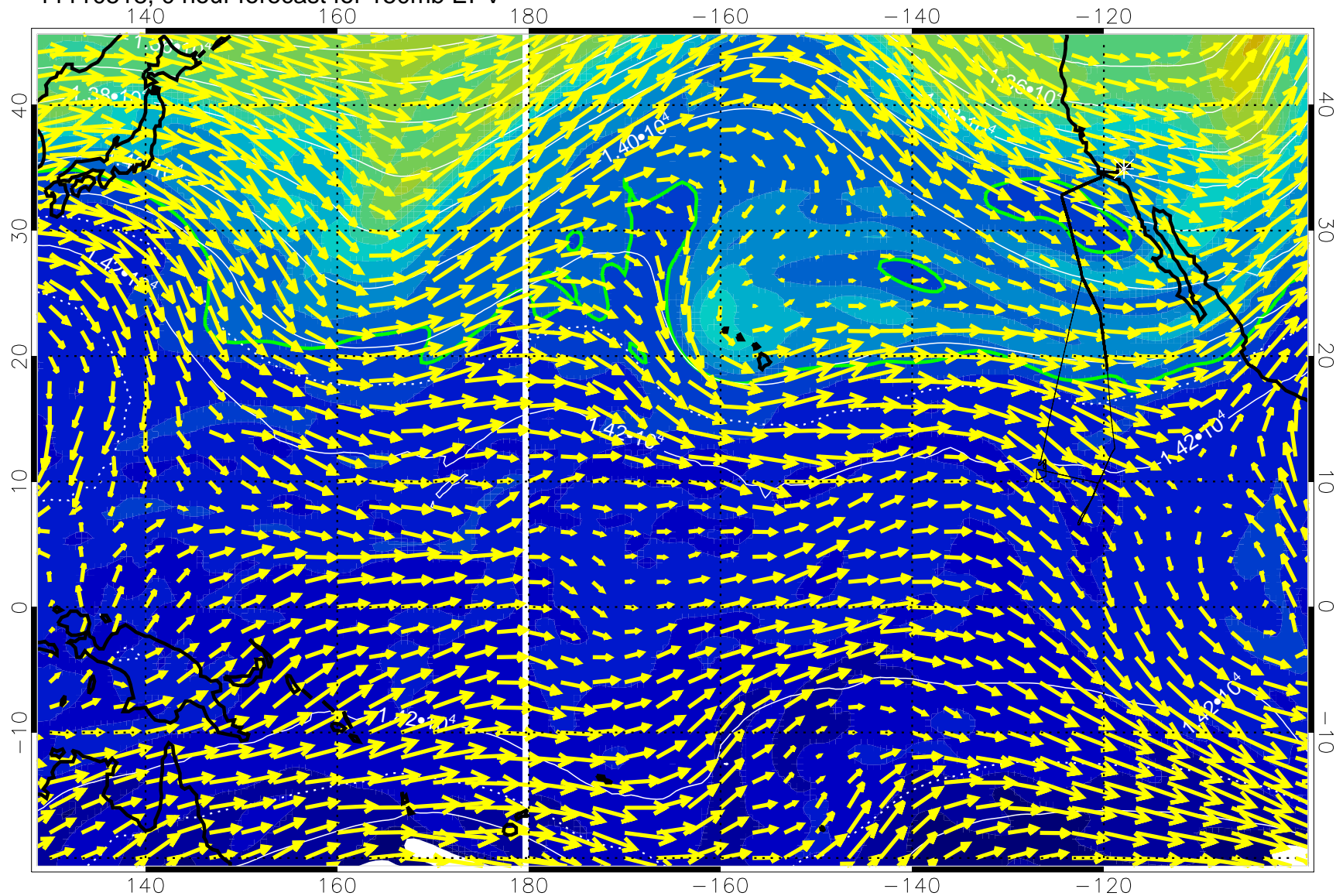
11110518, 0 hour forecast for 150mb EPV
