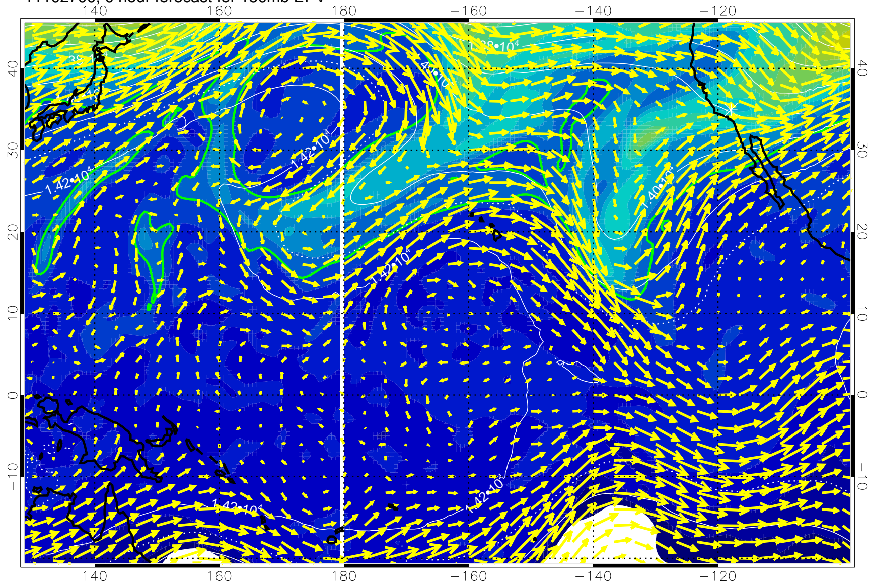
11102700, 0 hour forecast for 150mb EPV
