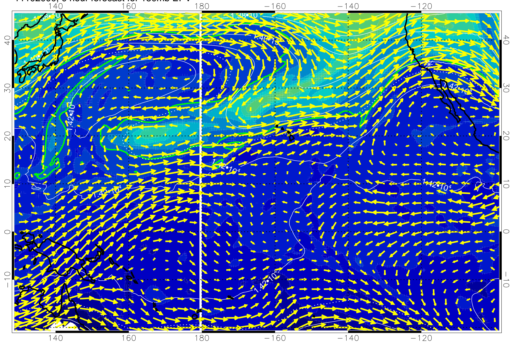
11102000, 0 hour forecast for 150mb EPV
