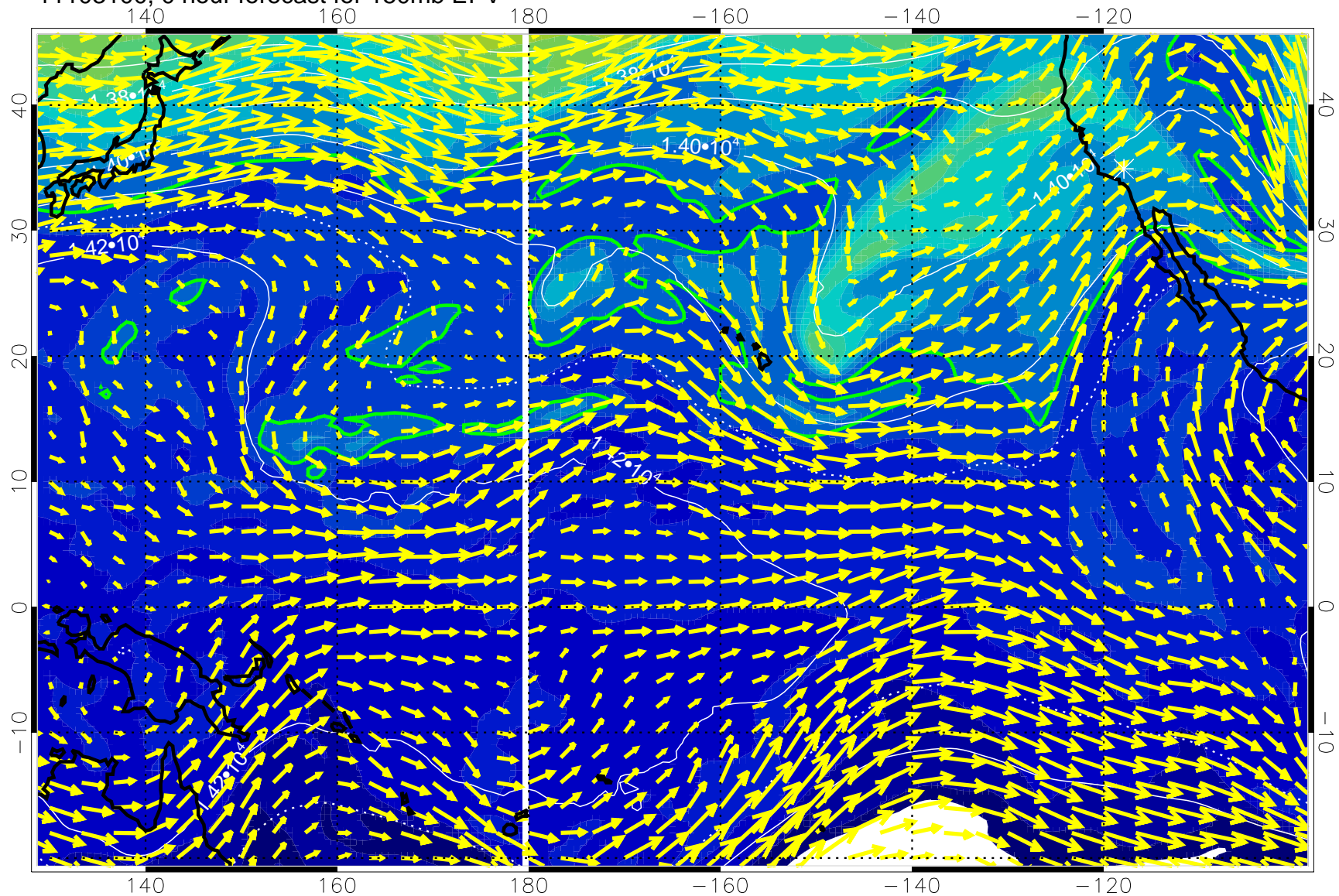
11103100, 0 hour forecast for 150mb EPV
