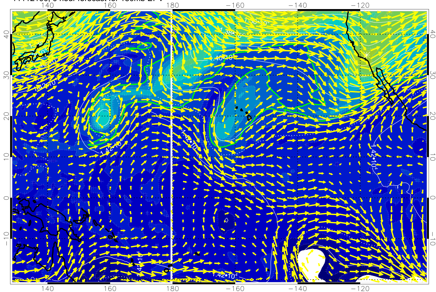
11112100, 0 hour forecast for 150mb EPV
