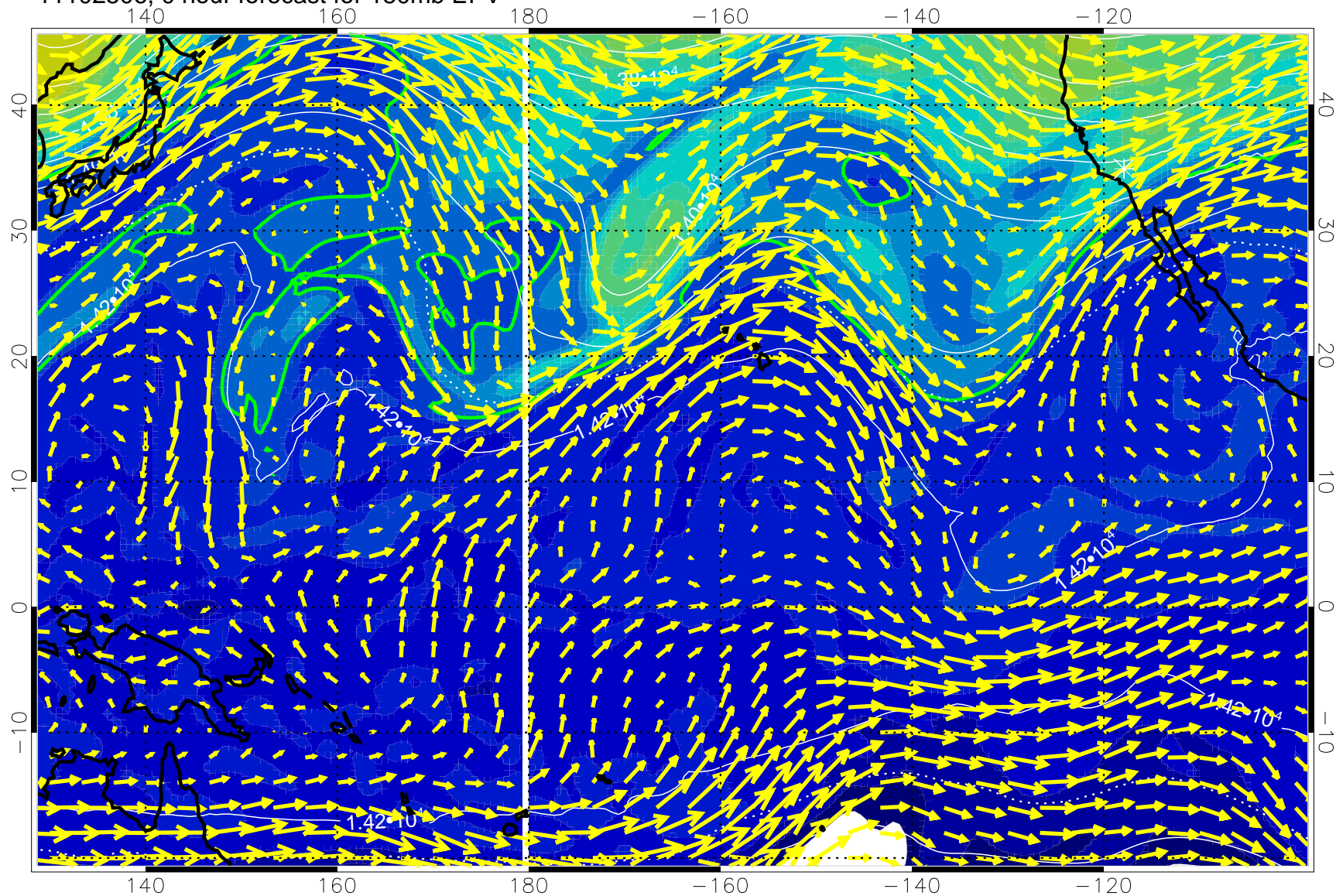
11102506, 0 hour forecast for 150mb EPV
