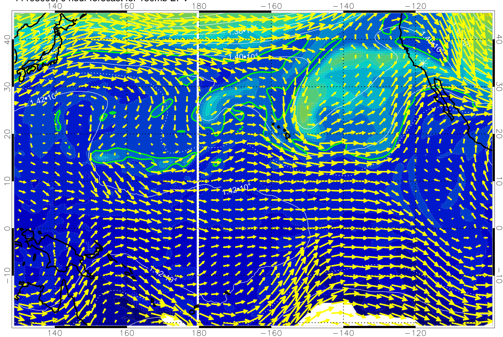
11103006, 0 hour forecast for 150mb EPV
