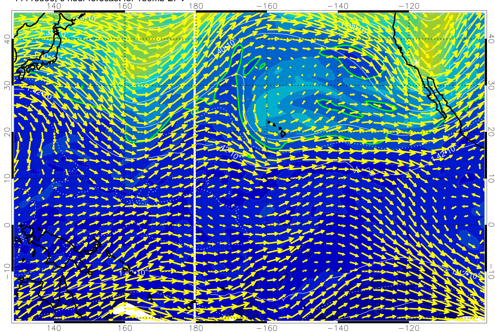
11110506, 0 hour forecast for 150mb EPV
