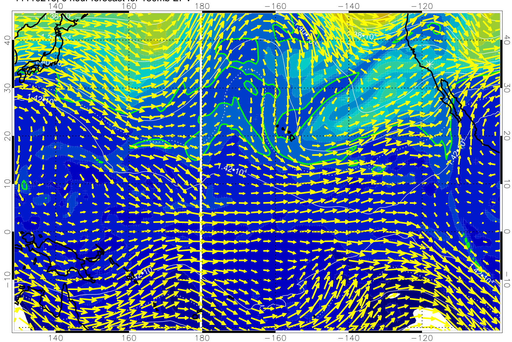
11110218, 0 hour forecast for 150mb EPV
