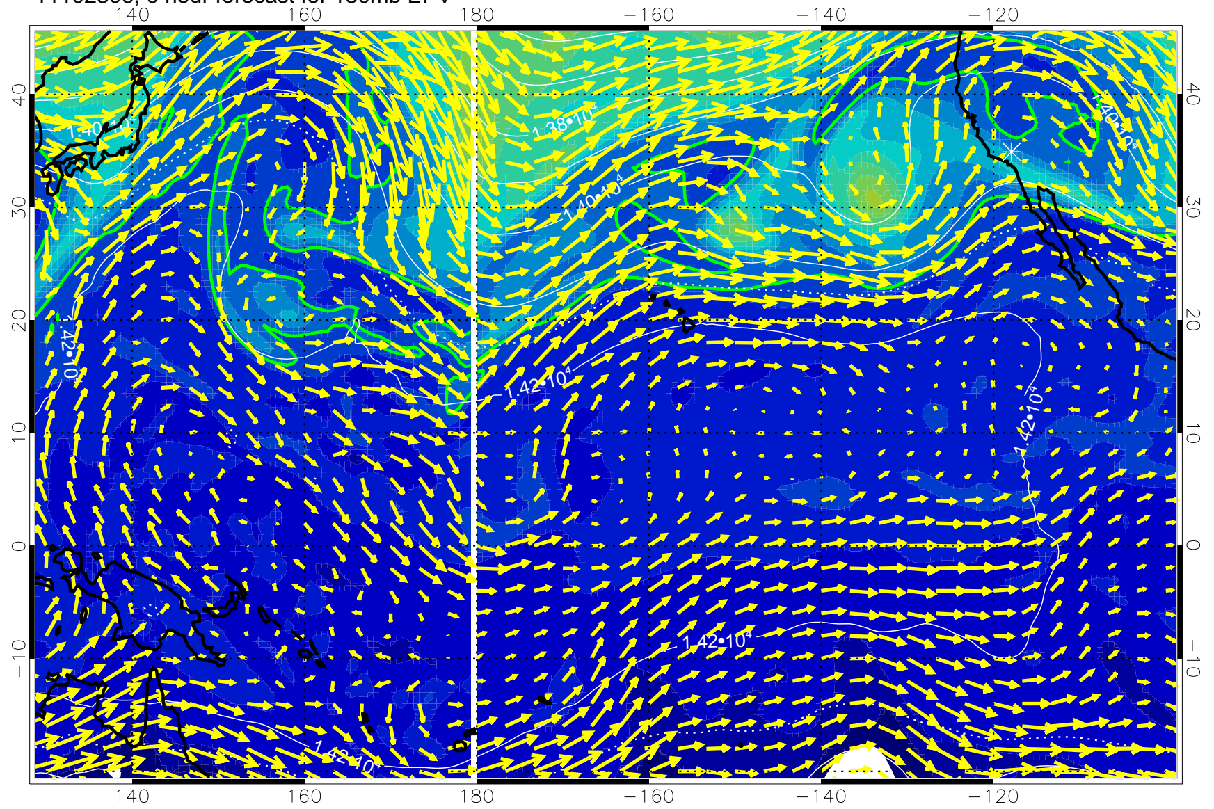
11102306, 0 hour forecast for 150mb EPV
