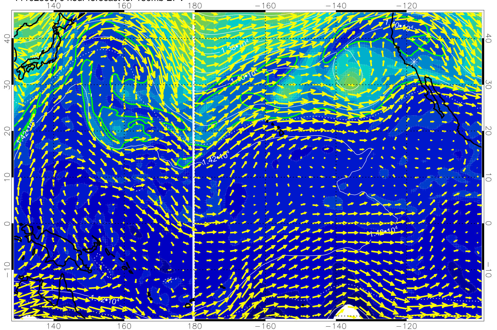
11102300, 0 hour forecast for 150mb EPV
