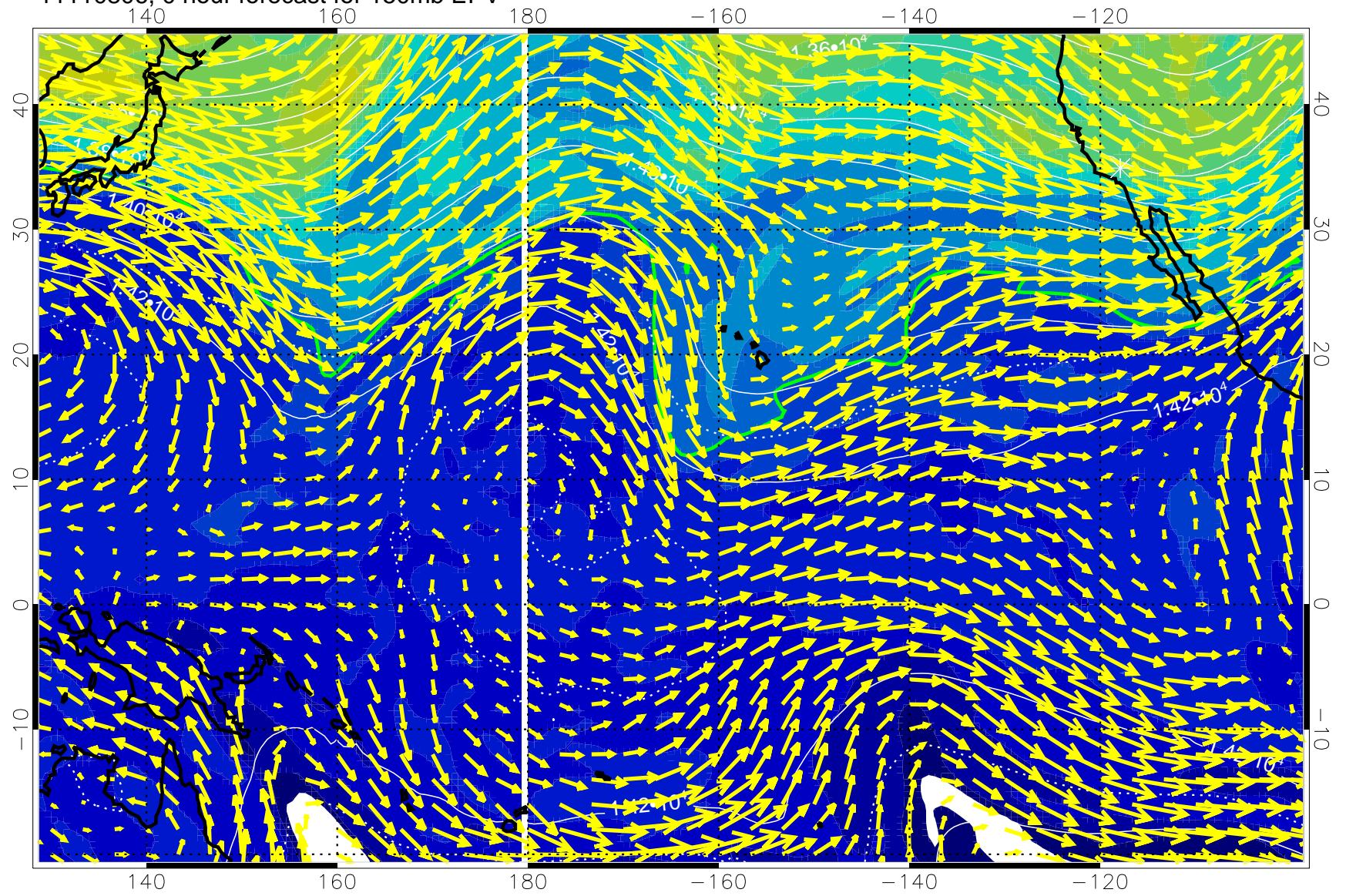
11110806, 0 hour forecast for 150mb EPV
