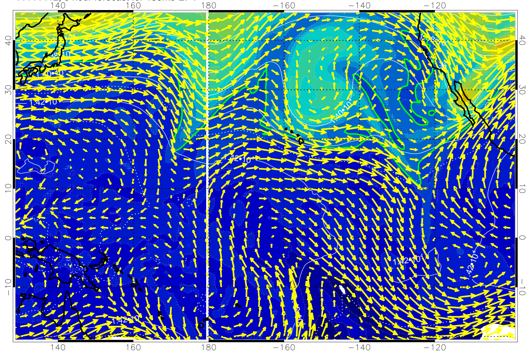
11111412, 0 hour forecast for 150mb EPV
