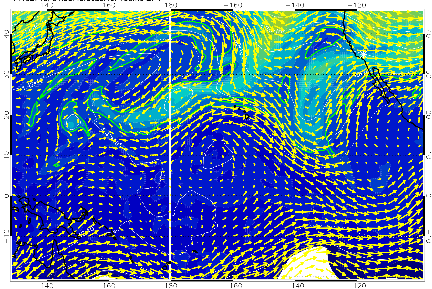
11102718, 0 hour forecast for 150mb EPV
