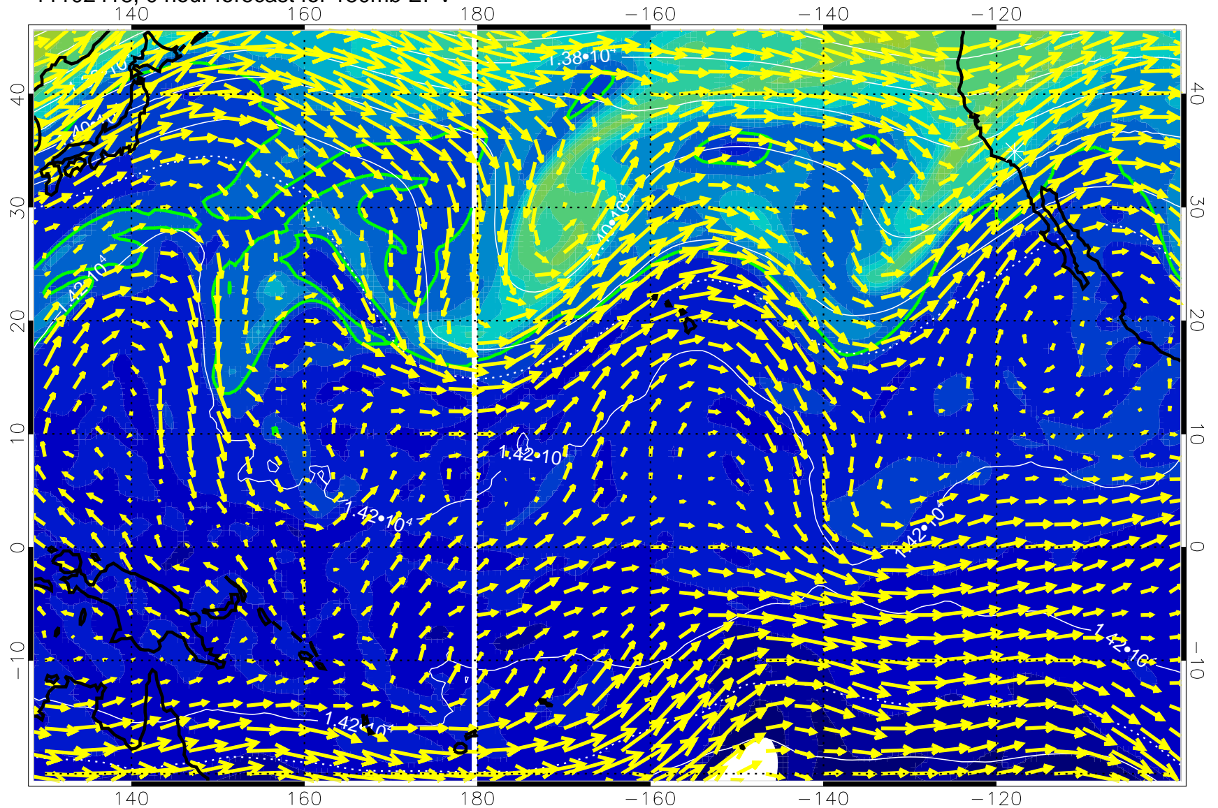
11102418, 0 hour forecast for 150mb EPV
