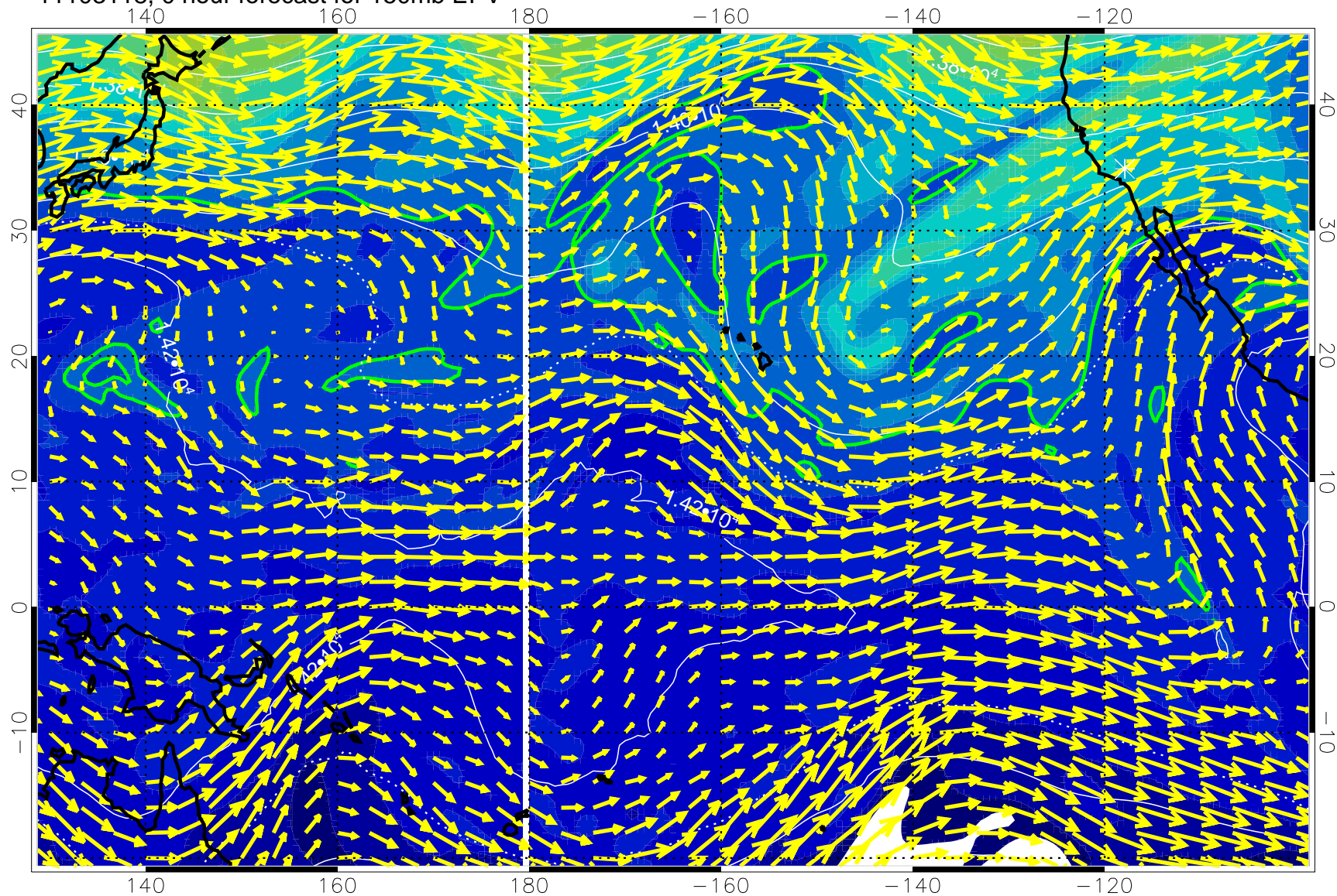
11103118, 0 hour forecast for 150mb EPV
