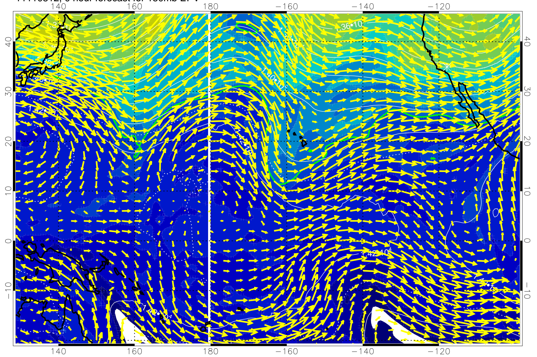
11110812, 0 hour forecast for 150mb EPV
