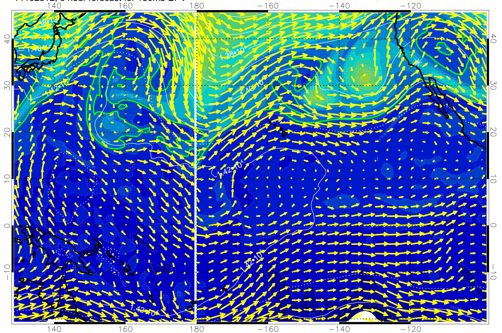
11102312, 0 hour forecast for 150mb EPV
