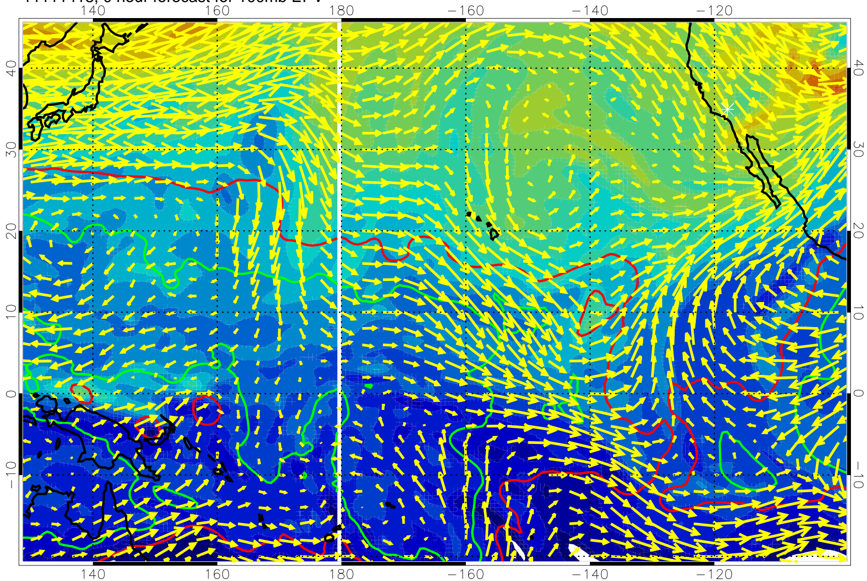
11111418, 0 hour forecast for 100mb EPV
