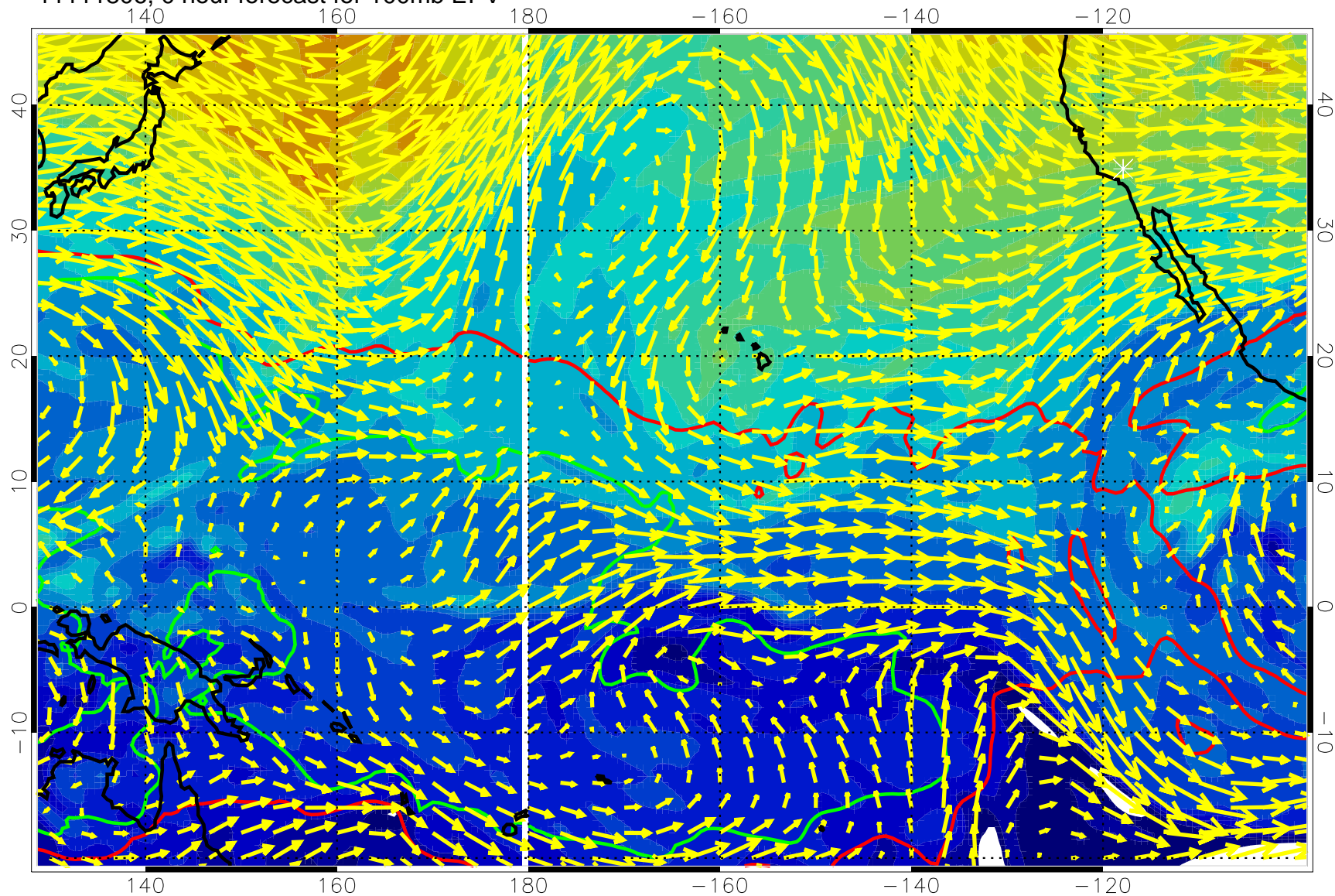
11111806, 0 hour forecast for 100mb EPV
