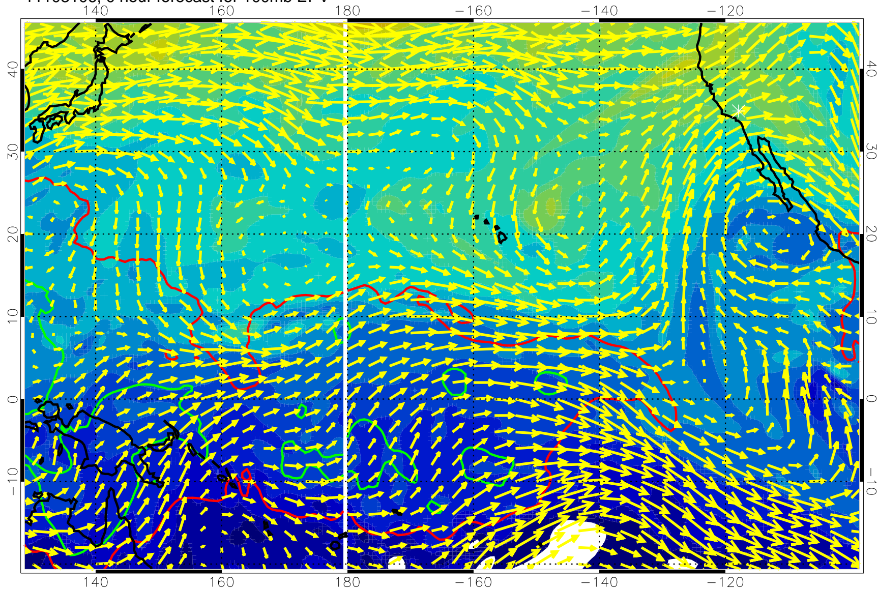
11103106, 0 hour forecast for 100mb EPV
