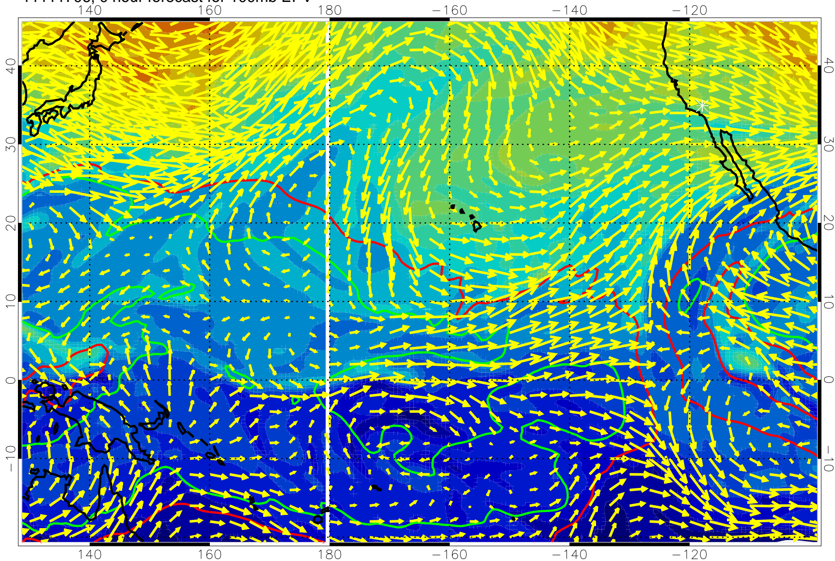
11111706, 0 hour forecast for 100mb EPV
