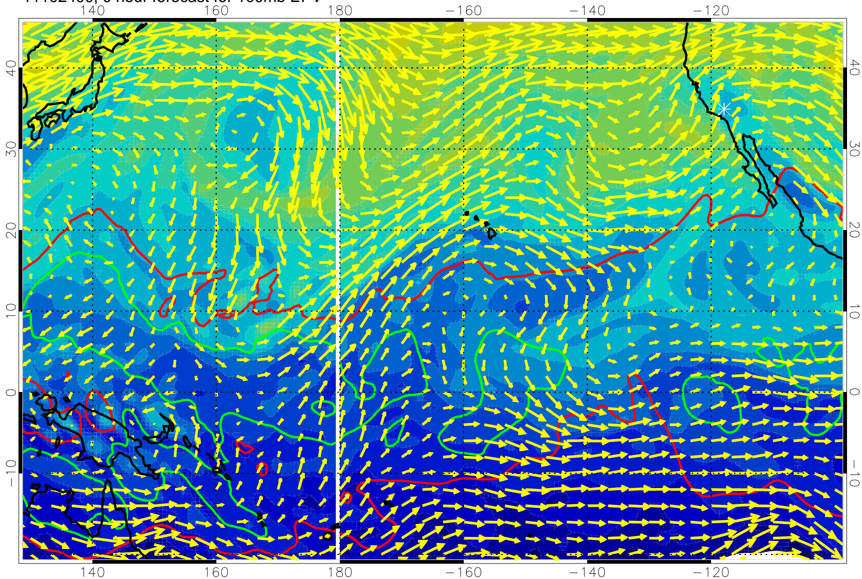
11102400, 0 hour forecast for 100mb EPV
