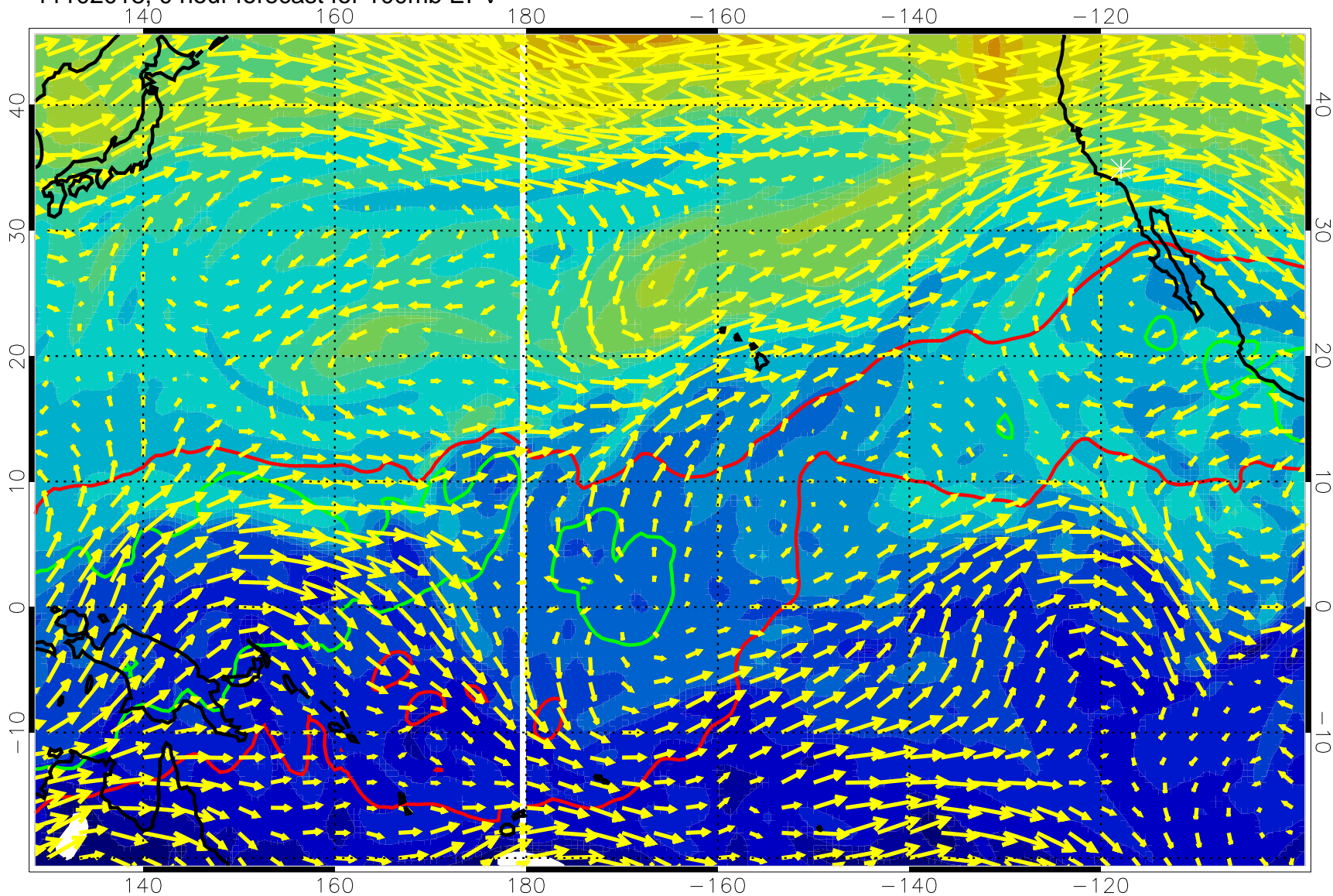
11102018, 0 hour forecast for 100mb EPV
