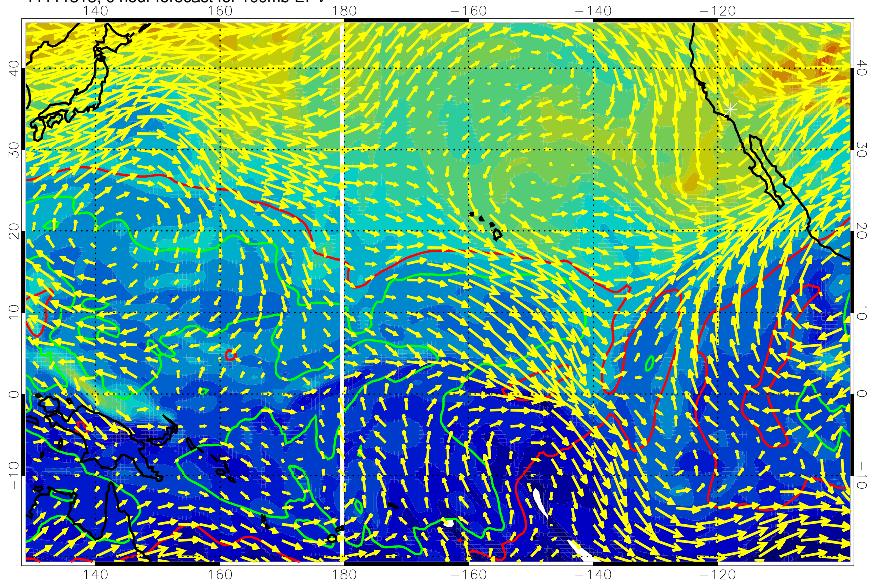
11111318, 0 hour forecast for 100mb EPV
