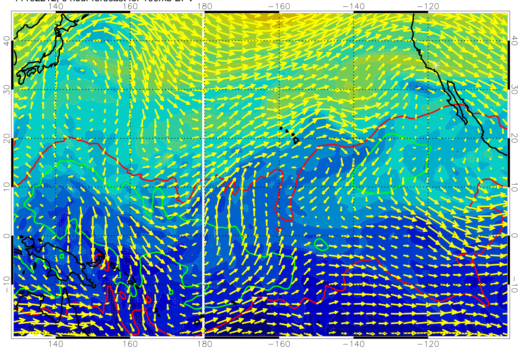
11102212, 0 hour forecast for 100mb EPV
