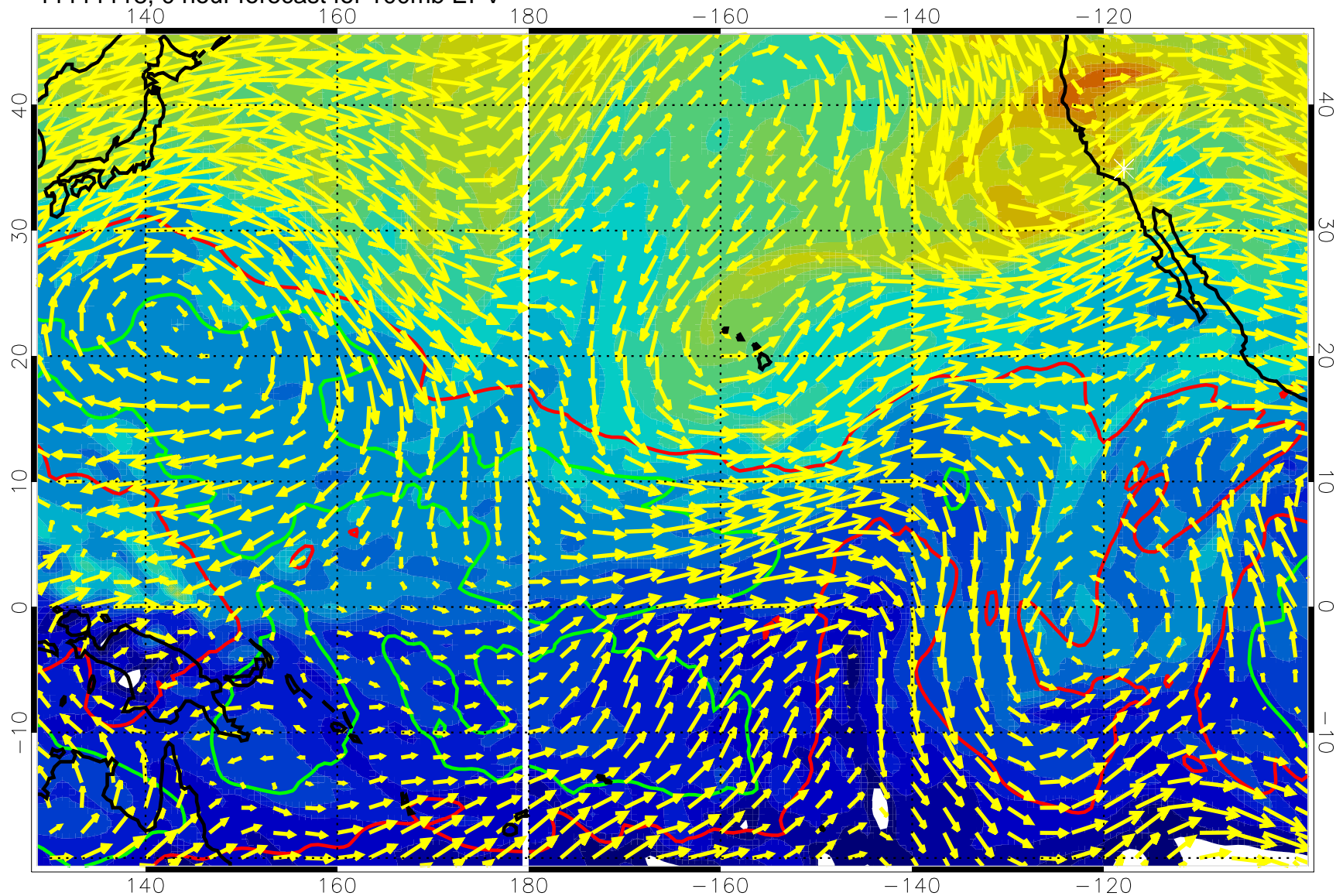
11111118, 0 hour forecast for 100mb EPV
