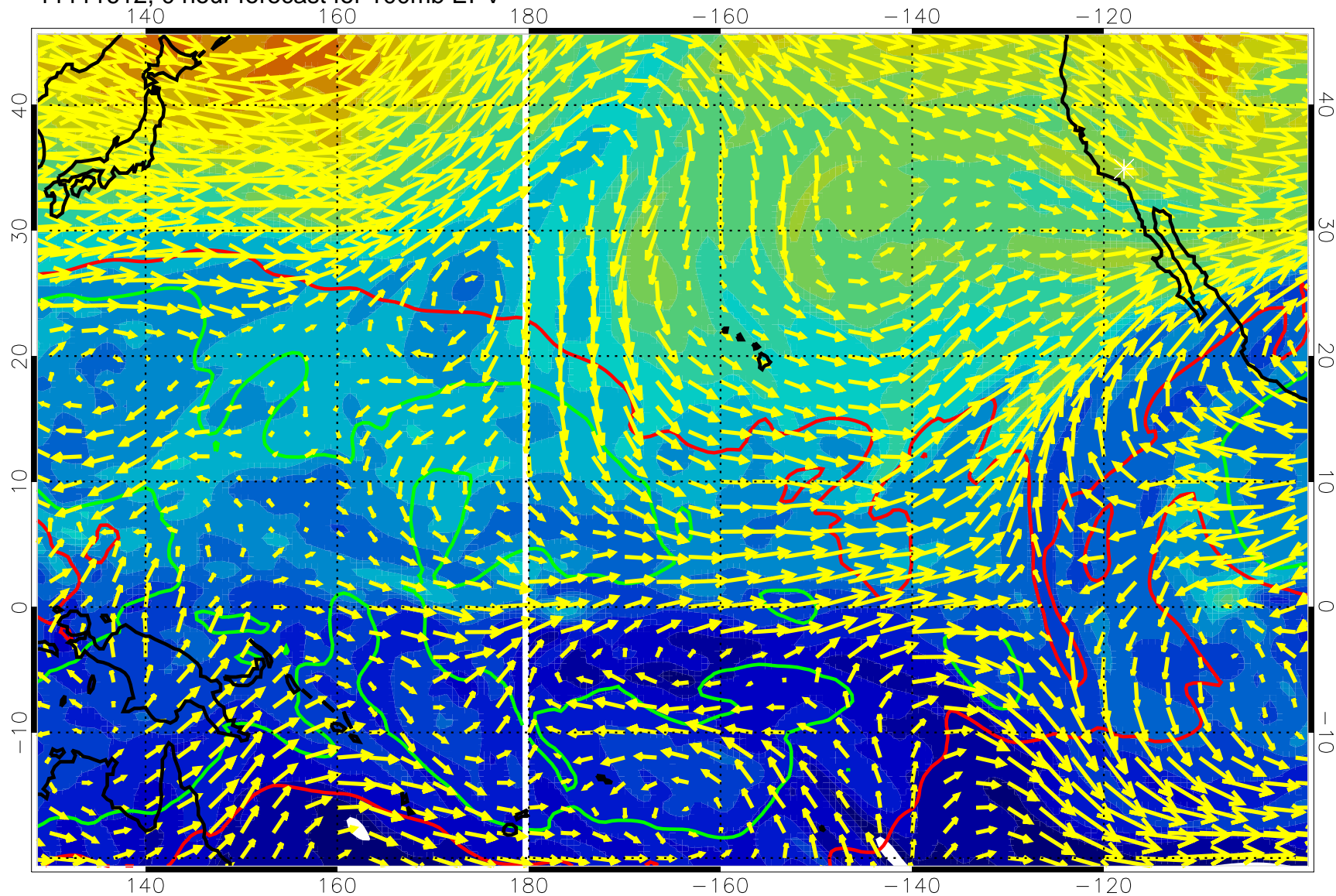
11111612, 0 hour forecast for 100mb EPV
