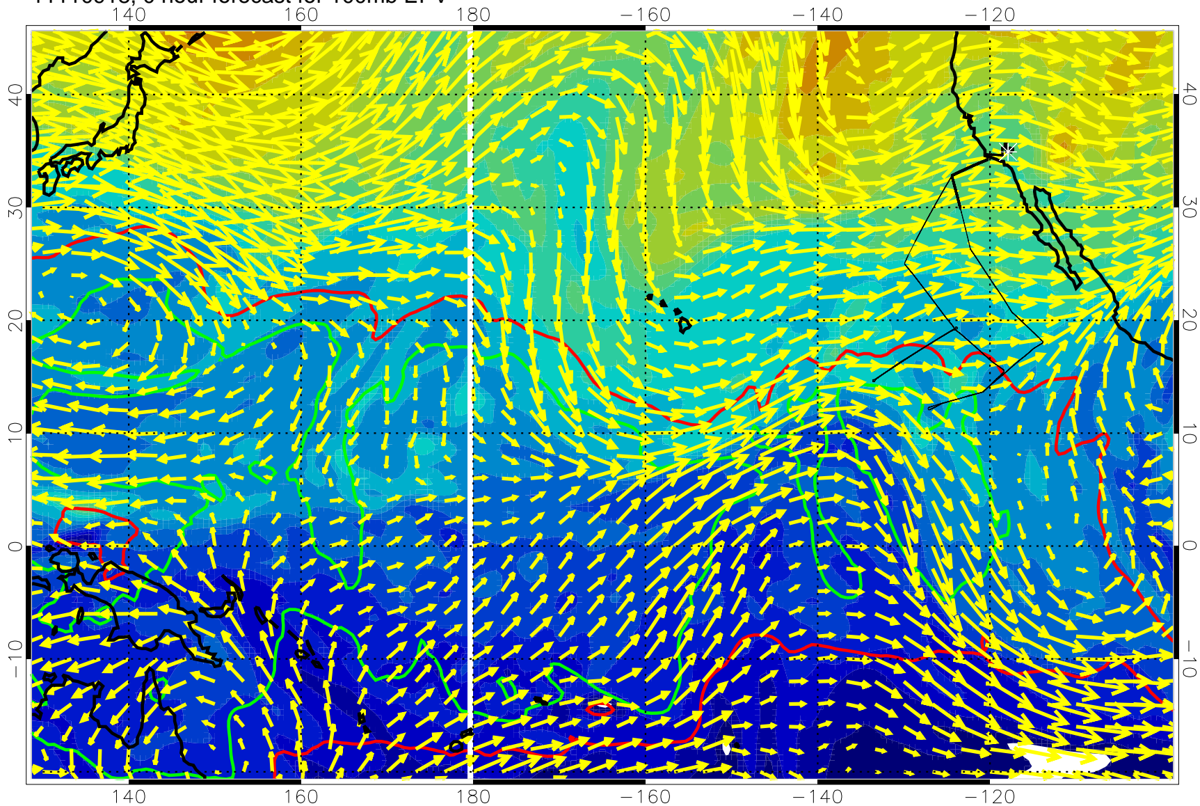
11110918, 0 hour forecast for 100mb EPV
