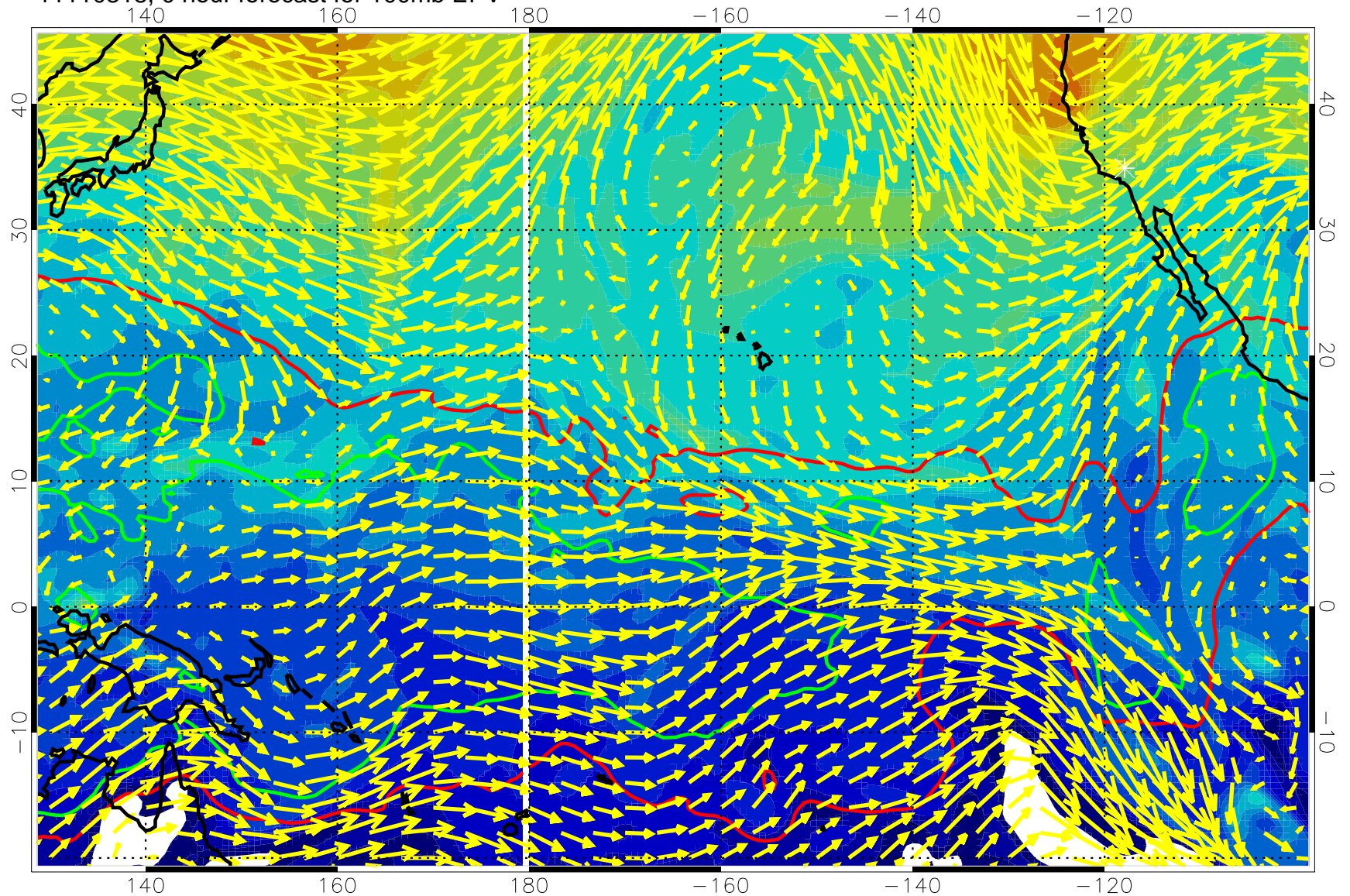
11110318, 0 hour forecast for 100mb EPV
