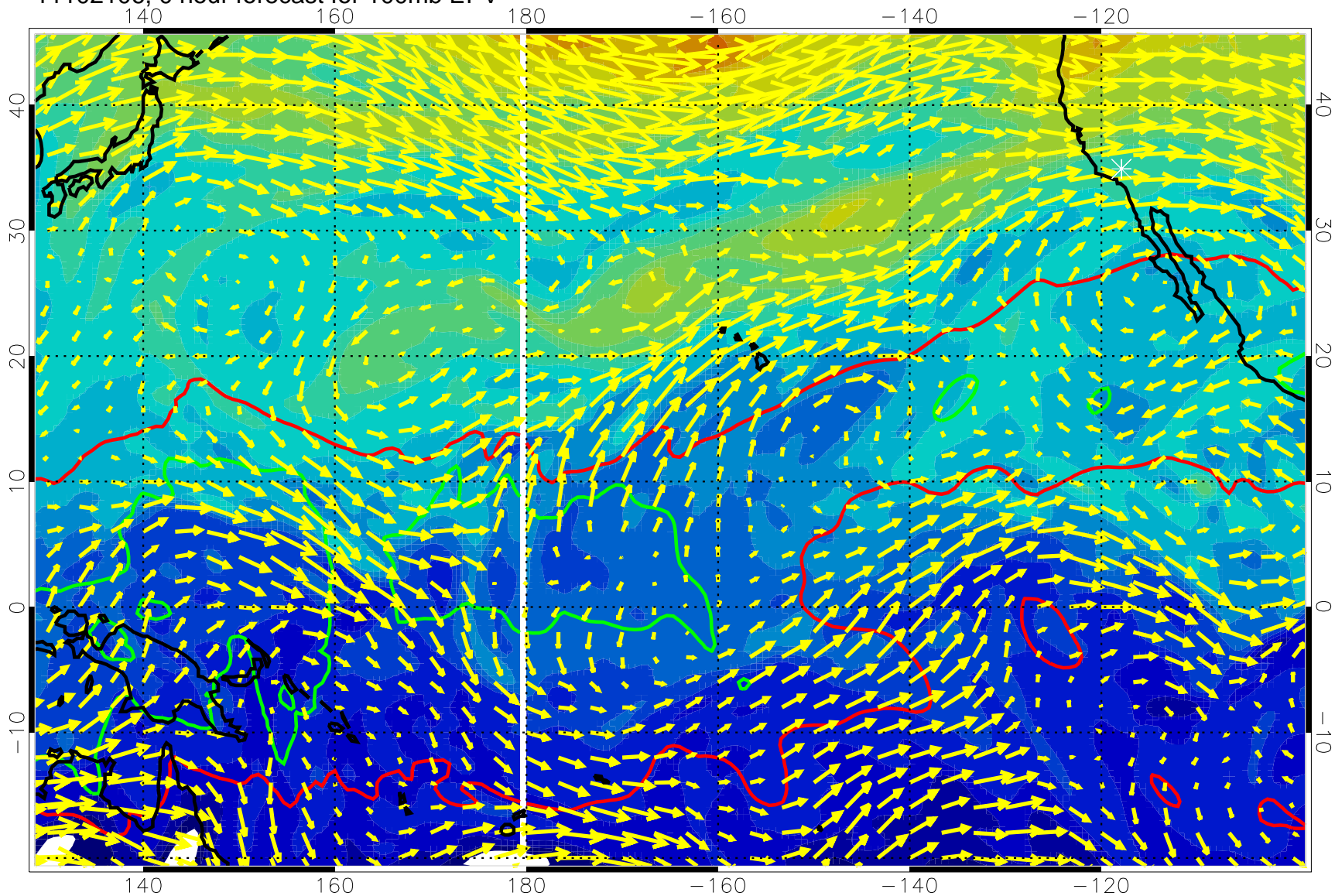
11102106, 0 hour forecast for 100mb EPV
