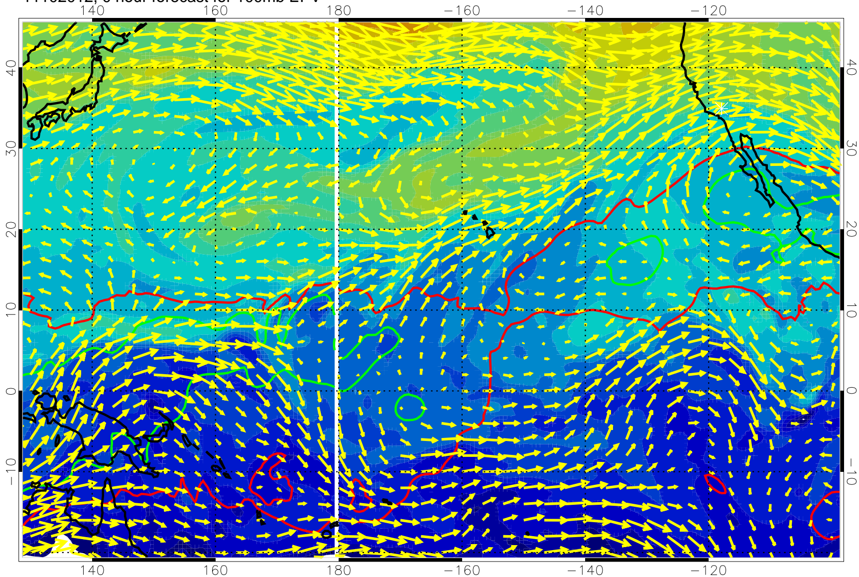
11102012, 0 hour forecast for 100mb EPV
