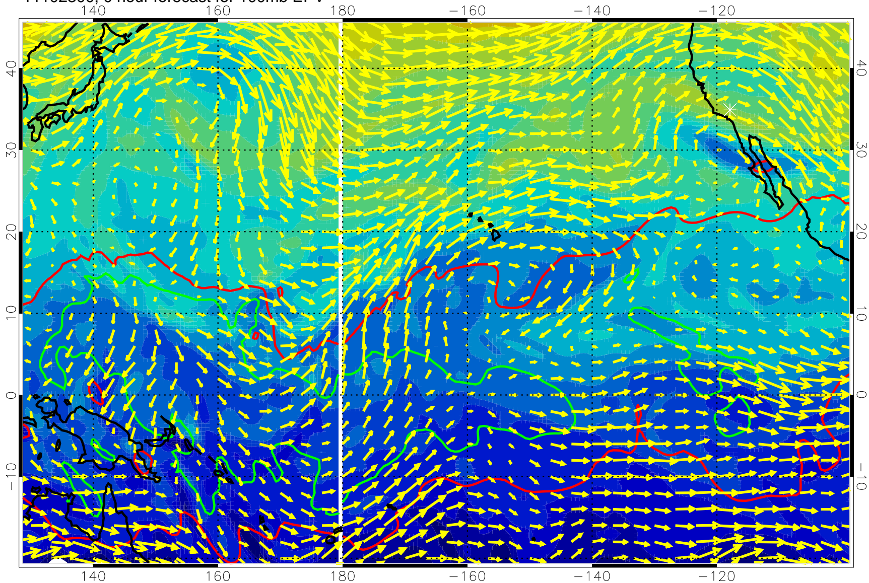
11102300, 0 hour forecast for 100mb EPV
