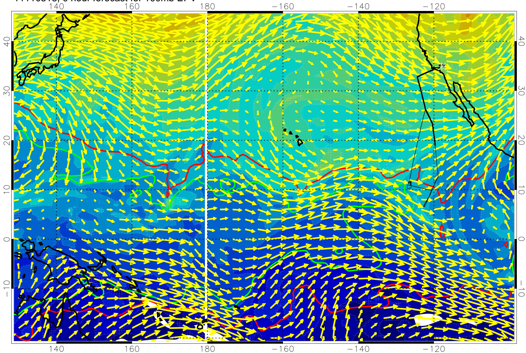
11110518, 0 hour forecast for 100mb EPV
