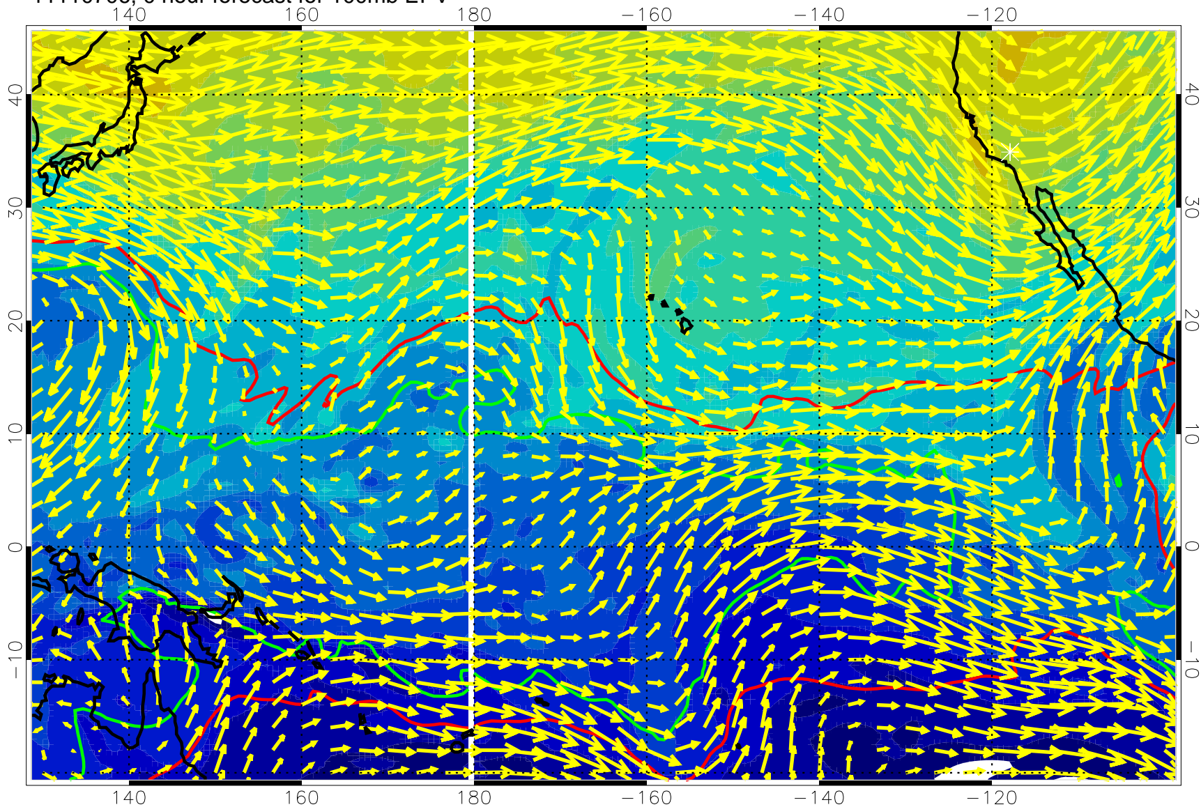
11110706, 0 hour forecast for 100mb EPV
