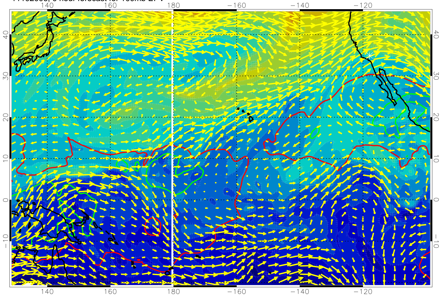
11102006, 0 hour forecast for 100mb EPV
