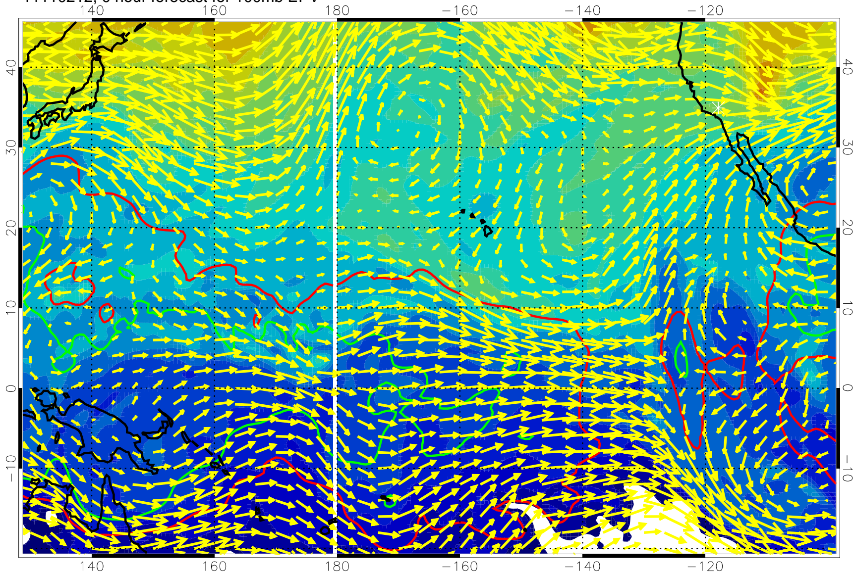
11110212, 0 hour forecast for 100mb EPV
