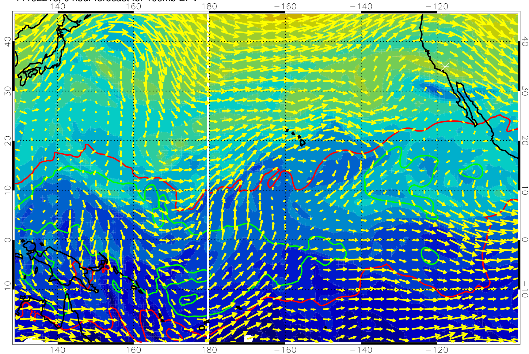
11102218, 0 hour forecast for 100mb EPV
