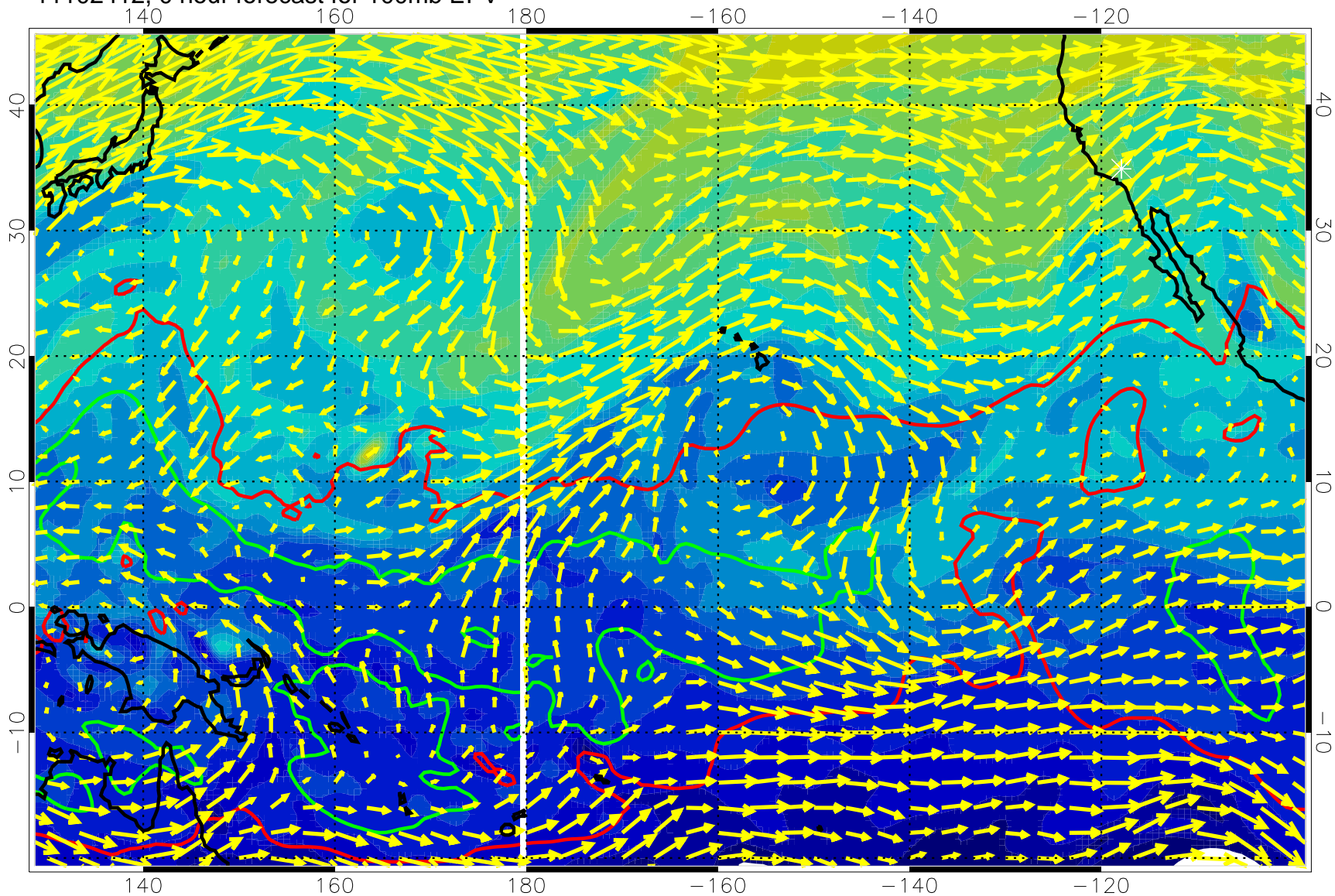
11102412, 0 hour forecast for 100mb EPV
