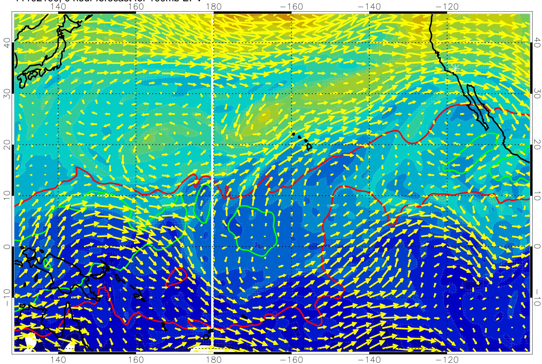
11102100, 0 hour forecast for 100mb EPV
