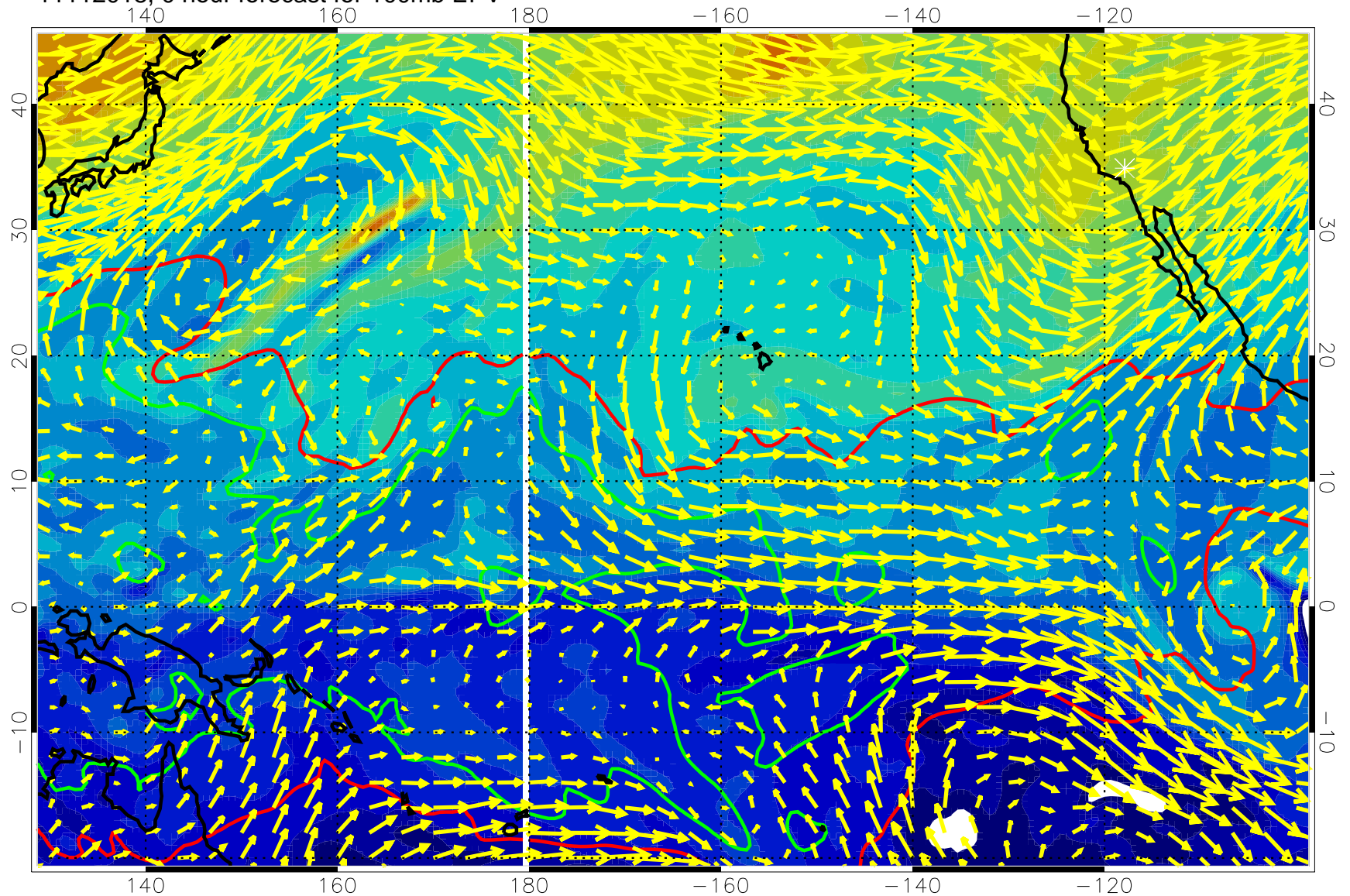
11112018, 0 hour forecast for 100mb EPV
