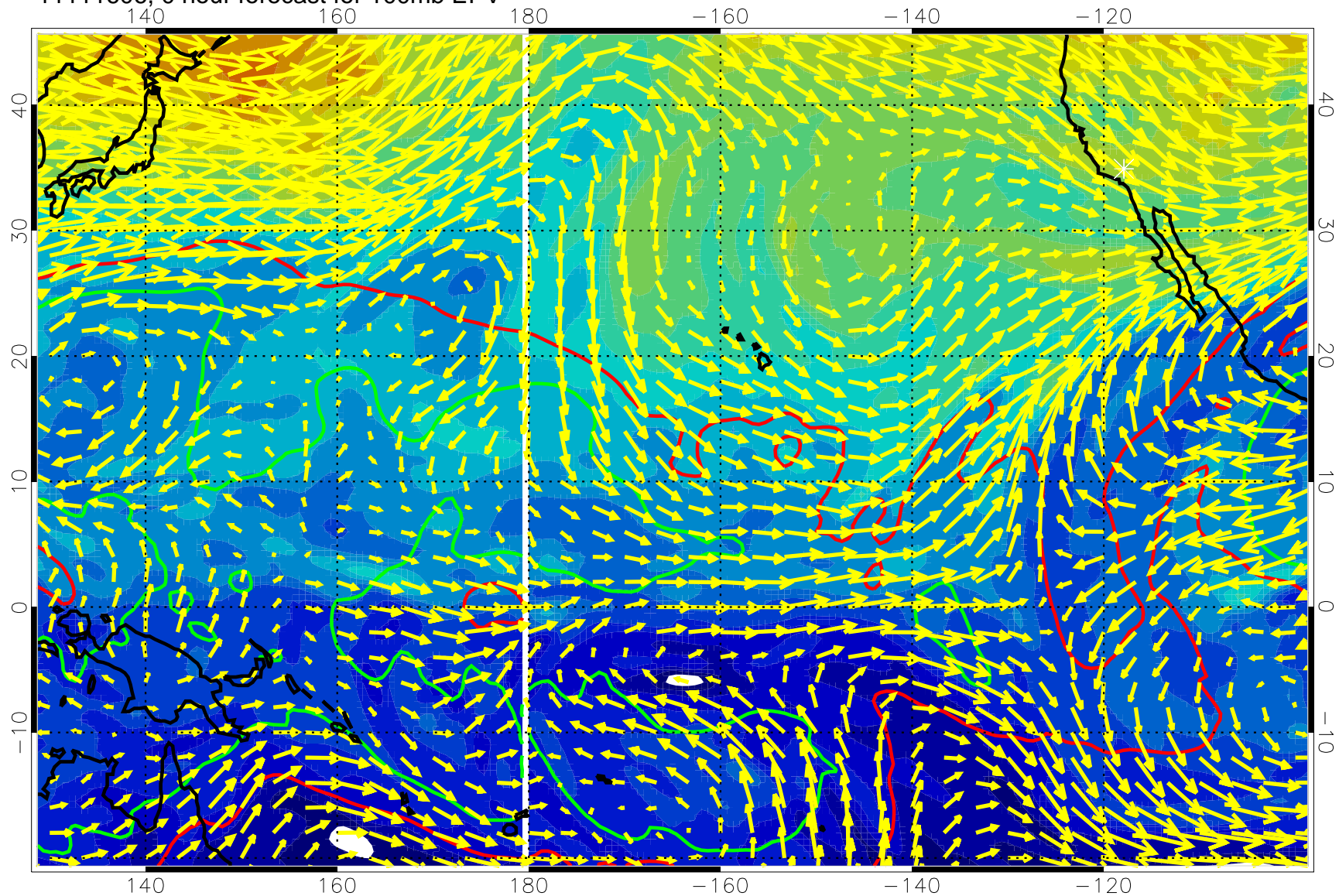
11111606, 0 hour forecast for 100mb EPV
