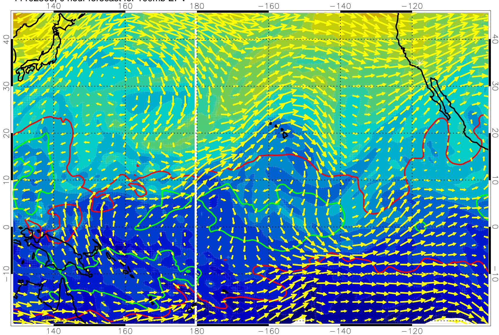
11102506, 0 hour forecast for 100mb EPV
