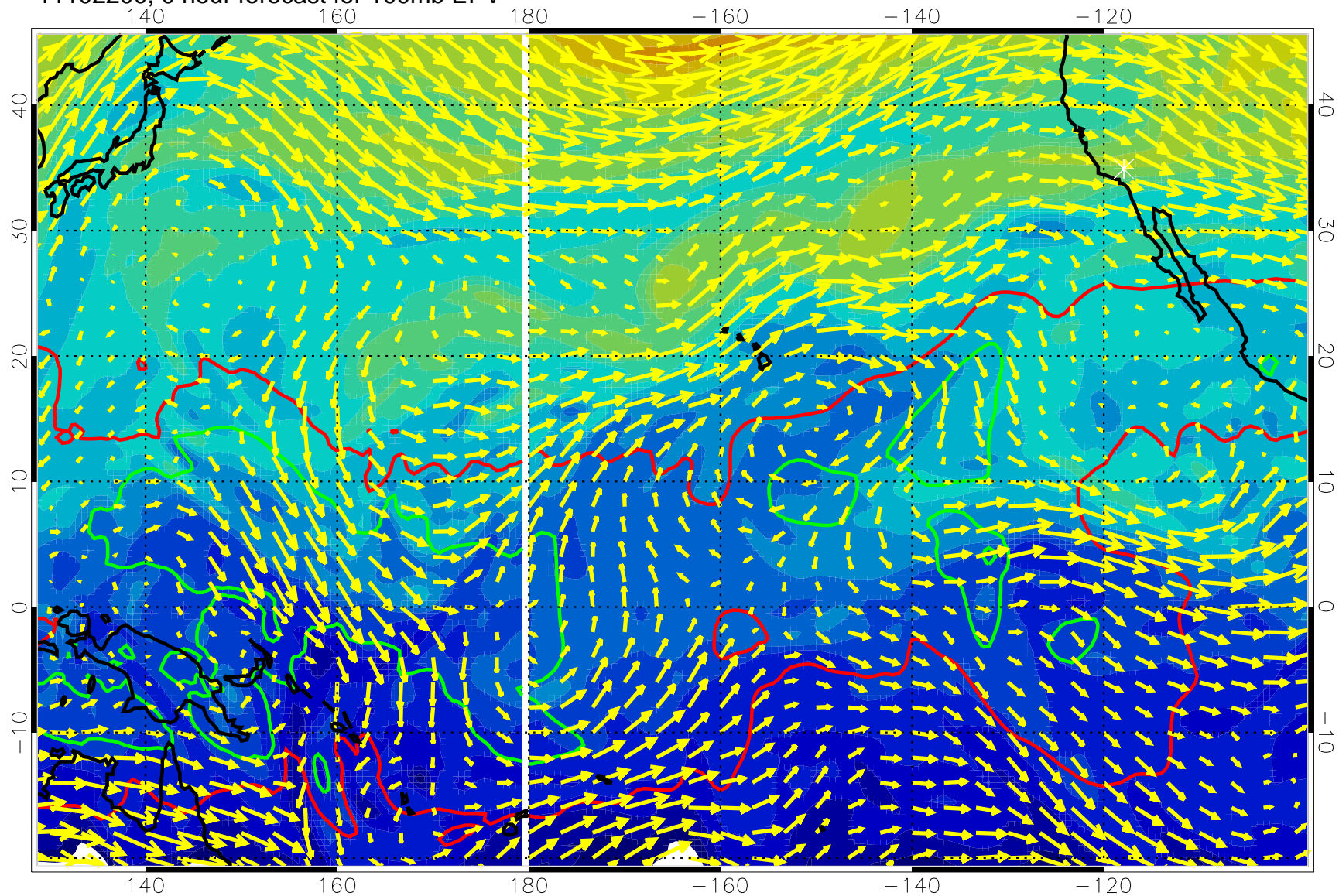
11102200, 0 hour forecast for 100mb EPV
