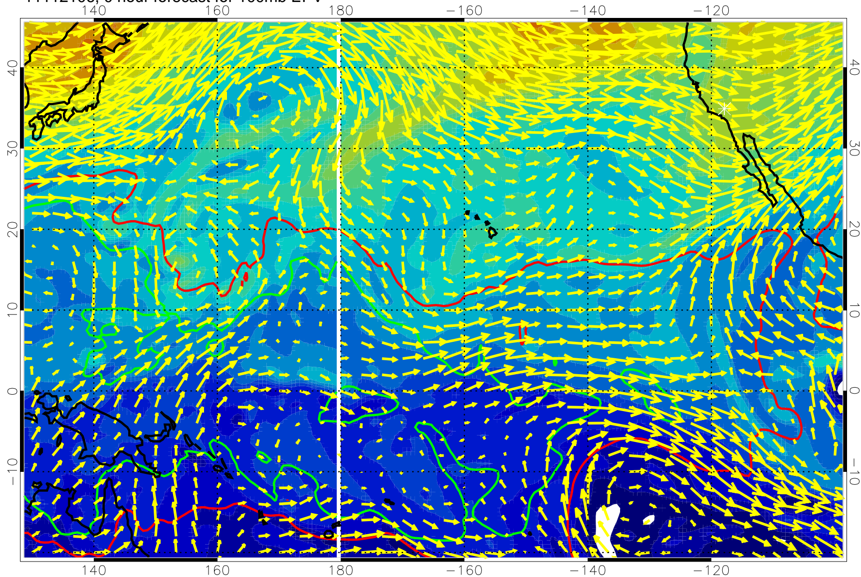
11112106, 0 hour forecast for 100mb EPV
