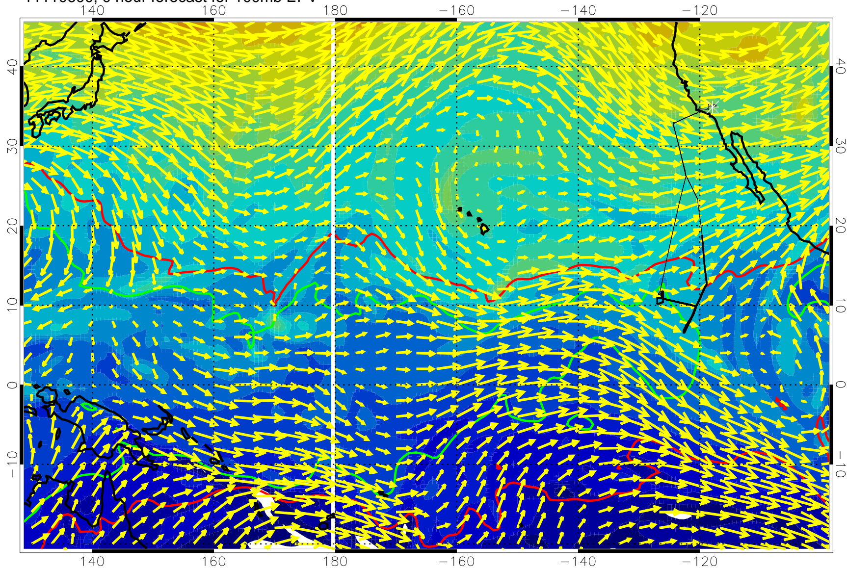
11110600, 0 hour forecast for 100mb EPV
