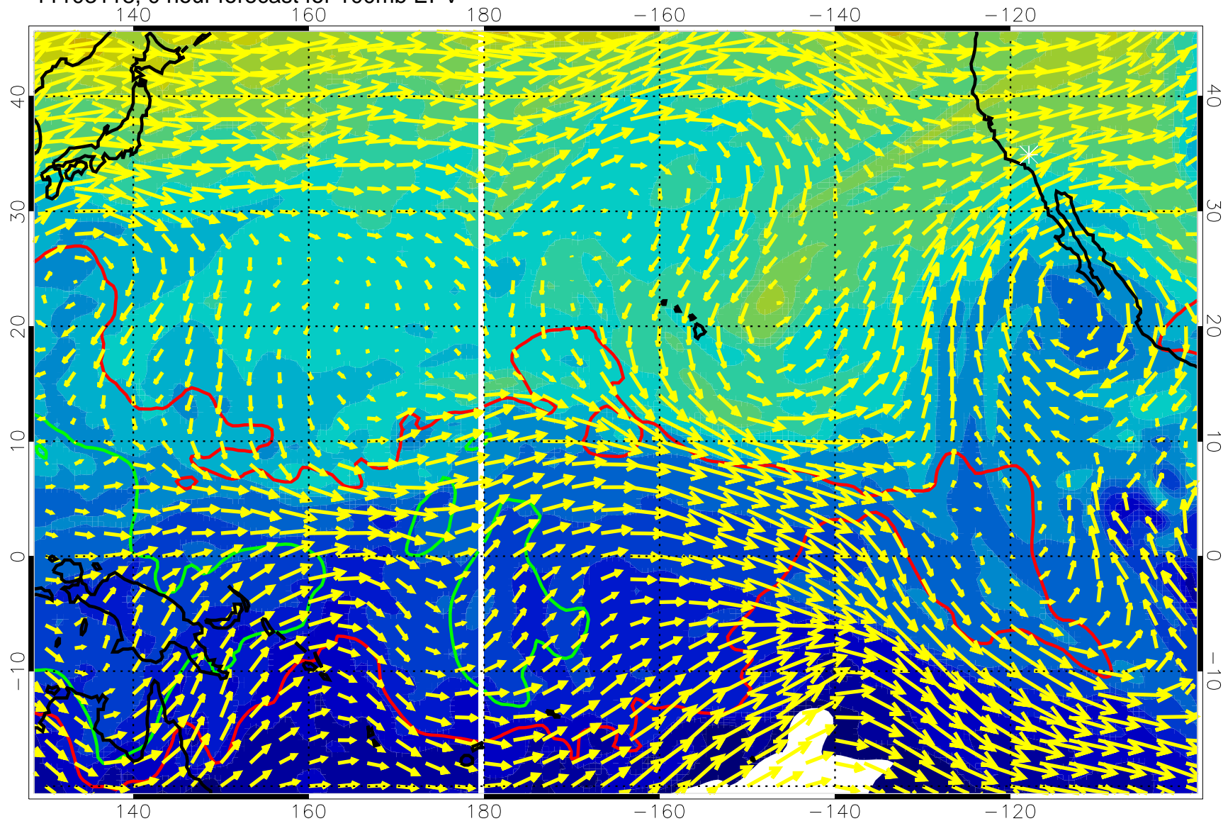
11103118, 0 hour forecast for 100mb EPV
