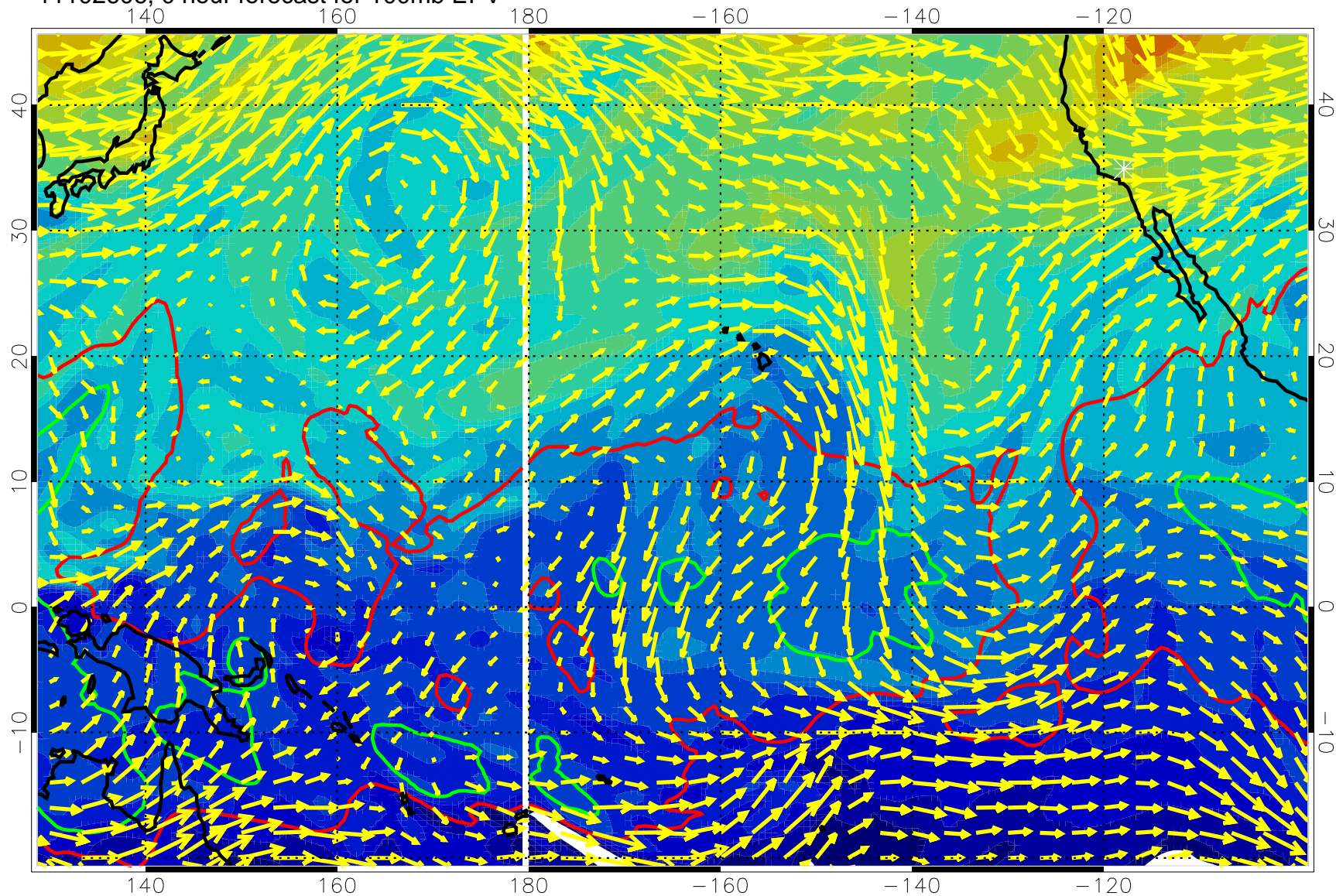
11102606, 0 hour forecast for 100mb EPV
