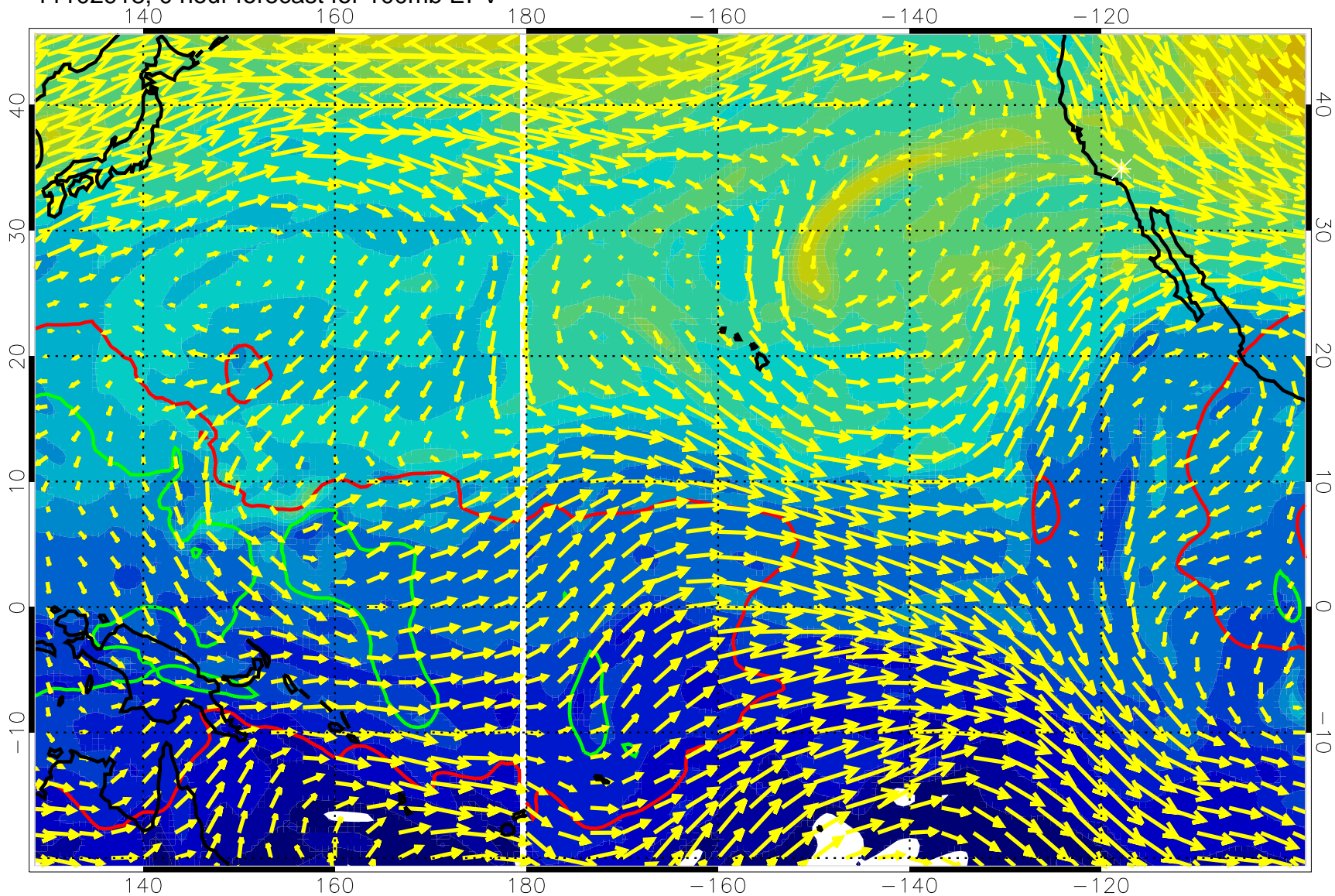
11102918, 0 hour forecast for 100mb EPV
