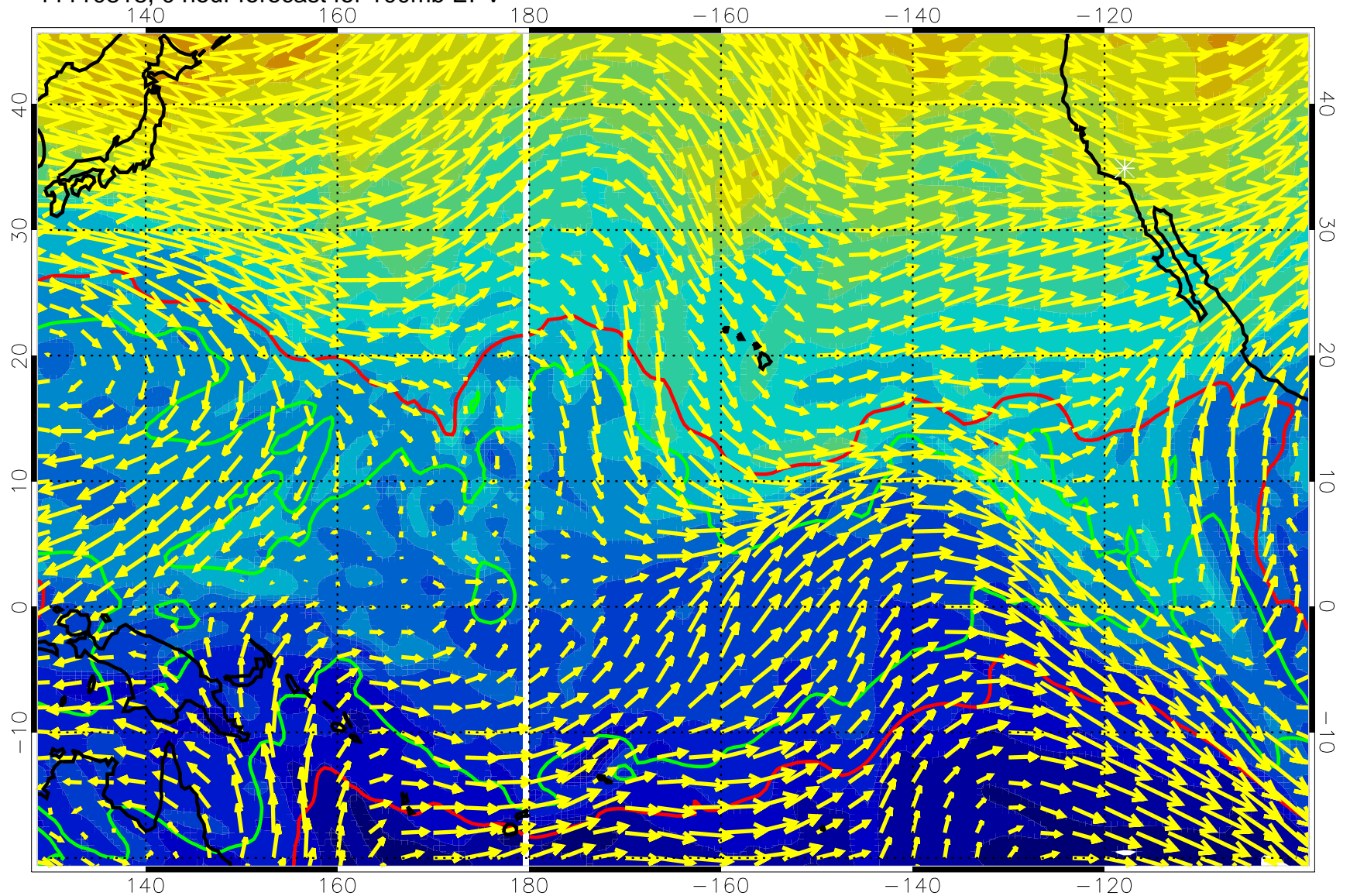
11110818, 0 hour forecast for 100mb EPV
