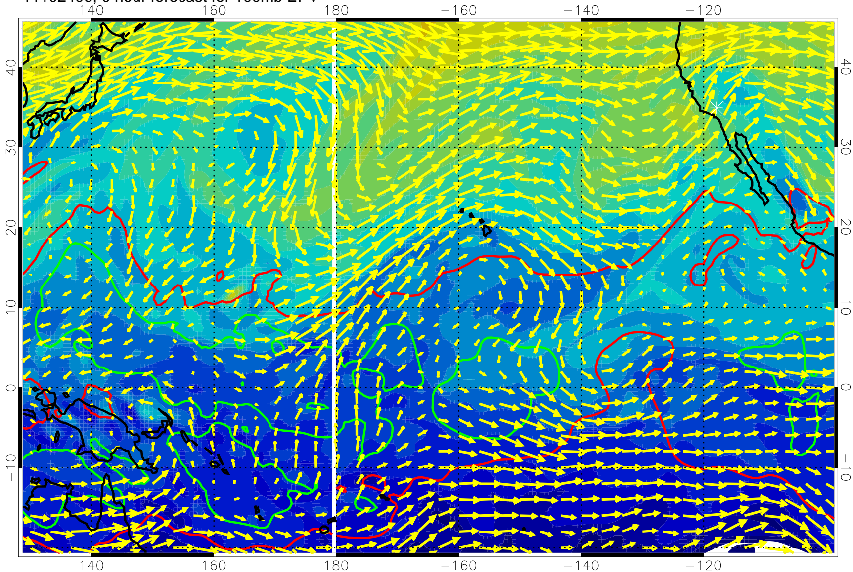
11102406, 0 hour forecast for 100mb EPV
