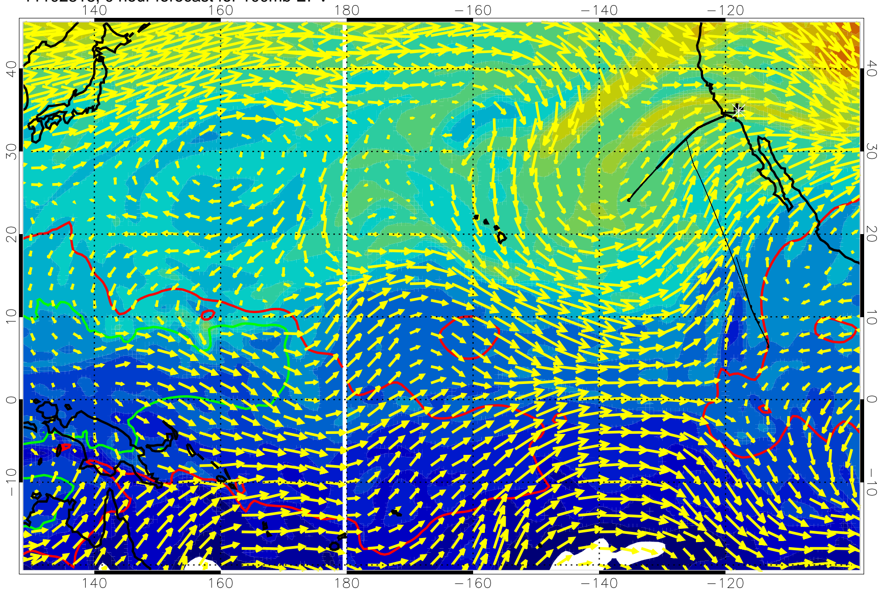
11102818, 0 hour forecast for 100mb EPV
