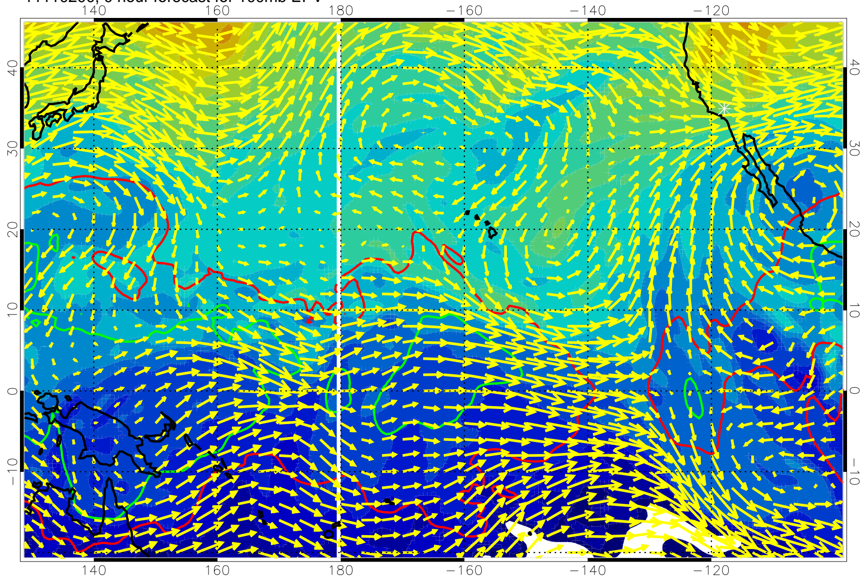
11110200, 0 hour forecast for 100mb EPV
