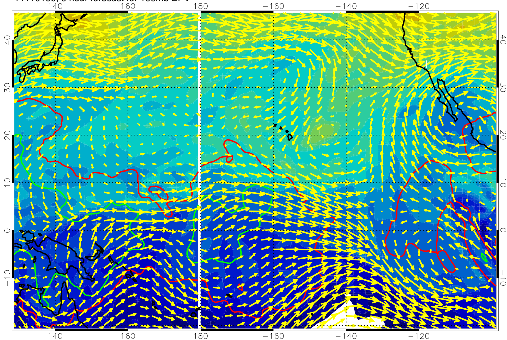
11110106, 0 hour forecast for 100mb EPV
