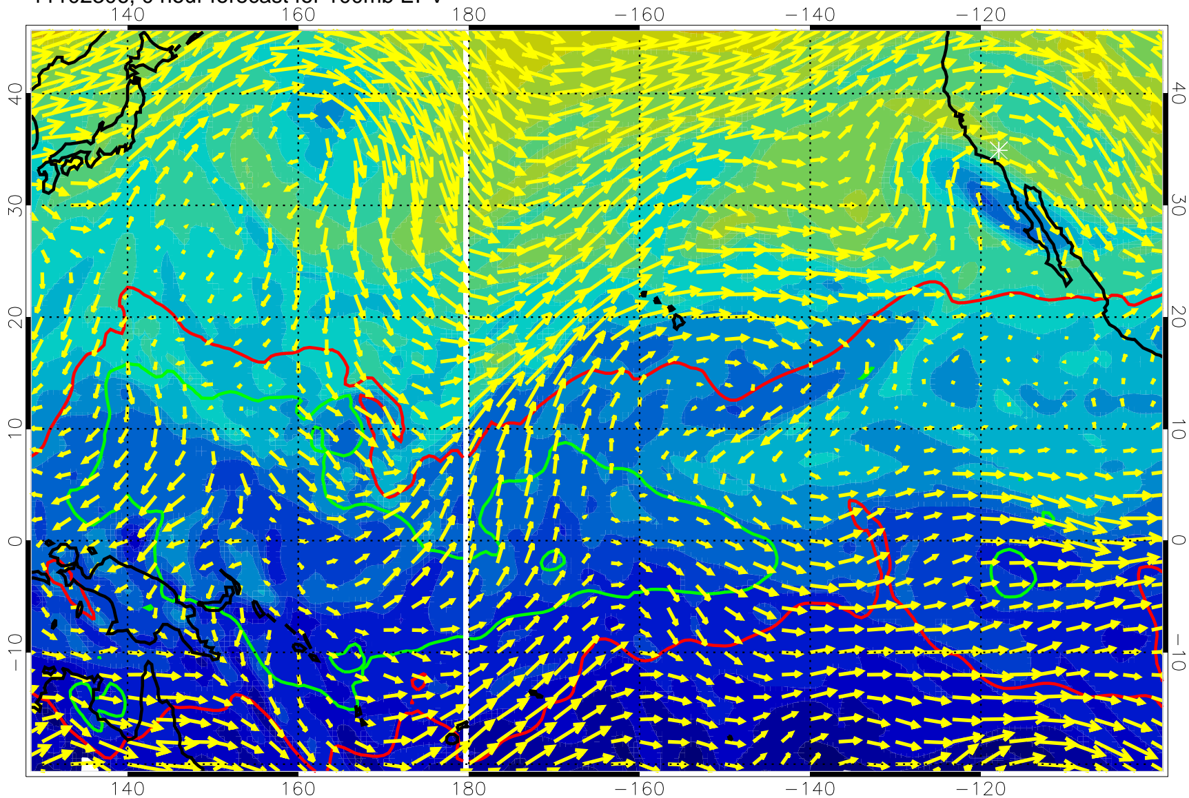
11102306, 0 hour forecast for 100mb EPV
