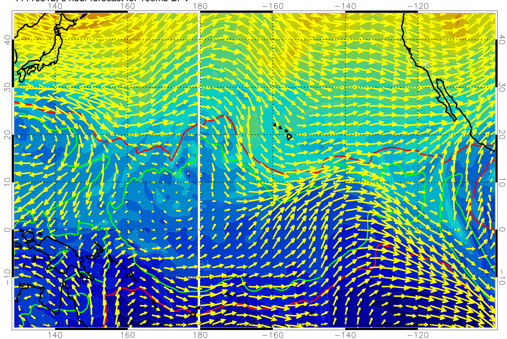
11110812, 0 hour forecast for 100mb EPV
