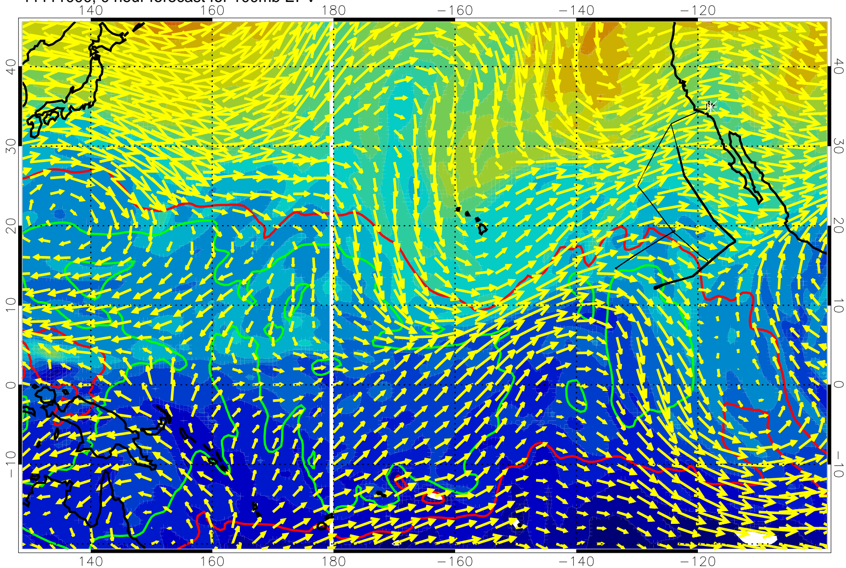
11111000, 0 hour forecast for 100mb EPV
