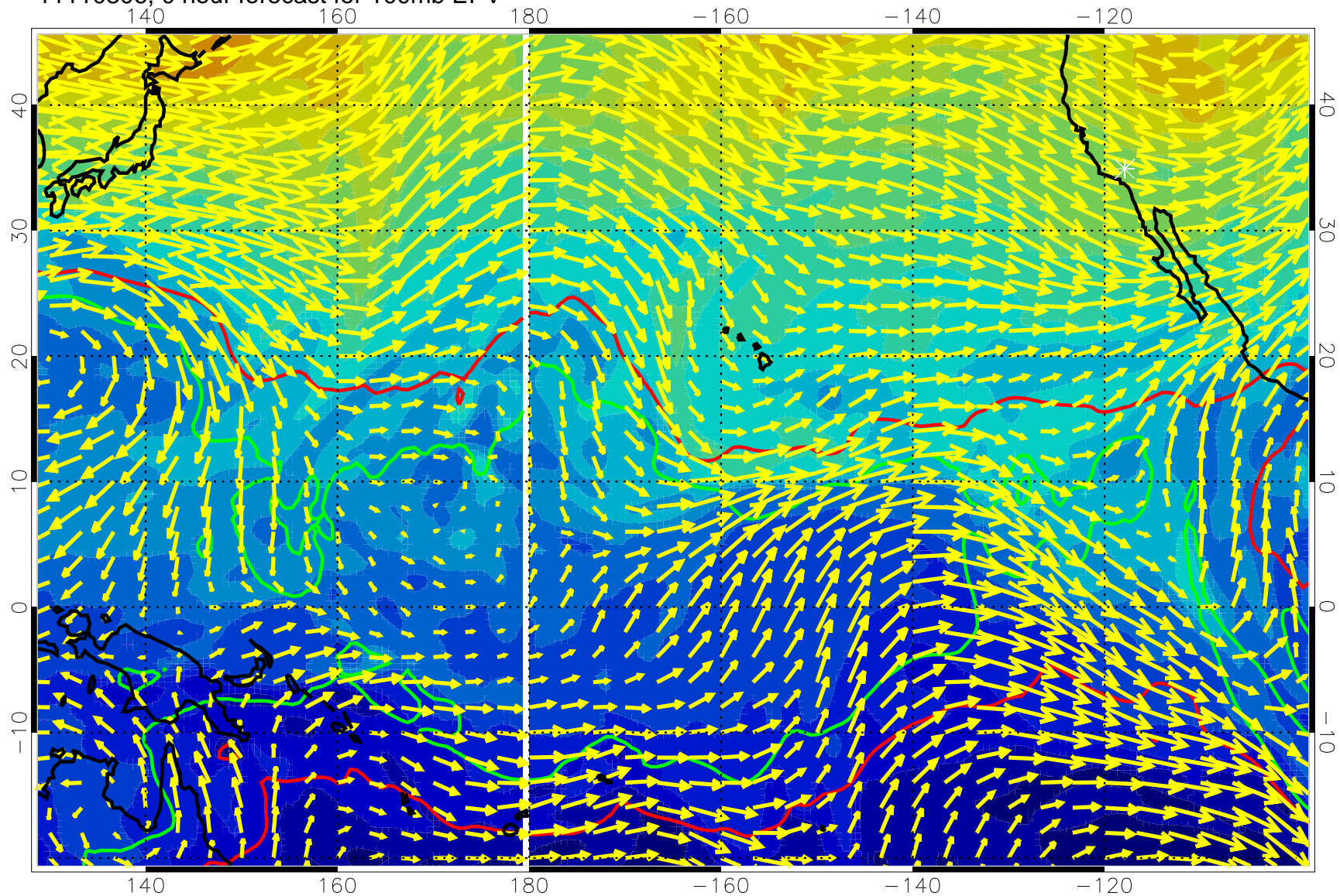
11110806, 0 hour forecast for 100mb EPV
