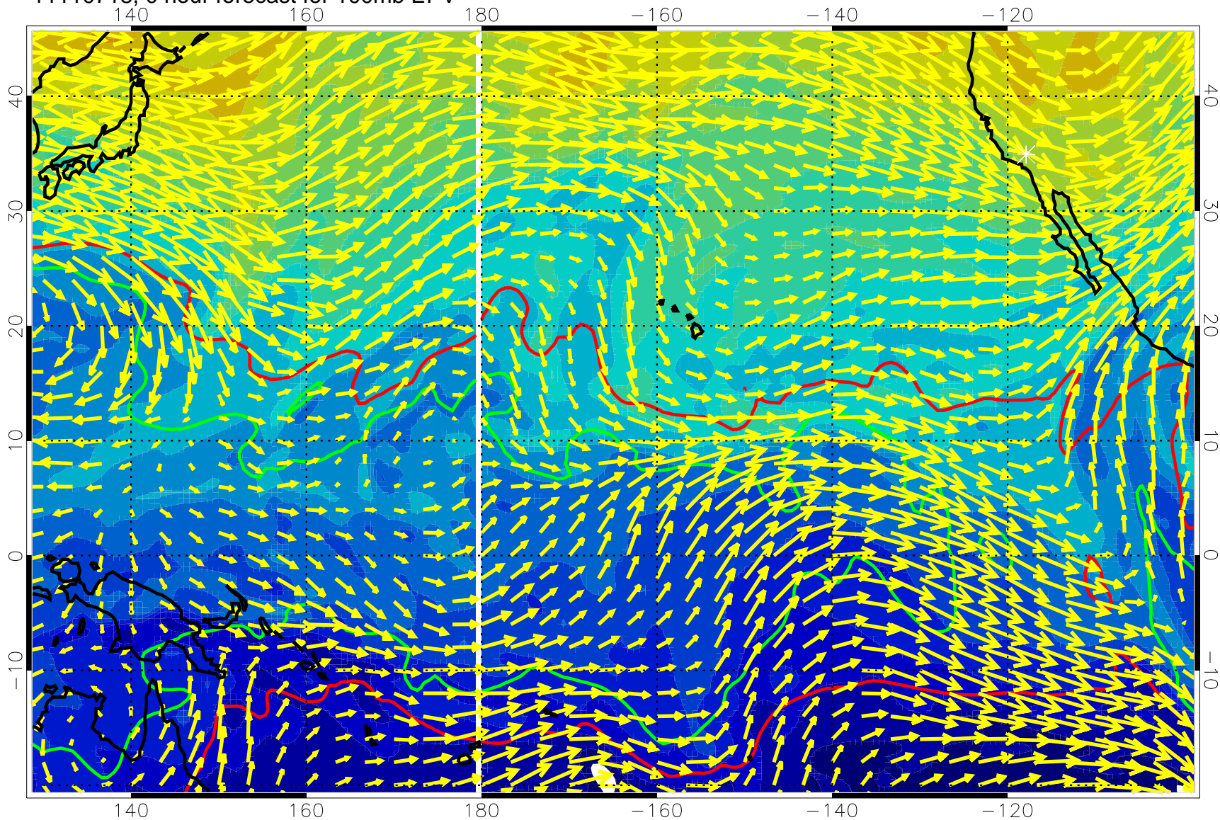
11110718, 0 hour forecast for 100mb EPV
