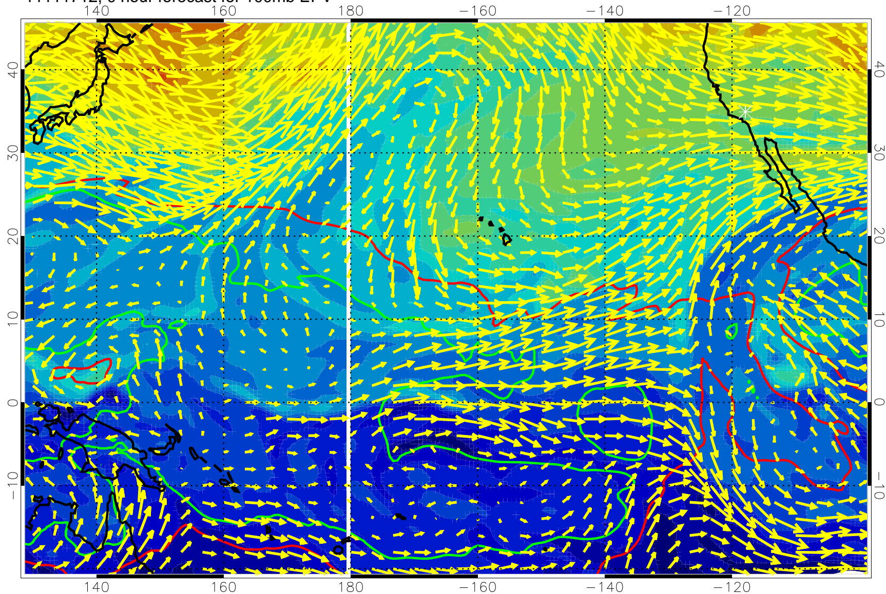
11111712, 0 hour forecast for 100mb EPV
