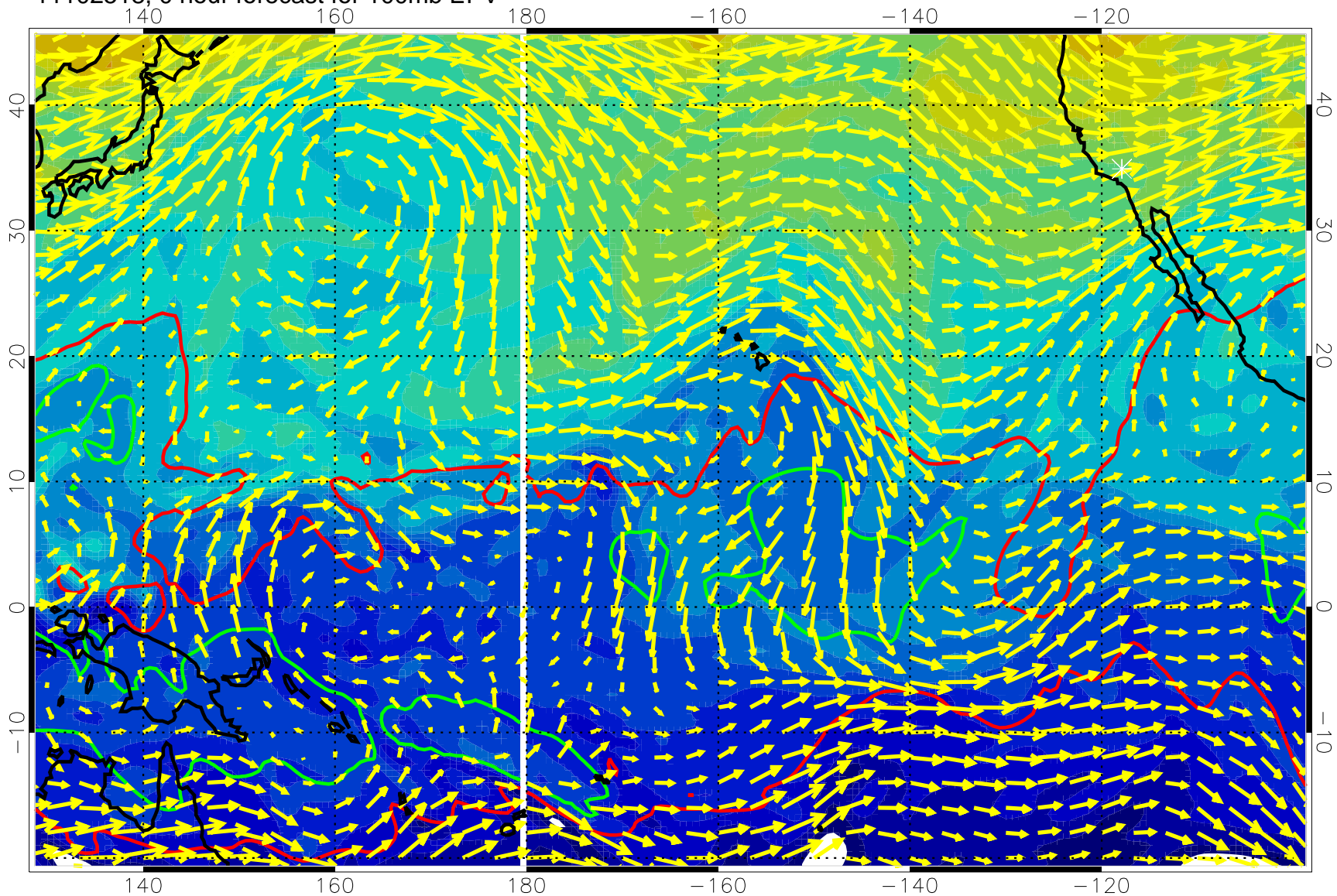
11102518, 0 hour forecast for 100mb EPV
