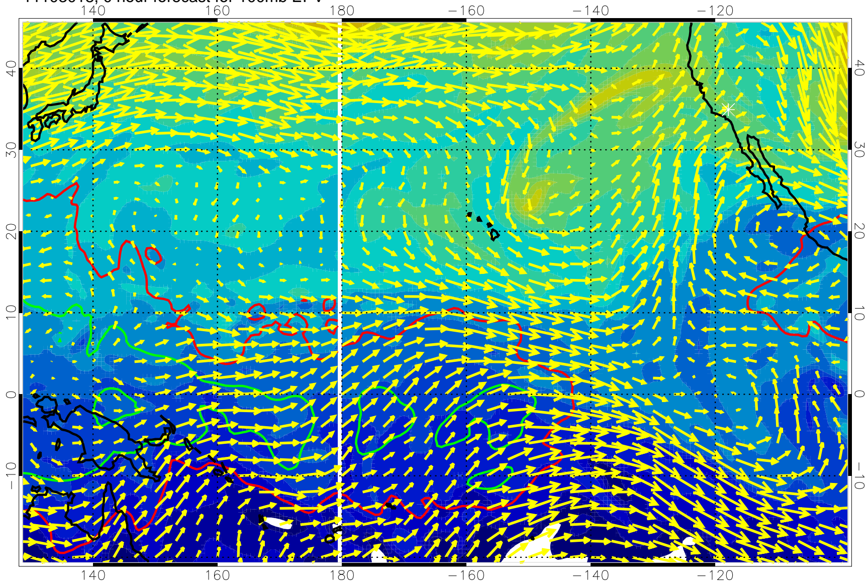
11103018, 0 hour forecast for 100mb EPV
