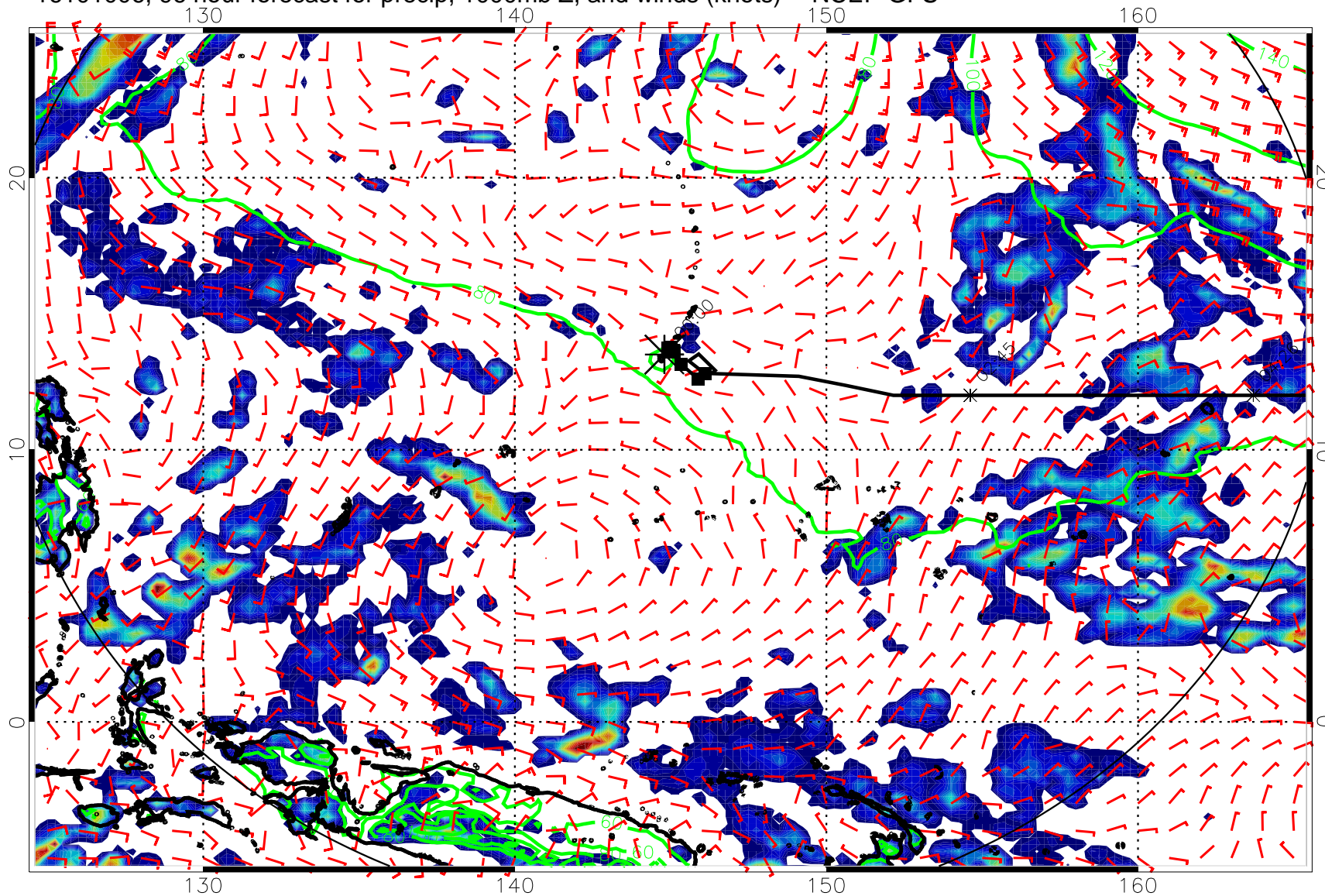
16101006, 96 hour forecast for precip, 1000mb Z, and winds (knots) -- NCEP GFS
