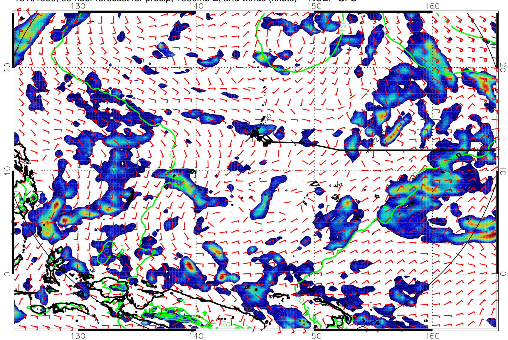
16101000, 90 hour forecast for precip, 1000mb Z, and winds (knots) -- NCEP GFS
