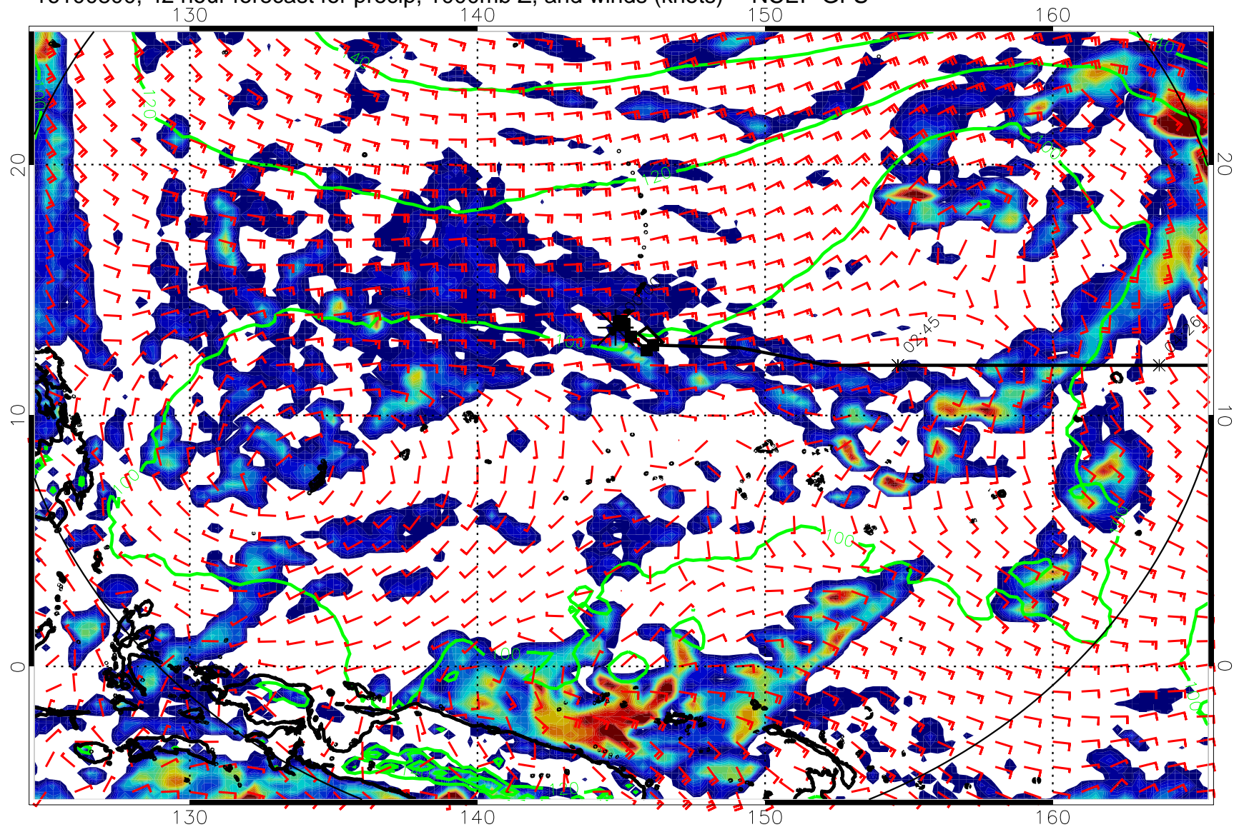
16100800, 42 hour forecast for precip, 1000mb Z, and winds (knots) -- NCEP GFS
