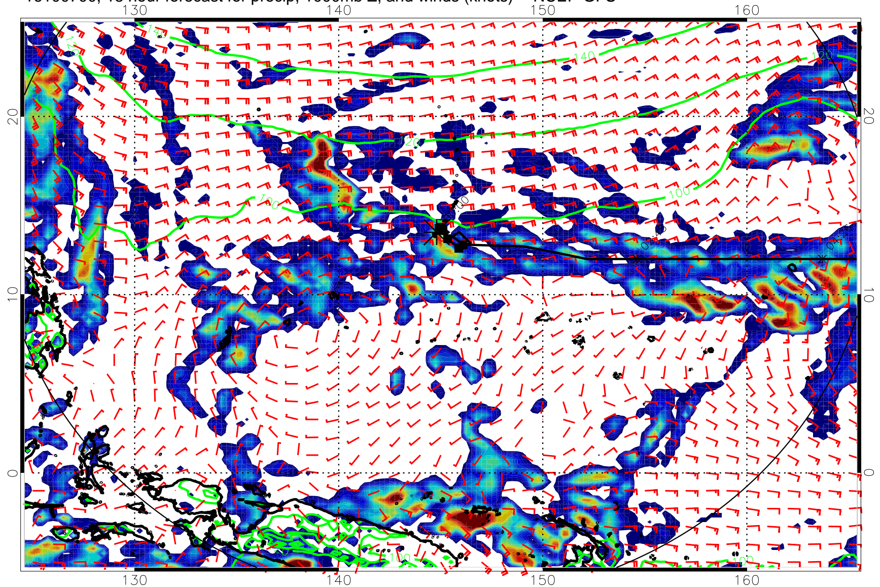
16100700, 18 hour forecast for precip, 1000mb Z, and winds (knots) -- NCEP GFS
