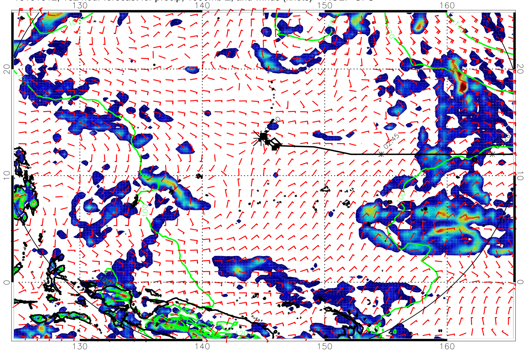
16101012, 102 hour forecast for precip, 1000mb Z, and winds (knots) -- NCEP GFS
