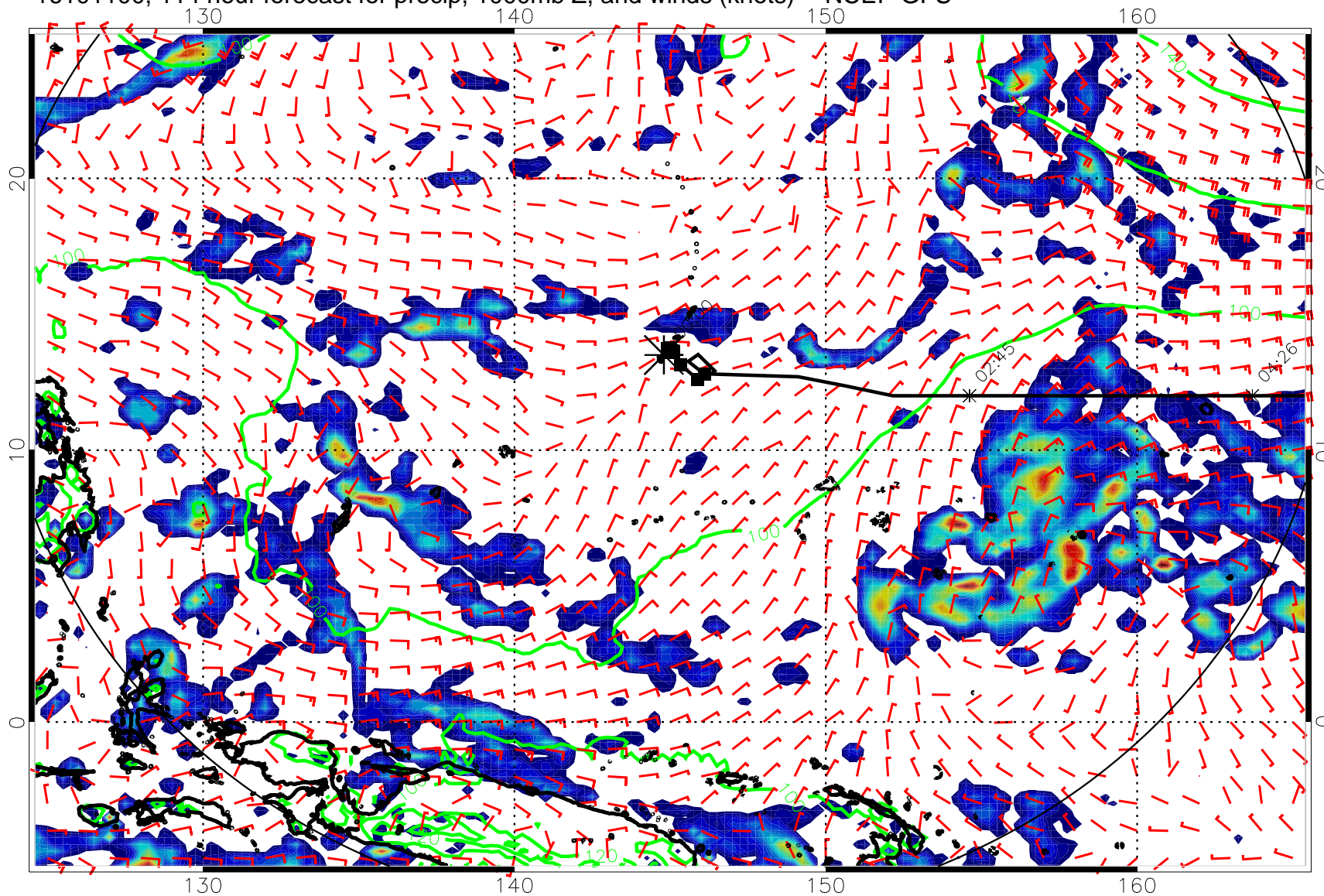
16101100, 114 hour forecast for precip, 1000mb Z, and winds (knots) -- NCEP GFS
