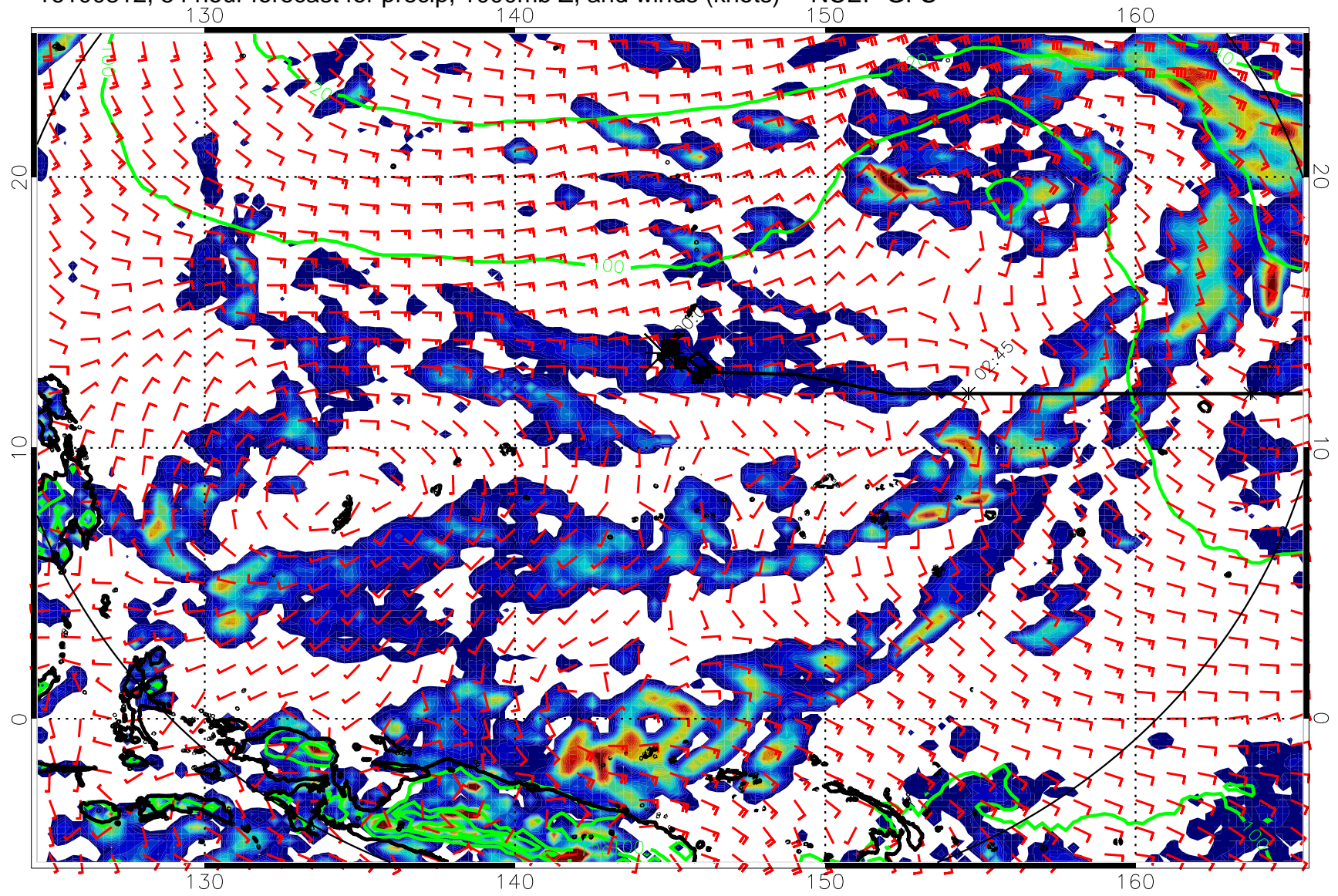
16100812, 54 hour forecast for precip, 1000mb Z, and winds (knots) -- NCEP GFS
