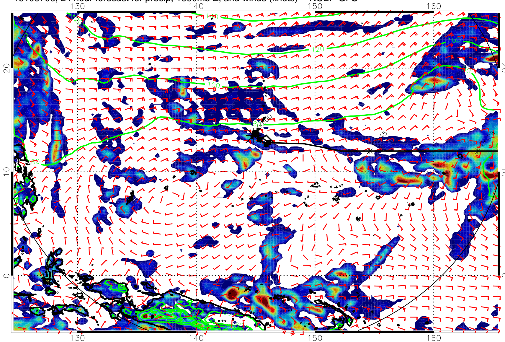
16100706, 24 hour forecast for precip, 1000mb Z, and winds (knots) -- NCEP GFS
