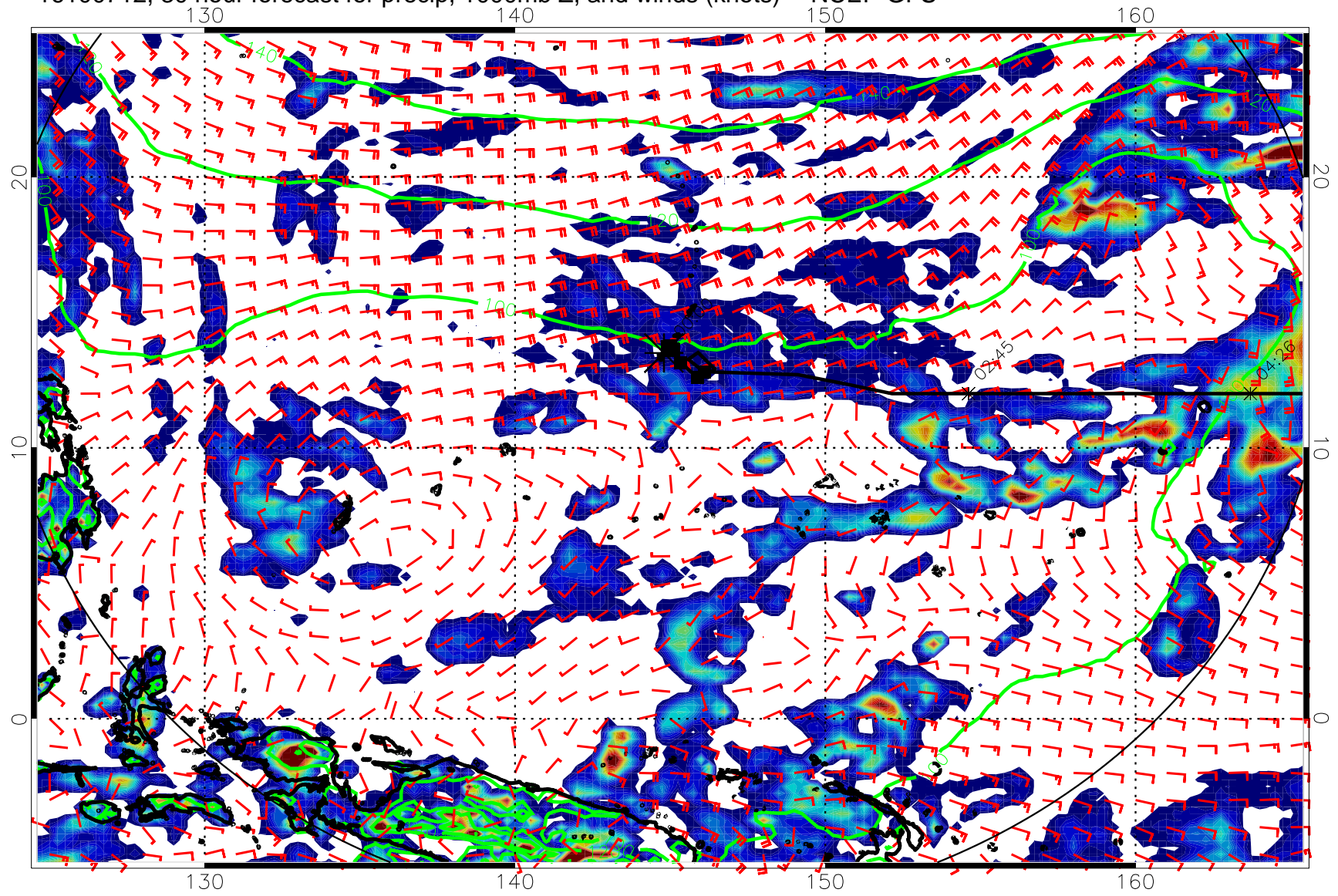
16100712, 30 hour forecast for precip, 1000mb Z, and winds (knots) -- NCEP GFS
