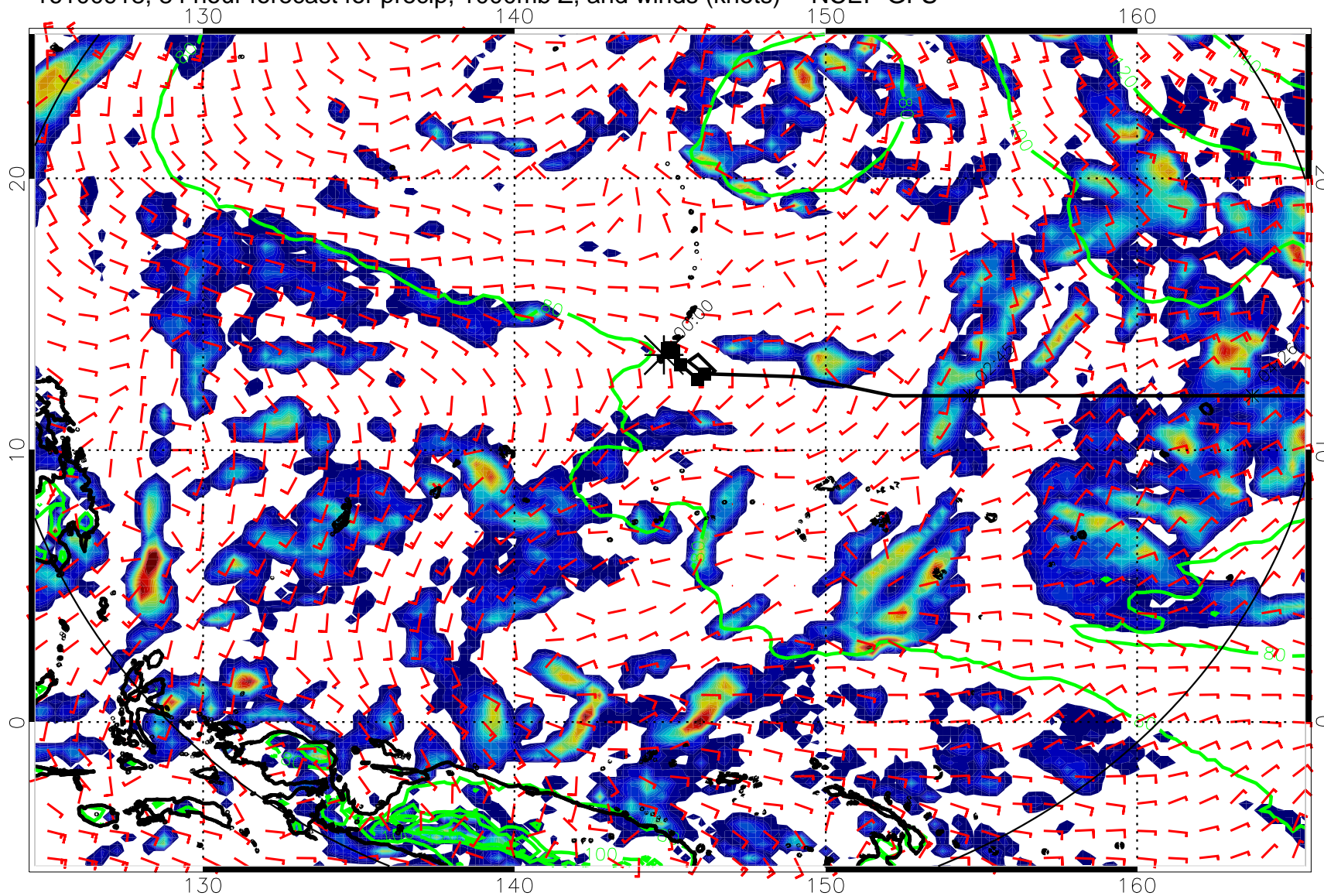
16100918, 84 hour forecast for precip, 1000mb Z, and winds (knots) -- NCEP GFS
