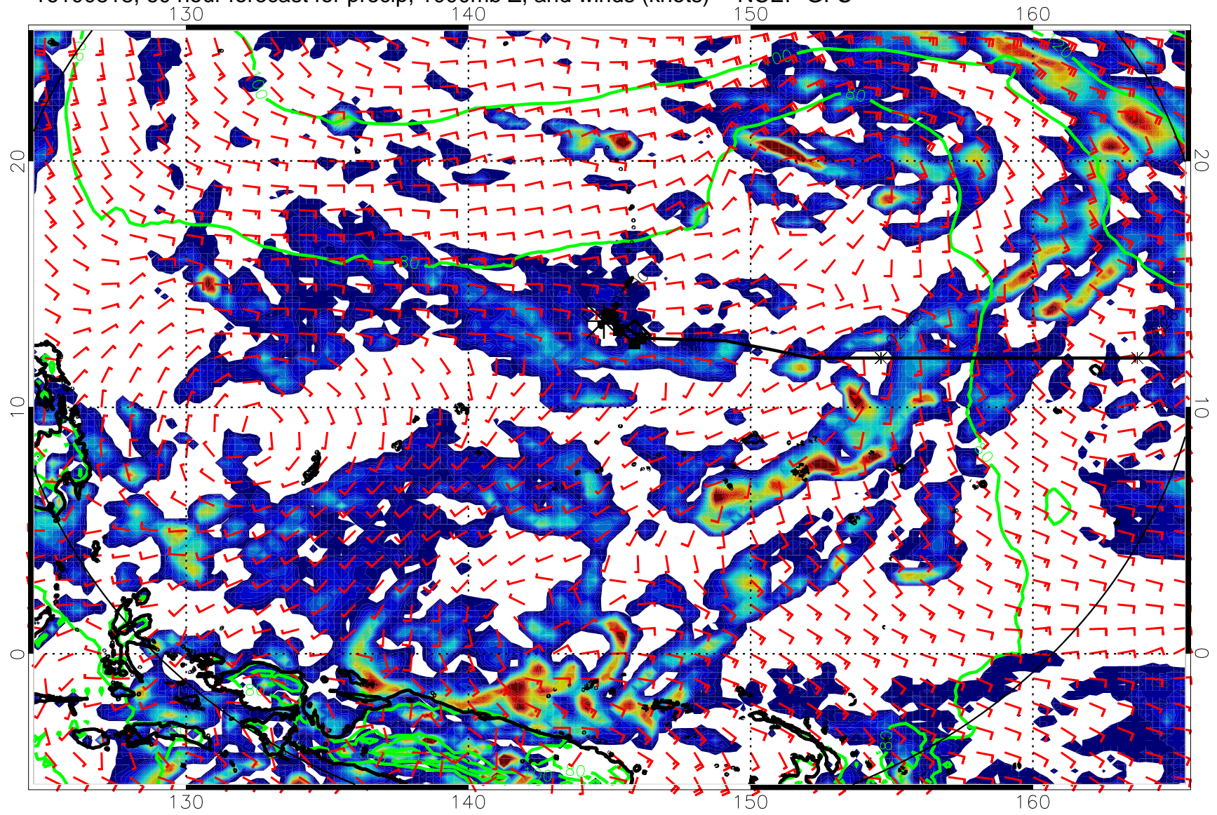
16100818, 60 hour forecast for precip, 1000mb Z, and winds (knots) -- NCEP GFS
