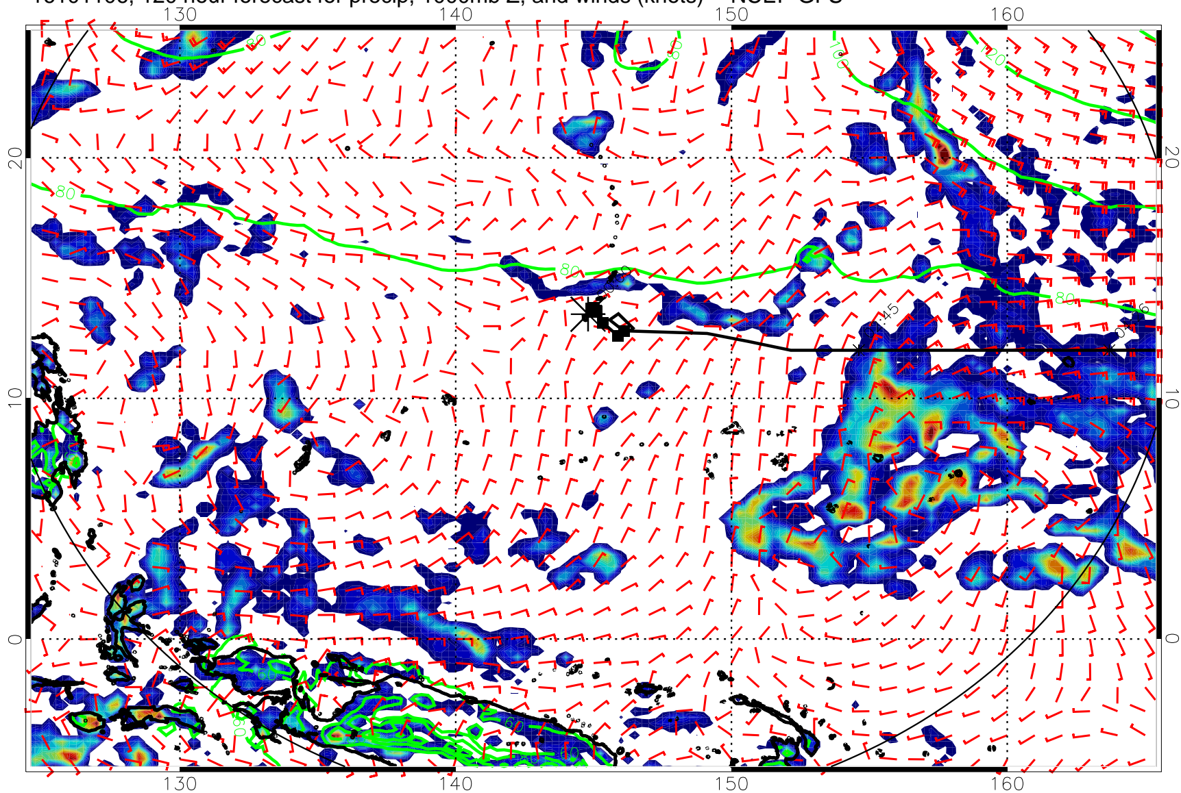
16101106, 120 hour forecast for precip, 1000mb Z, and winds (knots) -- NCEP GFS
