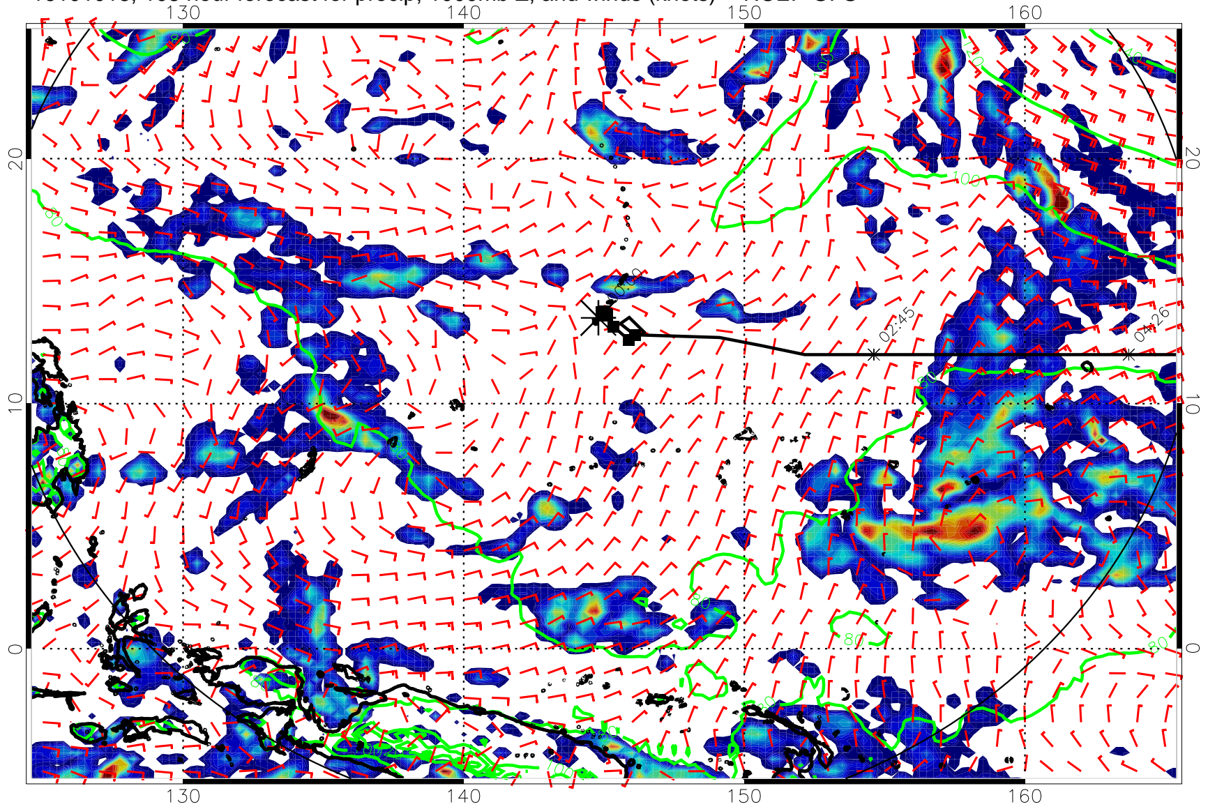
16101018, 108 hour forecast for precip, 1000mb Z, and winds (knots) -- NCEP GFS
