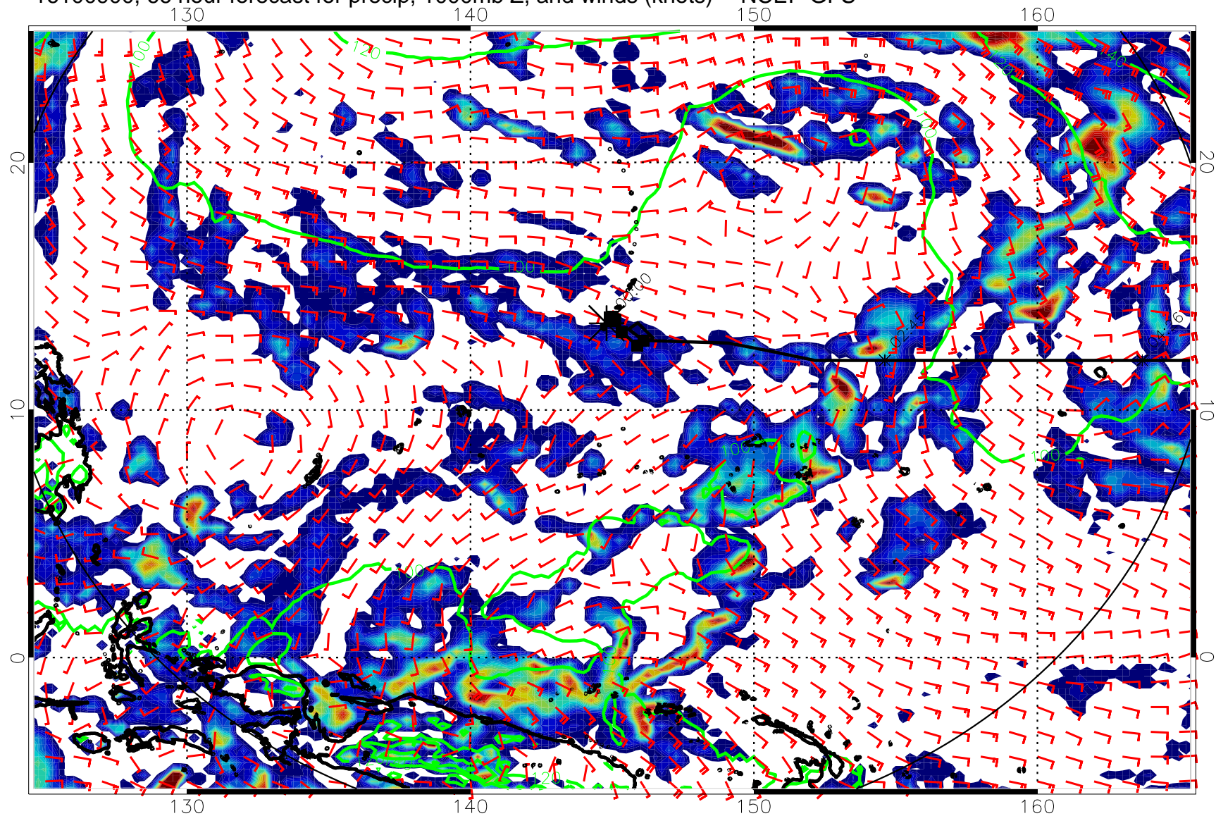
16100900, 66 hour forecast for precip, 1000mb Z, and winds (knots) -- NCEP GFS
