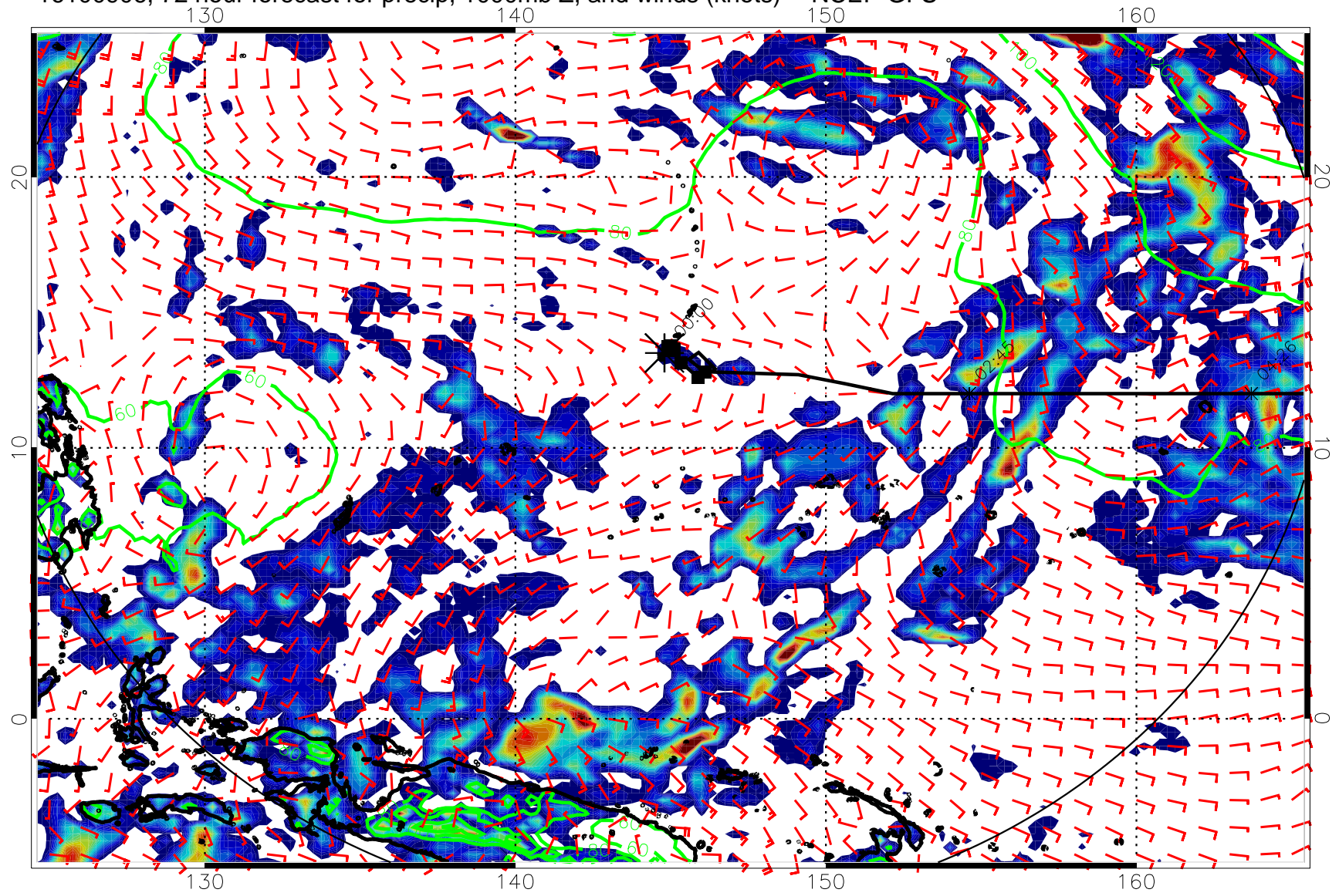
16100906, 72 hour forecast for precip, 1000mb Z, and winds (knots) -- NCEP GFS
