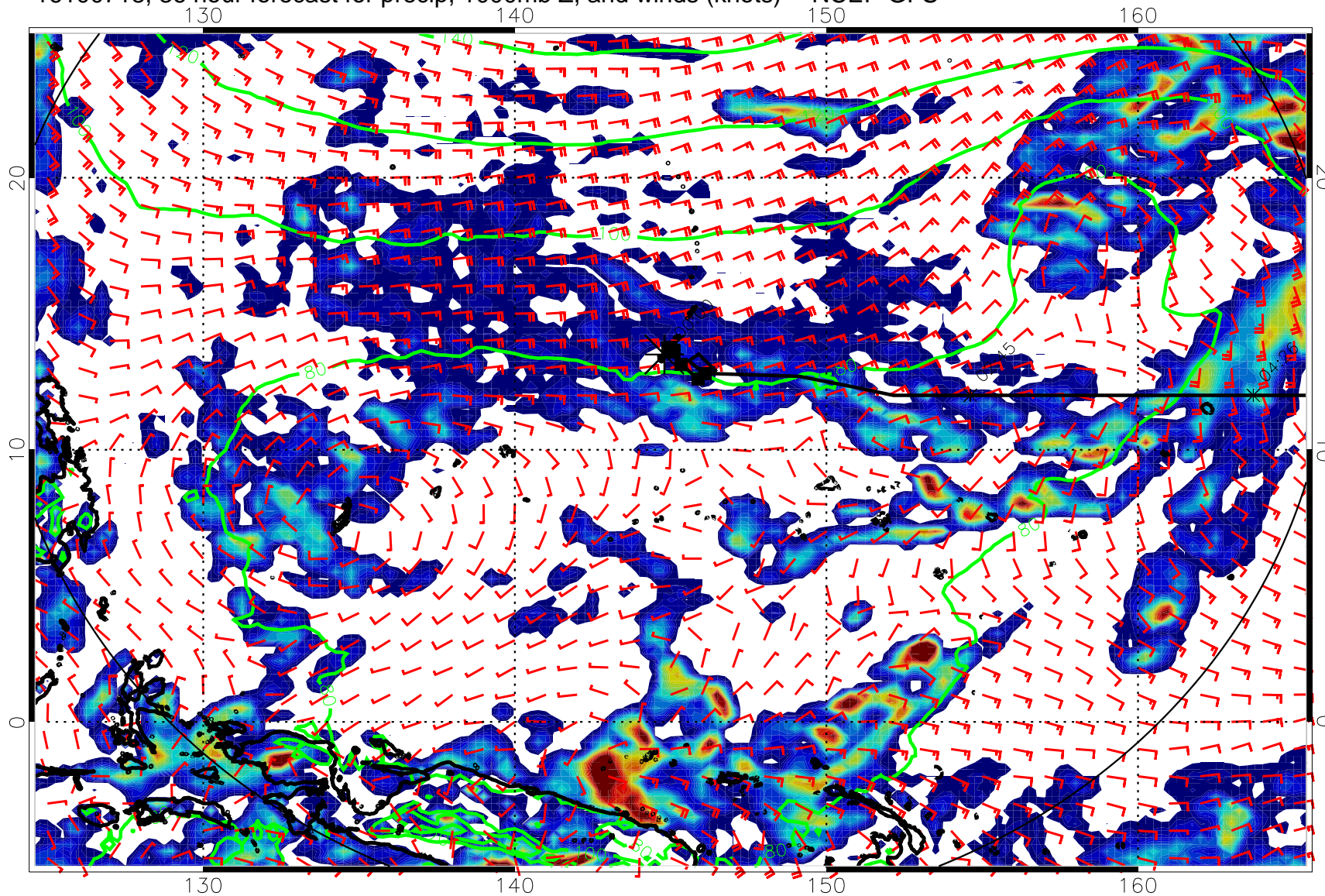
16100718, 36 hour forecast for precip, 1000mb Z, and winds (knots) -- NCEP GFS
