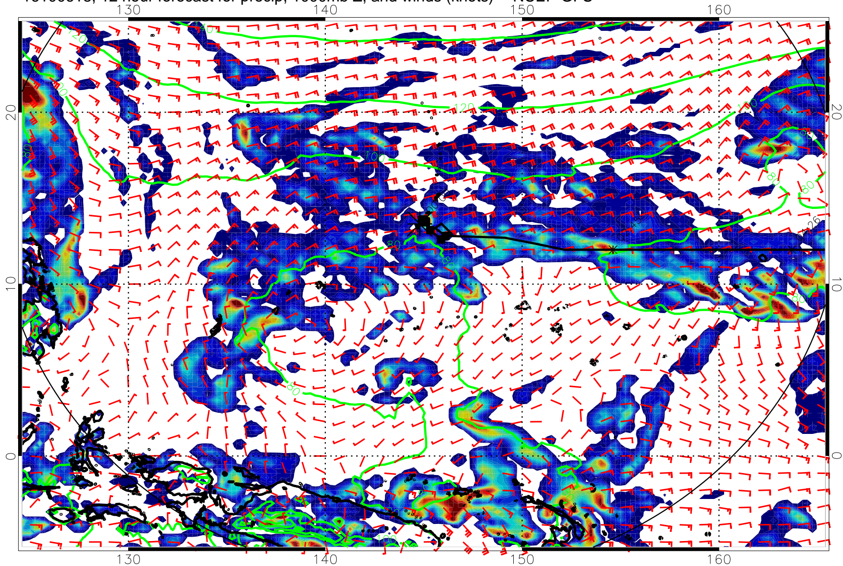
16100618, 12 hour forecast for precip, 1000mb Z, and winds (knots) -- NCEP GFS
