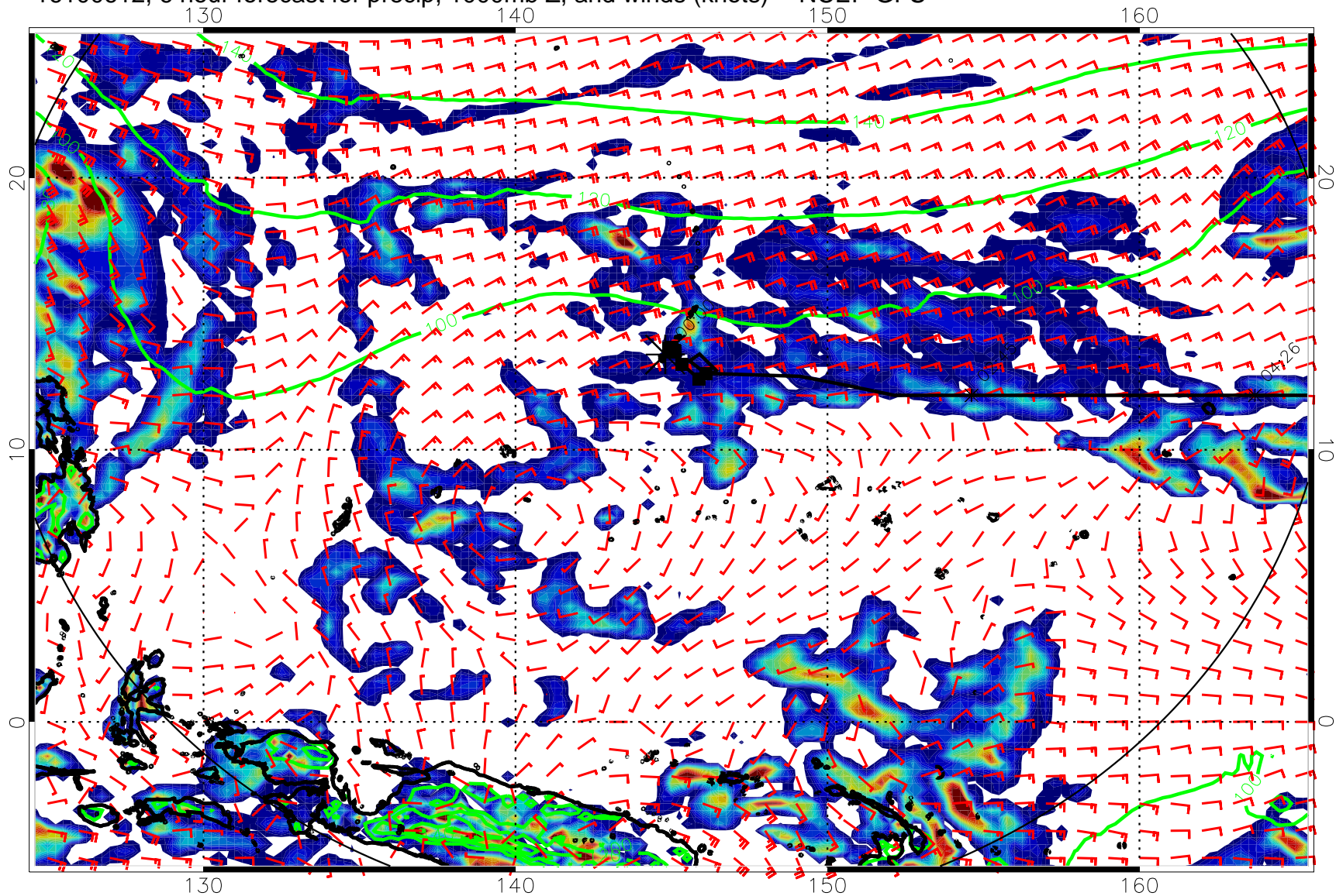
16100612, 6 hour forecast for precip, 1000mb Z, and winds (knots) -- NCEP GFS
