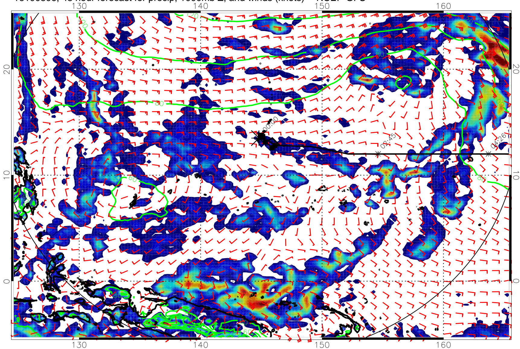
16100806, 48 hour forecast for precip, 1000mb Z, and winds (knots) -- NCEP GFS
