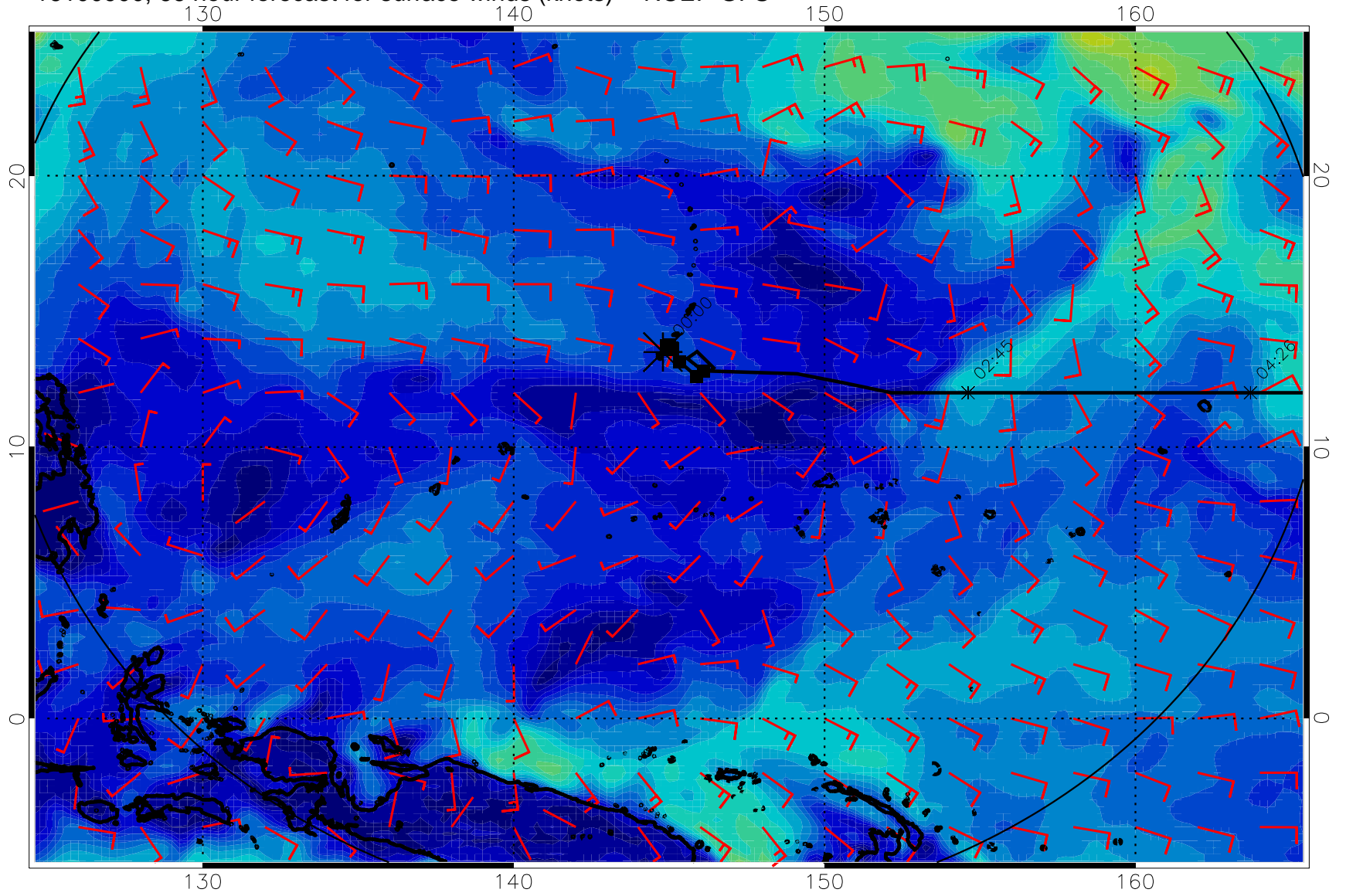
16100900, 66 hour forecast for surface winds (knots) -- NCEP GFS
