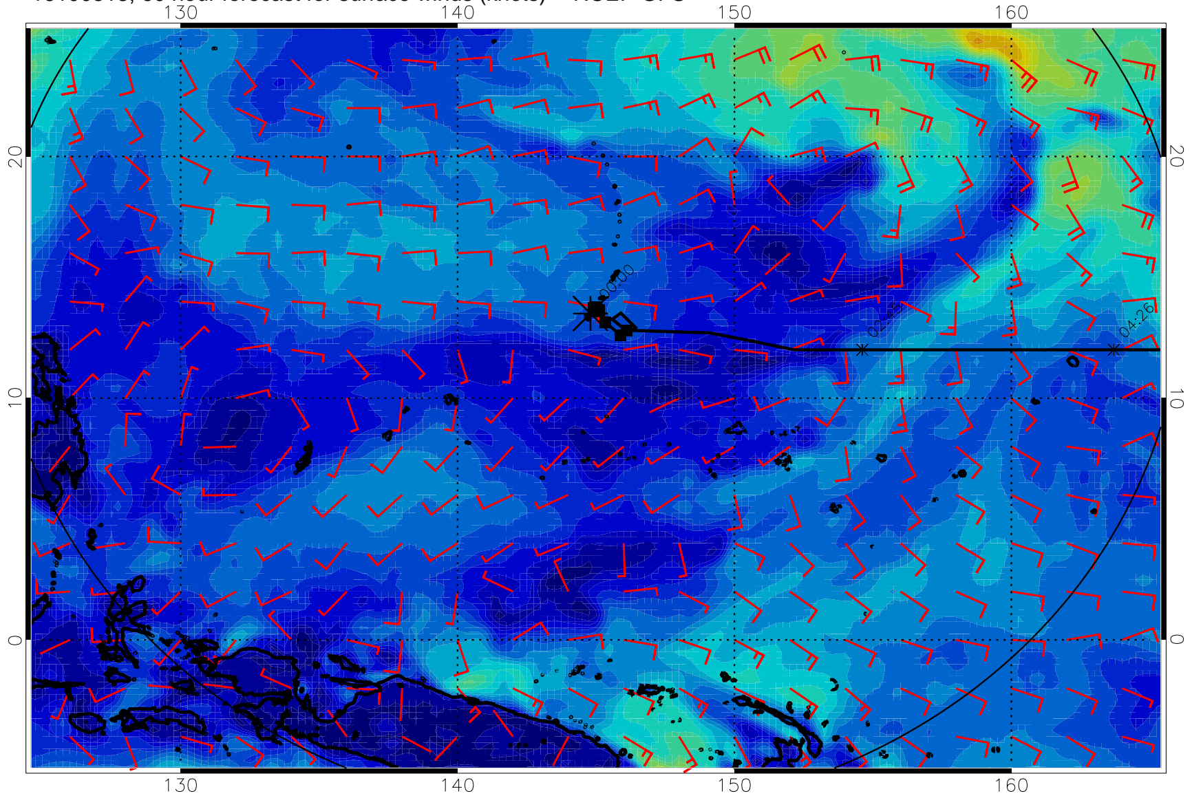
16100818, 60 hour forecast for surface winds (knots) -- NCEP GFS
