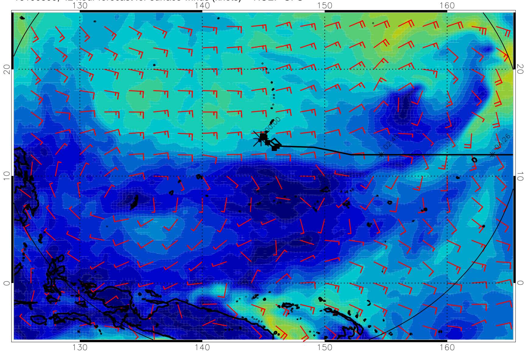
16100800, 42 hour forecast for surface winds (knots) -- NCEP GFS
