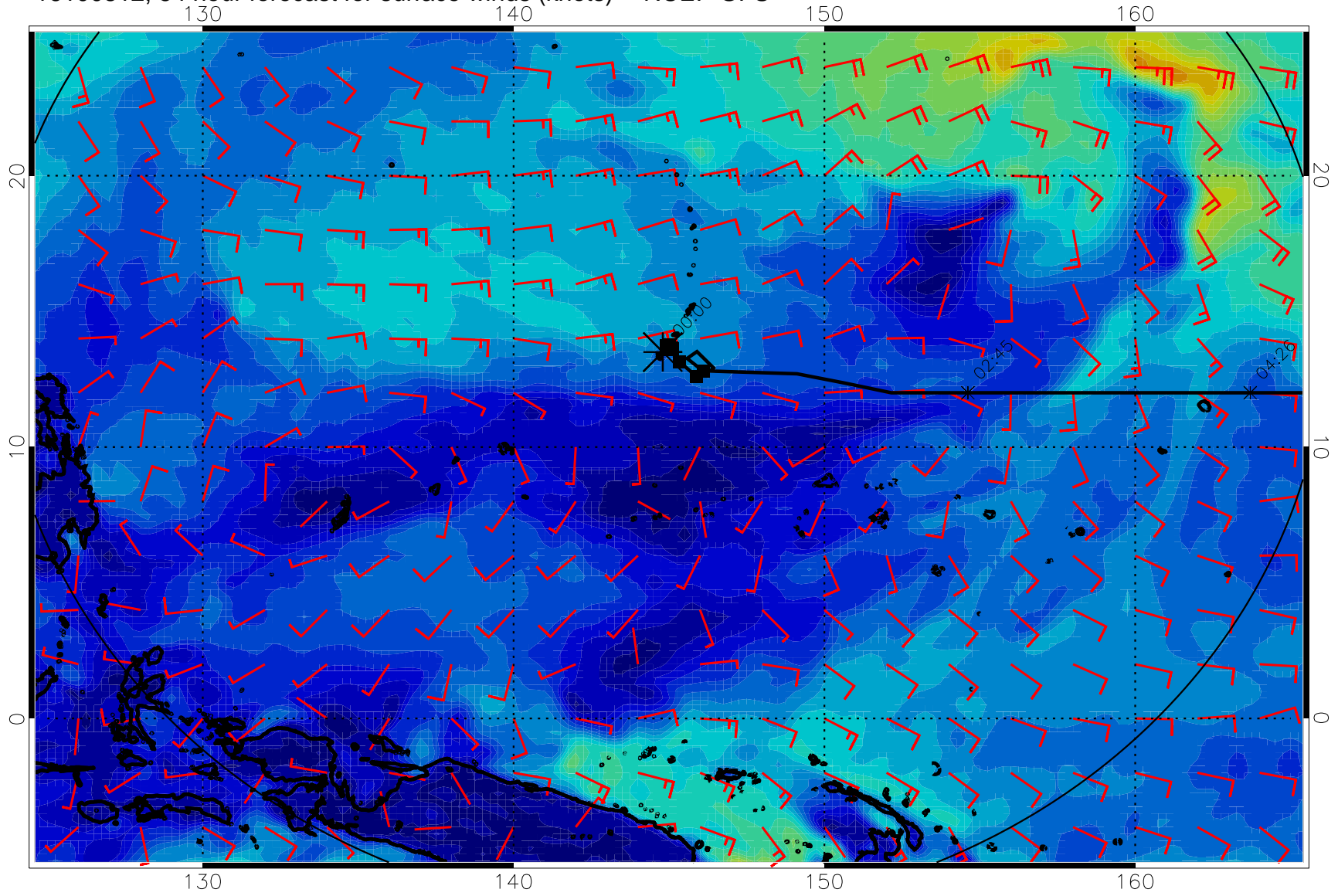
16100812, 54 hour forecast for surface winds (knots) -- NCEP GFS
