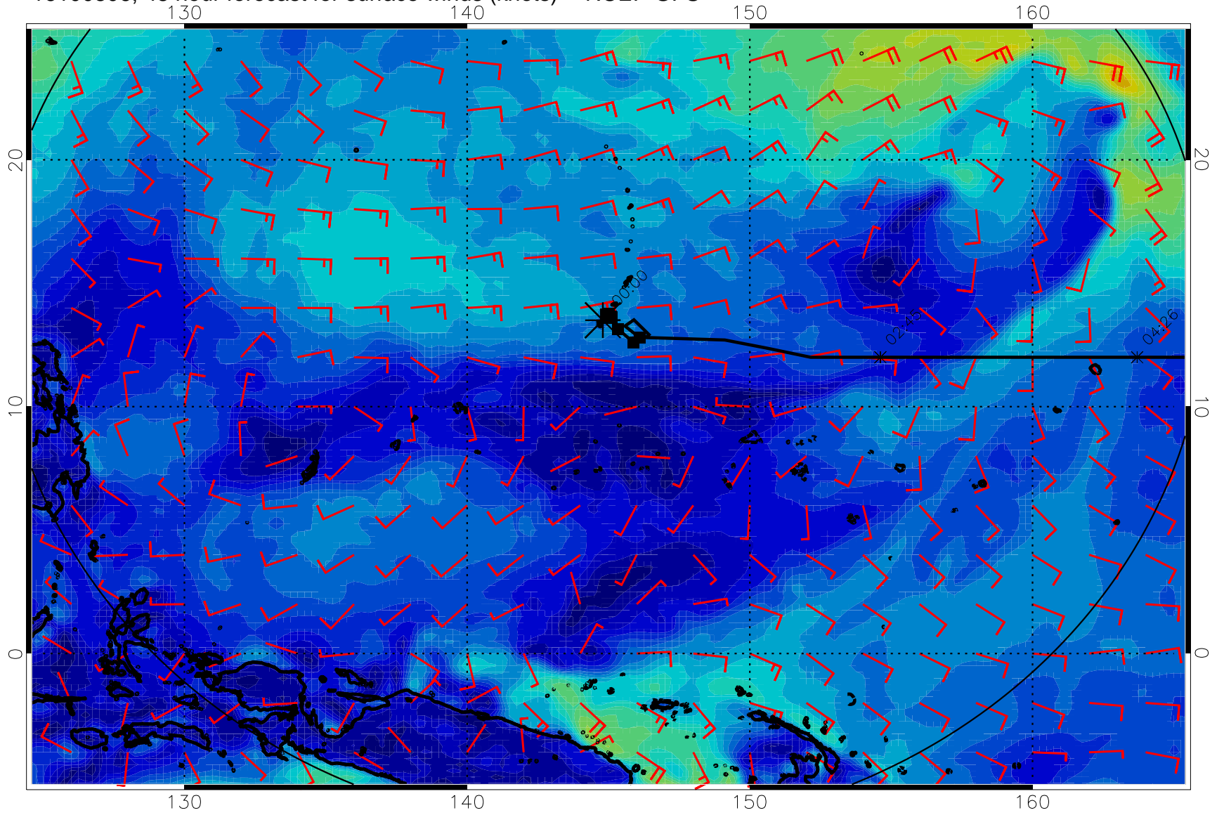
16100806, 48 hour forecast for surface winds (knots) -- NCEP GFS
