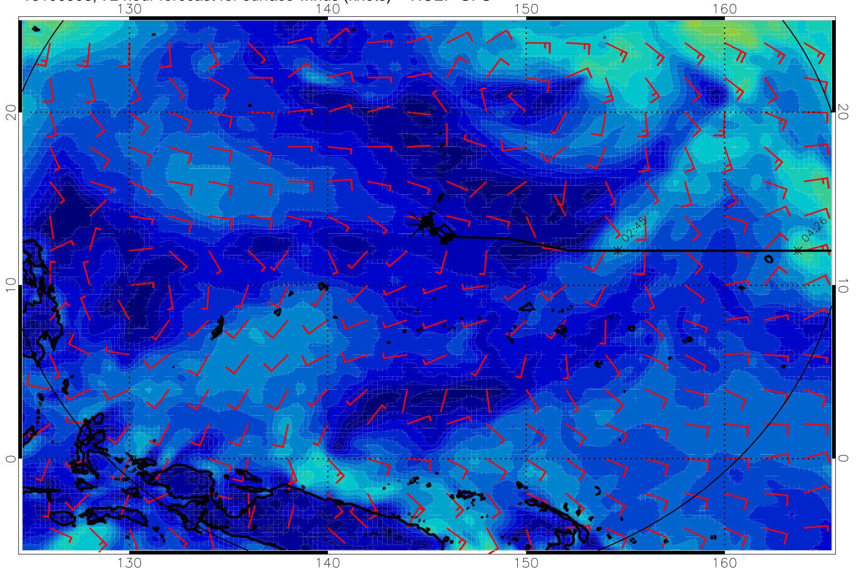
16100906, 72 hour forecast for surface winds (knots) -- NCEP GFS
