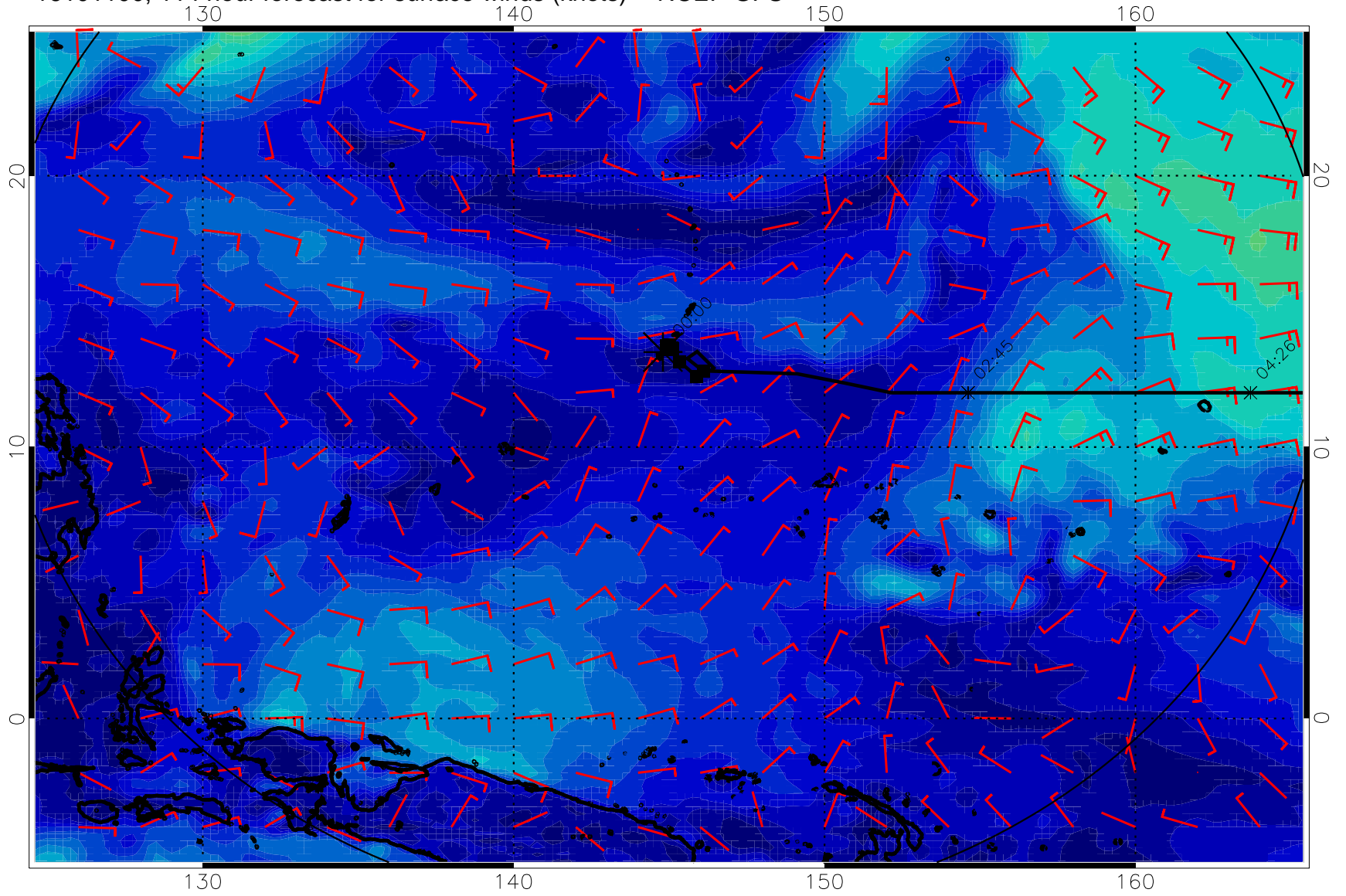
16101100, 114 hour forecast for surface winds (knots) -- NCEP GFS
