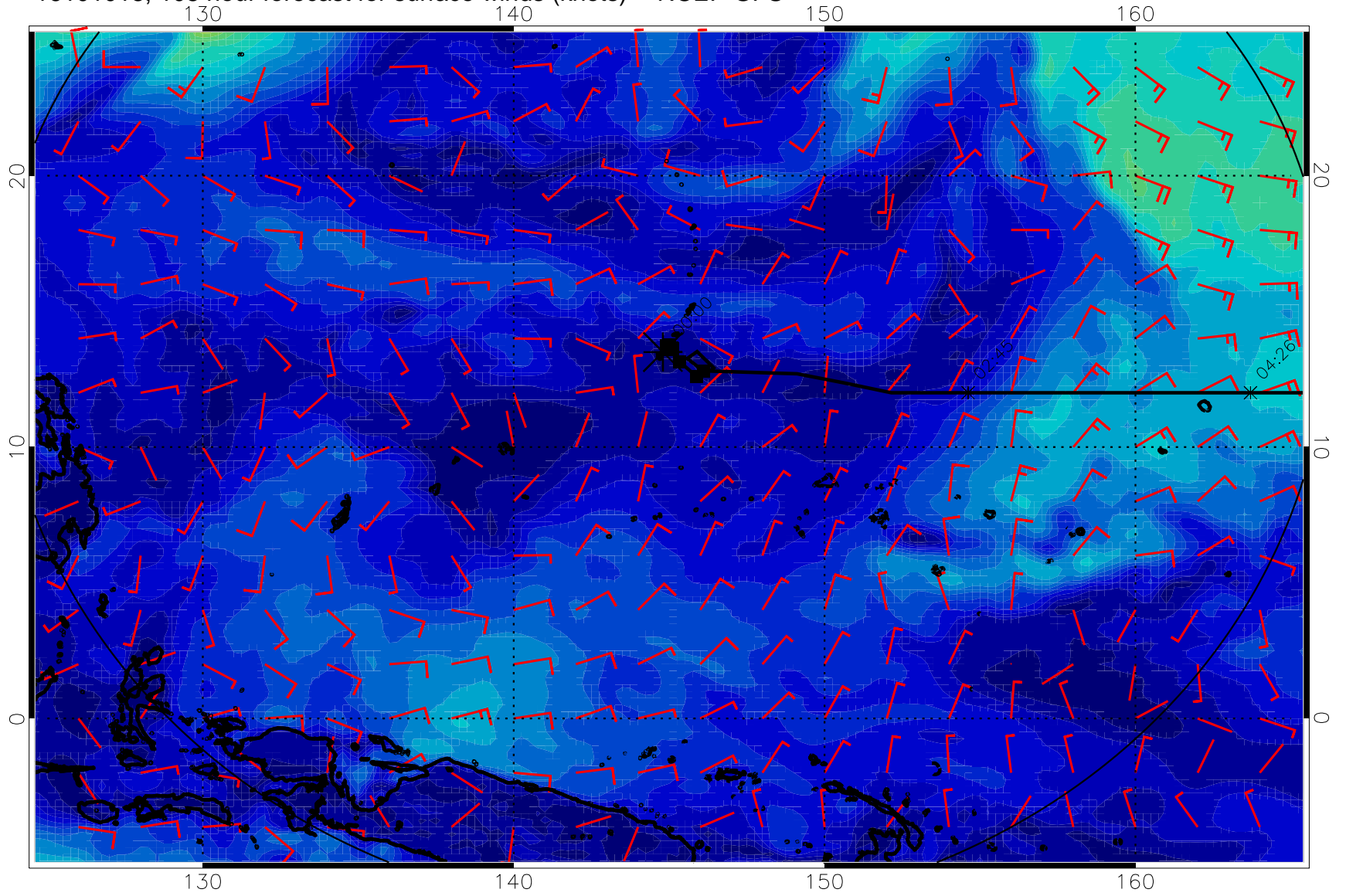
16101018, 108 hour forecast for surface winds (knots) -- NCEP GFS
