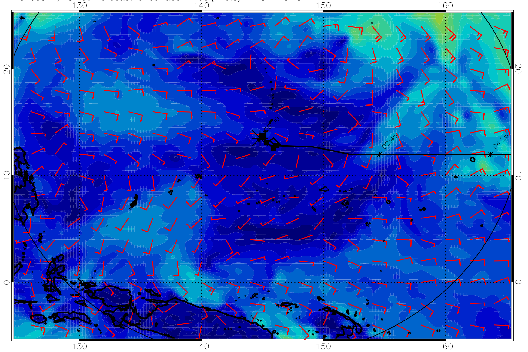
16100912, 78 hour forecast for surface winds (knots) -- NCEP GFS
