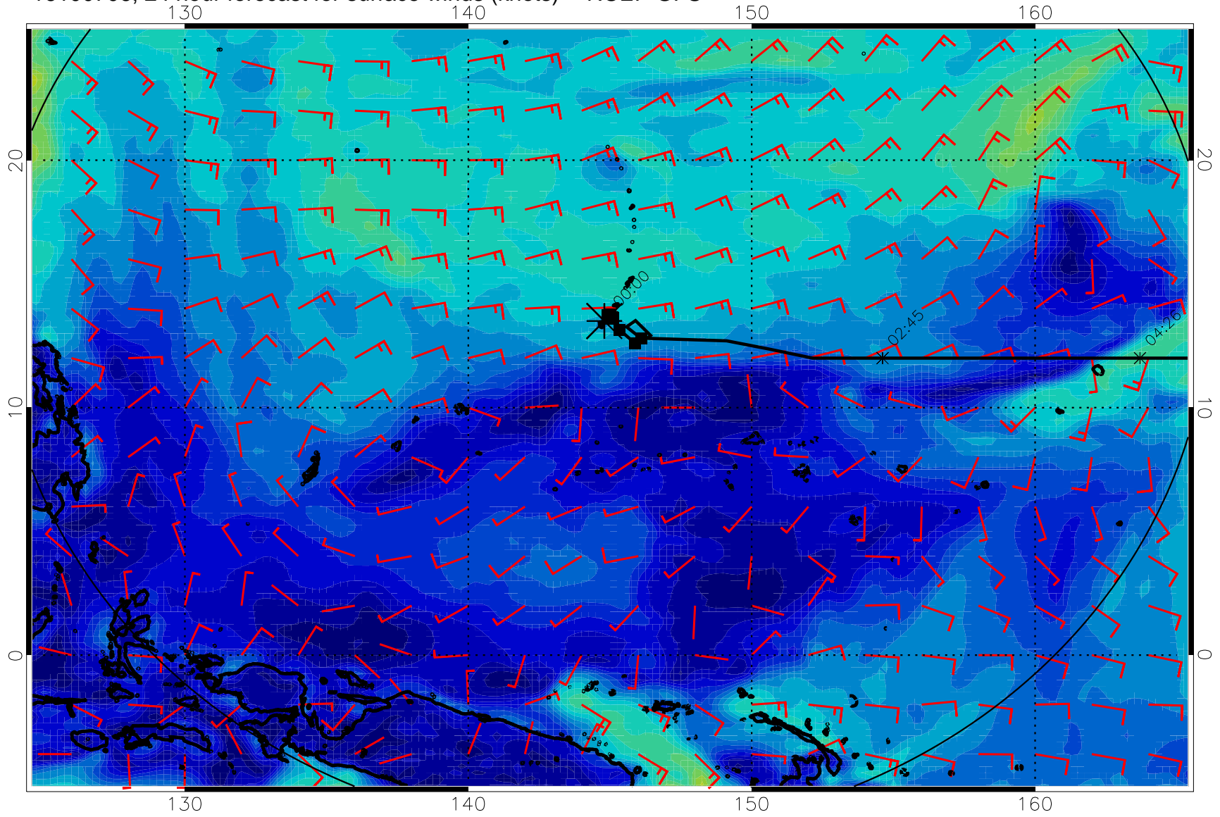
16100706, 24 hour forecast for surface winds (knots) -- NCEP GFS
