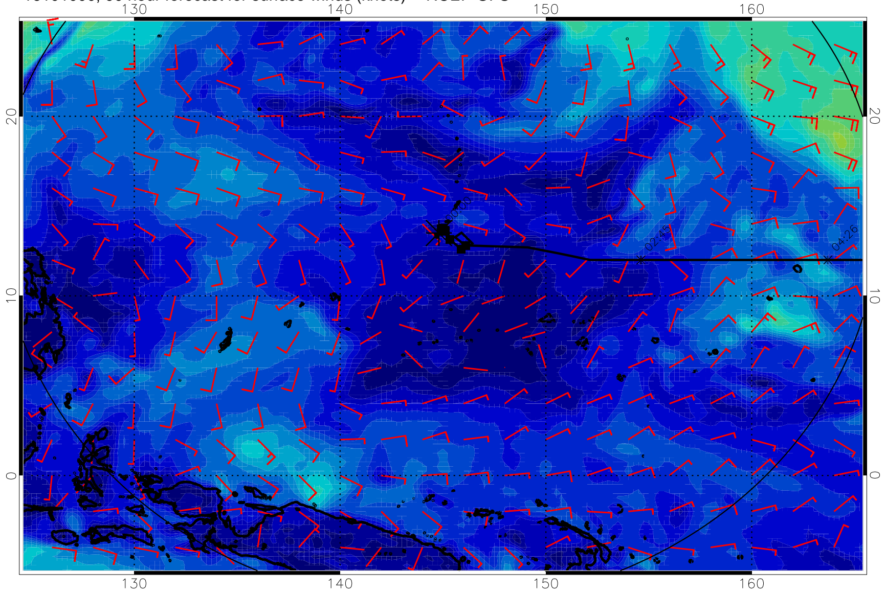
16101000, 90 hour forecast for surface winds (knots) -- NCEP GFS
