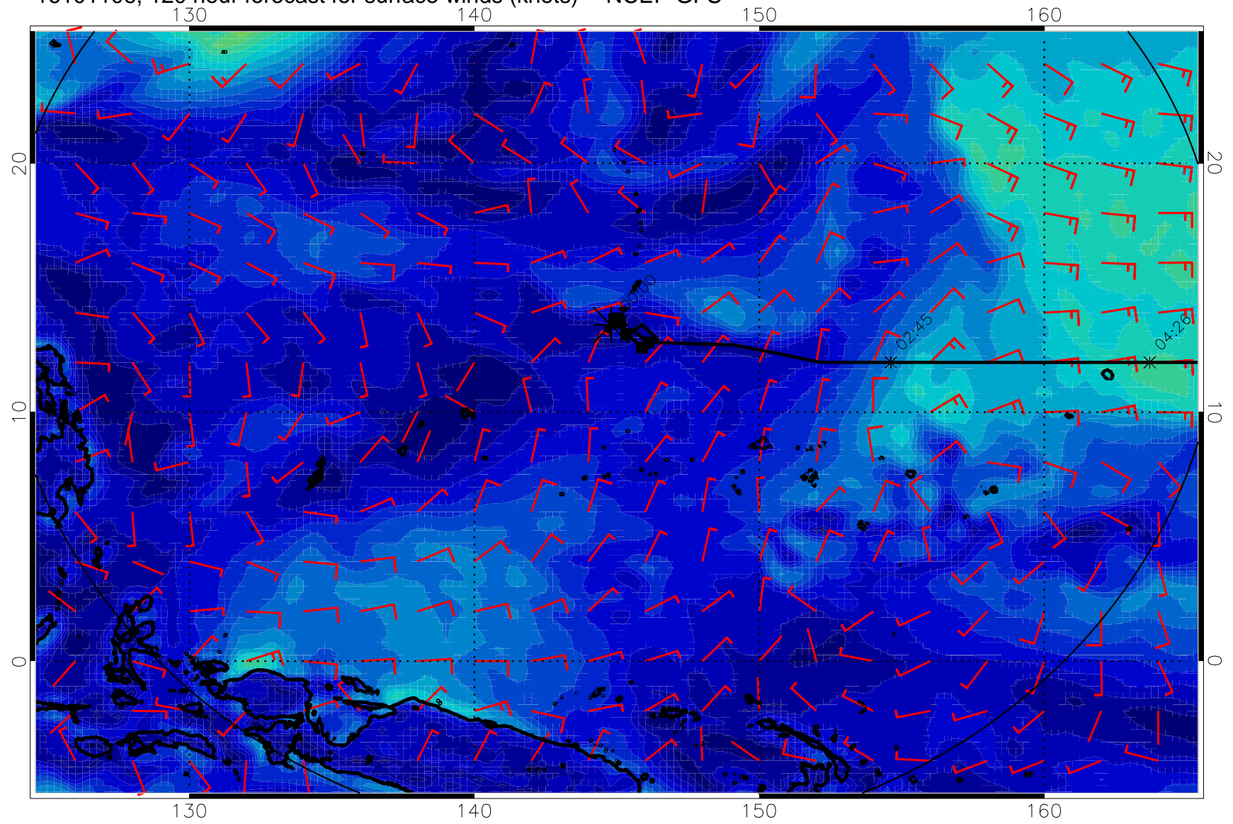
16101106, 120 hour forecast for surface winds (knots) -- NCEP GFS
