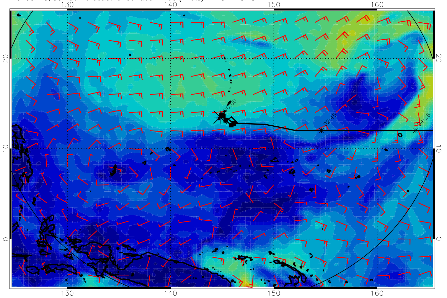
16100718, 36 hour forecast for surface winds (knots) -- NCEP GFS
