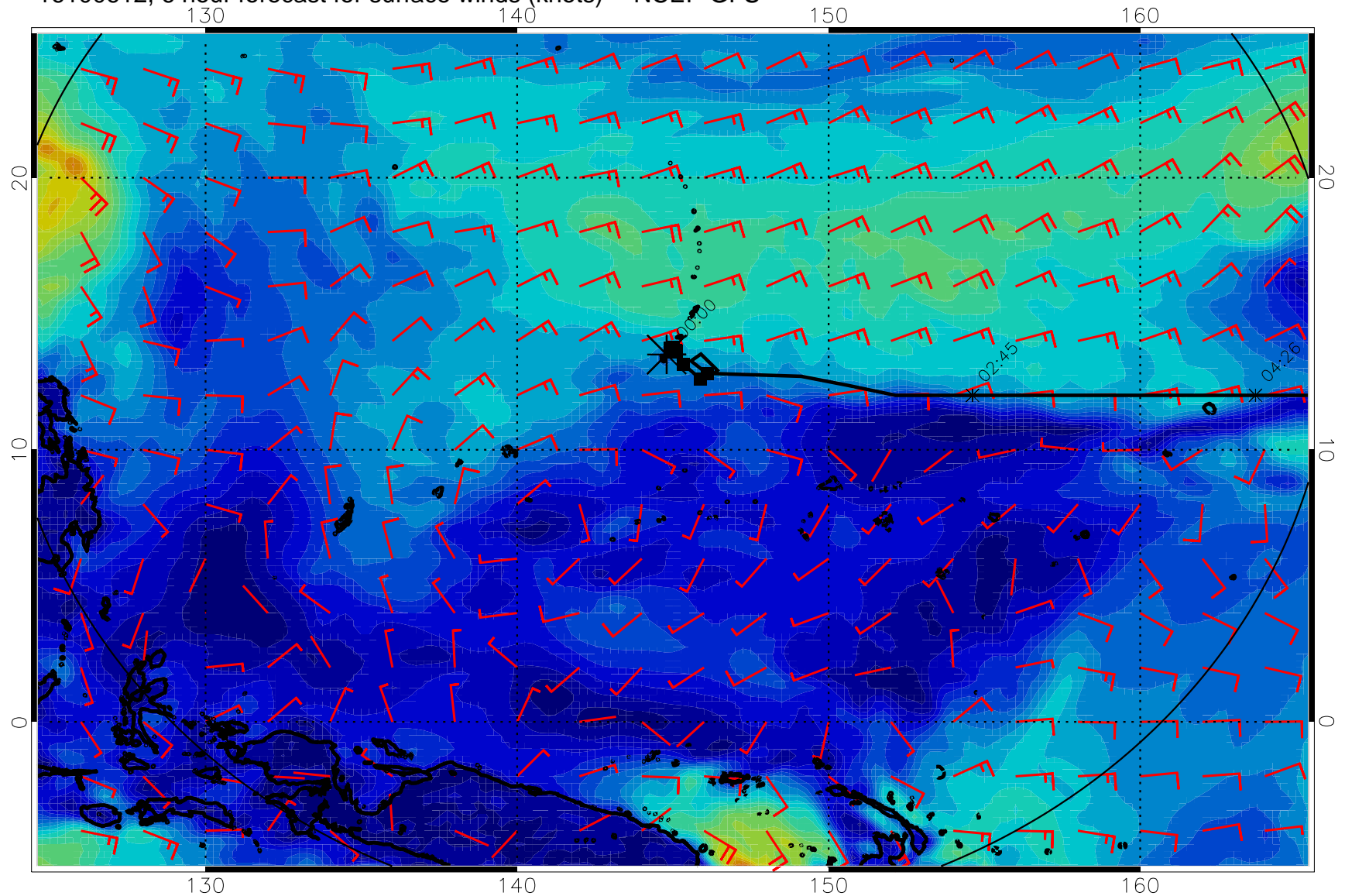
16100612, 6 hour forecast for surface winds (knots) -- NCEP GFS
