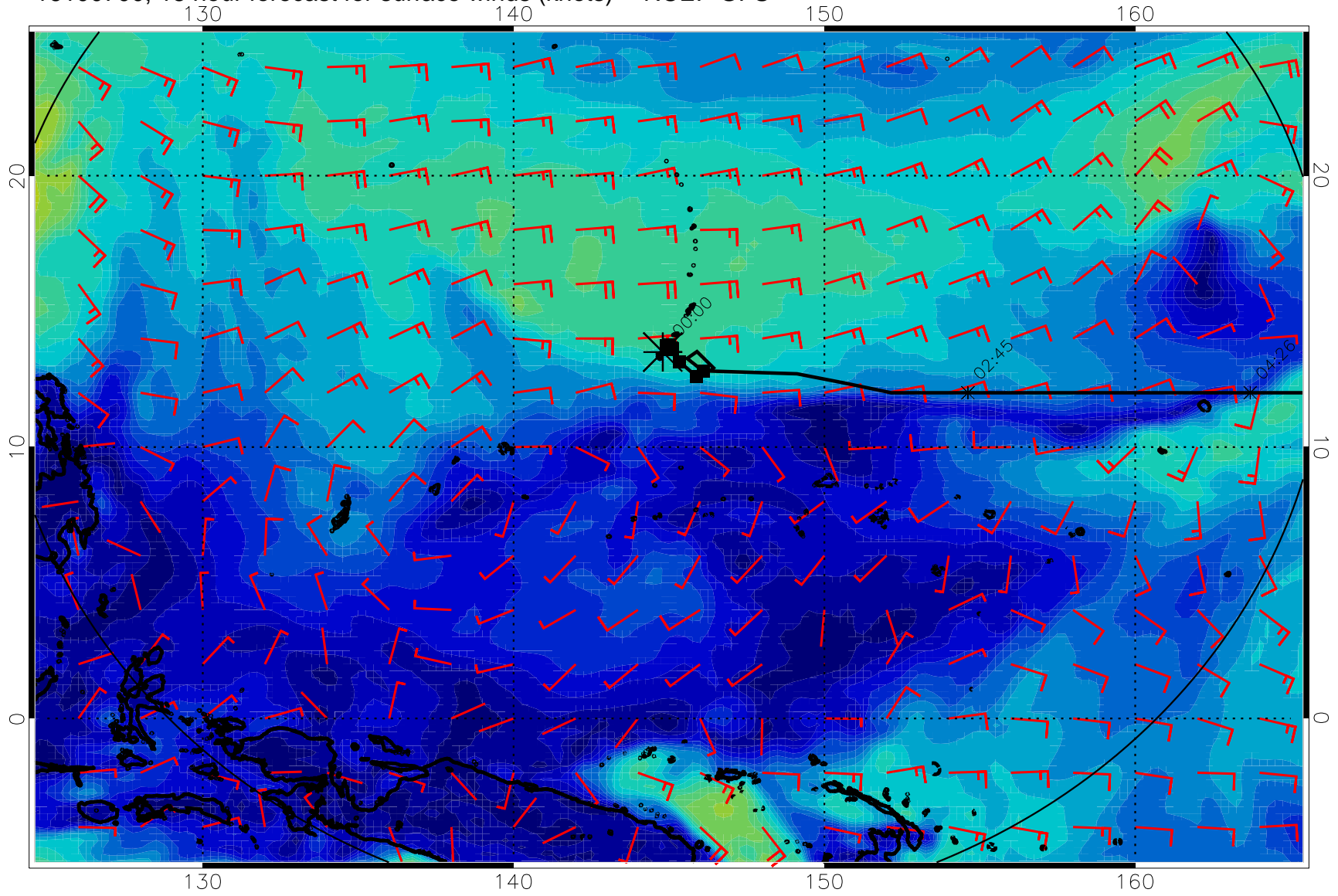
16100700, 18 hour forecast for surface winds (knots) -- NCEP GFS
