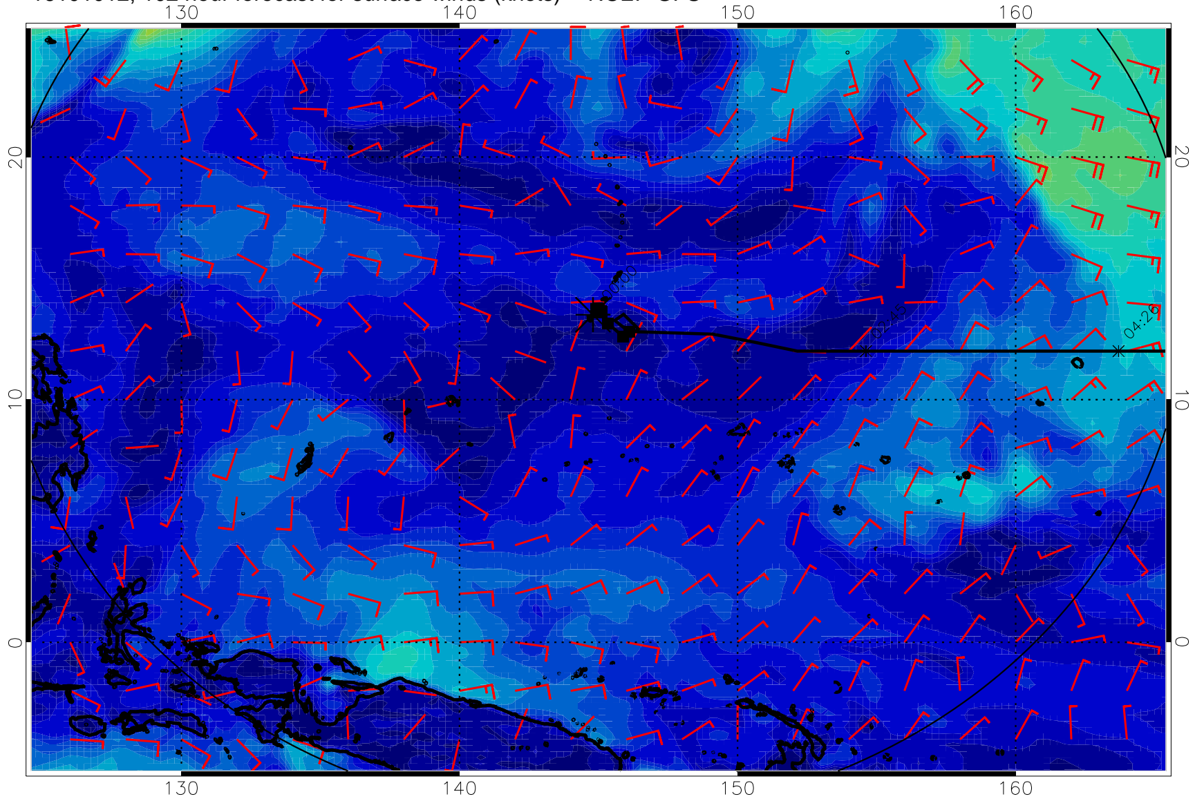
16101012, 102 hour forecast for surface winds (knots) -- NCEP GFS
