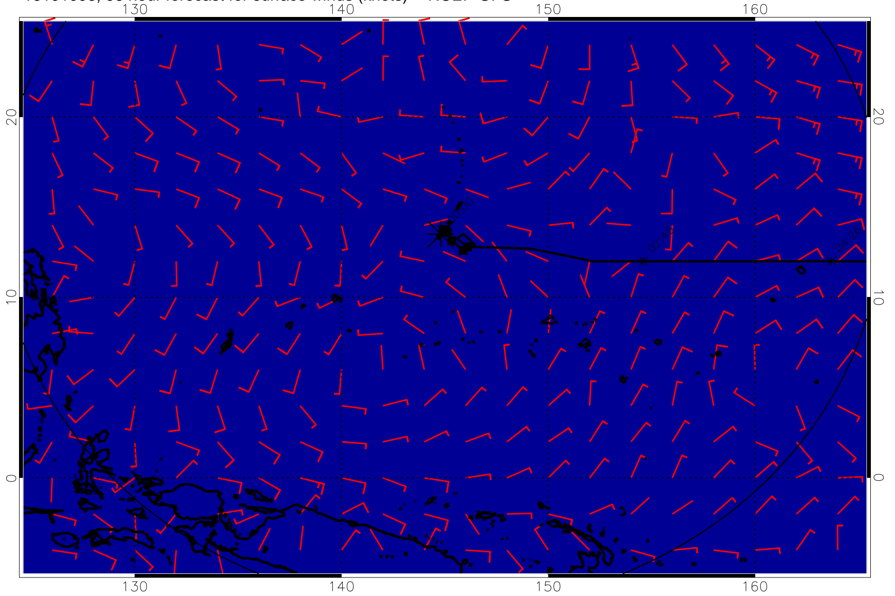
16101006, 96 hour forecast for surface winds (knots) -- NCEP GFS
