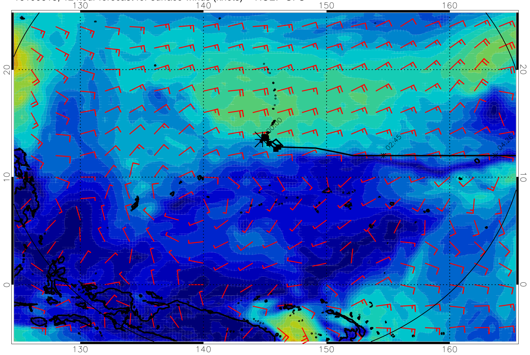
16100618, 12 hour forecast for surface winds (knots) -- NCEP GFS
