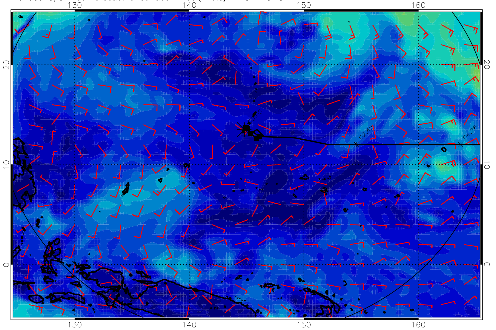
16100918, 84 hour forecast for surface winds (knots) -- NCEP GFS
