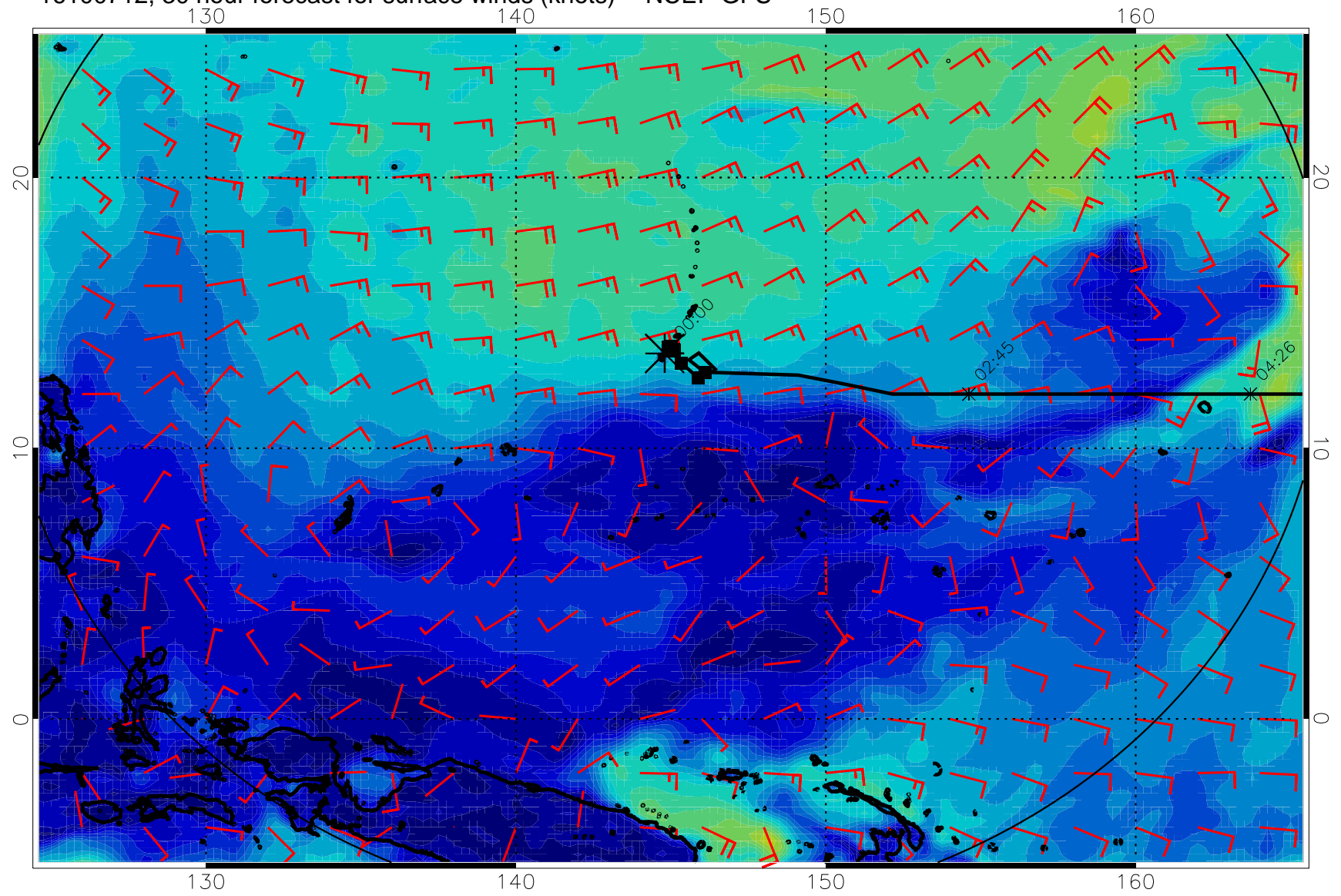
16100712, 30 hour forecast for surface winds (knots) -- NCEP GFS
