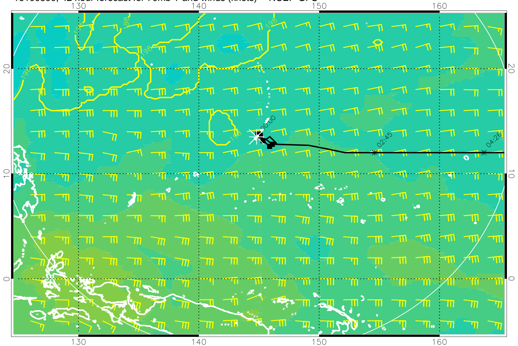
16100800, 42 hour forecast for 70mb T and winds (knots) -- NCEP GFS
