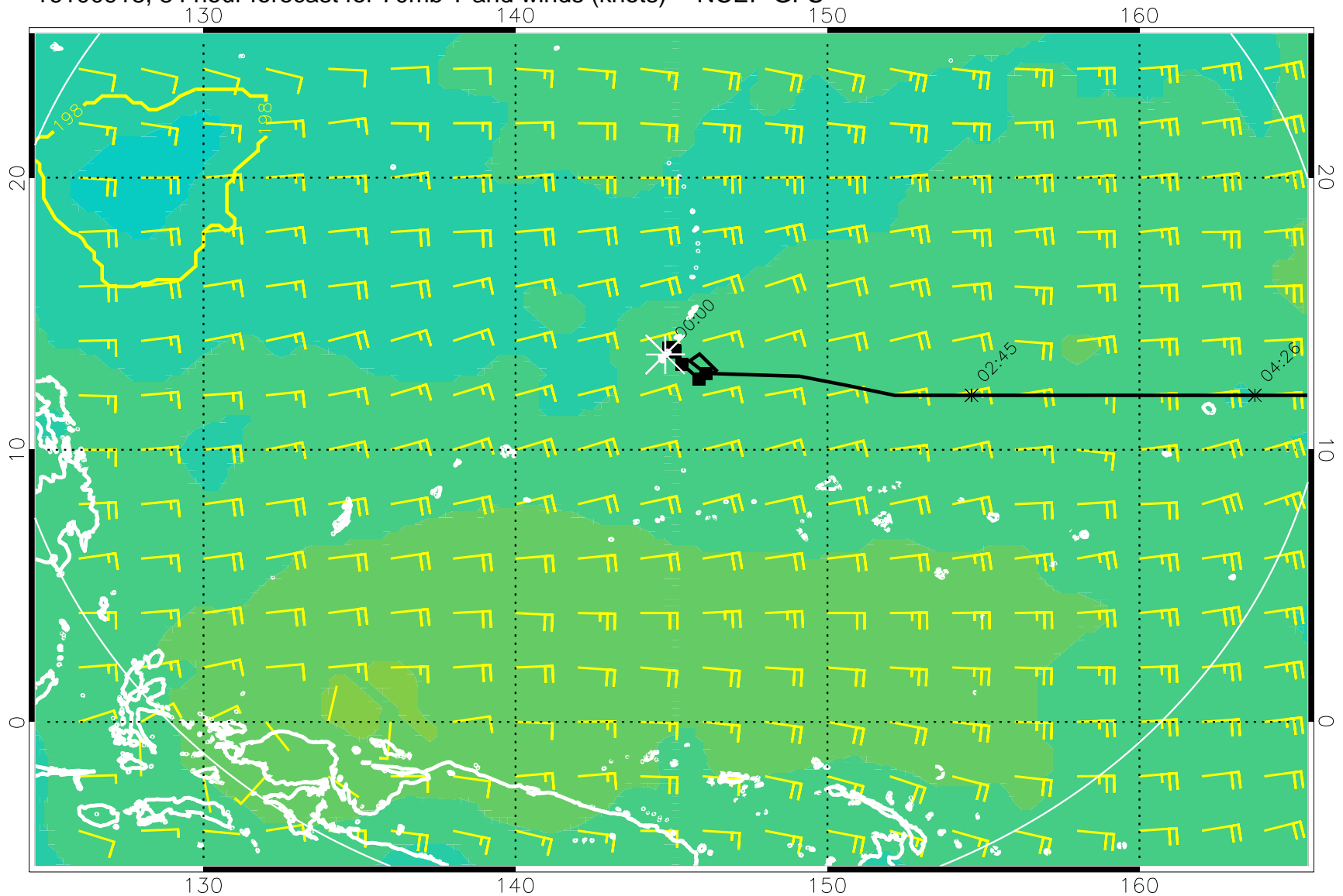
16100918, 84 hour forecast for 70mb T and winds (knots) -- NCEP GFS
