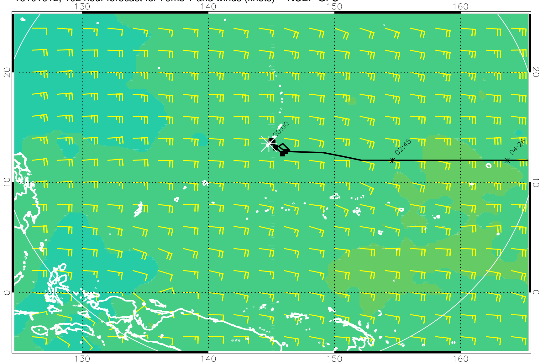
16101012, 102 hour forecast for 70mb T and winds (knots) -- NCEP GFS
