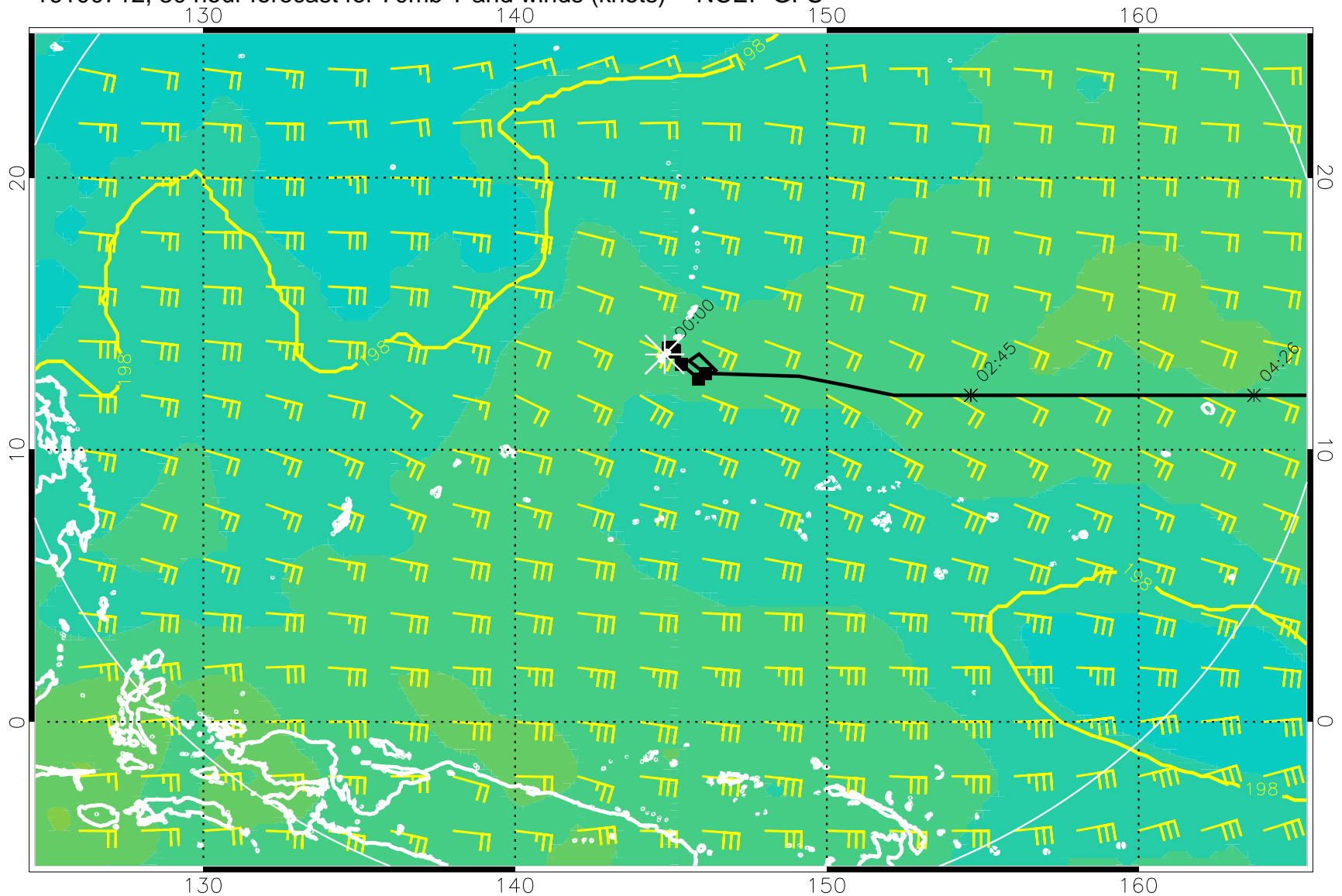
16100712, 30 hour forecast for 70mb T and winds (knots) -- NCEP GFS
