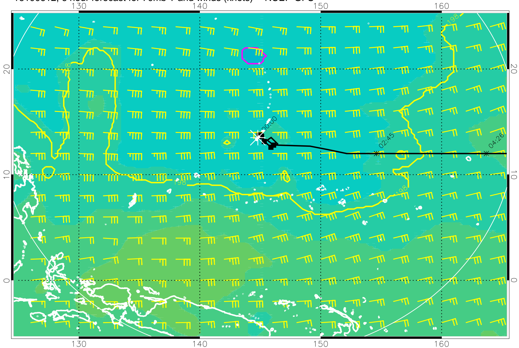
16100612, 6 hour forecast for 70mb T and winds (knots) -- NCEP GFS
