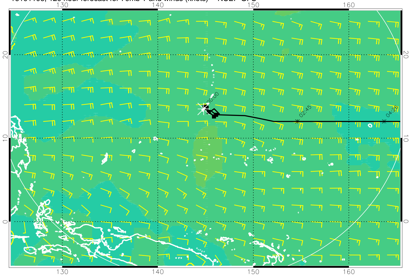
16101106, 120 hour forecast for 70mb T and winds (knots) -- NCEP GFS
