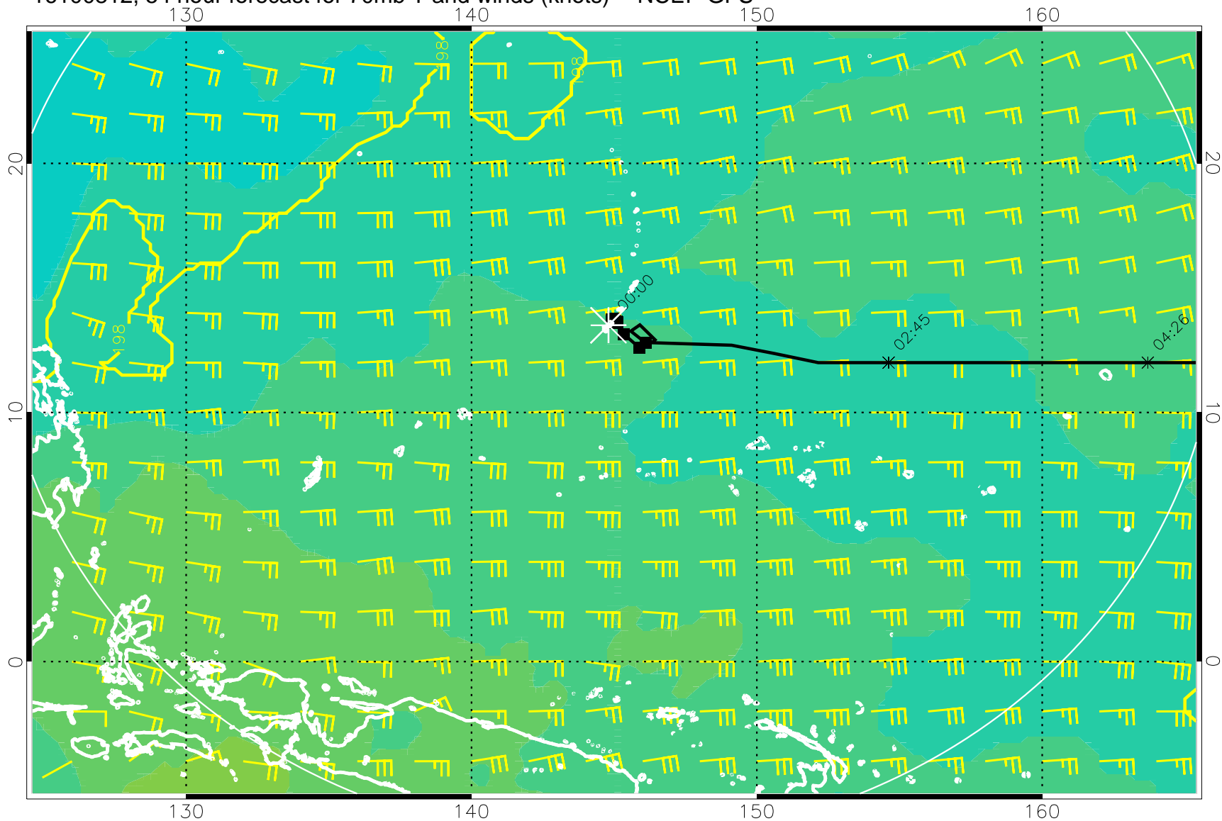
16100812, 54 hour forecast for 70mb T and winds (knots) -- NCEP GFS
