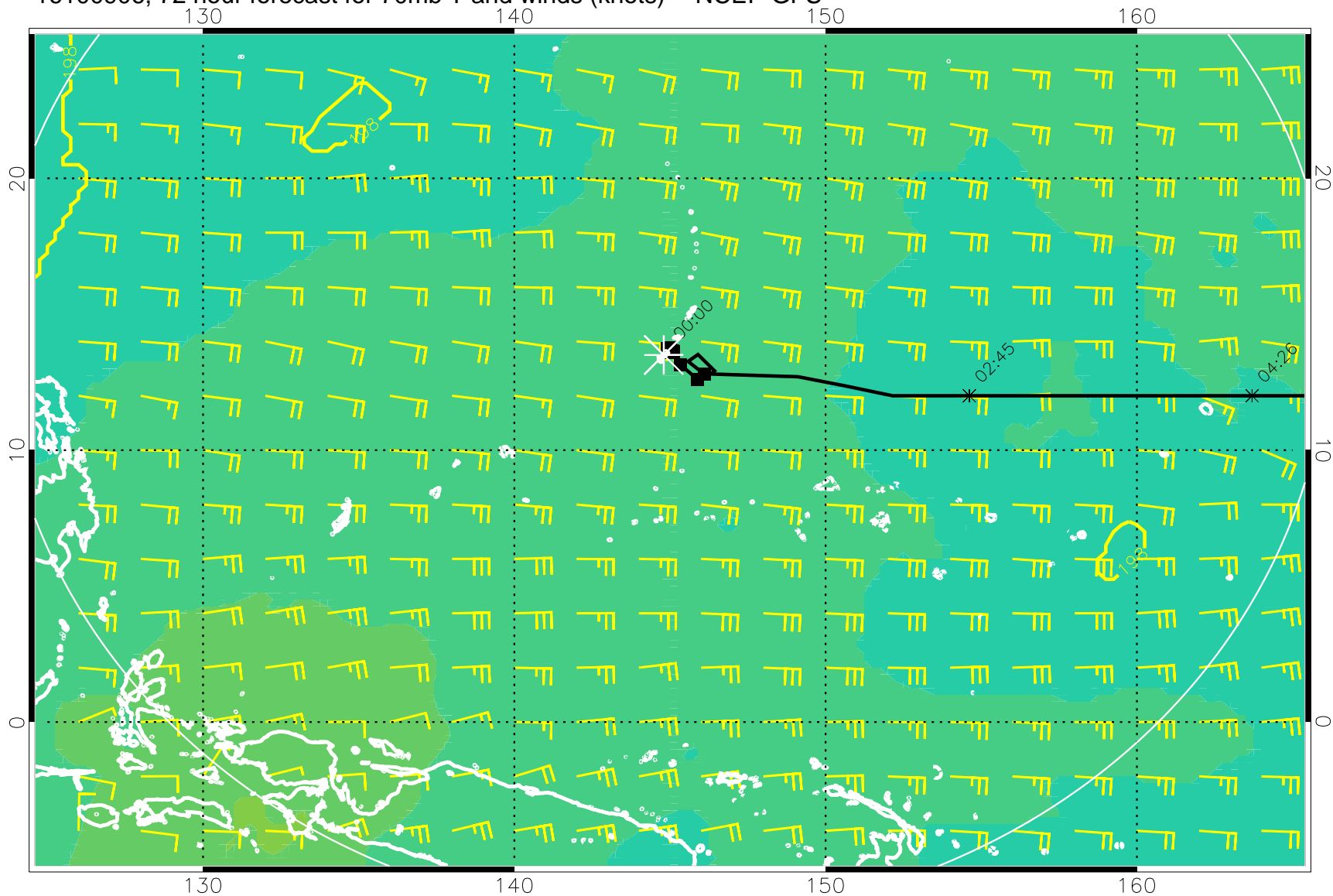
16100906, 72 hour forecast for 70mb T and winds (knots) -- NCEP GFS
