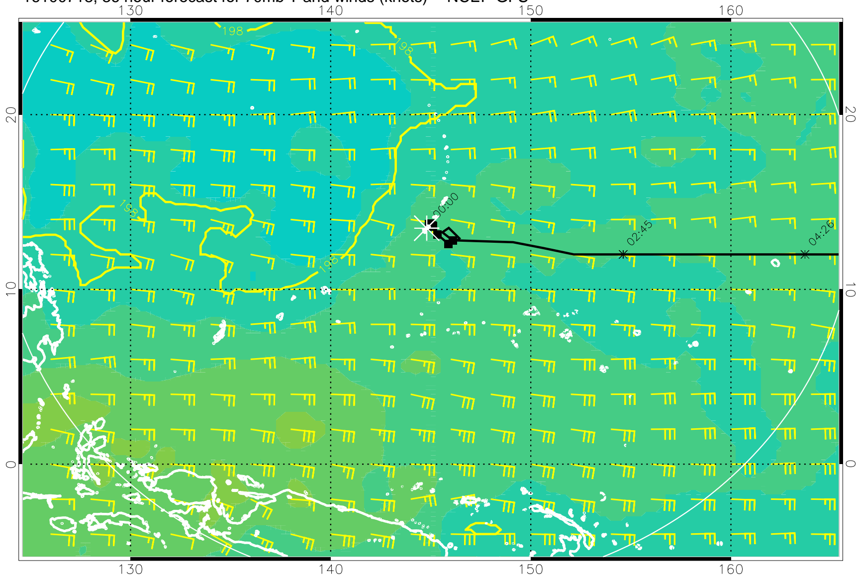
16100718, 36 hour forecast for 70mb T and winds (knots) -- NCEP GFS
