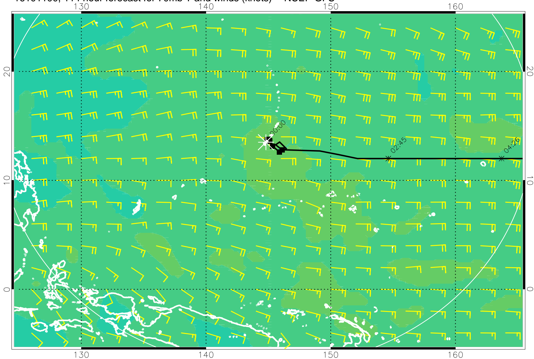
16101100, 114 hour forecast for 70mb T and winds (knots) -- NCEP GFS
