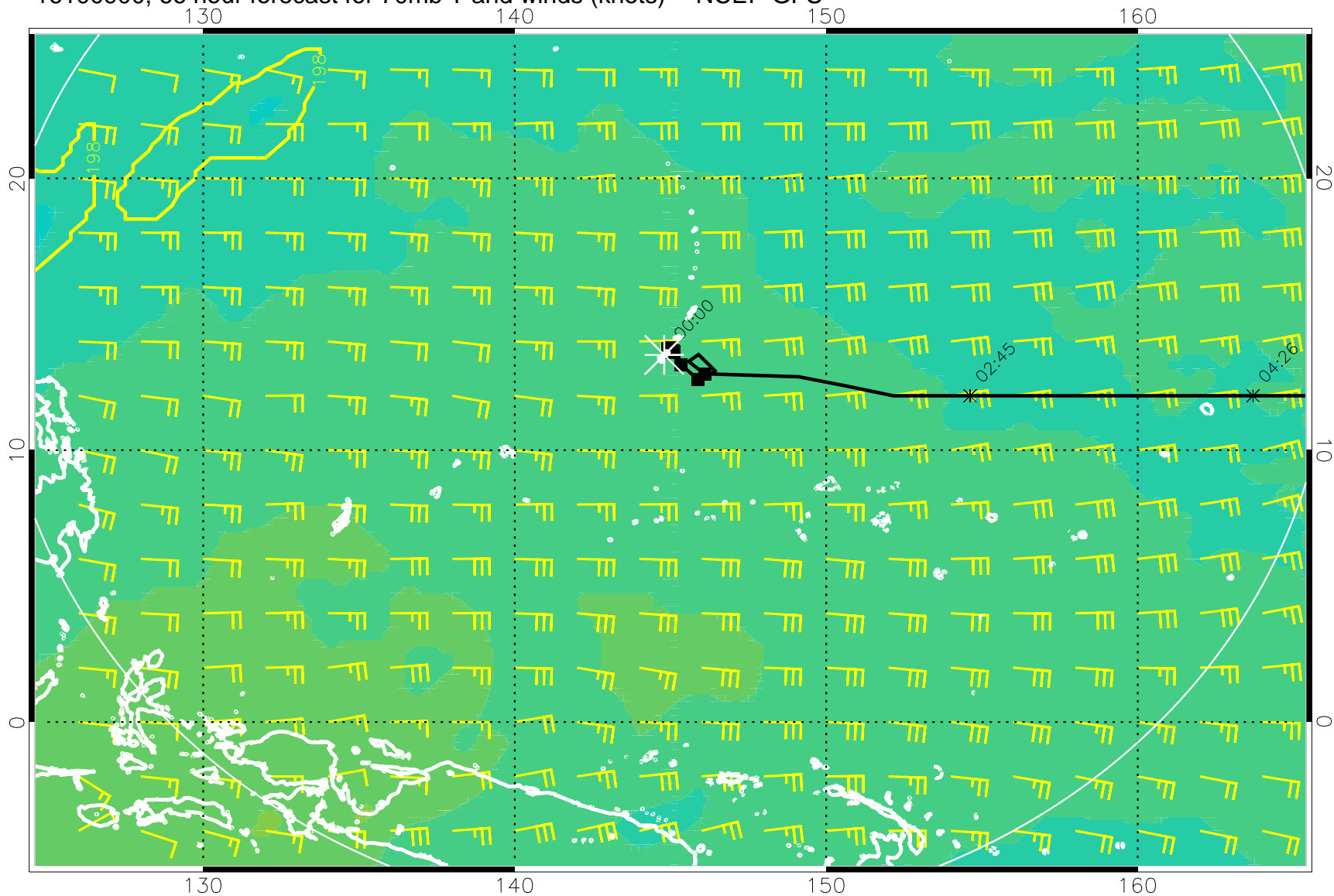
16100900, 66 hour forecast for 70mb T and winds (knots) -- NCEP GFS
