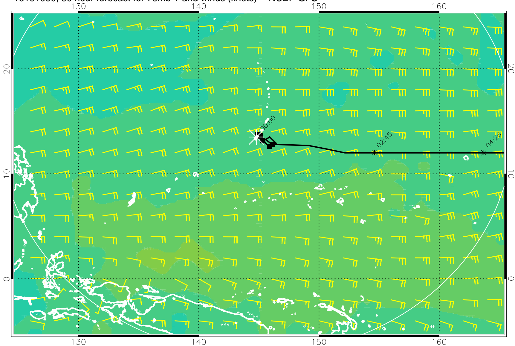
16101000, 90 hour forecast for 70mb T and winds (knots) -- NCEP GFS
