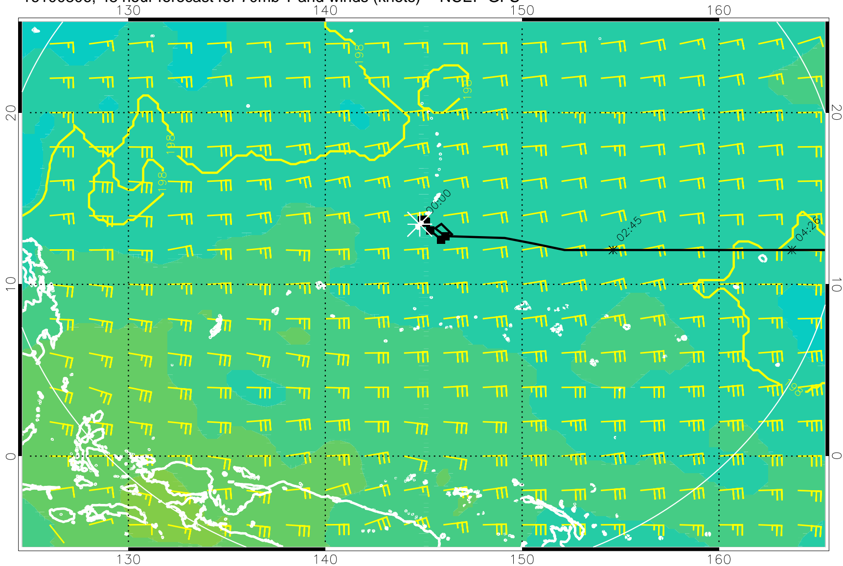
16100806, 48 hour forecast for 70mb T and winds (knots) -- NCEP GFS
