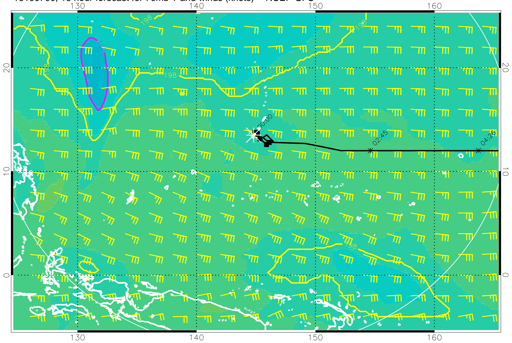
16100700, 18 hour forecast for 70mb T and winds (knots) -- NCEP GFS
