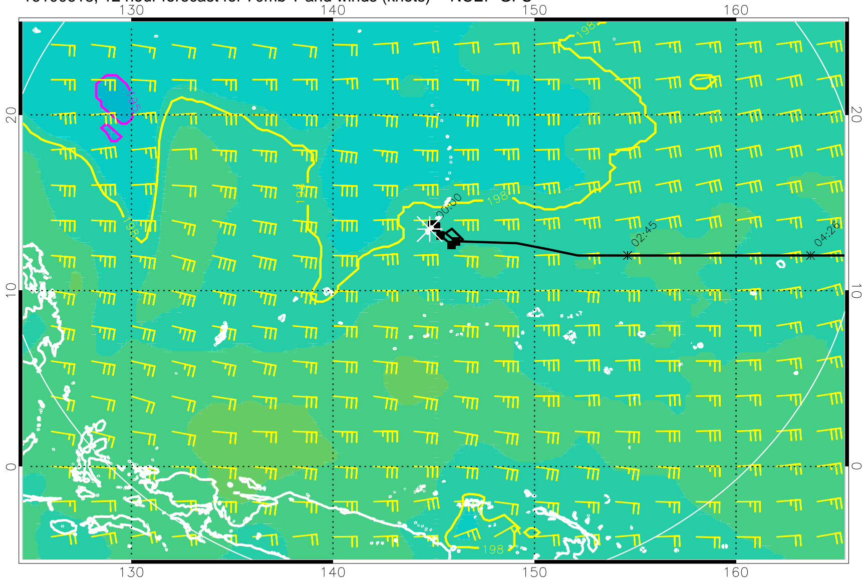
16100618, 12 hour forecast for 70mb T and winds (knots) -- NCEP GFS
