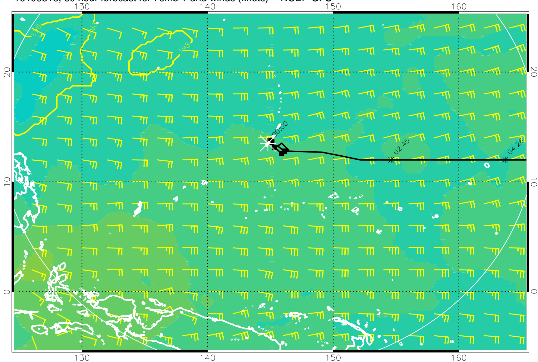
16100818, 60 hour forecast for 70mb T and winds (knots) -- NCEP GFS
