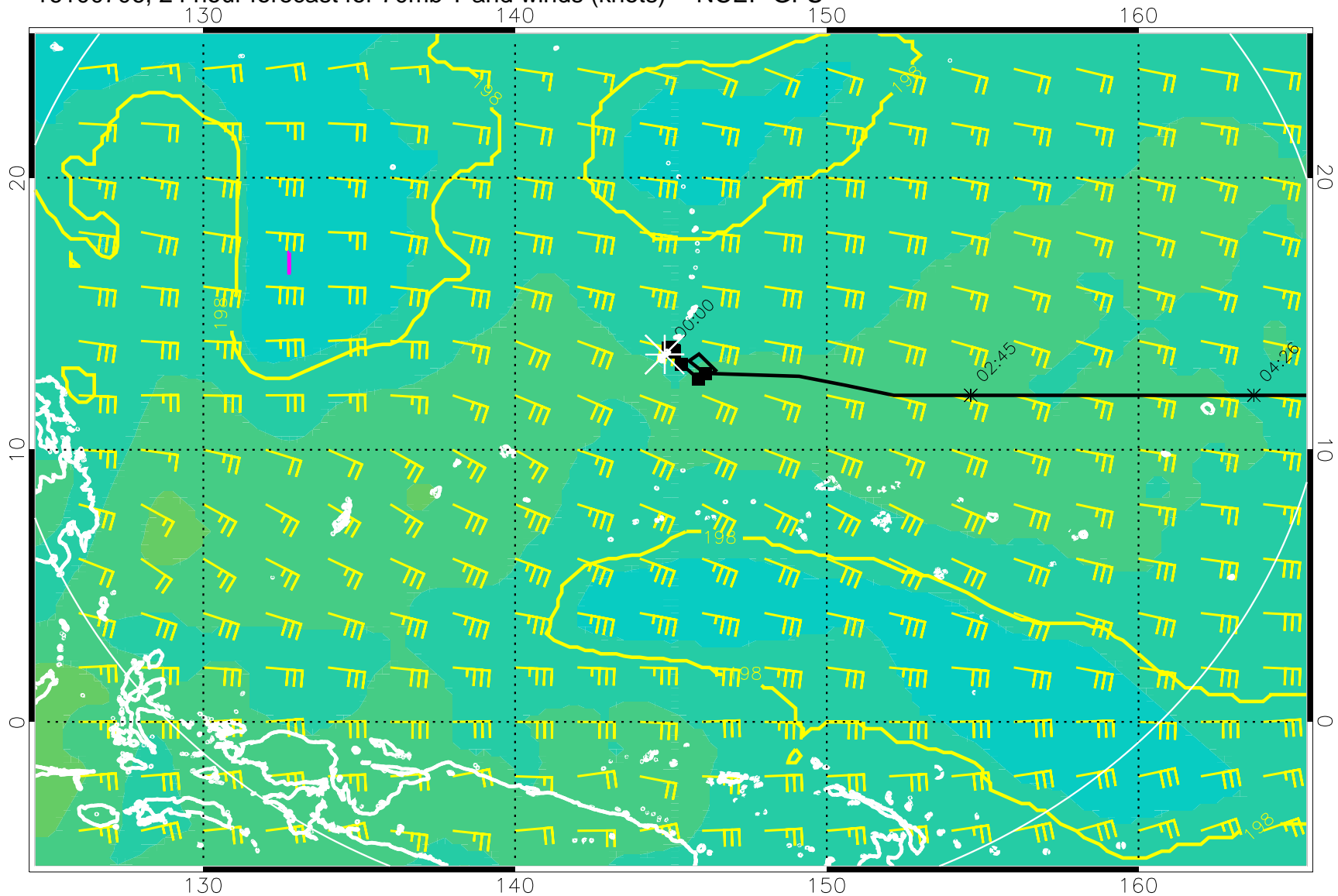
16100706, 24 hour forecast for 70mb T and winds (knots) -- NCEP GFS
