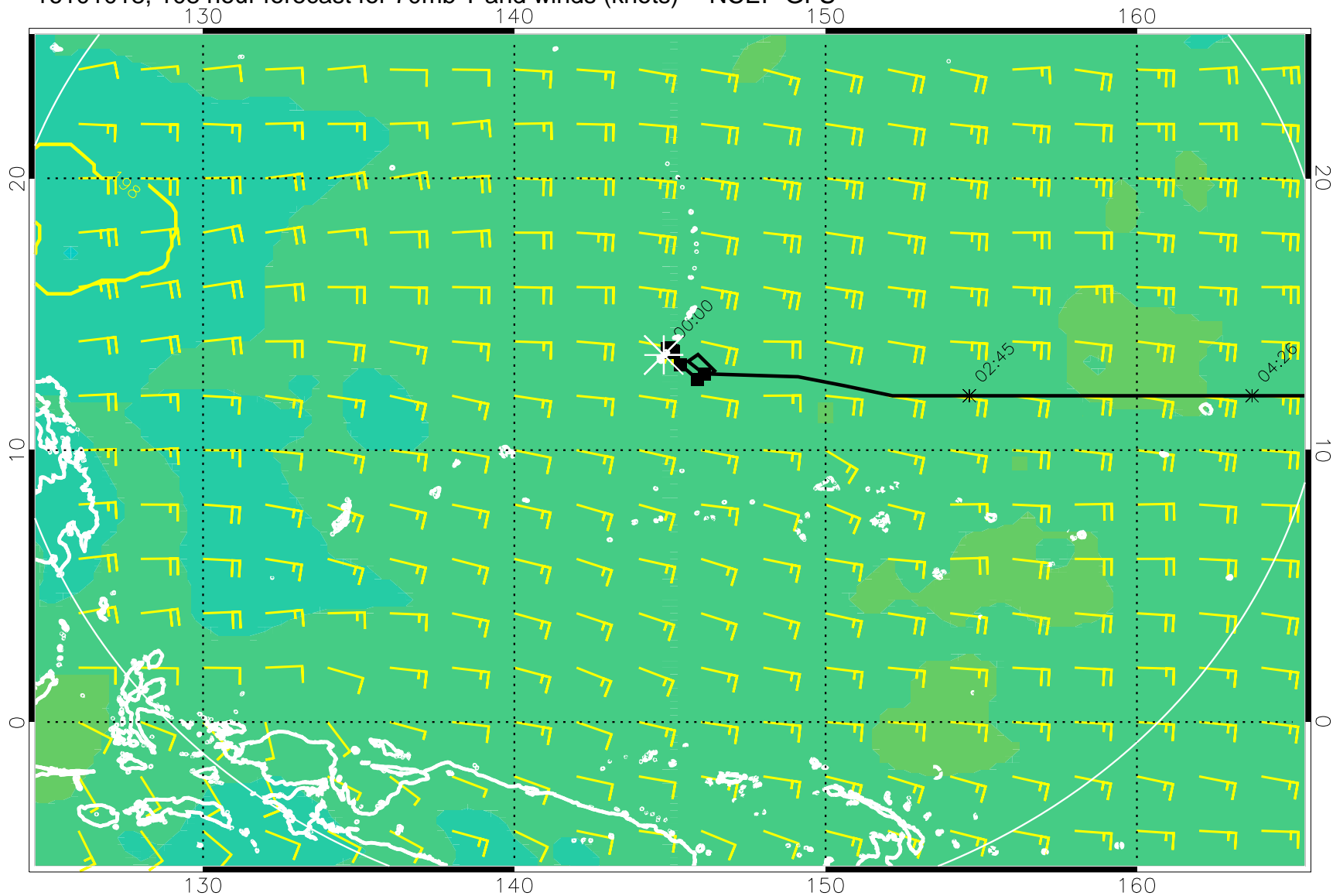
16101018, 108 hour forecast for 70mb T and winds (knots) -- NCEP GFS
