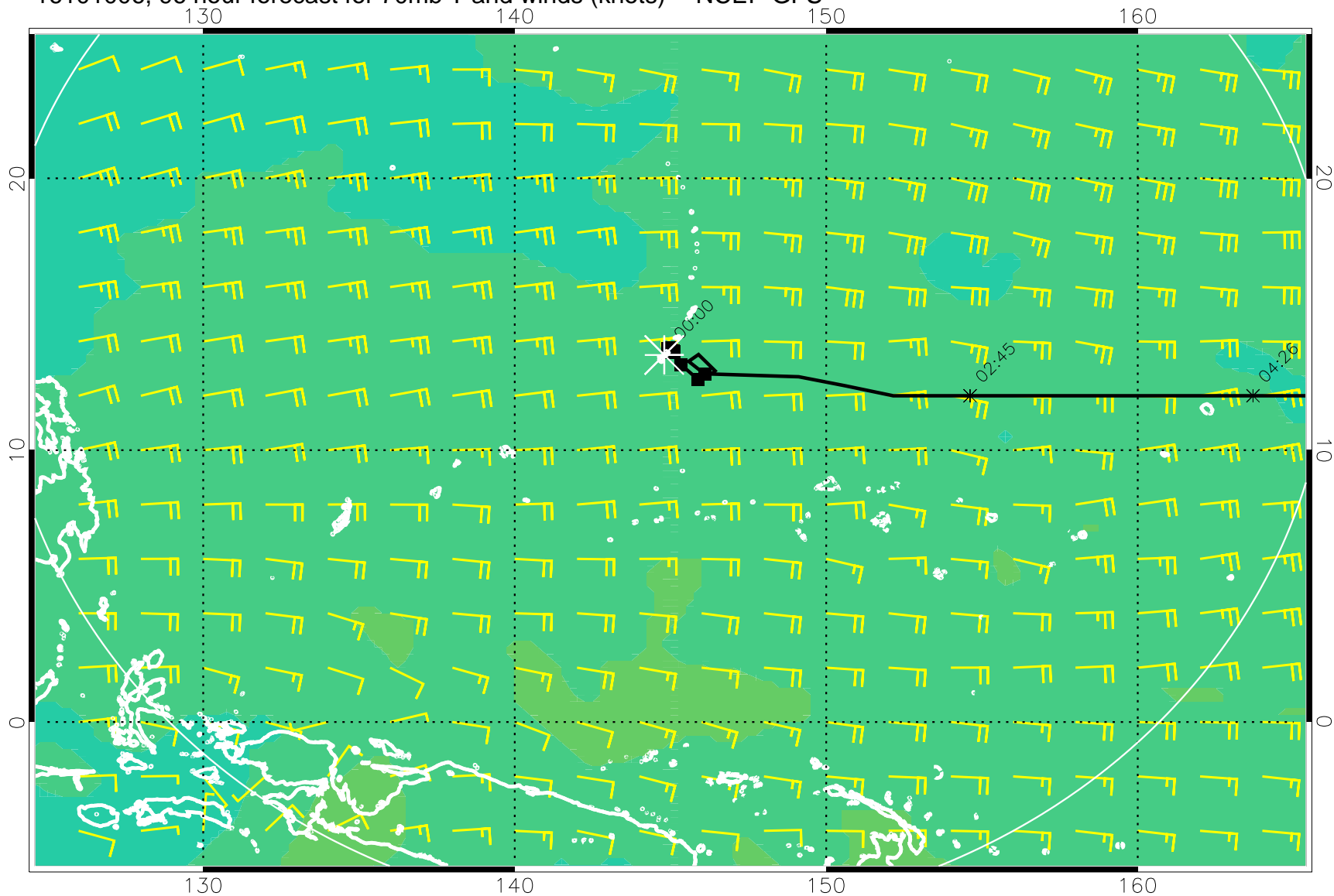
16101006, 96 hour forecast for 70mb T and winds (knots) -- NCEP GFS
