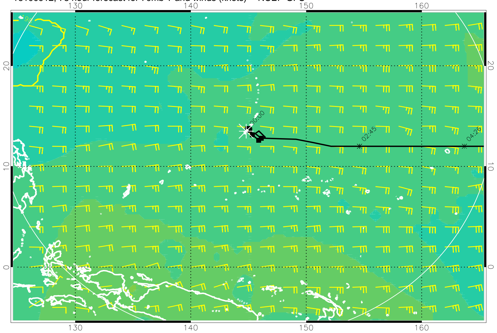
16100912, 78 hour forecast for 70mb T and winds (knots) -- NCEP GFS
