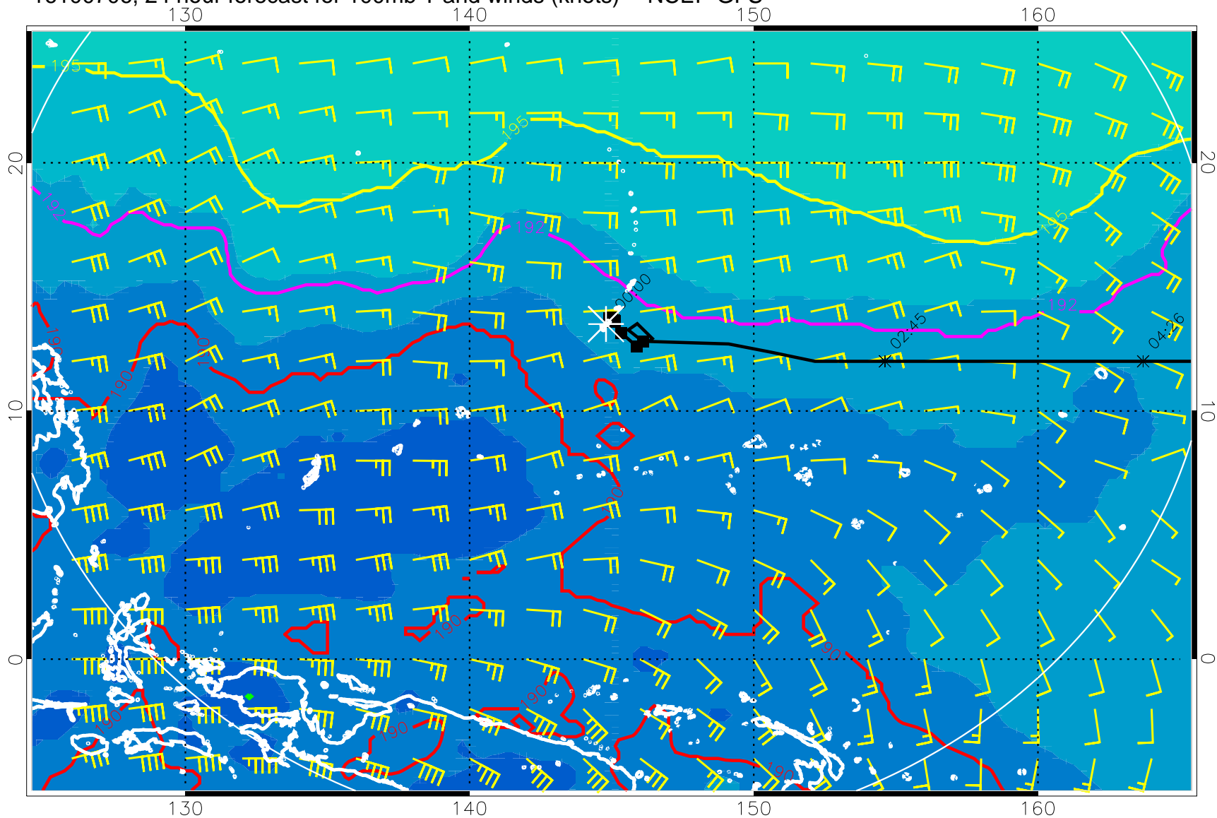
16100706, 24 hour forecast for 100mb T and winds (knots) -- NCEP GFS
