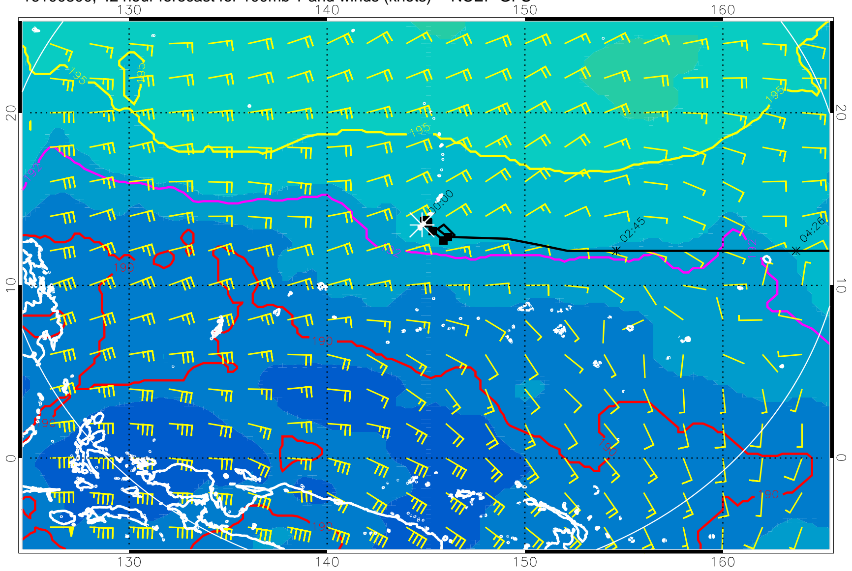
16100800, 42 hour forecast for 100mb T and winds (knots) -- NCEP GFS
