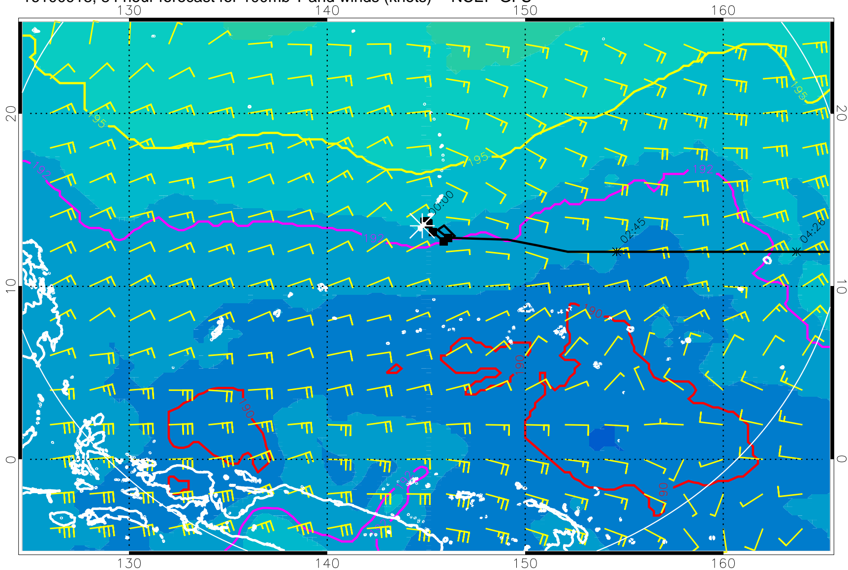
16100918, 84 hour forecast for 100mb T and winds (knots) -- NCEP GFS
