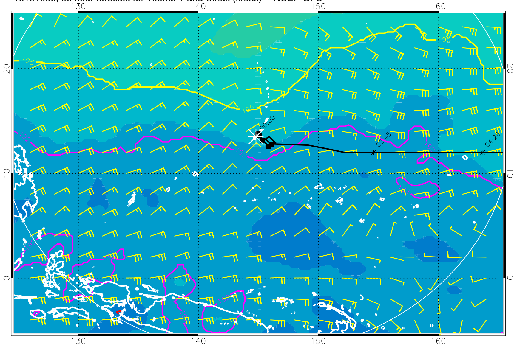
16101006, 96 hour forecast for 100mb T and winds (knots) -- NCEP GFS
