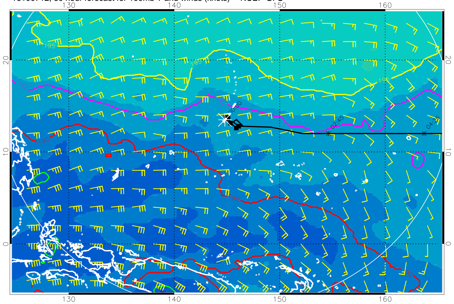
16100712, 30 hour forecast for 100mb T and winds (knots) -- NCEP GFS
