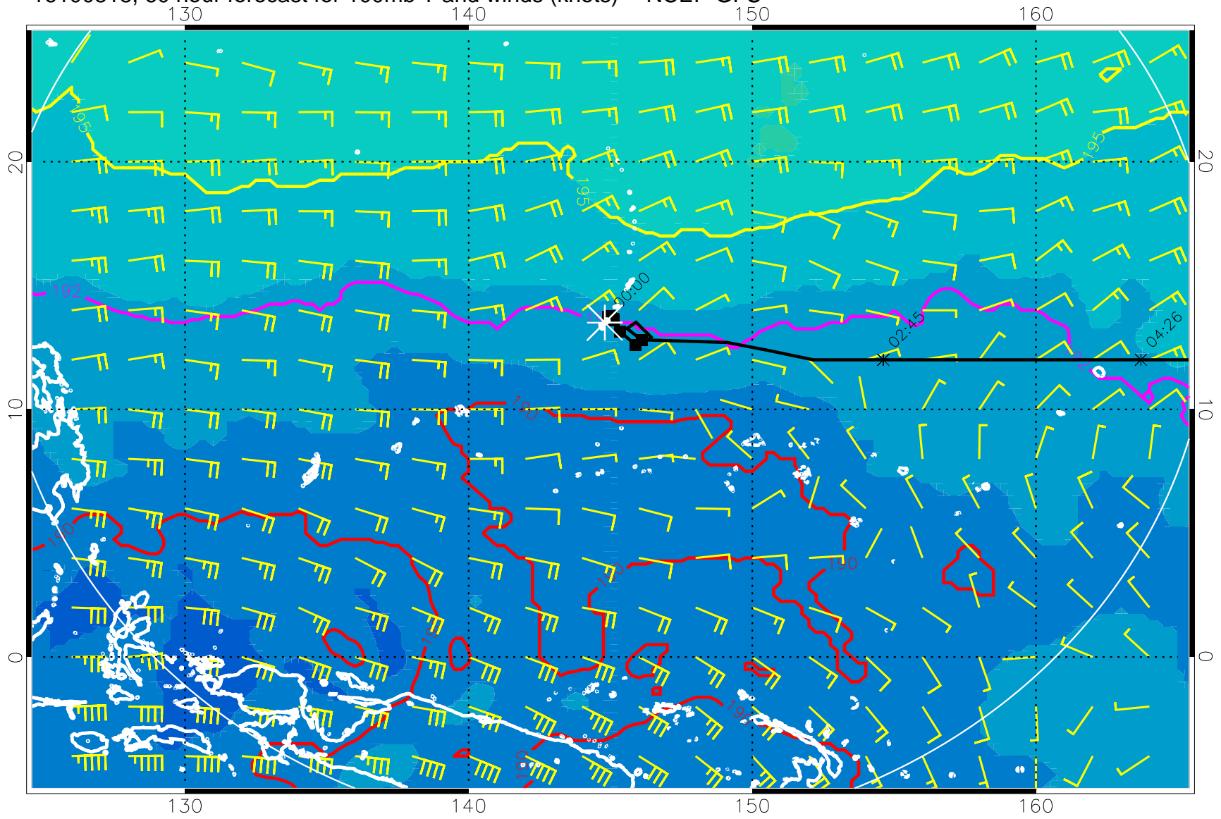
16100818, 60 hour forecast for 100mb T and winds (knots) -- NCEP GFS
