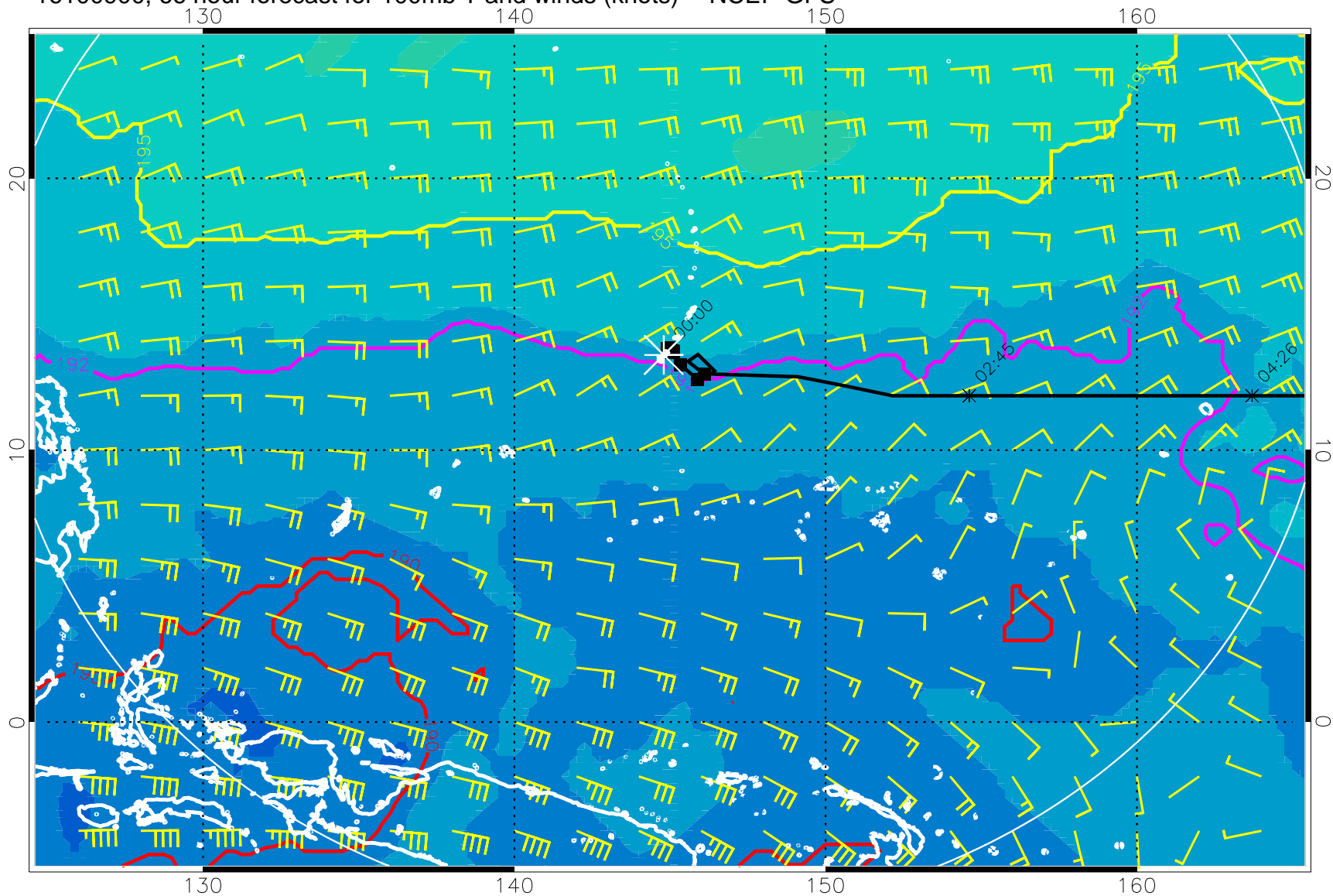
16100900, 66 hour forecast for 100mb T and winds (knots) -- NCEP GFS
