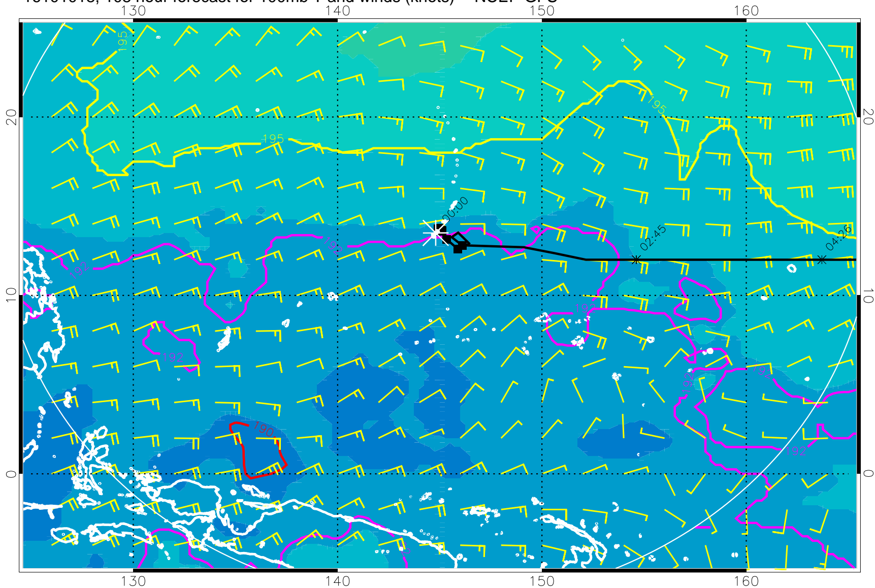
16101018, 108 hour forecast for 100mb T and winds (knots) -- NCEP GFS
