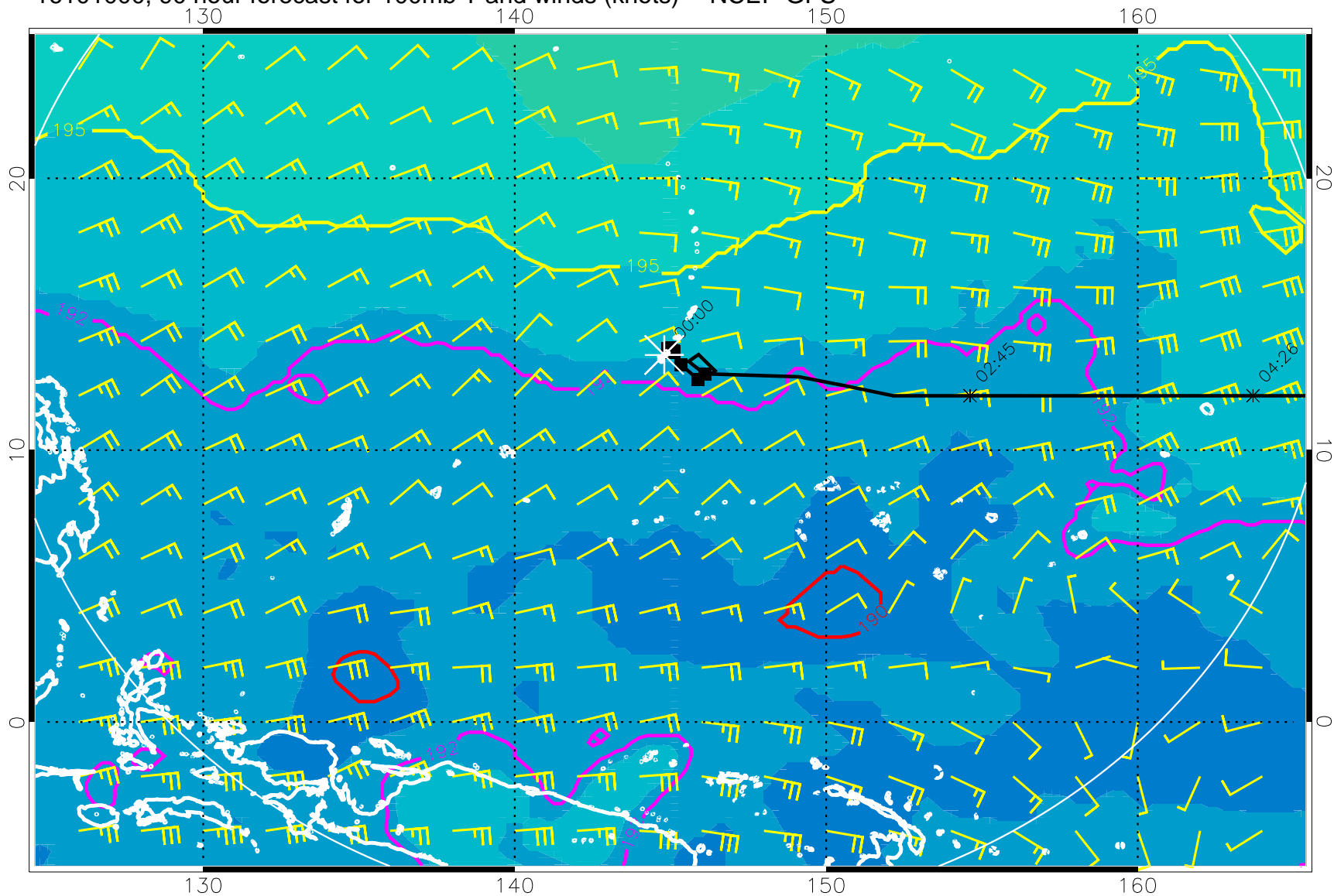
16101000, 90 hour forecast for 100mb T and winds (knots) -- NCEP GFS
