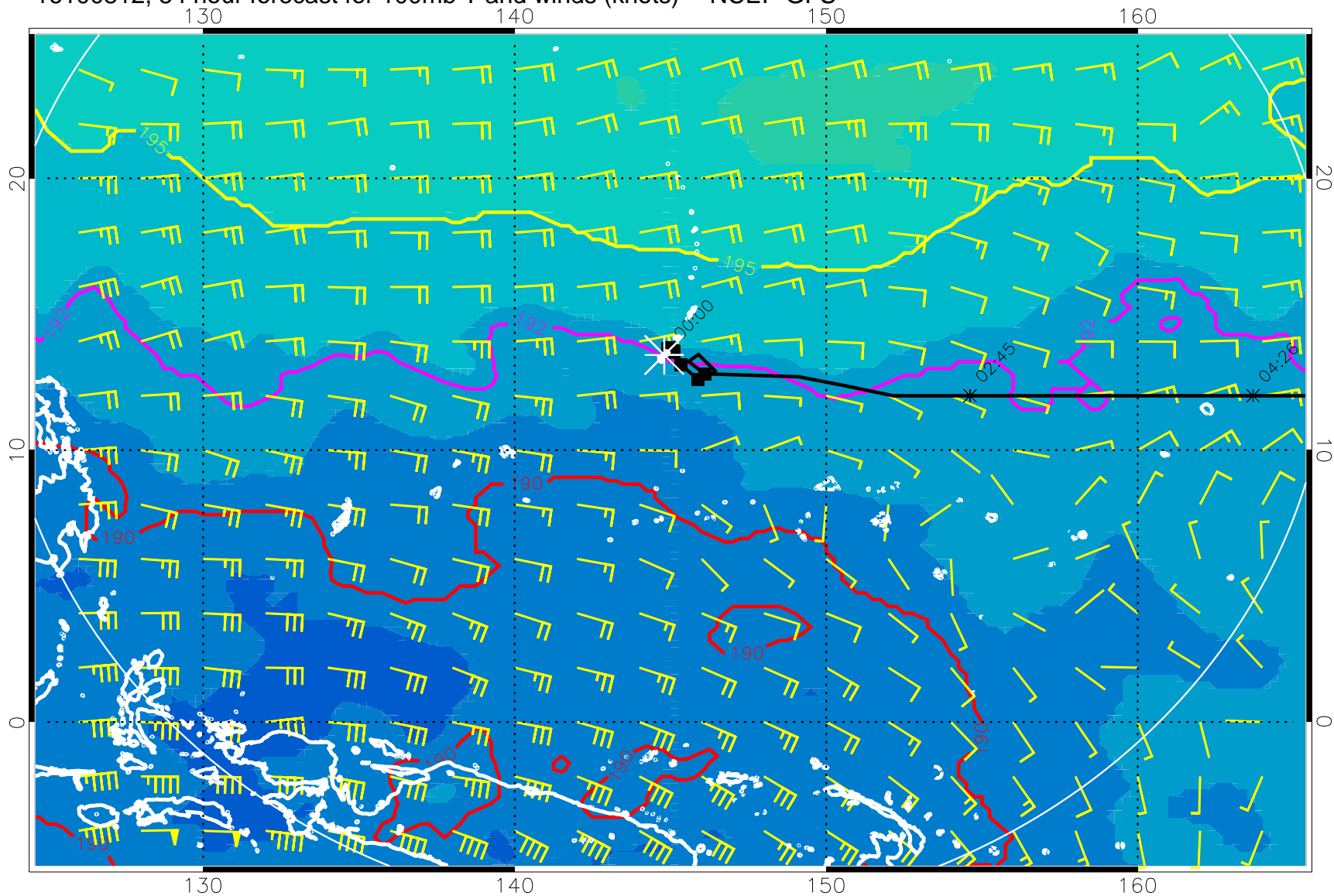
16100812, 54 hour forecast for 100mb T and winds (knots) -- NCEP GFS
