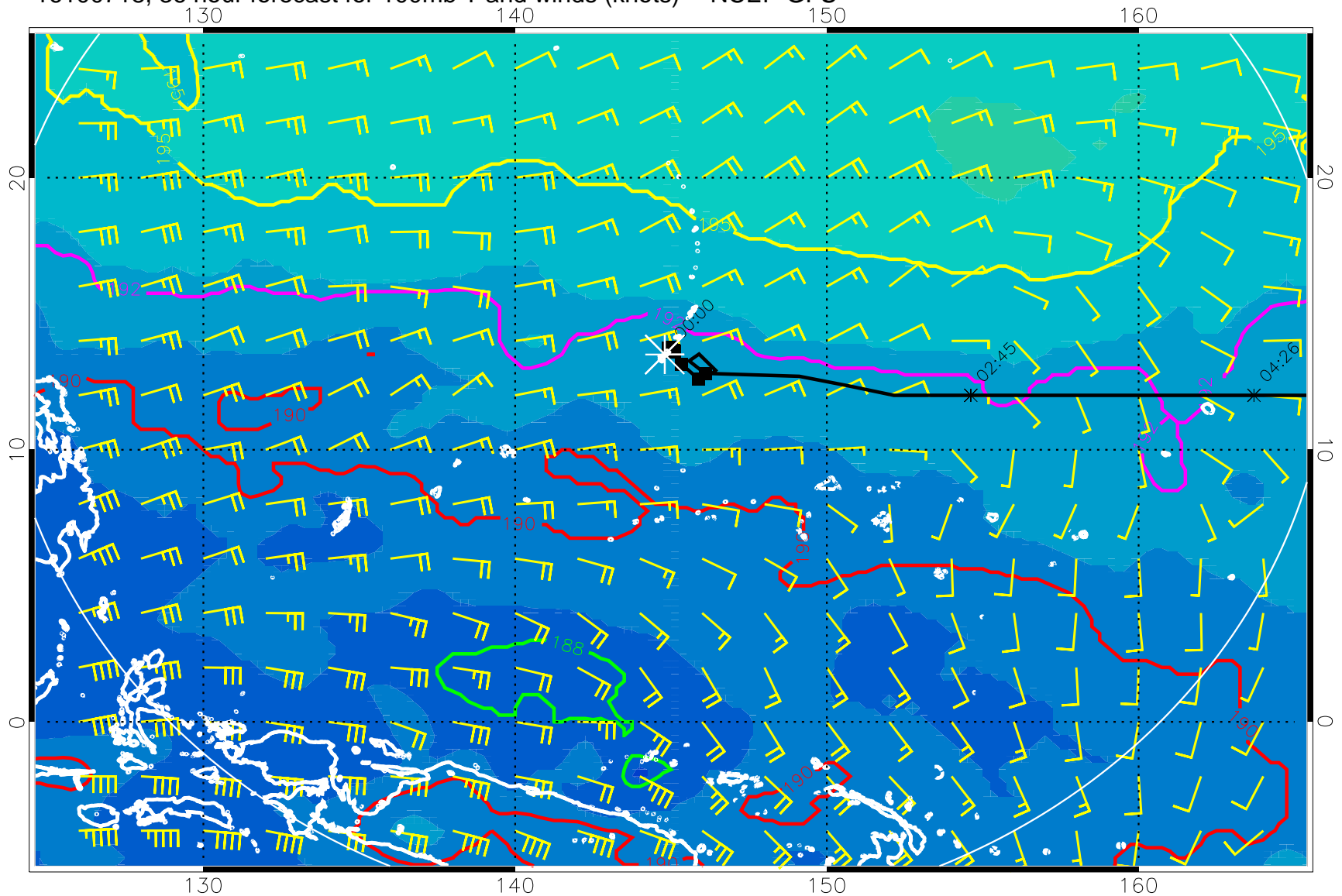
16100718, 36 hour forecast for 100mb T and winds (knots) -- NCEP GFS
