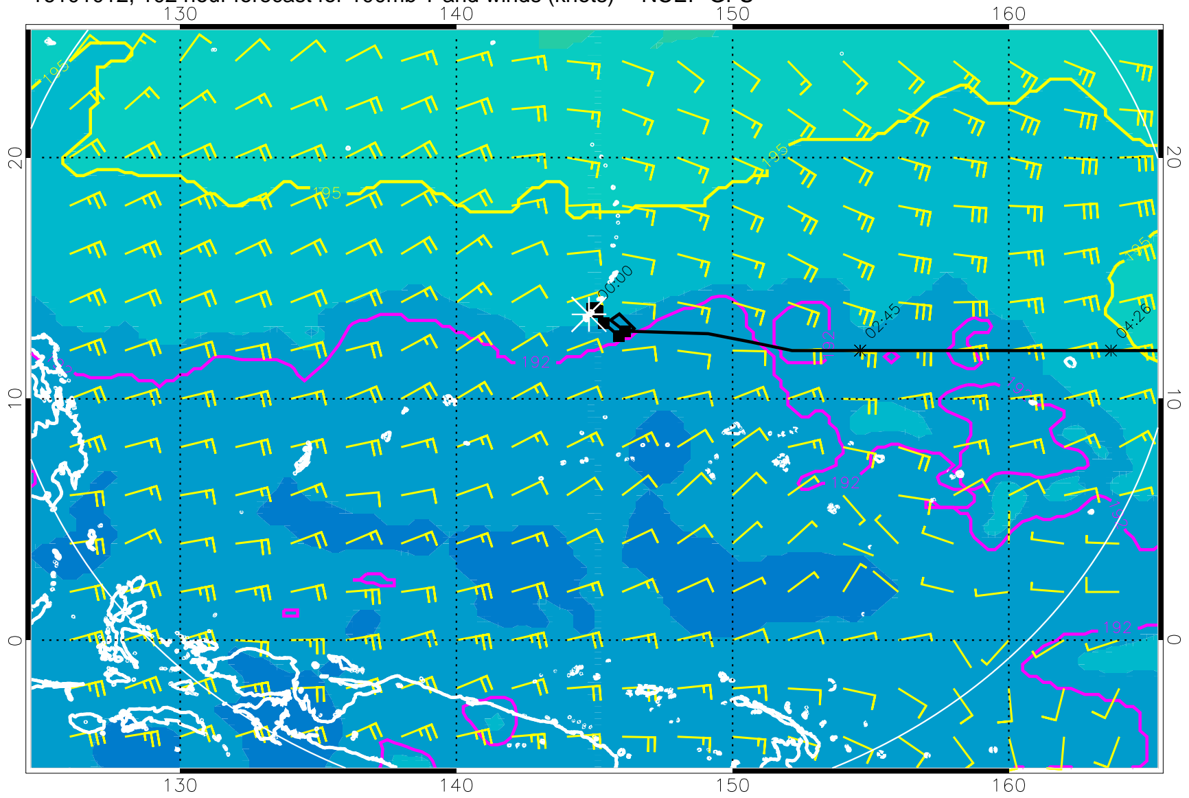
16101012, 102 hour forecast for 100mb T and winds (knots) -- NCEP GFS
