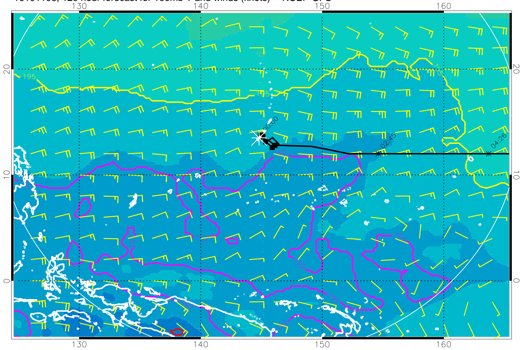
16101106, 120 hour forecast for 100mb T and winds (knots) -- NCEP GFS
