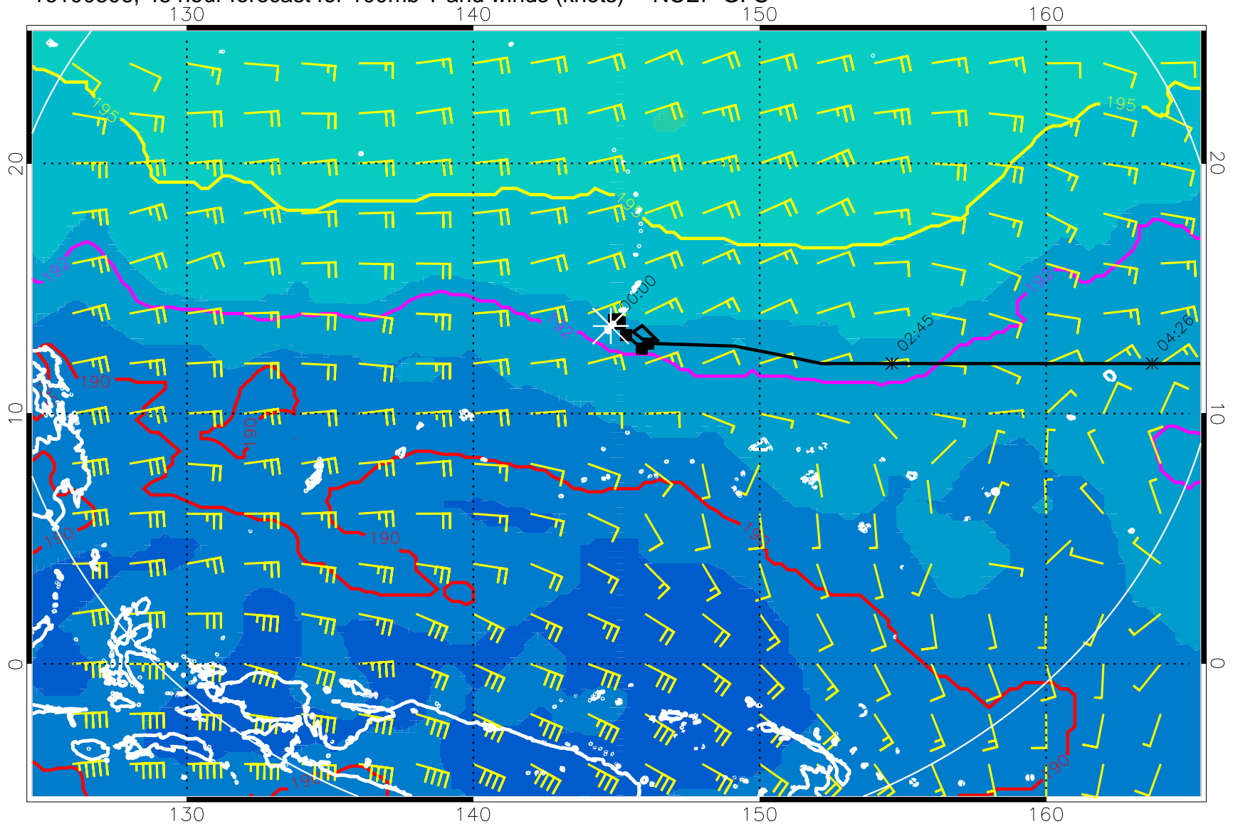
16100806, 48 hour forecast for 100mb T and winds (knots) -- NCEP GFS
