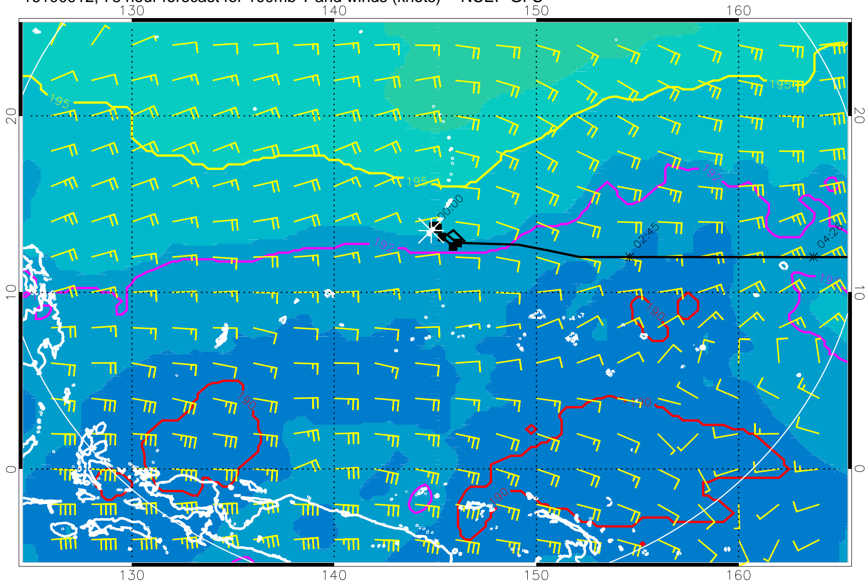
16100912, 78 hour forecast for 100mb T and winds (knots) -- NCEP GFS
