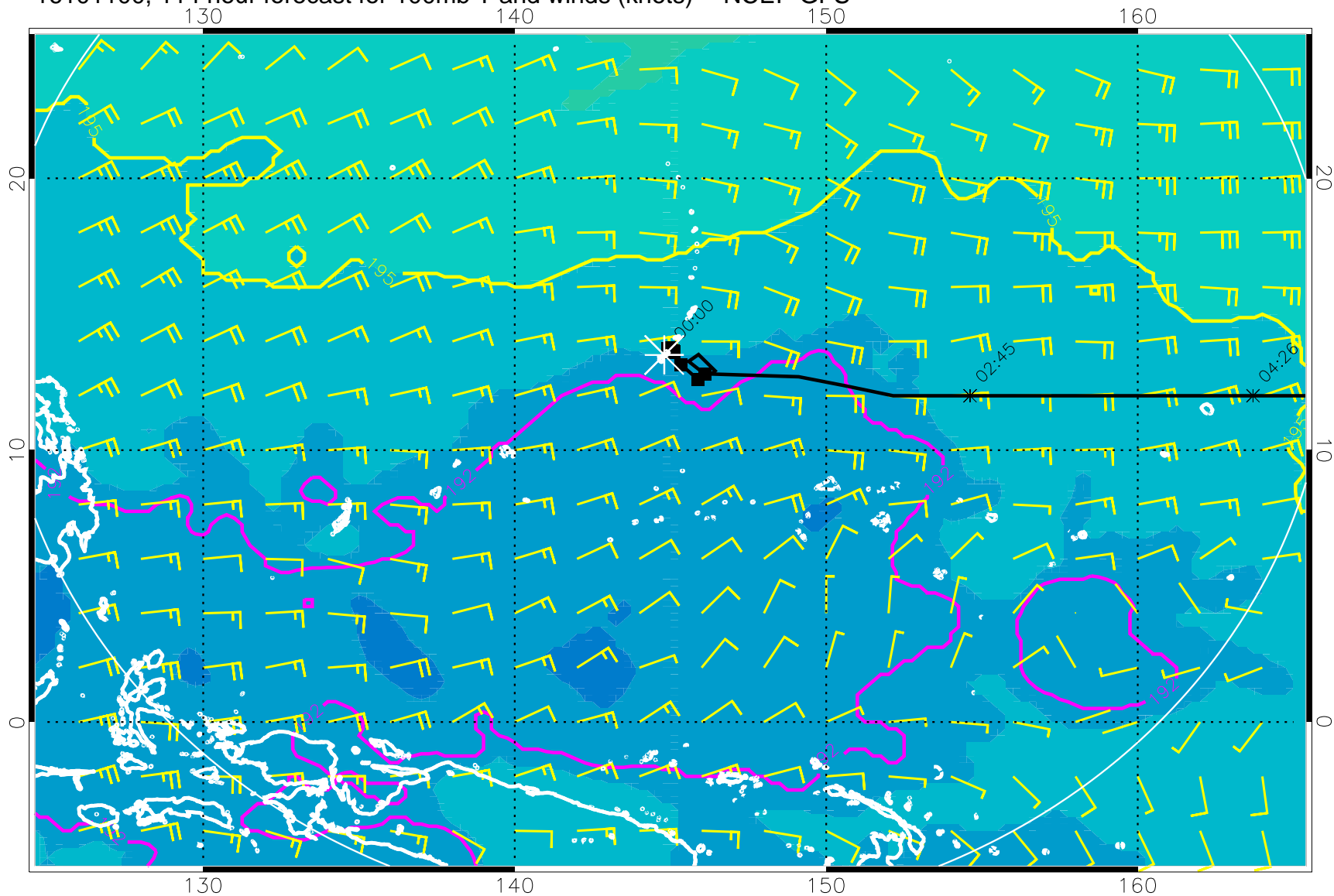
16101100, 114 hour forecast for 100mb T and winds (knots) -- NCEP GFS
