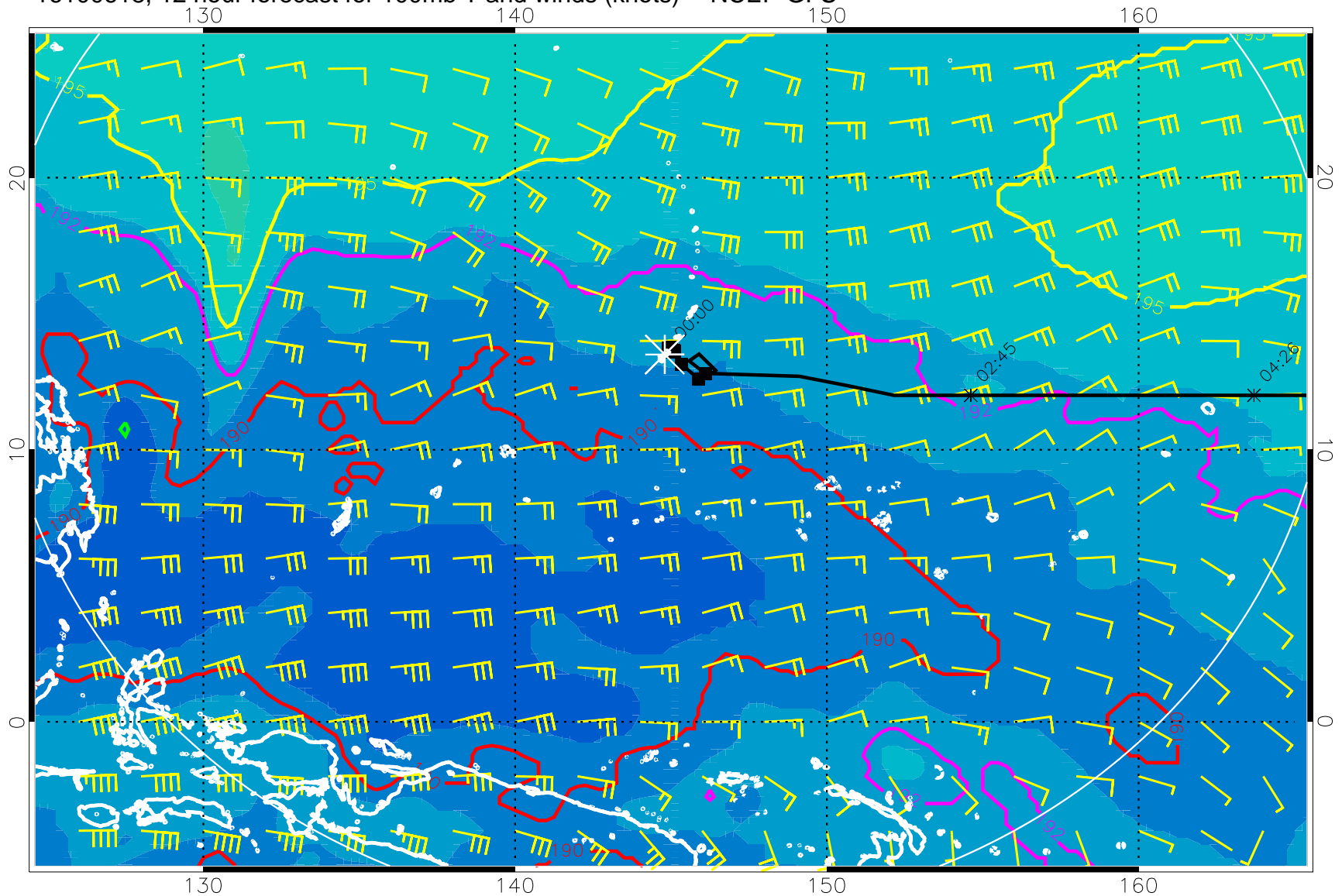
16100618, 12 hour forecast for 100mb T and winds (knots) -- NCEP GFS
