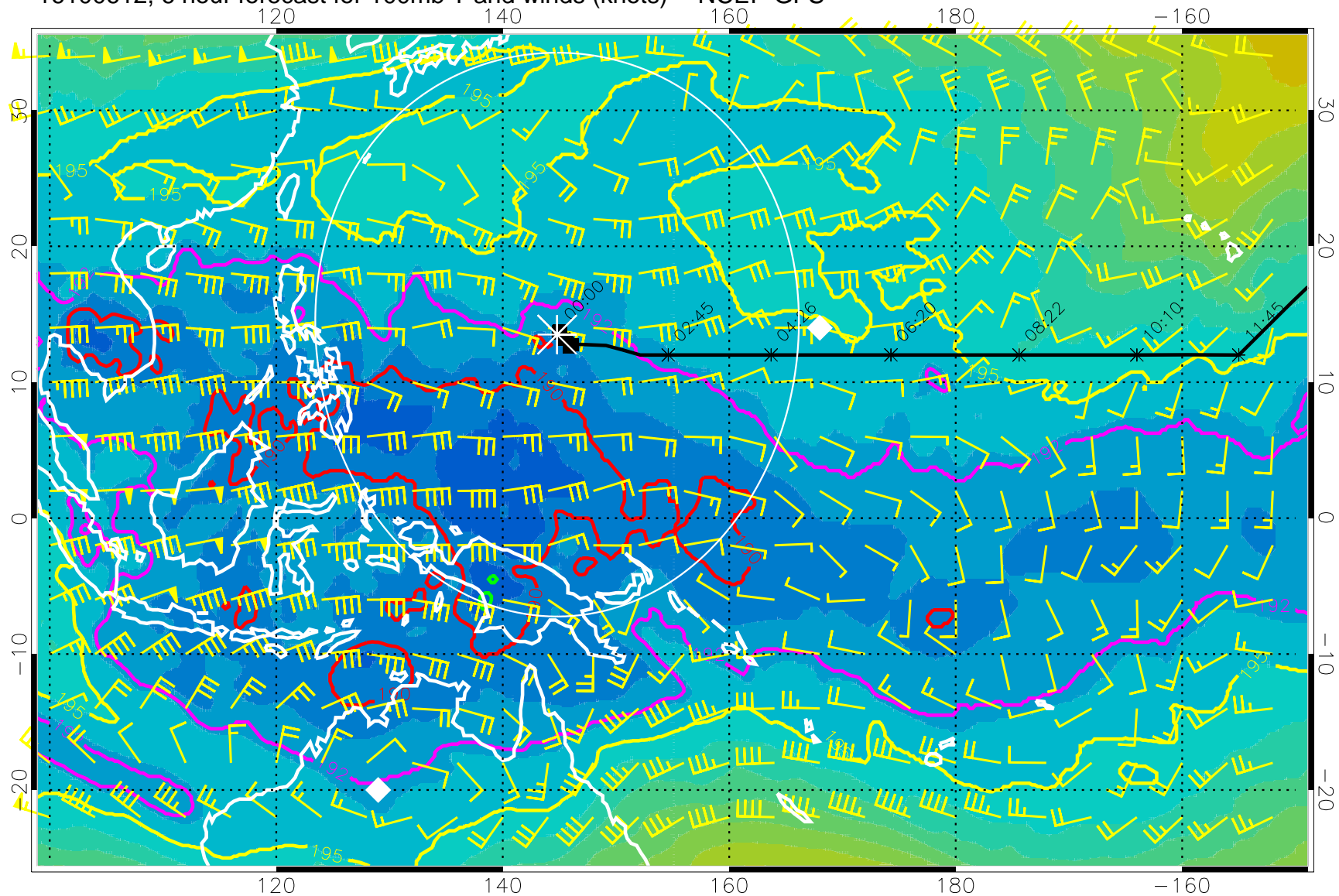
16100612, 6 hour forecast for 100mb T and winds (knots) -- NCEP GFS
