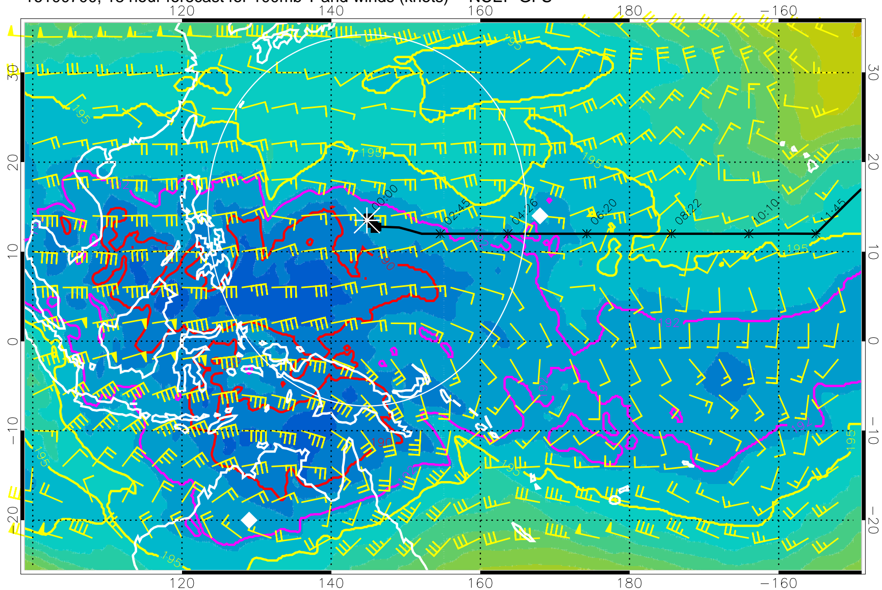
16100700, 18 hour forecast for 100mb T and winds (knots) -- NCEP GFS
