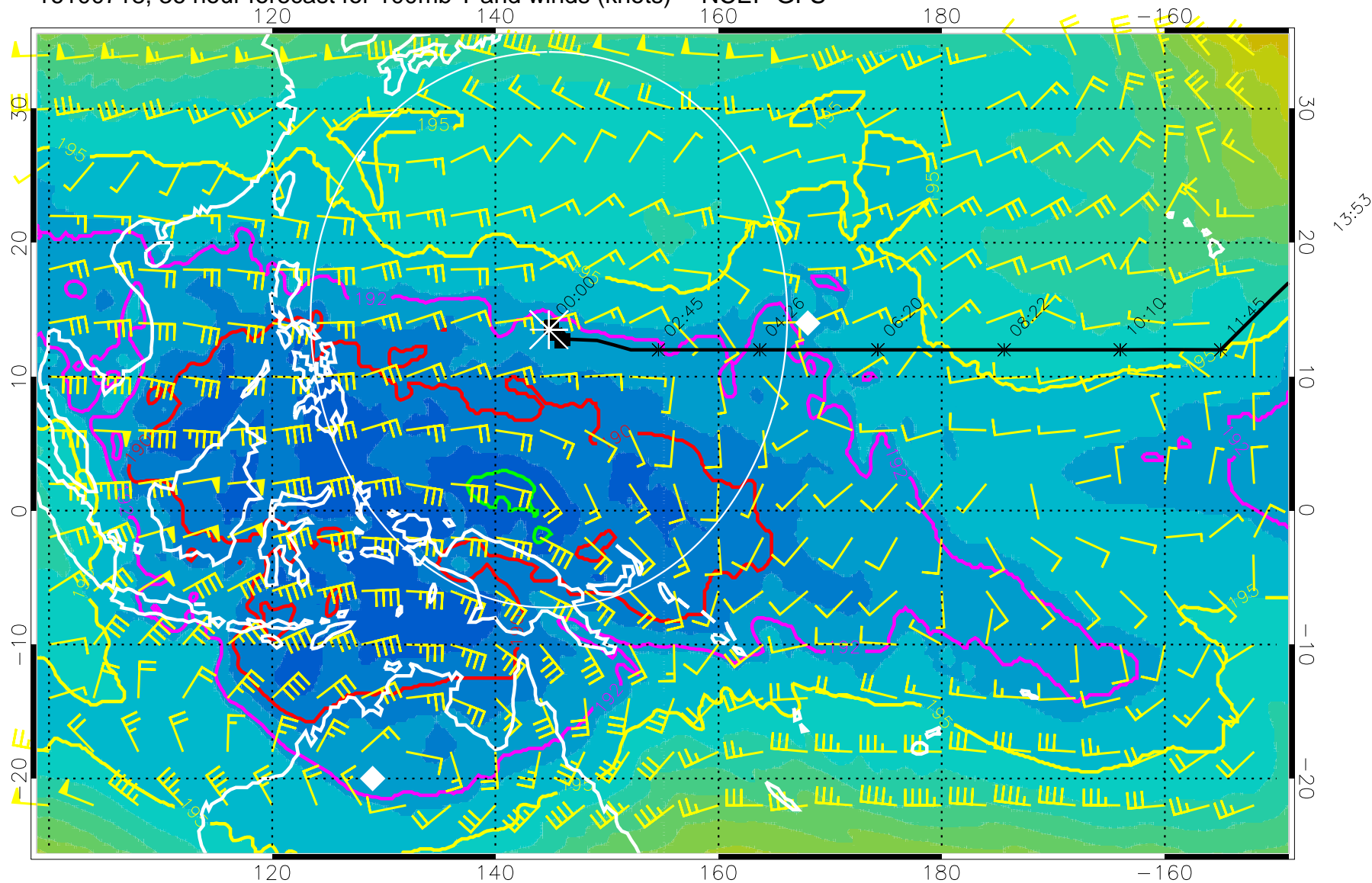
16100718, 36 hour forecast for 100mb T and winds (knots) -- NCEP GFS
