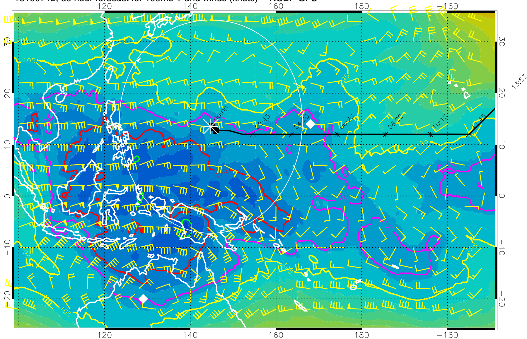
16100712, 30 hour forecast for 100mb T and winds (knots) -- NCEP GFS
