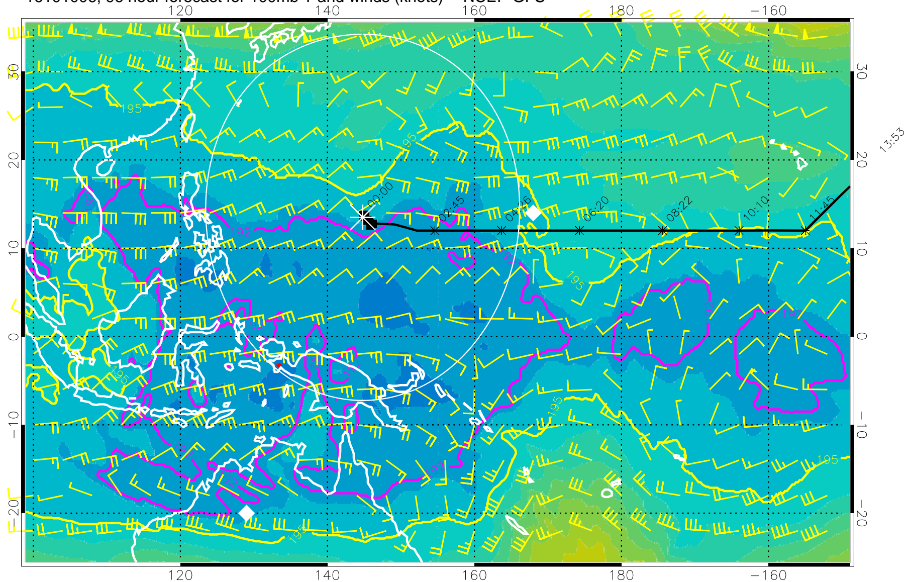
16101006, 96 hour forecast for 100mb T and winds (knots) -- NCEP GFS
