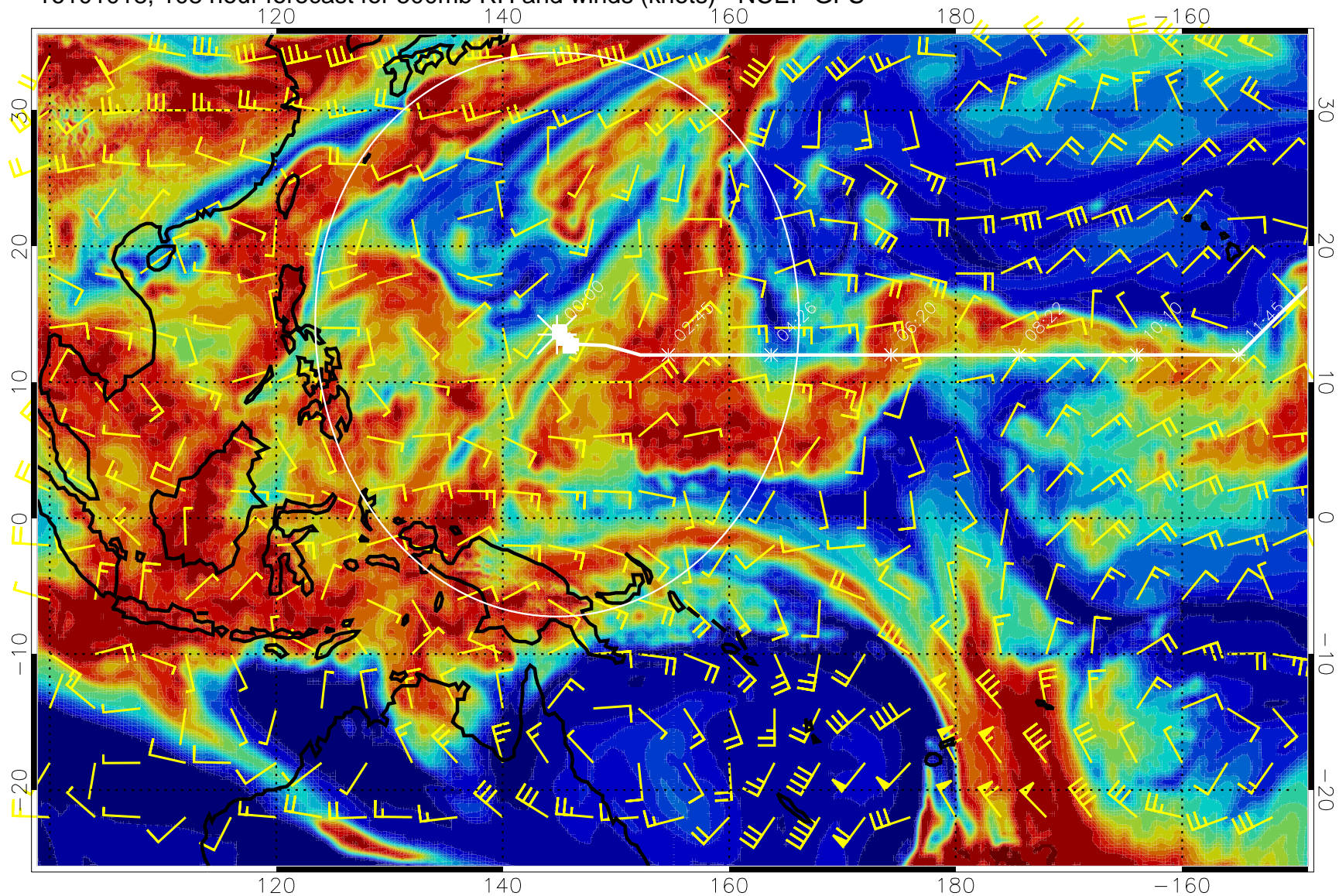
16101018, 108 hour forecast for 500mb RH and winds (knots) - NCEP GFS
