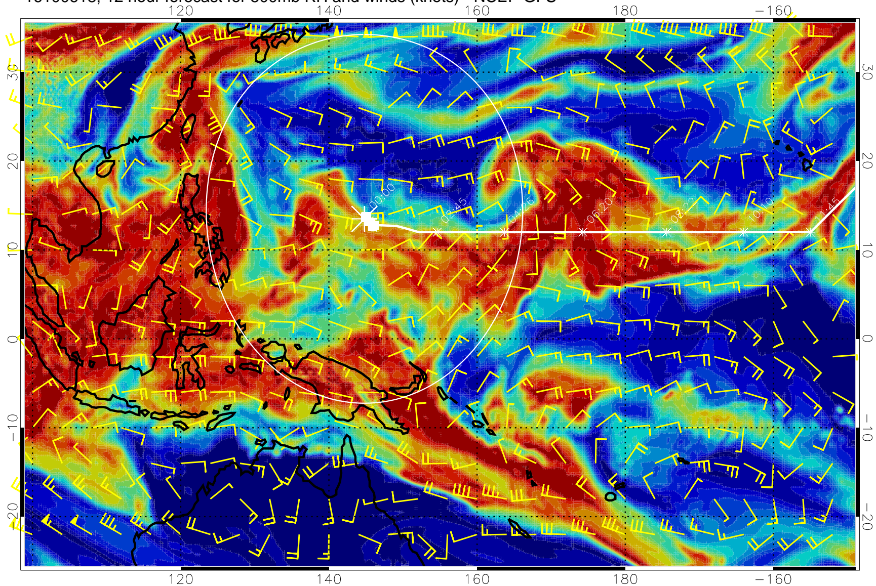
16100618, 12 hour forecast for 500mb RH and winds (knots) - NCEP GFS
