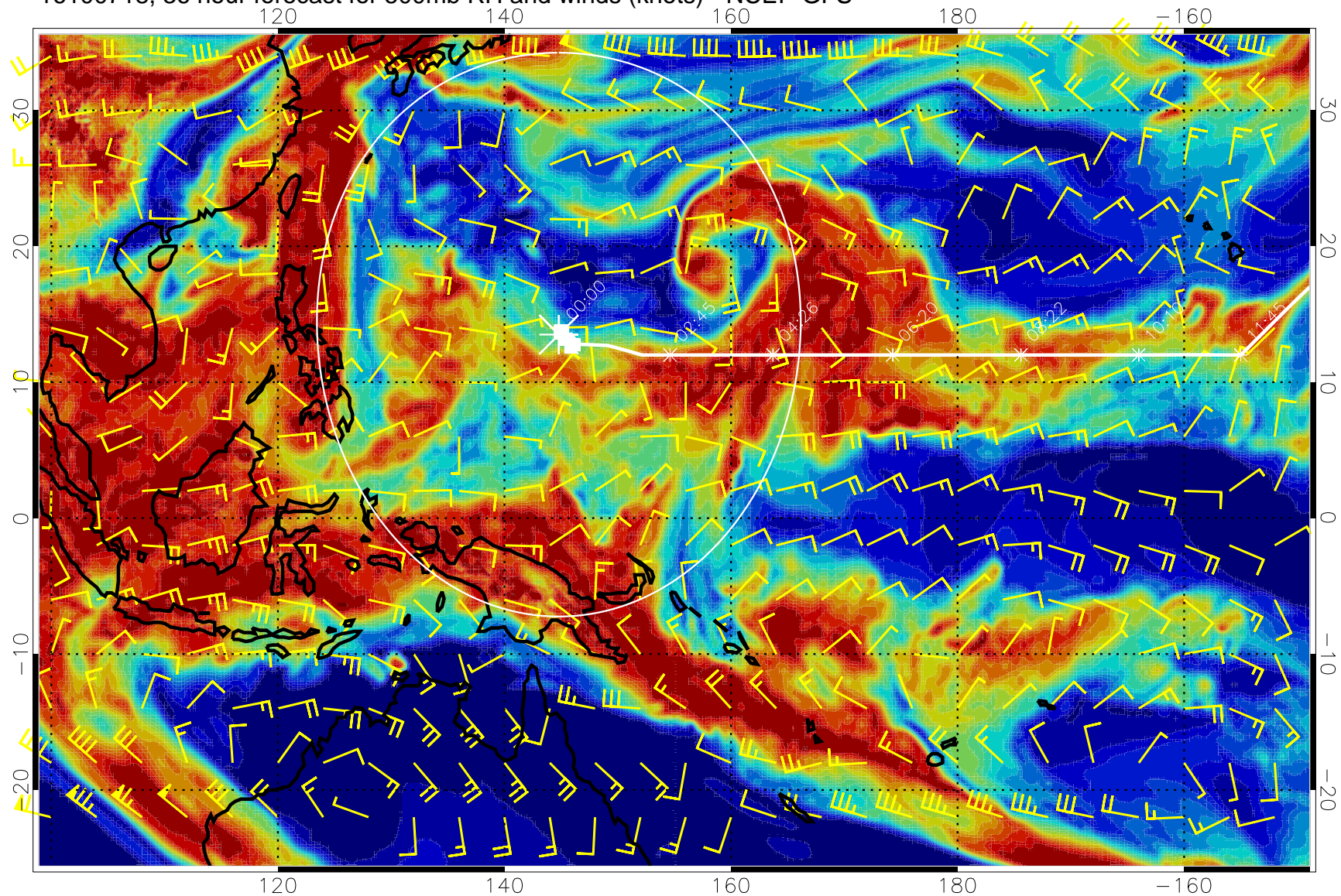
16100718, 36 hour forecast for 500mb RH and winds (knots) - NCEP GFS
