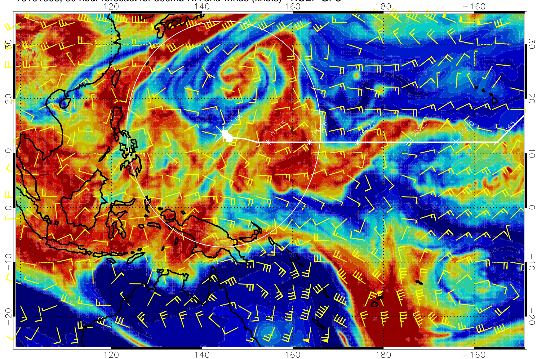
16101000, 90 hour forecast for 500mb RH and winds (knots) - NCEP GFS
