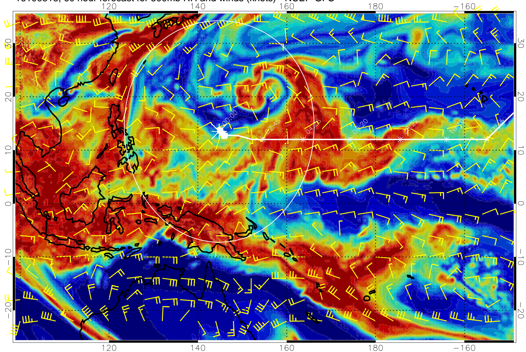
16100818, 60 hour forecast for 500mb RH and winds (knots) - NCEP GFS
