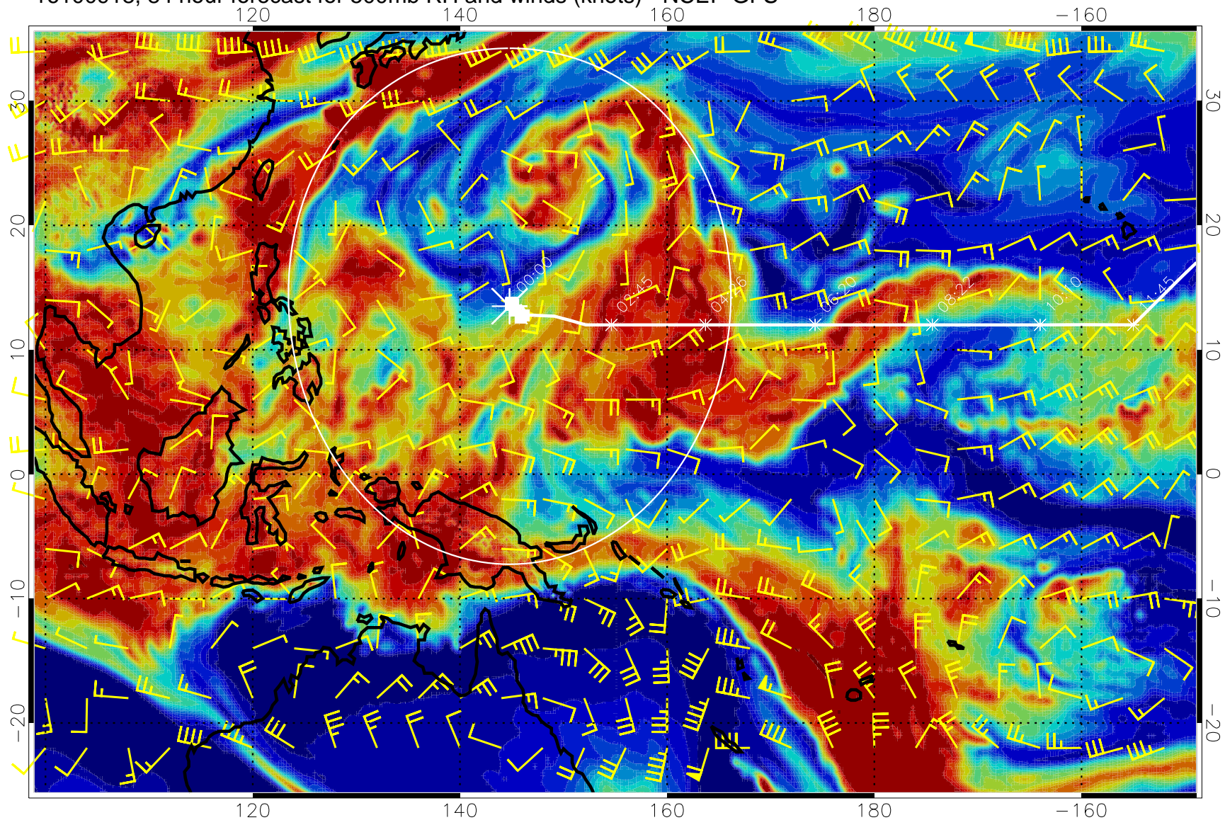
16100918, 84 hour forecast for 500mb RH and winds (knots) - NCEP GFS
