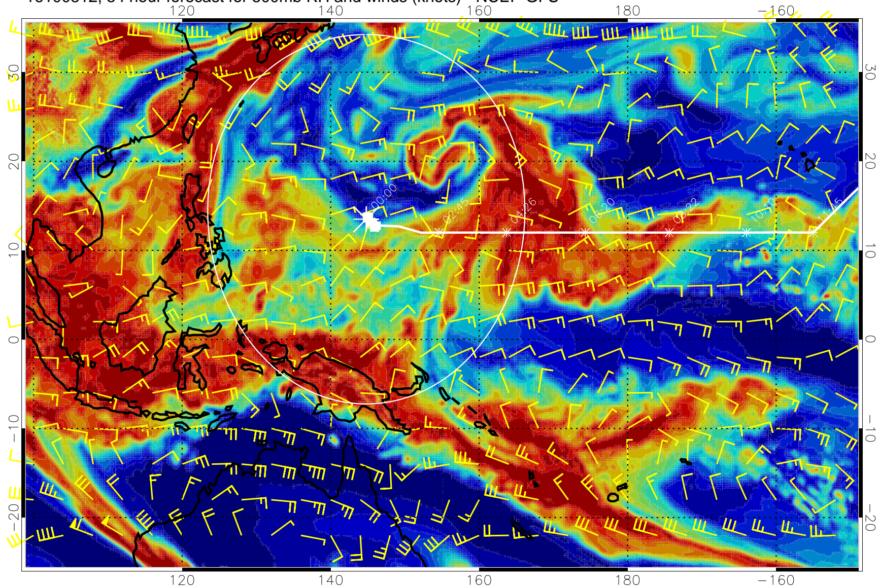
16100812, 54 hour forecast for 500mb RH and winds (knots) - NCEP GFS
