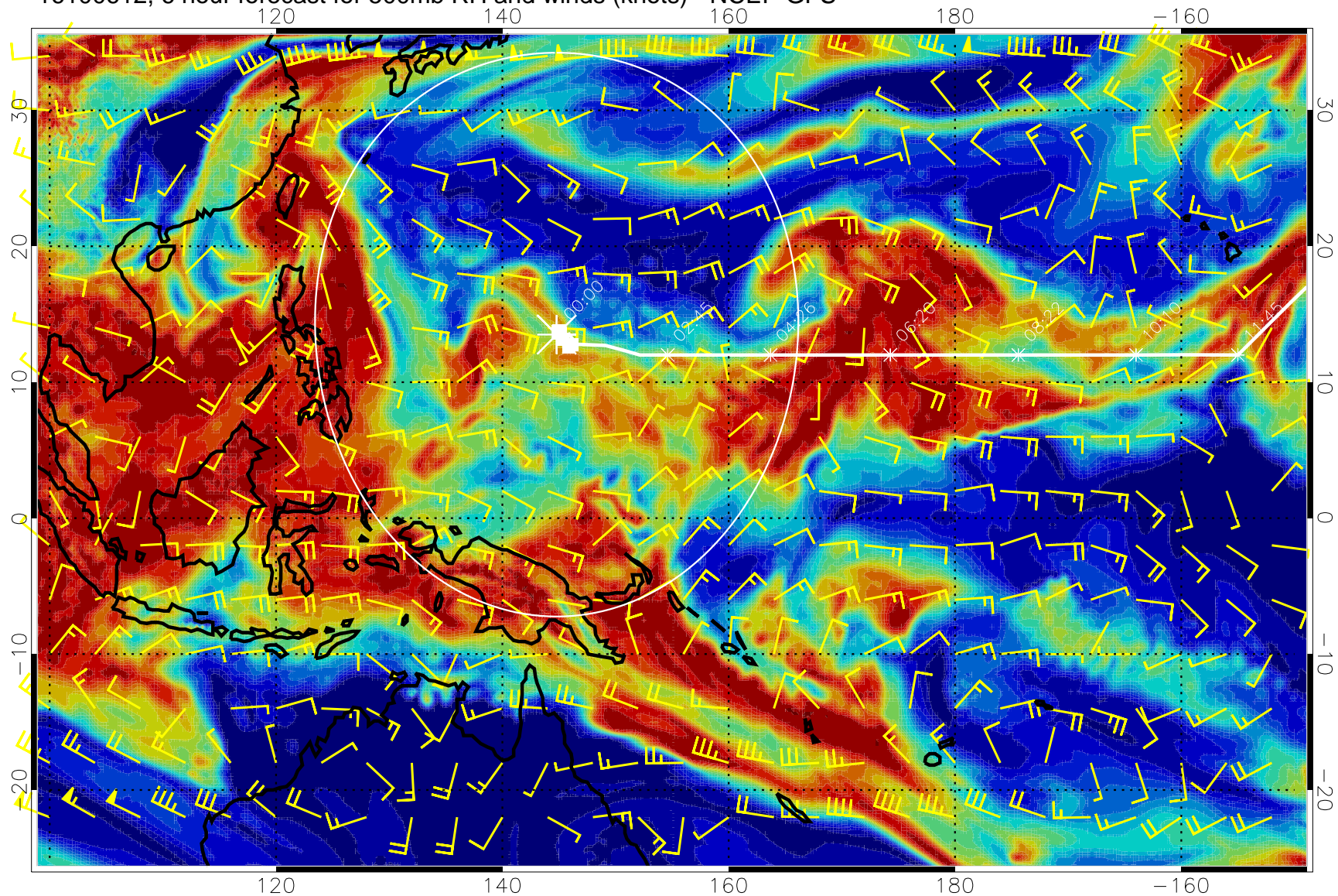
16100612, 6 hour forecast for 500mb RH and winds (knots) - NCEP GFS
