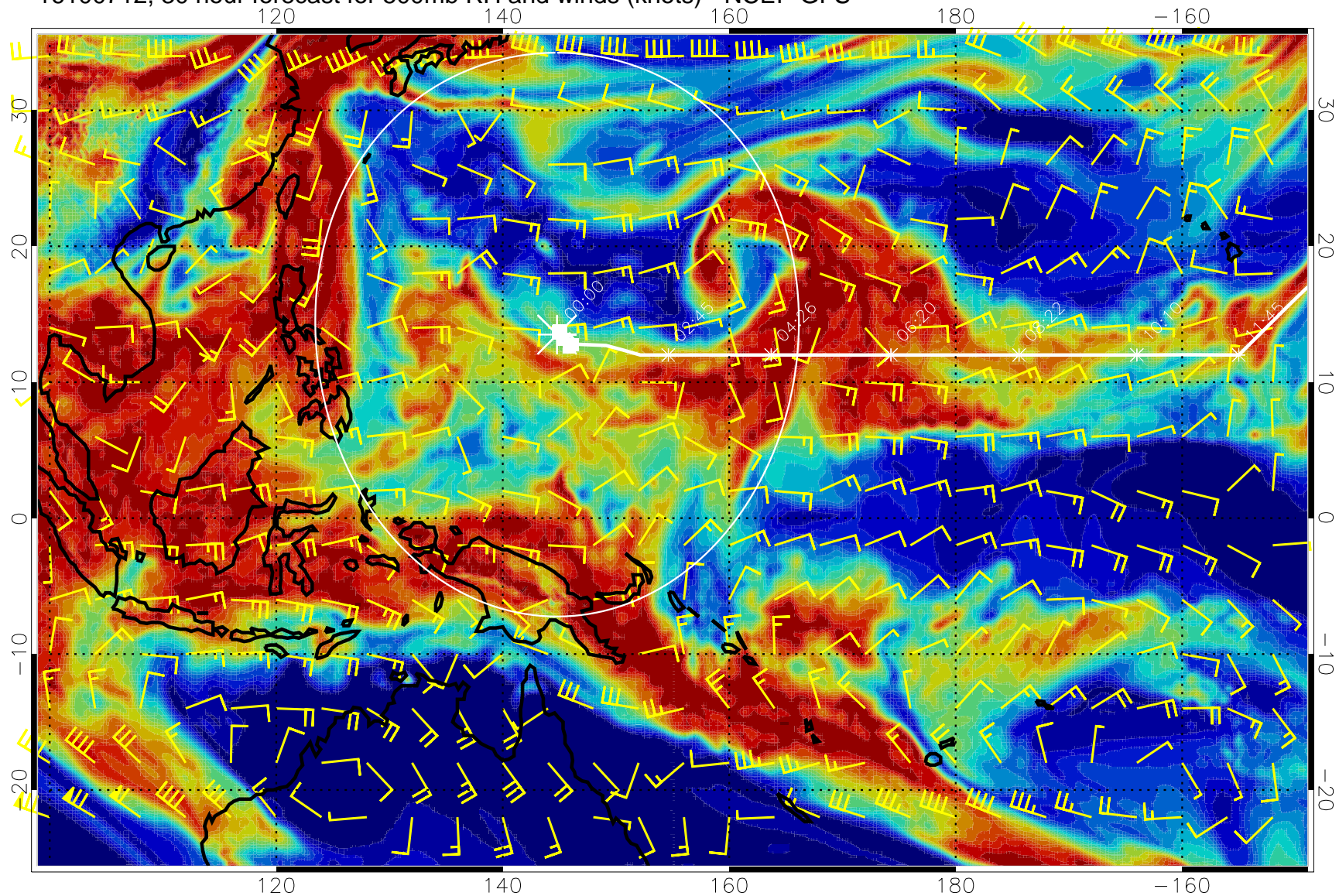
16100712, 30 hour forecast for 500mb RH and winds (knots) - NCEP GFS
