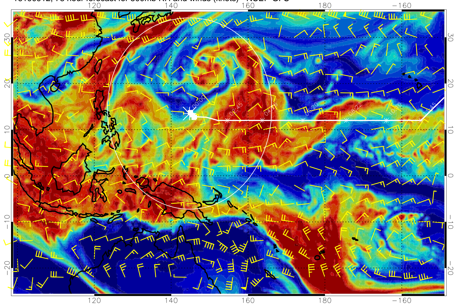
16100912, 78 hour forecast for 500mb RH and winds (knots) - NCEP GFS
