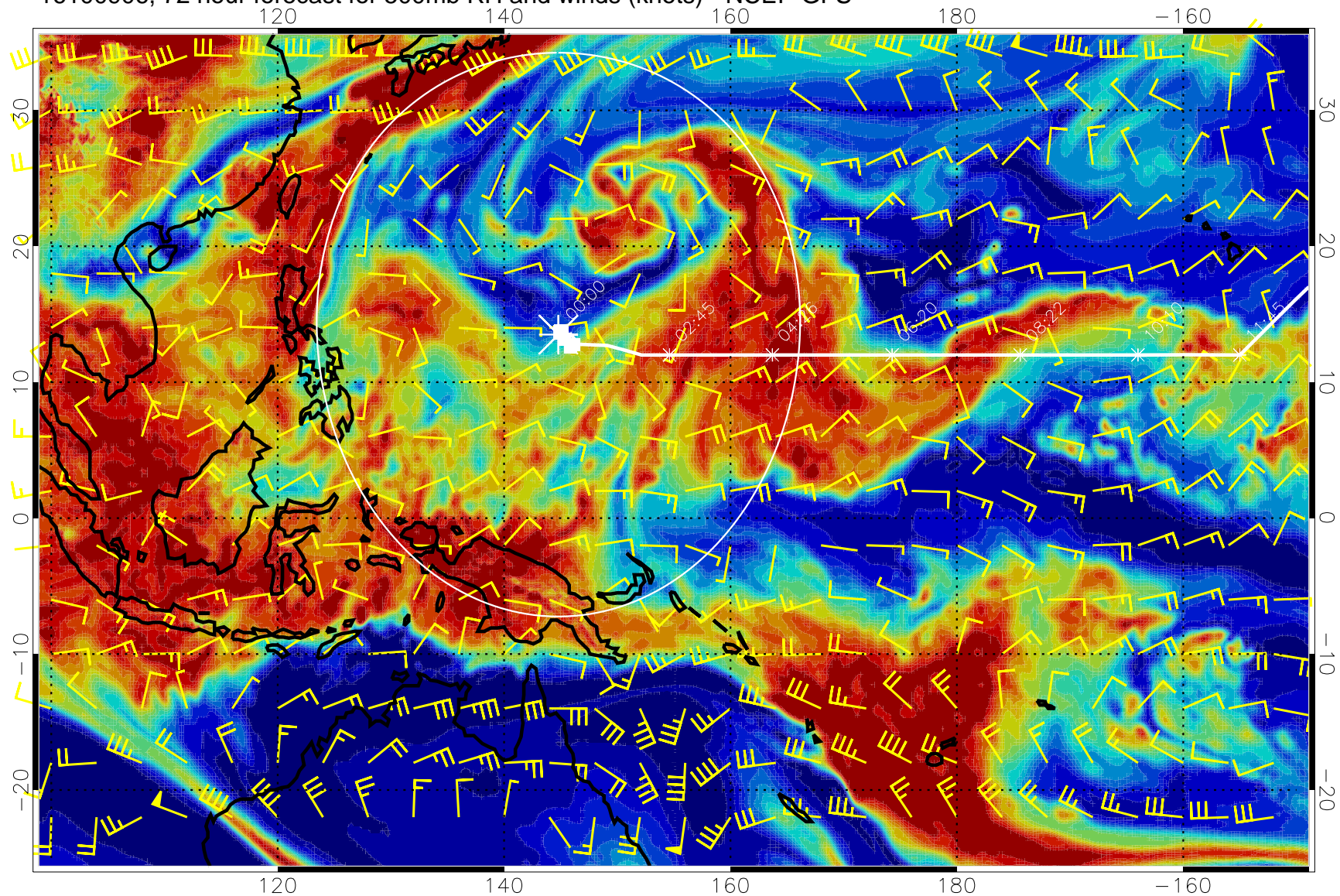
16100906, 72 hour forecast for 500mb RH and winds (knots) - NCEP GFS
