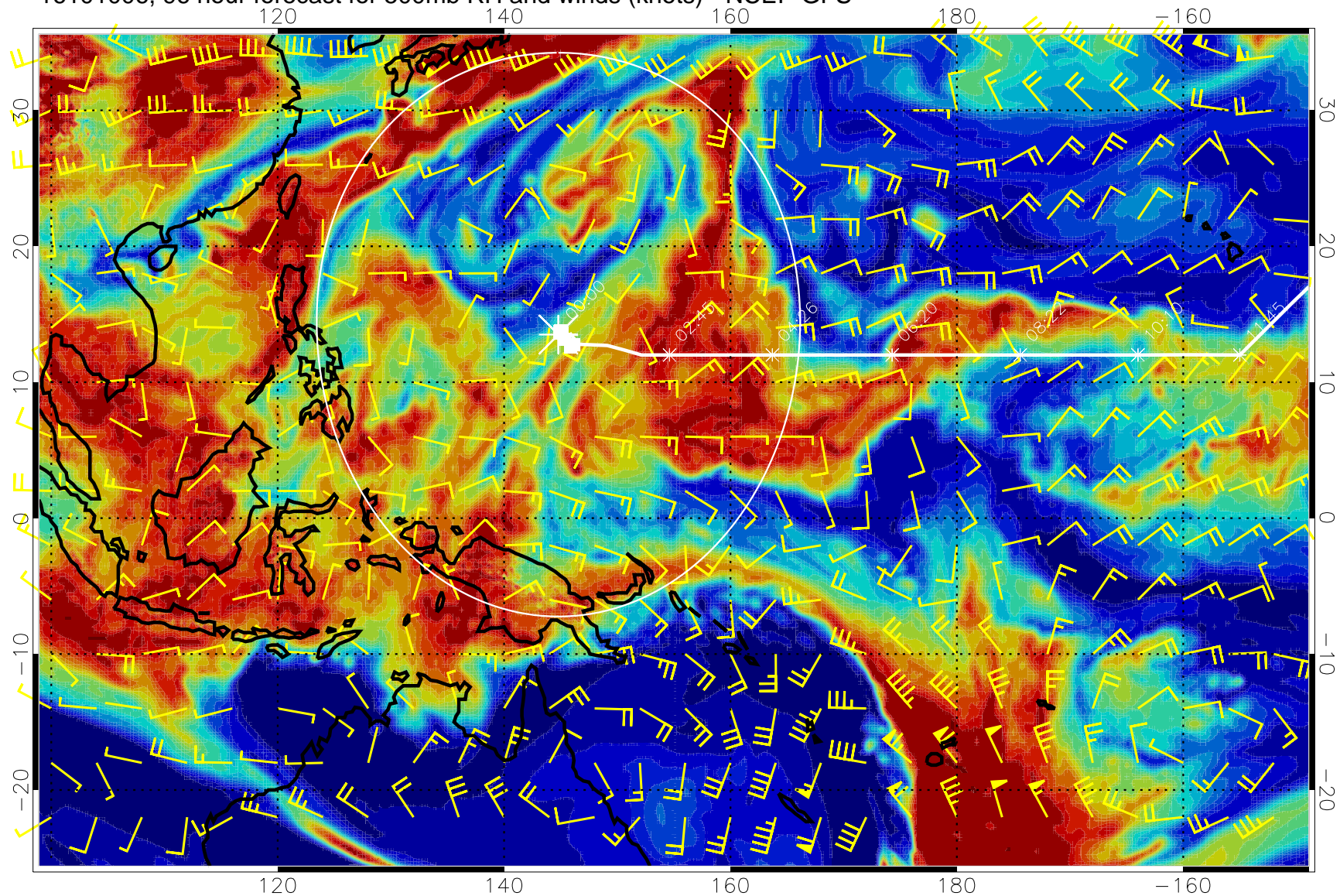
16101006, 96 hour forecast for 500mb RH and winds (knots) - NCEP GFS
