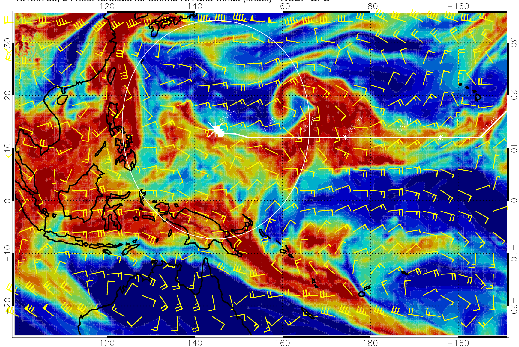
16100706, 24 hour forecast for 500mb RH and winds (knots) - NCEP GFS
