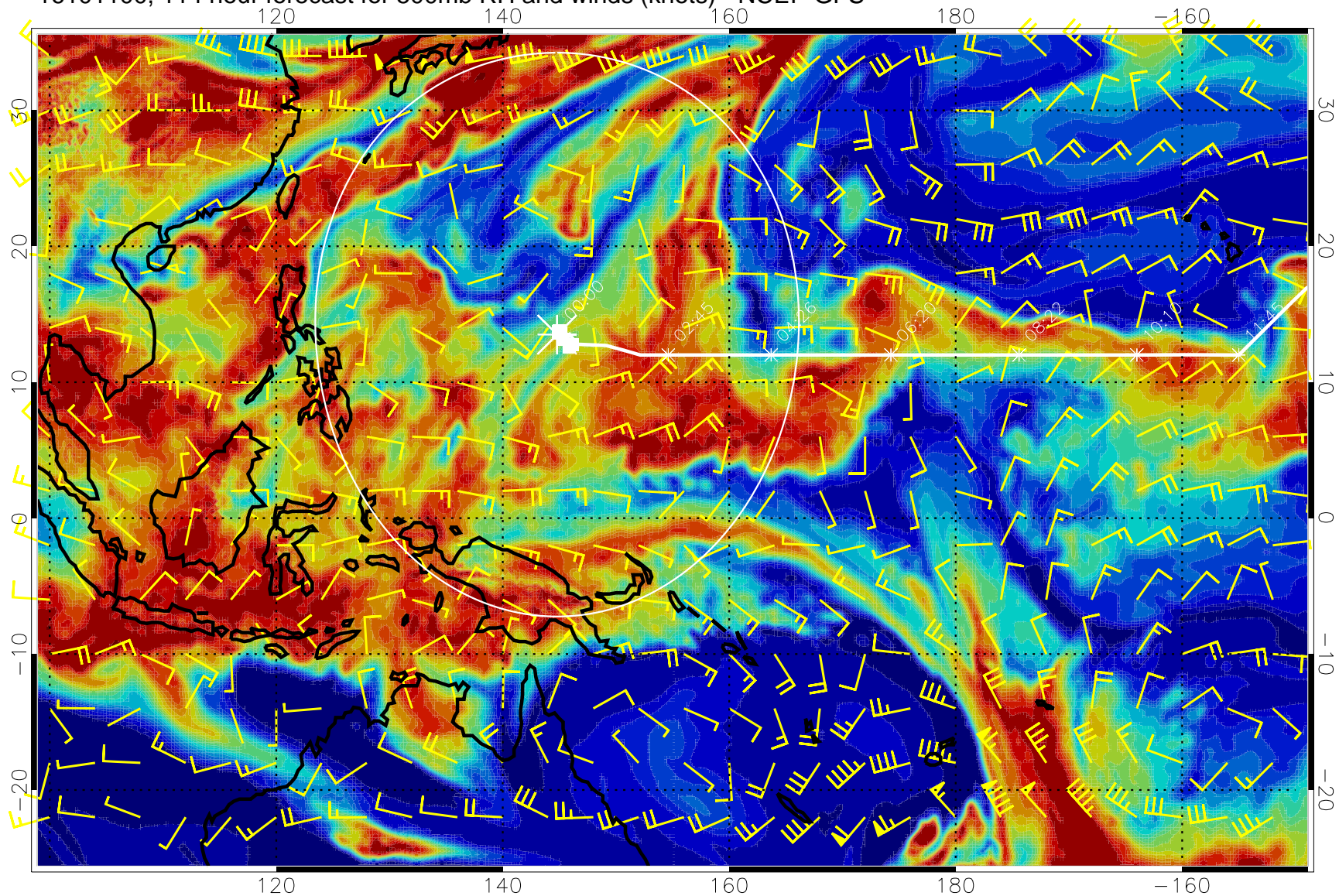
16101100, 114 hour forecast for 500mb RH and winds (knots) - NCEP GFS
