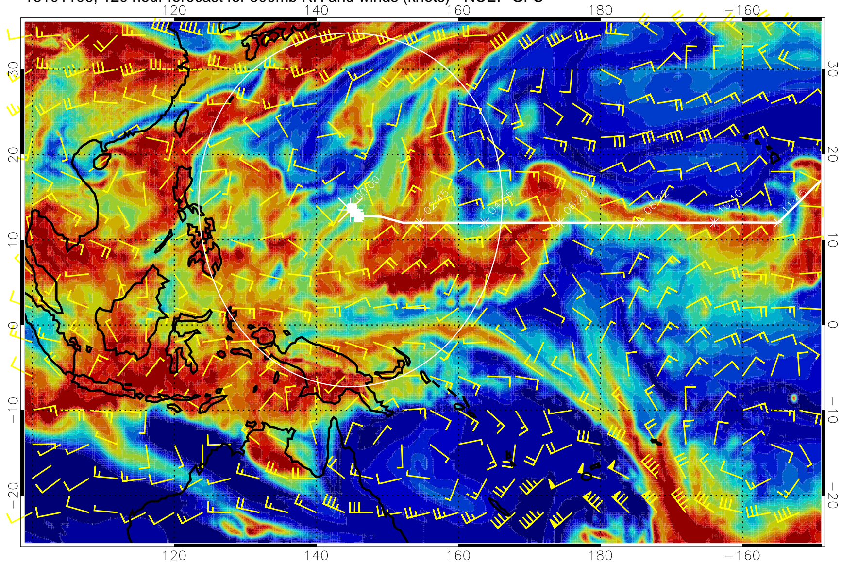
16101106, 120 hour forecast for 500mb RH and winds (knots) - NCEP GFS
