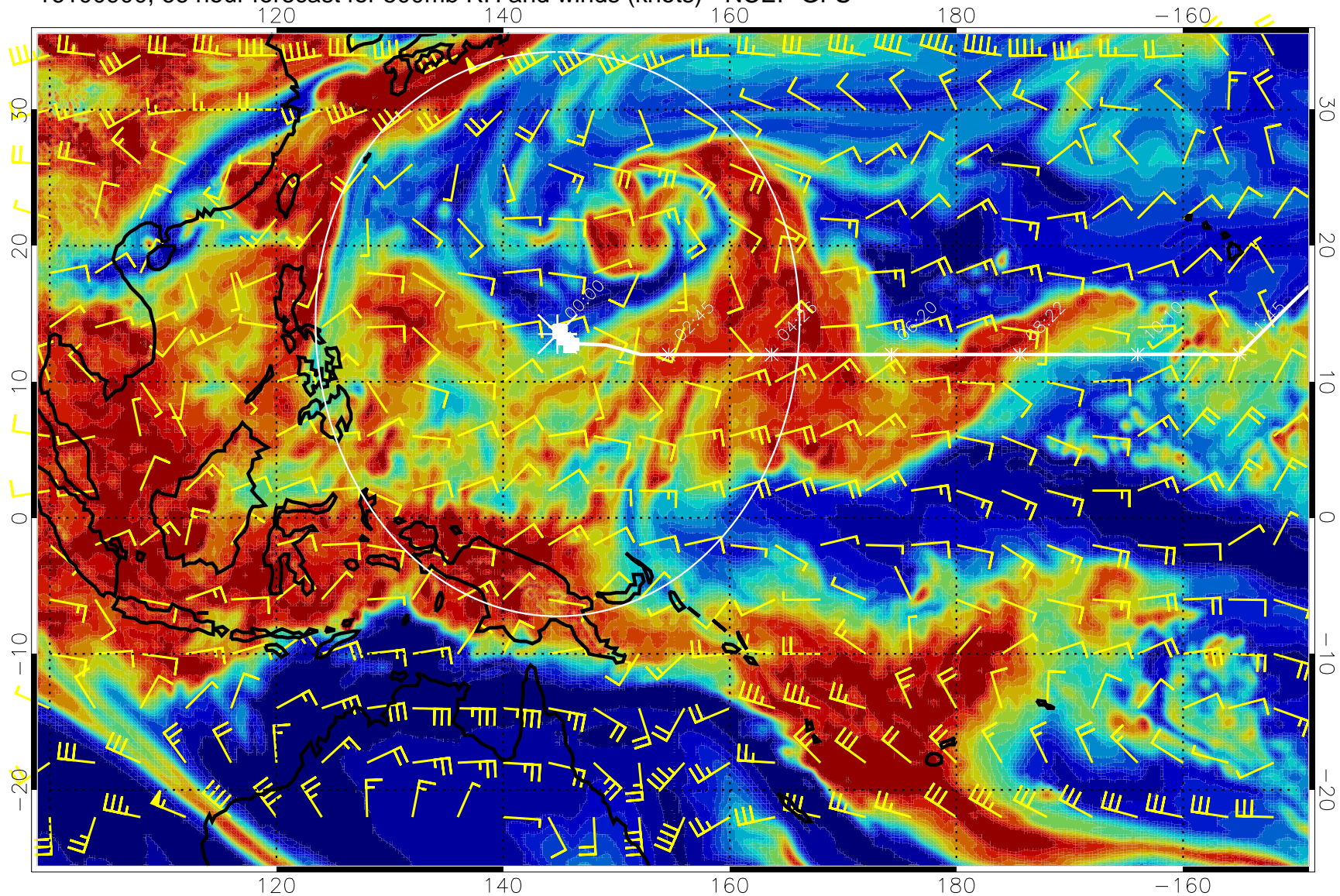
16100900, 66 hour forecast for 500mb RH and winds (knots) - NCEP GFS
