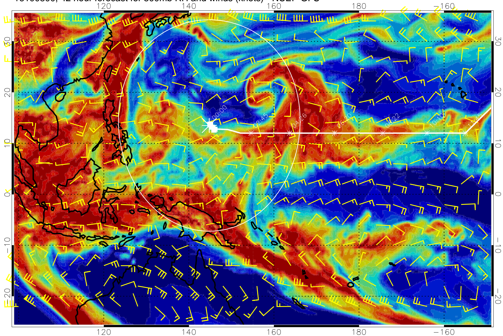
16100800, 42 hour forecast for 500mb RH and winds (knots) - NCEP GFS
