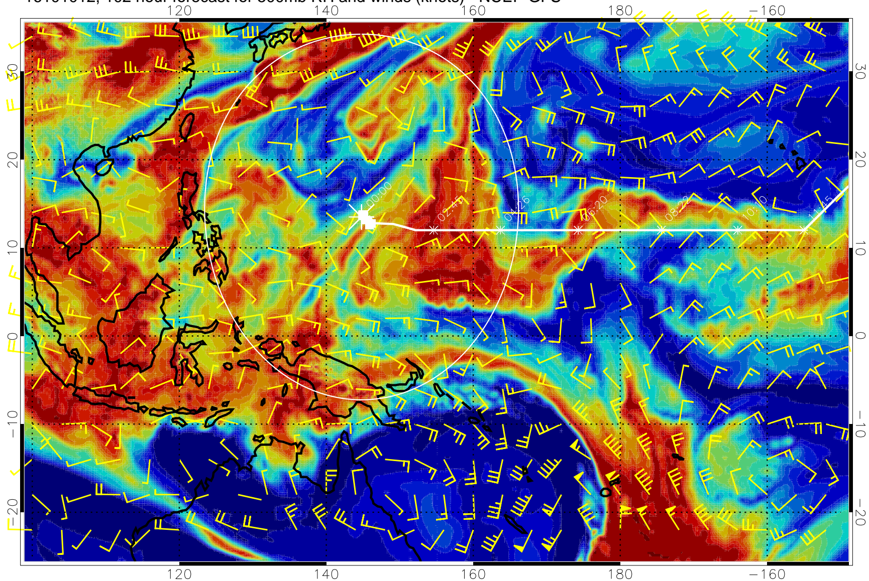
16101012, 102 hour forecast for 500mb RH and winds (knots) - NCEP GFS
