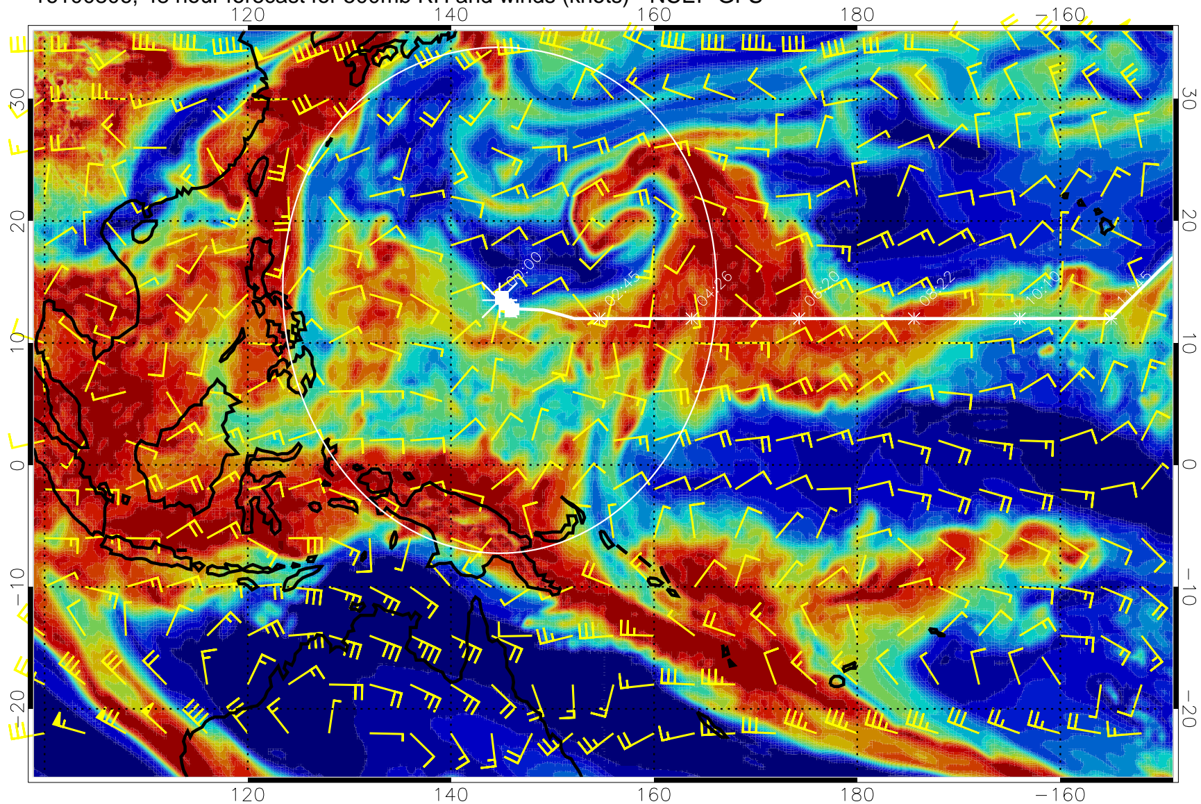
16100806, 48 hour forecast for 500mb RH and winds (knots) - NCEP GFS
