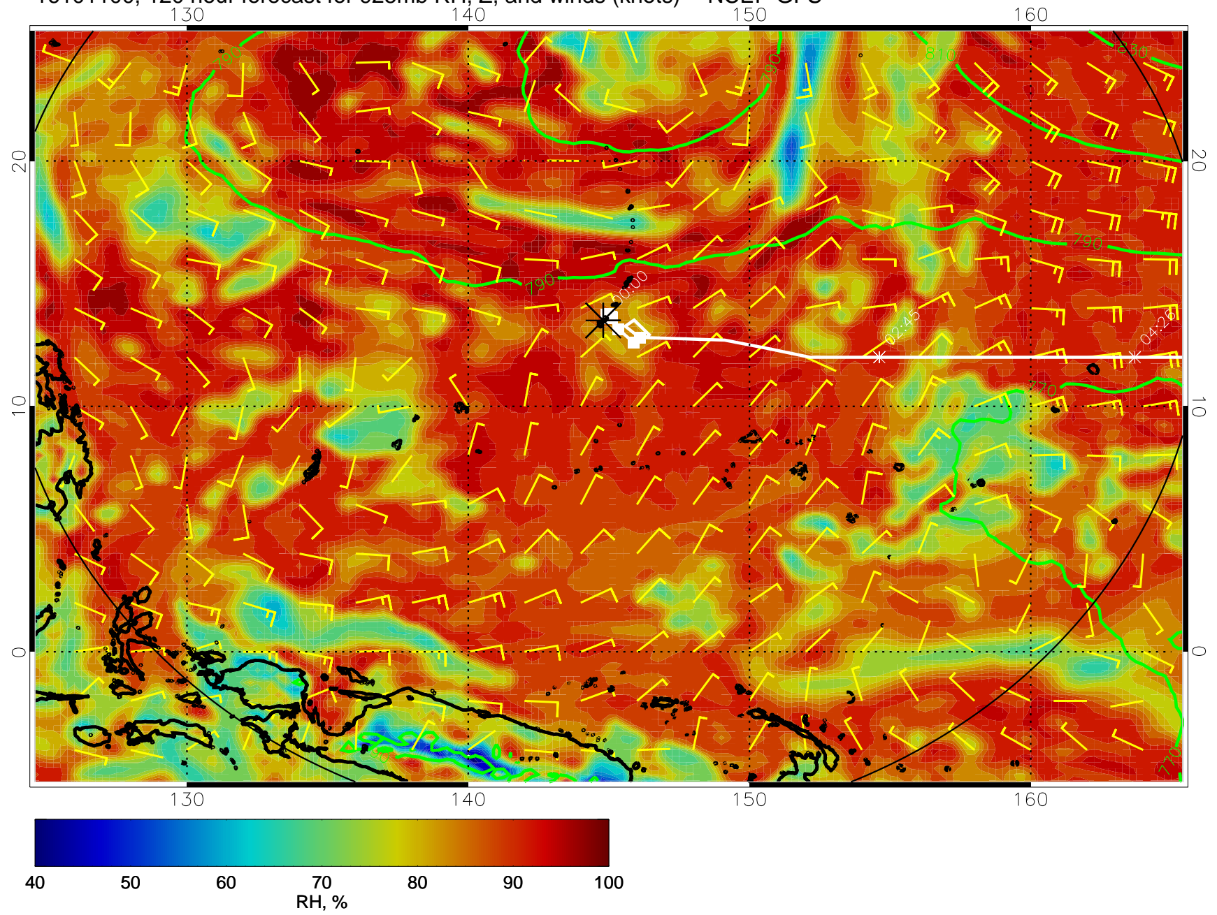
16101100, 120 hour forecast for 925mb RH, Z, and winds (knots) -- NCEP GFS
