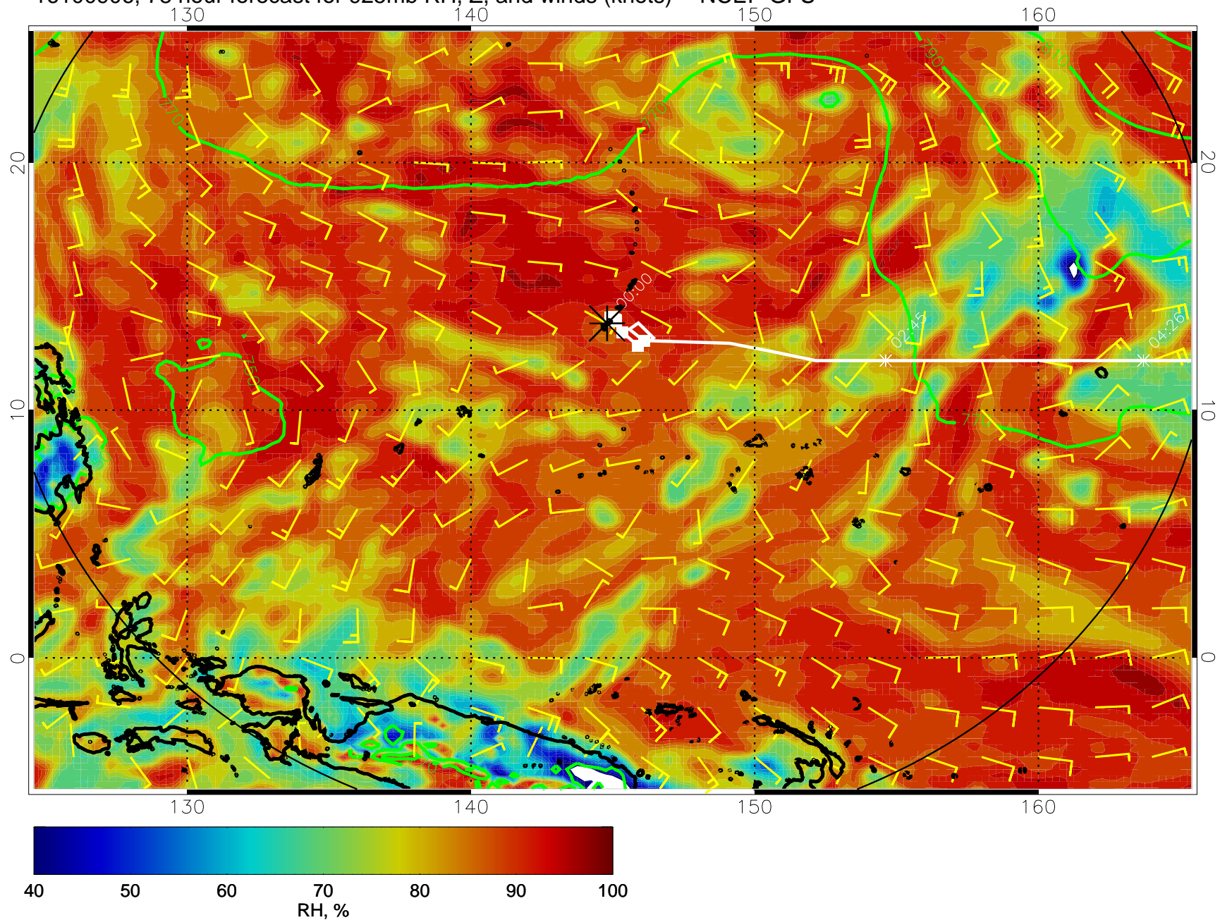
16100906, 78 hour forecast for 925mb RH, Z, and winds (knots) -- NCEP GFS
