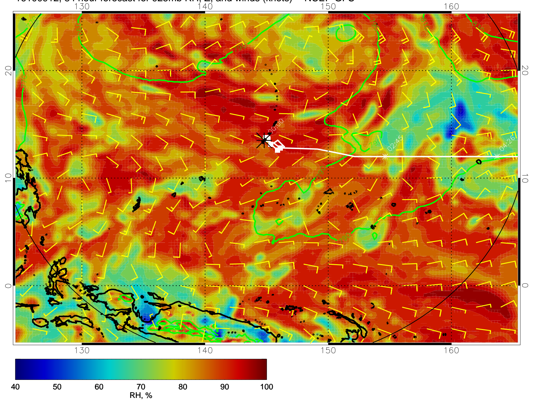
16100912, 84 hour forecast for 925mb RH, Z, and winds (knots) -- NCEP GFS
