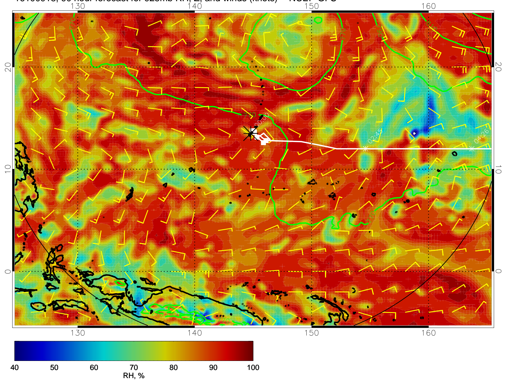
16100918, 90 hour forecast for 925mb RH, Z, and winds (knots) -- NCEP GFS
