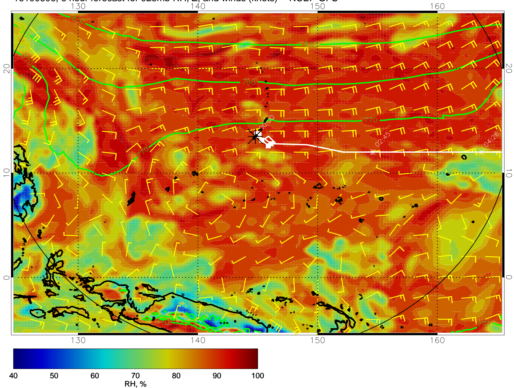
16100606, 6 hour forecast for 925mb RH, Z, and winds (knots) -- NCEP GFS
