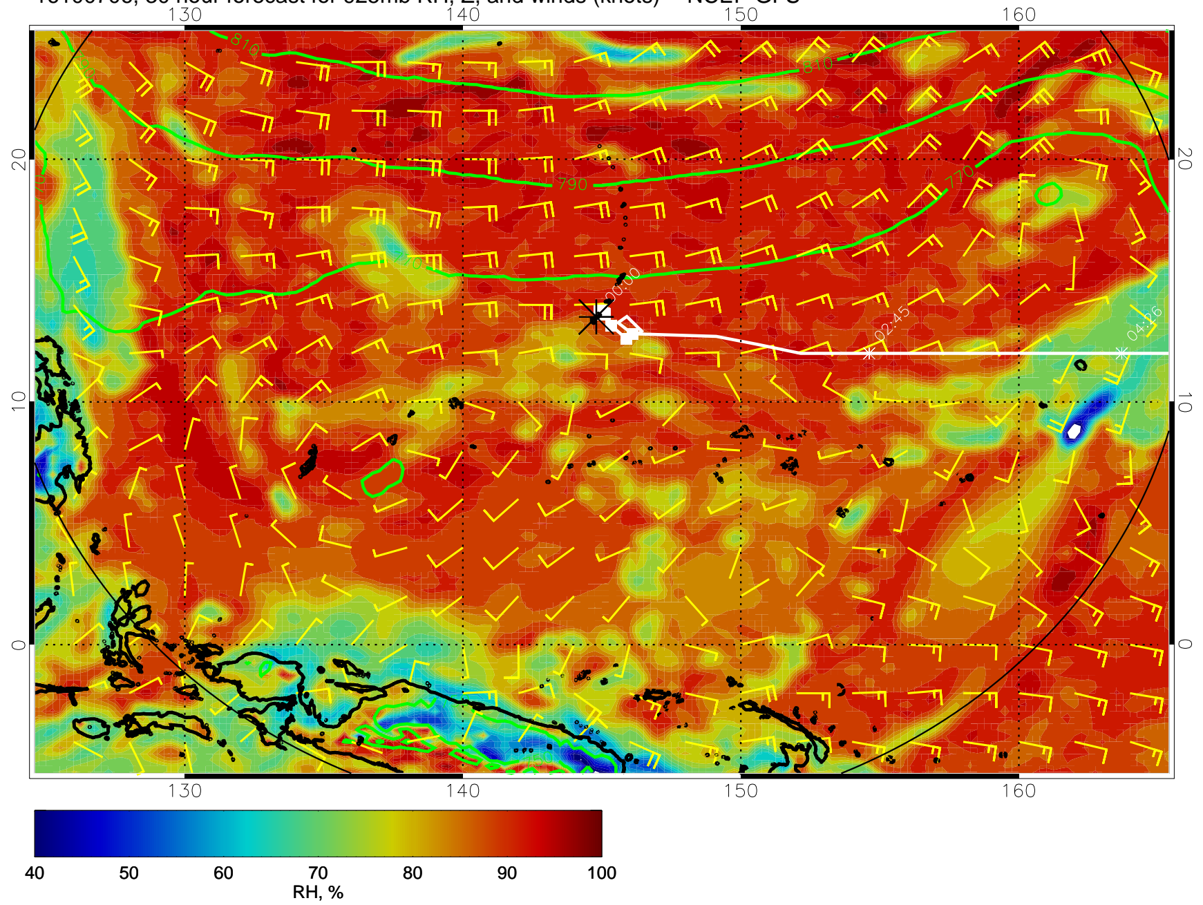
16100706, 30 hour forecast for 925mb RH, Z, and winds (knots) -- NCEP GFS
