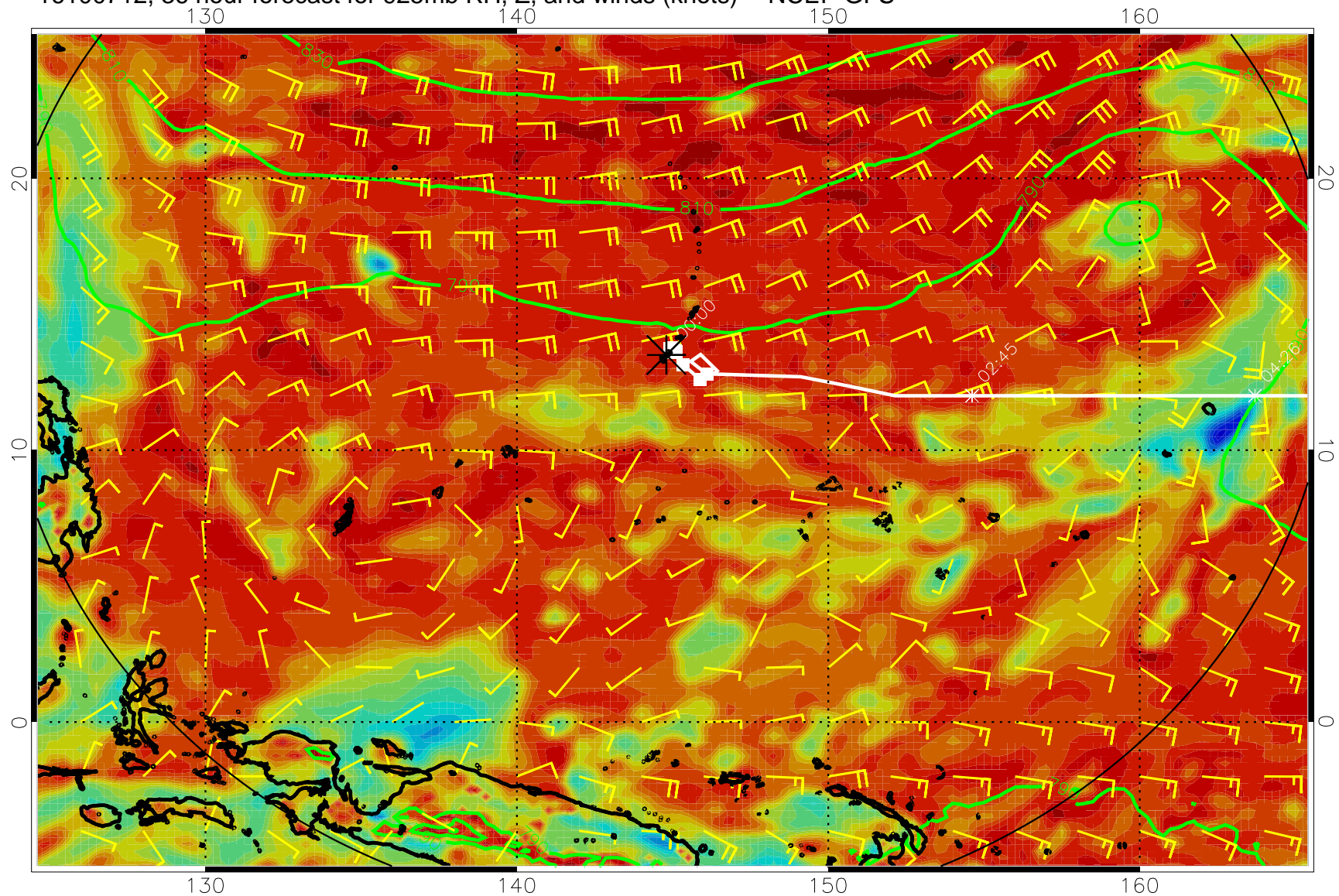
16100712, 36 hour forecast for 925mb RH, Z, and winds (knots) -- NCEP GFS
