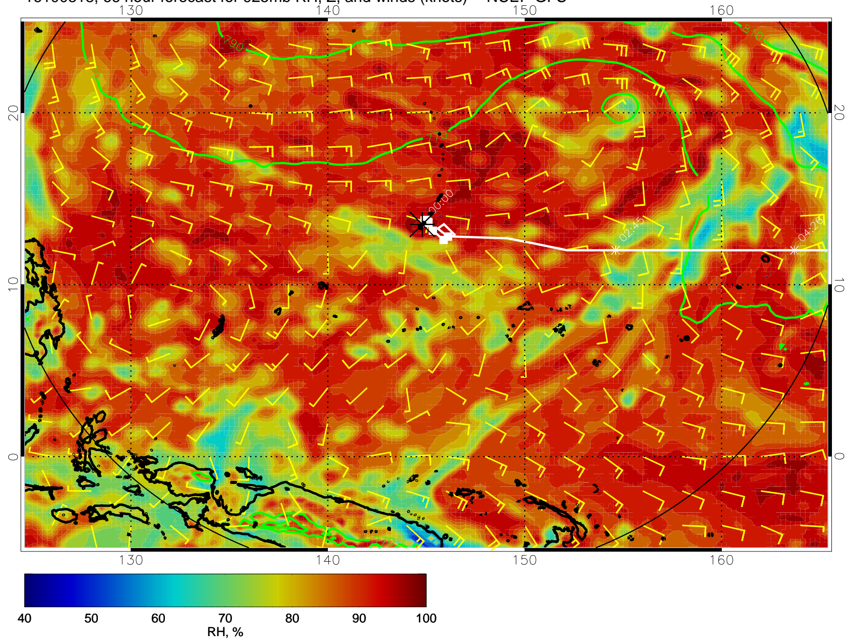
16100818, 66 hour forecast for 925mb RH, Z, and winds (knots) -- NCEP GFS
