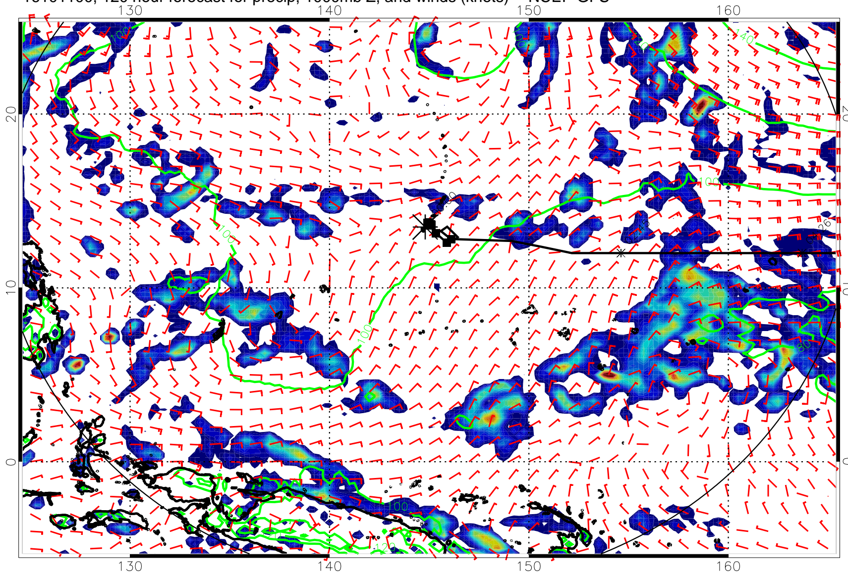
16101100, 120 hour forecast for precip, 1000mb Z, and winds (knots) -- NCEP GFS
