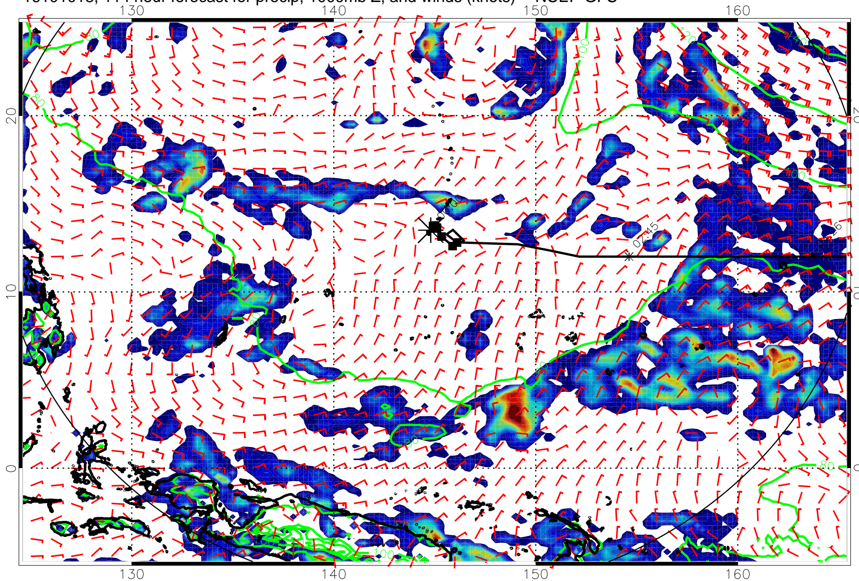
16101018, 114 hour forecast for precip, 1000mb Z, and winds (knots) -- NCEP GFS
