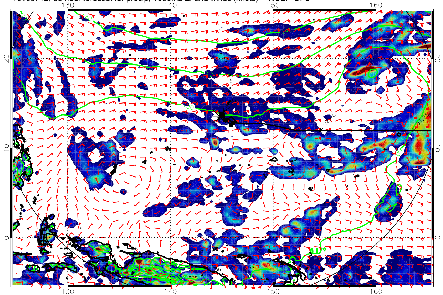
16100712, 36 hour forecast for precip, 1000mb Z, and winds (knots) -- NCEP GFS
