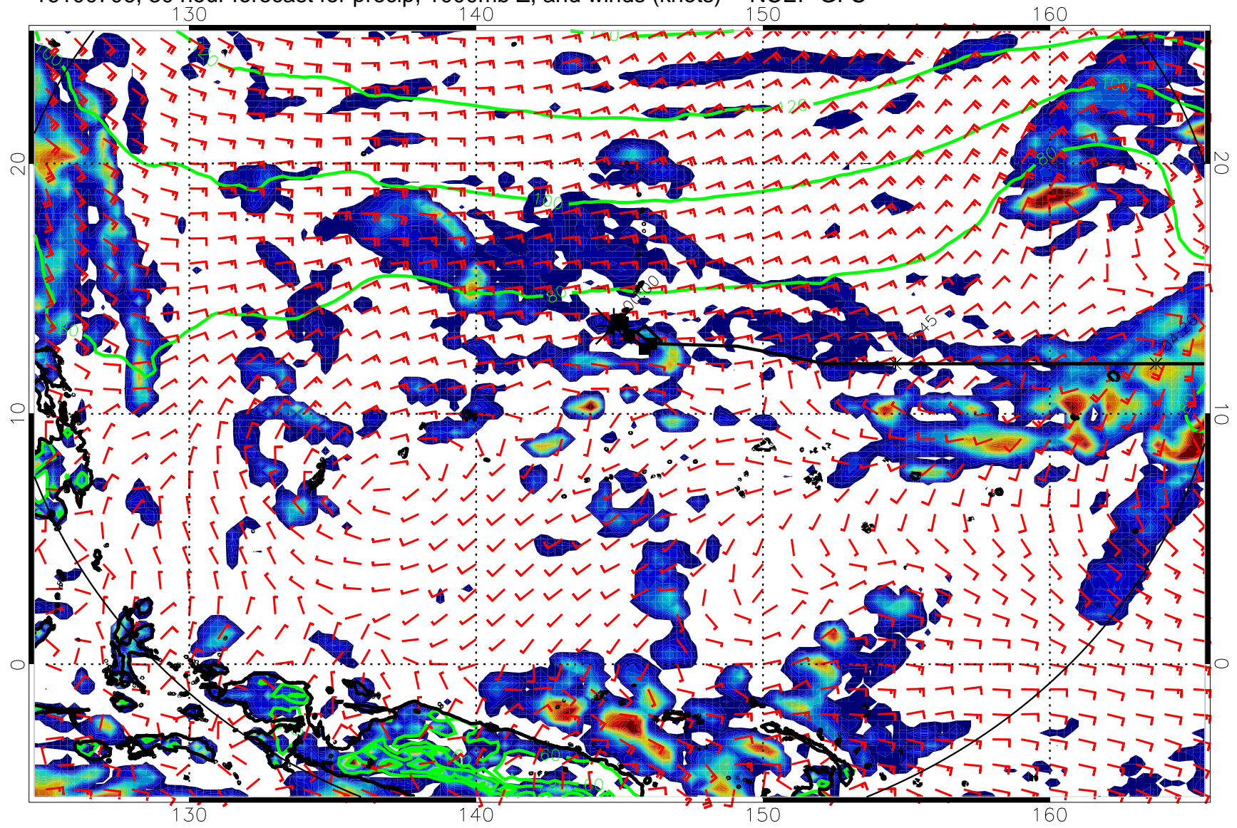
16100706, 30 hour forecast for precip, 1000mb Z, and winds (knots) -- NCEP GFS
