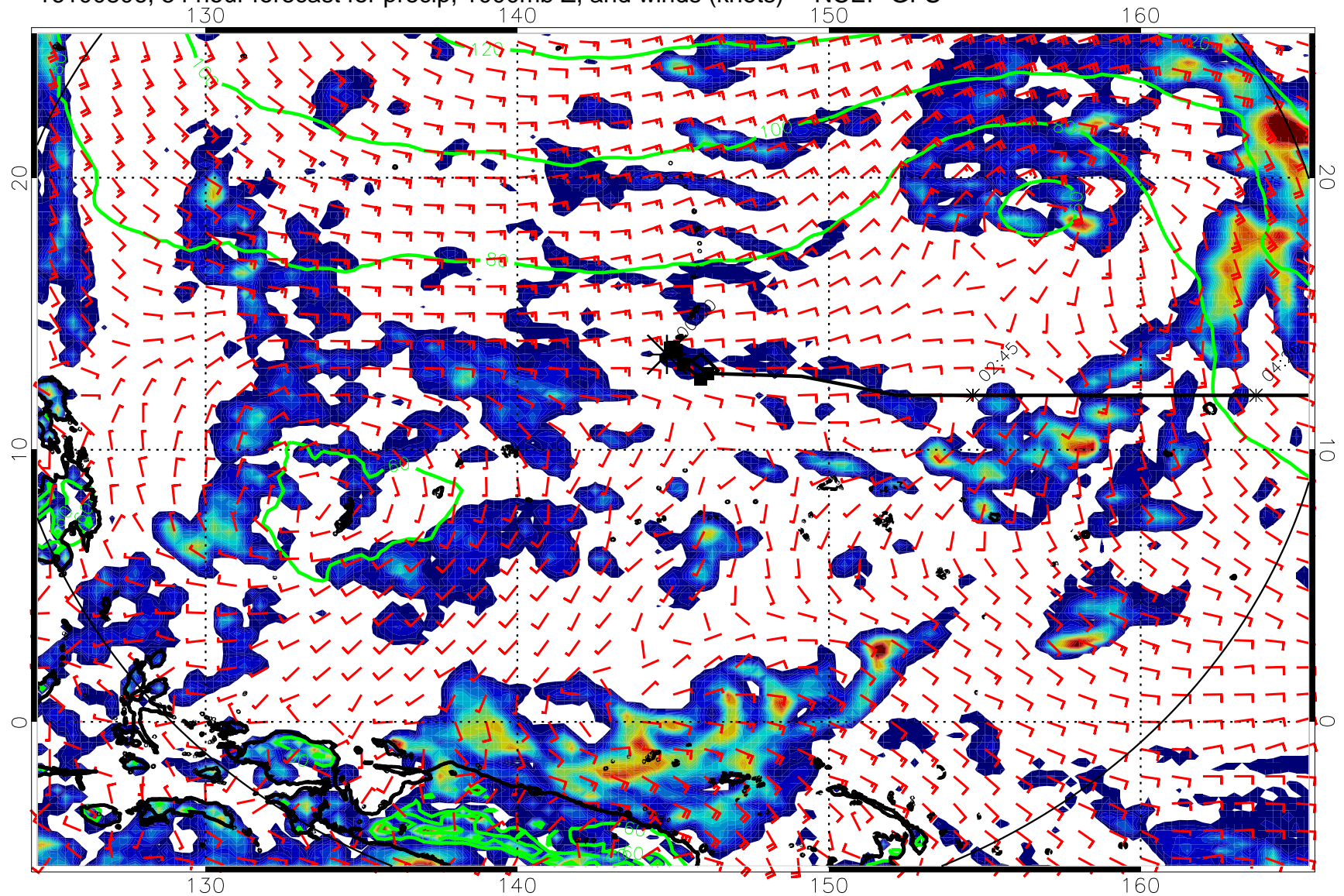
16100806, 54 hour forecast for precip, 1000mb Z, and winds (knots) -- NCEP GFS
