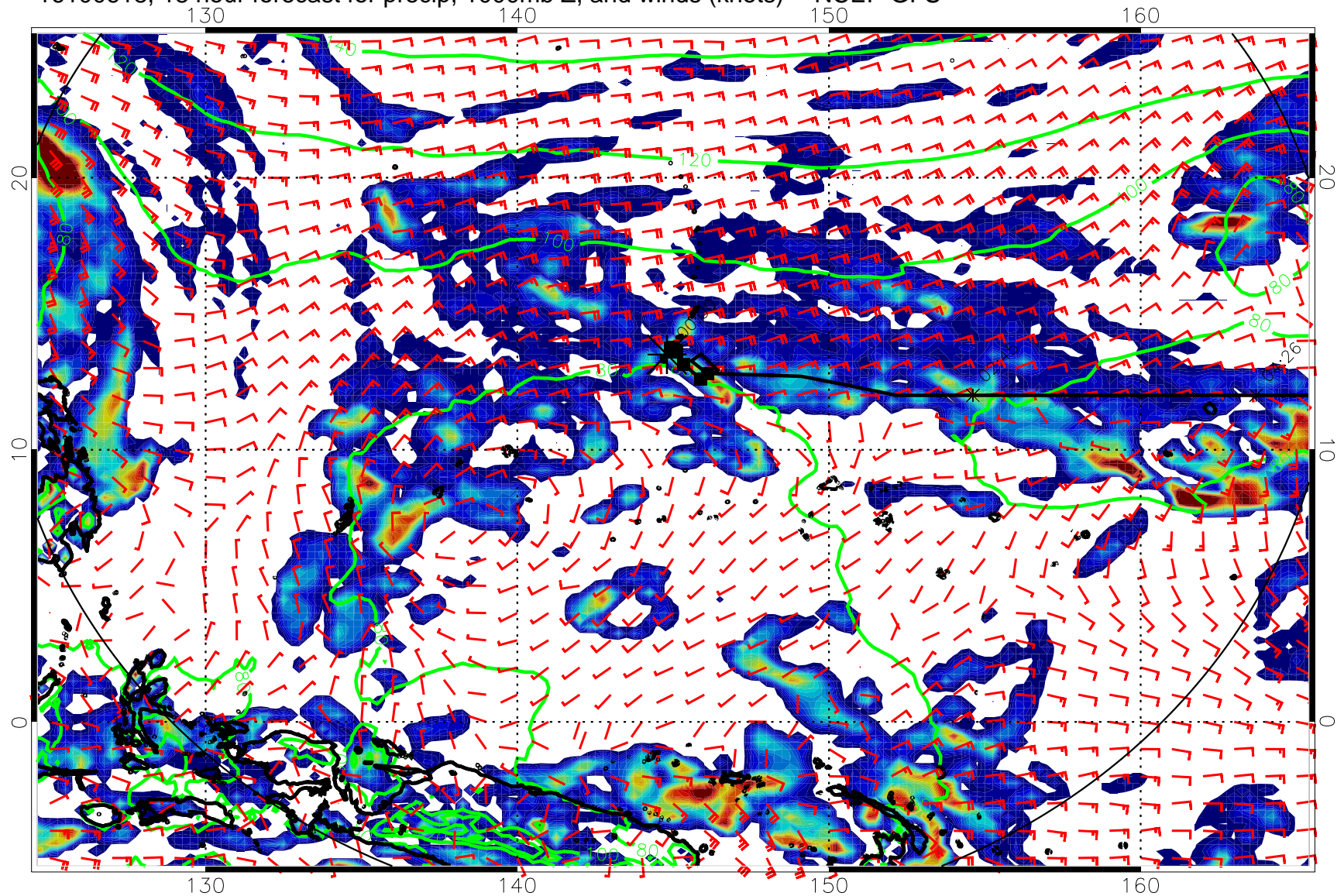
16100618, 18 hour forecast for precip, 1000mb Z, and winds (knots) -- NCEP GFS
