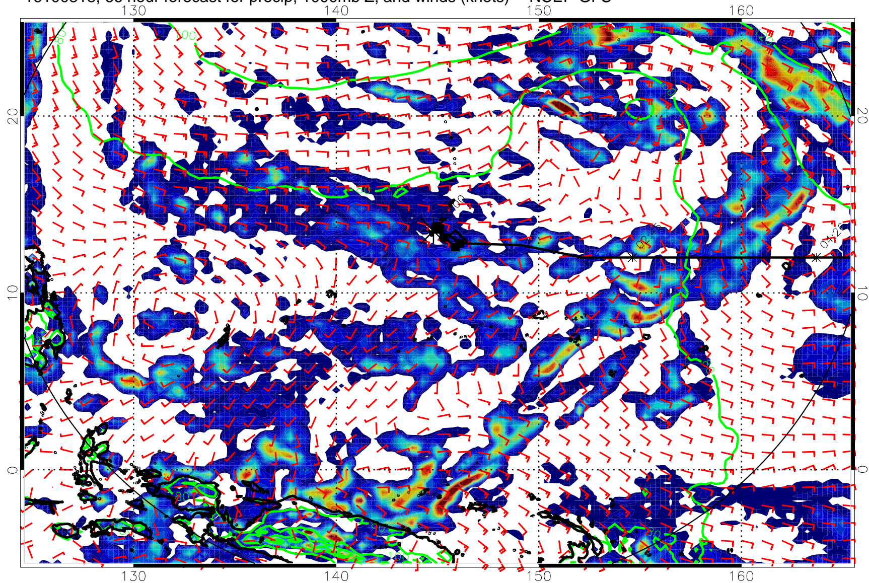
16100818, 66 hour forecast for precip, 1000mb Z, and winds (knots) -- NCEP GFS
