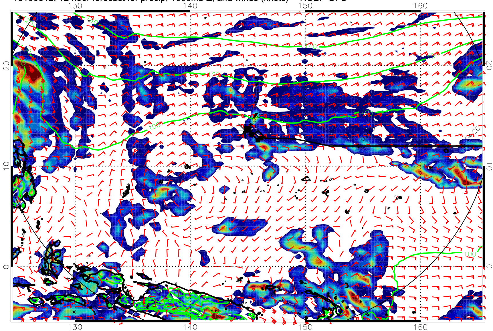
16100612, 12 hour forecast for precip, 1000mb Z, and winds (knots) -- NCEP GFS
