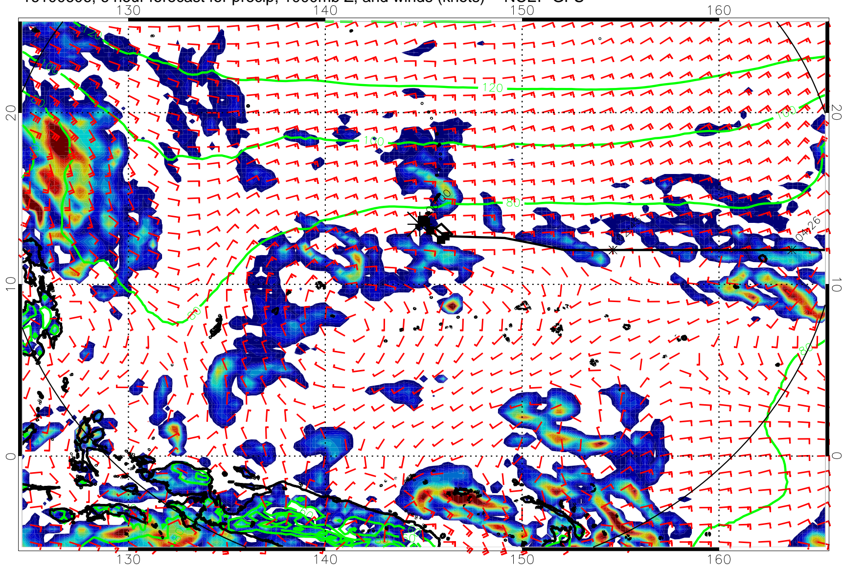
16100606, 6 hour forecast for precip, 1000mb Z, and winds (knots) -- NCEP GFS
