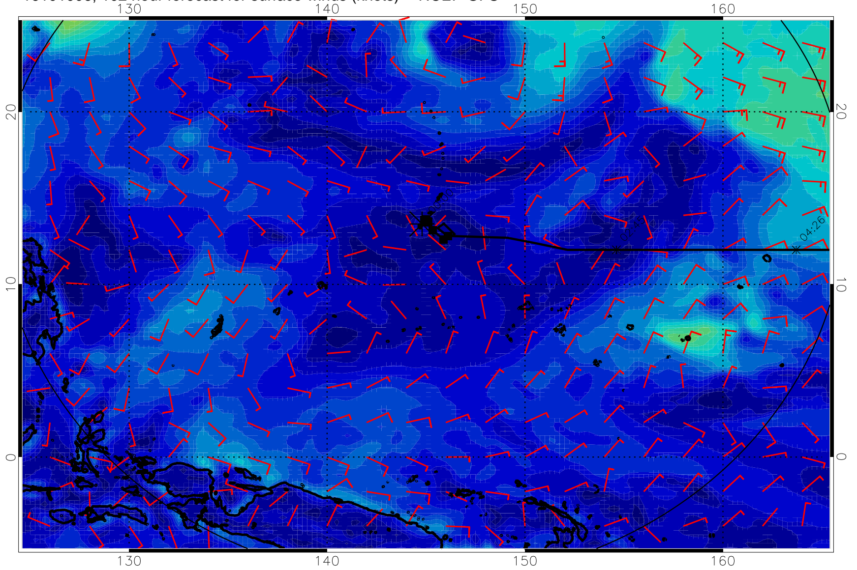
16101006, 102 hour forecast for surface winds (knots) -- NCEP GFS
