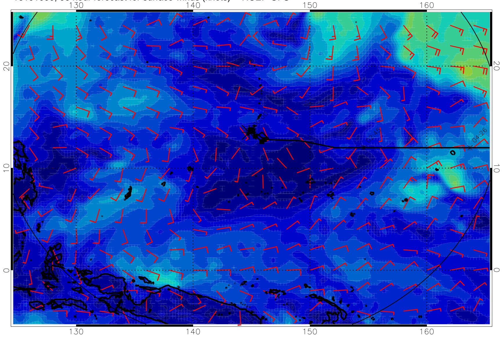
16101000, 96 hour forecast for surface winds (knots) -- NCEP GFS
