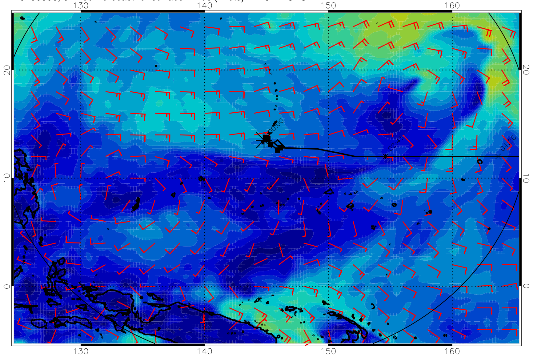
16100806, 54 hour forecast for surface winds (knots) -- NCEP GFS
