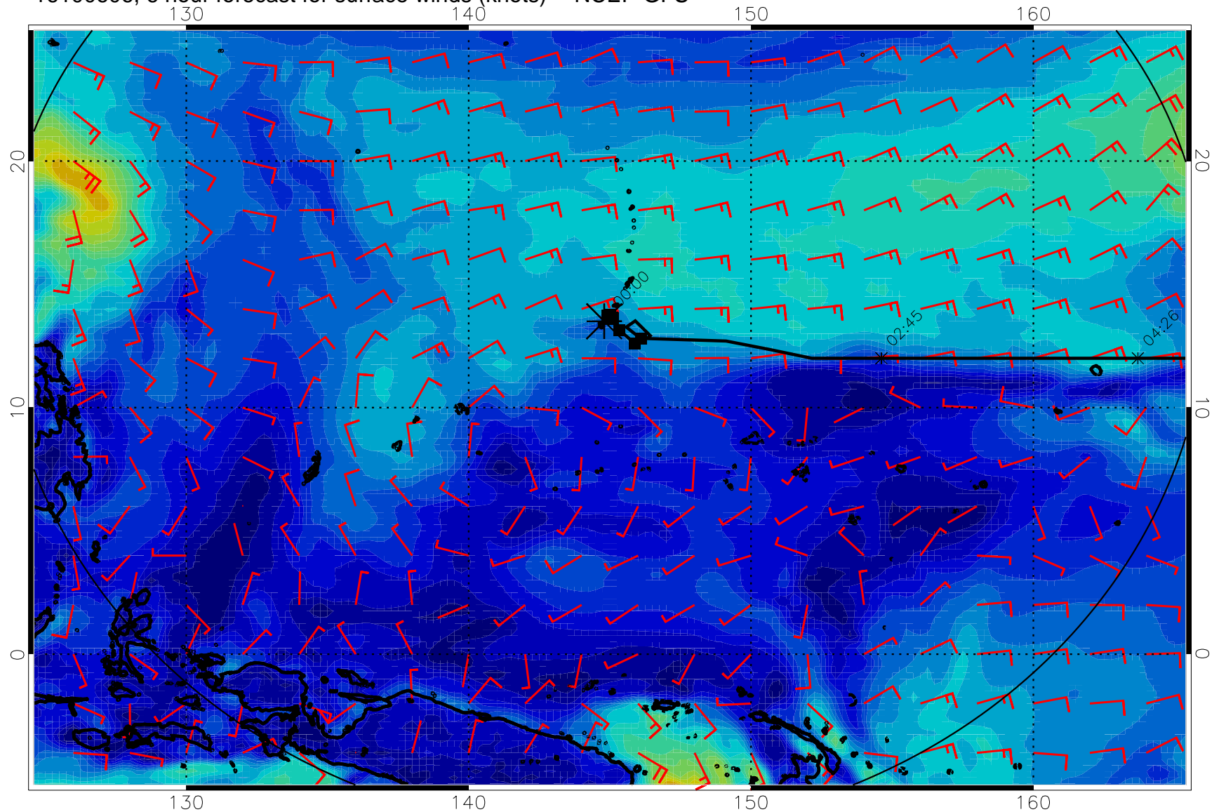
16100606, 6 hour forecast for surface winds (knots) -- NCEP GFS
