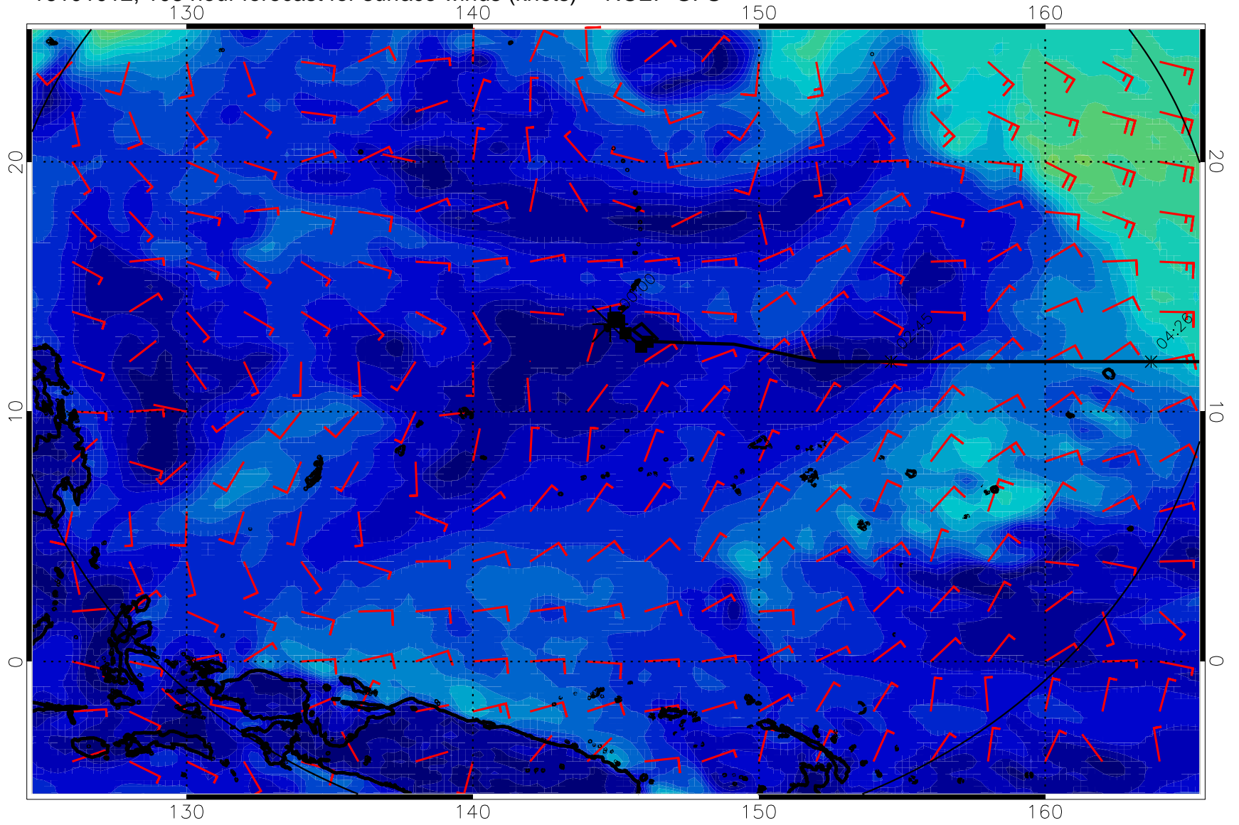
16101012, 108 hour forecast for surface winds (knots) -- NCEP GFS
