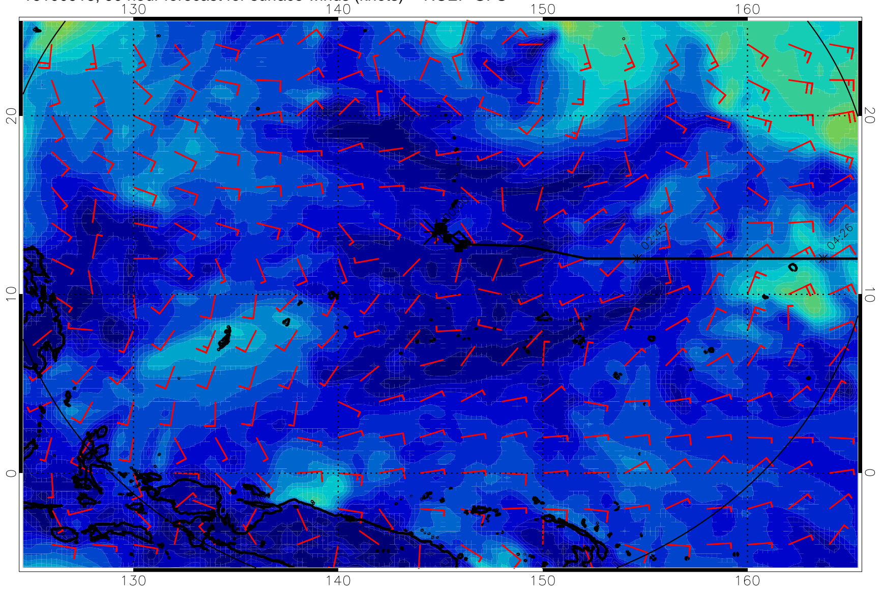
16100918, 90 hour forecast for surface winds (knots) -- NCEP GFS
