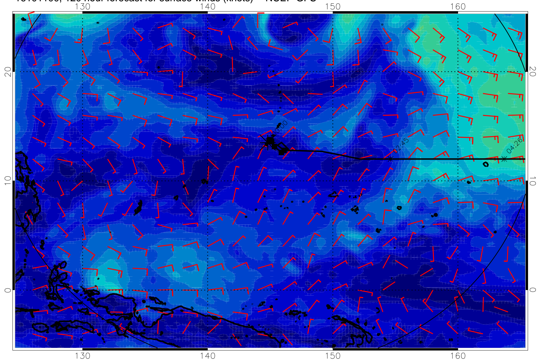
16101100, 120 hour forecast for surface winds (knots) -- NCEP GFS
