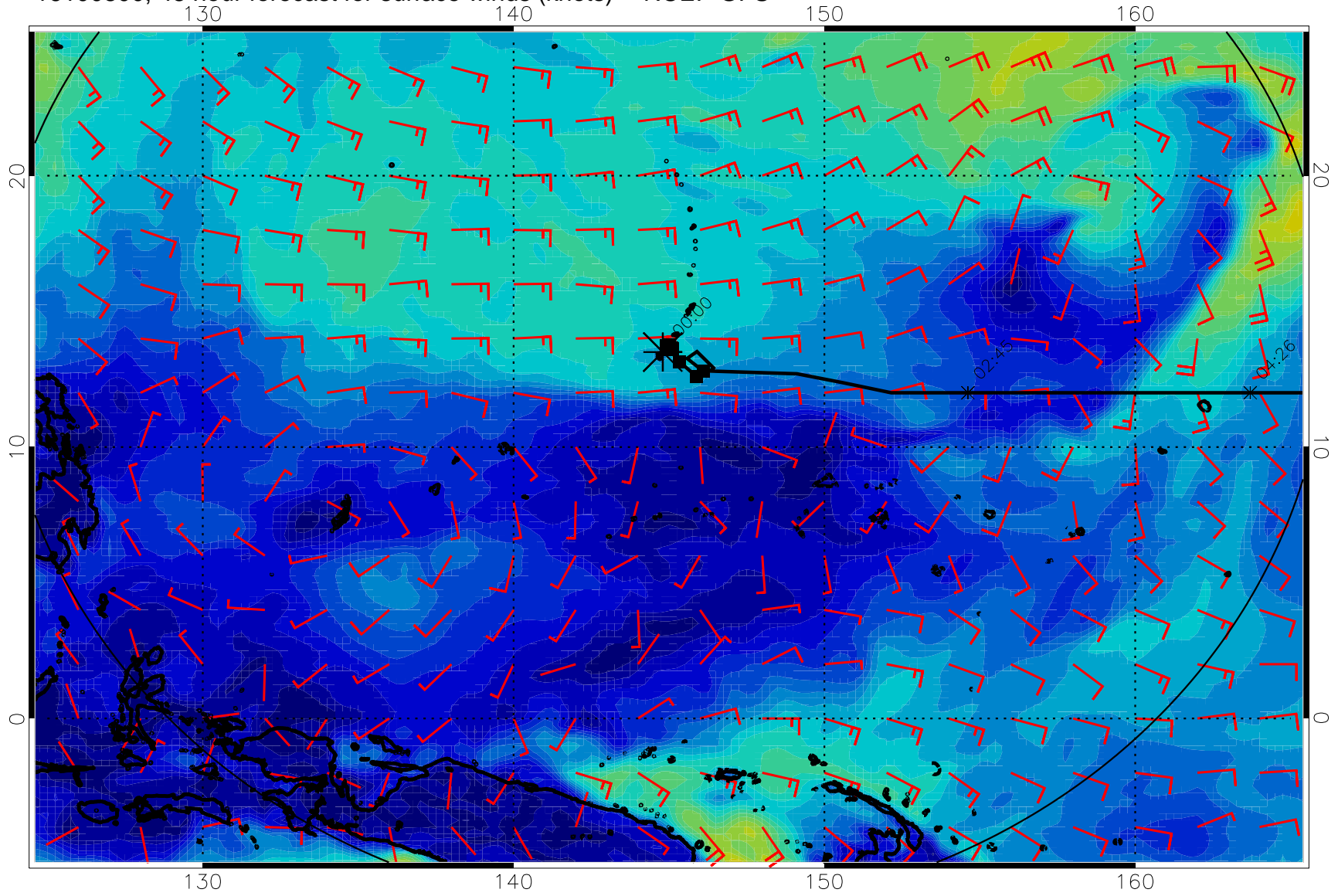
16100800, 48 hour forecast for surface winds (knots) -- NCEP GFS
