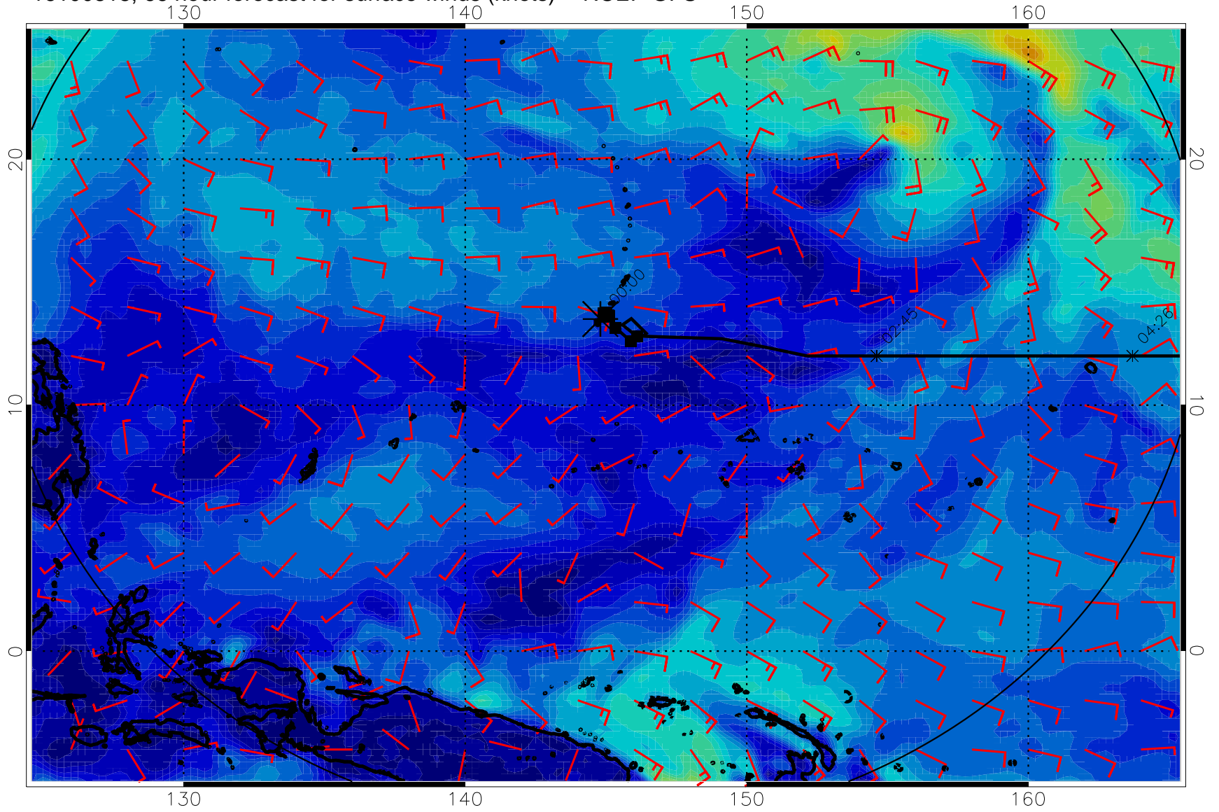
16100818, 66 hour forecast for surface winds (knots) -- NCEP GFS
