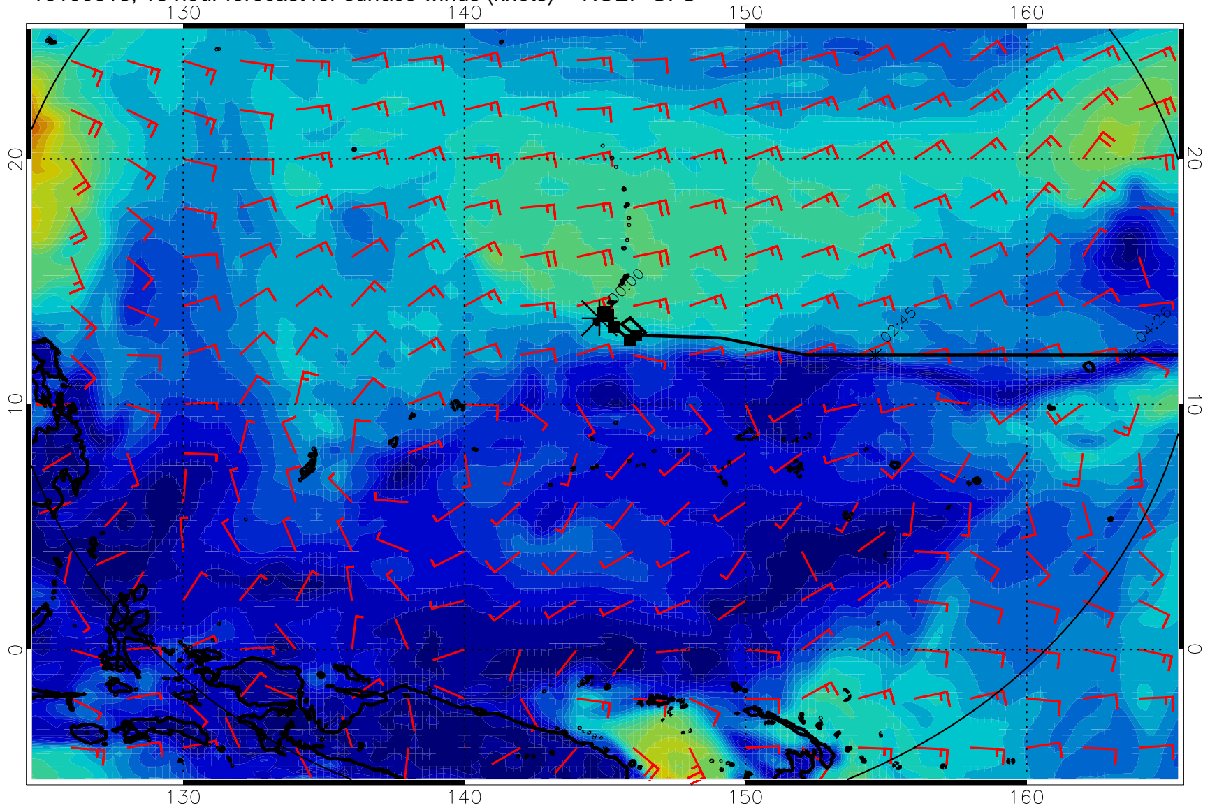
16100618, 18 hour forecast for surface winds (knots) -- NCEP GFS
