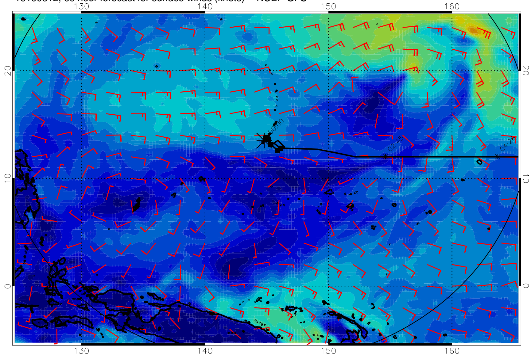
16100812, 60 hour forecast for surface winds (knots) -- NCEP GFS
