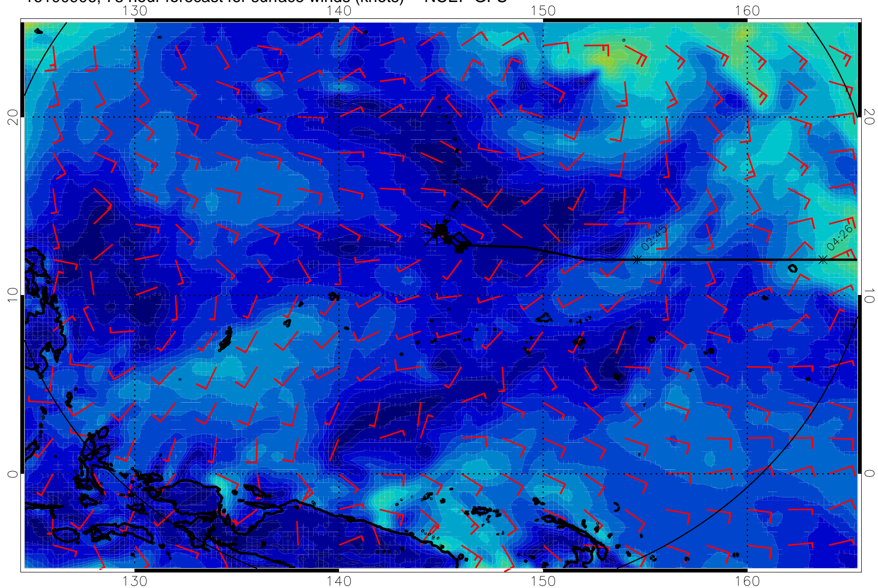
16100906, 78 hour forecast for surface winds (knots) -- NCEP GFS
