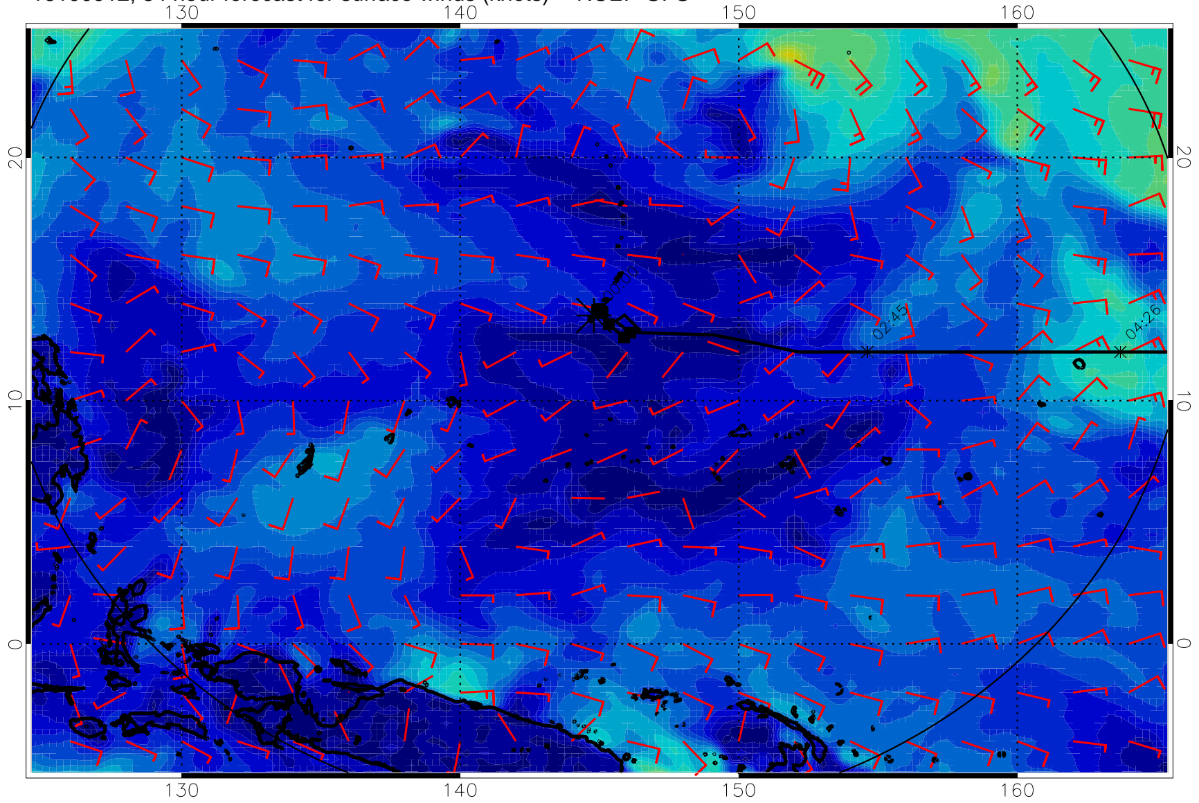
16100912, 84 hour forecast for surface winds (knots) -- NCEP GFS
