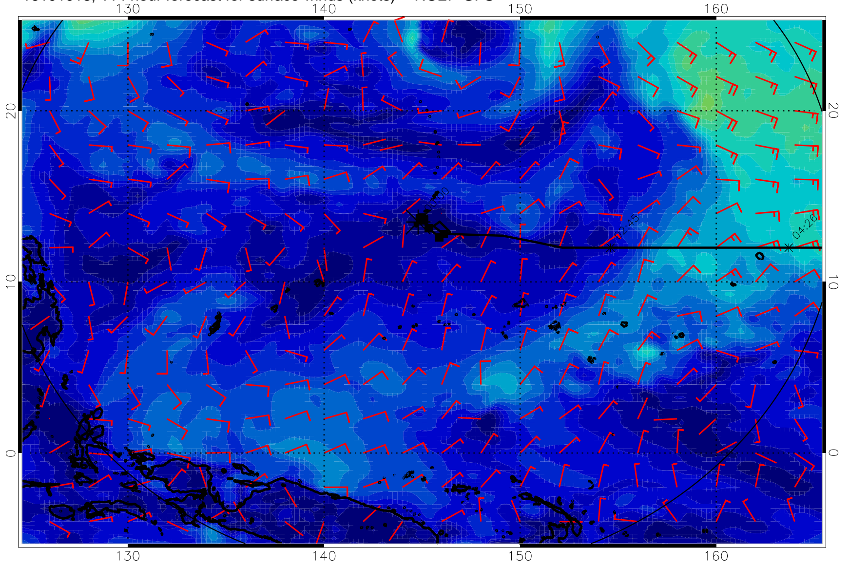
16101018, 114 hour forecast for surface winds (knots) -- NCEP GFS
