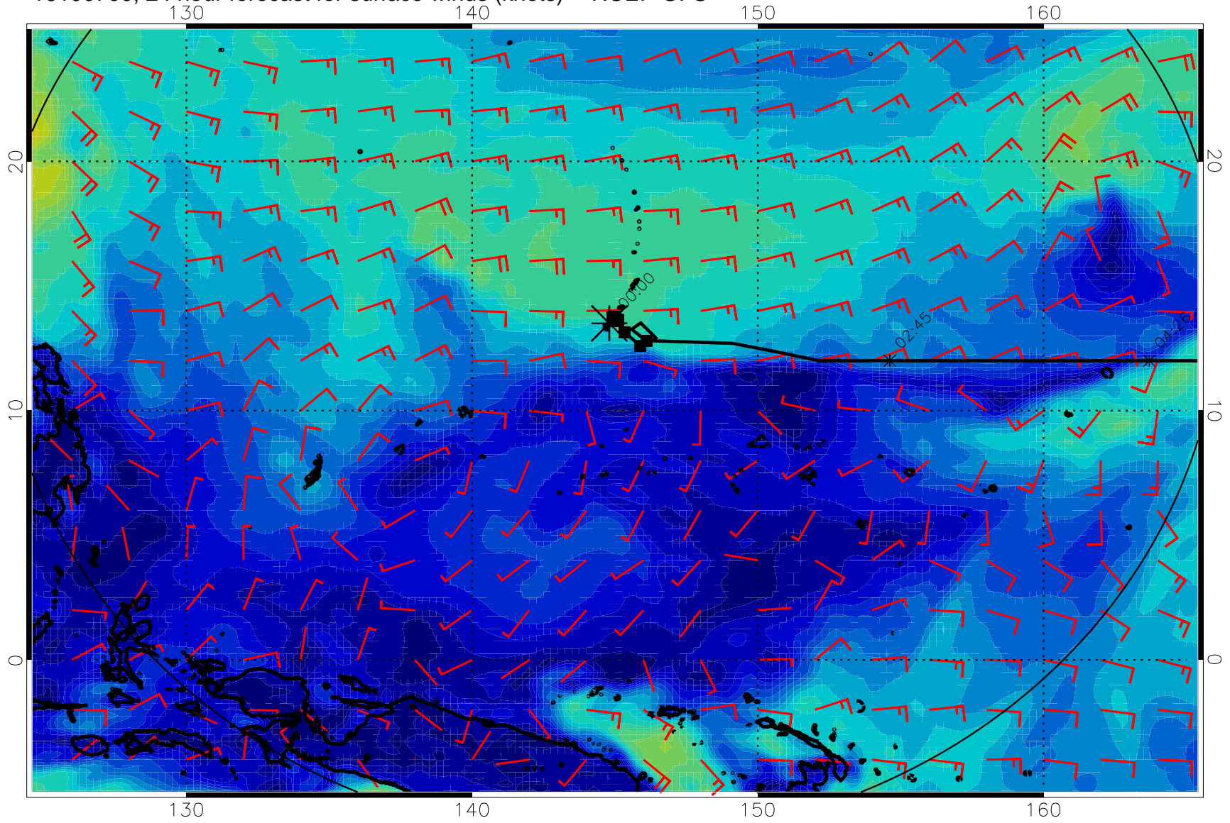
16100700, 24 hour forecast for surface winds (knots) -- NCEP GFS
