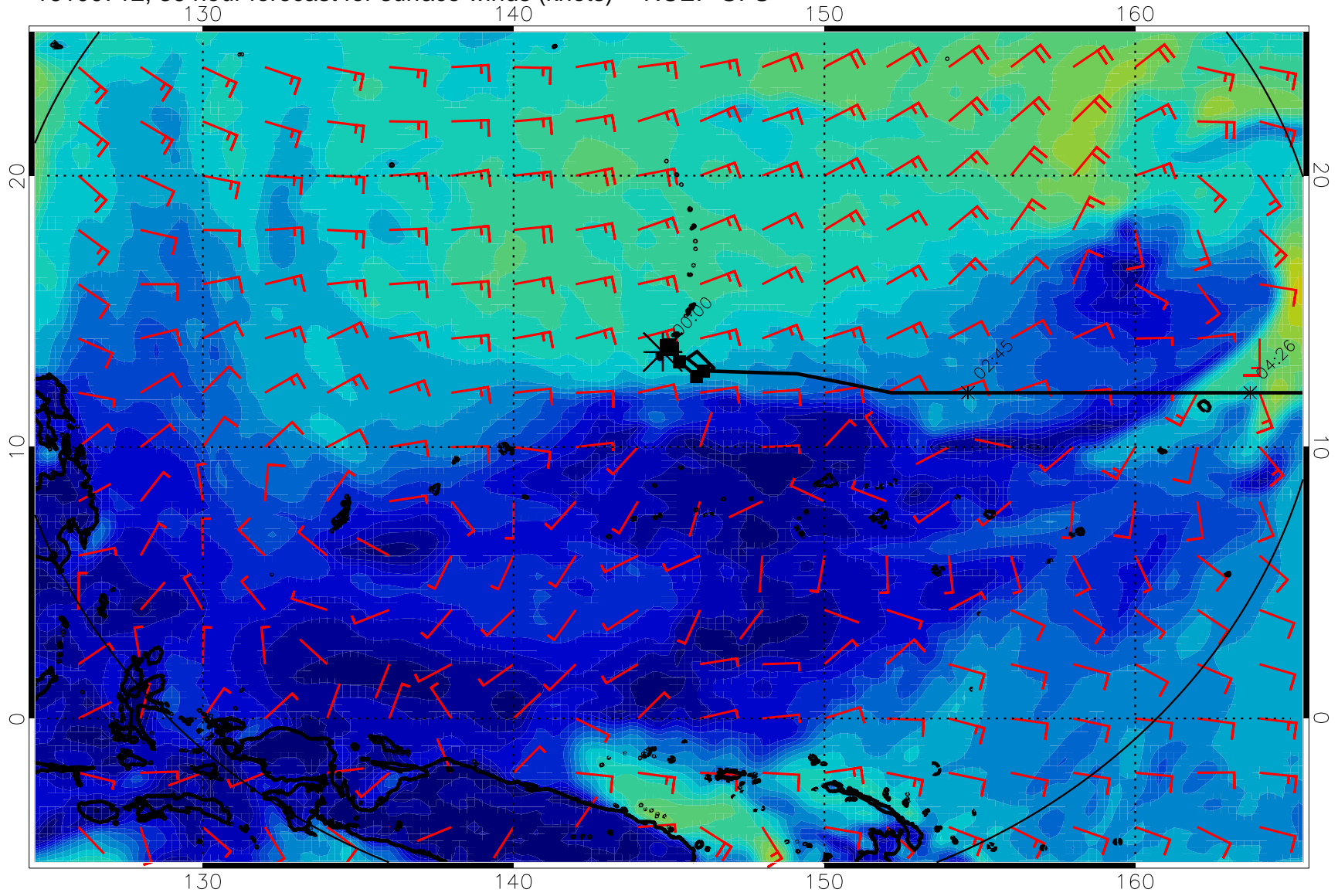
16100712, 36 hour forecast for surface winds (knots) -- NCEP GFS
