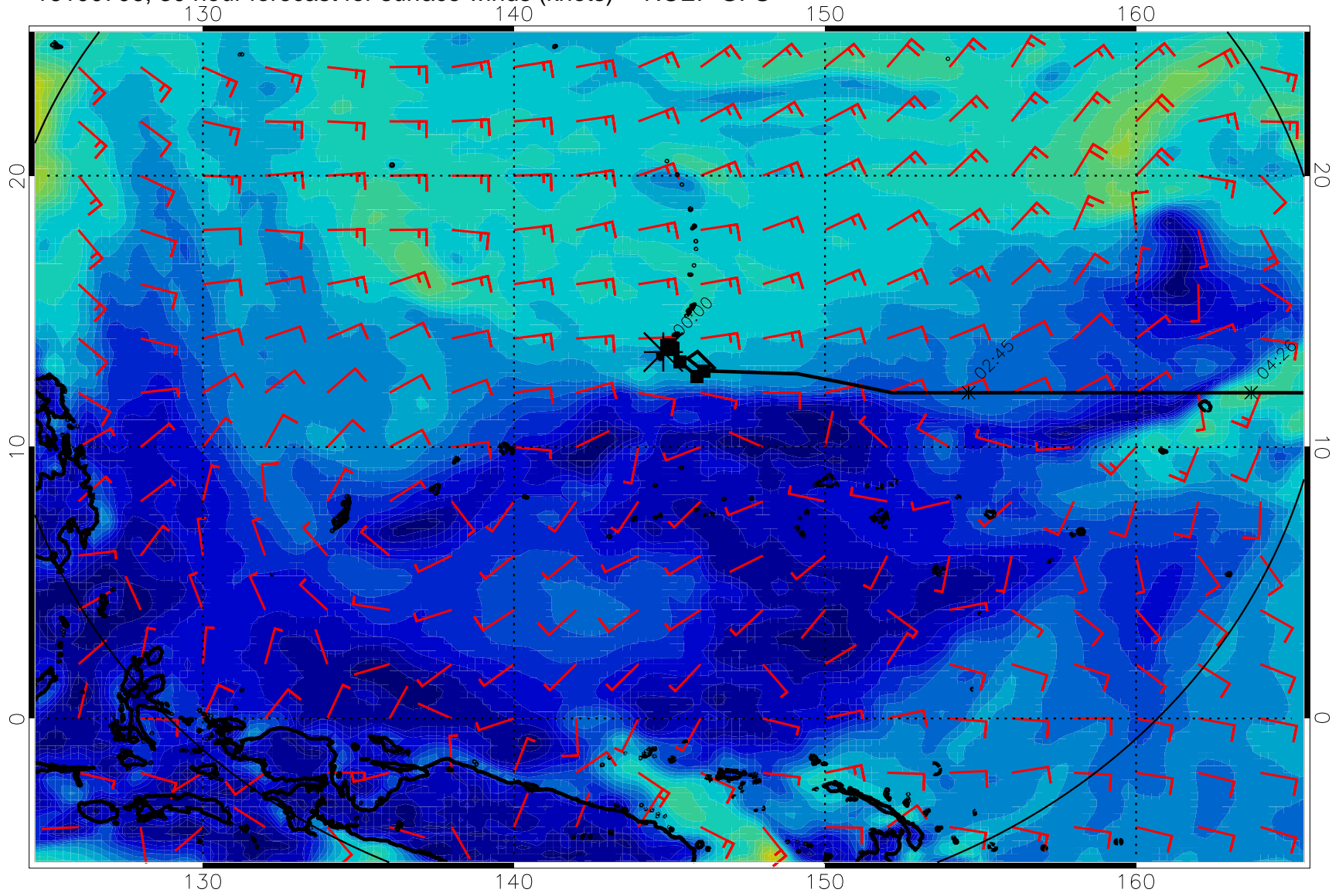
16100706, 30 hour forecast for surface winds (knots) -- NCEP GFS
