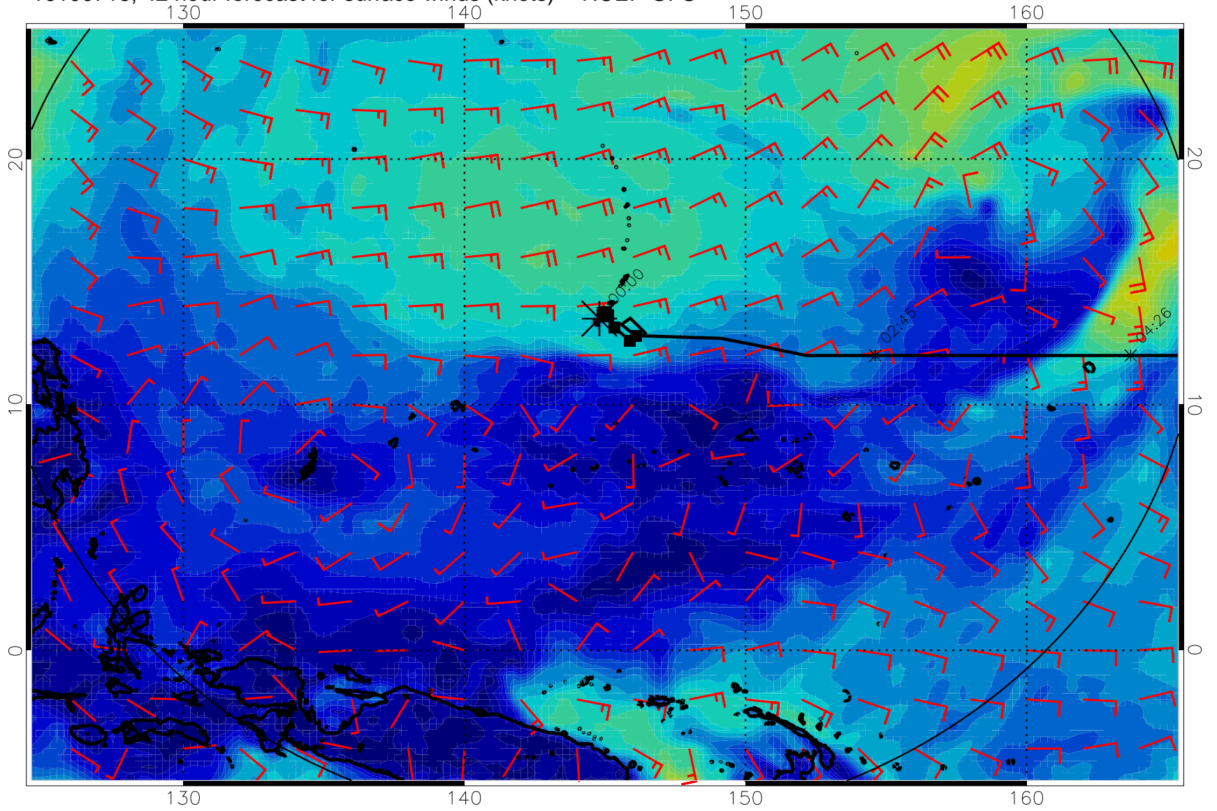
16100718, 42 hour forecast for surface winds (knots) -- NCEP GFS
