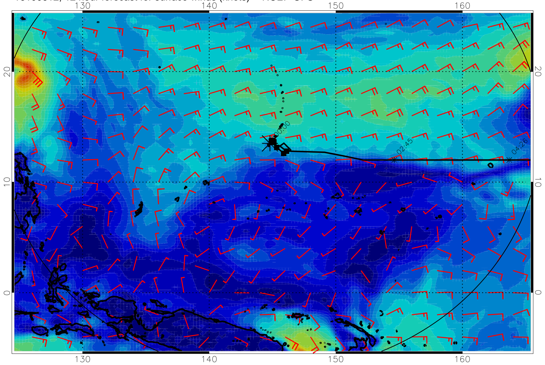
16100612, 12 hour forecast for surface winds (knots) -- NCEP GFS
