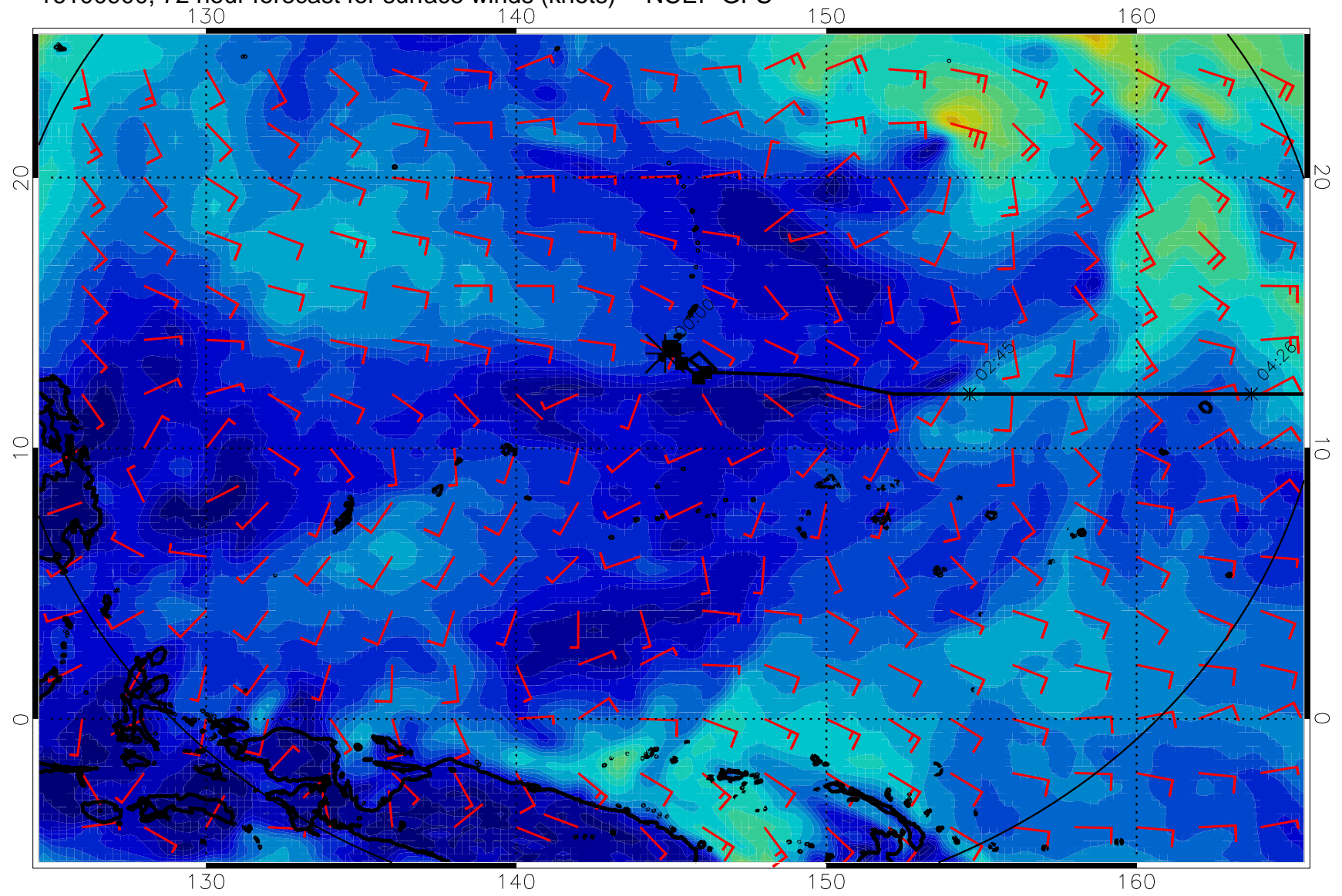
16100900, 72 hour forecast for surface winds (knots) -- NCEP GFS
