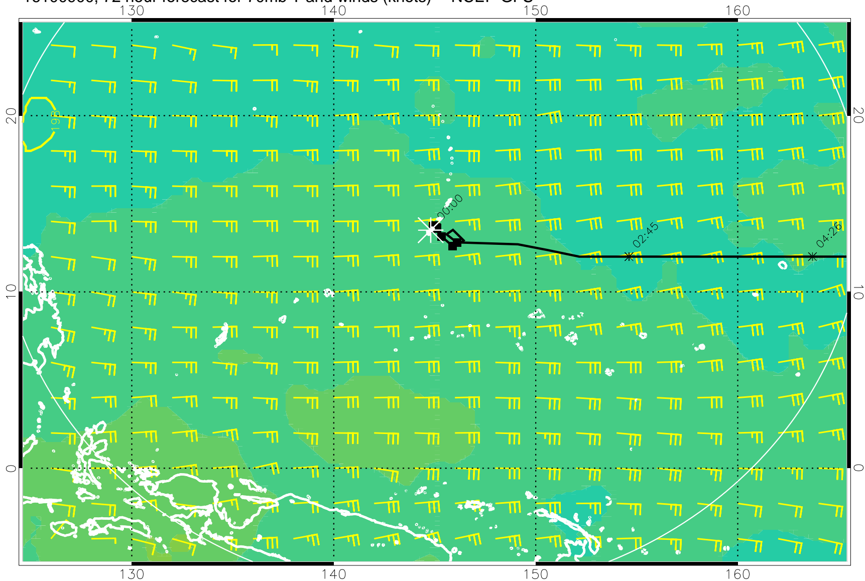
16100900, 72 hour forecast for 70mb T and winds (knots) -- NCEP GFS
