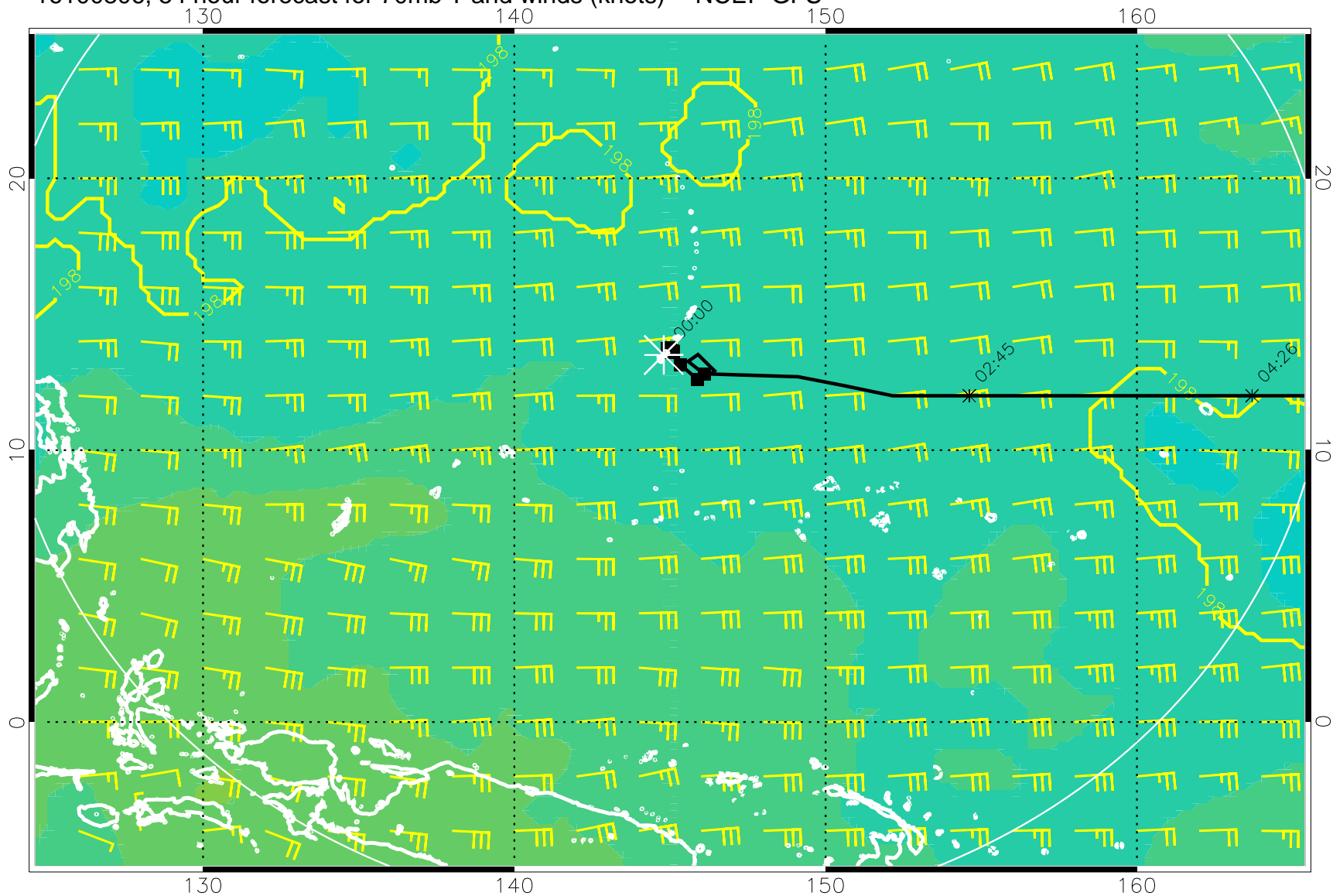
16100806, 54 hour forecast for 70mb T and winds (knots) -- NCEP GFS
