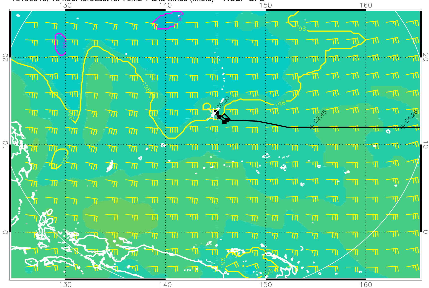
16100618, 18 hour forecast for 70mb T and winds (knots) -- NCEP GFS
