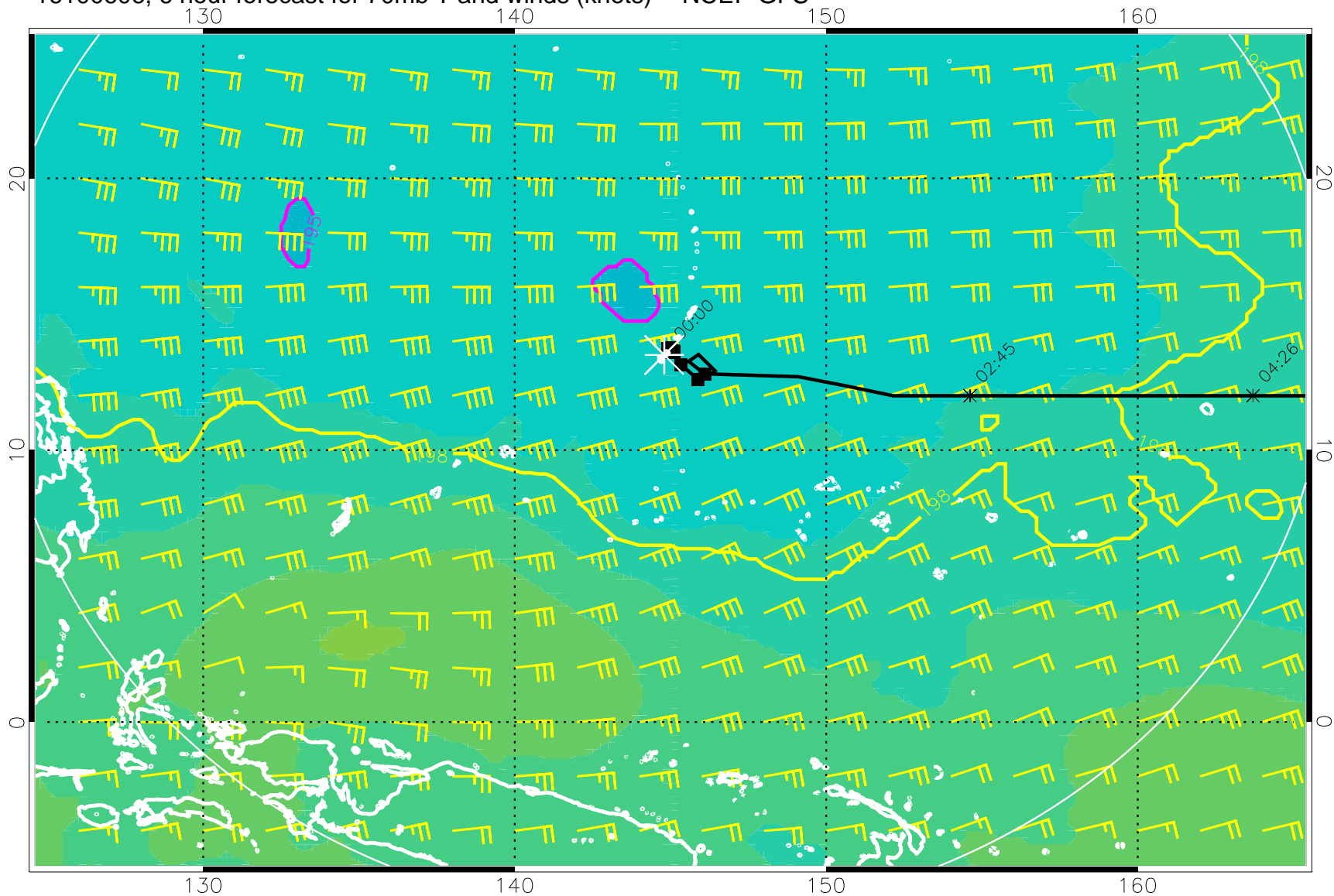
16100606, 6 hour forecast for 70mb T and winds (knots) -- NCEP GFS
