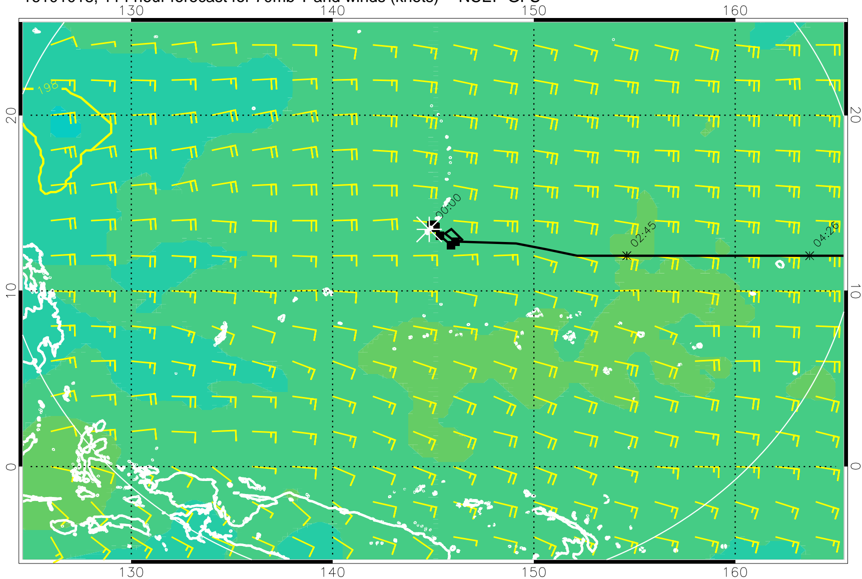
16101018, 114 hour forecast for 70mb T and winds (knots) -- NCEP GFS
