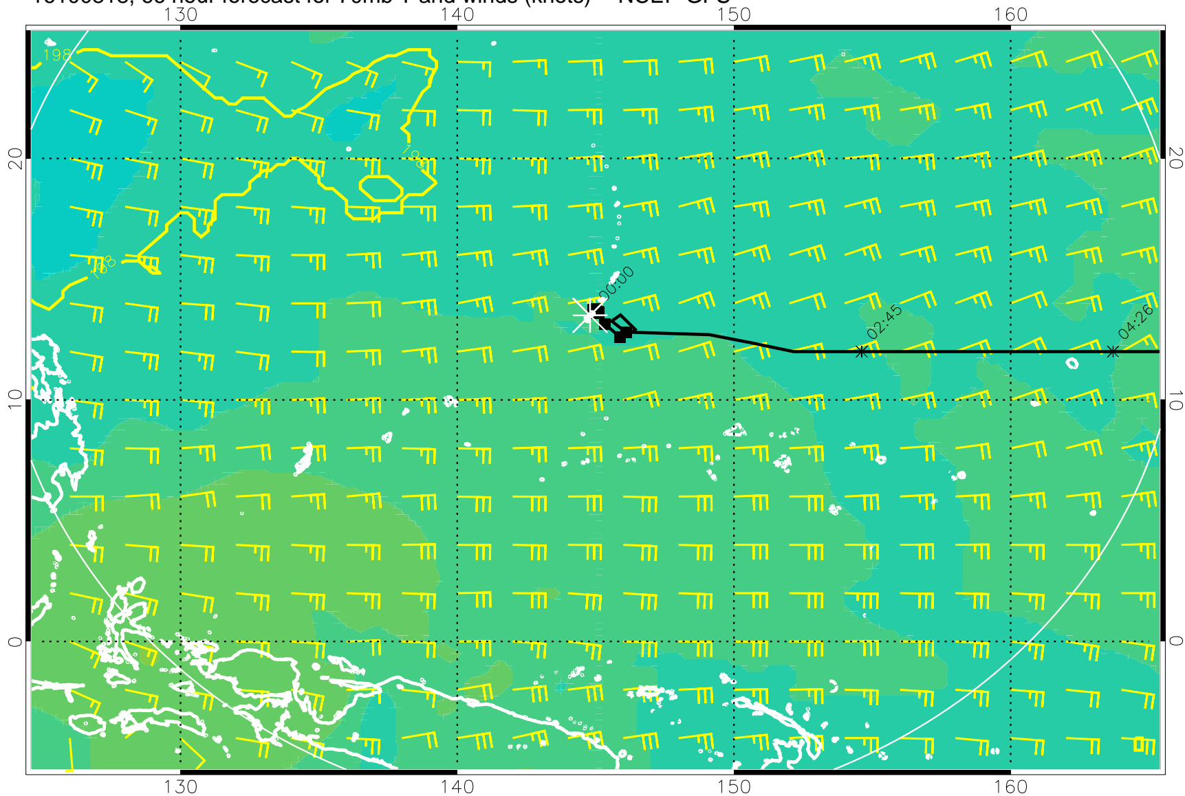
16100818, 66 hour forecast for 70mb T and winds (knots) -- NCEP GFS
