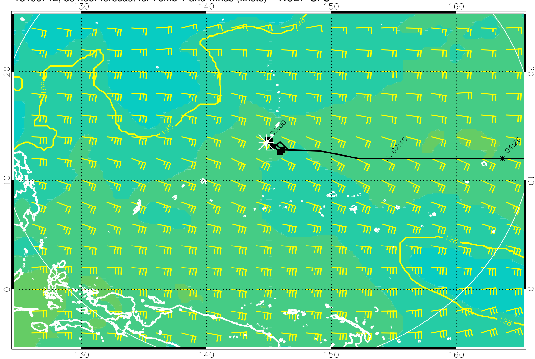
16100712, 36 hour forecast for 70mb T and winds (knots) -- NCEP GFS
