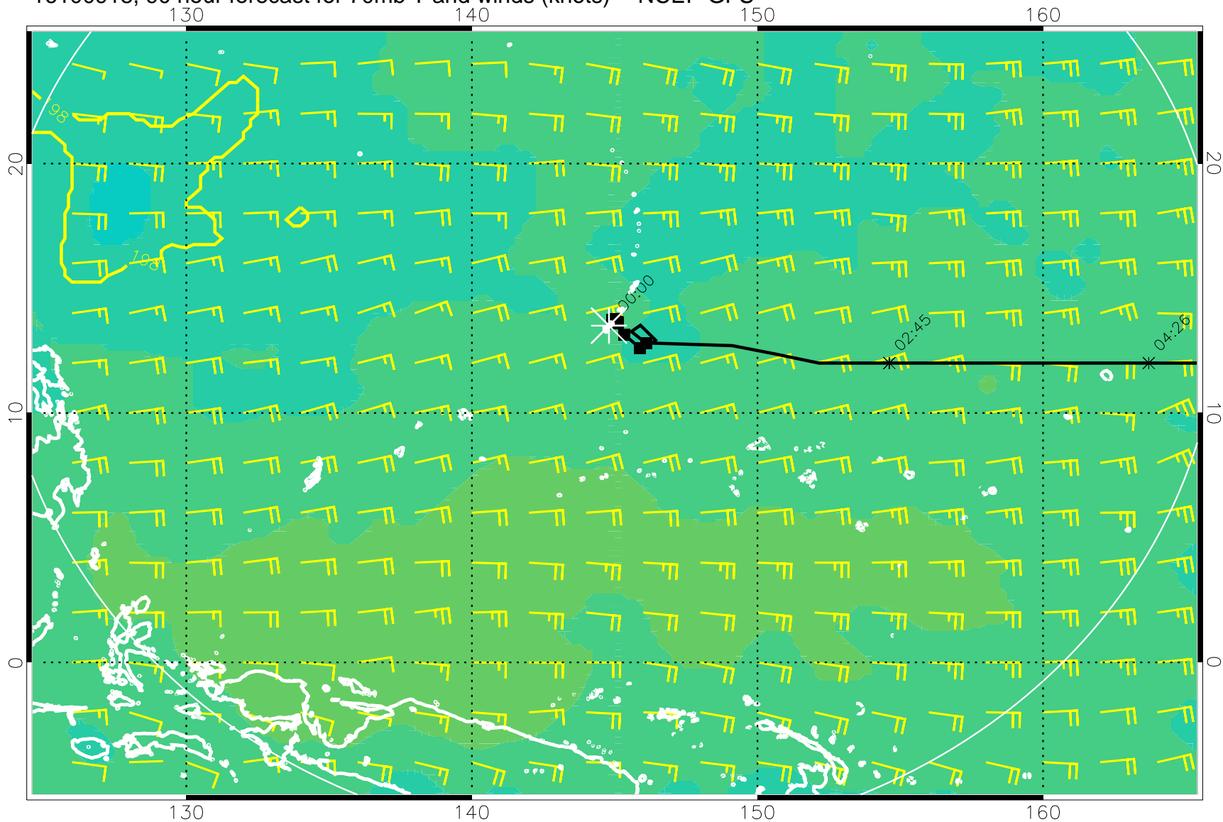
16100918, 90 hour forecast for 70mb T and winds (knots) -- NCEP GFS
