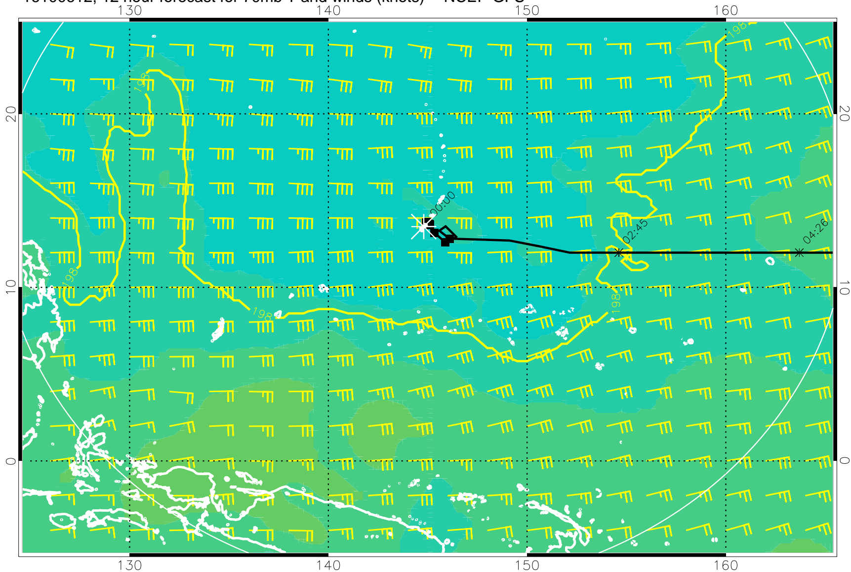
16100612, 12 hour forecast for 70mb T and winds (knots) -- NCEP GFS
