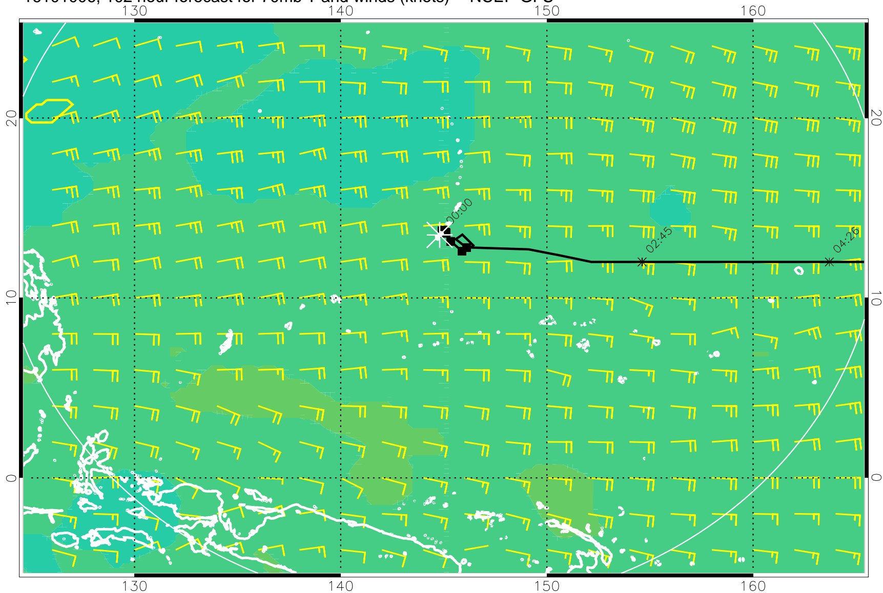
16101006, 102 hour forecast for 70mb T and winds (knots) -- NCEP GFS
