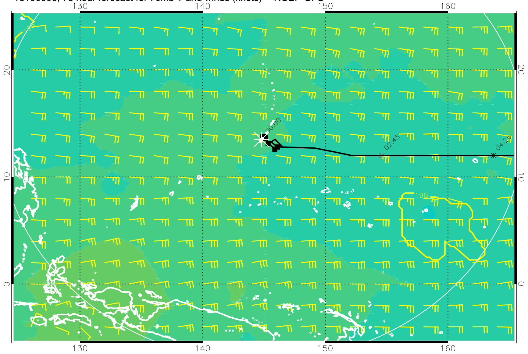
16100906, 78 hour forecast for 70mb T and winds (knots) -- NCEP GFS
