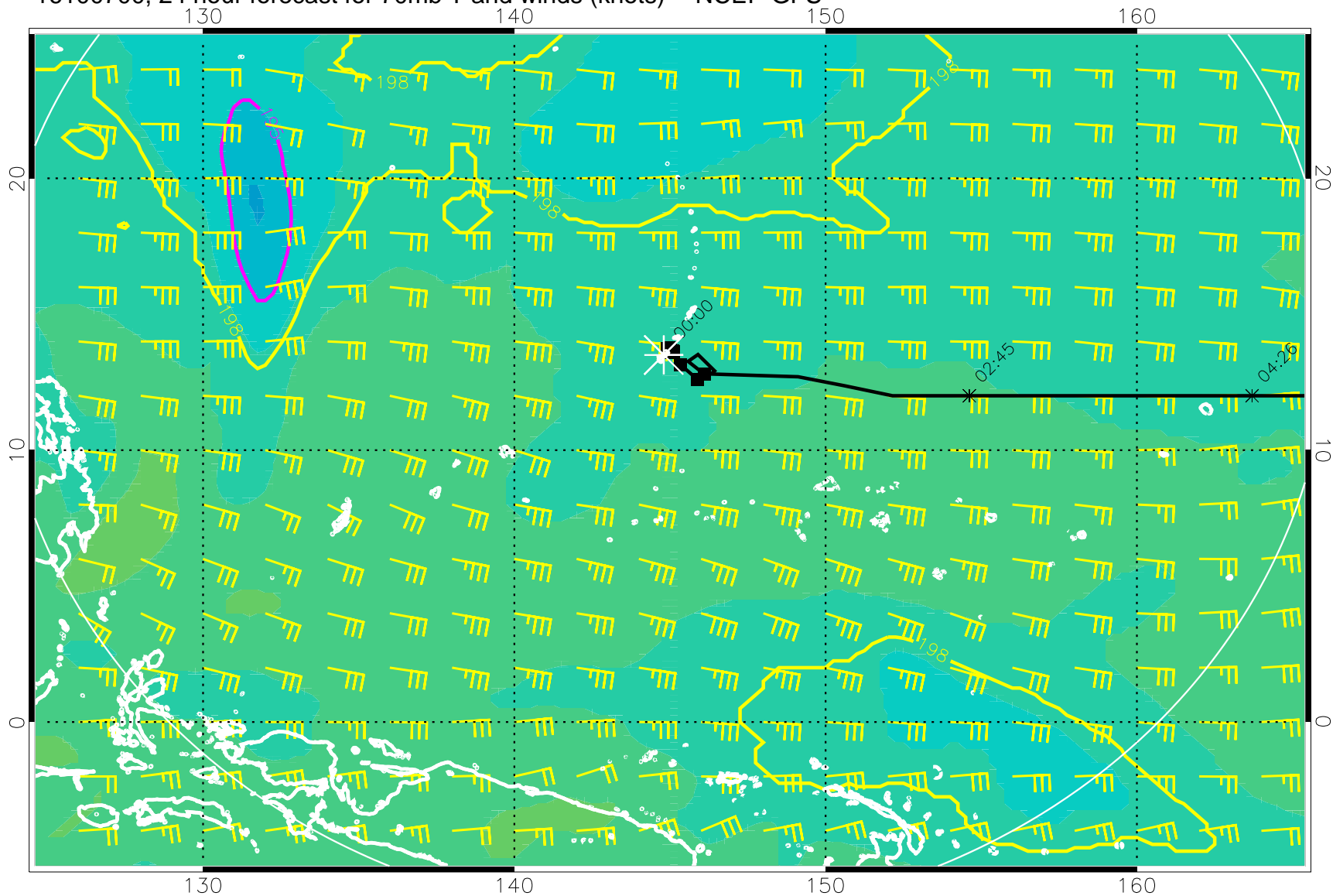
16100700, 24 hour forecast for 70mb T and winds (knots) -- NCEP GFS
