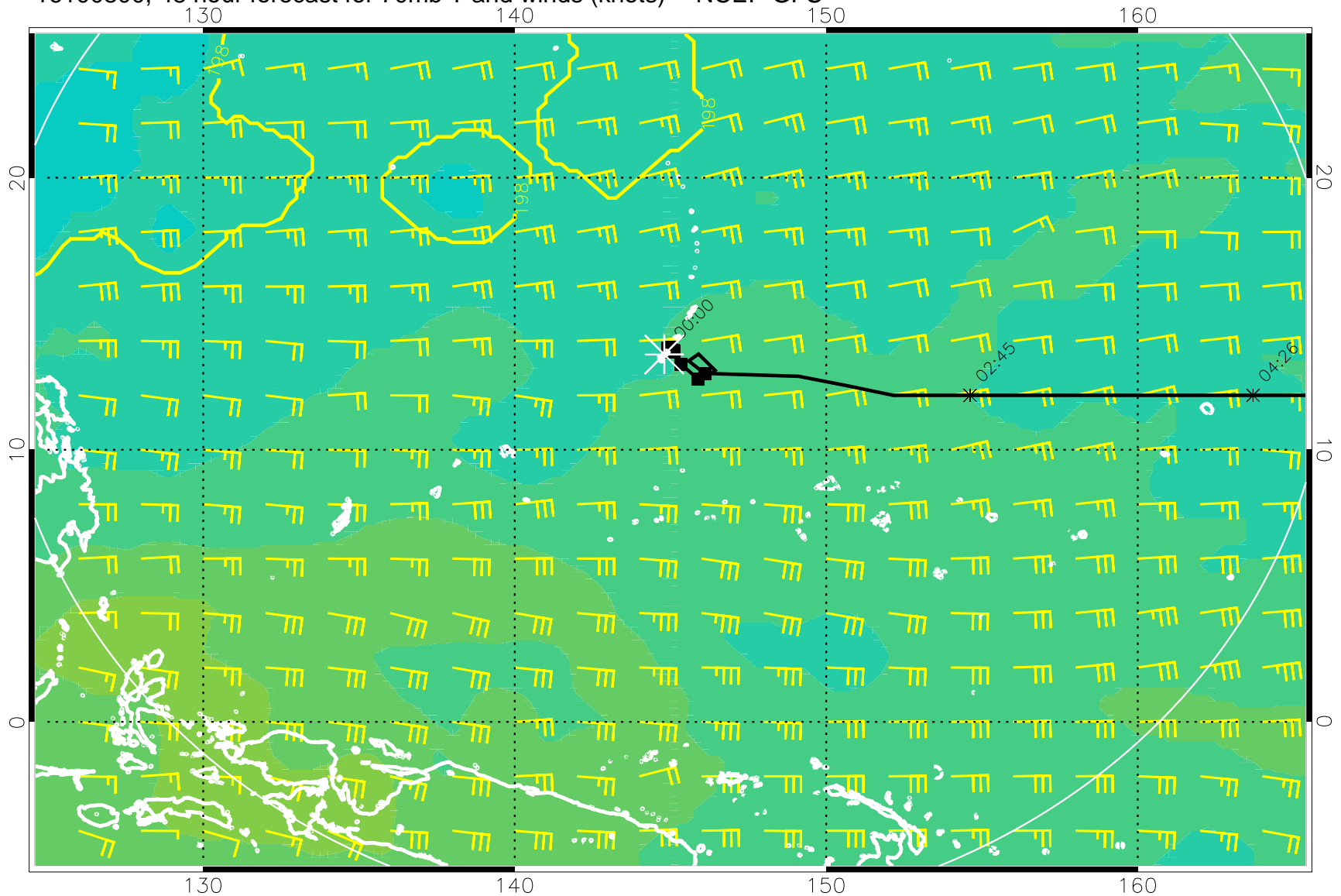
16100800, 48 hour forecast for 70mb T and winds (knots) -- NCEP GFS
