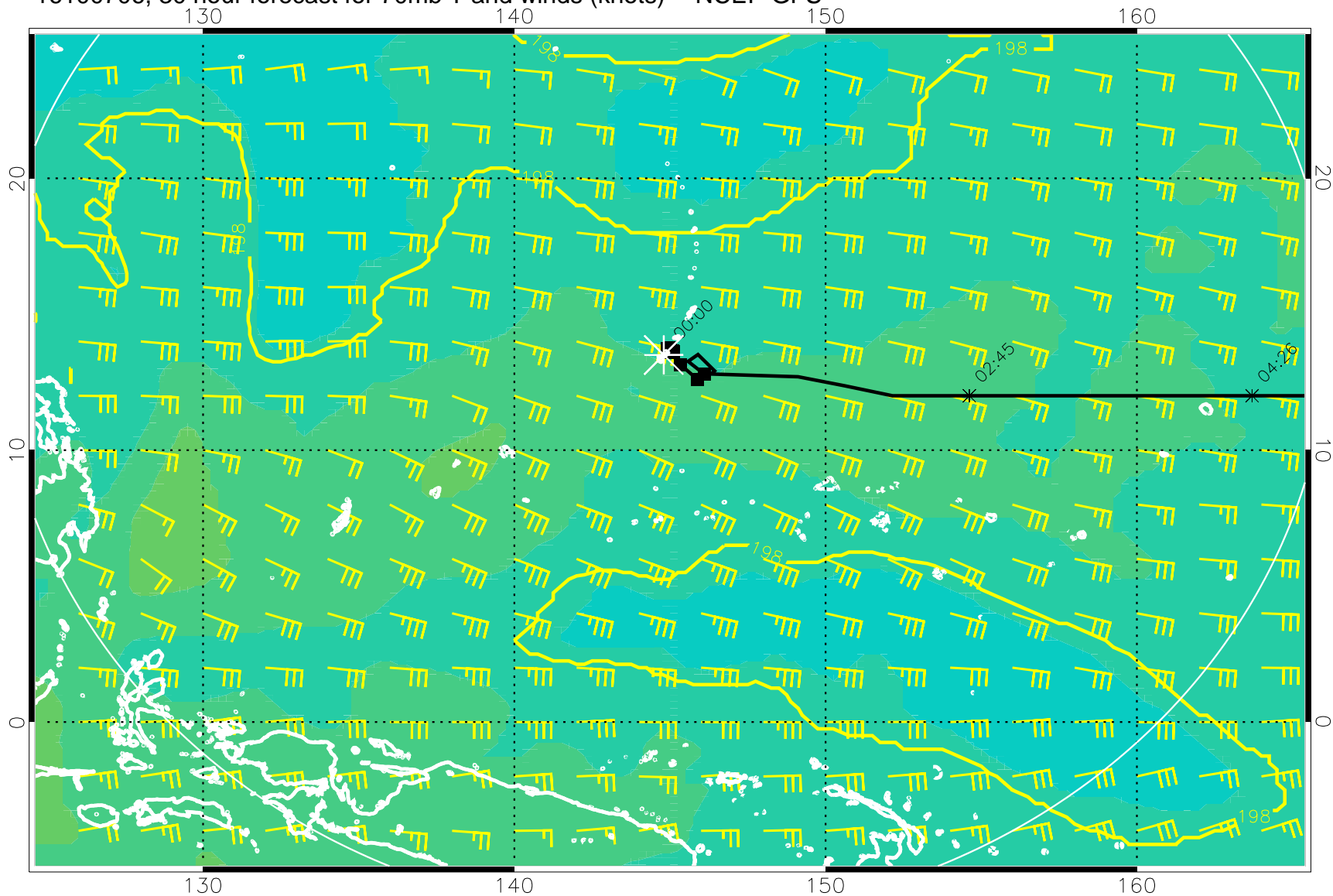
16100706, 30 hour forecast for 70mb T and winds (knots) -- NCEP GFS
