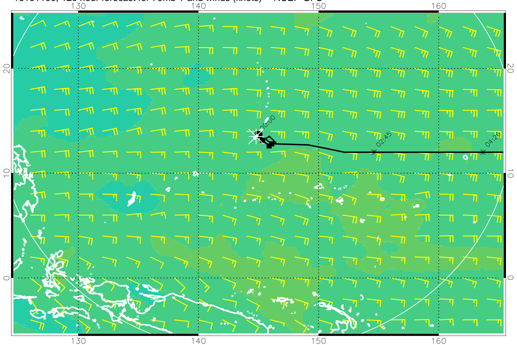
16101100, 120 hour forecast for 70mb T and winds (knots) -- NCEP GFS
