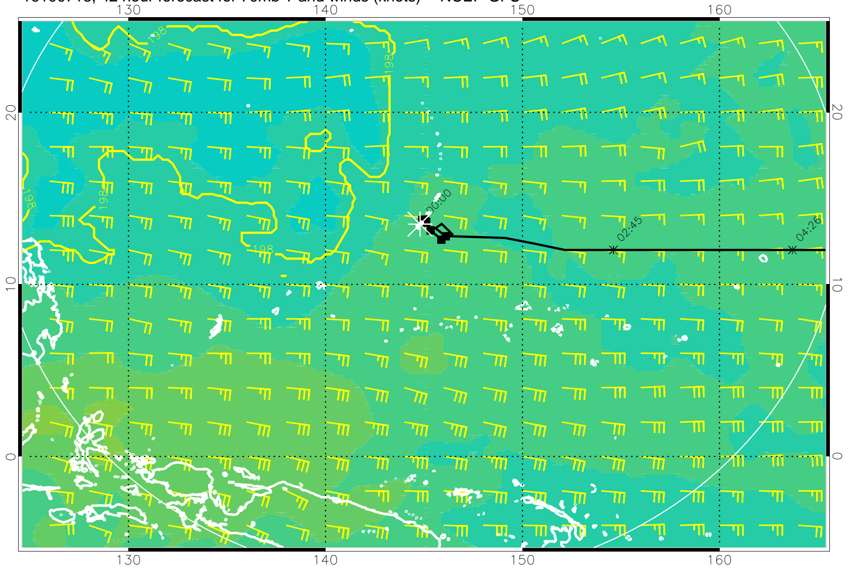
16100718, 42 hour forecast for 70mb T and winds (knots) -- NCEP GFS
