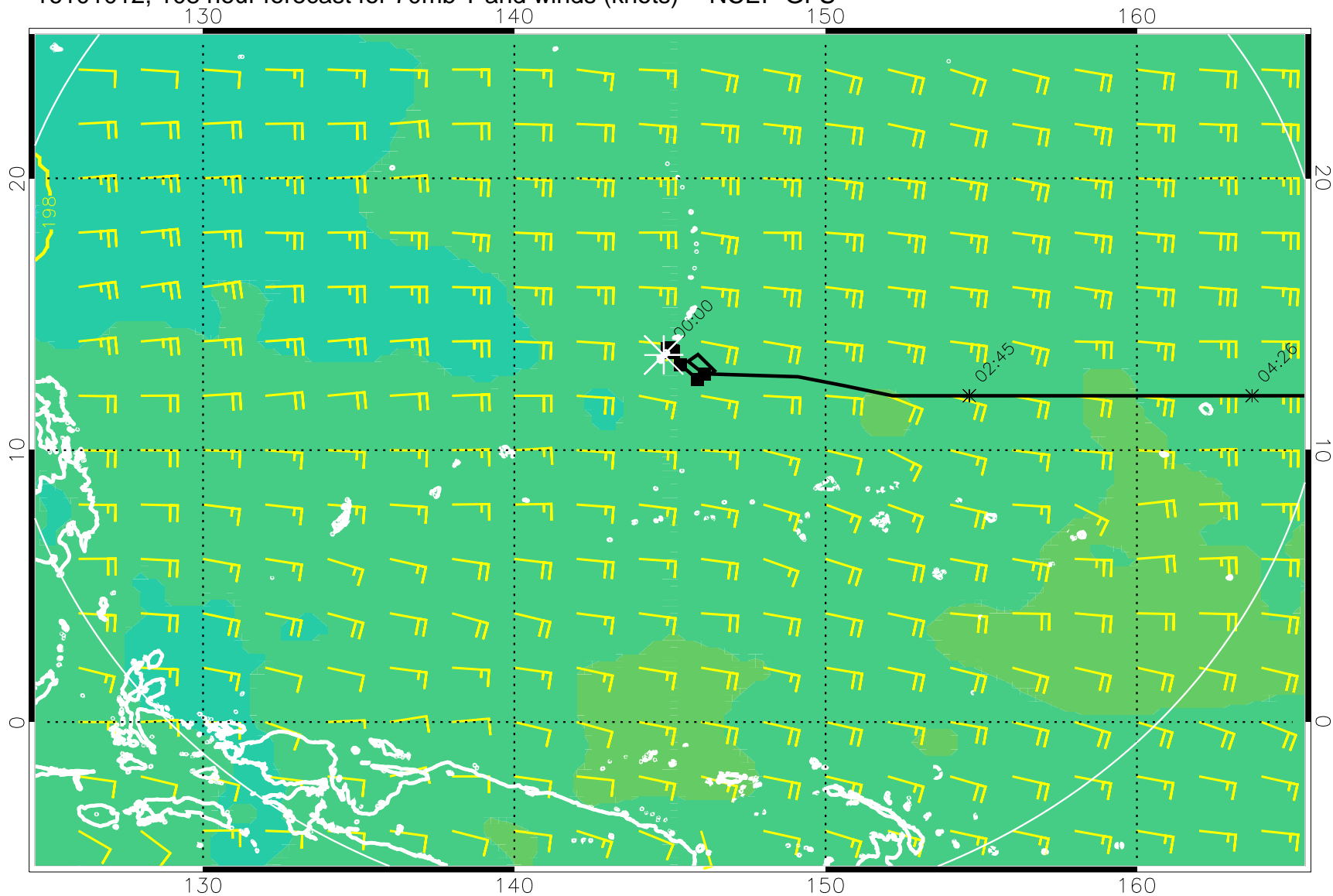
16101012, 108 hour forecast for 70mb T and winds (knots) -- NCEP GFS
