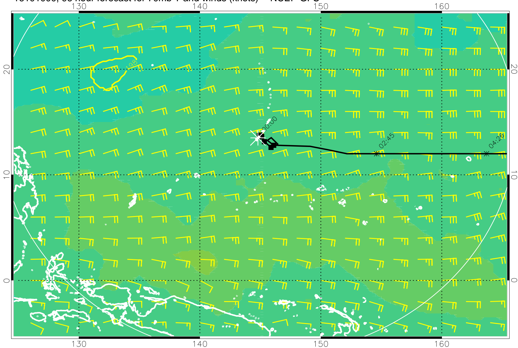
16101000, 96 hour forecast for 70mb T and winds (knots) -- NCEP GFS
