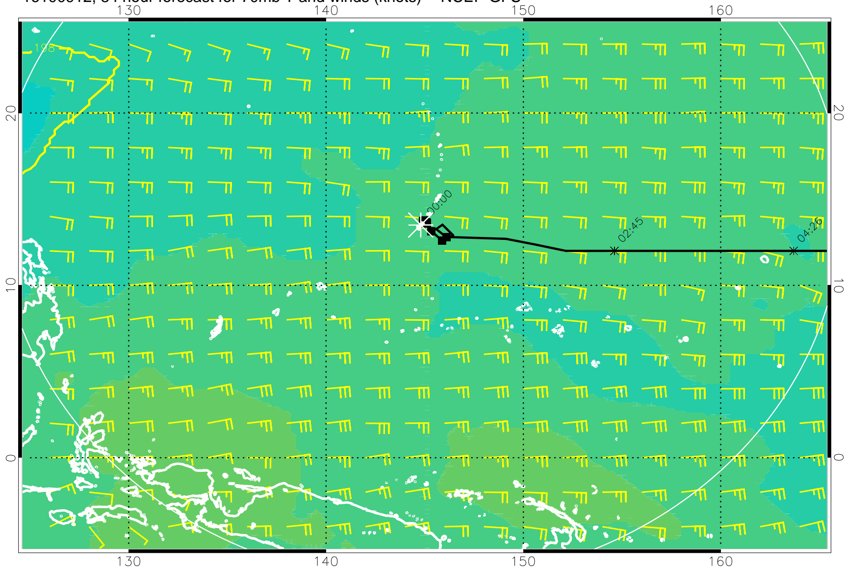
16100912, 84 hour forecast for 70mb T and winds (knots) -- NCEP GFS
