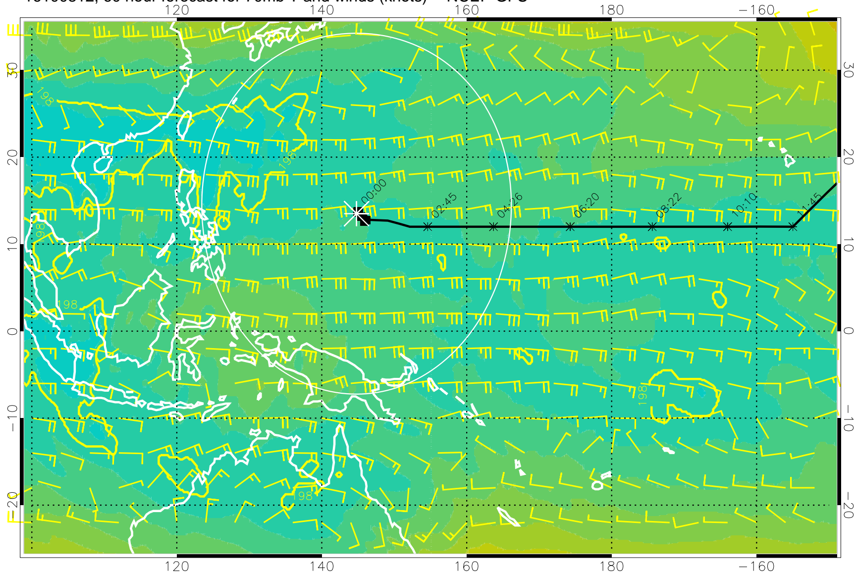
16100812, 60 hour forecast for 70mb T and winds (knots) -- NCEP GFS
