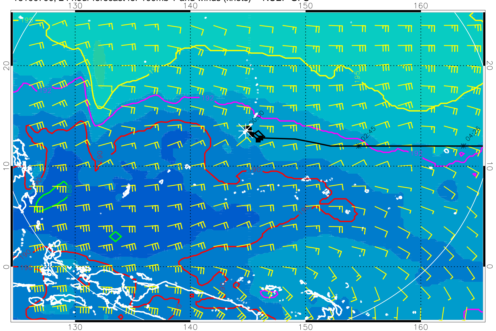
16100700, 24 hour forecast for 100mb T and winds (knots) -- NCEP GFS
