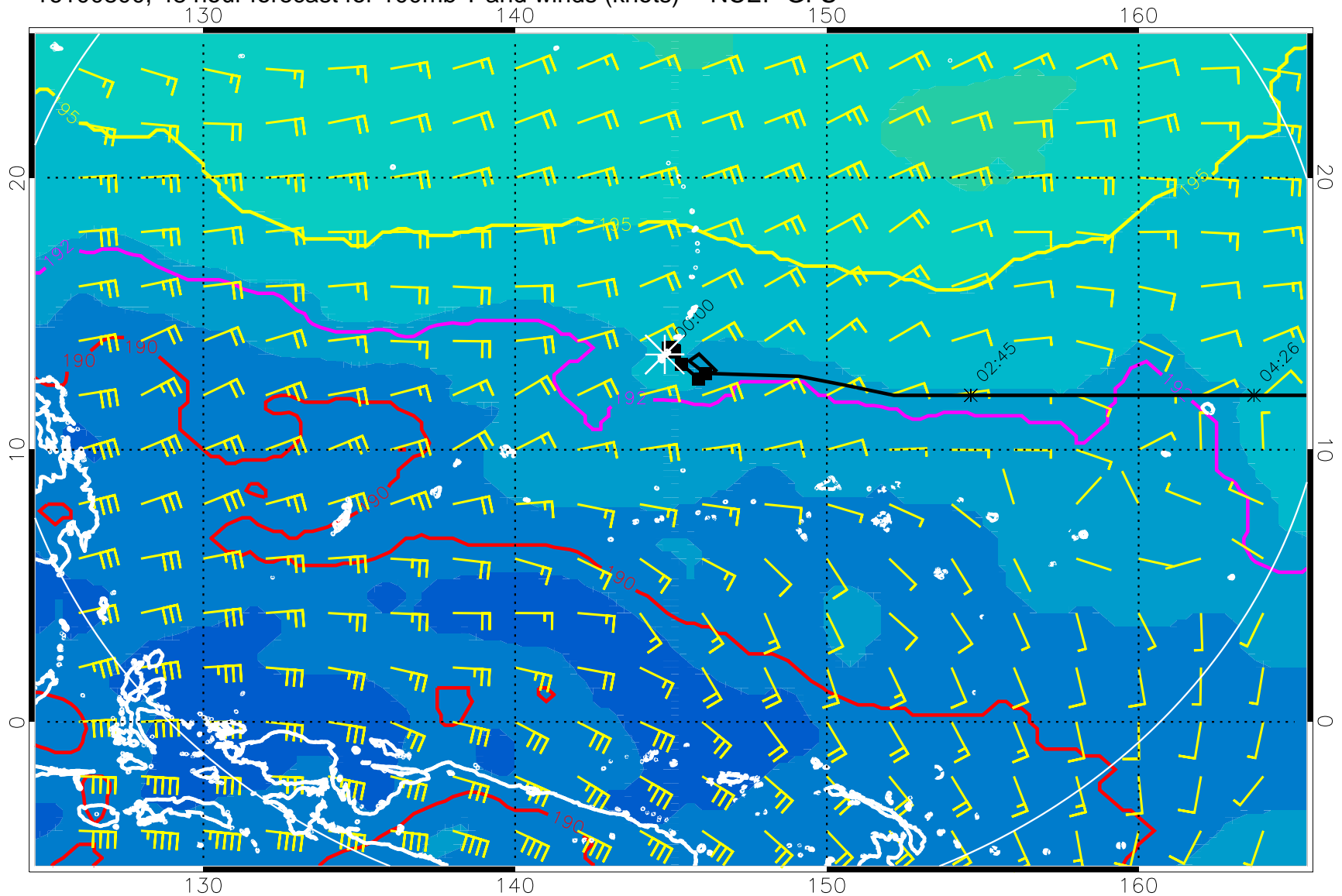
16100800, 48 hour forecast for 100mb T and winds (knots) -- NCEP GFS
