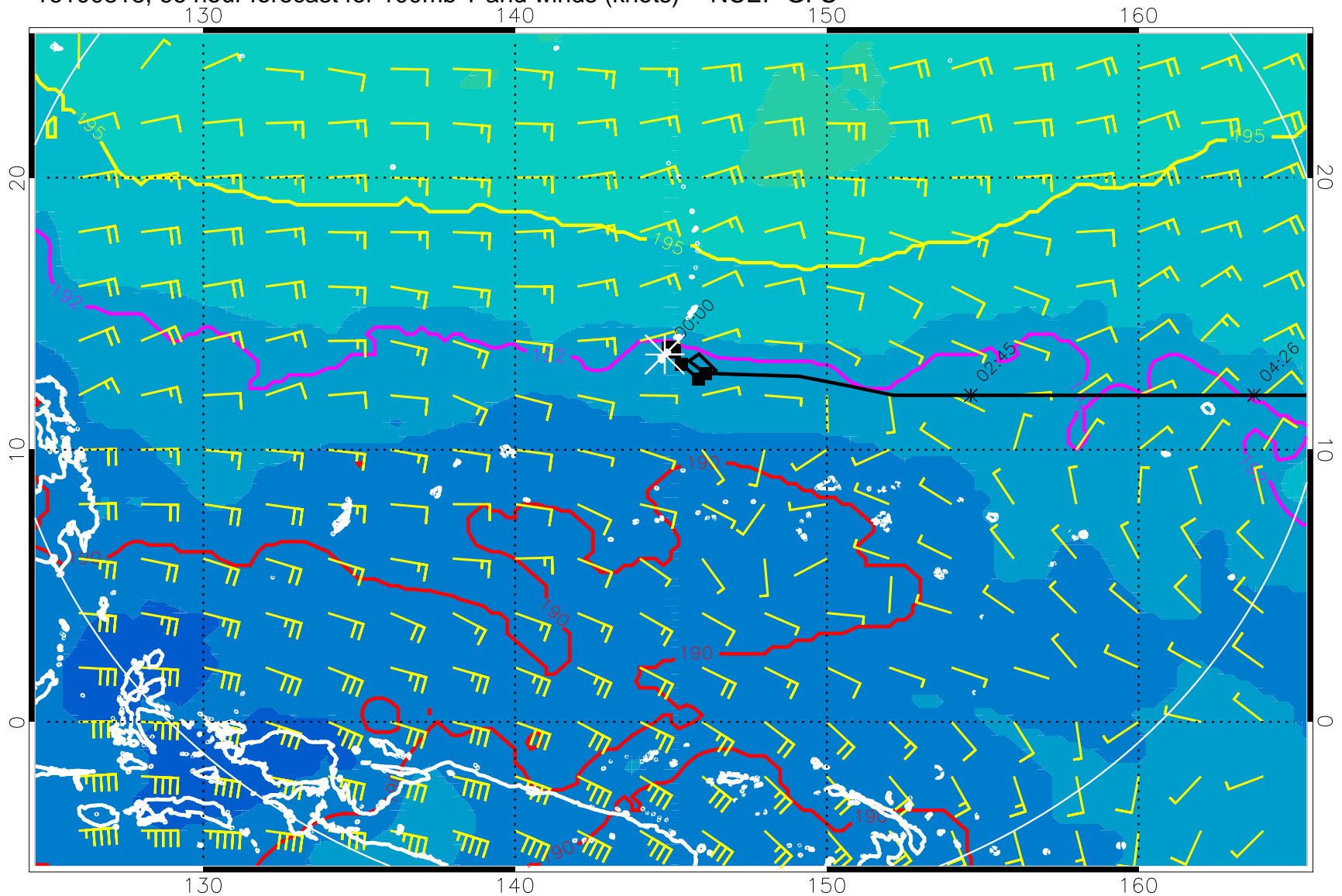
16100818, 66 hour forecast for 100mb T and winds (knots) -- NCEP GFS
