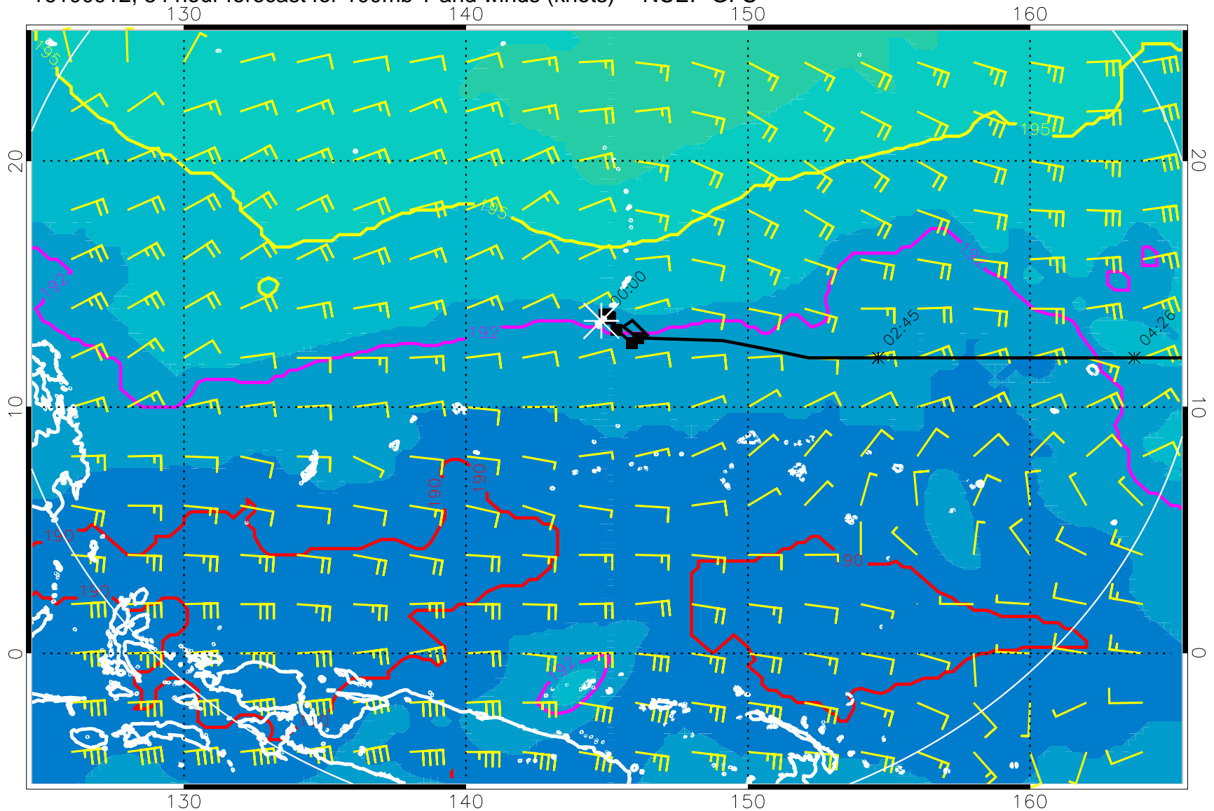
16100912, 84 hour forecast for 100mb T and winds (knots) -- NCEP GFS
