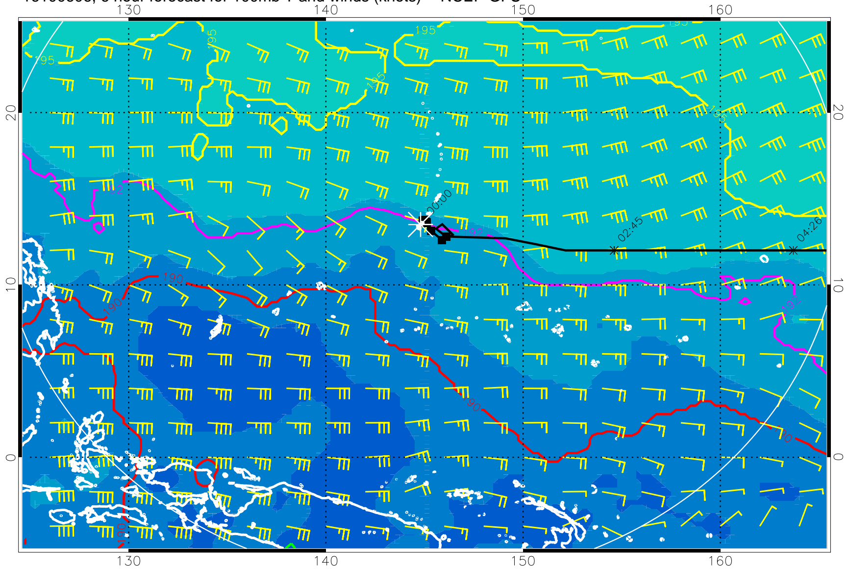
16100606, 6 hour forecast for 100mb T and winds (knots) -- NCEP GFS
