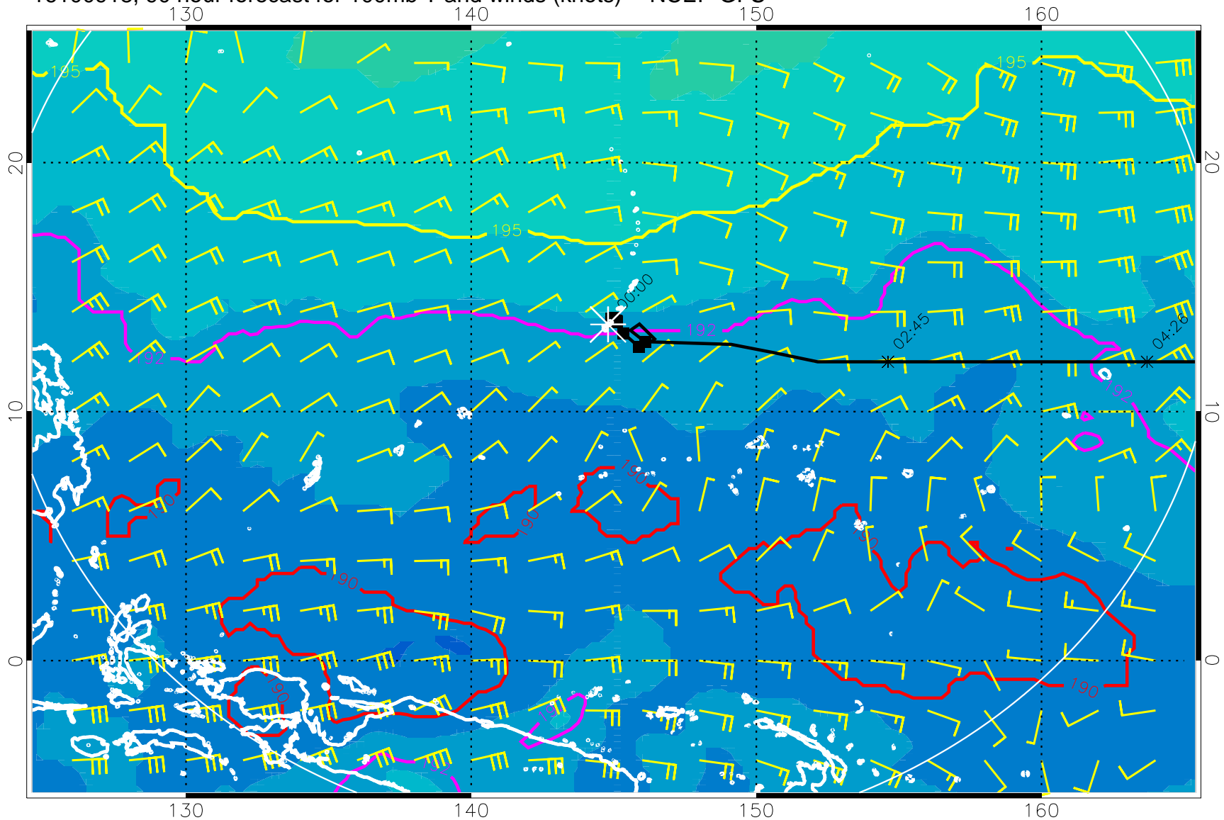
16100918, 90 hour forecast for 100mb T and winds (knots) -- NCEP GFS
