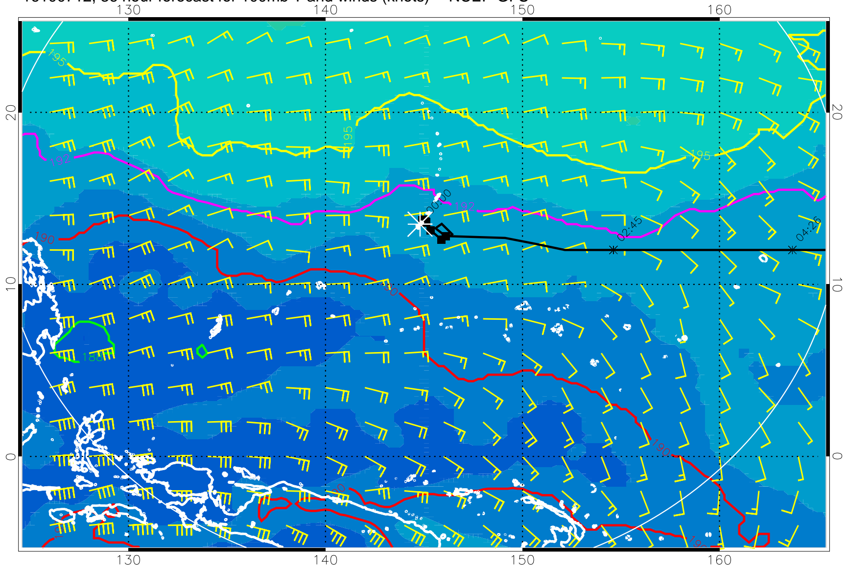
16100712, 36 hour forecast for 100mb T and winds (knots) -- NCEP GFS
