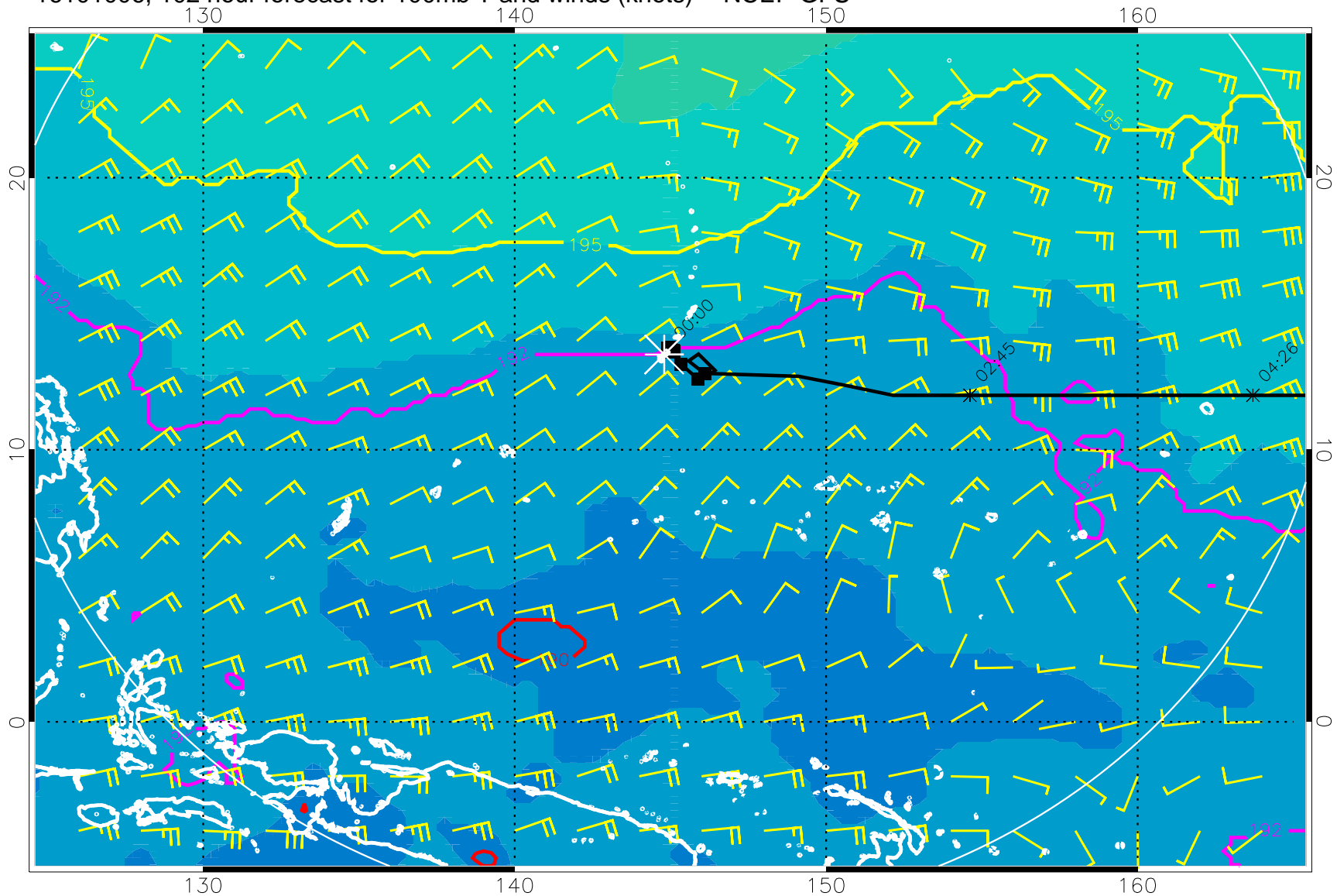
16101006, 102 hour forecast for 100mb T and winds (knots) -- NCEP GFS
