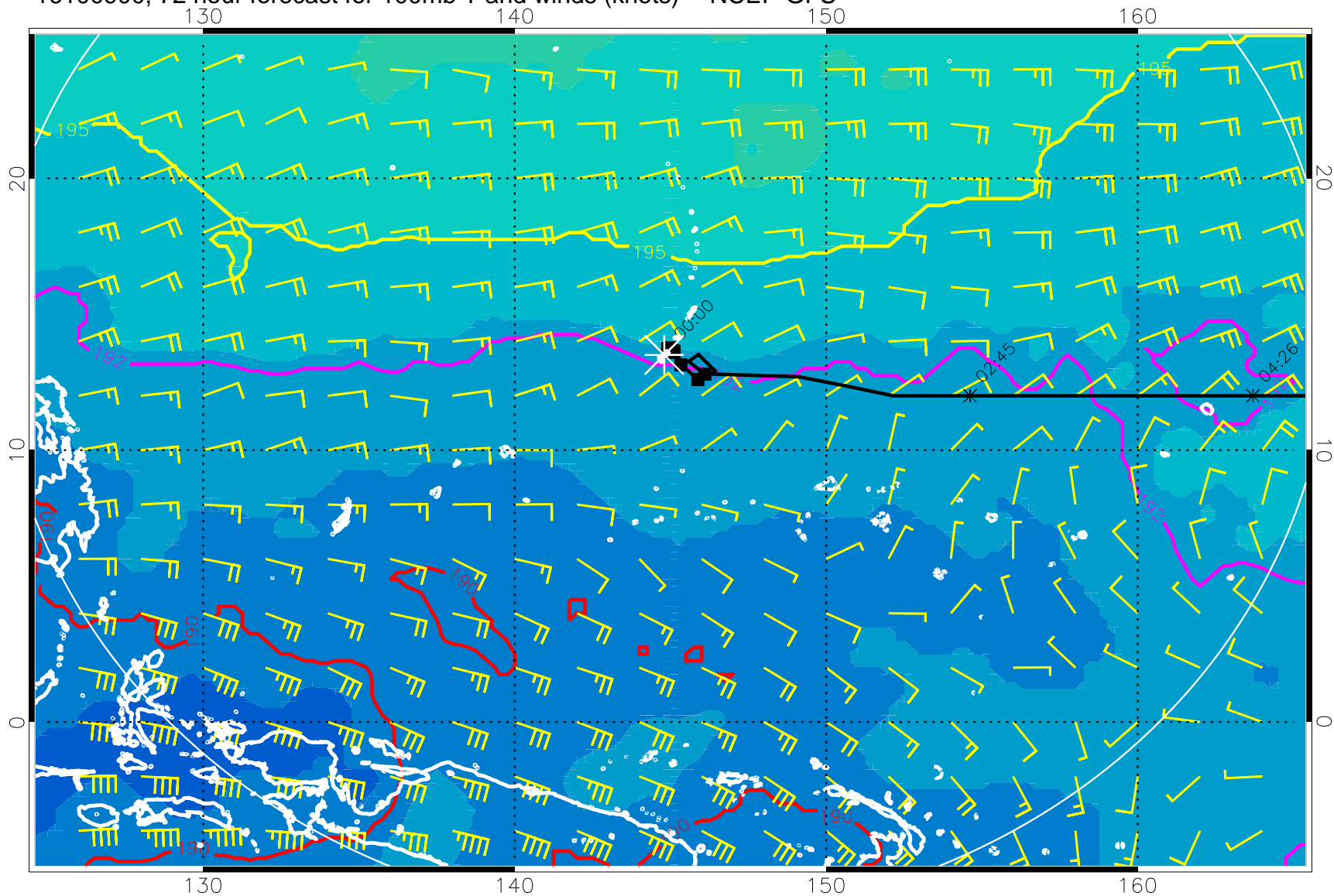
16100900, 72 hour forecast for 100mb T and winds (knots) -- NCEP GFS
