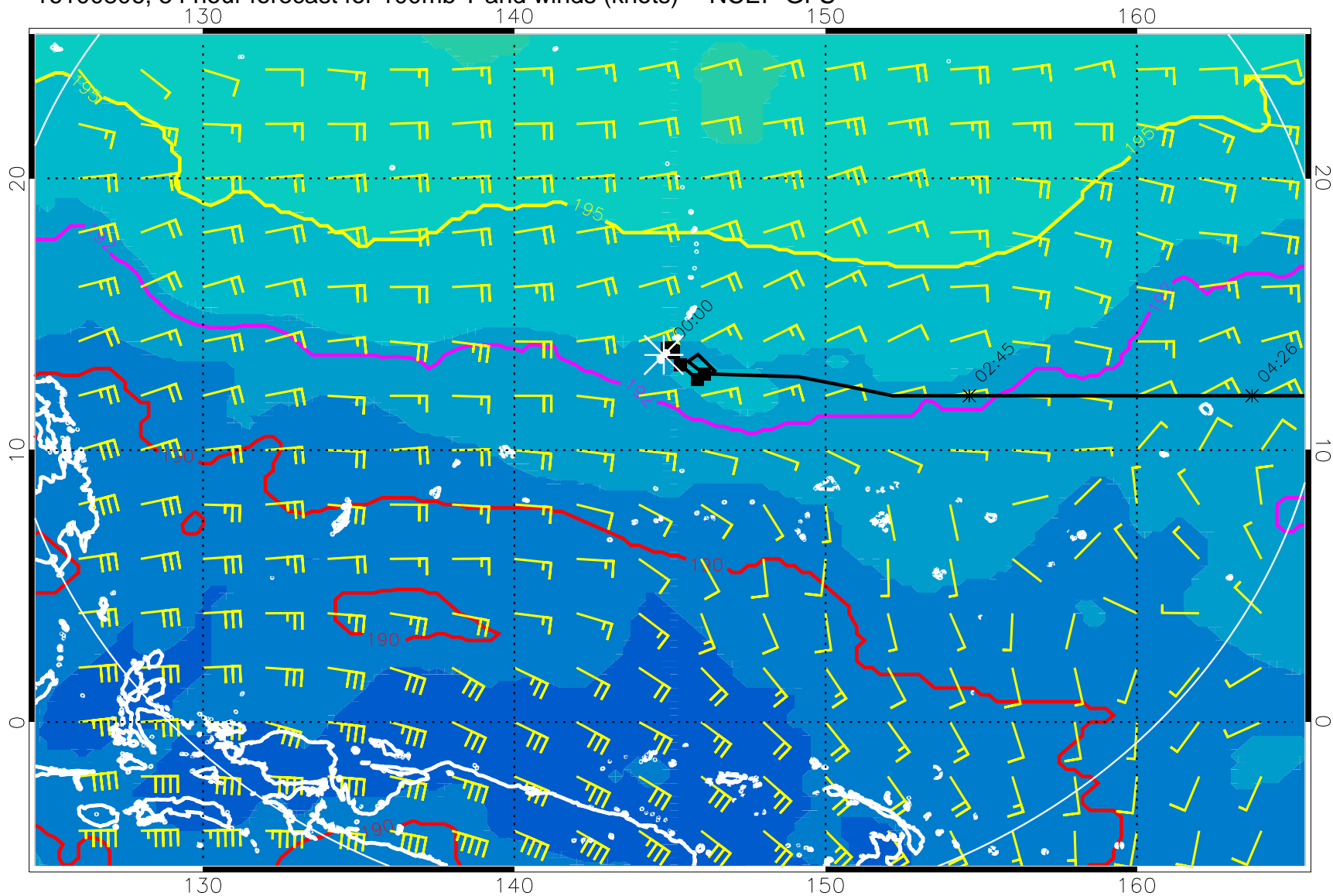
16100806, 54 hour forecast for 100mb T and winds (knots) -- NCEP GFS
