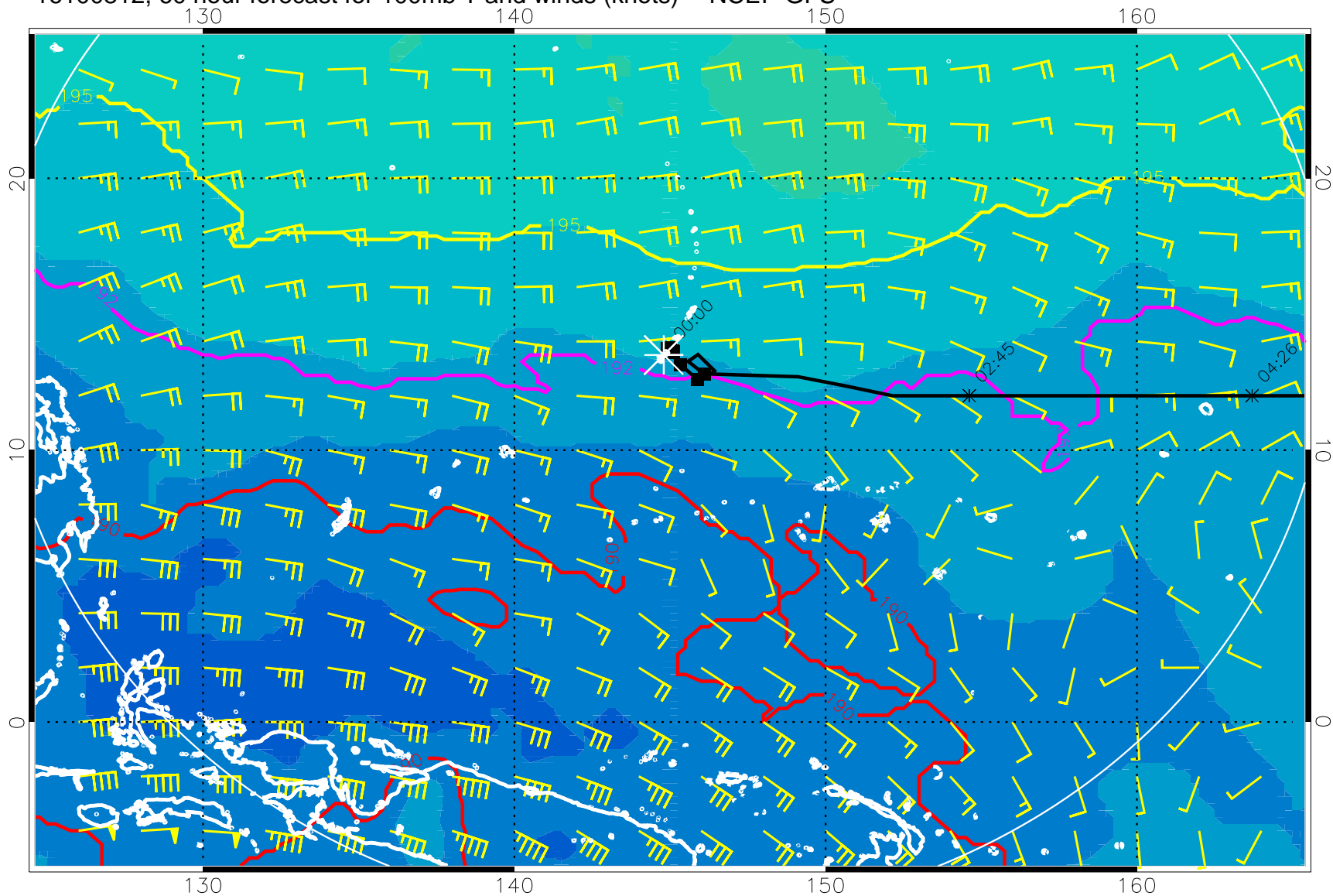
16100812, 60 hour forecast for 100mb T and winds (knots) -- NCEP GFS
