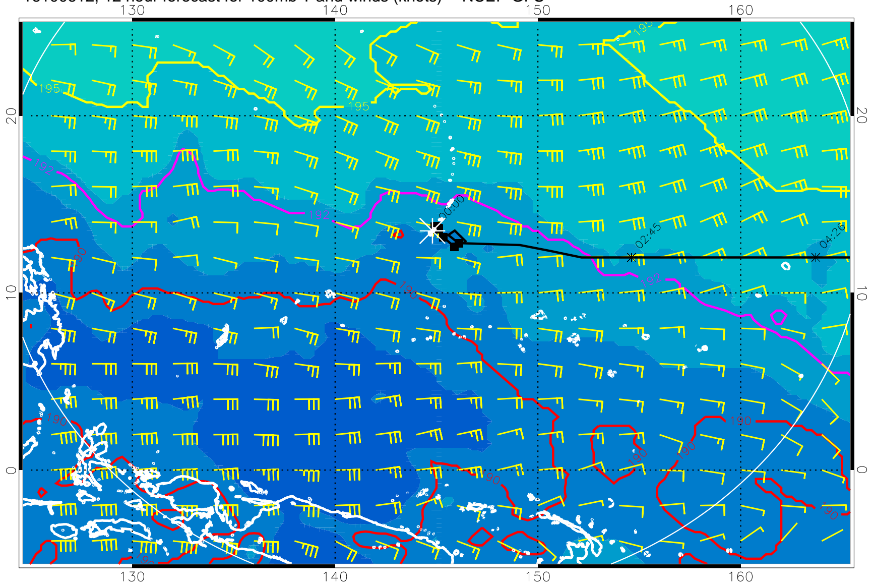
16100612, 12 hour forecast for 100mb T and winds (knots) -- NCEP GFS
