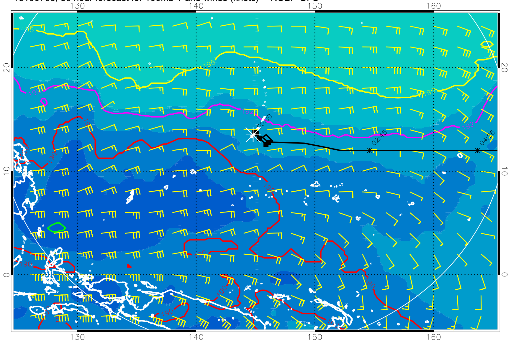
16100706, 30 hour forecast for 100mb T and winds (knots) -- NCEP GFS
