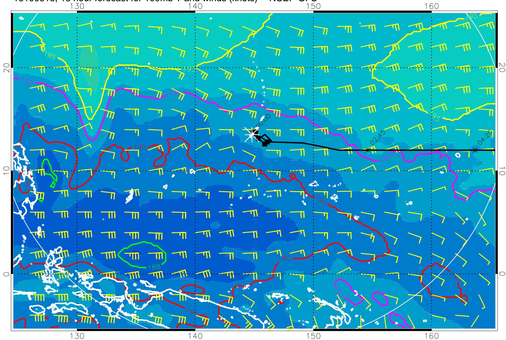
16100618, 18 hour forecast for 100mb T and winds (knots) -- NCEP GFS
