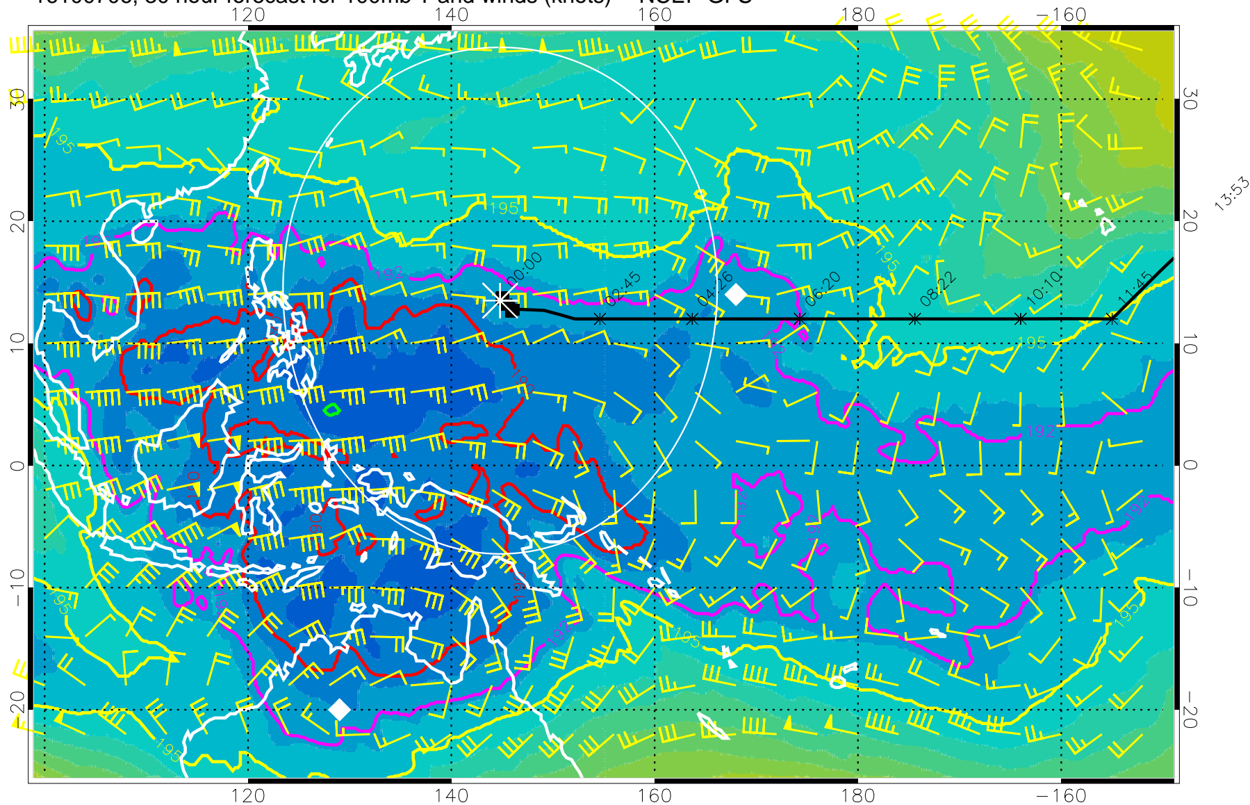
16100706, 30 hour forecast for 100mb T and winds (knots) -- NCEP GFS
