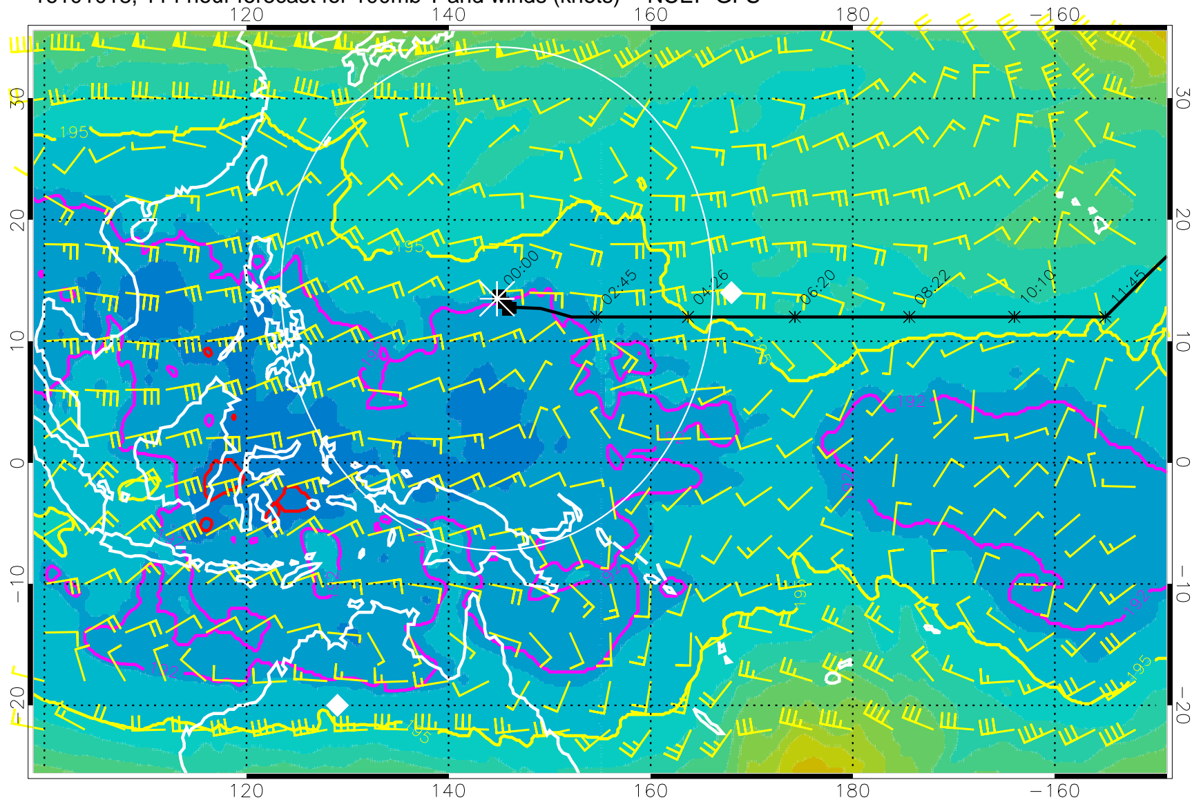
16101018, 114 hour forecast for 100mb T and winds (knots) -- NCEP GFS
