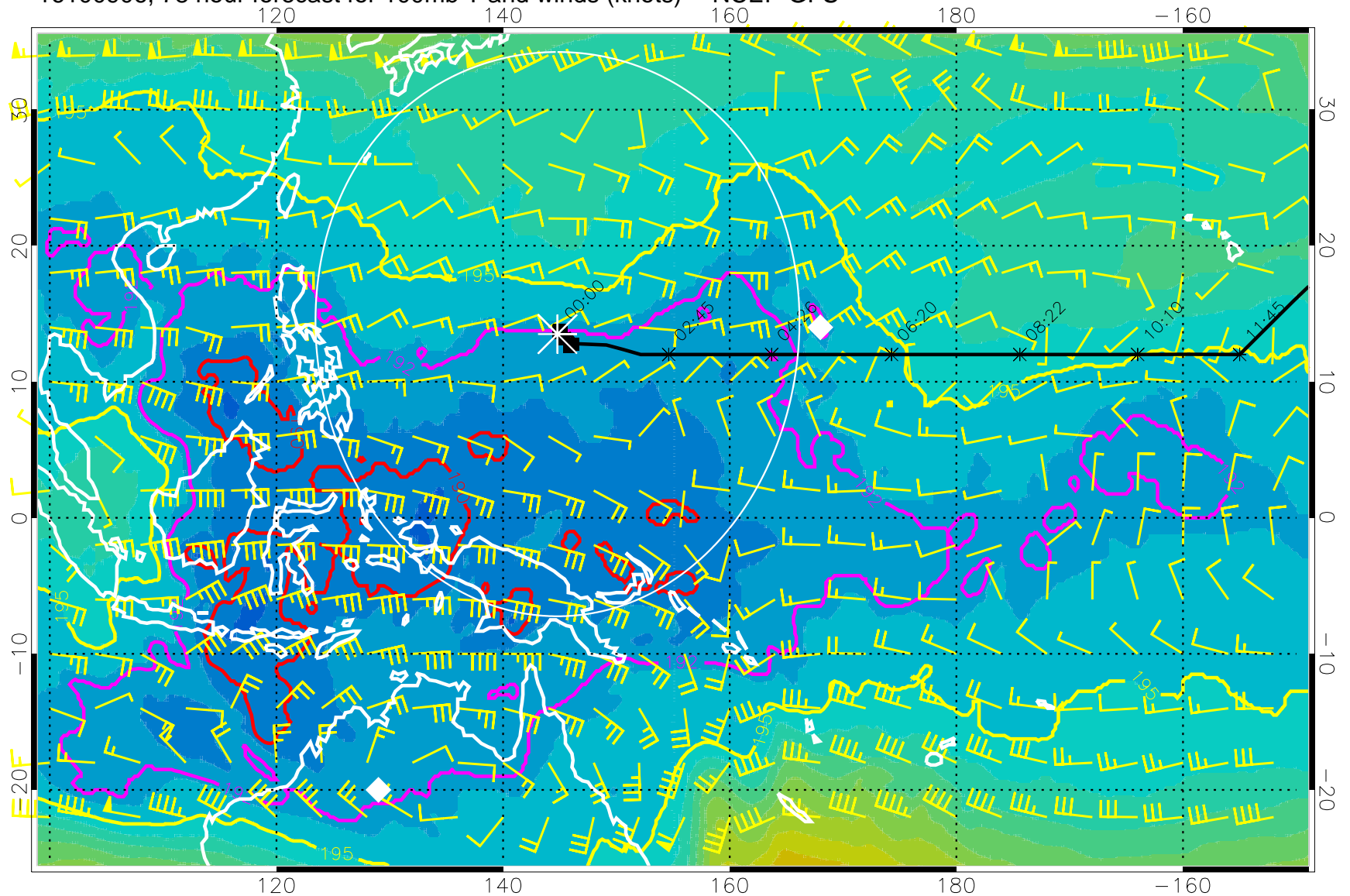
16100906, 78 hour forecast for 100mb T and winds (knots) -- NCEP GFS
