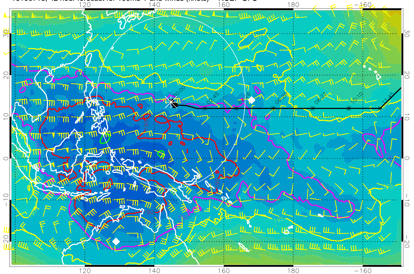
16100718, 42 hour forecast for 100mb T and winds (knots) -- NCEP GFS
