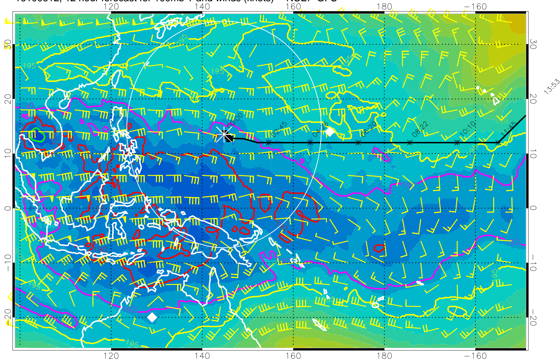
16100612, 12 hour forecast for 100mb T and winds (knots) -- NCEP GFS
