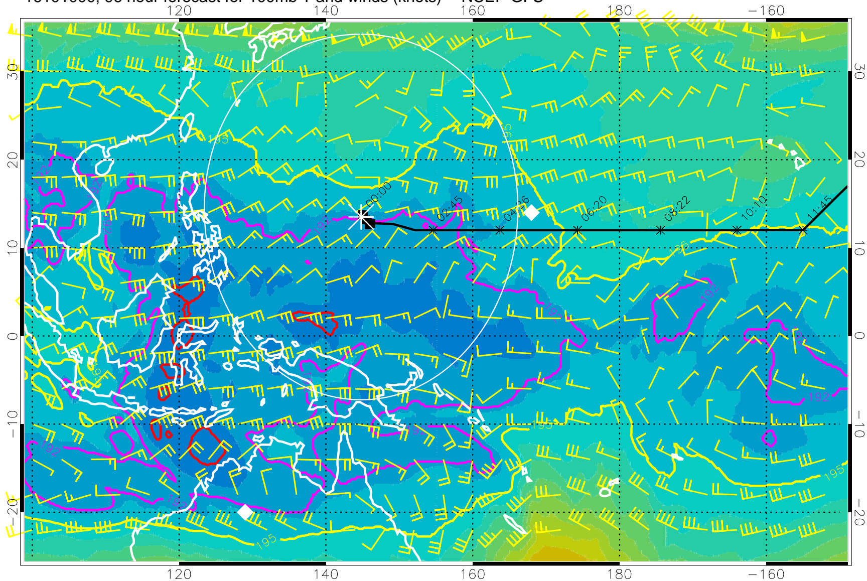
16101000, 96 hour forecast for 100mb T and winds (knots) -- NCEP GFS
