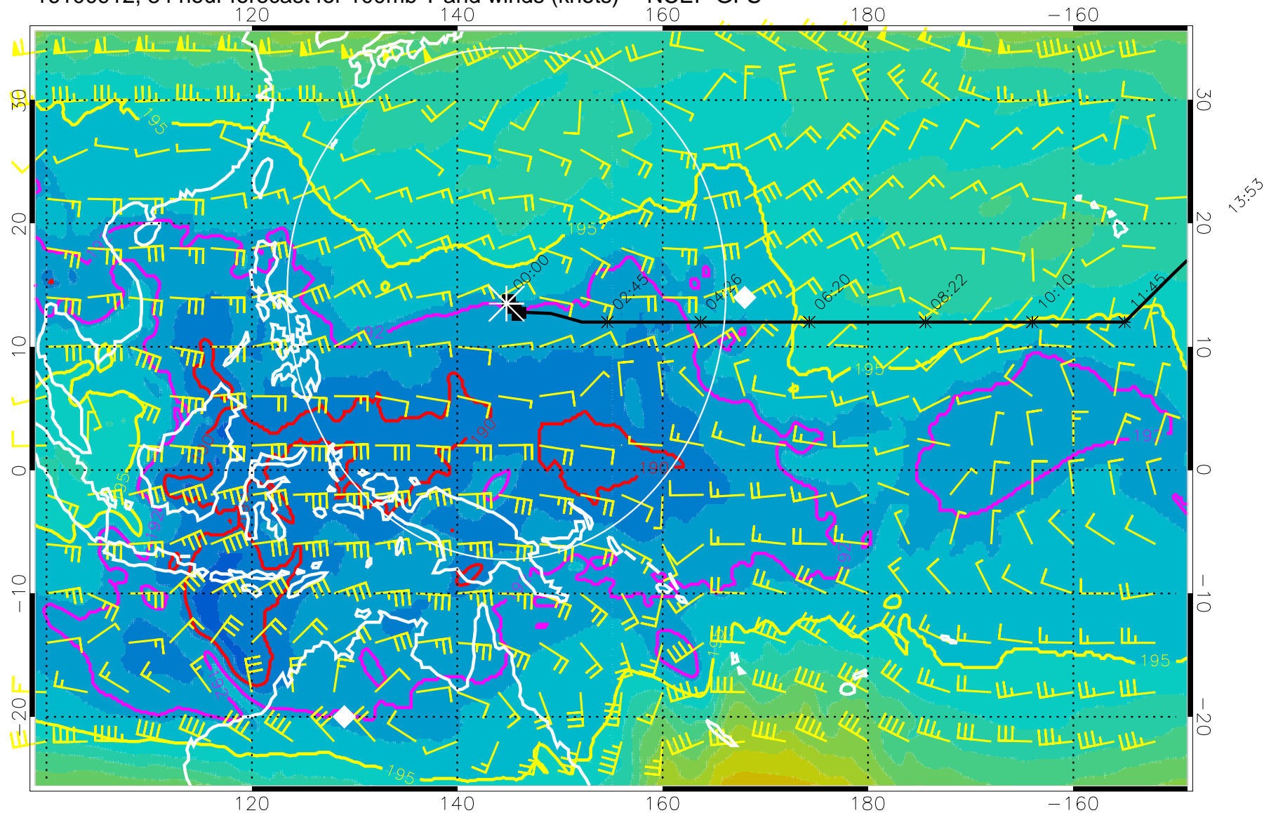
16100912, 84 hour forecast for 100mb T and winds (knots) -- NCEP GFS
