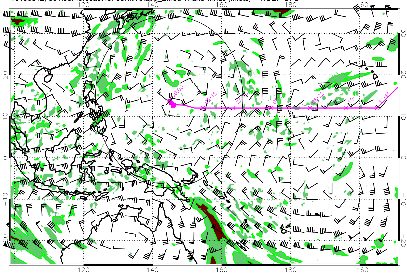
16100812, 60 hour forecast for 36Kft Knapp_Ellrod TI and winds (knots) -- NCEP GFS
