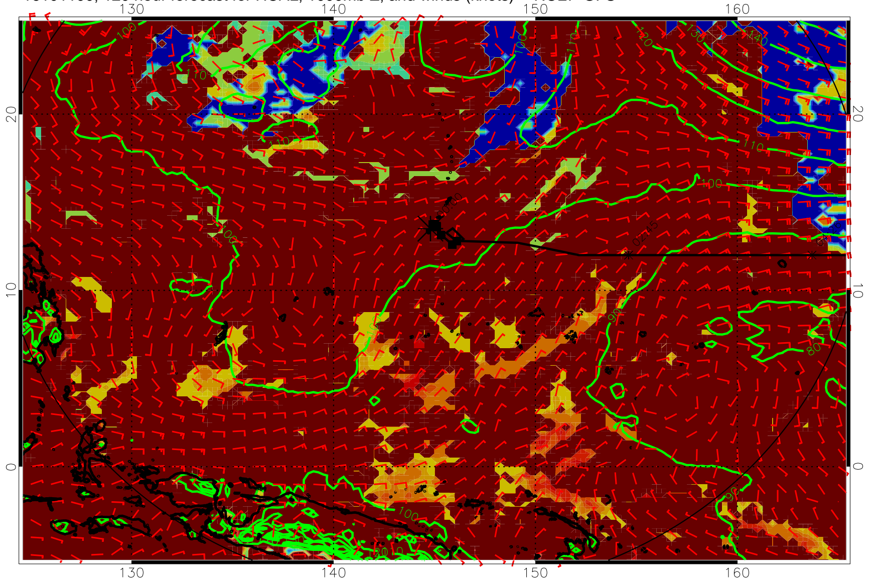
16101100, 120 hour forecast for HCAL, 1000mb Z, and winds (knots) -- NCEP GFS
