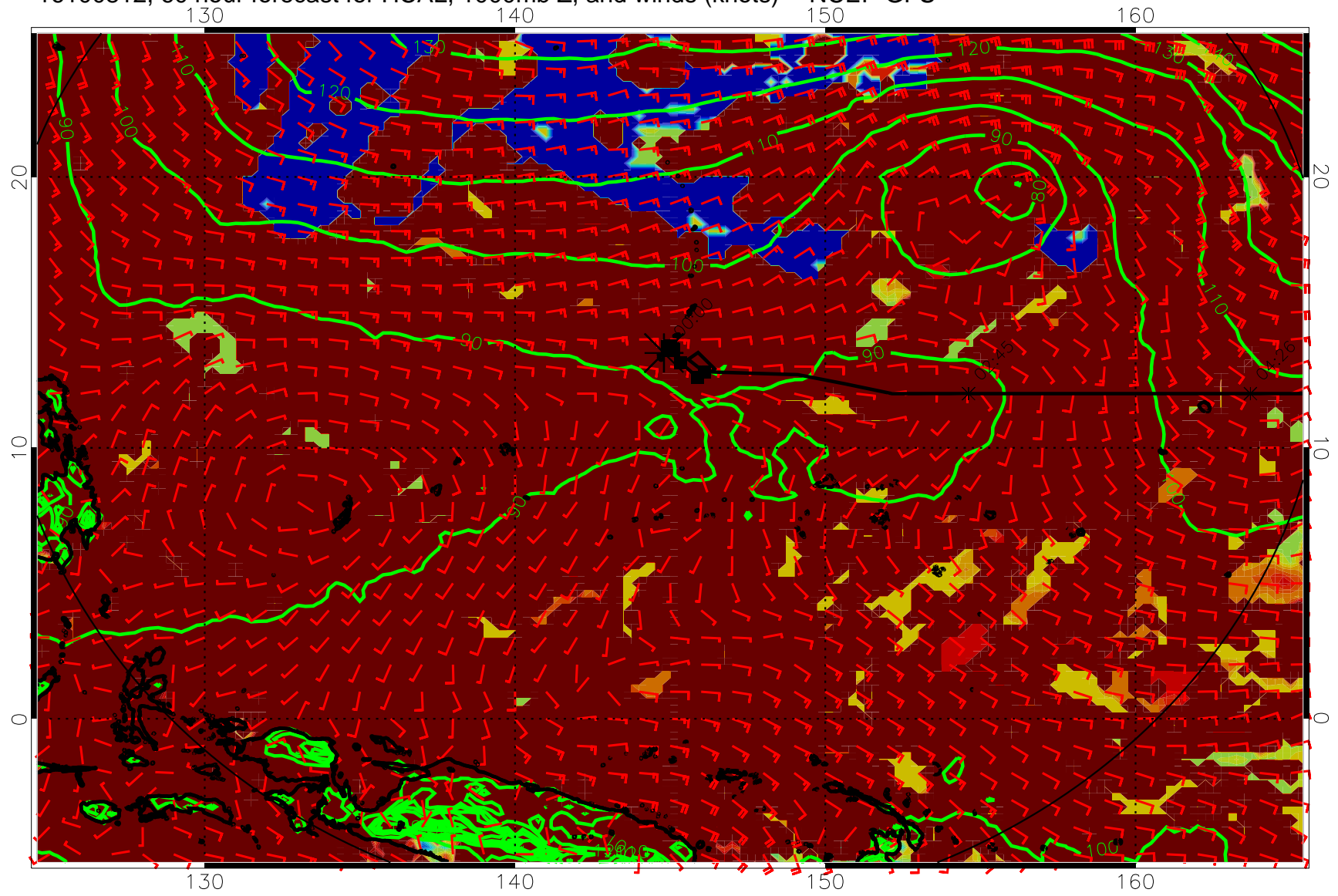
16100812, 60 hour forecast for HCAL, 1000mb Z, and winds (knots) -- NCEP GFS
