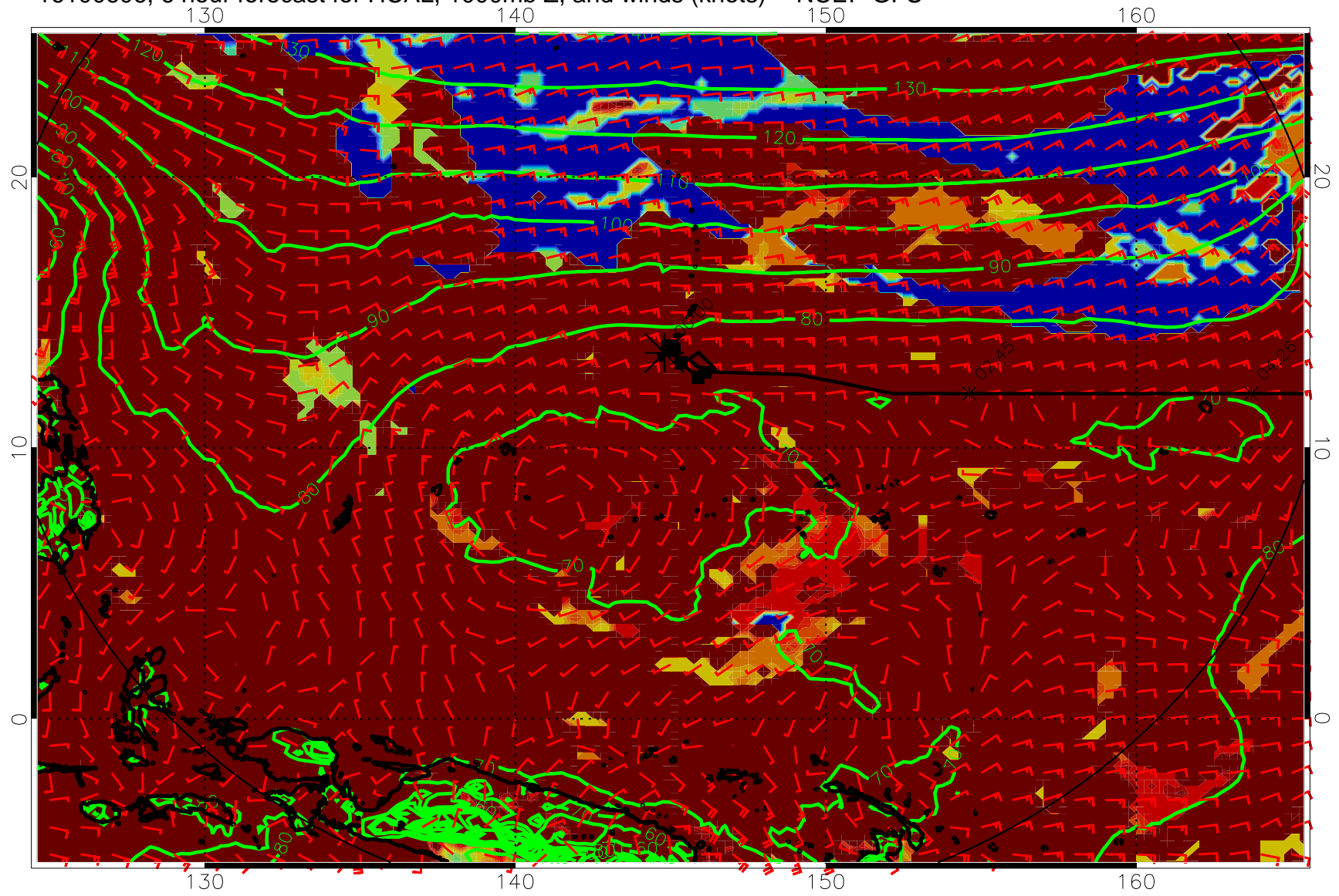
16100606, 6 hour forecast for HCAL, 1000mb Z, and winds (knots) -- NCEP GFS
