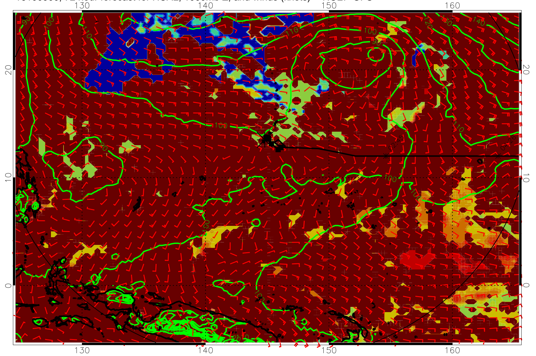
16100900, 72 hour forecast for HCAL, 1000mb Z, and winds (knots) -- NCEP GFS
