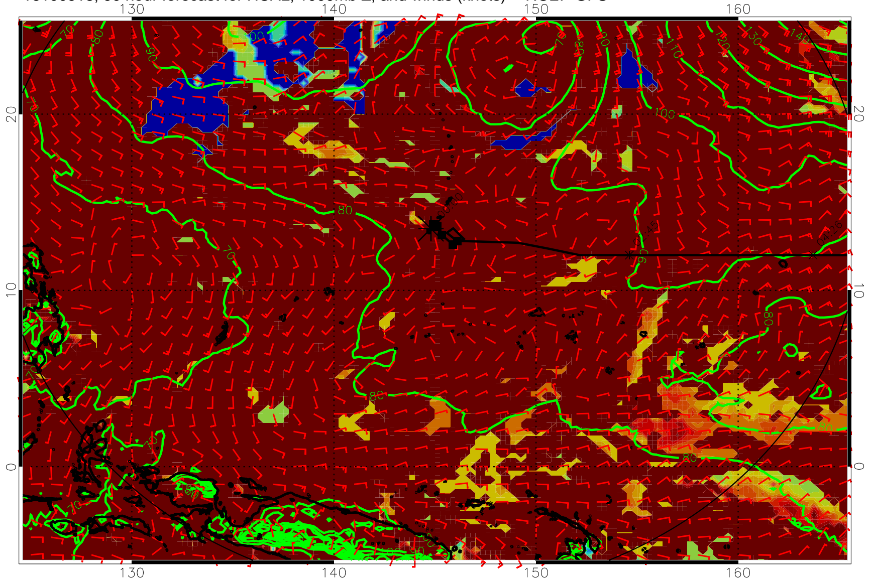
16100918, 90 hour forecast for HCAL, 1000mb Z, and winds (knots) -- NCEP GFS
