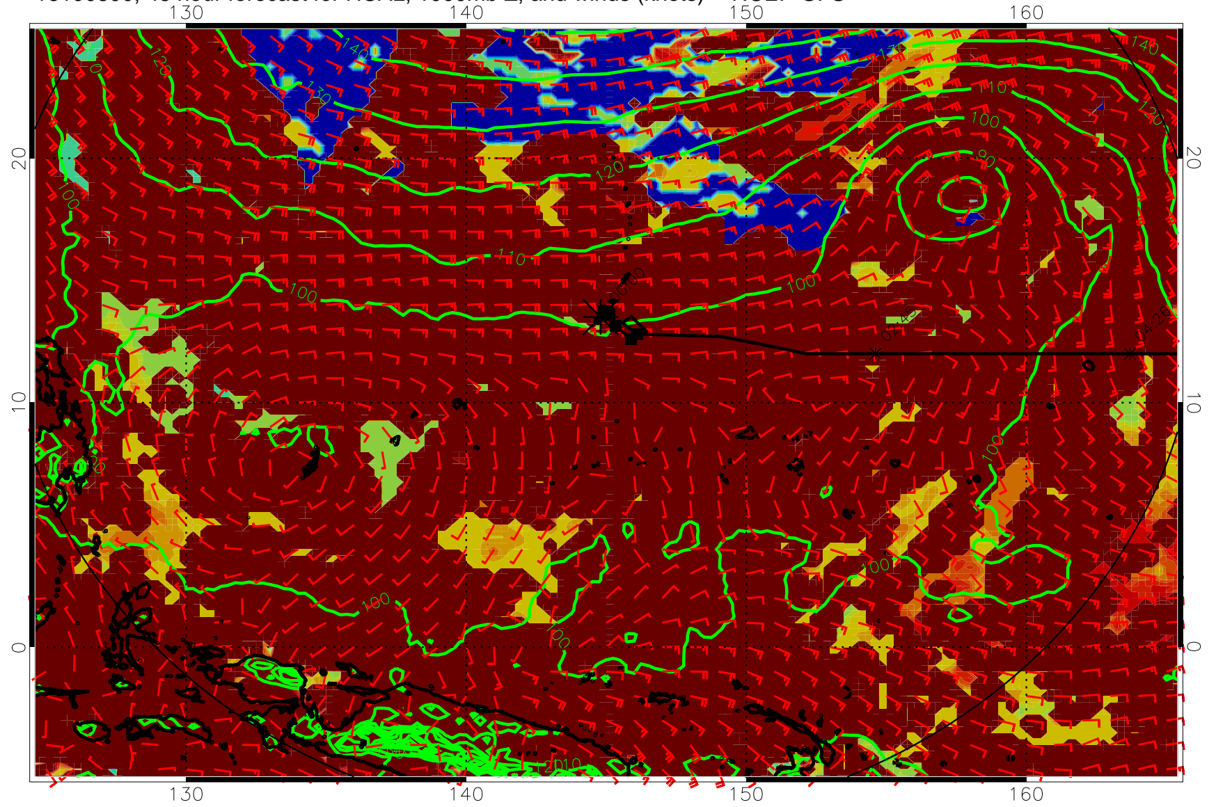
16100800, 48 hour forecast for HCAL, 1000mb Z, and winds (knots) -- NCEP GFS
