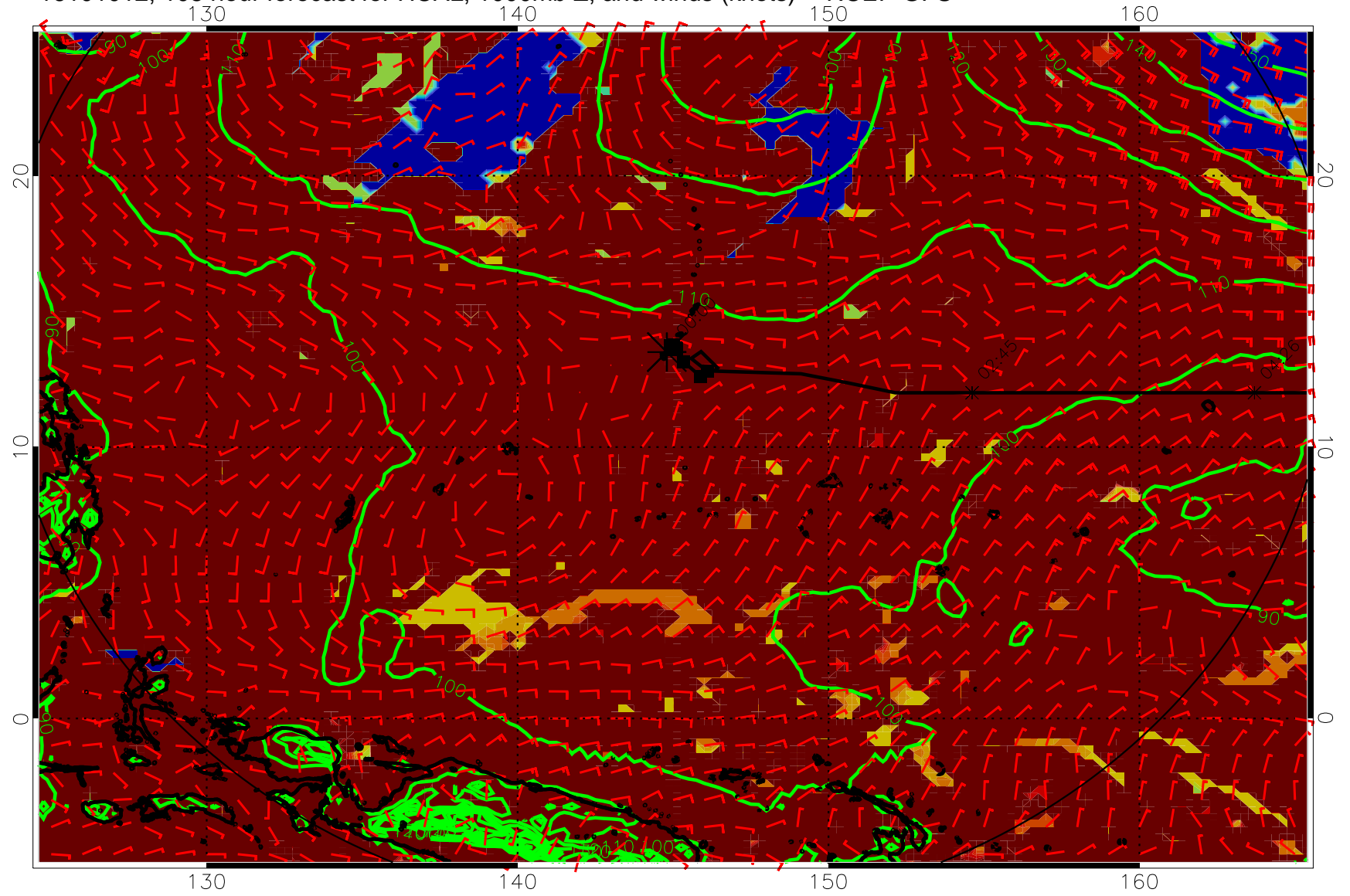
16101012, 108 hour forecast for HCAL, 1000mb Z, and winds (knots) -- NCEP GFS
