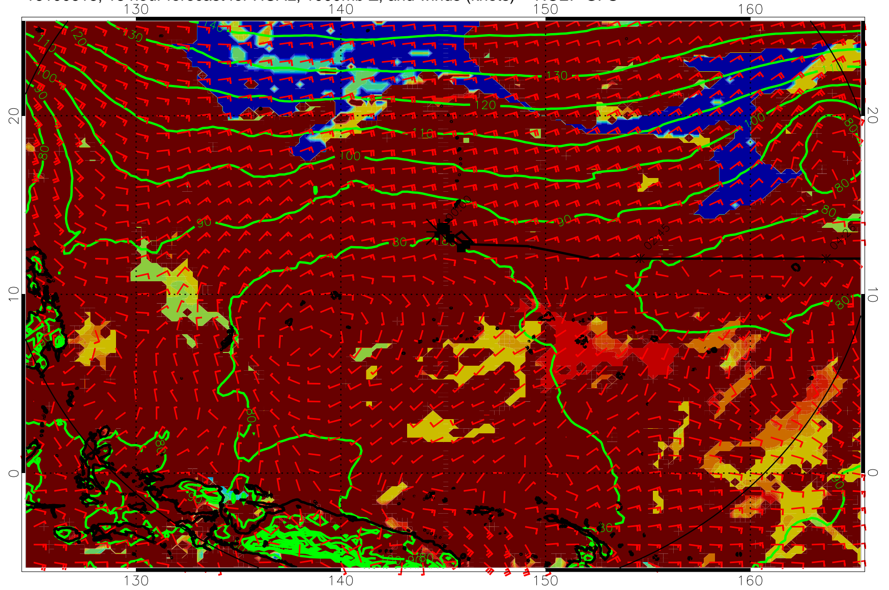
16100618, 18 hour forecast for HCAL, 1000mb Z, and winds (knots) -- NCEP GFS
