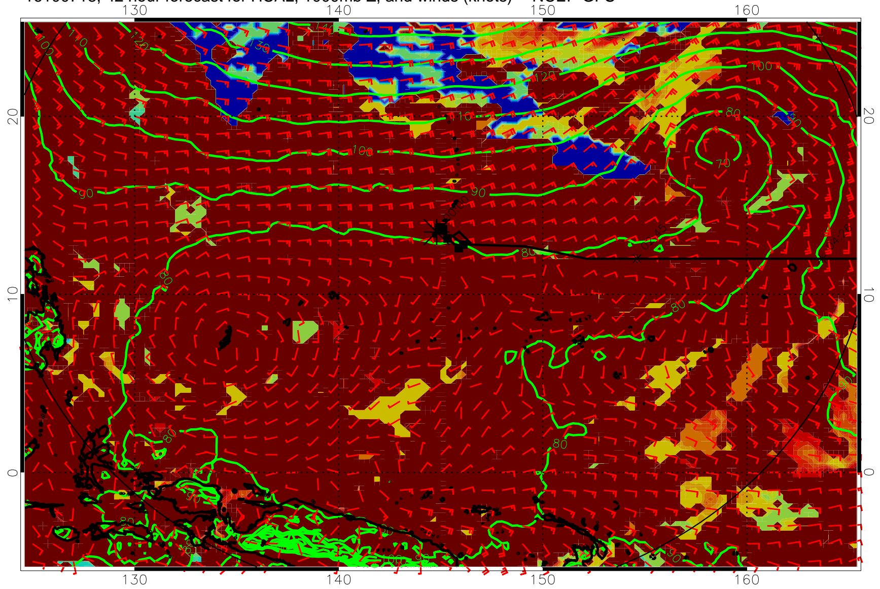
16100718, 42 hour forecast for HCAL, 1000mb Z, and winds (knots) -- NCEP GFS
