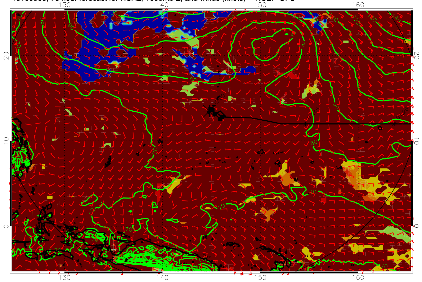
16100906, 78 hour forecast for HCAL, 1000mb Z, and winds (knots) -- NCEP GFS
