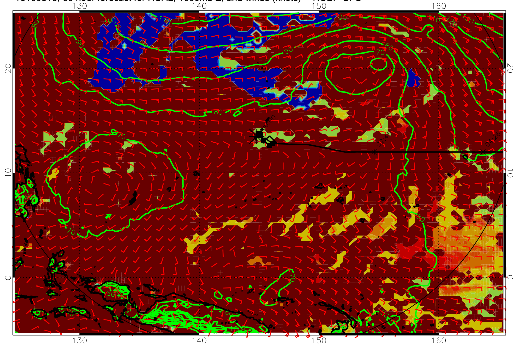
16100818, 66 hour forecast for HCAL, 1000mb Z, and winds (knots) -- NCEP GFS
