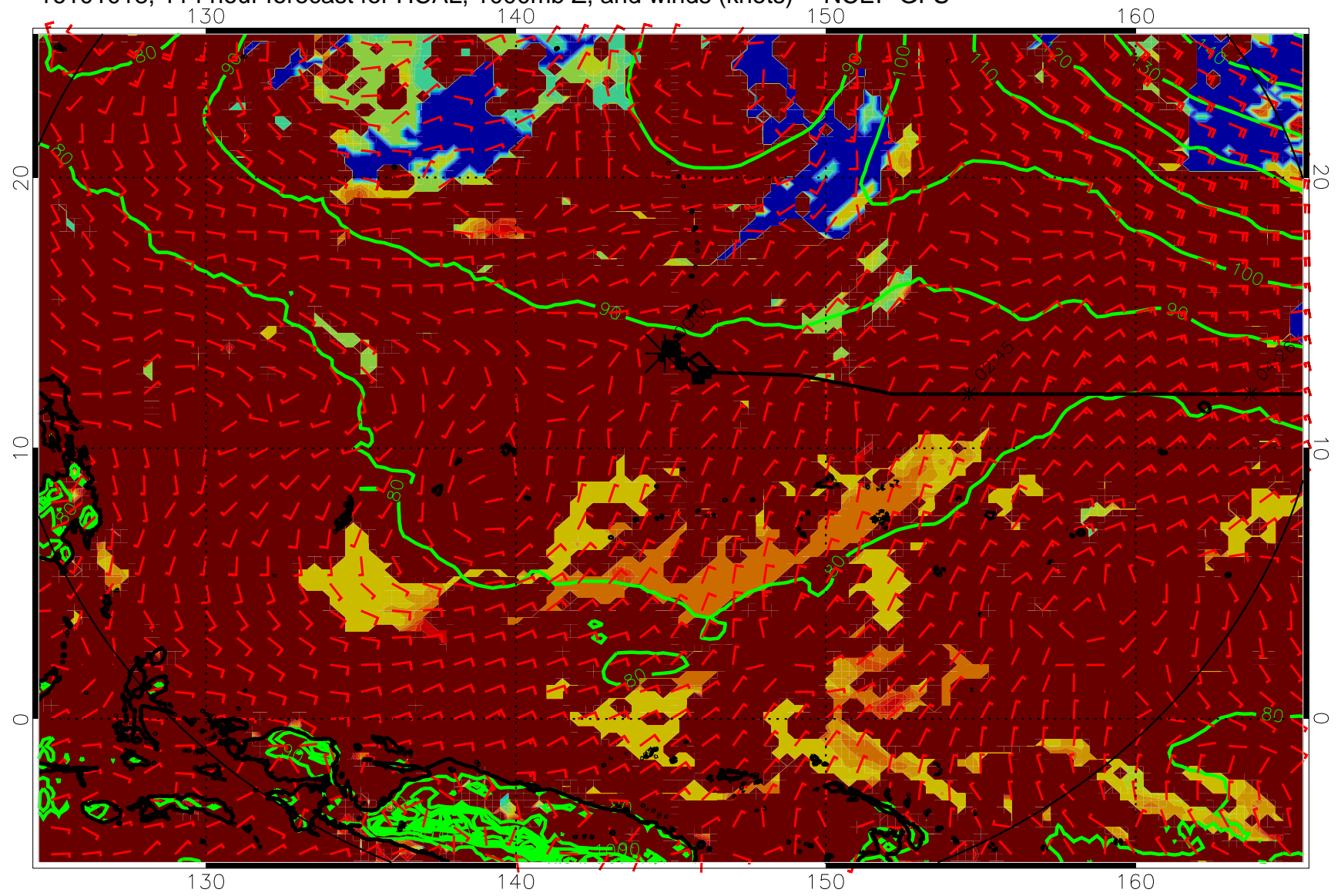
16101018, 114 hour forecast for HCAL, 1000mb Z, and winds (knots) -- NCEP GFS
