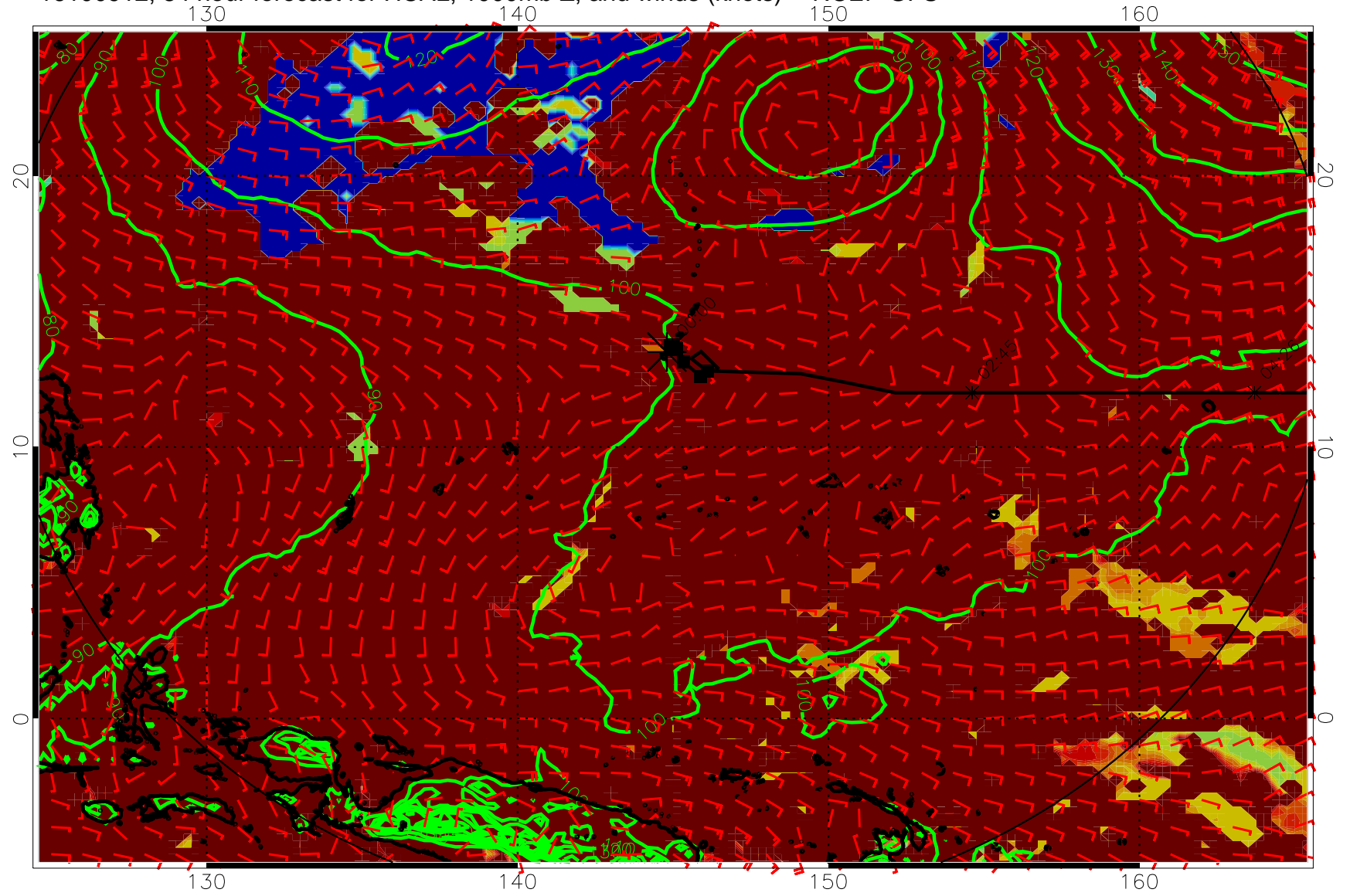
16100912, 84 hour forecast for HCAL, 1000mb Z, and winds (knots) -- NCEP GFS
