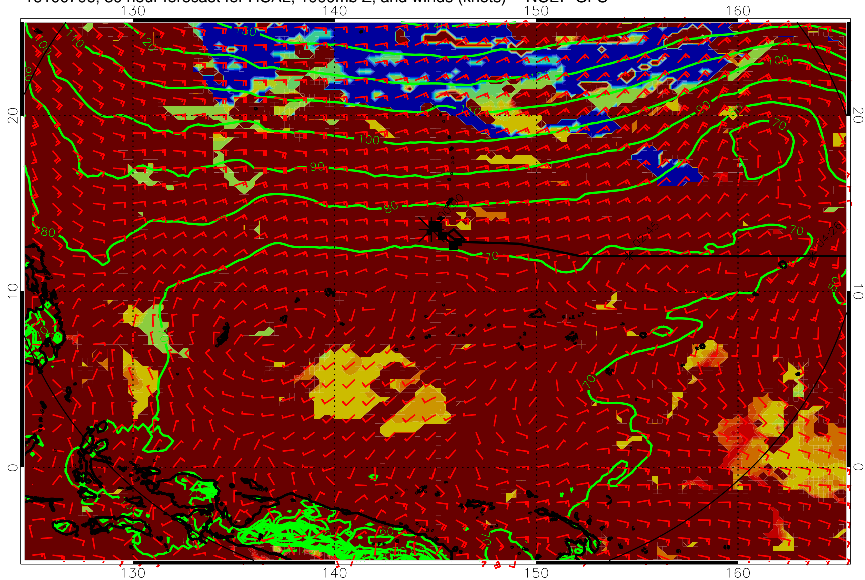
16100706, 30 hour forecast for HCAL, 1000mb Z, and winds (knots) -- NCEP GFS
