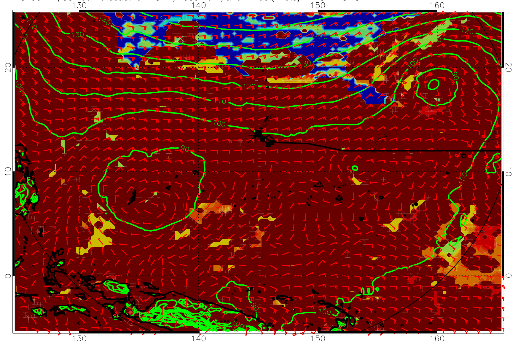
16100712, 36 hour forecast for HCAL, 1000mb Z, and winds (knots) -- NCEP GFS
