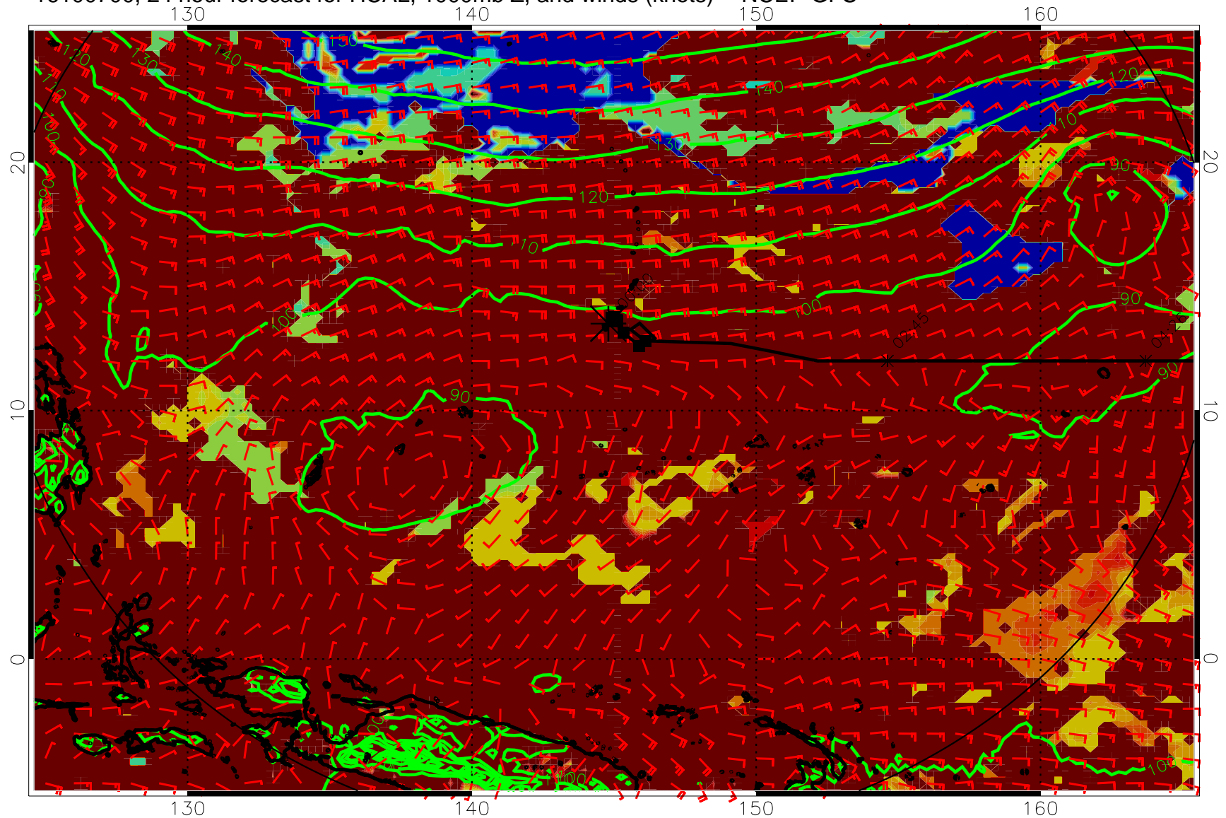
16100700, 24 hour forecast for HCAL, 1000mb Z, and winds (knots) -- NCEP GFS
