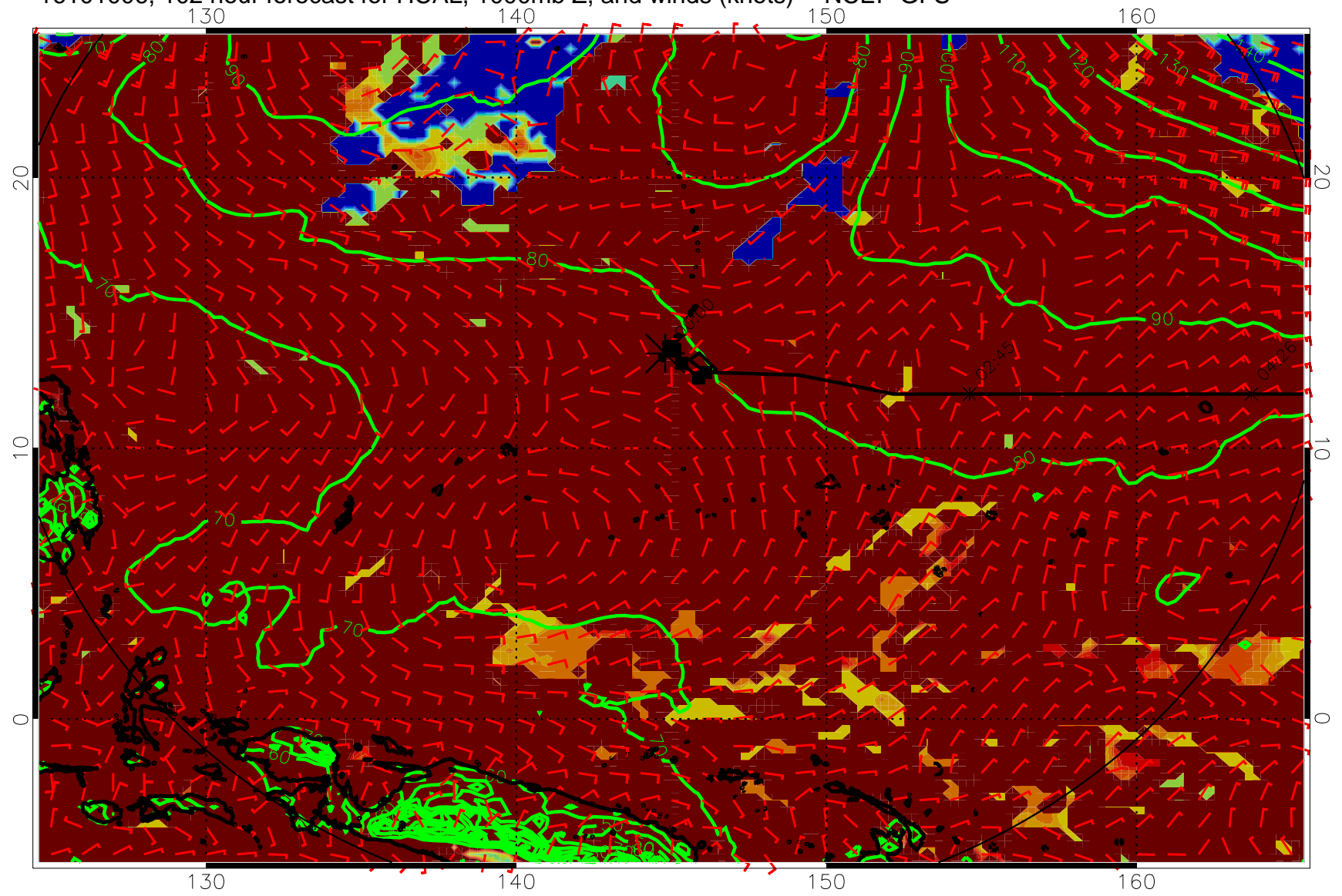
16101006, 102 hour forecast for HCAL, 1000mb Z, and winds (knots) -- NCEP GFS
