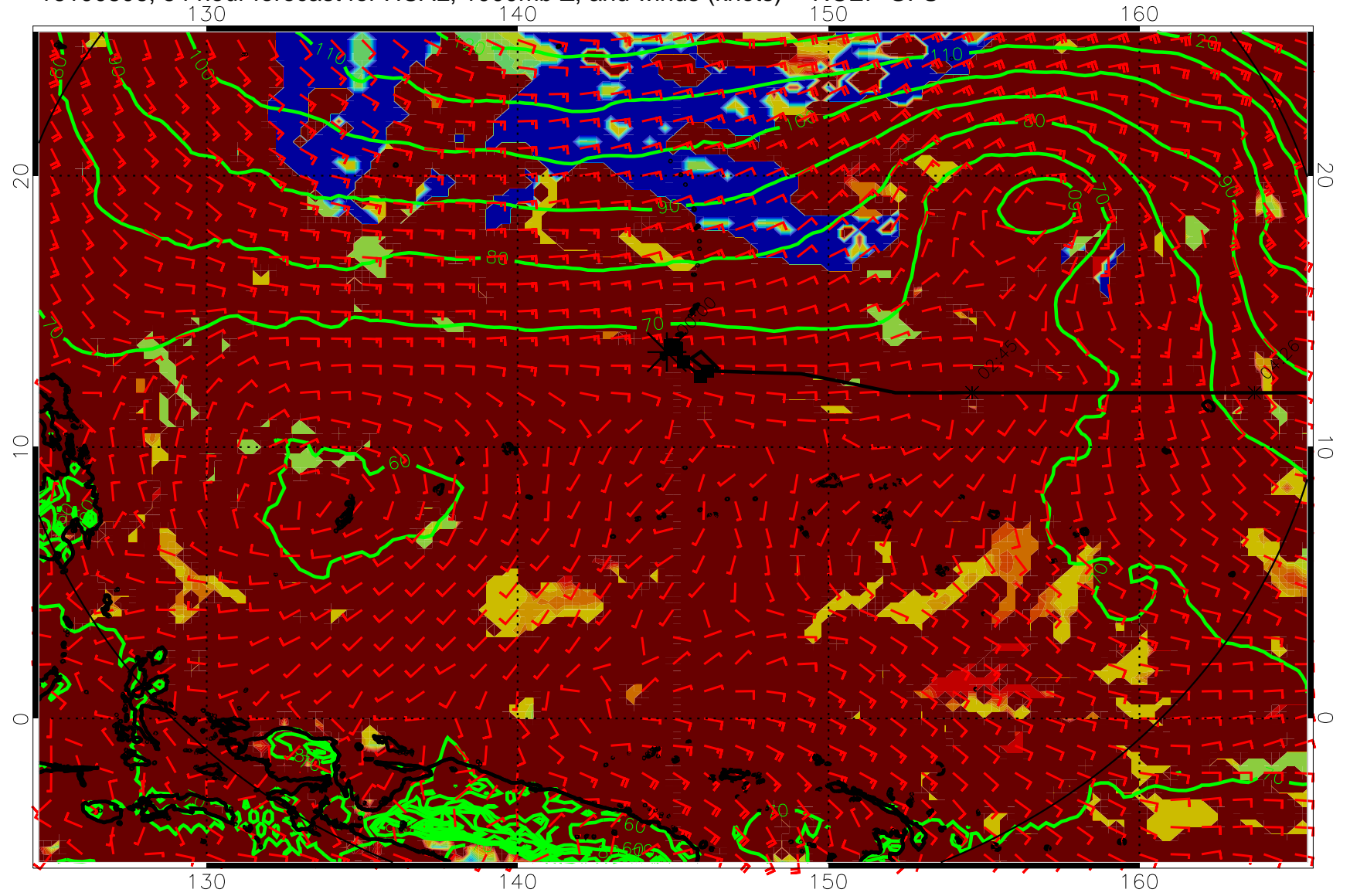
16100806, 54 hour forecast for HCAL, 1000mb Z, and winds (knots) -- NCEP GFS
