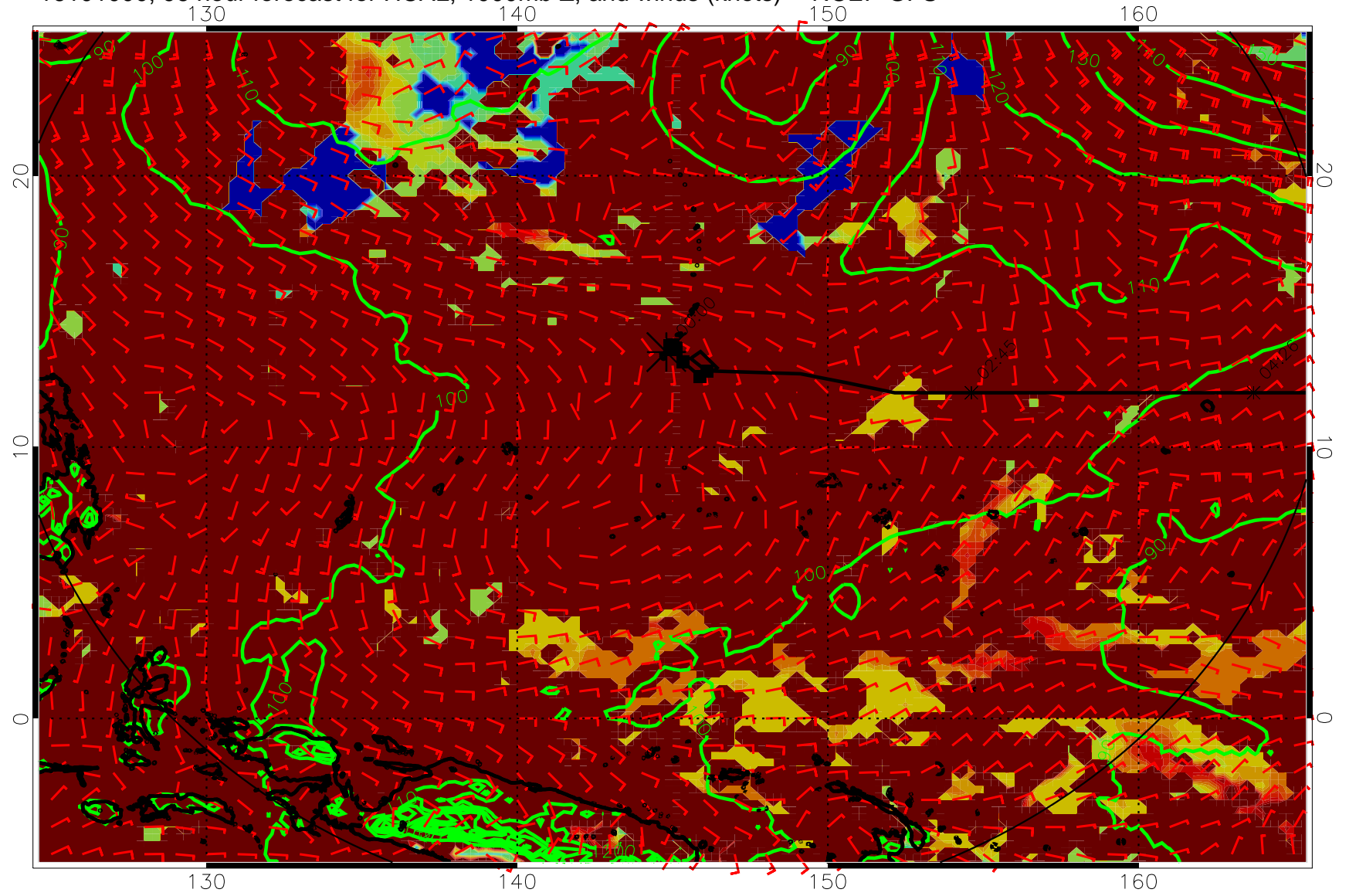
16101000, 96 hour forecast for HCAL, 1000mb Z, and winds (knots) -- NCEP GFS
