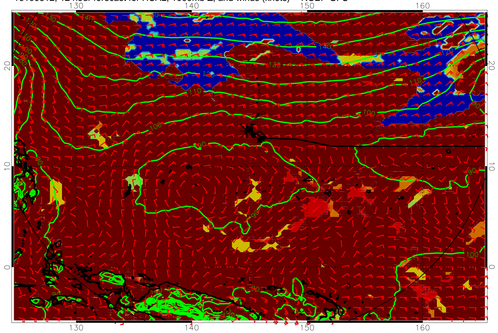
16100612, 12 hour forecast for HCAL, 1000mb Z, and winds (knots) -- NCEP GFS
