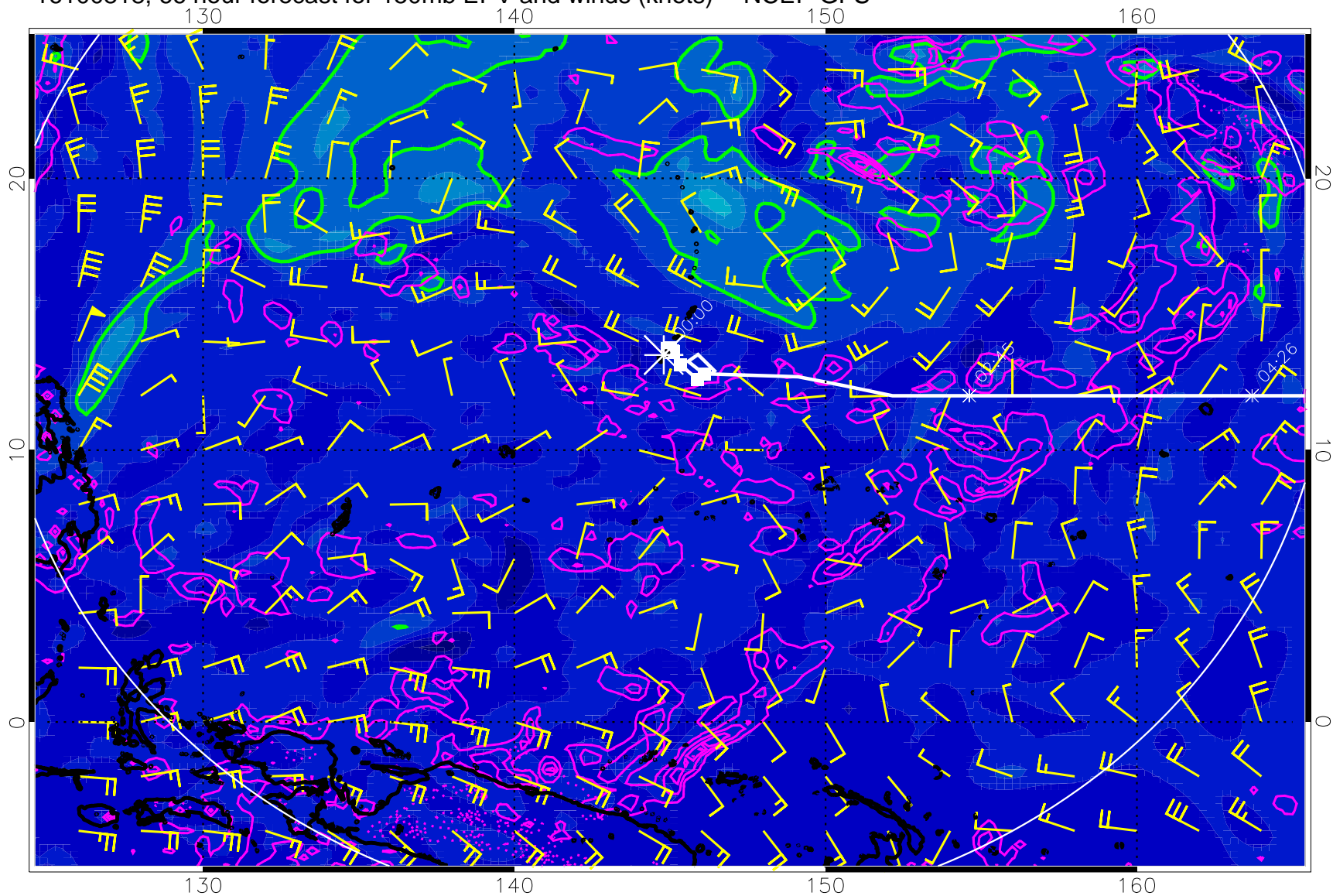
16100818, 66 hour forecast for 150mb EPV and winds (knots) -- NCEP GFS
