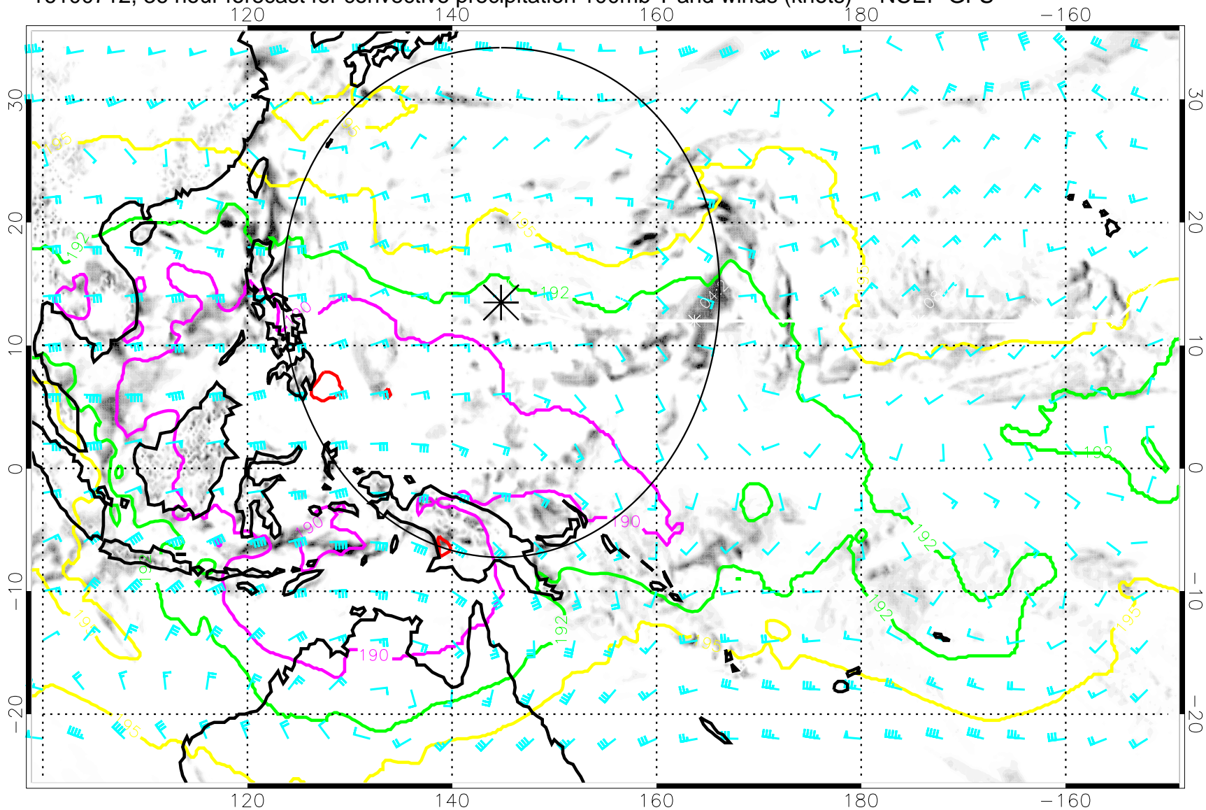
16100712, 36 hour forecast for convective precipitation 100mb T and winds (knots) -- NCEP GFS
