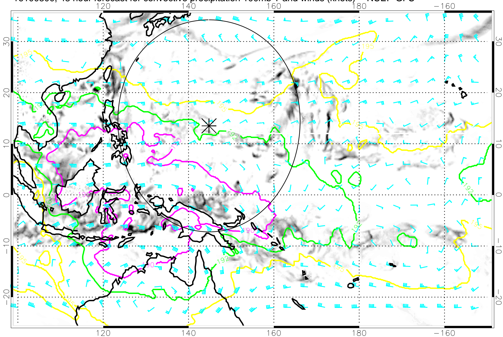
16100800, 48 hour forecast for convective precipitation 100mb T and winds (knots) -- NCEP GFS
