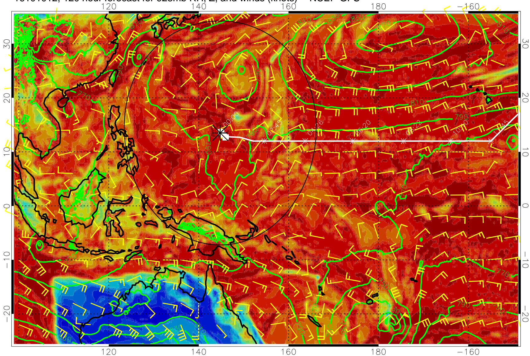
16101012, 120 hour forecast for 925mb RH, Z, and winds (knots) -- NCEP GFS
