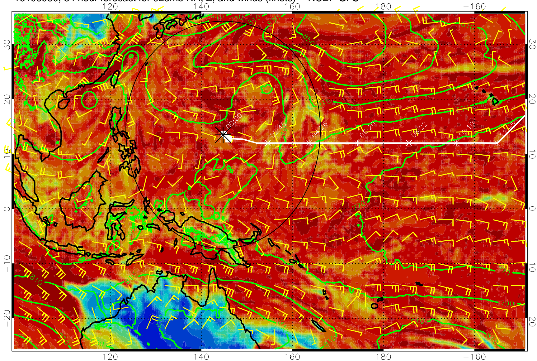
16100900, 84 hour forecast for 925mb RH, Z, and winds (knots) -- NCEP GFS
