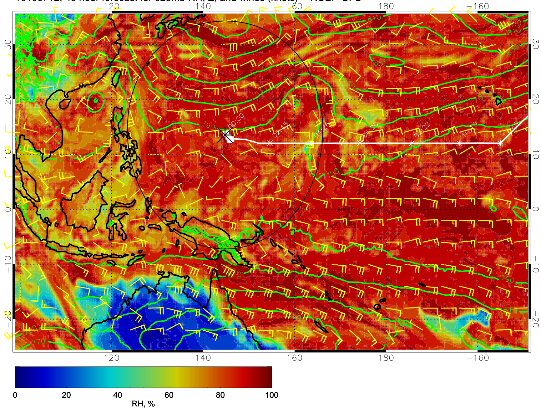
16100712, 48 hour forecast for 925mb RH, Z, and winds (knots) -- NCEP GFS
