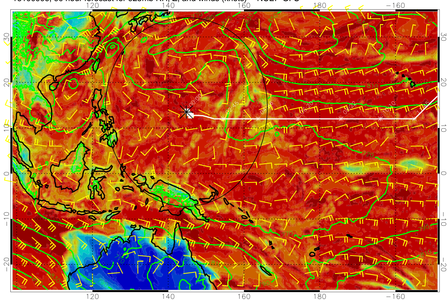
16100906, 90 hour forecast for 925mb RH, Z, and winds (knots) -- NCEP GFS
