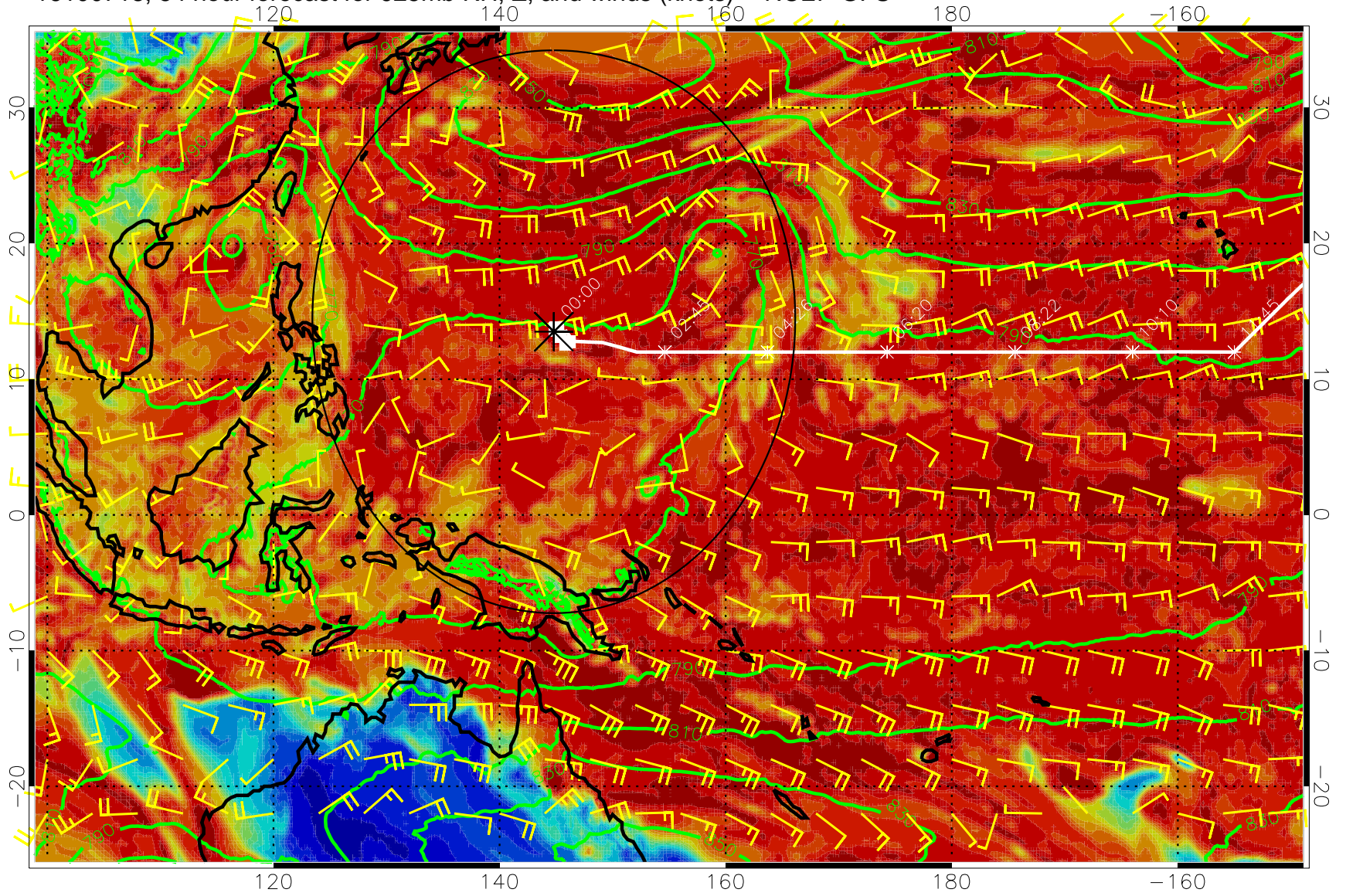
16100718, 54 hour forecast for 925mb RH, Z, and winds (knots) -- NCEP GFS
