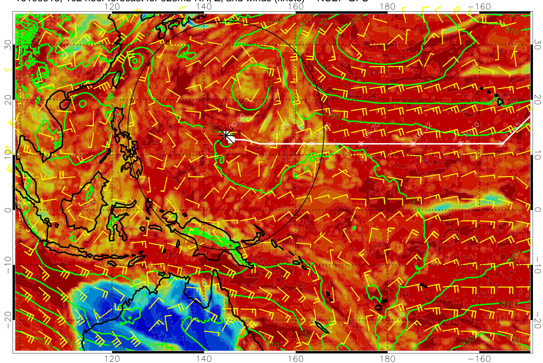
16100918, 102 hour forecast for 925mb RH, Z, and winds (knots) -- NCEP GFS
