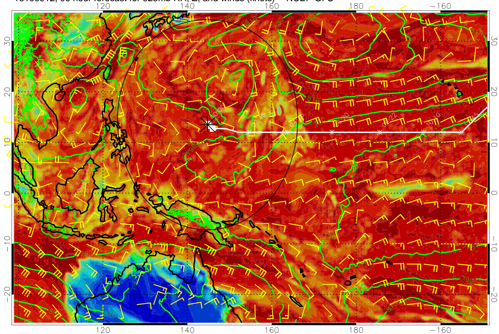
16100912, 96 hour forecast for 925mb RH, Z, and winds (knots) -- NCEP GFS
