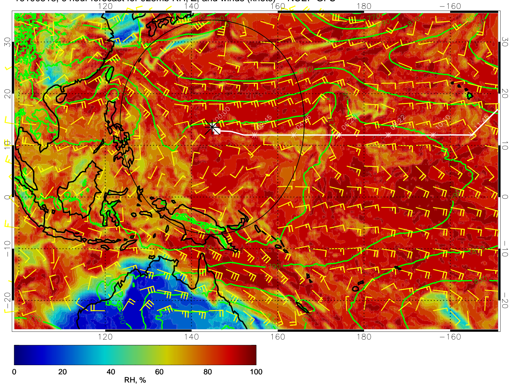
16100518, 6 hour forecast for 925mb RH, Z, and winds (knots) -- NCEP GFS
