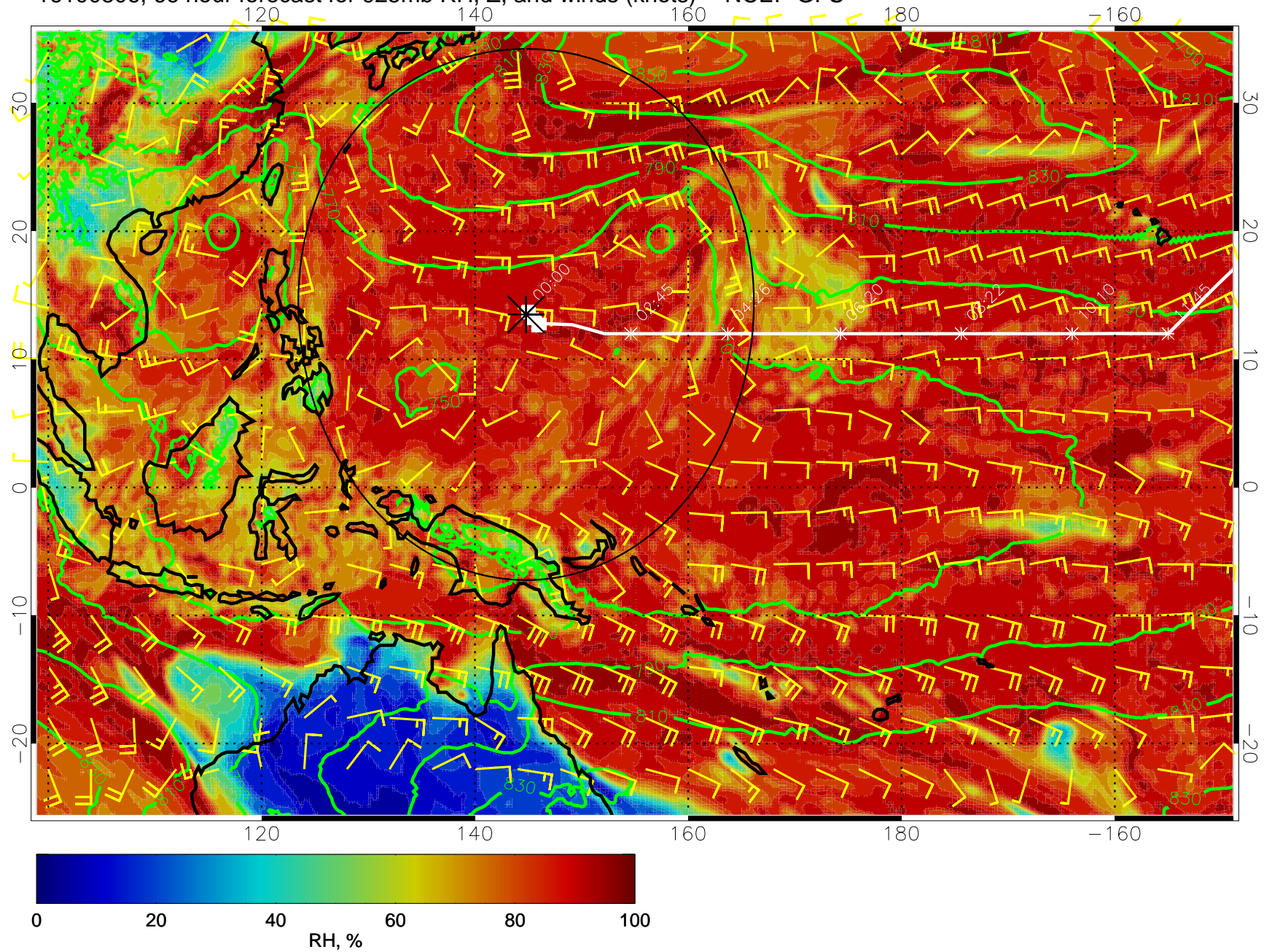
16100806, 66 hour forecast for 925mb RH, Z, and winds (knots) -- NCEP GFS
