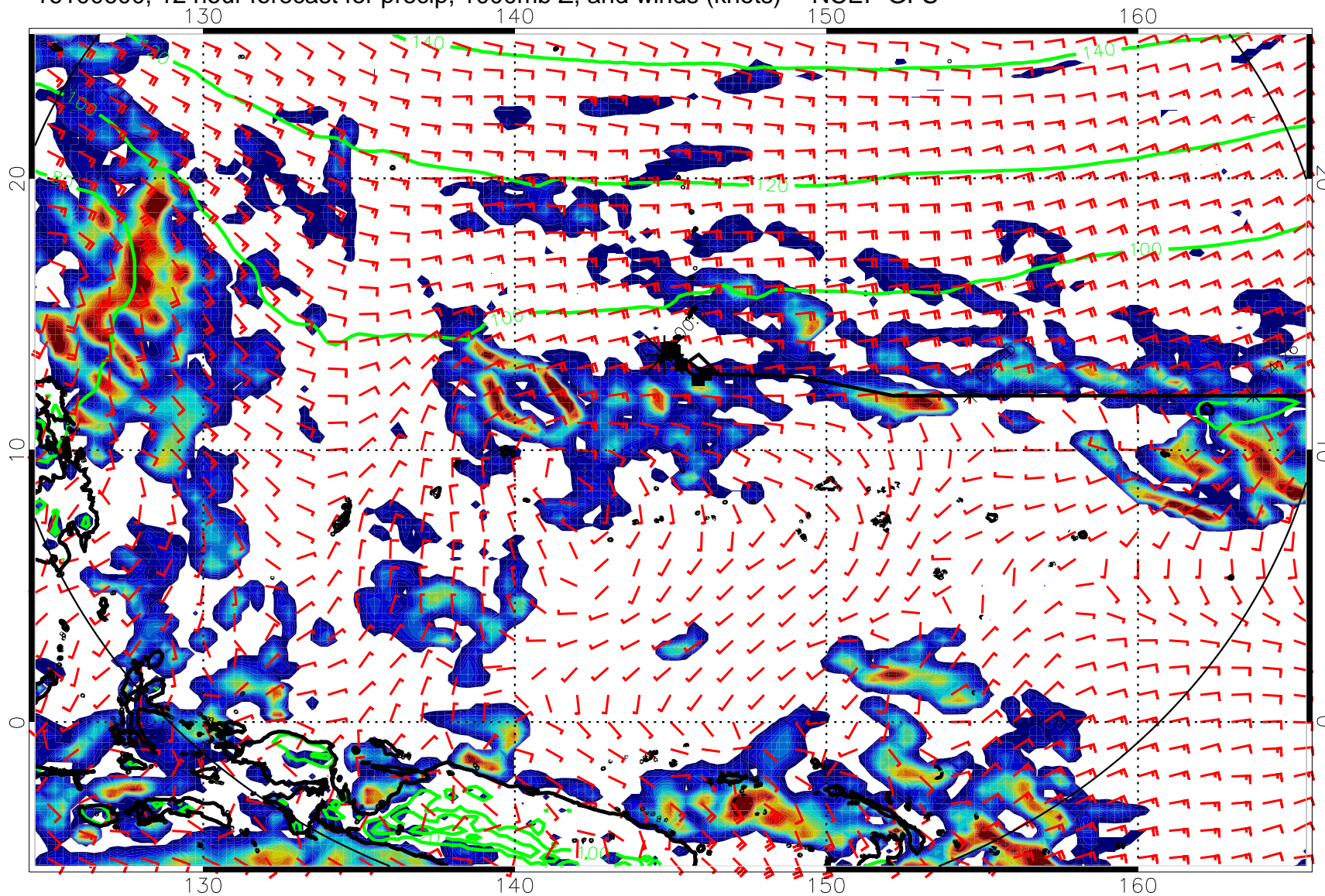
16100600, 12 hour forecast for precip, 1000mb Z, and winds (knots) -- NCEP GFS
