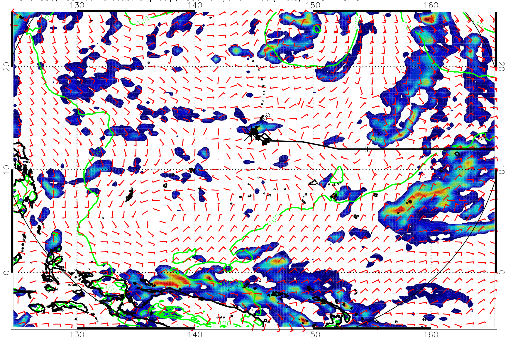
16101000, 108 hour forecast for precip, 1000mb Z, and winds (knots) -- NCEP GFS
