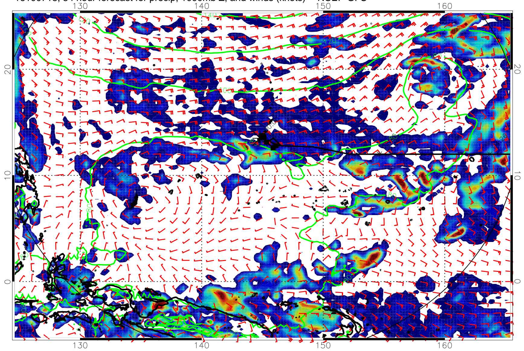
16100718, 54 hour forecast for precip, 1000mb Z, and winds (knots) -- NCEP GFS
