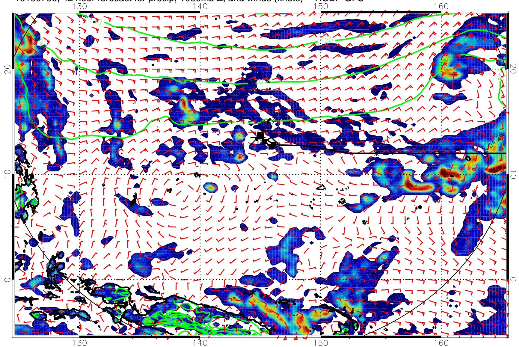
16100706, 42 hour forecast for precip, 1000mb Z, and winds (knots) -- NCEP GFS
