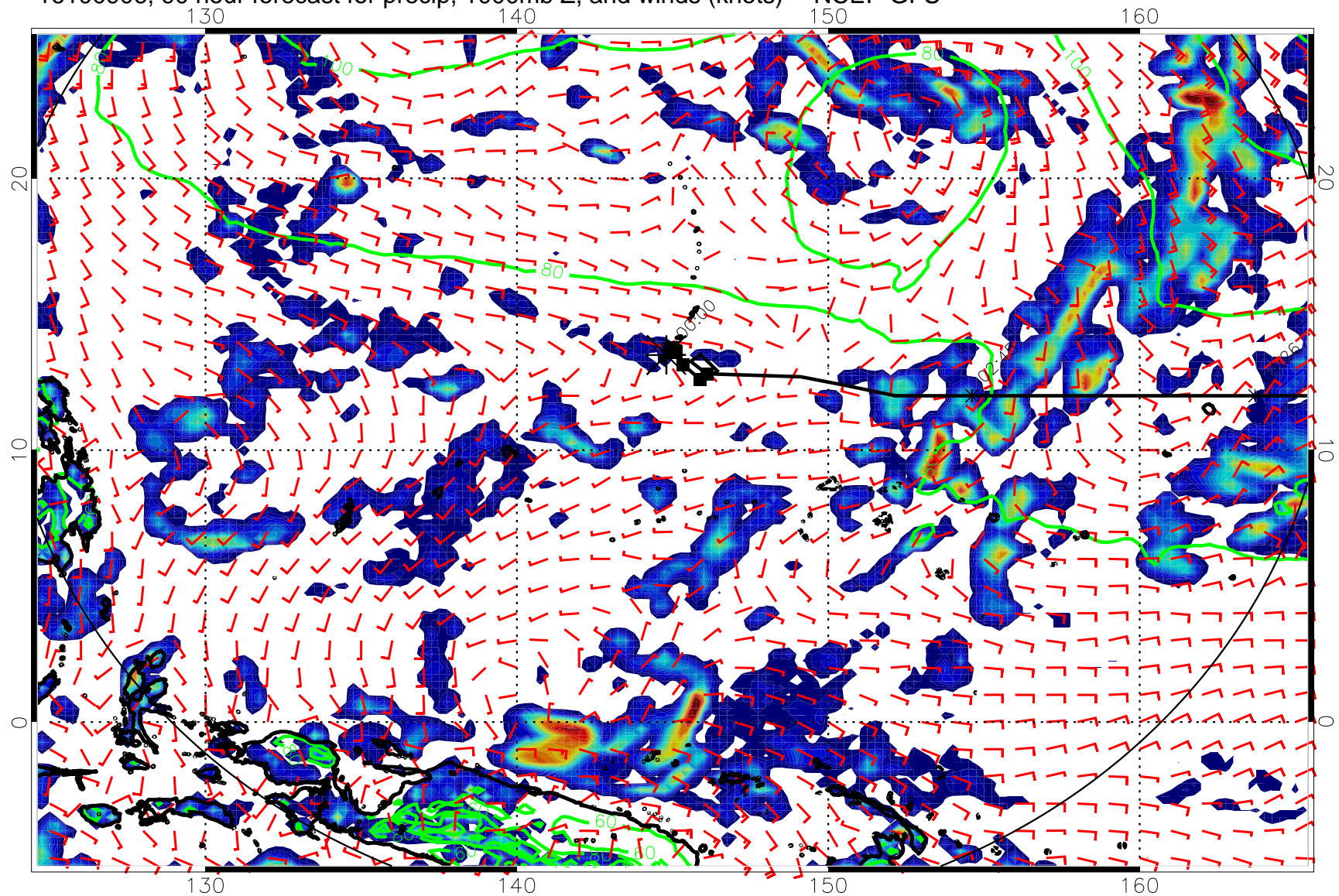
16100906, 90 hour forecast for precip, 1000mb Z, and winds (knots) -- NCEP GFS
