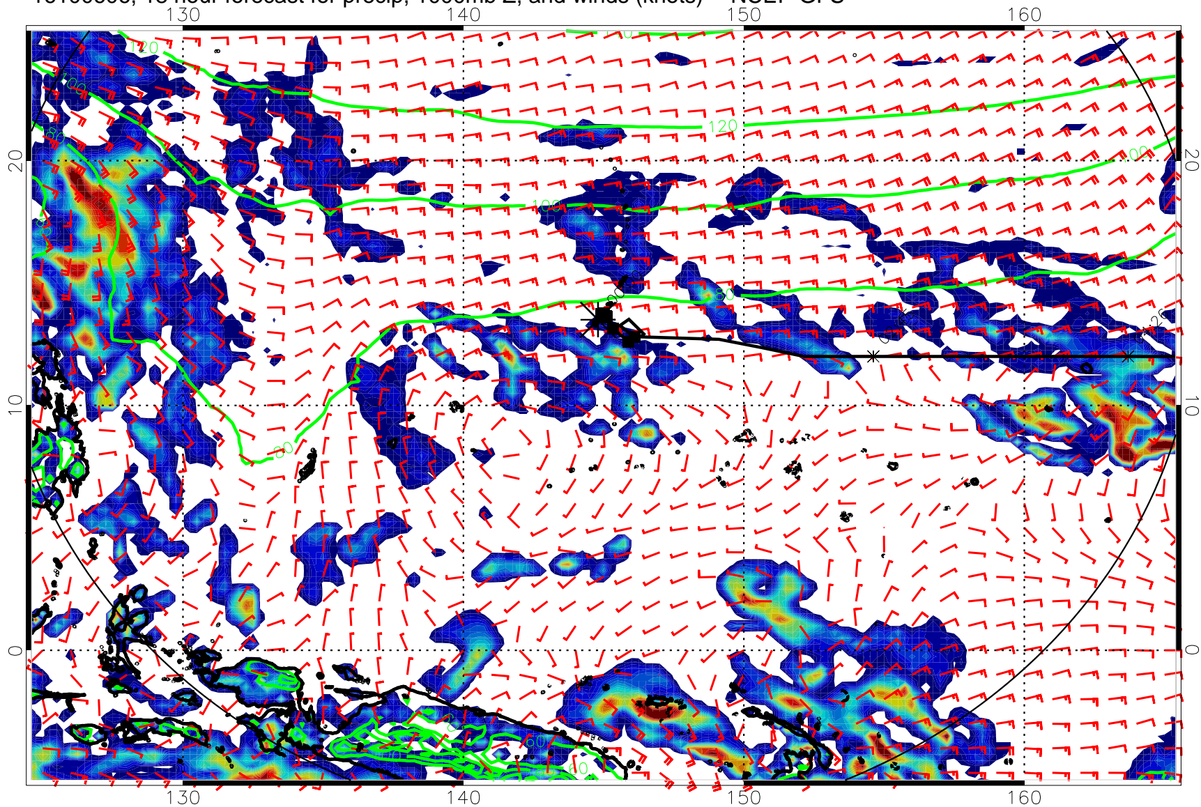
16100606, 18 hour forecast for precip, 1000mb Z, and winds (knots) -- NCEP GFS
