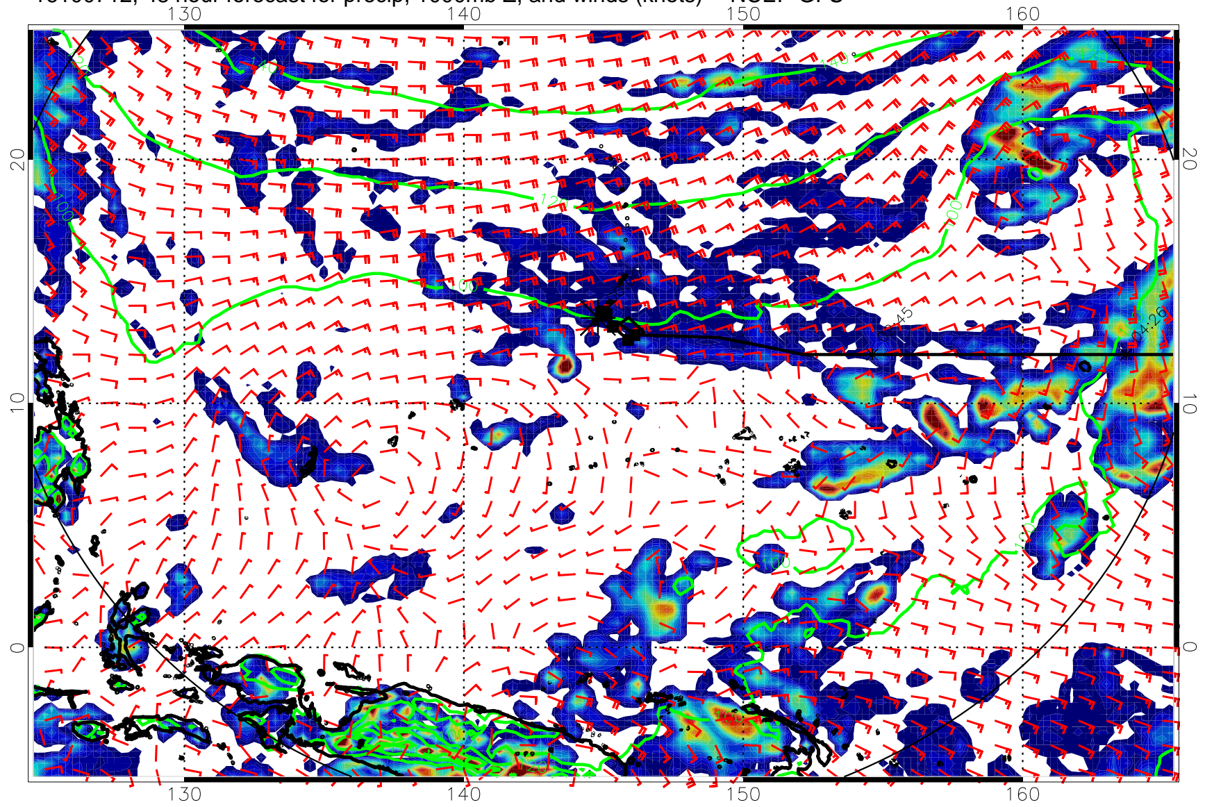
16100712, 48 hour forecast for precip, 1000mb Z, and winds (knots) -- NCEP GFS
