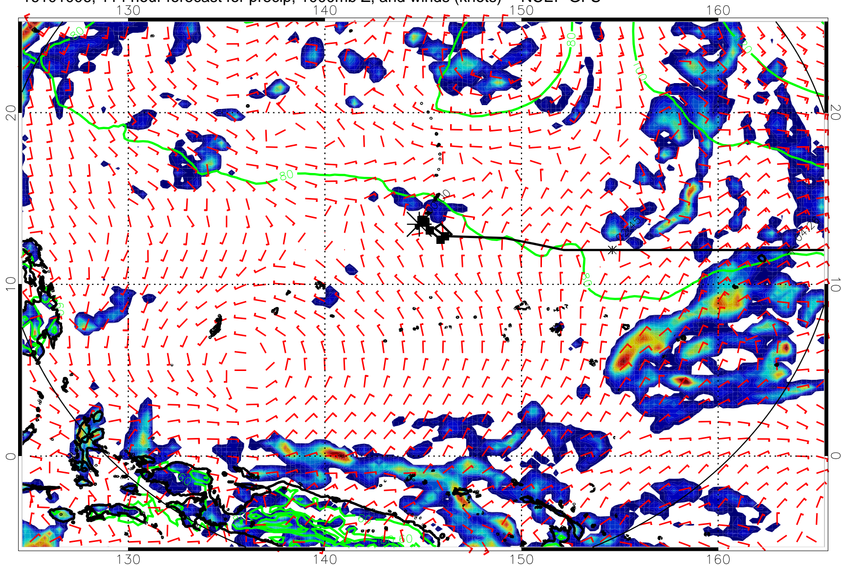
16101006, 114 hour forecast for precip, 1000mb Z, and winds (knots) -- NCEP GFS
