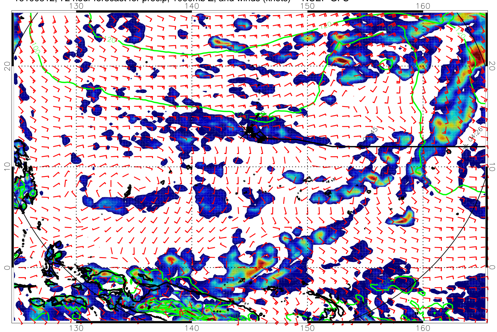
16100812, 72 hour forecast for precip, 1000mb Z, and winds (knots) -- NCEP GFS
