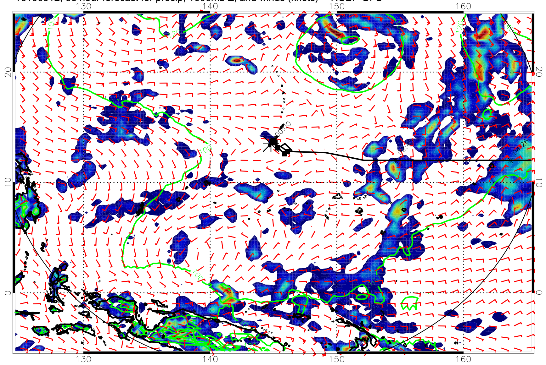
16100912, 96 hour forecast for precip, 1000mb Z, and winds (knots) -- NCEP GFS
