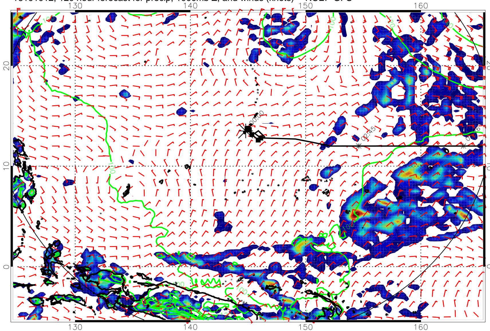
16101012, 120 hour forecast for precip, 1000mb Z, and winds (knots) -- NCEP GFS
