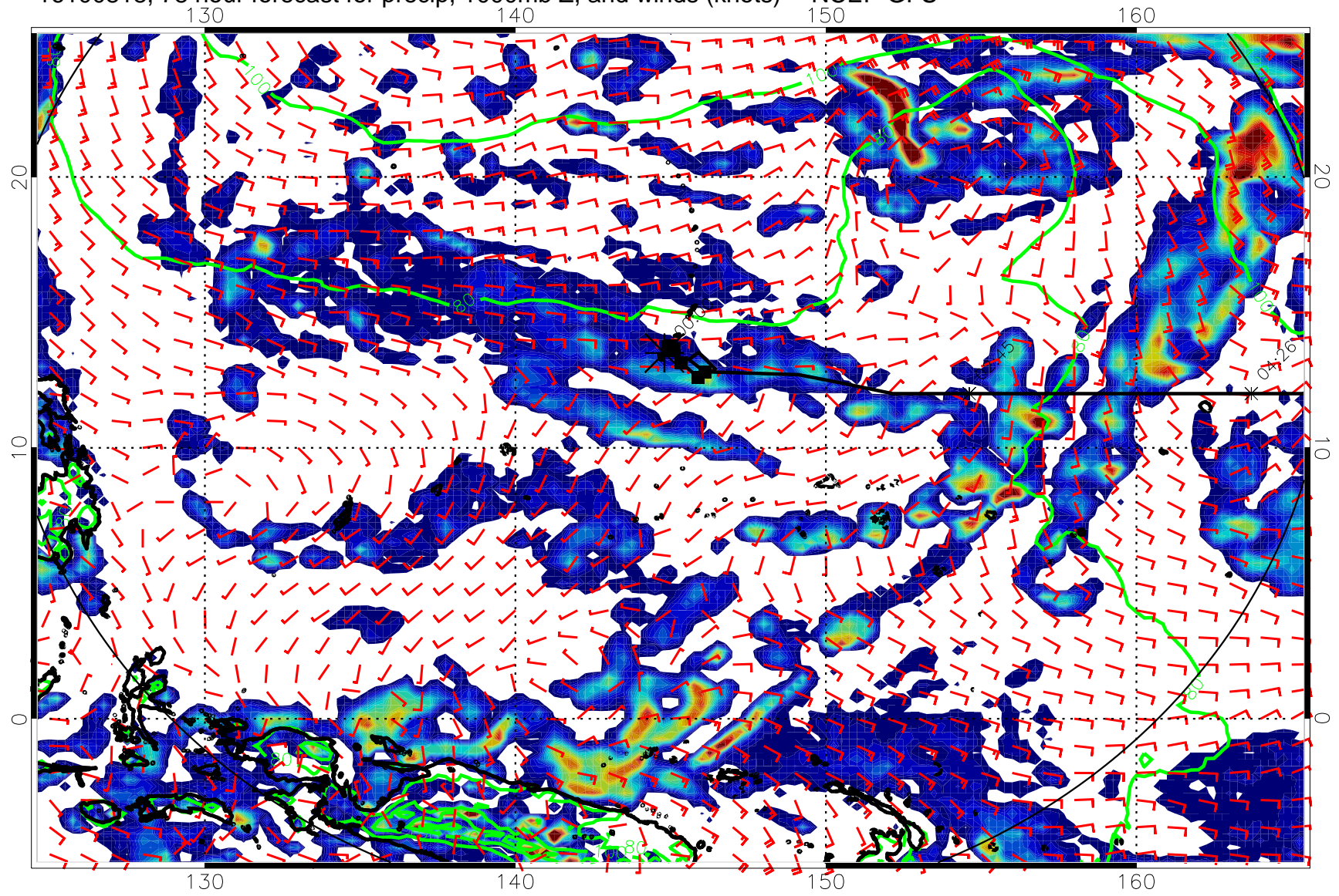
16100818, 78 hour forecast for precip, 1000mb Z, and winds (knots) -- NCEP GFS
