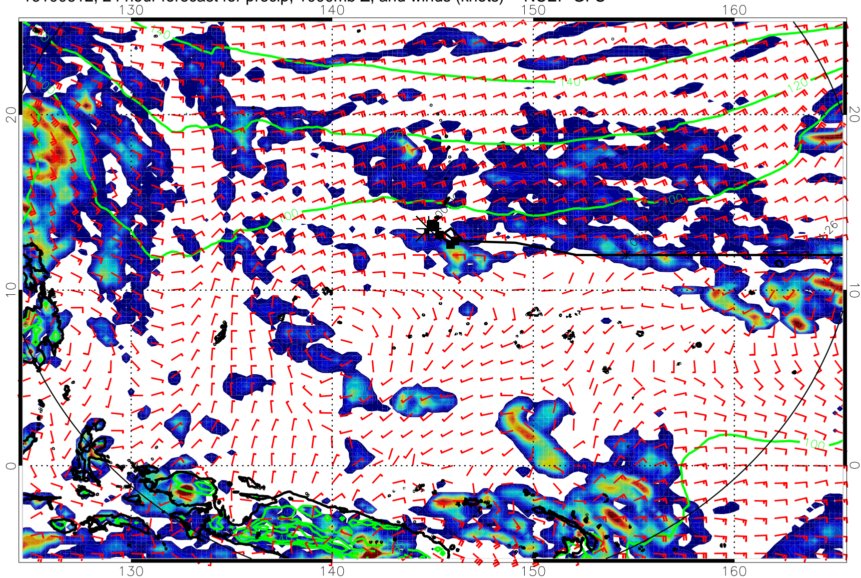
16100612, 24 hour forecast for precip, 1000mb Z, and winds (knots) -- NCEP GFS
