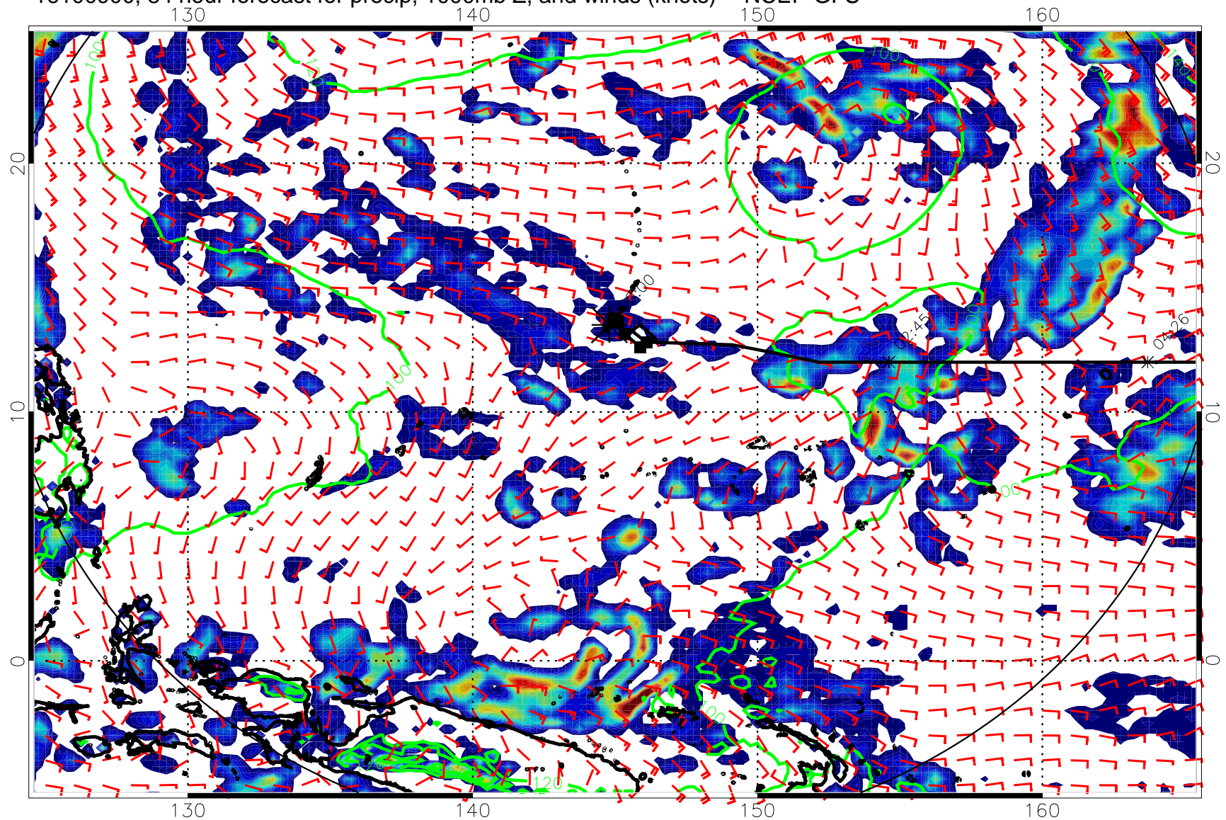
16100900, 84 hour forecast for precip, 1000mb Z, and winds (knots) -- NCEP GFS
