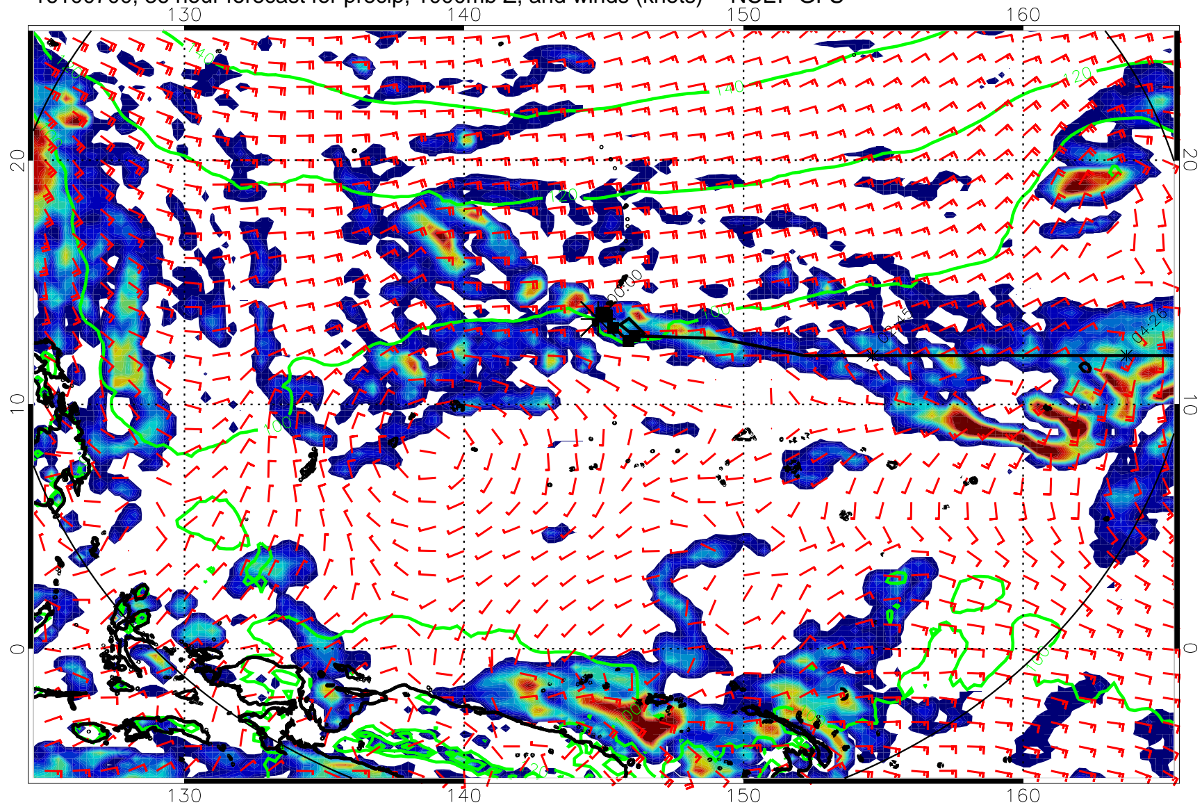
16100700, 36 hour forecast for precip, 1000mb Z, and winds (knots) -- NCEP GFS
