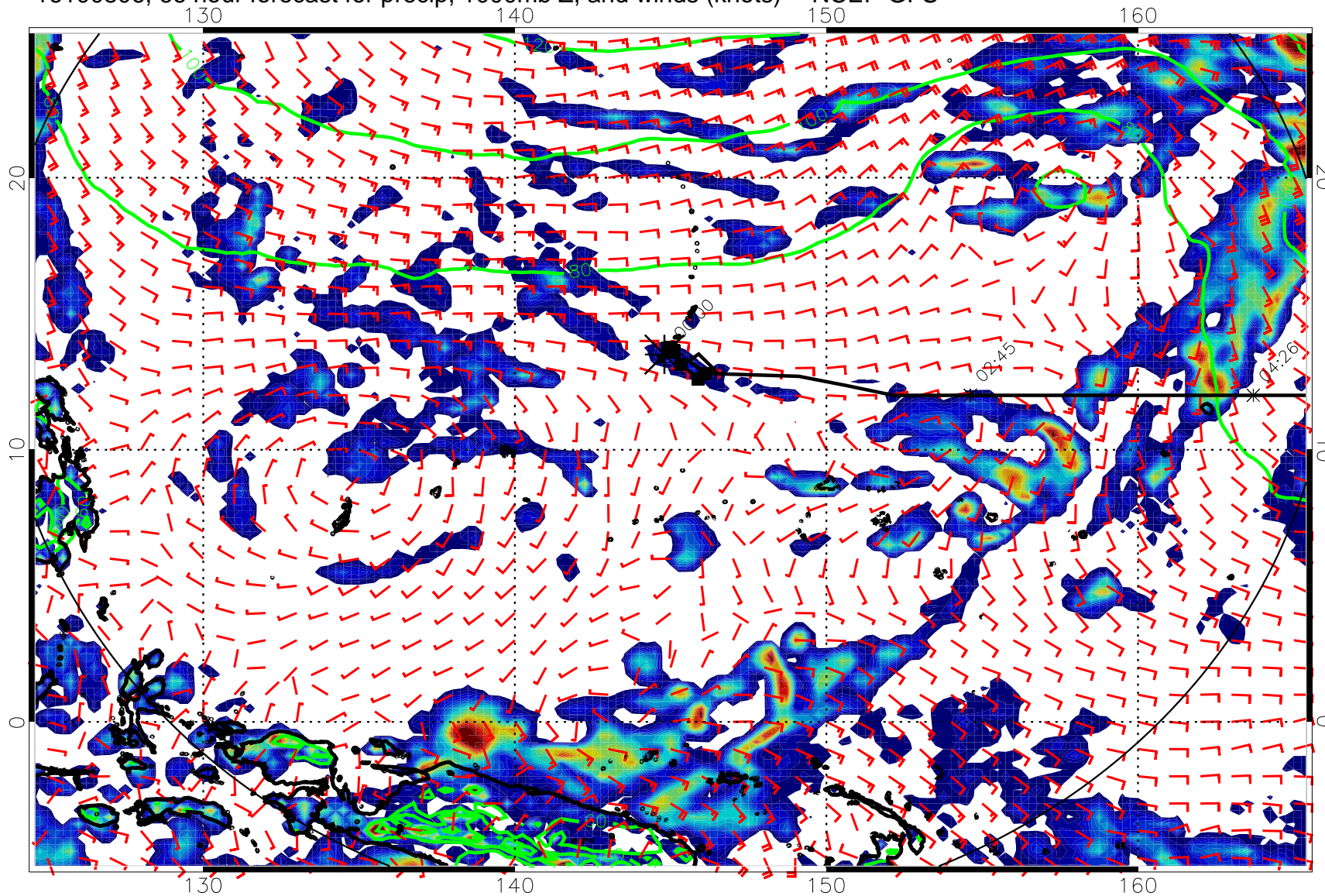
16100806, 66 hour forecast for precip, 1000mb Z, and winds (knots) -- NCEP GFS
