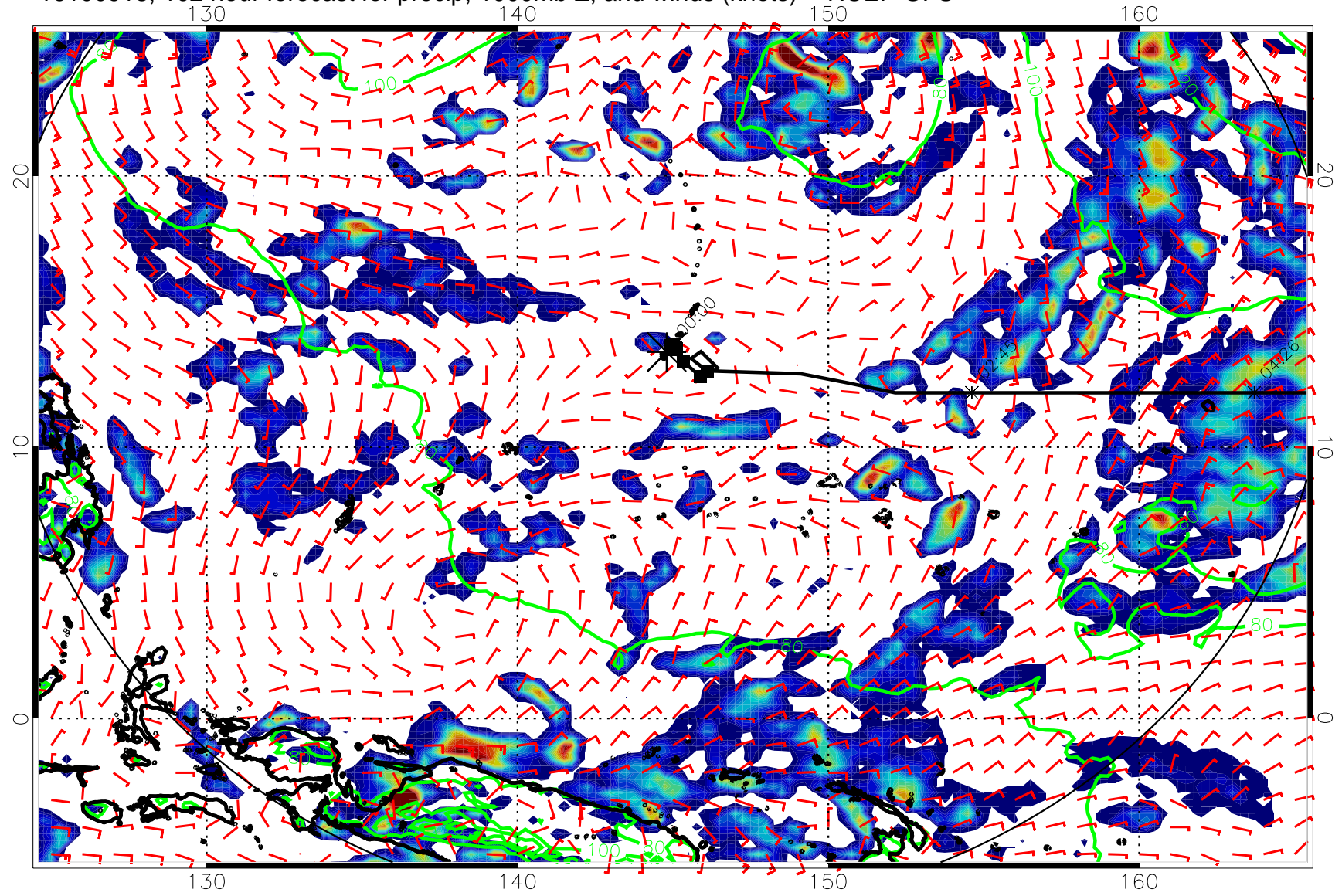
16100918, 102 hour forecast for precip, 1000mb Z, and winds (knots) -- NCEP GFS
