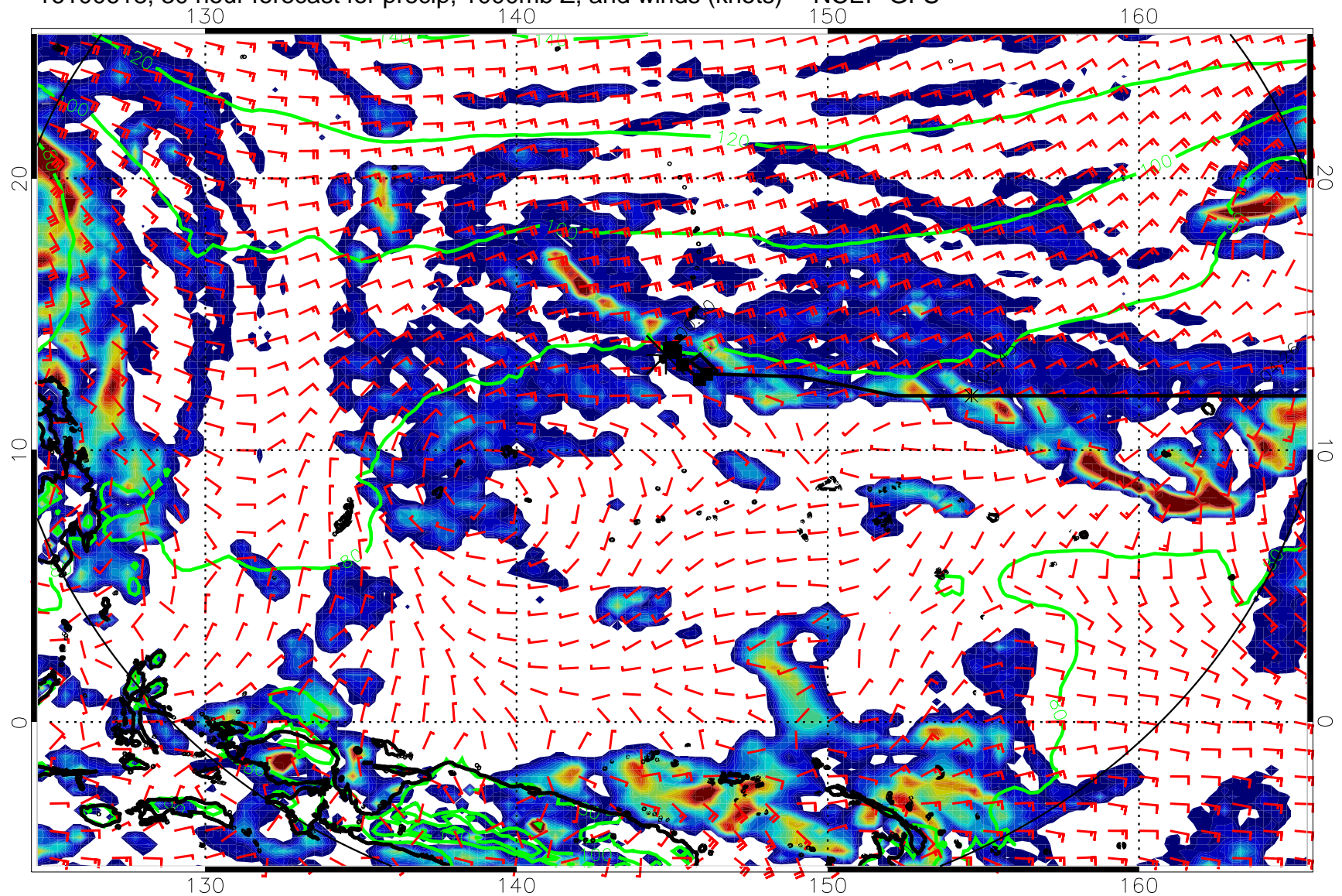
16100618, 30 hour forecast for precip, 1000mb Z, and winds (knots) -- NCEP GFS
