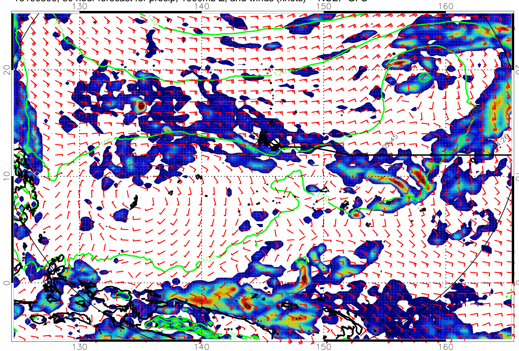
16100800, 60 hour forecast for precip, 1000mb Z, and winds (knots) -- NCEP GFS
