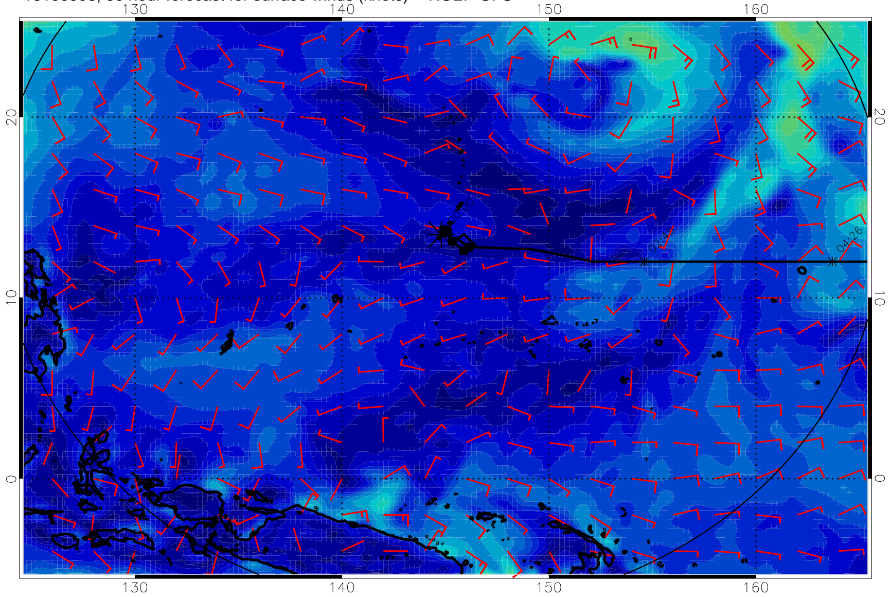
16100906, 90 hour forecast for surface winds (knots) -- NCEP GFS
