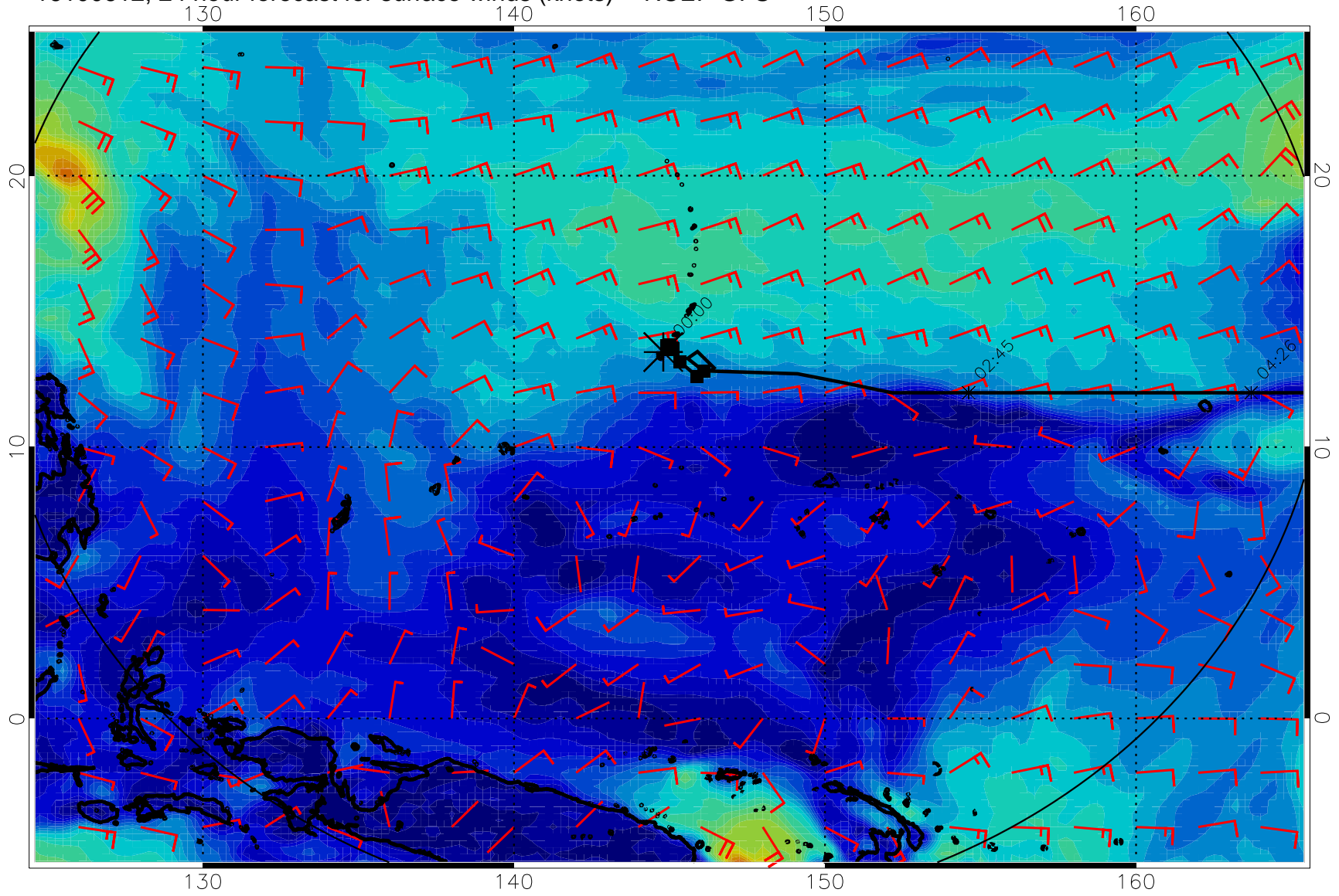
16100612, 24 hour forecast for surface winds (knots) -- NCEP GFS
