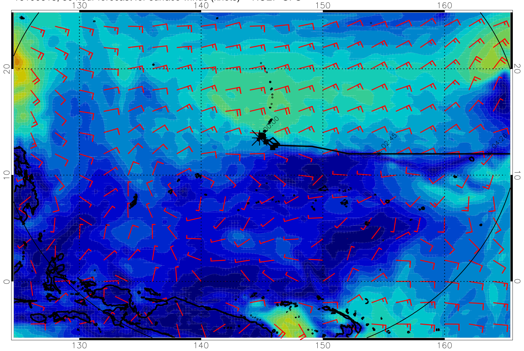
16100618, 30 hour forecast for surface winds (knots) -- NCEP GFS
