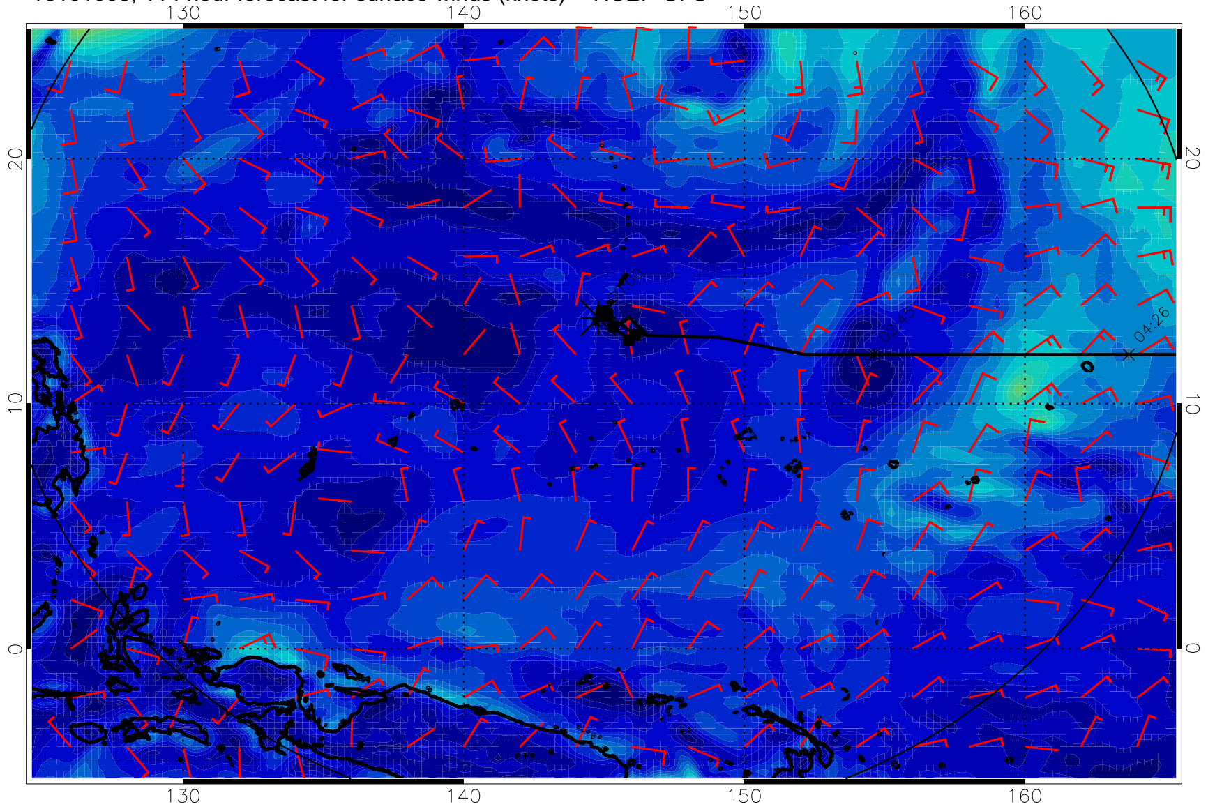
16101006, 114 hour forecast for surface winds (knots) -- NCEP GFS
