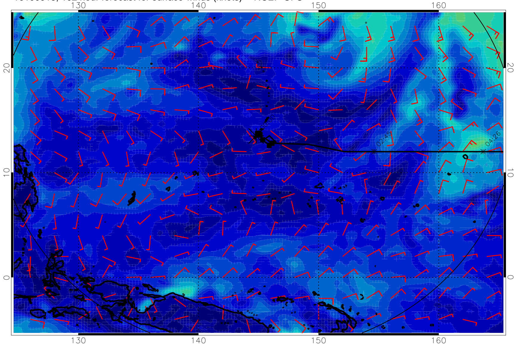
16100918, 102 hour forecast for surface winds (knots) -- NCEP GFS
