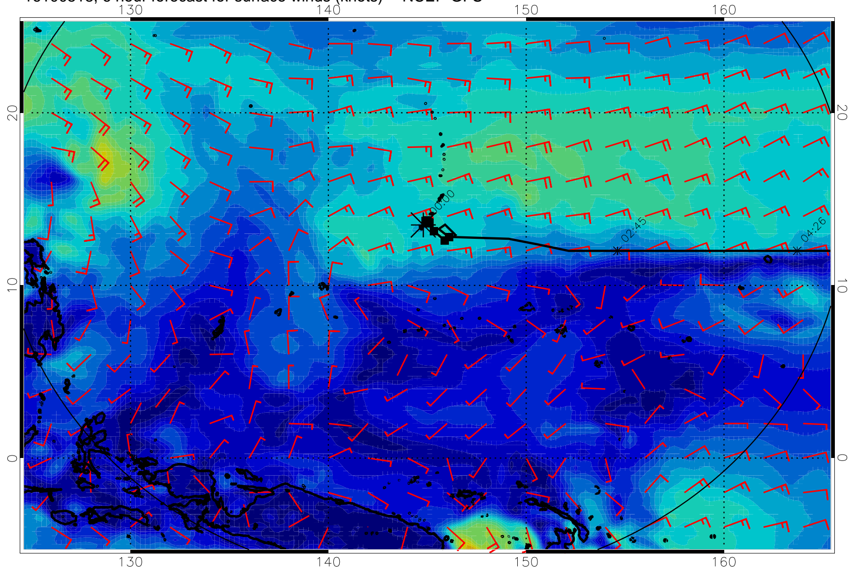
16100518, 6 hour forecast for surface winds (knots) -- NCEP GFS
