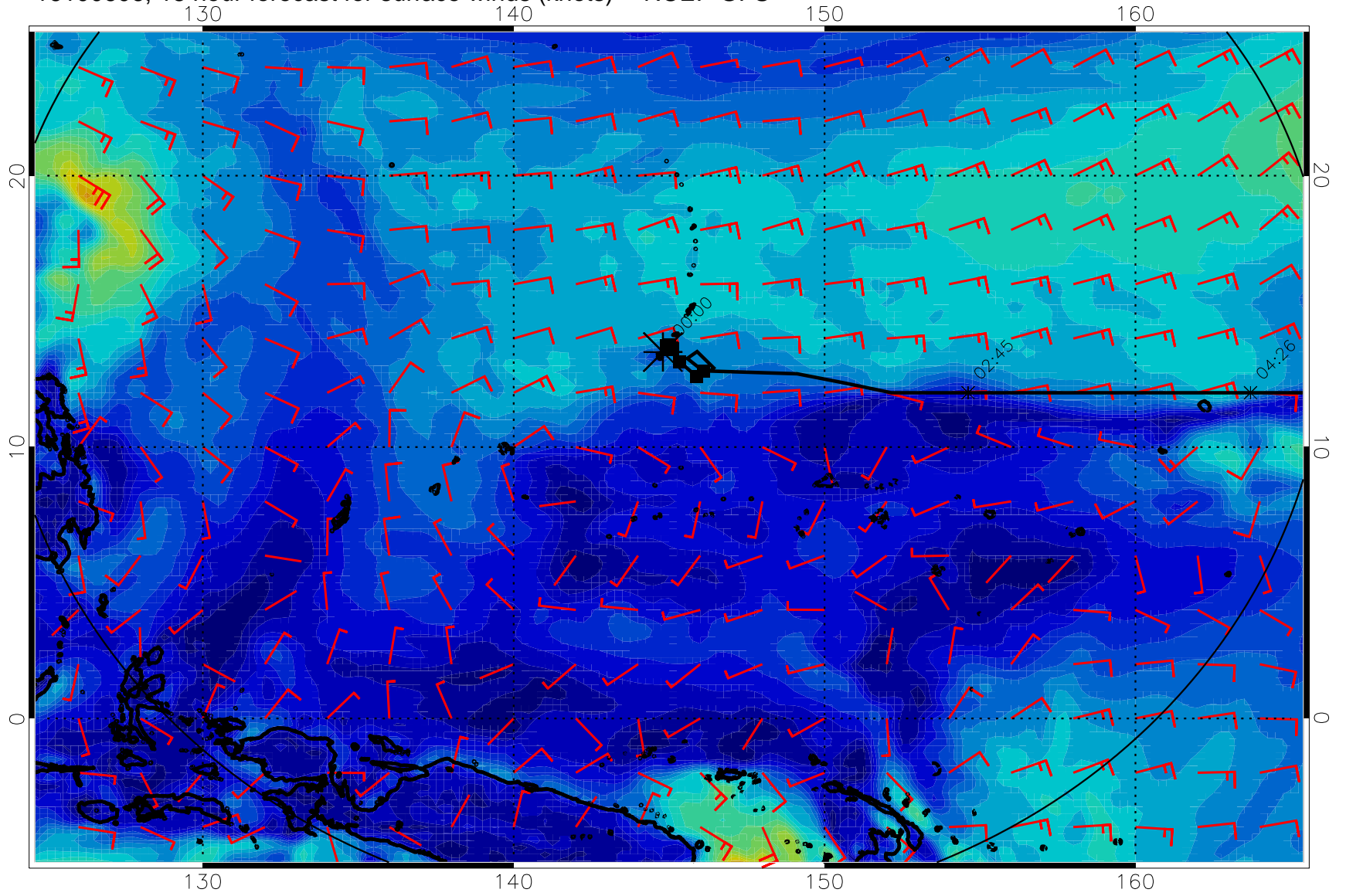
16100606, 18 hour forecast for surface winds (knots) -- NCEP GFS
