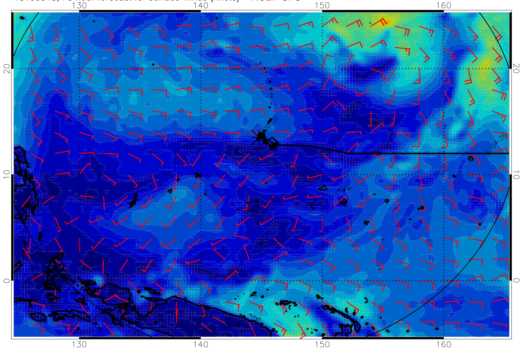
16100818, 78 hour forecast for surface winds (knots) -- NCEP GFS
