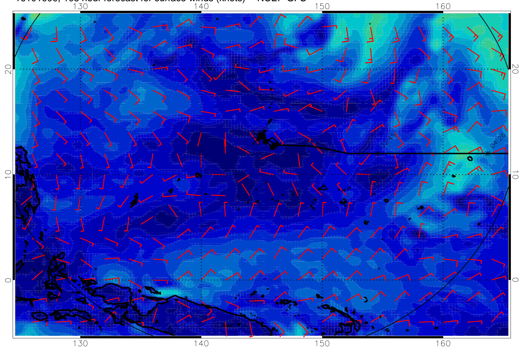
16101000, 108 hour forecast for surface winds (knots) -- NCEP GFS
