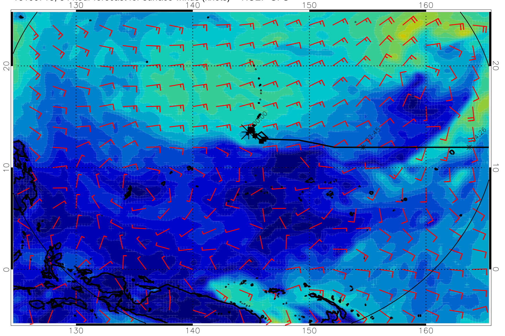
16100718, 54 hour forecast for surface winds (knots) -- NCEP GFS
