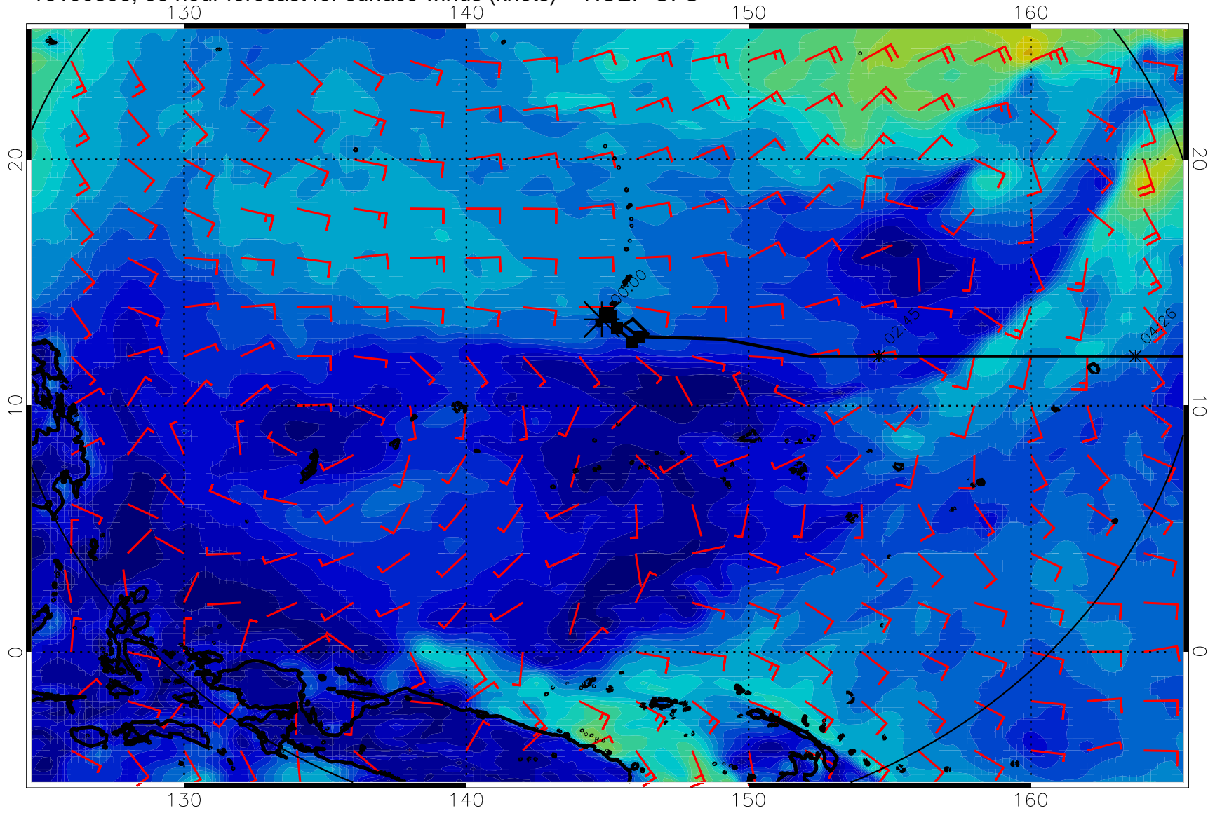
16100806, 66 hour forecast for surface winds (knots) -- NCEP GFS
