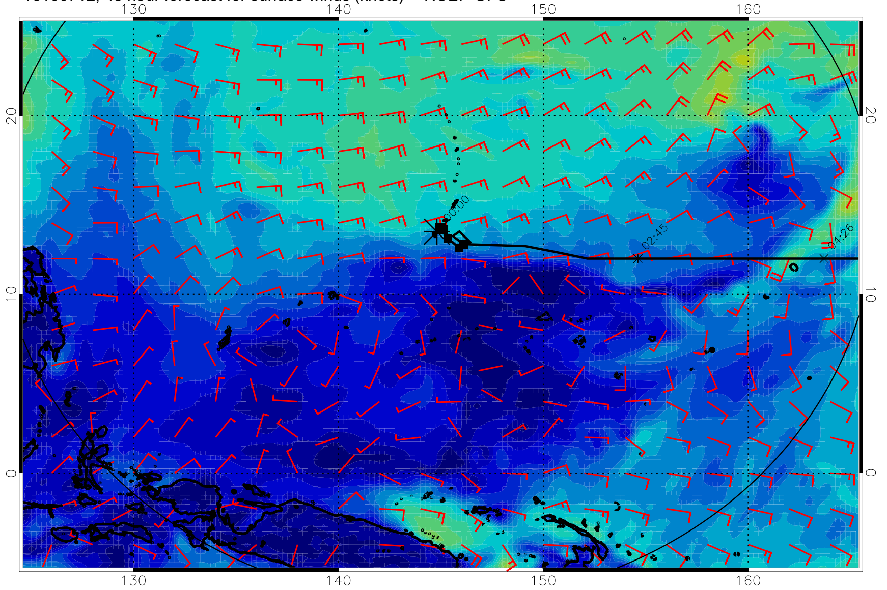
16100712, 48 hour forecast for surface winds (knots) -- NCEP GFS
