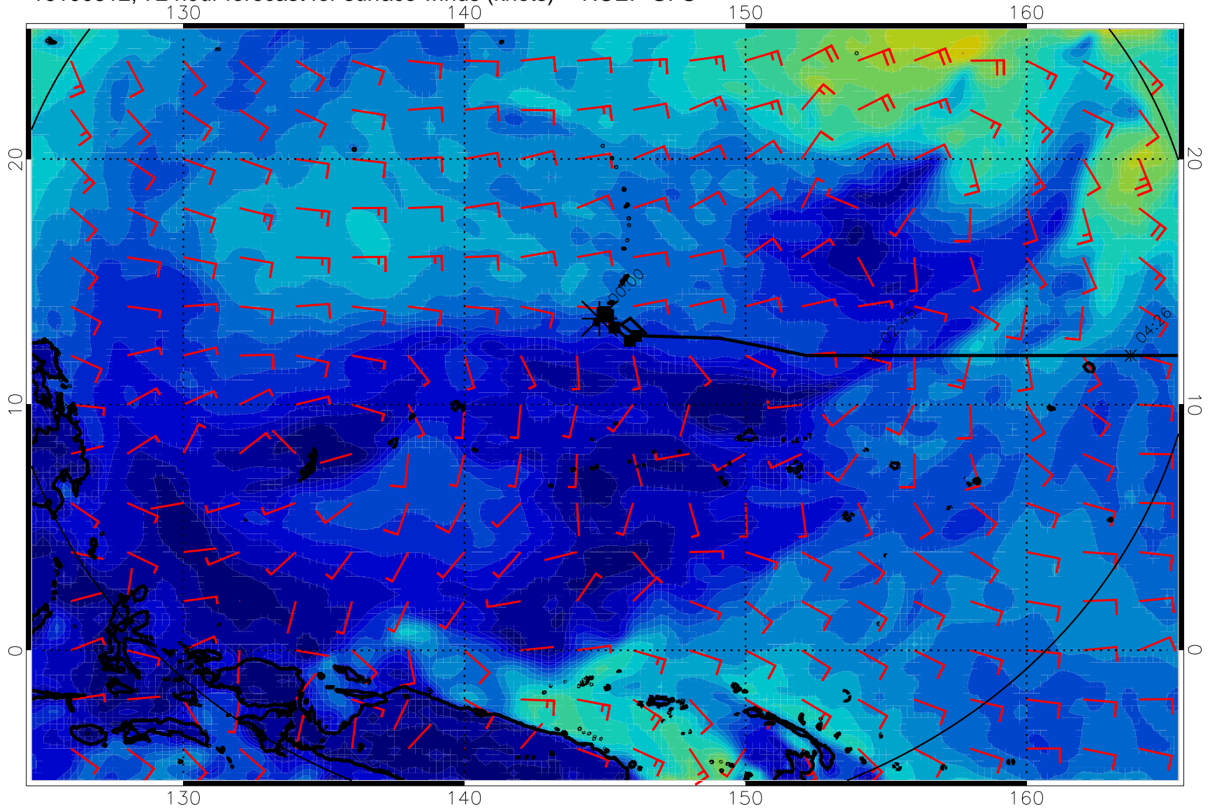
16100812, 72 hour forecast for surface winds (knots) -- NCEP GFS
