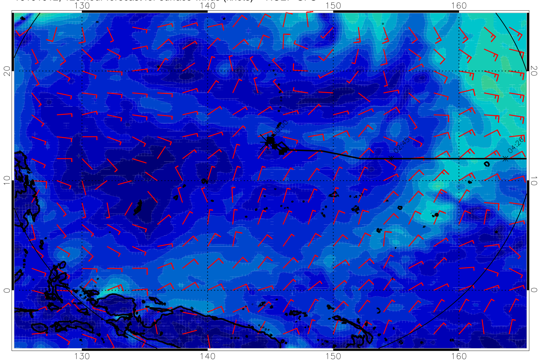
16101012, 120 hour forecast for surface winds (knots) -- NCEP GFS
