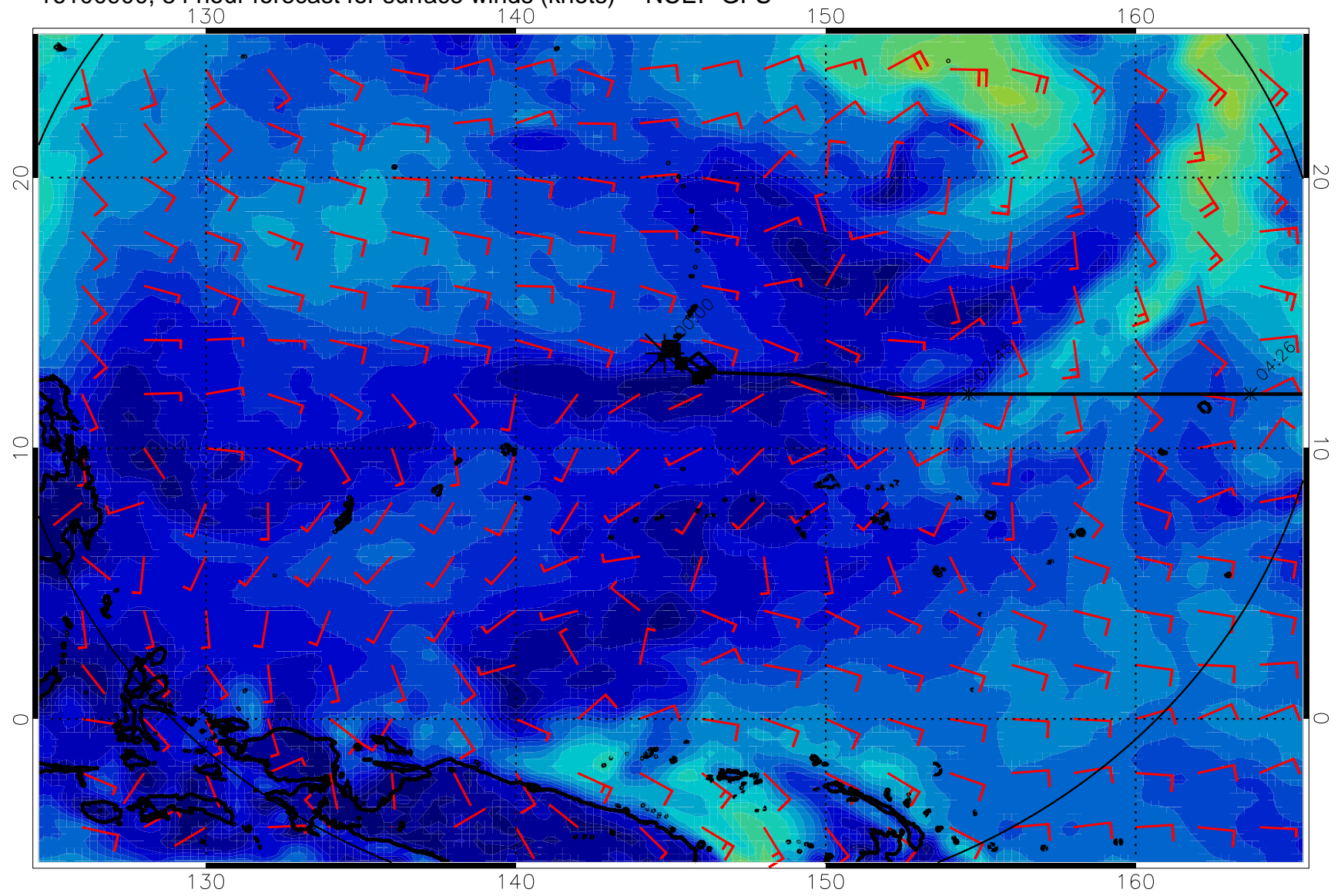
16100900, 84 hour forecast for surface winds (knots) -- NCEP GFS
