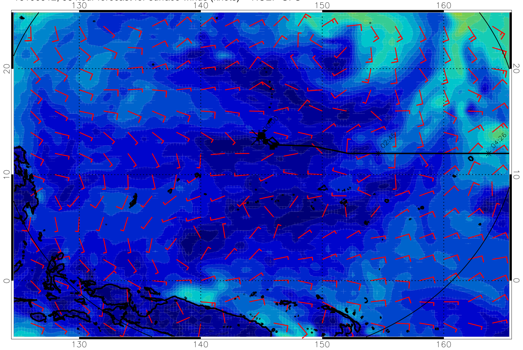
16100912, 96 hour forecast for surface winds (knots) -- NCEP GFS
