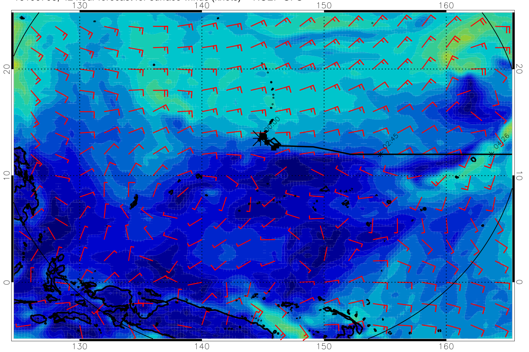
16100706, 42 hour forecast for surface winds (knots) -- NCEP GFS
