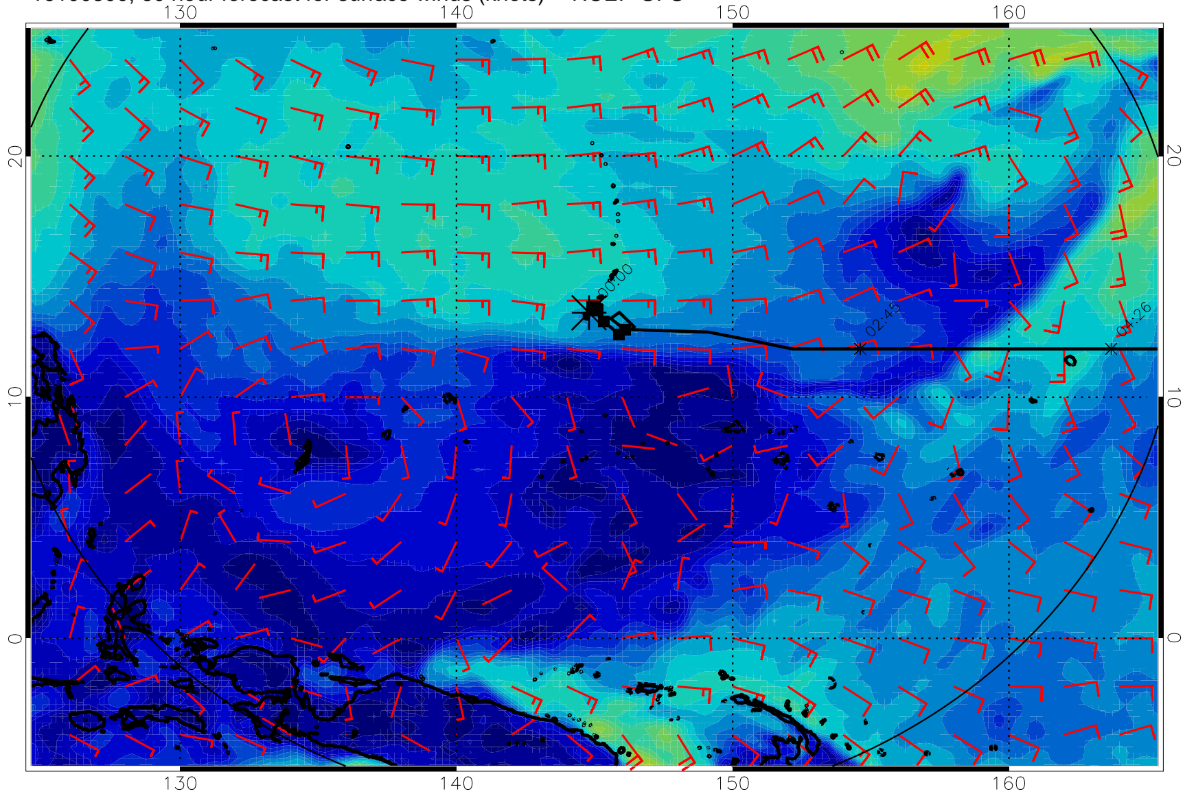
16100800, 60 hour forecast for surface winds (knots) -- NCEP GFS
