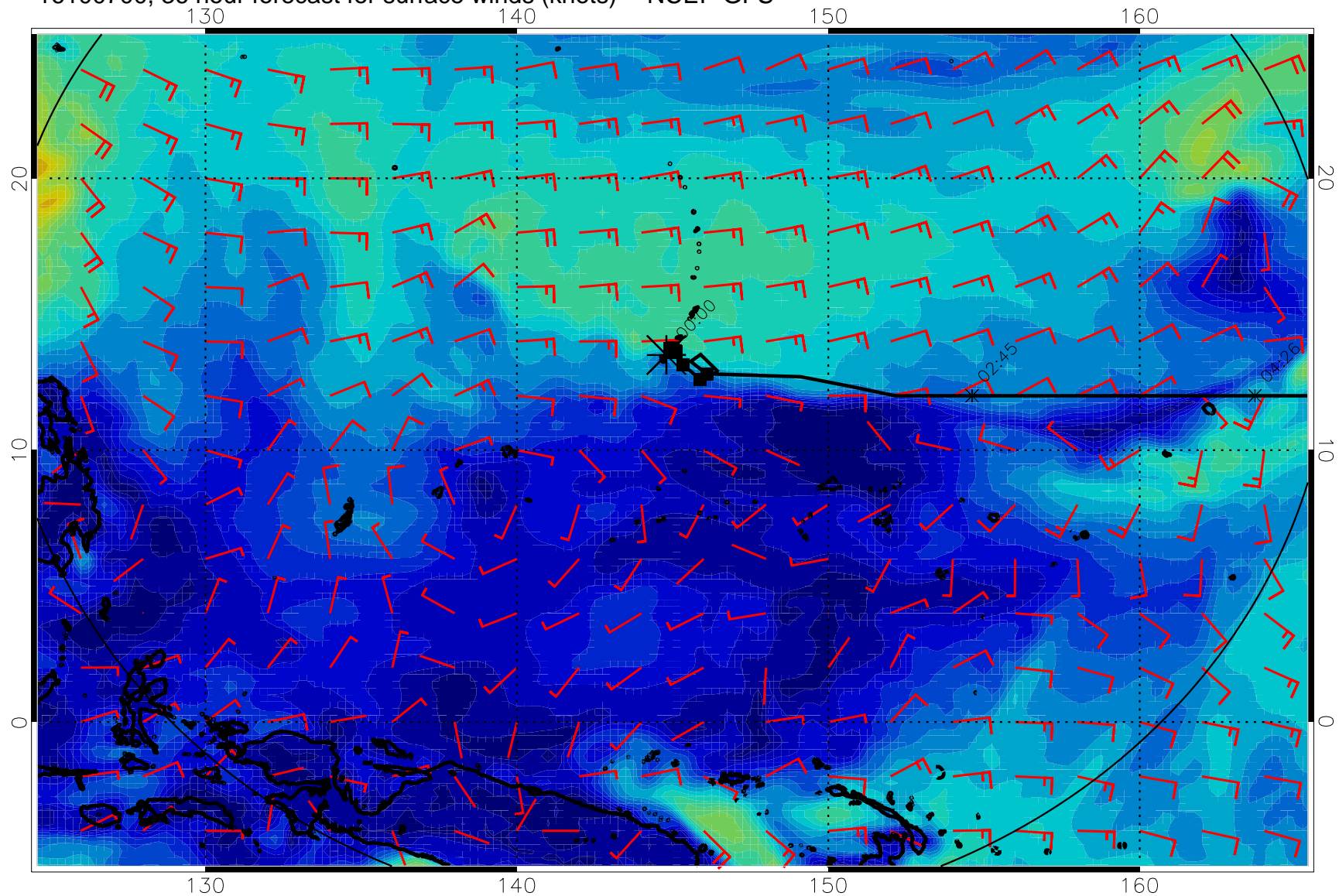
16100700, 36 hour forecast for surface winds (knots) -- NCEP GFS
