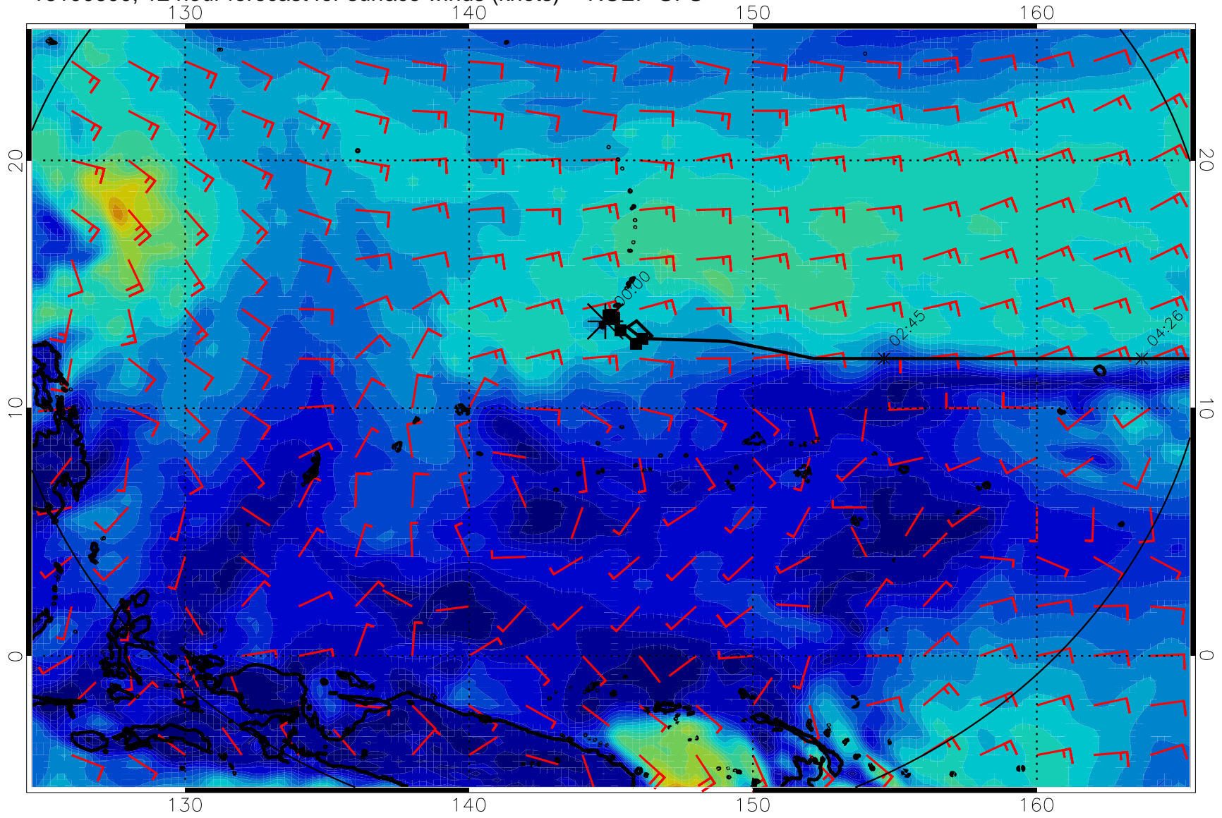
16100600, 12 hour forecast for surface winds (knots) -- NCEP GFS
