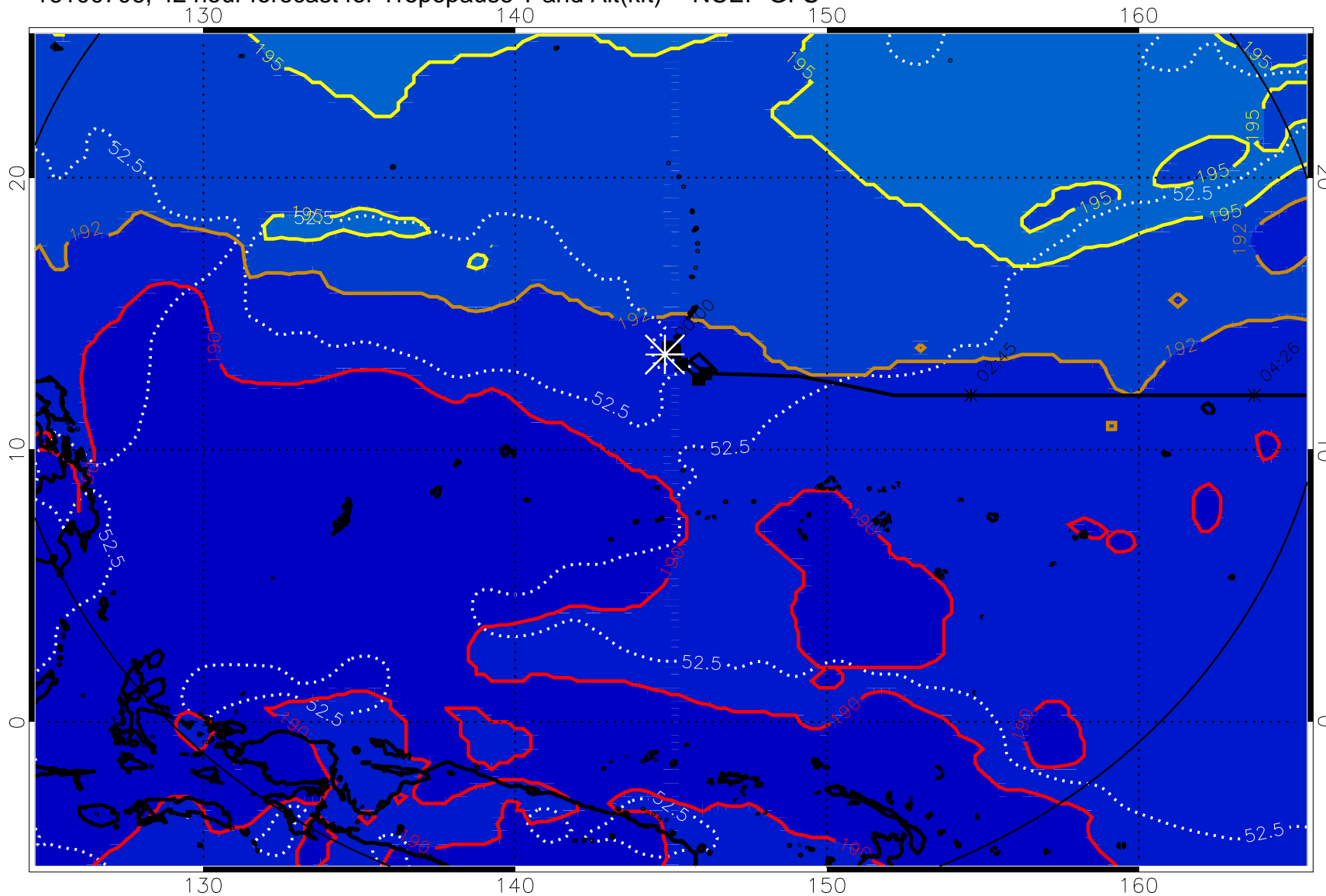
16100706, 42 hour forecast for Tropopause T and Alt(kft) -- NCEP GFS
